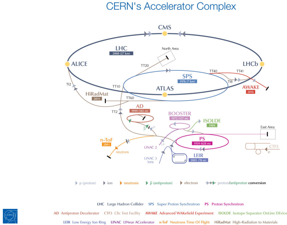
Figure 14: CERN accelerator complex [44].
