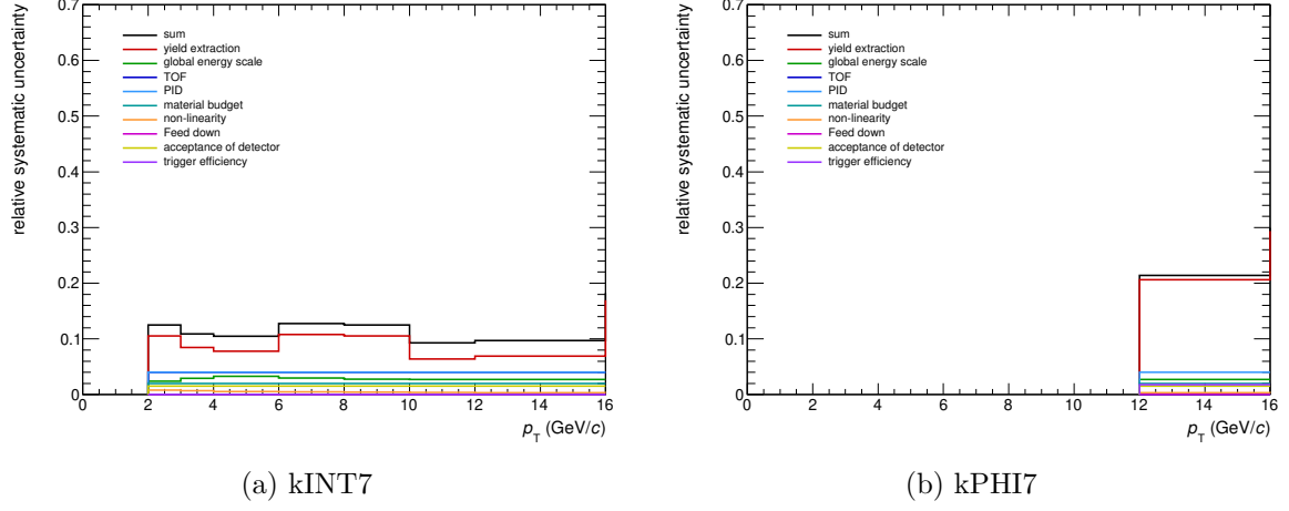
Figure 91: The summary of systematic uncertainties of the \eta measurement in Pb–Pb collisions at \sqrt{s_{NN}} = 5.02 TeV (40-60 %)
