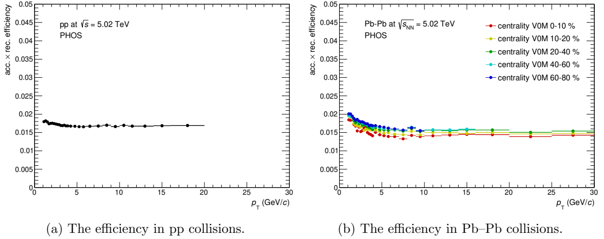
Figure 105: Acceptance \times reconstruction efficiencies in pp and Pb–Pb collisions at \sqrt{s_{NN}} = 5.02 TeV
