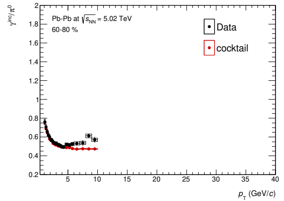
(f) The \gamma^{\text{inc}}/\pi^0 ratio in 60-80% Pb-Pb collisions.
