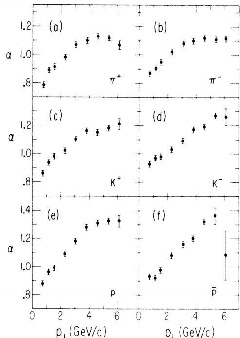
Figure 7: Power parameter \alpha vs. p_T [15].
