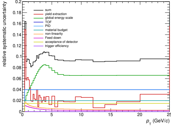
(a) kINT7
