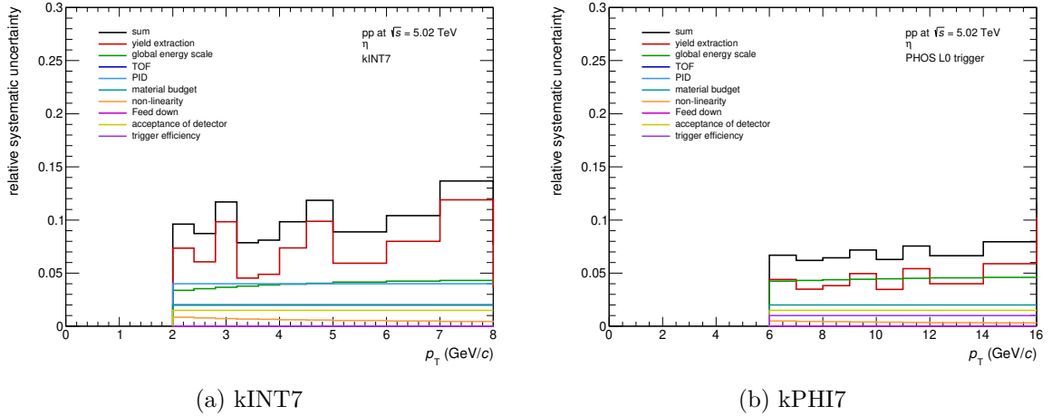
Figure 81: The summary of systematic uncertainties of the \eta measurement in pp collisions at \sqrt{s} = 5.02 TeV
