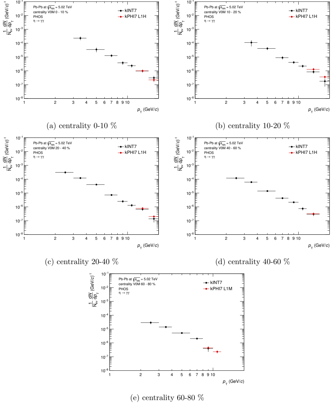
Figure 60: Raw yields of \eta in Pb-Pb collisions at \sqrt{s_{NN}} = 5.02 TeV
