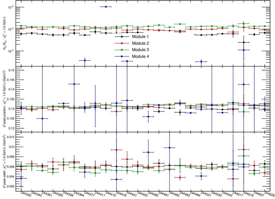
Figure 146: \pi^0 yield, peak position and sigma in each run in LHC15n.
