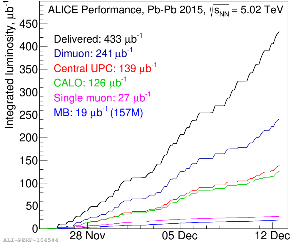
Figure 34: The integrated luminosity in Pb–Pb collisions at \sqrt{s_{NN}} = 5.02 TeV taken in 2015.
