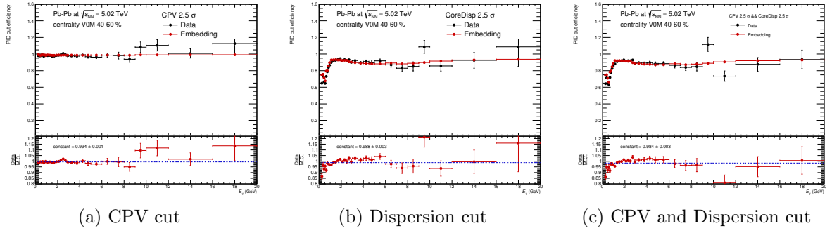
Figure 77: PID cut efficiency as a function of photon energy in Pb-Pb collisions at \sqrt{s_{NN}} = 5.02 TeV centrality 40-60%.
