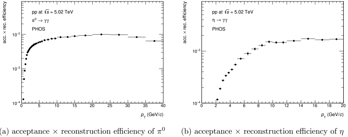
Figure 51: acceptance \times reconstruction efficiency of neutral mesons in pp collisions at \sqrt{s} = 5.02 TeV with PHOS
