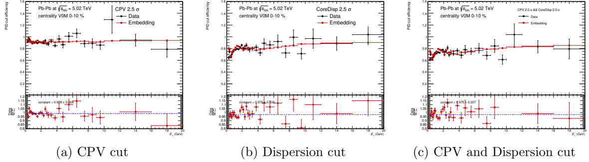
Figure 74: PID cut efficiency as a function of photon energy in Pb-Pb collisions at \sqrt{s_{NN}} = 5.02 TeV centrality 0-10%.
