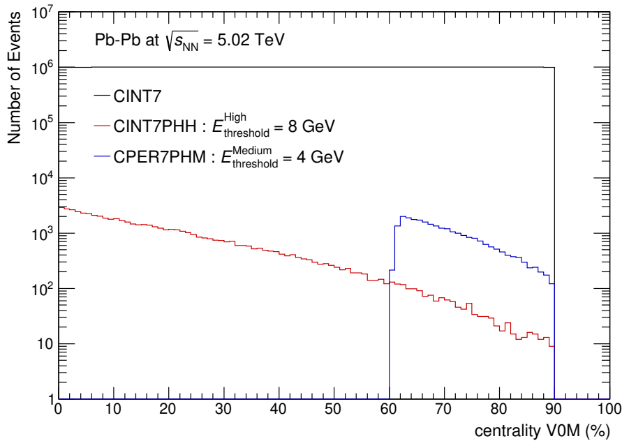
Figure 56: Centrality V0M distributions in Pb–Pb collisions at \sqrt{s_{NN}} = 5.02 TeV (2015)
