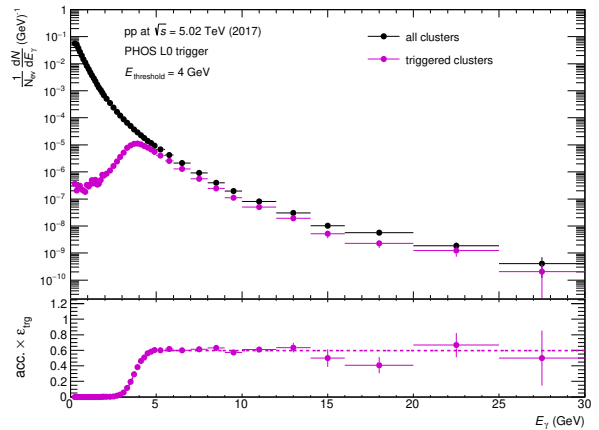
Figure 53: PHOS L0 trigger efficiency in pp collisions at \sqrt{s} = 5.02 TeV
