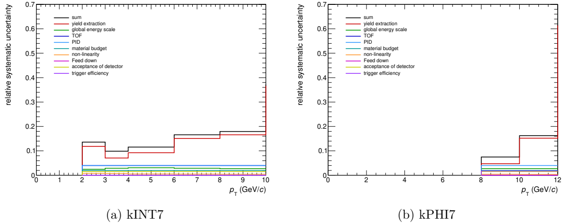
Figure 92: The summary of systematic uncertainties of the \eta measurement in Pb–Pb collisions at \sqrt{s_{NN}} = 5.02 TeV (60-80 %)
