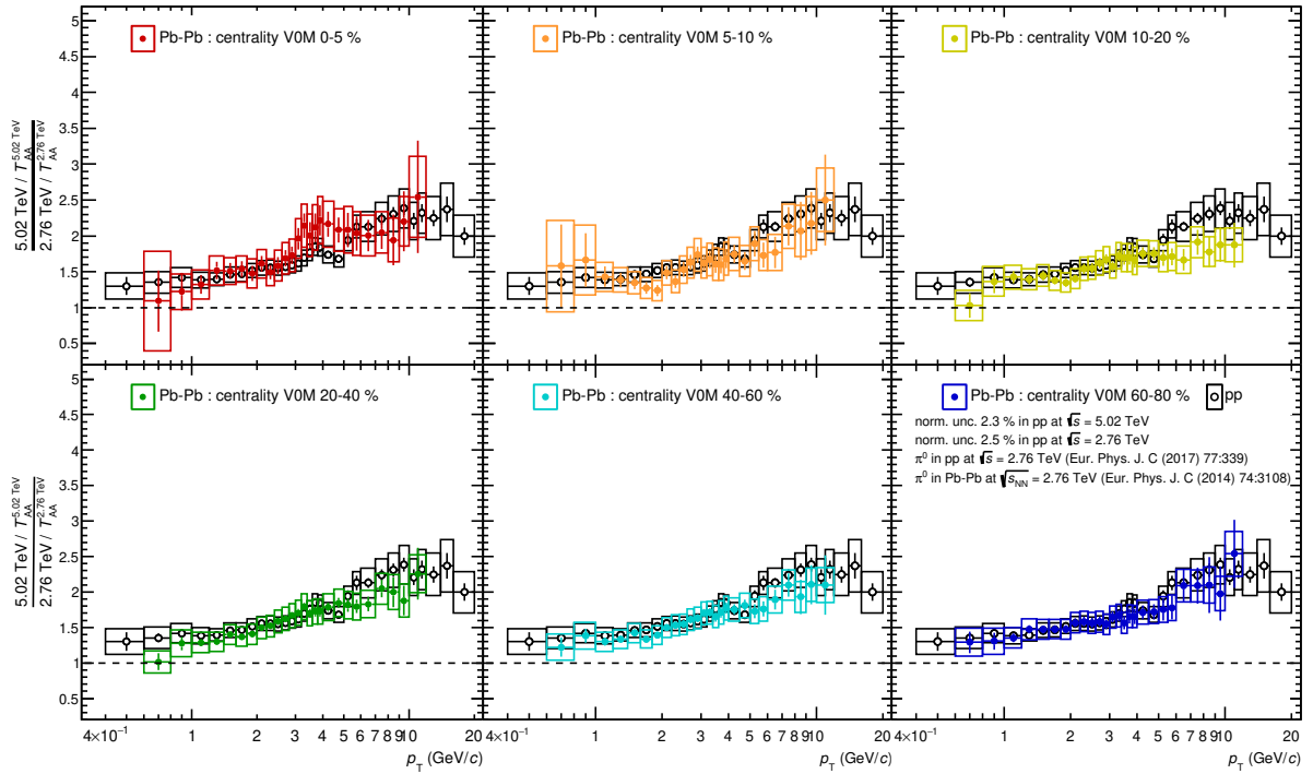
Figure 95: Comparison of p_T spectra for \pi^0 between \sqrt{s_{NN}} = 5.02 and 2.76 TeV in Pb–Pb collisions
