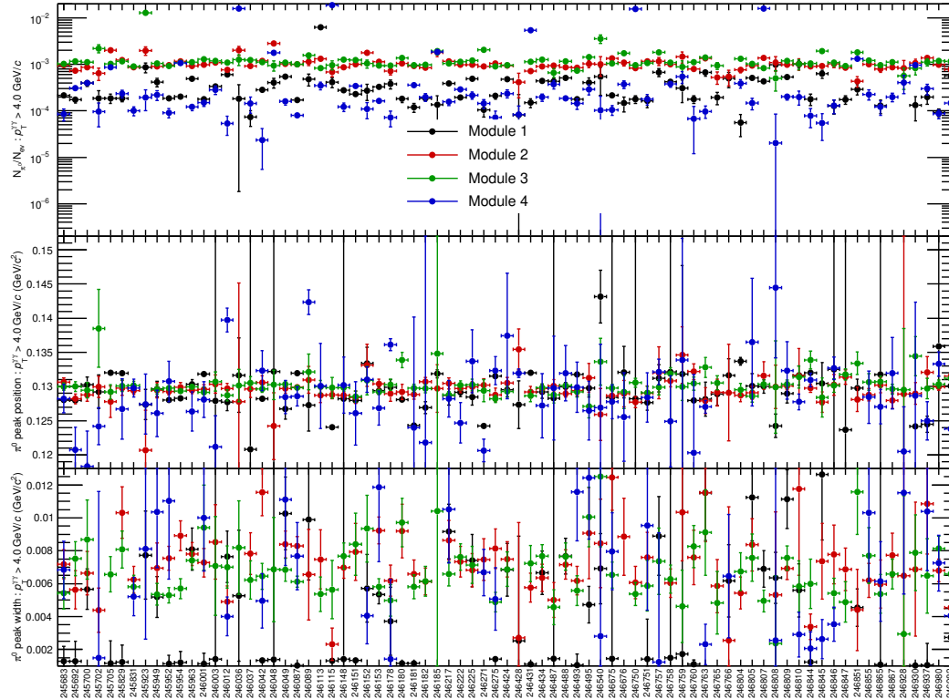
Figure 38: \pi^0 yield, peak position and sigma in each run in LHC15o pass1.
