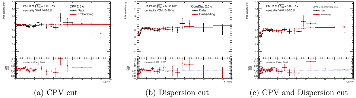
Figure 75: PID cut efficiency as a function of photon energy in Pb-Pb collisions at \sqrt{s_{NN}} = 5.02 TeV centrality 10-20%.
