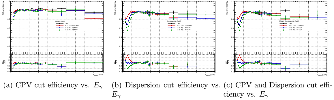
Figure 143: \gamma -ID cut efficiency as a function of photon energy. (12.5 MeV is default value in M.C.)
