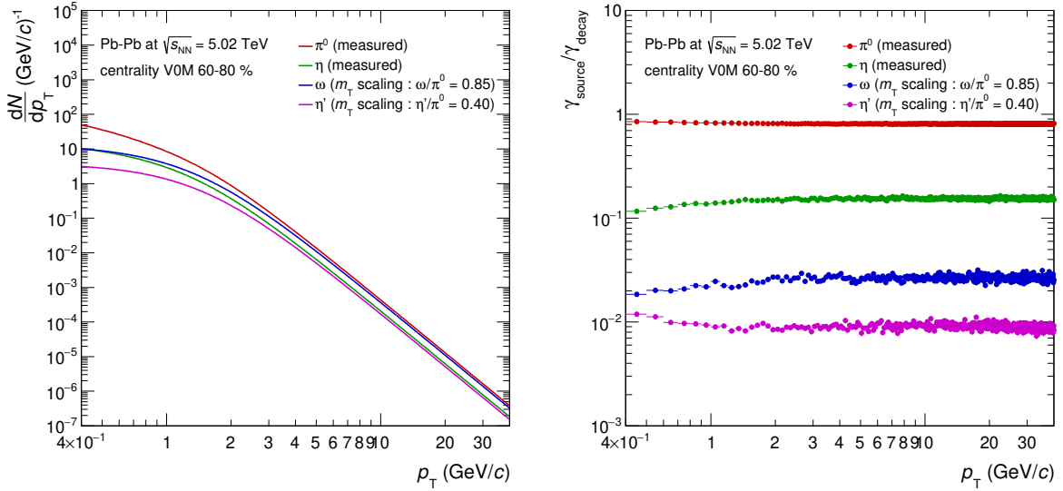
(a) The input p_T spectra from different mesons. (b) The fraction of each decay photon source.
