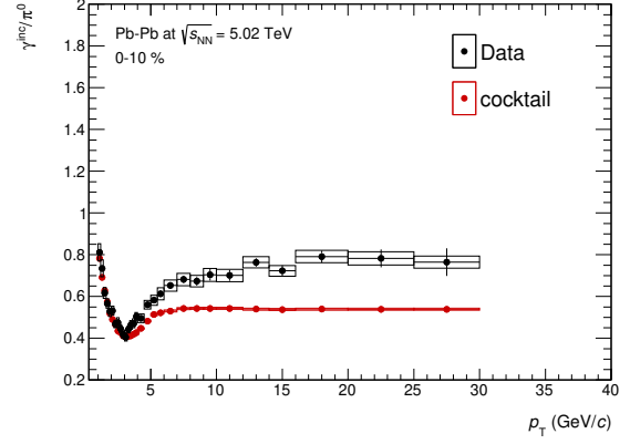
(b) The \gamma^{\text{inc}}/\pi^0 ratio in 0-10% Pb-Pb collisions.
