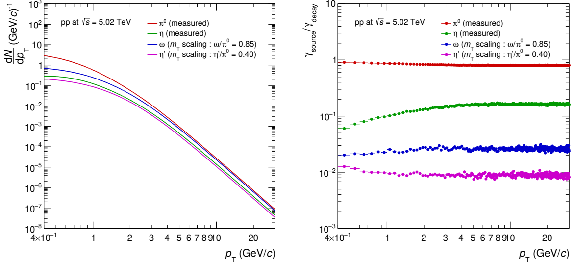
(a) The input p_T spectra from different mesons.
