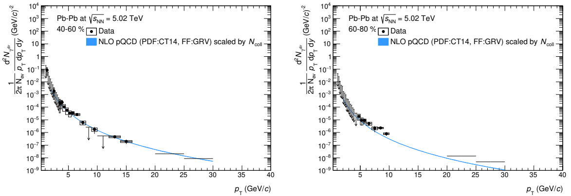
(e) The invariant yield of direct photons in 40-60% Pb–Pb collisions. (f) The invariant yield of direct photons in 60-80% Pb–Pb collisions.
