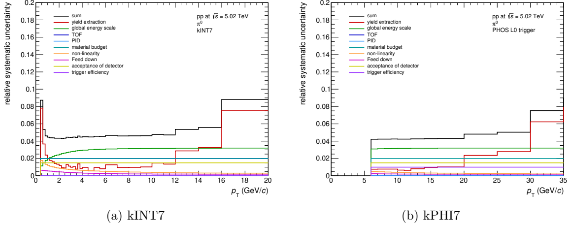
Figure 80: The summary of systematic uncertainties of the \pi^0 measurement in pp collisions at \sqrt{s} = 5.02 TeV
