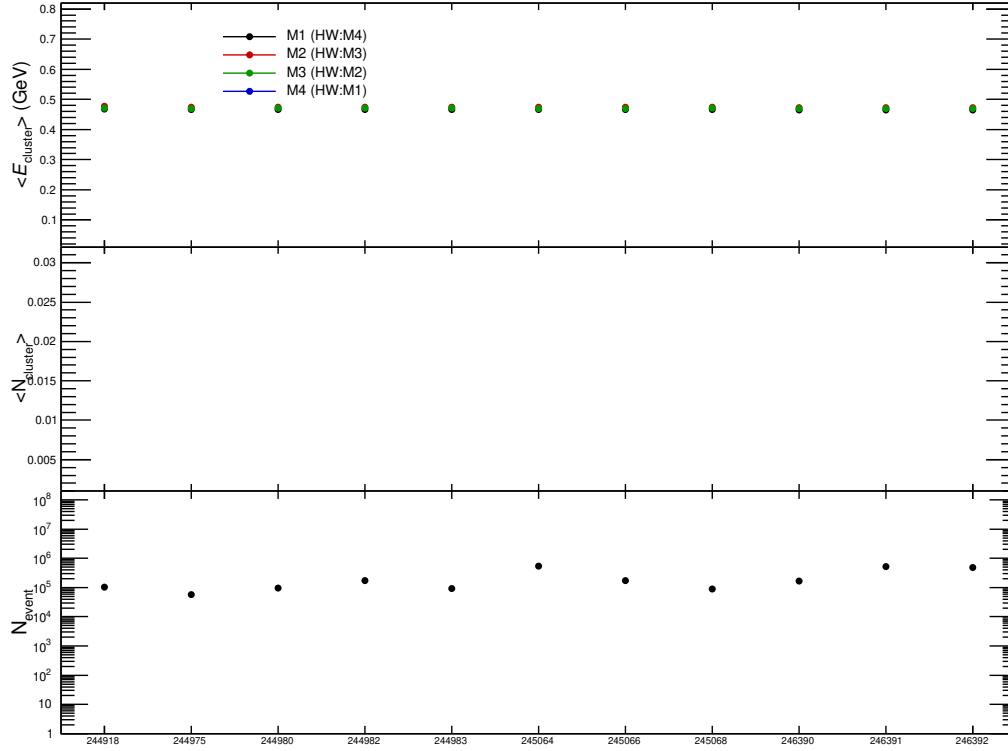
Figure 37: The average cluster energy and number of hits in each run on PHOS in LHC15o lowIR pass5.
