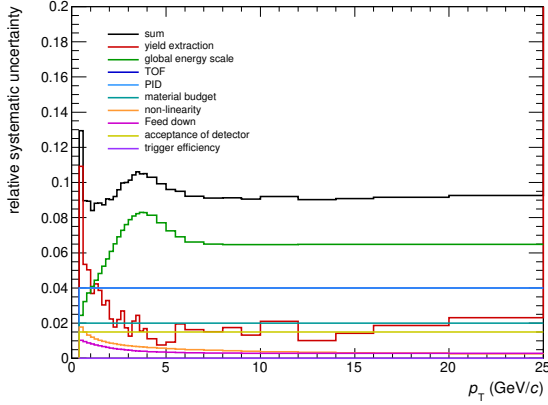
(a) kINT7
