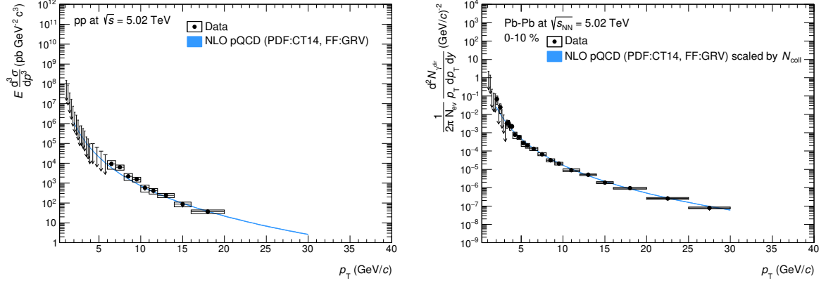
(a) The production cross section of direct photons in pp collisions. (b) The invariant yield of direct photons in 0-10% Pb–Pb collisions.
