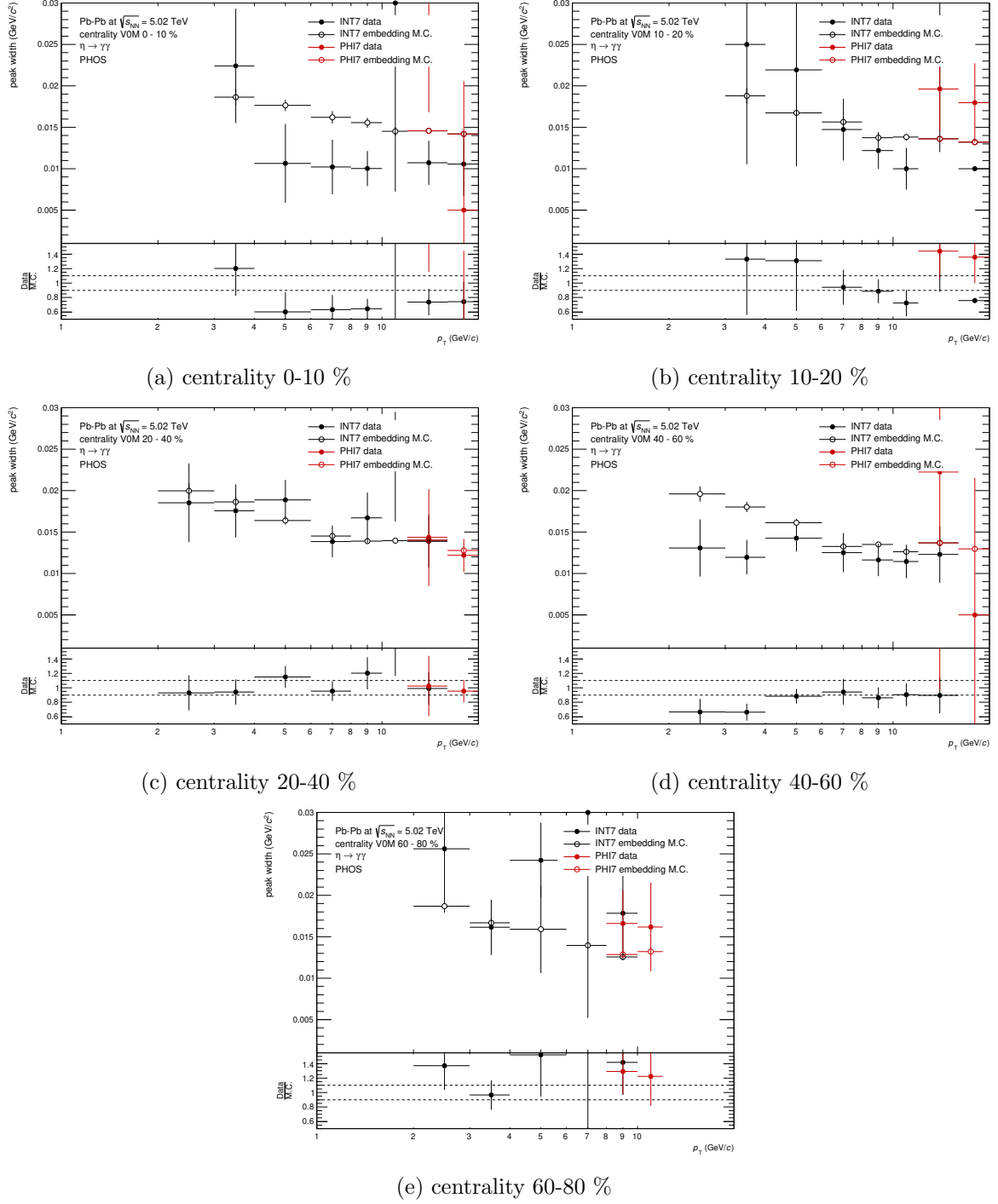
Figure 65: \eta peak width in Pb-Pb collisions at \sqrt{s_{NN}} = 5.02 TeV for different centrality classes
