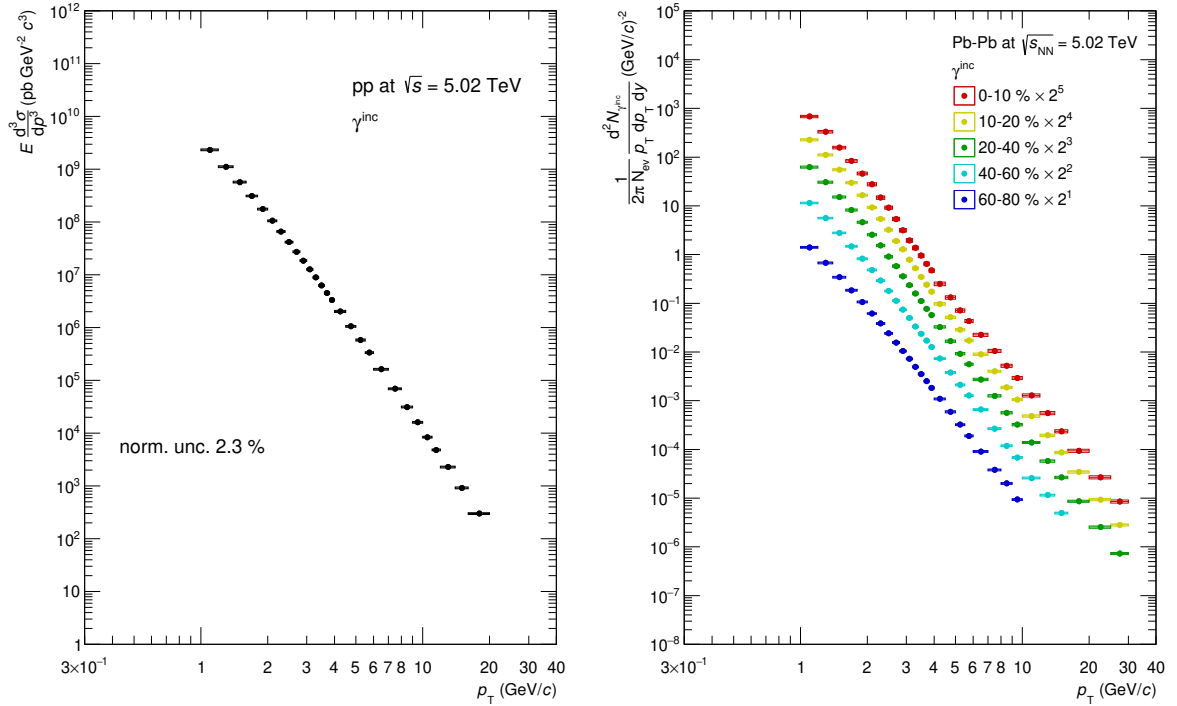
(a) The production cross section of inclusive photons in pp collisions at \sqrt{s} = 5.02 TeV. (b) Invariant yields of inclusive photons in Pb–Pb collisions at \sqrt{s_{\text{NN}}} = 5.02 TeV.
