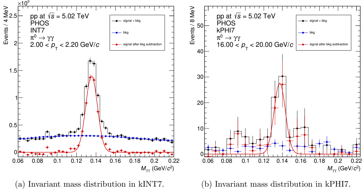
Figure 149: \pi^0 peak in kINT7 and kPHI7. An energy threshold of PHOS L0 trigger was 3 GeV in 2015
