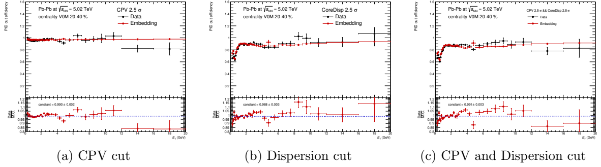
Figure 76: PID cut efficiency as a function of photon energy in Pb-Pb collisions at \sqrt{s_{NN}} = 5.02 TeV centrality 20-40%.
