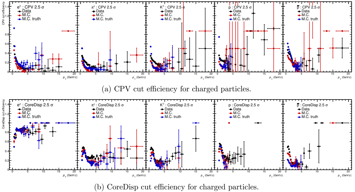
Figure 109: PID cut efficiencies for identified charged particles in pp collisions at \sqrt{s} = 5.02 TeV. From left to right, e^\pm , \pi^\pm , K^\pm , p and \bar{p} . Black for data, red for M.C. DDA, blue for M.C. truth.
