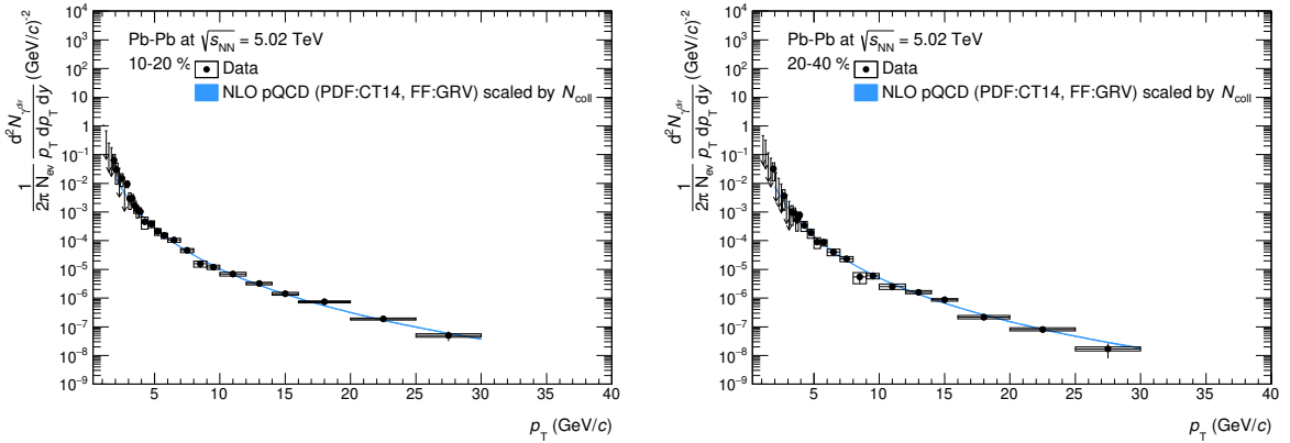
(c) The invariant yield of direct photons in 10-20% Pb–Pb collisions. (d) The invariant yield of direct photons in 20-40% Pb–Pb collisions.
