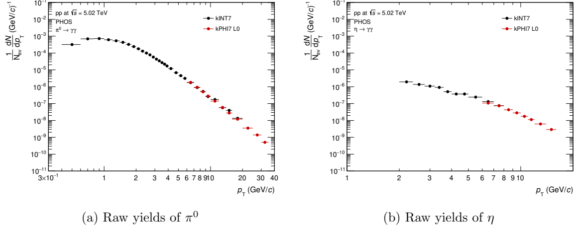
Figure 48: Raw yields of neutral mesons in pp collisions at \sqrt{s} = 5.02 TeV
