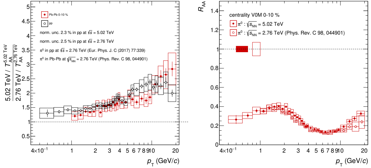
(a) The ratio of p_{\text{T}} spectrum for \pi^0 .
