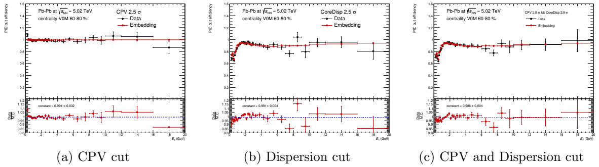
Figure 78: PID cut efficiency as a function of photon energy in Pb-Pb collisions at \sqrt{s_{NN}} = 5.02 TeV centrality 60-80%.
