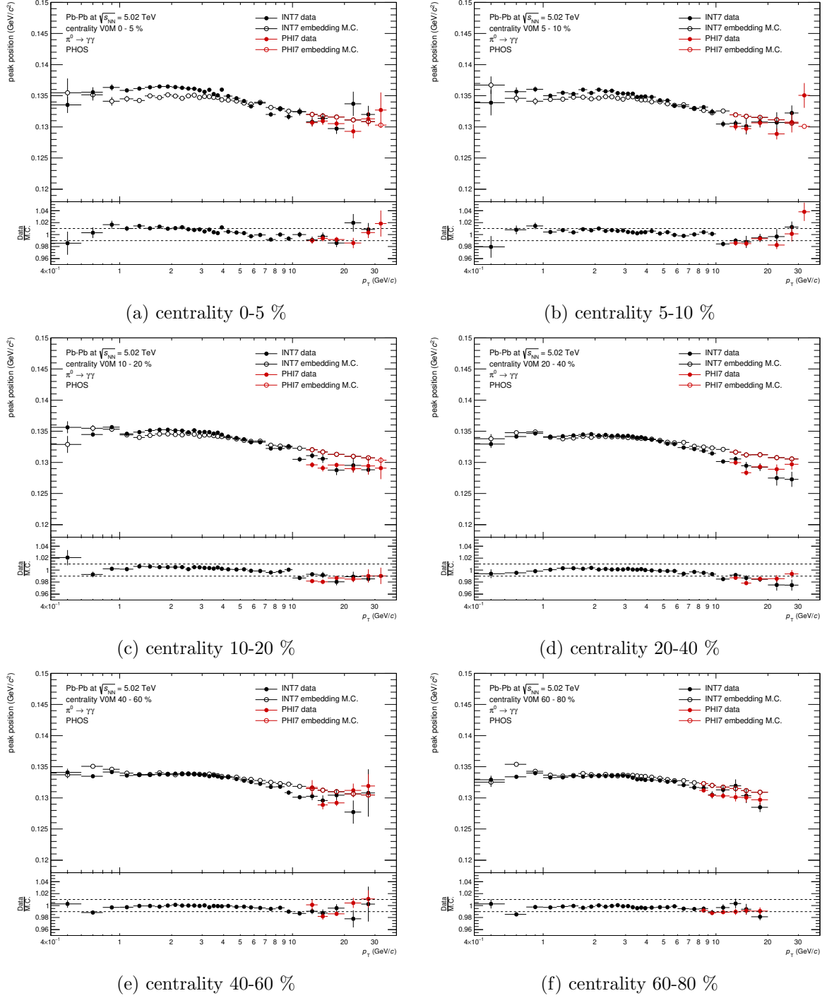
Figure 62: \pi^0 peak position in Pb-Pb collisions at \sqrt{s_{NN}} = 5.02 TeV for different centrality classes
