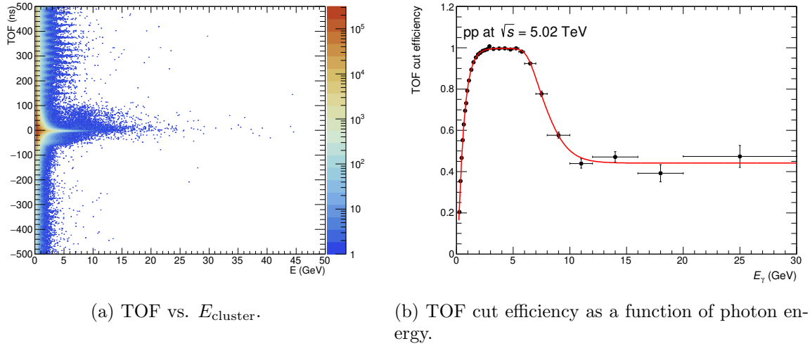
Figure 52: The cluster timing distribution and TOF cut efficiency
