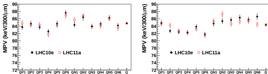
Figure 3.5: Two examples of the MPVs of single chips. Measurements for 2 different data taking periods are plotted. The first 6 bins on the X-axis show gains for the P-sides chips and the next 6 for the N-side chips. The last bin shows the MPV for entire module.
