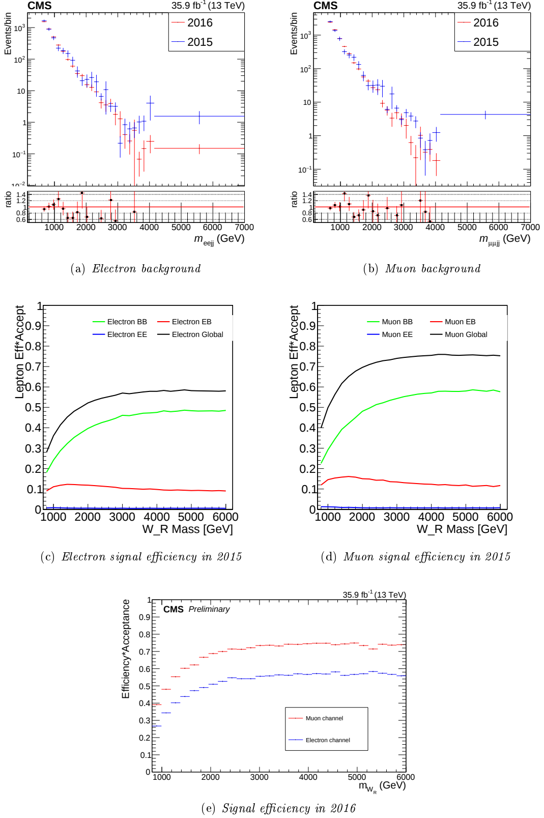
Figure 4.46: Comparison of expected backgrounds and signal efficiencies for 2015 and 2016.
