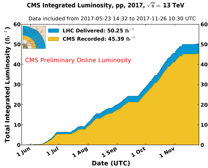
Figure 2.6: Online integrated luminosity (values published by CMS at the time of data taking, not including any later improvements in the calibration) delivered by the LHC (in blue) and recorded by CMS (in yellow) in 2017 proton-proton collisions.
