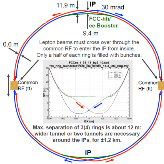
Figure 5.17: Layout of the FCC collider.
