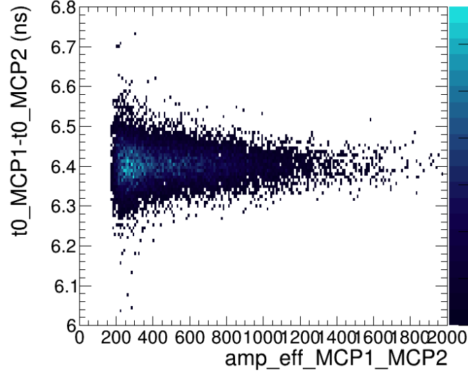
Figure 3.27: Time difference distribution between the two MCPs as a function of their effective amplitude.
