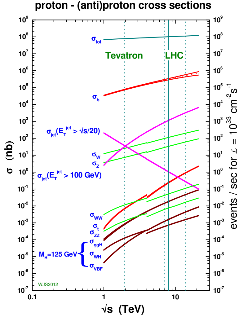
Figure 2.2: Expected production cross section for signal and background processes at hadron colliders as a function of the center-of-mass energy [96].
