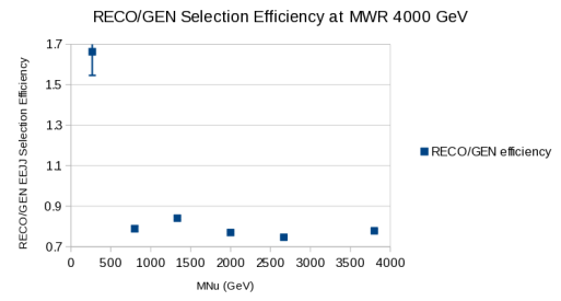
(b) Electron channel, m_{W_R} = 4 TeV
