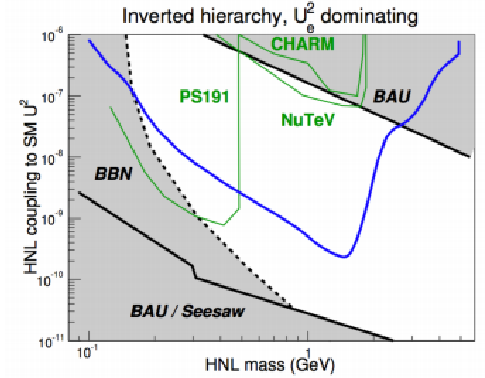
Figure 5.9: Experimental and cosmological bounds on the search for heavy neutral leptons. The exclusion limit at 90% CL SHiP could set in the case of no signal, assuming a model [185] with inverted hierarchy and a dominant electron coupling, U_e^2 : U_\mu^2 : U_\tau^2 = 48 : 1 : 1 , is represented by the blue line.
