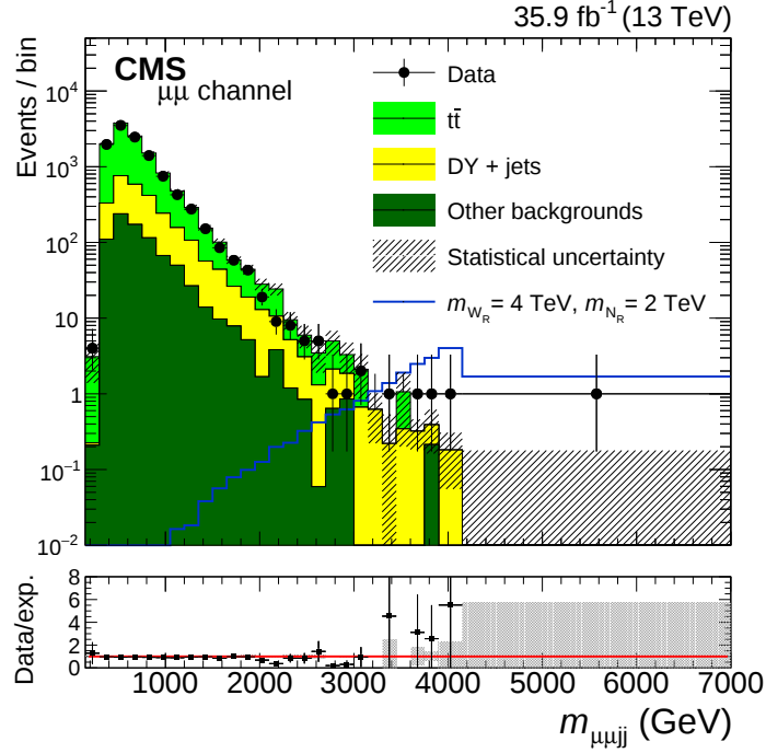
(b) Muon channel
