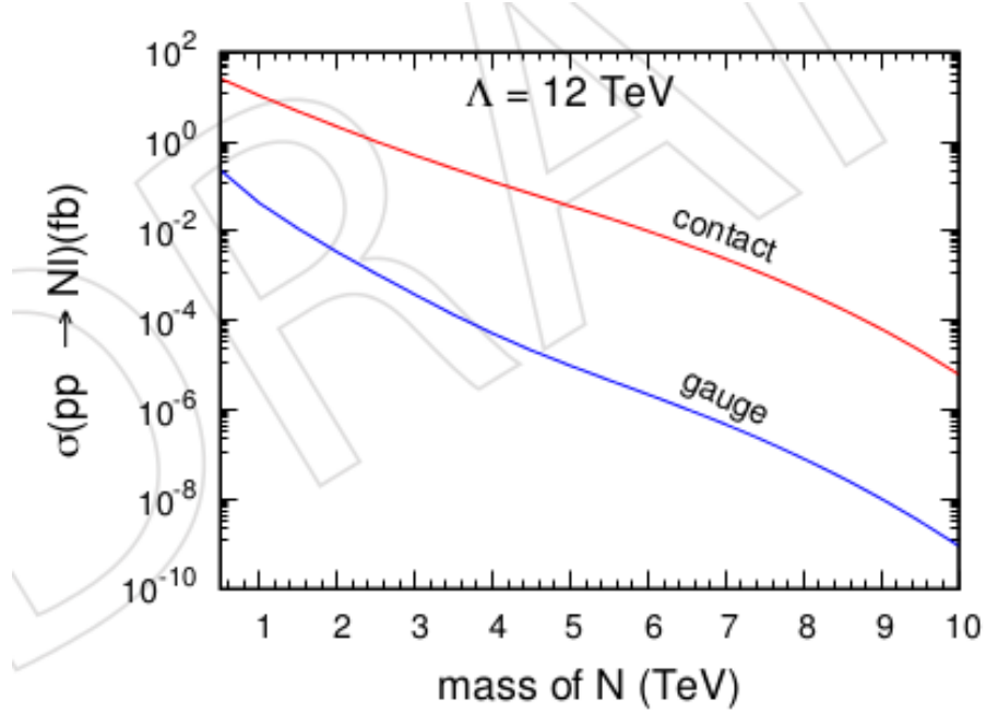
Figure 5.14: Production cross section of the heavy composite Majorana neutrino for gauge and contact interaction at \Lambda = 12 TeV for pp collisions at \sqrt{s} = 14 TeV. [193]
