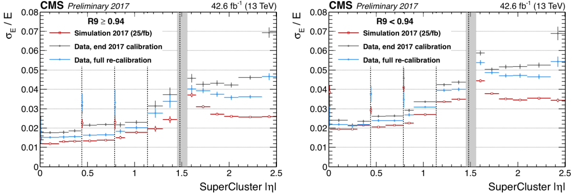
Figure 2.27: Relative electron energy resolution in bins of pseudorapidity for the barrel and the endcaps, using electrons from Z \rightarrow e^+e^- decays. The resolution is shown for very low bremsstrahlung electrons (named “golden”, with R_9 > 0.94 ) on the left, and for high bremsstrahlung electrons ( R_9 < 0.94 ) on the right, plotted separately for data and MC events. The relative resolution \sigma_E/E is extracted from an unbinned likelihood fit to Z \rightarrow e^+e^- events, using a Voigtian (a Landau convoluted with a Gaussian) as the signal model. The ECAL conditions used in the simulation (red points) reflect the status of the detector as predicted after 25\text{fb}^{-1} of data-taking in 2017. The resolution is affected by the amount of material in front of the ECAL and is degraded in the vicinity of the ECAL modules boundaries, indicated by the vertical dashed lines in the plot. Also, the resolution improves significantly after a dedicated calibration using the full 2017 dataset (blue points) with respect to the end-of-year (EOY) 2017 calibration (gray points) for which only time dependent effects were corrected for. The grey band at |\eta| \approx 1.5 marks the barrel-endcap transition region excluded from the photon fiducial region used in the H \rightarrow \gamma\gamma analysis.
