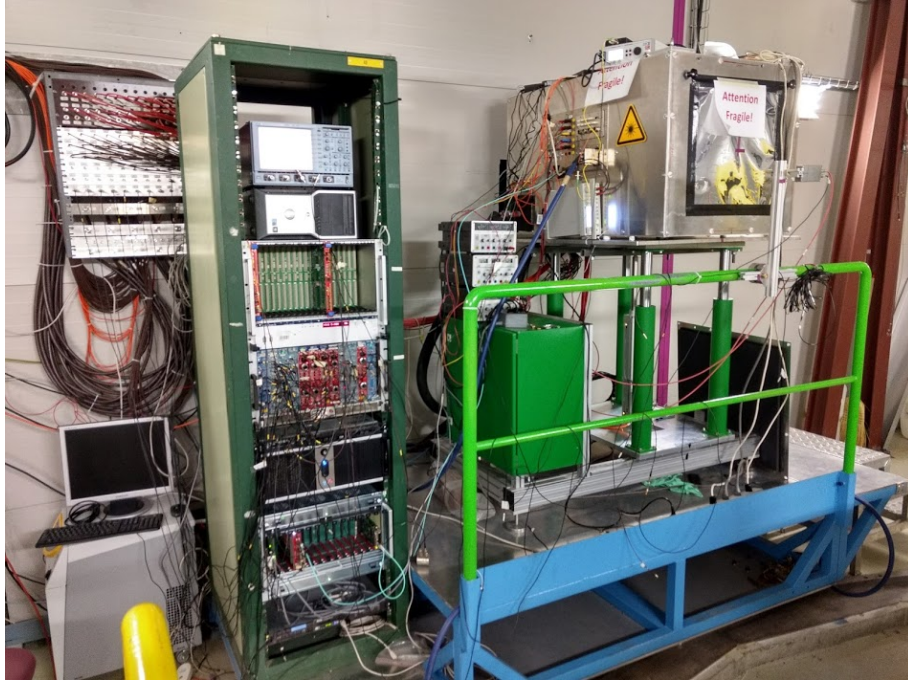
Figure 3.13: Picture of the test beam setup: the digitizer is on the left, while on the right there is the box in which the crystal matrix, the VFE and FE boards are installed.
