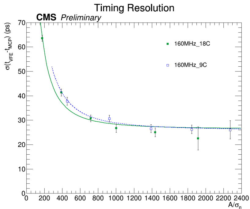
Figure 3.32: Time resolution given by the difference between a crystal and the second MCP as a function of the normalized amplitude for 160MHz and 18°/9° C.
