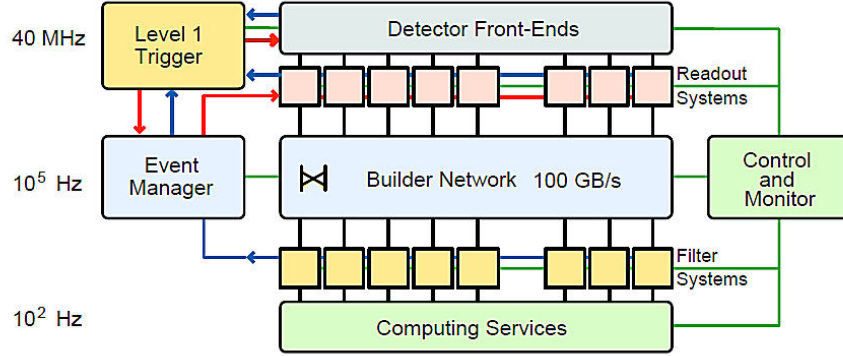
Figure 2.35: Scheme of the DAQ system.
