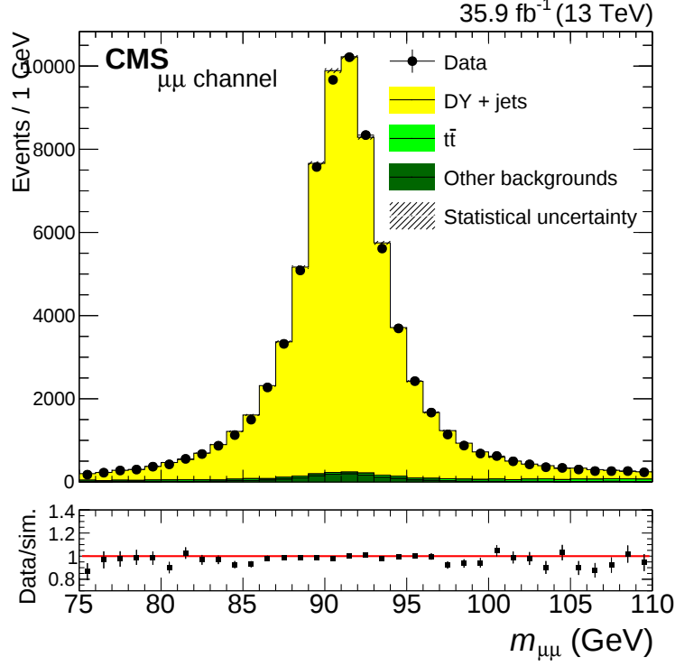
Figure 4.15: Z \rightarrow \mu^+\mu^- Z \rightarrow \mu\mu events in the low- m_{\ell\ell} CR after application of trigger, ID, isolation, and DY normalization SFs and momentum corrections. The uncertainty bands on the simulated background histograms only include statistical uncertainties. The uncertainty bars in the ratio plots represent the combined statistical uncertainties of data and simulation.
