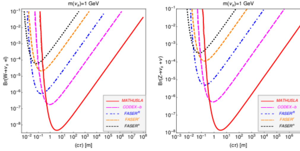
Figure 5.11: Sensitivity estimates in the branching ratio versus decay length plane for FASER, MATHUSLA, and CODEX-b for neutrinos from W (Z) boson production on the left (right).
