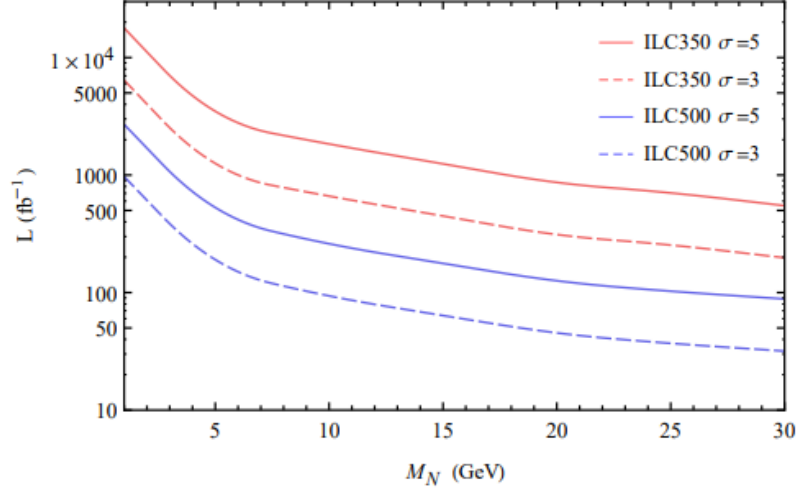
Figure 5.26: Integrated luminosity necessary for observing the Majorana neutrino at the 3\sigma (dashed line) and 5\sigma (solid line) levels at ILC with \sqrt{s} = 350 GeV (red) and \sqrt{s} = 500 GeV (blue) [200].
