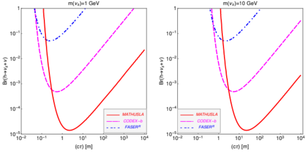
Figure 5.12: Sensitivity estimates in the branching ratio versus decay length plane for FASER, MATHUSLA, and CODEX-b for neutrinos from H boson production: for m_N = 1 GeV on the left and for m_N = 10 GeV on the right.
