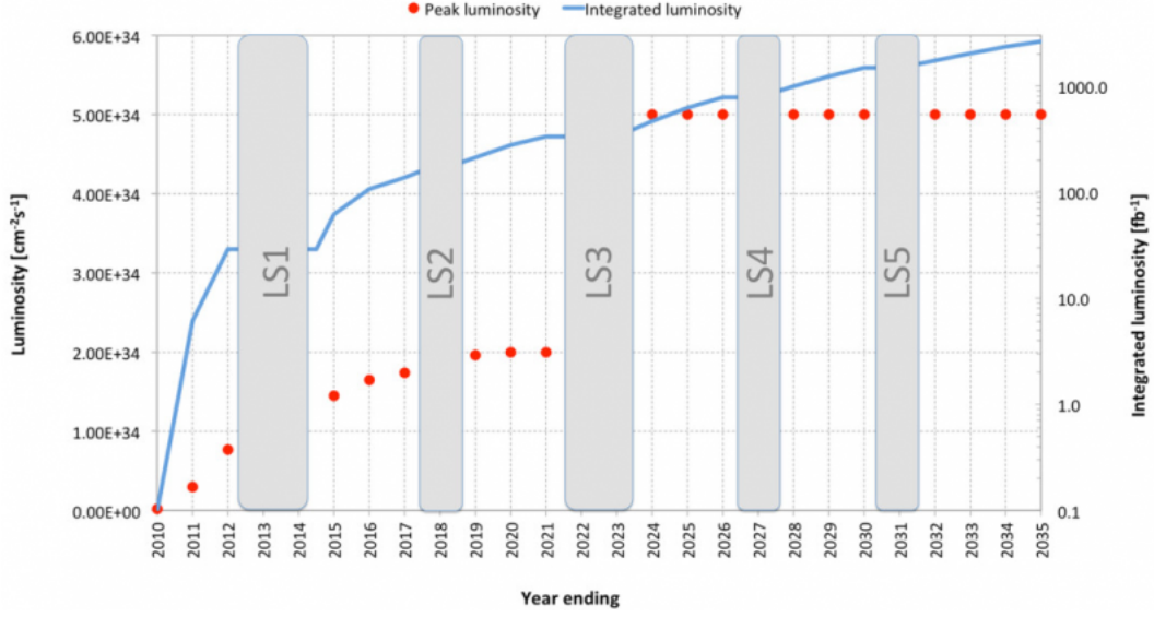
Figure 3.1: Timeline and luminosity reached by LHC and HL-LHC.
