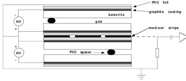
Figure 2.32: Section of a double gap resistive plate chamber.
