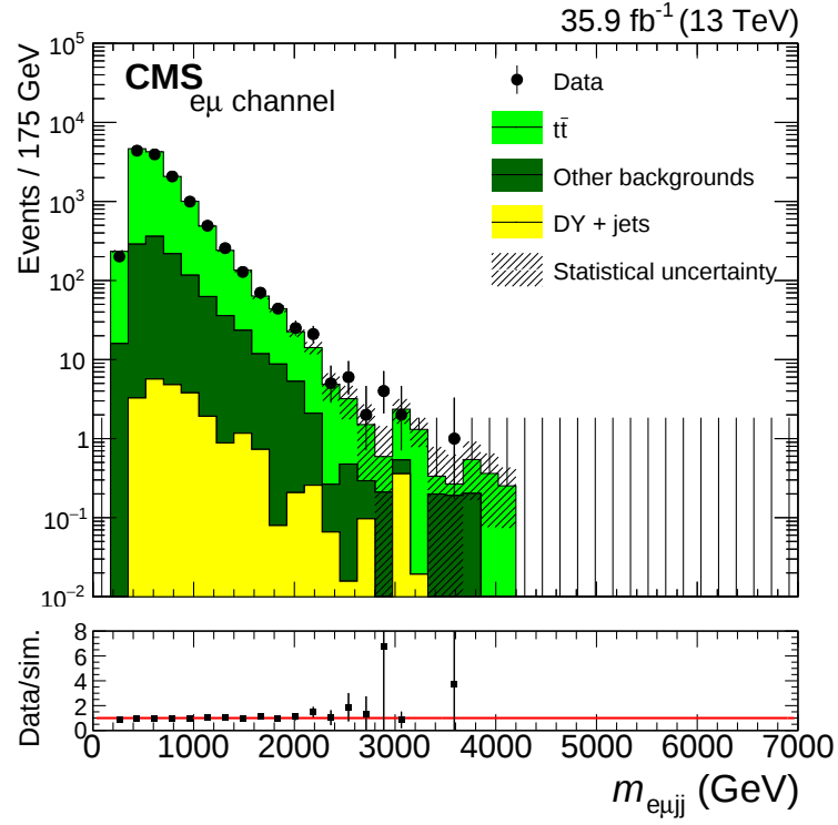
Figure 4.19: The m_{\ell\ell jj} distribution for data and simulated events in the flavour-sideband CR with all SFs applied. The uncertainty bands on the simulated background histograms only include statistical uncertainties. The uncertainty bars in the ratio plots represent the combined statistical uncertainties of data and simulation.
