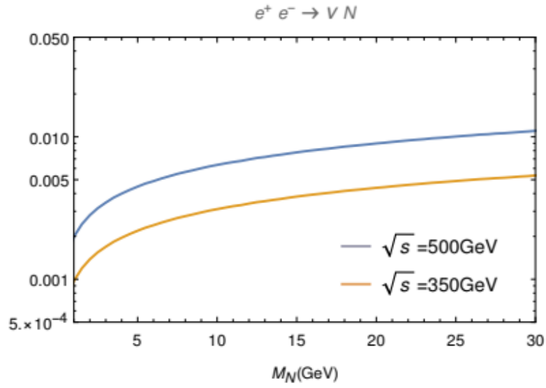
Figure 5.25: Cross sections of e^+e^- \rightarrow \nu N as a function of m_N at ILC [200].
