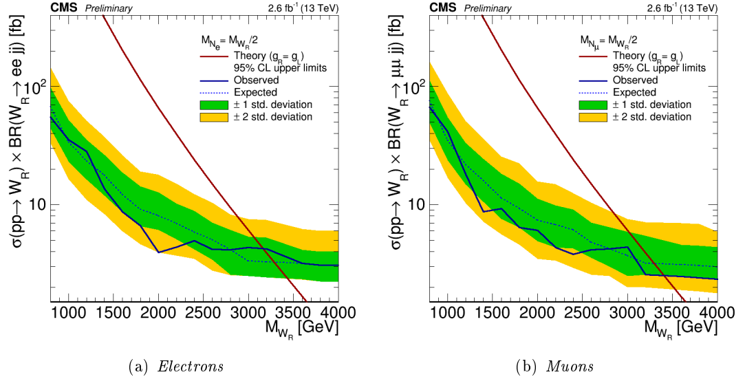
Figure 1.8: The 95% CL exclusion limit for W_R boson production cross section times branching fraction, computed as a function of m_{W_R} assuming m_{N_R} = \frac{1}{2}m_{W_R} , for the 2015 analysis.
