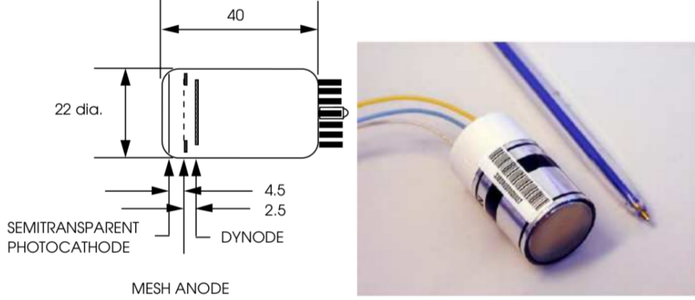
Figure 2.20: Left: VPT layout. Right: Photo of a VPT detector.
