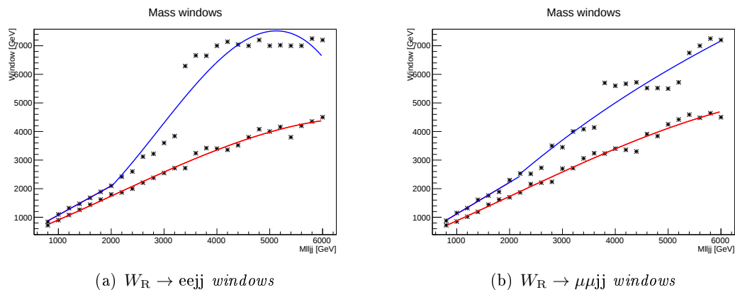
Figure C.1: Mass window edges optimized for Punzi signal significance. Windows are smoothed out by fitting a third degree polynomial.
