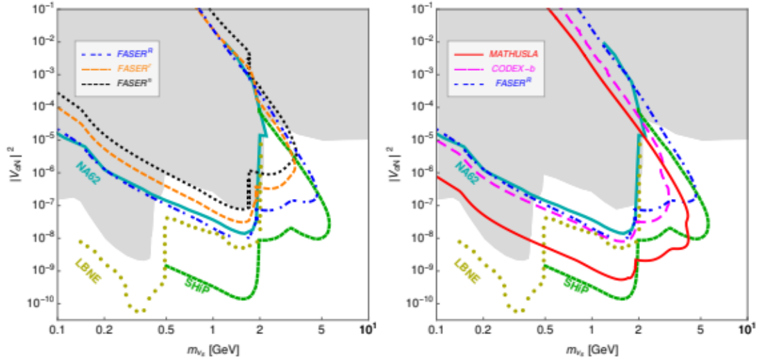
Figure 5.13: Sensitivity estimates in the mixing angle |V_{\alpha N}|^2 versus neutrino mass m_N for the different variants of FASER on the left, and for FASER, MATHUSLA, CODEX-b, SHiP, NA62 and LBNE on the right.
