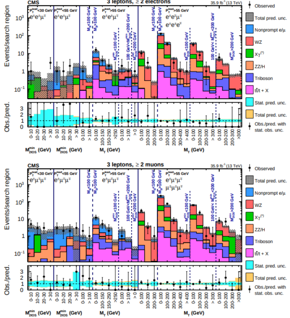
Figure 5.1: Observed and expected event yields as a function of M_{2\ell OS}^{min} and M_T for events with at least two electrons (top), and with at least two muons (bottom) in the trilepton channel. The contribution of each background source is shown. The first 8 bins of each figure correspond to the low-mass region, while the rest displays the high-mass region. [170]
