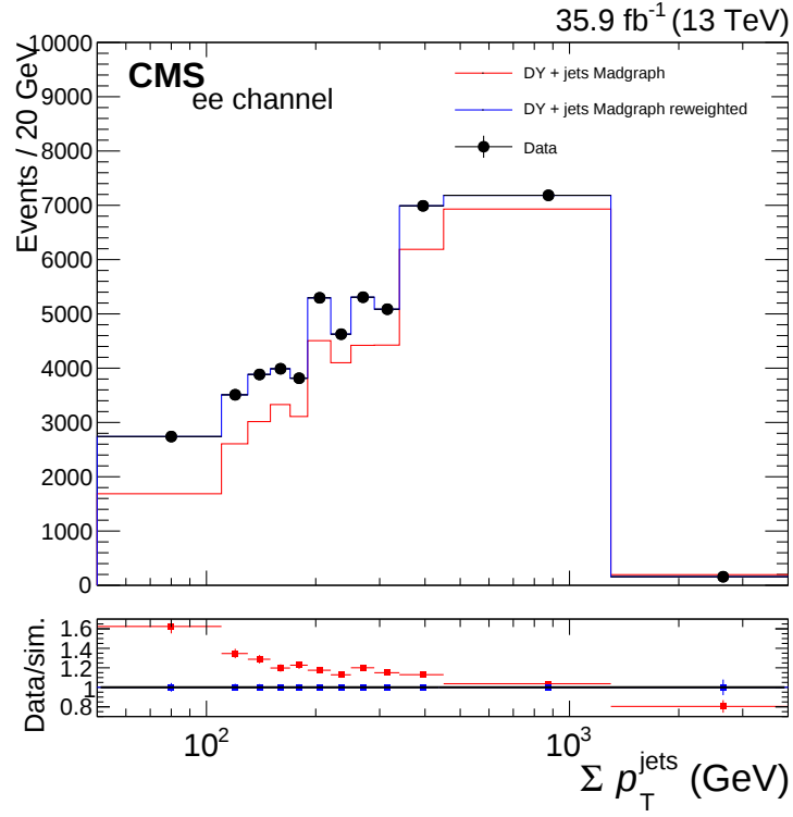
(a) Electron channel
