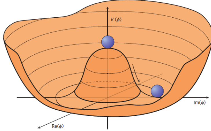
Figure 1.2: “Mexican hat” shape of the Higgs potential.
