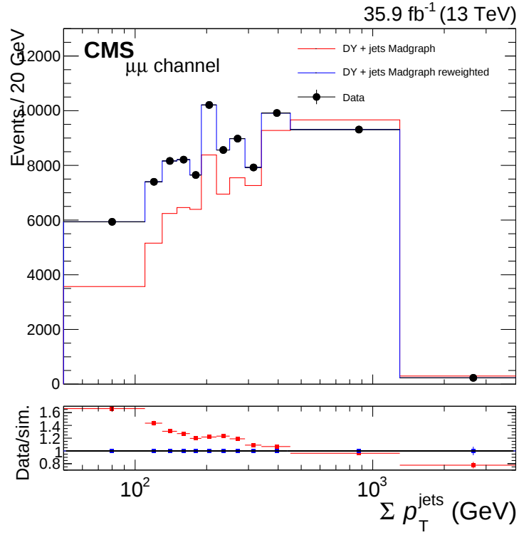
(b) Muon channel
