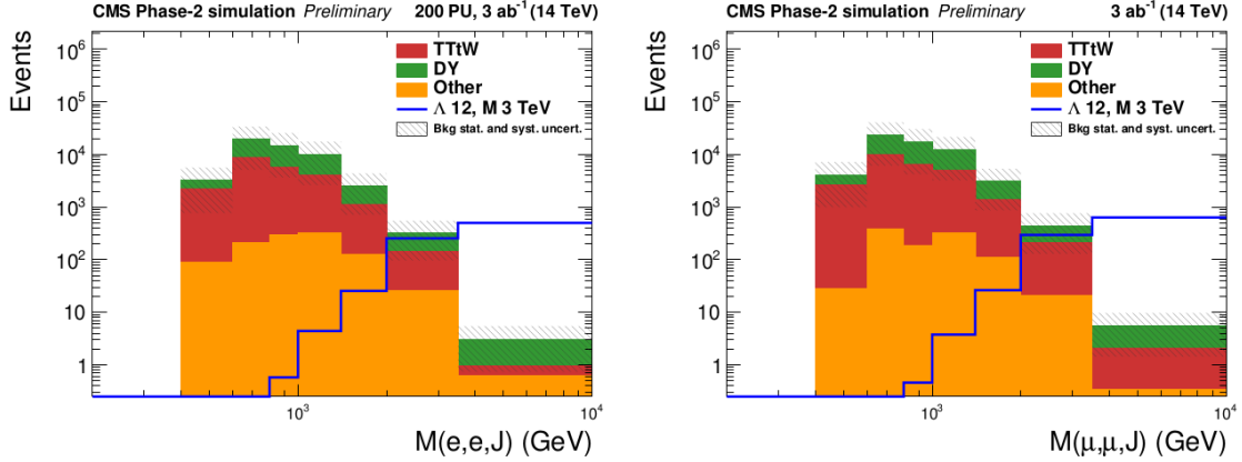
Figure 5.15: Distribution of the variable M(\ell\ell J) for backgrounds (stacked plots) and expected signal (blue line) in the signal region, considering the model parameters \Lambda = 12 TeV and M_N = 3 TeV, for the eeqq channel (left) and for the \mu\mu qq channel (right). The background uncertainties are the combined statistical and systematic uncertainties. [193]
