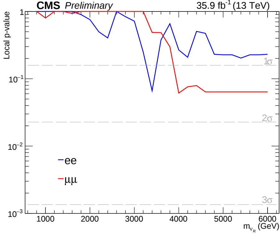
Figure 4.49: Local p-value as a function of m_{N_R} for the electron (blue) and the muon (red) channels.
