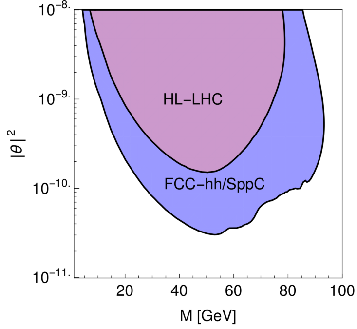
Figure 5.22: Projections on the mixing angle between one HNL and a lepton as a function of the HNL mass for FCC-hh and HL-LHC [197].
