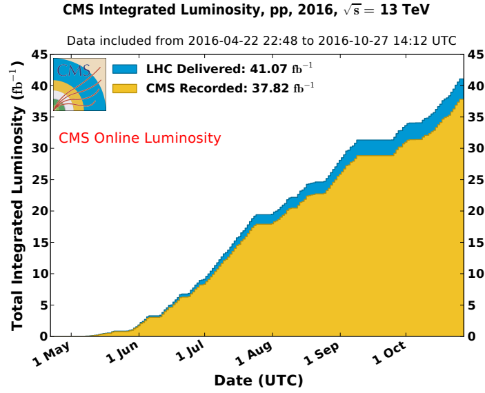
Figure 2.5: Online integrated luminosity (values published by CMS at the time of data taking, not including any later improvements in the calibration) delivered by the LHC (in blue) and recorded by CMS (in yellow) in 2016 proton-proton collisions.
