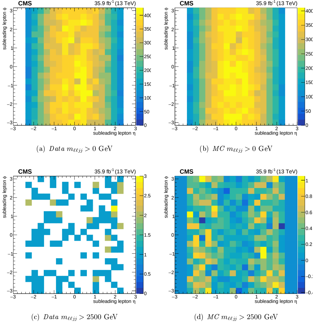
Figure 4.37: 2D distributions of subleading muon \eta vs \phi in events with m_{\ell\ell jj} > 2.5 TeV (bottom) and for all m_{\ell\ell jj} (top) in the low- m_{\ell\ell} CR.
