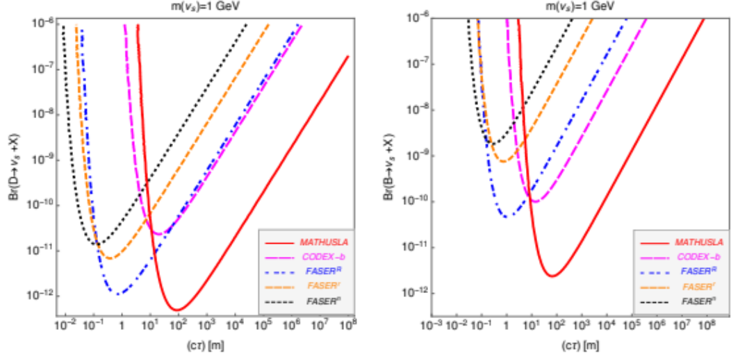
Figure 5.10: Sensitivity estimates in the branching ratio versus decay length plane for FASER, MATHUSLA, and CODEX-b for neutrinos from D-meson (B-mesons) decays on the left (right).
