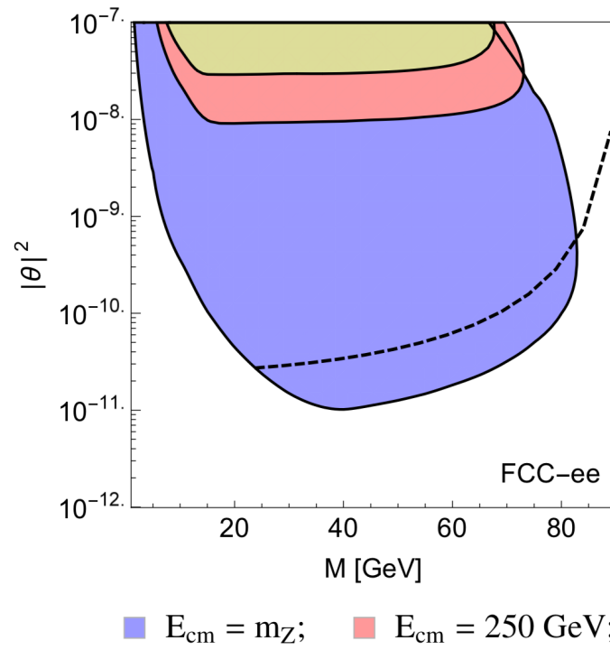
Figure 5.21: Projections on the mixing angle between one HNL and a lepton as a function of the HNL mass for FCC-ee [197].
