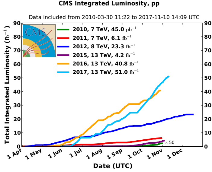
Figure 2.7: Cumulative integrated luminosity delivered by LHC to CMS during stable beams for proton-proton collisions in different years of data taking.
