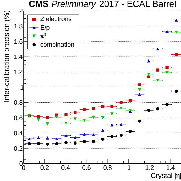
Figure 2.26: The precision for measuring the channel inter-calibration constants from Z \rightarrow e^+e^- , \pi \rightarrow \gamma\gamma decays, and electrons arising from W and Z boson decays compared to the tracker response ( E/p ), is shown as a function of |\eta| in the ECAL barrel detectors using the data collected in 2017. The precision of the Z \rightarrow e^+e^- inter-calibrations, in red, is at the level of the systematic errors. The precision of the E/p inter-calibrations, in blue, is still dominated by the statistical errors for |\eta| > 1 . The green points represent the precision of the intercalibration constants obtained using photons from \pi^0 \rightarrow \gamma\gamma decays. The black points represent the precision of the combination of the three methods (weighted average).
