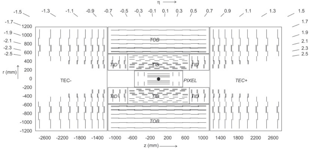
Figure 2.13: Overview of the CMS tracker, where each line represents a detector module.
