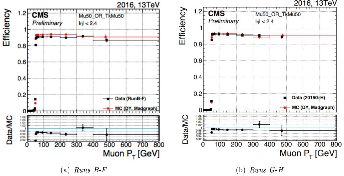
Figure 4.8: Efficiency of HLT\_Mu50 OR HLT\_TkMu50 triggers given offline muons passing high- p_T ID requirements as a function of muon p_T [86].
