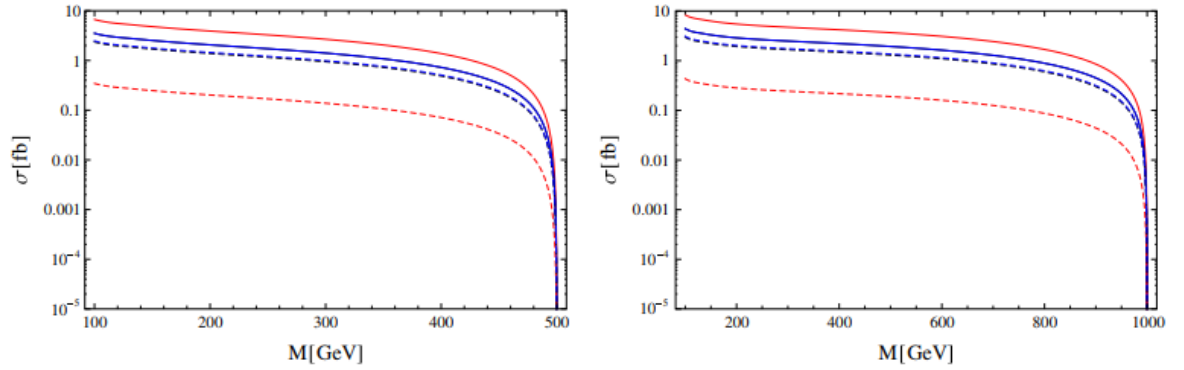
Figure 5.28: Production cross section of the e^+e^- \rightarrow n\bar{u}_l N_l process, followed by the decays N \rightarrow lW ( l = e, \mu, \tau ) and W \rightarrow q\bar{q}' , as a function of the heavy neutrino mass at \sqrt{s} = 500 GeV on the left and at 1 TeV on the right [200].
