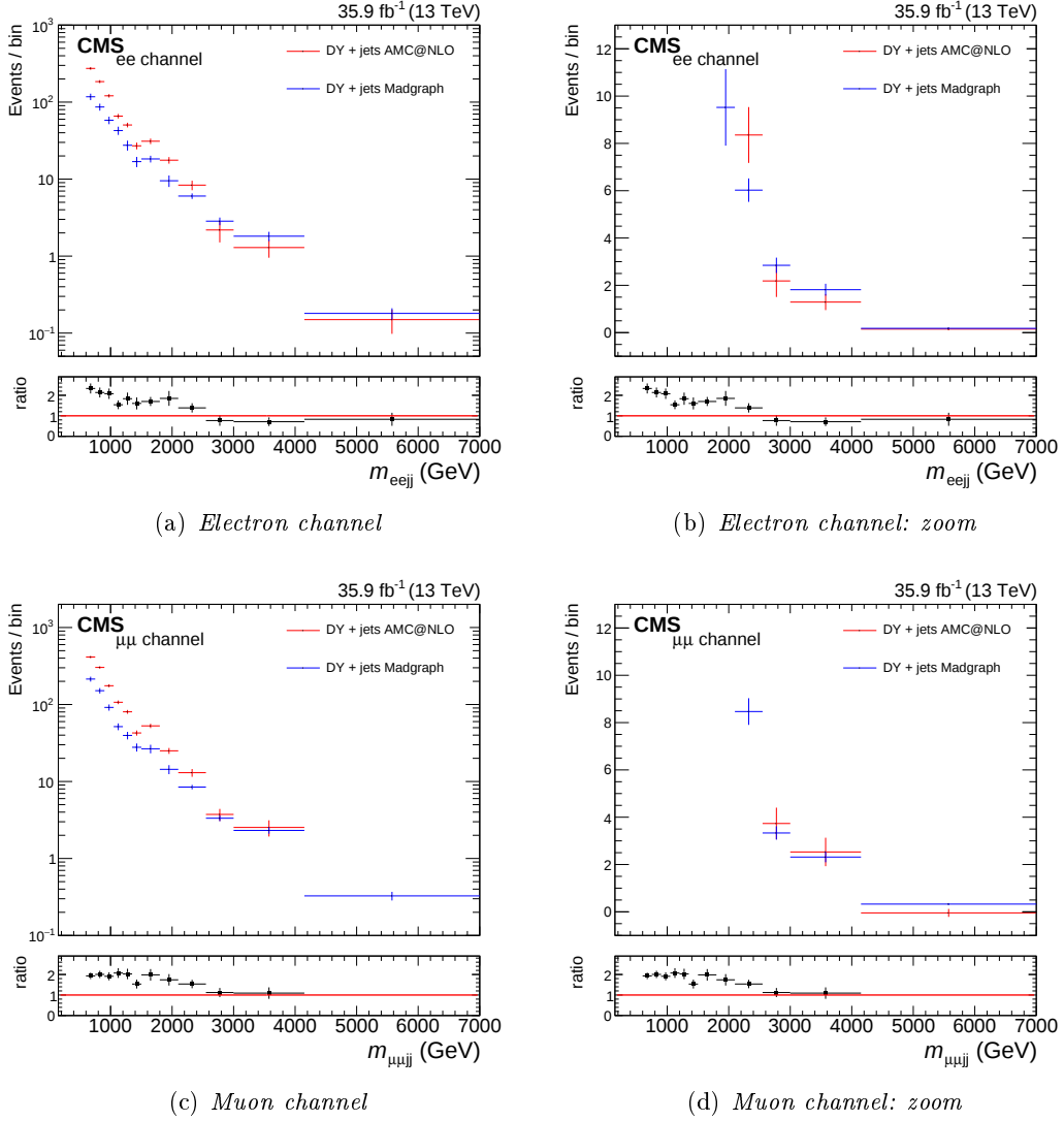
Figure 4.26: The m_{\ell\ell jj} distribution in the signal region for MC estimate from AMC@NLO and MADGRAPH.
