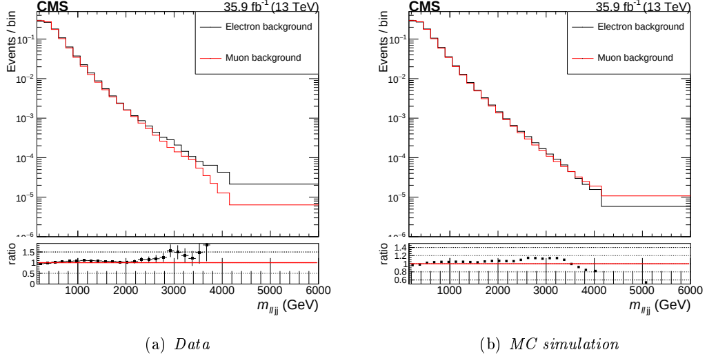
Figure 4.32: The m_{\ell\ell jj} cumulative distributions for electrons and muons and the ratio of electron events over muon events.
