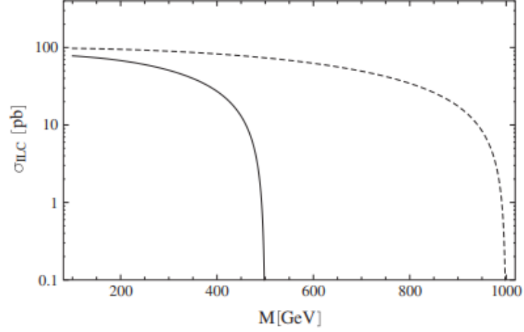
Figure 5.27: Total production cross section of the e^+e^- \rightarrow \bar{\nu}_l N_l process at the ILC with \sqrt{s} = 500 GeV (solid line) and 1 TeV (dashed line) [200].
