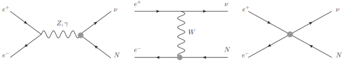
Figure 5.24: Feynman diagrams for the e^+e^- \rightarrow \nu N process [200].
