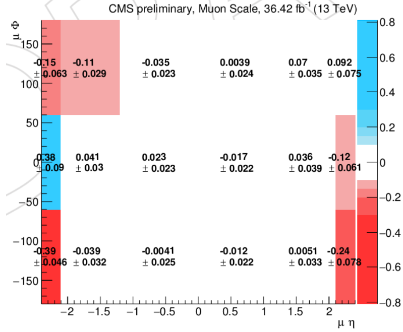
Figure 4.13: Scale bias (in %) of the “generalized endpoint” method [86] for muons with p_T > 200 (100) GeV in the region |\eta| < 2.1 ( > 2.1 ) in different \eta and \phi ranges.
