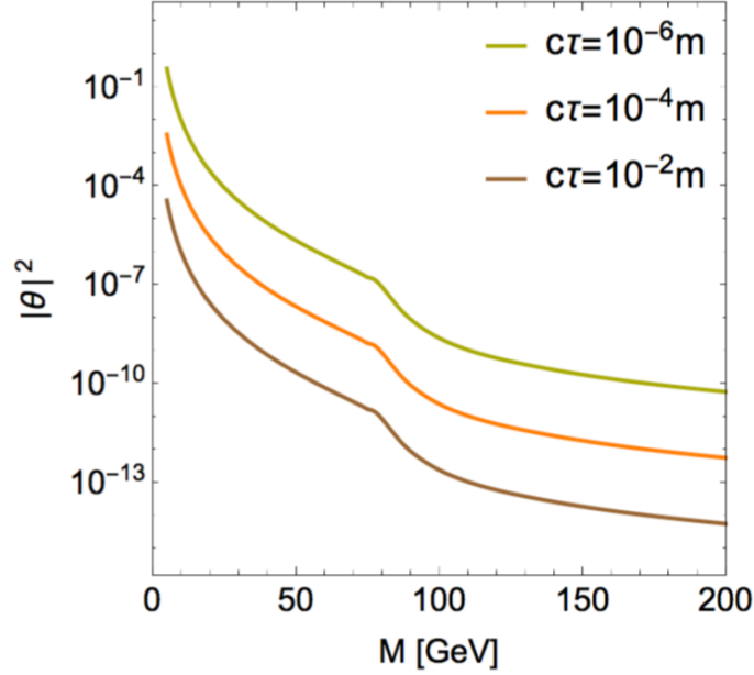
Figure 5.20: Projections on the mixing angle between one HNL and a lepton as a function of the HNL mass for different lifetimes.
