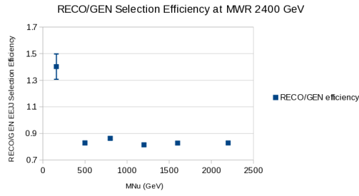
(a) Electron channel, m_{W_R} = 2.4 TeV
