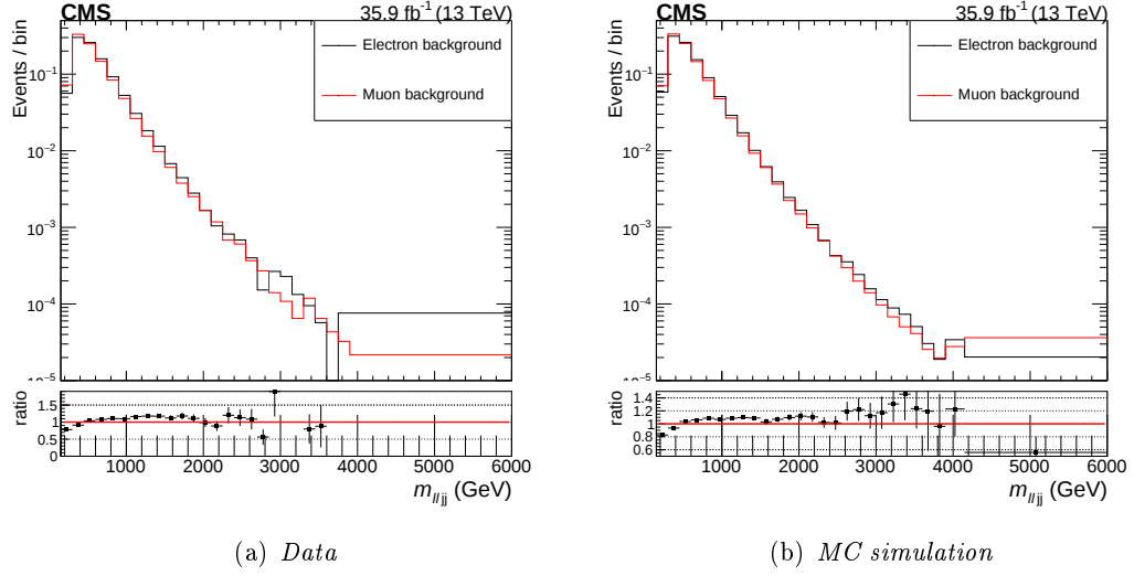
Figure 4.30: The m_{\ell\ell jj} distributions for electrons and muons and the ratio of electron events over muon events.
