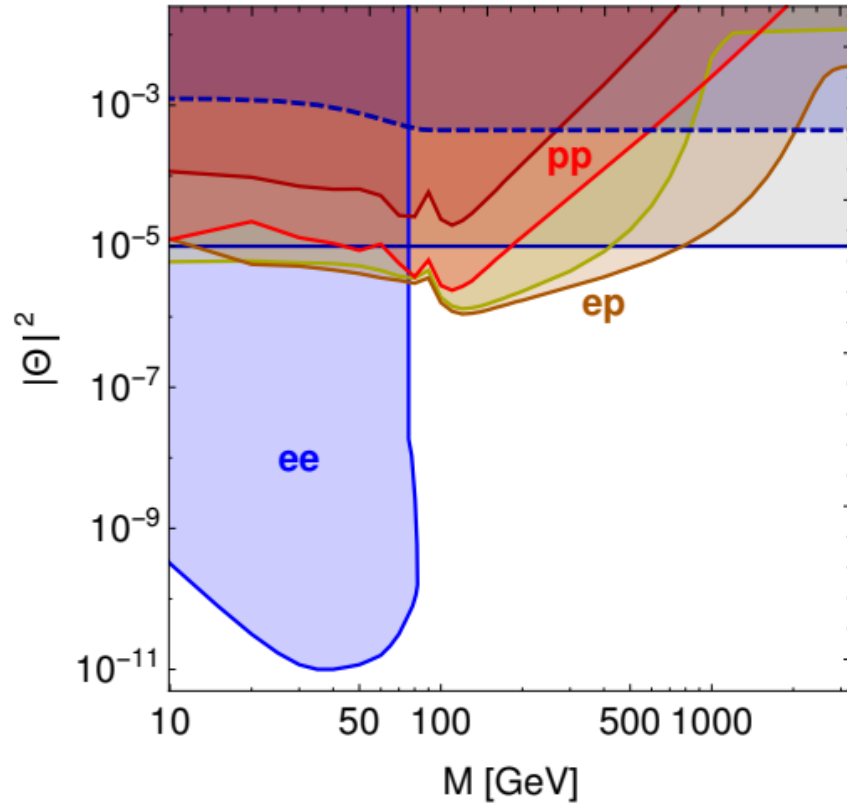
Figure 5.29: Sensitivities of the FCC- ee (blue line), FCC- hh (red line), and FCC- eh (brown line) colliders, including the HL-LHC (dark-red line) and the LHeC (yellow line) [197]. The solid and dashed horizontal blue line denotes the sensitivity to |\theta_e|^2 + |\theta_\mu|^2 and |\theta_\tau|^2 , respectively.
