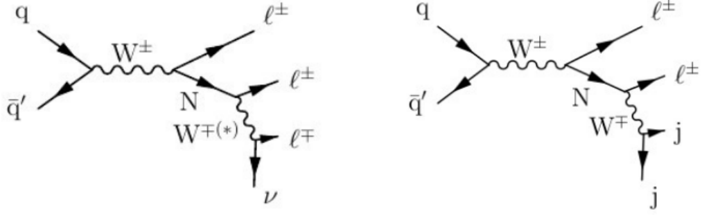
Figure 1.3: The Feynmann diagram for the heavy neutrino decay into a W boson and a lepton, with the W decaying into a lepton and a light neutrino (on the left) or into a pair of quarks (on the right).
