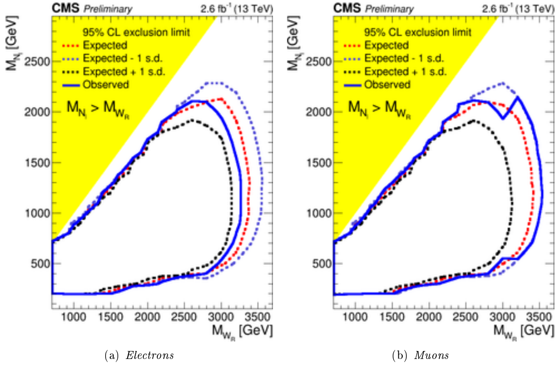
Figure 1.9: The 95% CL exclusion region in the (m_{W_R}, m_{N_R}) plane for the 2015 analysis. Neutrino masses greater than m_{W_R} (yellow region) are not considered in this search.
