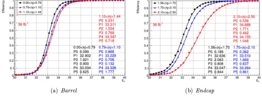
Figure 4.9: Efficiency of electrons passing offline ID requirements to match a L1 candidate with E_T > 33 GeV as a function of E_T [86].
