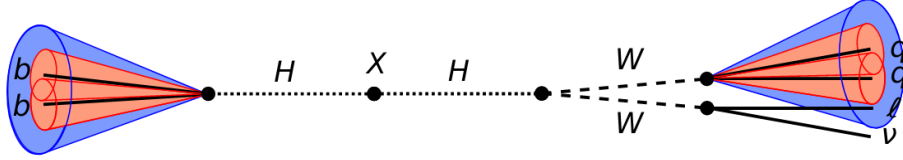
Figure 4.1.: Graphical representation of the boosted X \rightarrow HH \rightarrow b\bar{b}WW^* \rightarrow b\bar{b}qq\ell\nu topology as seen in the detector. The heavy resonance X shown in the center decays into a pair of Higgs bosons, which are seen back-to-back. They further decay into a pair of b -jets and two W bosons. The W bosons then finally decay into two quark jets, a lepton and a corresponding neutrino.
