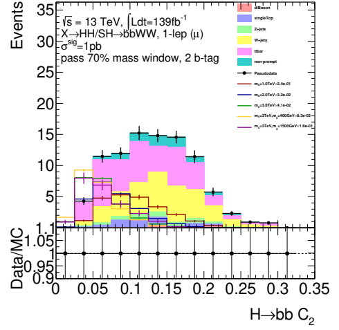
(f) SRf2, C_2^{H \rightarrow b\bar{b}}
