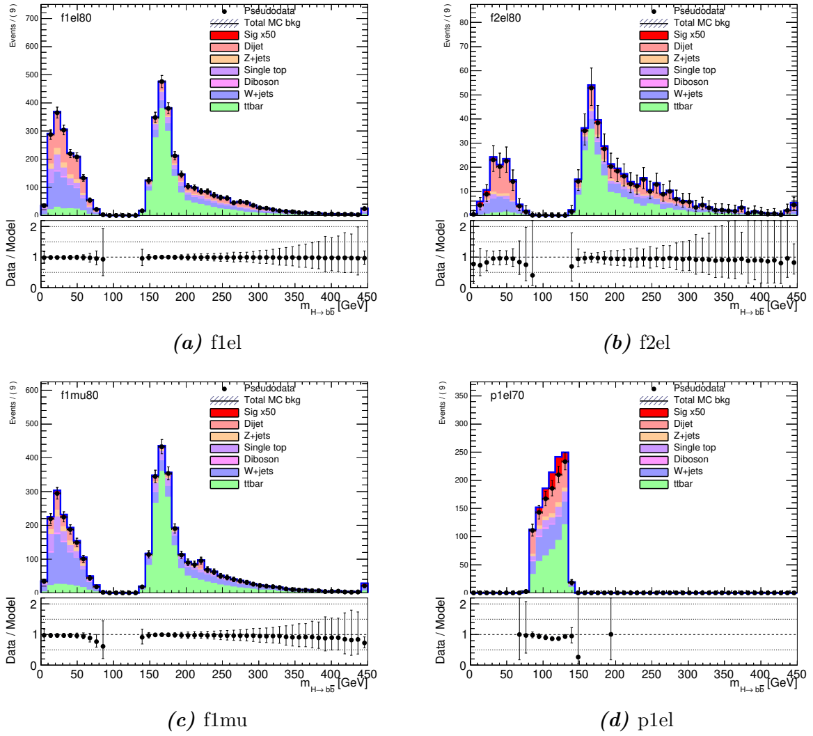
Figure 4.10.: Distributions of the m_{\text{TAR}}^{H \rightarrow b\bar{b}} variable in the four VRs of the 3P+1F case with dijet MC sample as a proxy for the QCD background. The data points correspond to the pseudodata which is set to the background only estimate. The signal here is the sum of all HH signal samples and scaled up by a factor of 50. The deviations in the ratio plots show the signal contribution.
