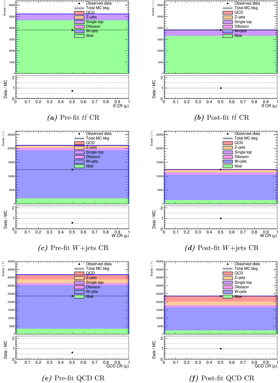
Figure 6.1.: Background composition in the t\bar{t} , W +jets and QCD CRs before and after performing the background normalisation fits. These plots correspond to the iteration with the data-driven non-prompt lepton backgrounds.
