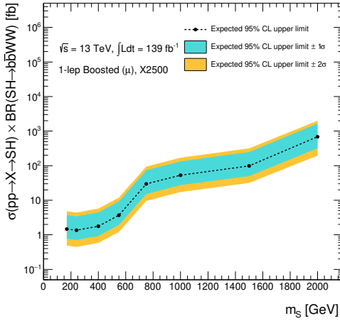
(e) m_X = 2.5 TeV
