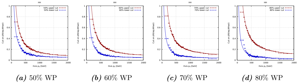
Figure B.2.: Different WPs for \Delta R(\ell, W_{\text{had}}) windows dependent on p_T^{H_{\text{vis}}} [98].
