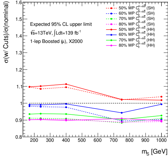
(c) SH samples with m_X = 2.0 \text{ TeV}
