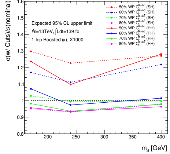
(b) SH samples with m_X = 1.0 \text{ TeV}
