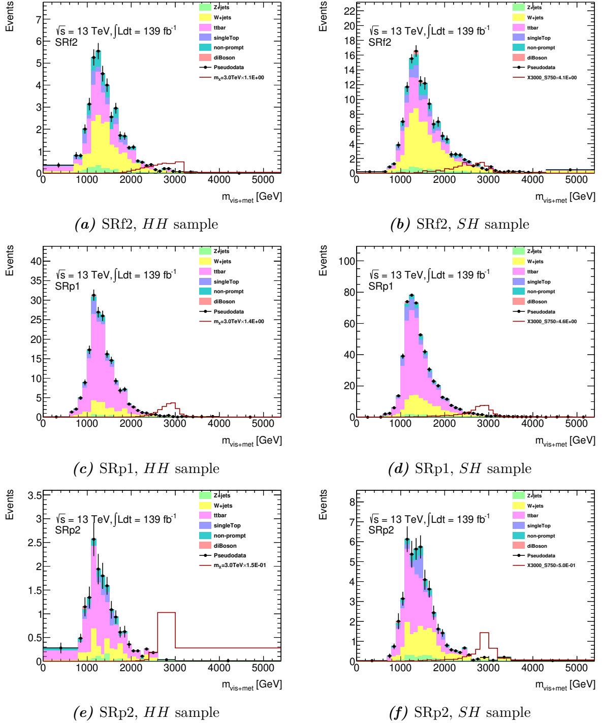
Figure 6.3.: Pre-fit distributions of m_{\text{vis+met}} in all three SRs with variable bin widths for m_X = 3.0 TeV HH sample, and m_X = 3.0 TeV and m_S = 750 GeV SH sample. The signal has been scaled up to 10% of the total background.
