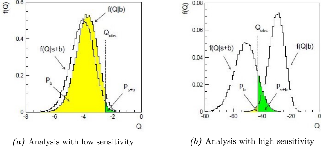
Figure 2.9.: Graphical representation of the ingredients for the \text{CL}_s procedure [52]. Here Q_{\text{obs}} is the observed test statistic, and f(Q|s+b) and f(Q|b) are the PDFs for the signal+background ( \mu = 1 ) and background-only ( \mu = 0 ) hypotheses, respectively.
