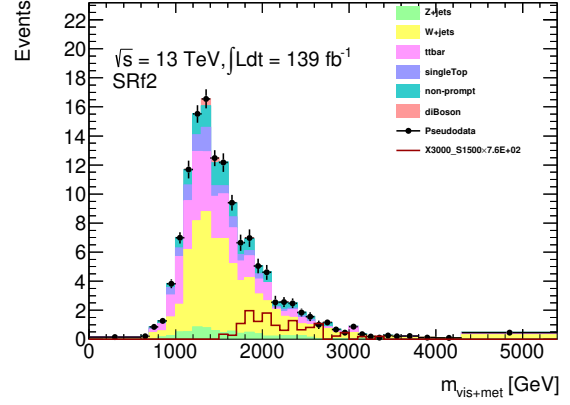
(b) SRf2, m_X = 3.0 TeV and m_S = 1500 GeV
