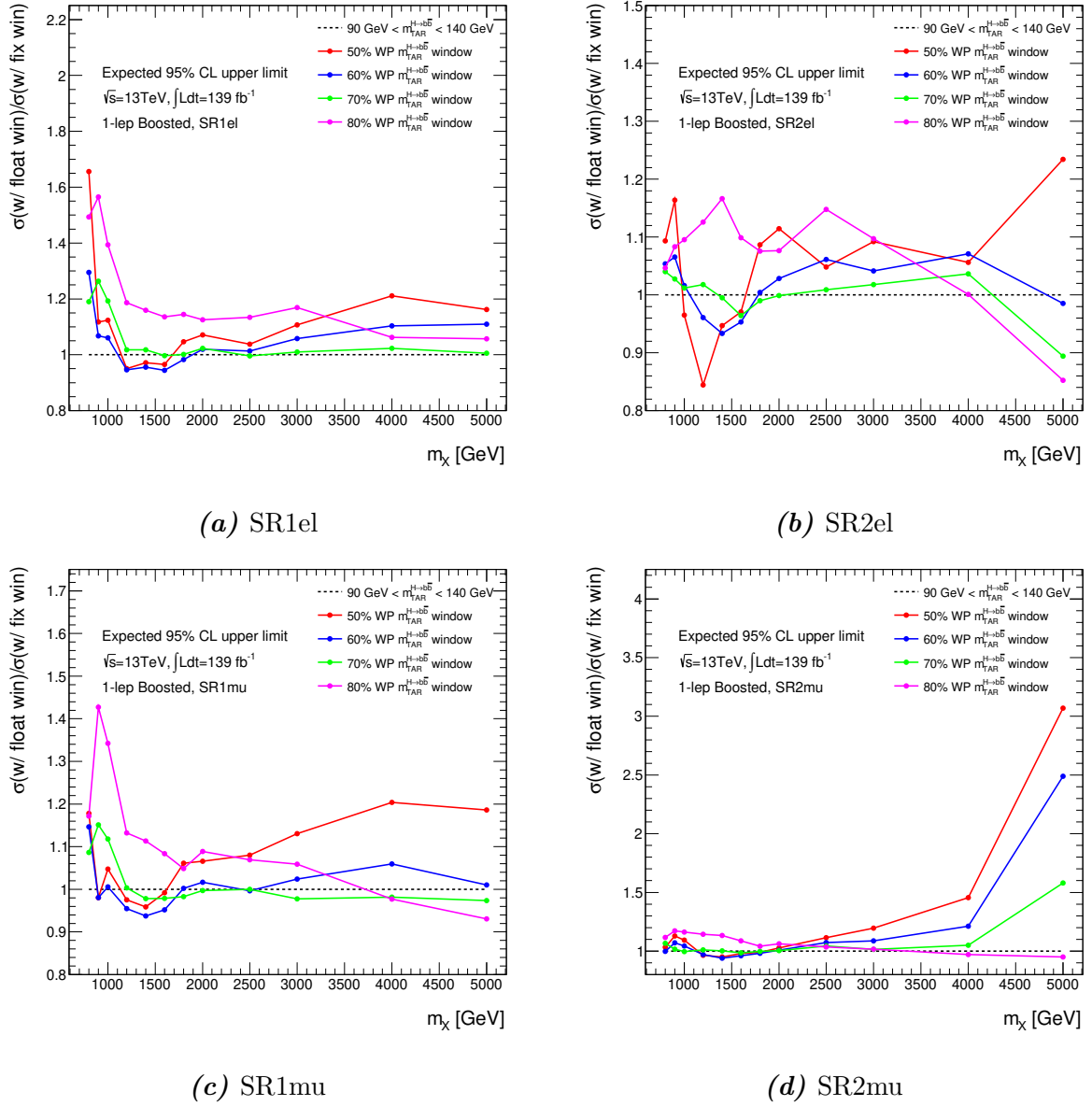
Figure 4.6.: Ratio of expected 95% C.L. exclusion limits on \sigma(pp \rightarrow X \rightarrow HH) with floating m_{\text{TAR}}^{H \rightarrow b\bar{b}} window to those with fixed 90 \text{ GeV} < m_{\text{TAR}}^{H \rightarrow b\bar{b}} < 140 \text{ GeV} in all four SRs. Only statistical uncertainties are included in shown expected exclusion limits.
