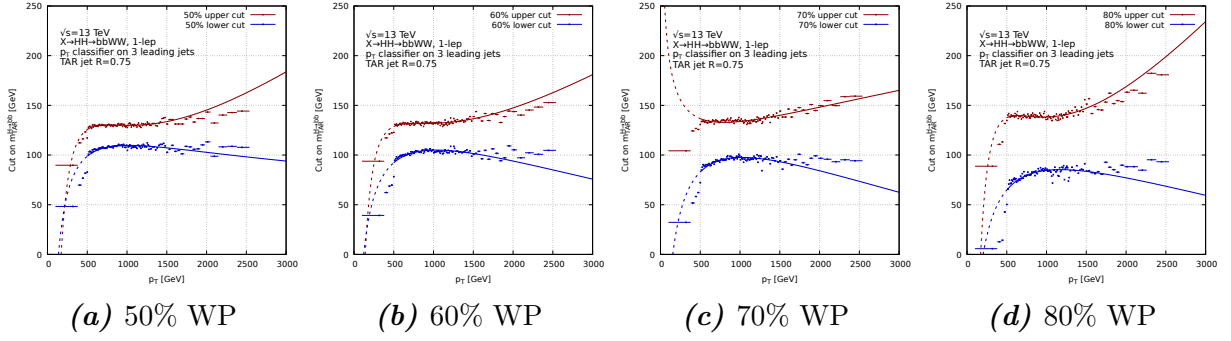
Figure B.1.: Different WPs for m_{\text{TAR}}^{H \rightarrow b\bar{b}} windows dependent on p_T^{H \rightarrow b\bar{b}} [98].
