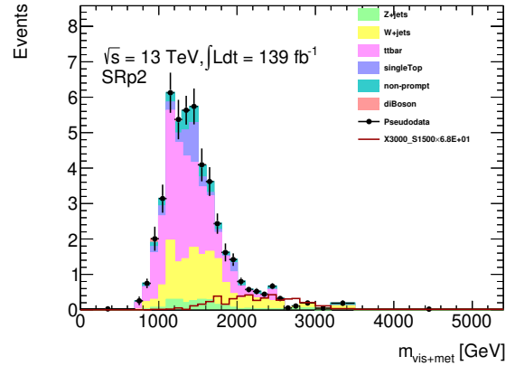
(f) SRp2, m_X = 3.0 TeV and m_S = 1500 GeV
