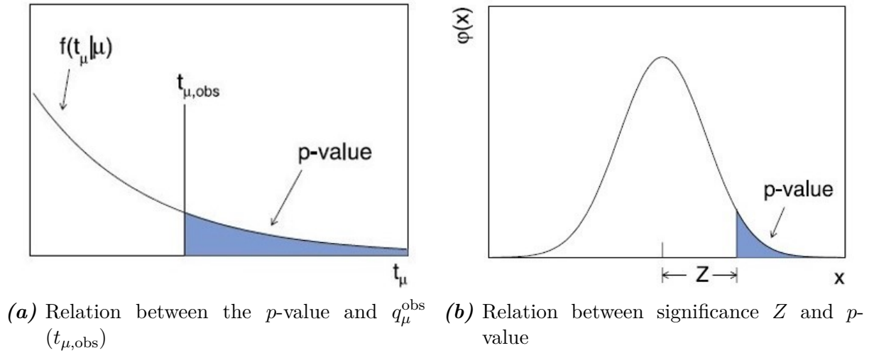
Figure 2.8.: Graphical representation of PDF \mathcal{P}(q_\mu|\mu) ( f(t_\mu|\mu) ), observed test statistic q_\mu^{\text{obs}}(t_{\mu,\text{obs}}) , p -value and significance Z [51].
