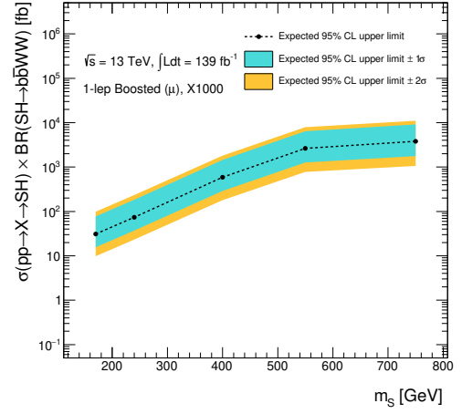
(b) m_X = 1.0 TeV
