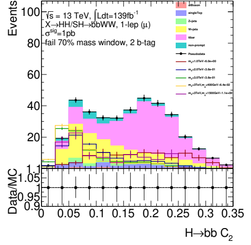
(b) SRf2, C_2^{H \rightarrow b\bar{b}}
