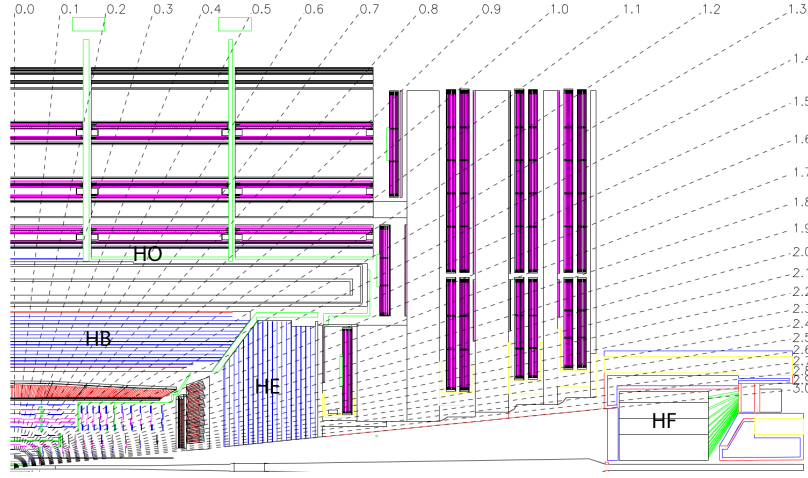
Figure 2.11: Representation of a quarter of the hadronic calorimeter in the longitudinal plane, indicating the locations of the Hadron Barrel (HB), Endcap (HE), Outer (HO) and Forward (HF) subdetectors. Taken from Ref. [117].
