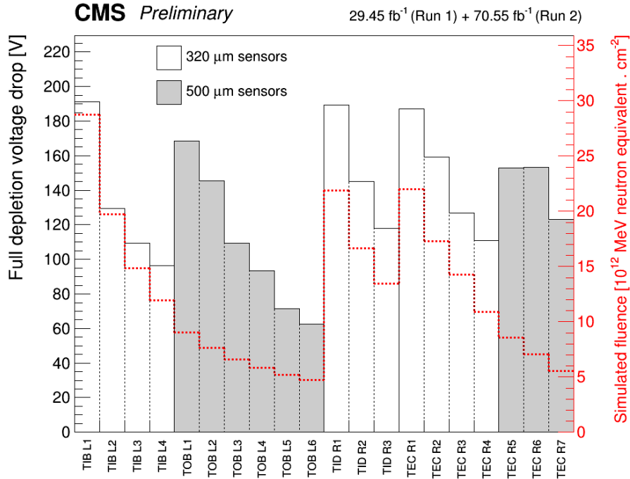
Figure 3.13: Average decrease of V_{FD} for each layer of the strip tracker, computed as the difference between the values measured at the time of the tracker construction and the values obtained by the analysis of a full scan performed in September 2017. The average fluence for each layer is shown by the red line. This figure was made public [203].
