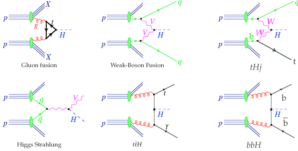
Figure 1.13: LO Feynman diagrams for the main production modes of the Higgs boson. Taken from Ref. [85].
