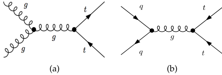
Figure 1.9: Tree-level Feynman diagrams for top quark pair production via (a) gluon fusion and (b) quark-antiquark annihilation.
