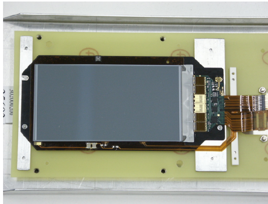
Figure 2.9: Single-sided TIB module. The 512 strips are read-out by 4 APV chips on the right-hand side. Taken from Ref. [158].
