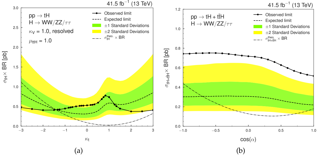
Figure 5.16: (a) Observed and expected 95% CL upper limits on the tH cross section times H \rightarrow WW^* + \tau\tau + ZZ^* branching ratio as a function of \kappa_t , assuming \kappa_V = 1 . The \kappa_t -dependent contribution from t\bar{t}H is kept fixed in the fit ( \mu_{t\bar{t}H} = 1 ), while the signal strength \mu_{tH} of the tH signal is allowed to float. (b) Observed and expected 95% CL upper limits on the tH + t\bar{t}H cross section times H \rightarrow WW^* + \tau\tau + ZZ^* branching ratio as a function of \cos(\alpha) . Expected limits are derived from background-only Asimov datasets. These figures were produced by the other PhD within the framework of the t\bar{t}H group, using templates I provided.
