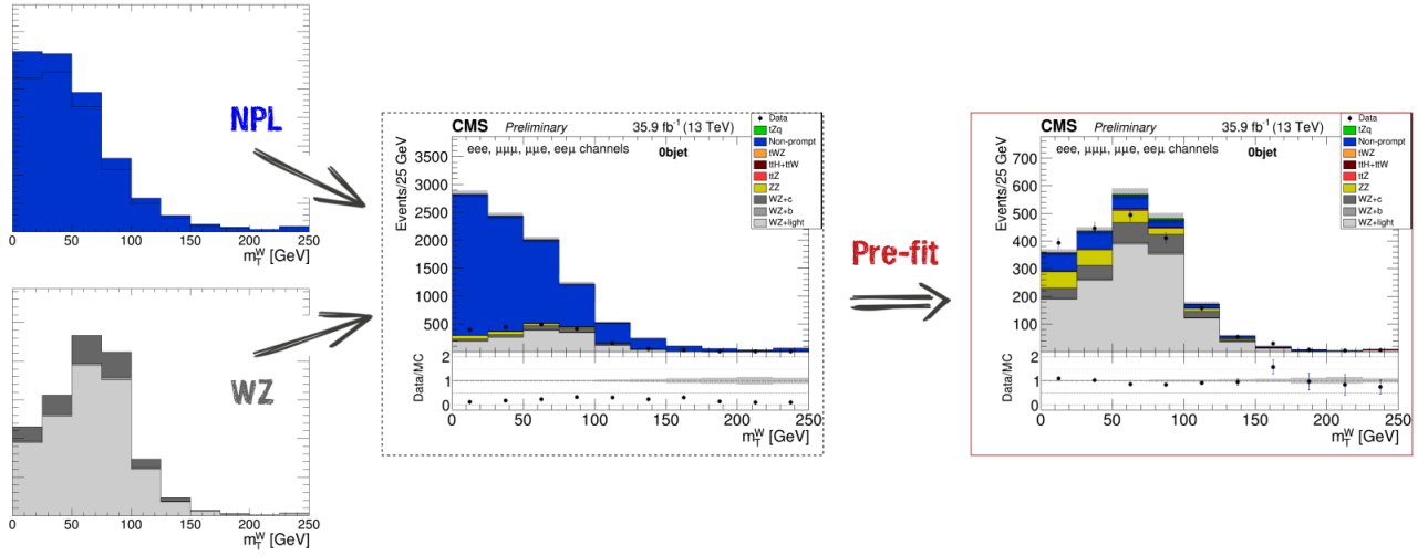
Figure 4.6: Sketch of the procedure used to obtain the "pre-fit" normalizations of the NPL samples. The fit is performed in the Objet control region dominated by the WZ+jets process (split depending on the jet flavour) and DY+jets events in association with a NPL. A fit is performed to the m_T(W) variable, and only the normalizations of the NPL backgrounds may vary.
