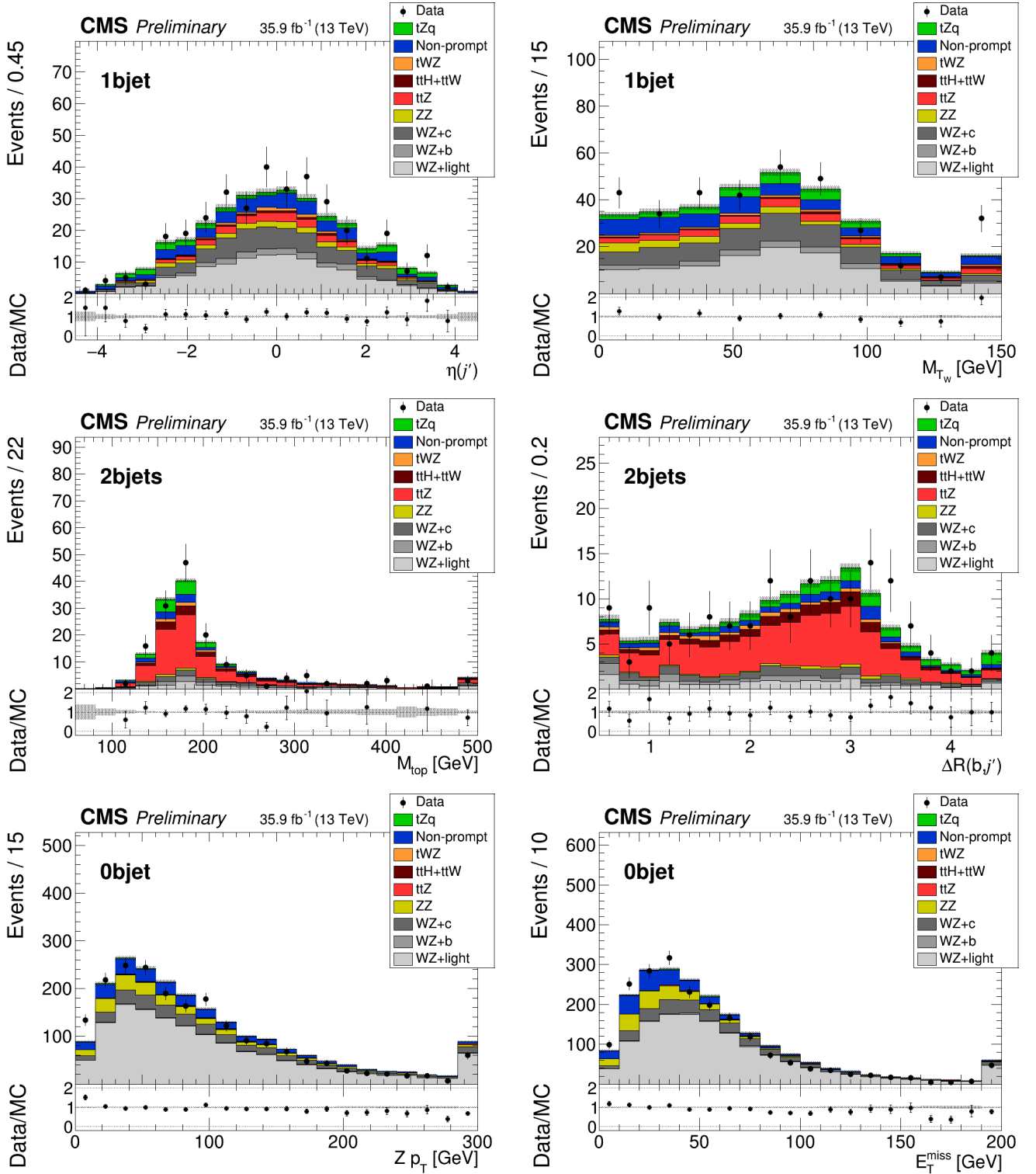
Figure 4.5: Distributions of several kinematic observables in the 1bjet signal region (top), 2bjets control region (middle) and 0bjet control region (bottom). The 4 channels are summed. The MC simulations of SM processes (stacked histograms) are compared to the data (black dots). The grey shaded areas represent the MC statistical uncertainty only, and do not include systematic uncertainties. From top to bottom and left to right, the following quantities are represented: \eta of the recoiling jet; m_T(W) ; the mass of the reconstructed top quark; \Delta R separation between the b-tagged jet associated with the top quark decay and the recoiling jet; p_T of the Z boson; E_T^{\text{miss}} .
