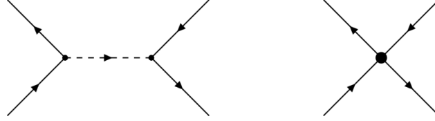
Figure 1.15: Illustration of the basic concept of an EFT. An interaction mediated by a new, yet undiscovered particle (left) is considered as a contact interaction (right) for simplification.
