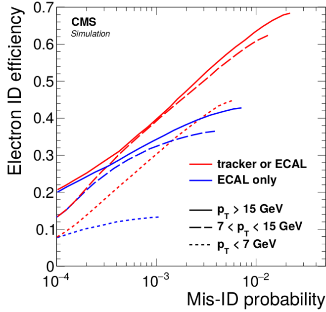
Figure 2.14: Comparison of the efficiency to reconstruct and identify electrons ( p_T > 2 GeV, |\eta| < 2.4 ) from b-hadrons decays versus the probability to misidentify jets as electrons, using 2 different algorithms on simulated events, motivating the combination of the ECAL and tracker information for the seeding of electrons. Taken from Ref. [173].
