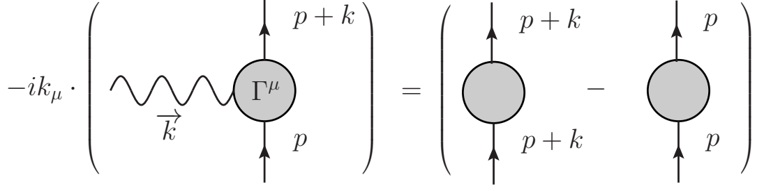
Figure 2.1: Diagrammatic description of an application of the Ward-Takahashi identity in QED. On the left hand-side the contraction between the photon polarization vector was replaced by its momentum. The vertex and the propagators are the exact ones.
