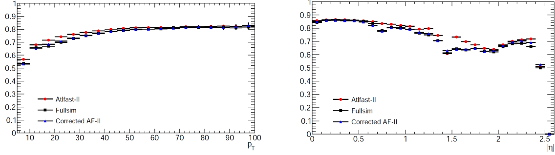
Figure 7.3: The electron p_T and \eta distribution for the comparison of ATLFAST-II to full simulation. Better agreement is seen with additional corrections. [74]
