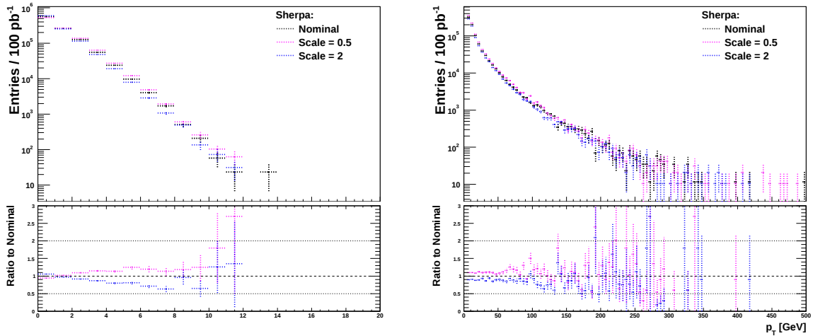
Figure 9.11: Jet multiplicity (left) and p_T (right) distributions for the comparison of Sherpa for varied scales. The variations have similar trends to that of ALPGEN.
