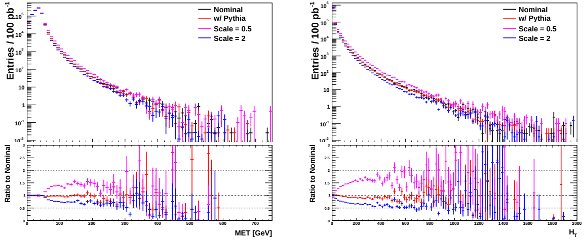
Figure 9.9: E_T (left) and H_T (right) distributions for the comparison of ALPGEN for varied scales. Clear differences are seen for scale variations.
