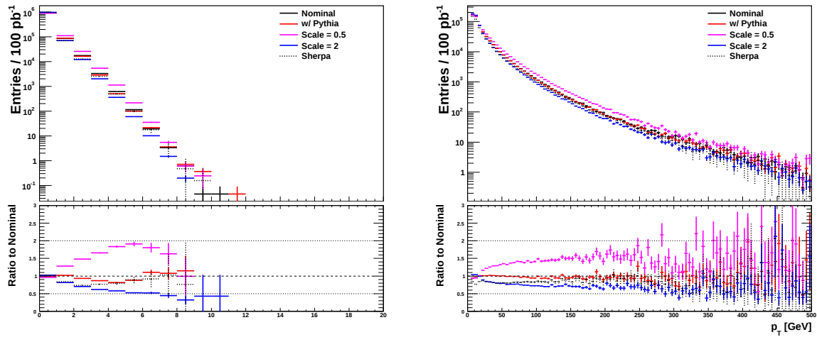
Figure 9.14: Jet multiplicity distributions for preselected jets with p_T > 30 GeV (left) and the p_T distribution for the hardest jet (right) for the comparison of ALPGEN with Sherpa.
