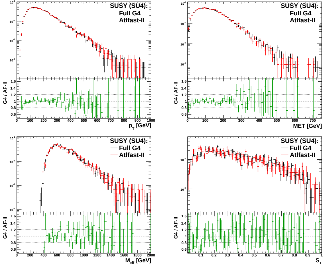
Figure 7.4: The distributions of the p_T of the leading jet (after cut2), the \cancel{E}_T (after cut 3), the M_{eff} (after cut 5) and the S_T (after cut 6) for SUSY signal events. The results obtained from full simulation (black) and ATLFAST-II (red) are superimposed.
