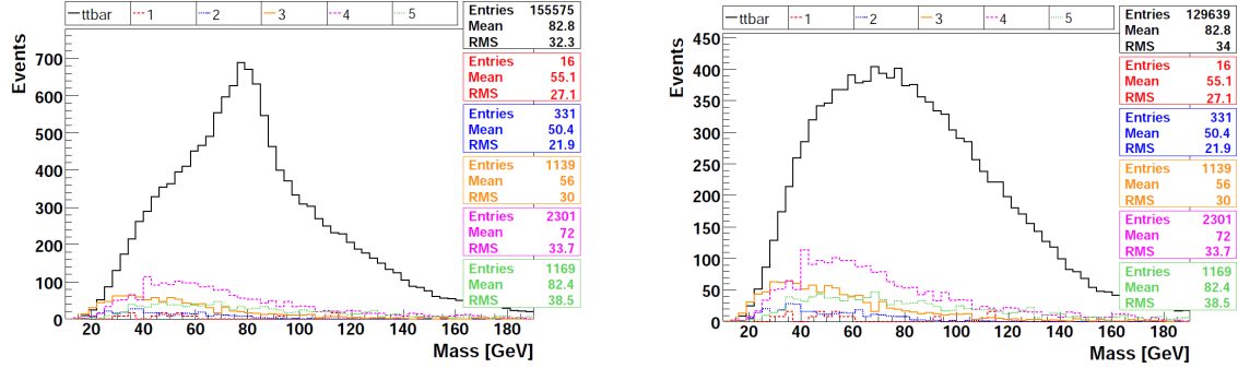
Figure 8.3: The W mass distribution from t\bar{t} with the W+nJets ( n \in [1,5] ) samples overlaid for 100 pb^{-1} . The left plot shows all samples while the right plots has the correctly assigned hypotheses removed and therefore only shows background.
