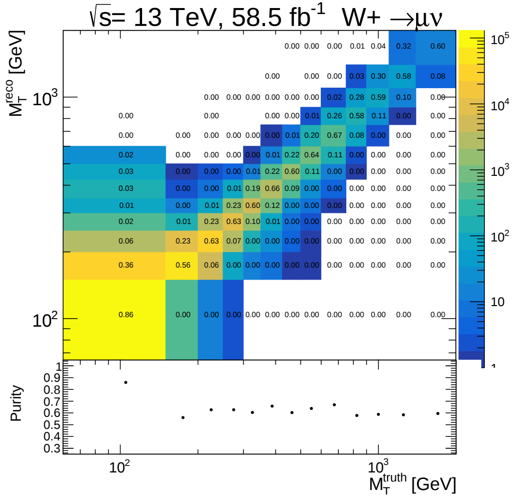
Figure E26.: Migration matrix M_{\text{reco},\text{truth}} for the W^+ \rightarrow \mu^+ \nu MC16e signal process. The upper panel shows the m_T^W truth level vs the m_T^W reconstruction level events. The given numbers show the ratio of the number of events in each bin to the total number of reconstructed event in the given mass bin. The diagonal of the upper panel gives the purity in the lower panel.
