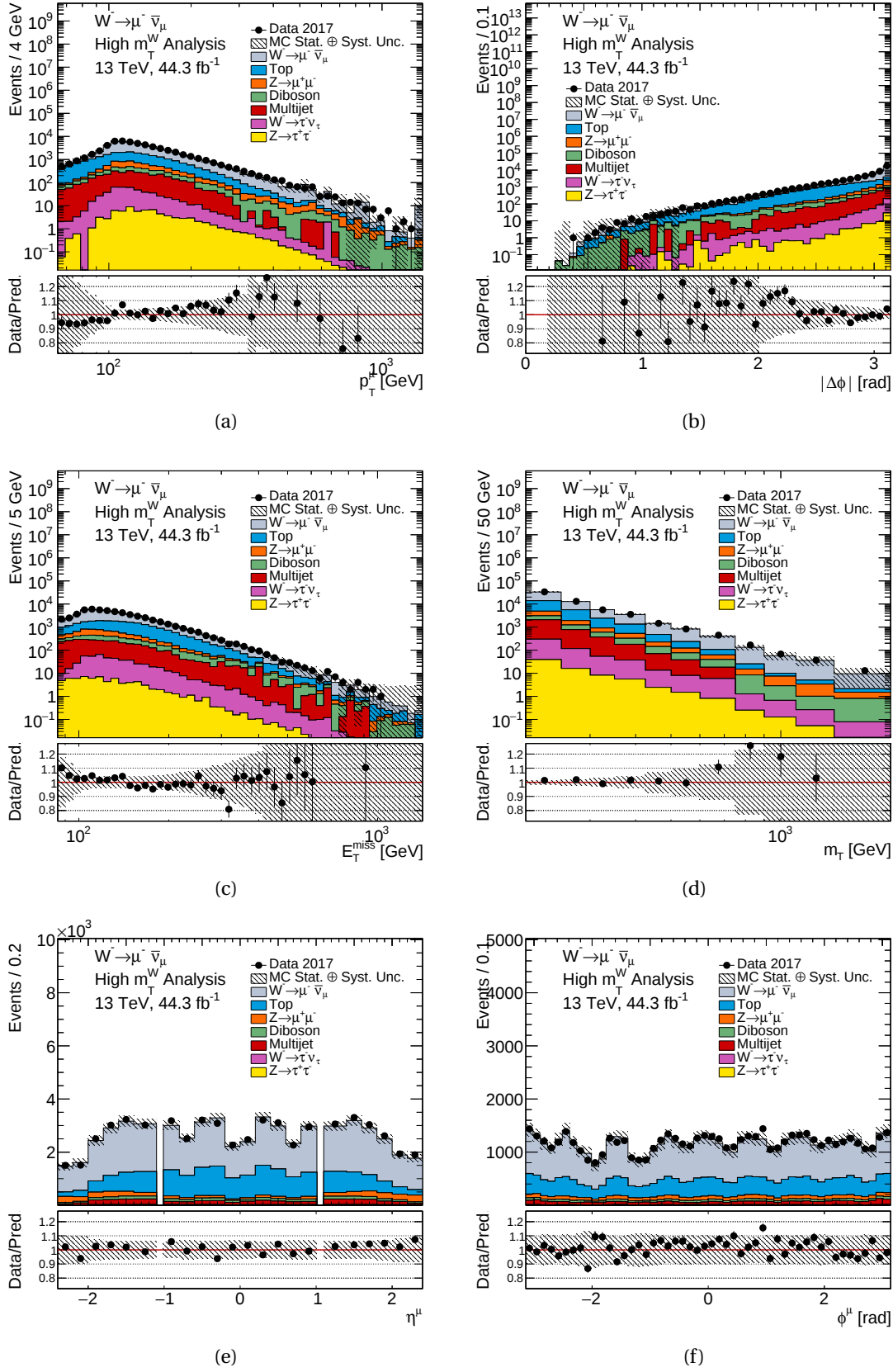
Figure E.11.: MC16d W^- \rightarrow \mu^- \bar{\nu}_\mu control distributions for p_T^\mu , |\Delta\phi| , E_T^{\text{miss}} , m_T , \eta^\mu and \phi^\mu . The data contribution is shown with black points, the signal and the background contributions with solid lines. In the shaded band, systematic experimental uncertainties have been combined with the MC statistical uncertainties. The data statistical uncertainties are shown on the data points. Luminosity uncertainties have not been included.
