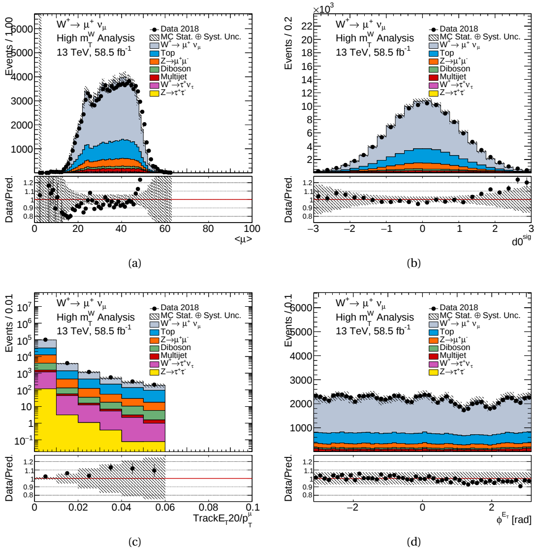
Figure E.17.: MC16e W^+ \rightarrow \mu^+ \nu control distributions for \langle \mu \rangle , d0^{sig} , TrackE_{T20}/p_T^\mu and \phi_{E_T}^{miss} . The data contribution is shown with black points, the signal and the background contributions with solid lines. In the shaded band, systematic experimental uncertainties have been combined with the MC statistical uncertainties. The data statistical uncertainties are shown on the data points. Luminosity uncertainties have not been included.
