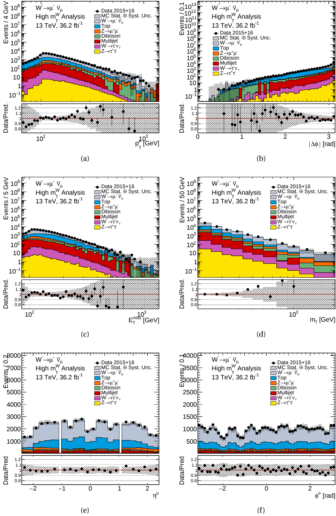
Figure E.4.: MC16a W^- \rightarrow \mu^- \bar{\nu} control distributions for p_T^\mu , |\Delta\phi| , E_T^{\text{miss}} , m_T , \eta^\mu and \phi^\mu . The data contribution is shown with black points, the signal and the background contributions with solid lines. In the shaded band, systematic experimental uncertainties have been combined with the MC statistical uncertainties. The data statistical uncertainties are shown on the data points. Luminosity uncertainties have not been included.
