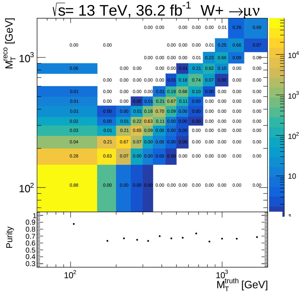
Figure E22.: Migration matrix M_{\text{reco},\text{truth}} for the W^+ \rightarrow \mu^+ \nu MC16a signal process. The upper panel shows the m_T^W truth level vs the m_T^W reconstruction level events. The given numbers show the ratio of the number of events in each bin to the total number of reconstructed event in the given mass bin. The diagonal of the upper panel gives the purity in the lower panel.
