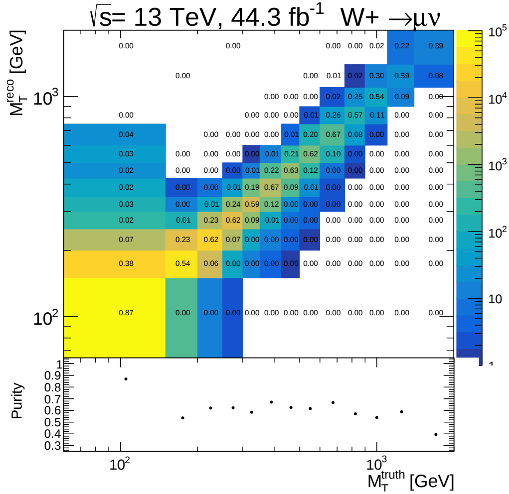
Figure E24.: Migration matrix M_{\text{reco},\text{truth}} for the W^+ \rightarrow \mu^+ \nu MC16d signal process. The upper panel shows the m_T^W truth level vs the m_T^W reconstruction level events. The given numbers show the ratio of the number of events in each bin to the total number of reconstructed event in the given mass bin. The diagonal of the upper panel gives the purity in the lower panel.
