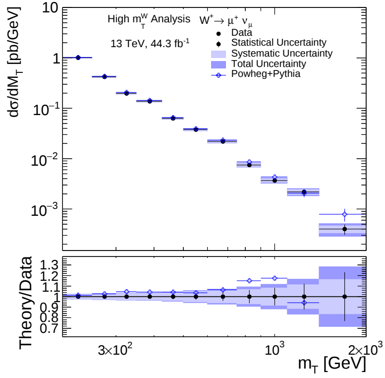
(a) W^+
