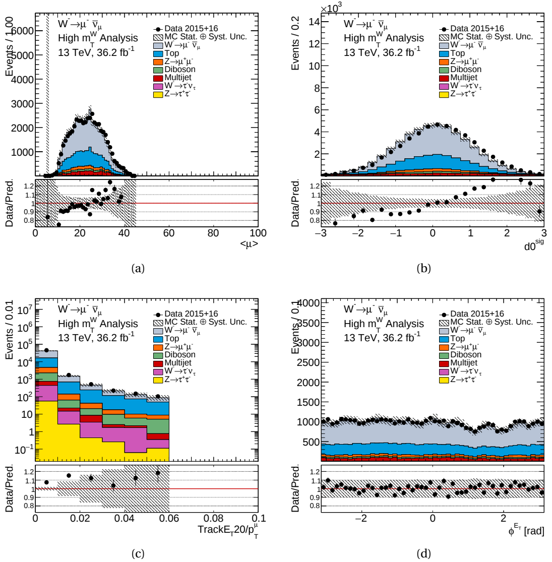
Figure E.5.: MC16a W^- \rightarrow \mu^- \nu control distributions for \langle \mu \rangle , d_0^{sig} , TrackE_T20/p_T^\mu and \phi^{E_T^{miss}} . The data contribution is shown with black points, the signal and the background contributions with solid lines. In the shaded band, systematic experimental uncertainties have been combined with the MC statistical uncertainties. The data statistical uncertainties are shown on the data points. Luminosity uncertainties have not been included.
