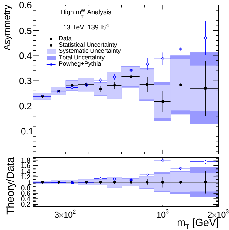
Figure 10.9.: Muon charge asymmetry binned in m_T^W calculated using Equation 10.2. Statistical and systematic uncertainties are included in the uncertainty band. Statistical and systematic uncertainties are included in the uncertainty band. The dark blue band shows the total uncertainty. The ratio is between the measured data and the truth (prediction) distributions.
