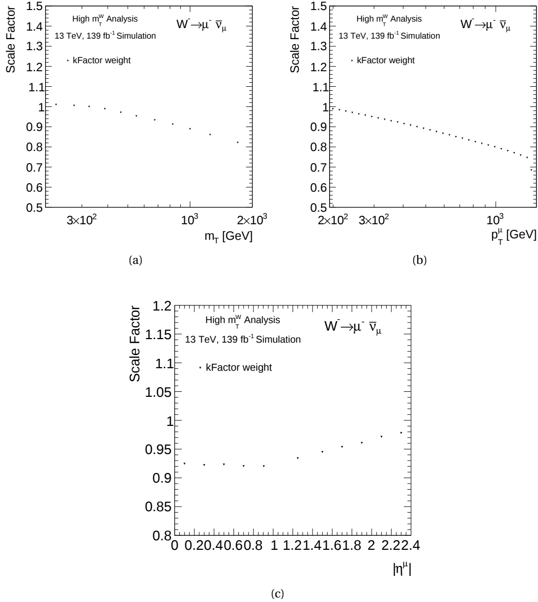
Figure B.5.: Scale Factor plots for average k-Factor efficiency. These plots are for W^- \rightarrow \mu^- \bar{\nu} for the combination of Monte Carlo campaigns, MC16a, MC16d, MC16e. The plots show average k-Factor as a function of transverse mass m_T (a), p_T^\mu (b) and |\eta^\mu| (c).
