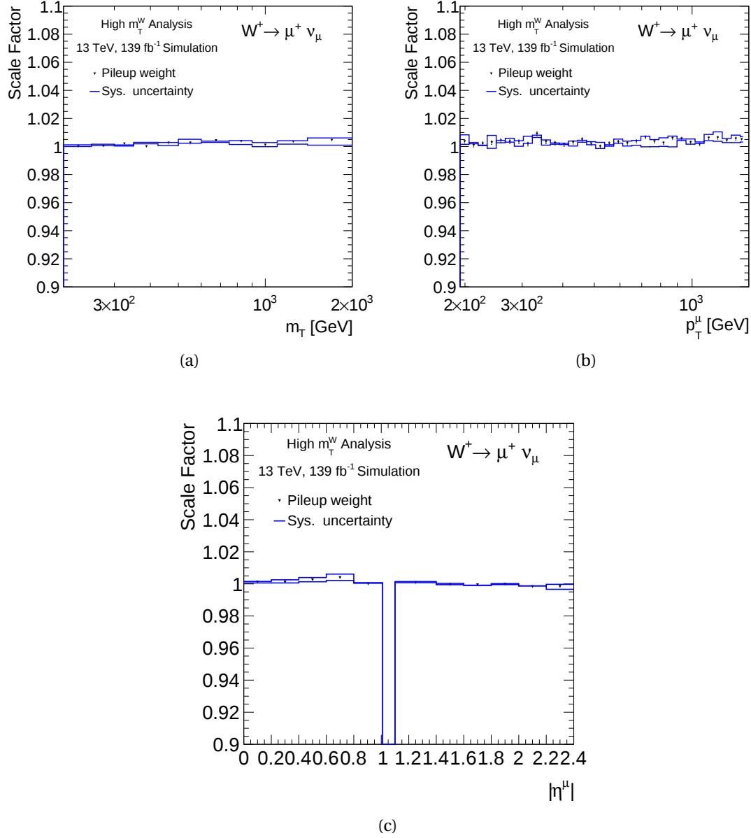
Figure B.9.: Plots for average pileup weight. These plots are for W^+ \rightarrow \mu^+ \nu for the combination of Monte Carlo campaigns, MC16a, MC16d, MC16e. The plots show average pileup weight as a function of transverse mass m_T (a), p_T^\mu (b) and |\eta^\mu| (c). The individual systematics and statistical for one standard deviation are shown in blue and red.
