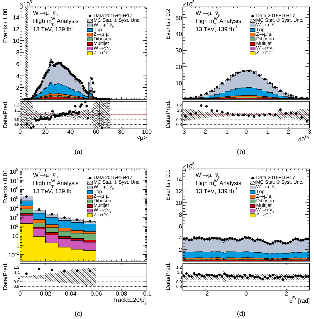
Figure 9.5.: W^- \rightarrow \mu^- \bar{\nu} control distributions for \langle \mu \rangle , d0^{sig} , TrackE_{T20}/p_T^\mu and \phi^{E_T^{miss}} . The data contribution is shown with black points, the signal and the background contributions with solid lines. In the shaded band, systematic experimental uncertainties have been combined with the MC statistical uncertainties. The statistical data uncertainties are shown on the data points. Luminosity uncertainties have not been included.
