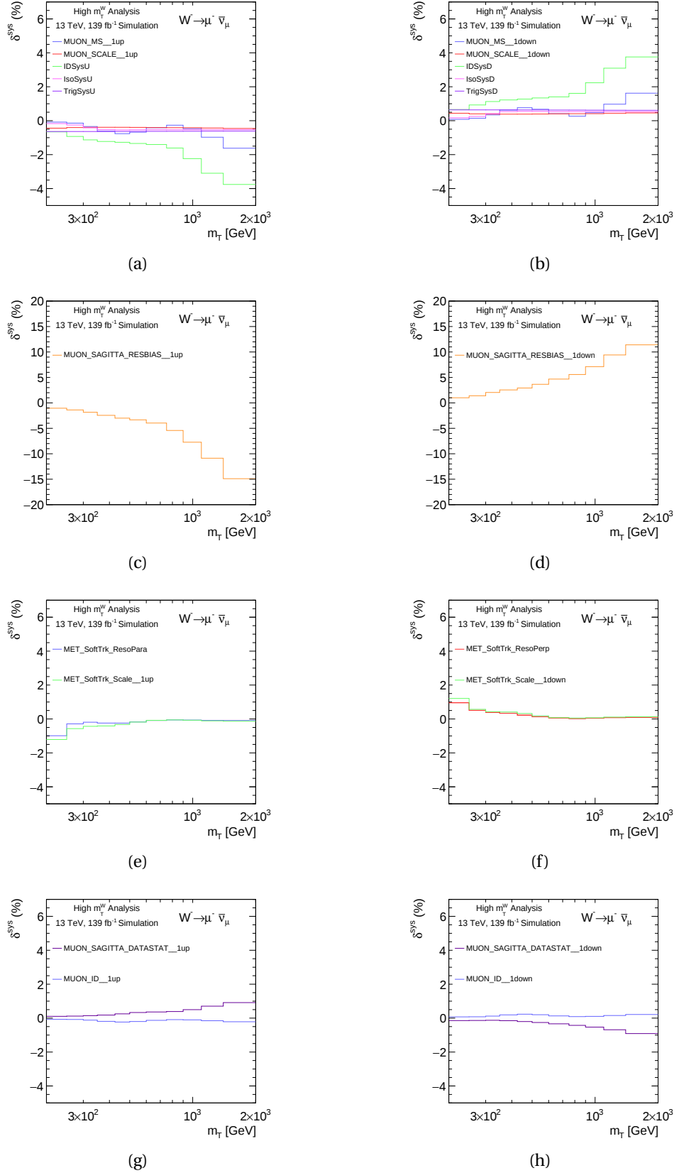
Figure 8.4.: Individual contributions to the systematic variations in Run-2 for W^- \rightarrow \mu^- \bar{\nu} in the measurement binning for m_T . The plots on the left show the up variations and those on the right show the down variations. All values are presented in percentages. Plots (a) and (b) show the muon scale and resolution uncertainties along with the muon scale identification, isolation and trigger scale factor uncertainties. Plots (c) and (d) display the muon sagitta resolution bias uncertainty. Plots (e) and (f) show the missing energy soft track uncertainties. The labels in the legend of both plots are the conventional names given by the JetEtMiss group. "MET" stands for missing energy, "SofTrk" refers to soft track E_T^{miss} and "ResoPara" and "ResoPerp" refers to the resolution uncertainty on the parallel and perpendicular component. Plots (g) and (h) display the muon sagitta data statistical and muon identification uncertainty.
