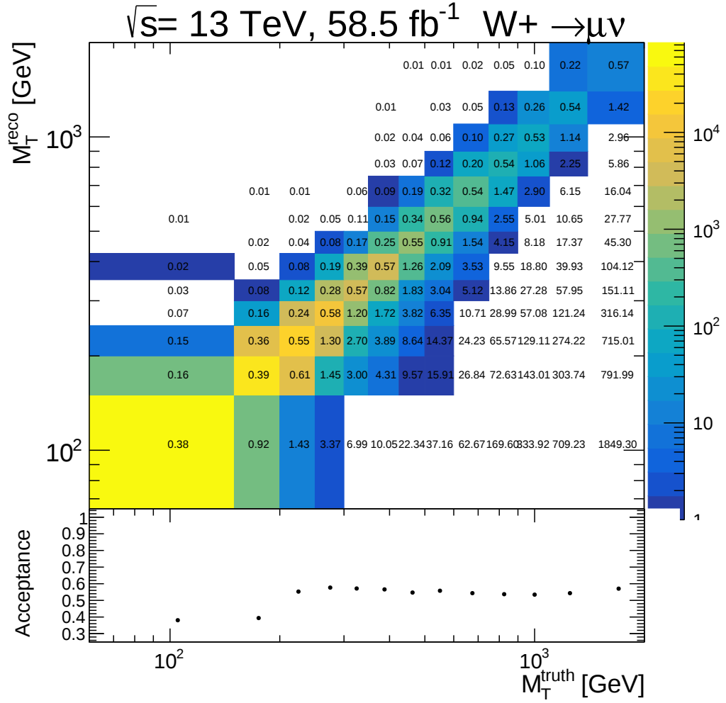
Figure E15.: Acceptance for the W^+ \rightarrow \mu^+ \nu MC16e signal process. The upper panel shows the m_T^W truth level vs the m_T^W reconstruction level events. The given numbers show the ratio of the total number of truth events in each bin to the total number of reconstructed events in each bin. The diagonal of the upper panel gives the acceptance in the lower panel.
