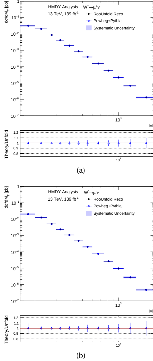
Figure 10.7.: Closure test for unfolding using RooUnfold . Here the reconstruction Monte Carlo has been used in place of real measured data. The unfolding matrix is constructed using truth ( POWHEG+PYTHIA ) and reconstruction-level information. Therefore, by definition, the reconstruction events must identically unfold to the truth level, as shown in the ratio panel. The full systematic and statistical uncertainties are not included.
