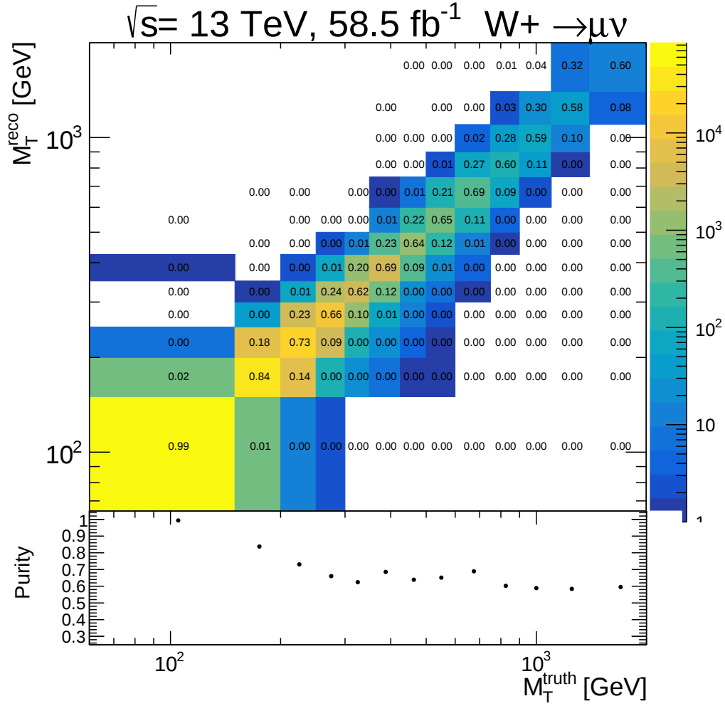
Figure E14.: Purity for the W^+ \rightarrow \mu^+ \nu MC16e signal process. The upper panel shows the m_T^W truth level vs the m_T^W reconstruction level events. The given numbers show the ratio of the number of events in each bin to the total number of reconstructed event in the given mass bin. The diagonal of the upper panel gives the purity in the lower panel.
