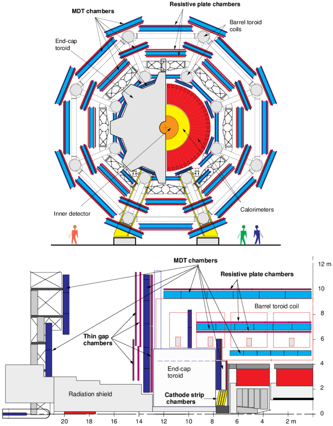
Figure 3.10.: ATLAS cross and side view of the Muon System [66].
