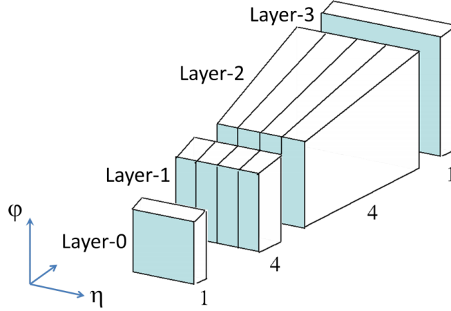
Figure 4.1.: SuperCell configuration in a LAr trigger tower for Run-3 after upgrading the LAr Calorimeter readout/trigger. The dimension of the object depicted in the sketch is 0.1 \times 0.1 in \eta and \phi in all layers. Ten E_T values are provided from the "1-4-4-1" structure. Layer-0 here corresponds to the pre-scaler [78].
