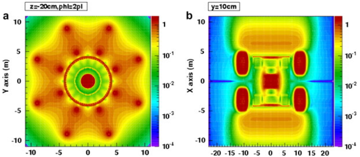
Figure 3.4.: ATLAS magnetic field shown in a) transverse cross-section of the magnetic field in the centre of the magnet system (not including endcap toroids) b) longitudinal cross-section showing central solenoid, end cap toroids and barrel toroids [51].
