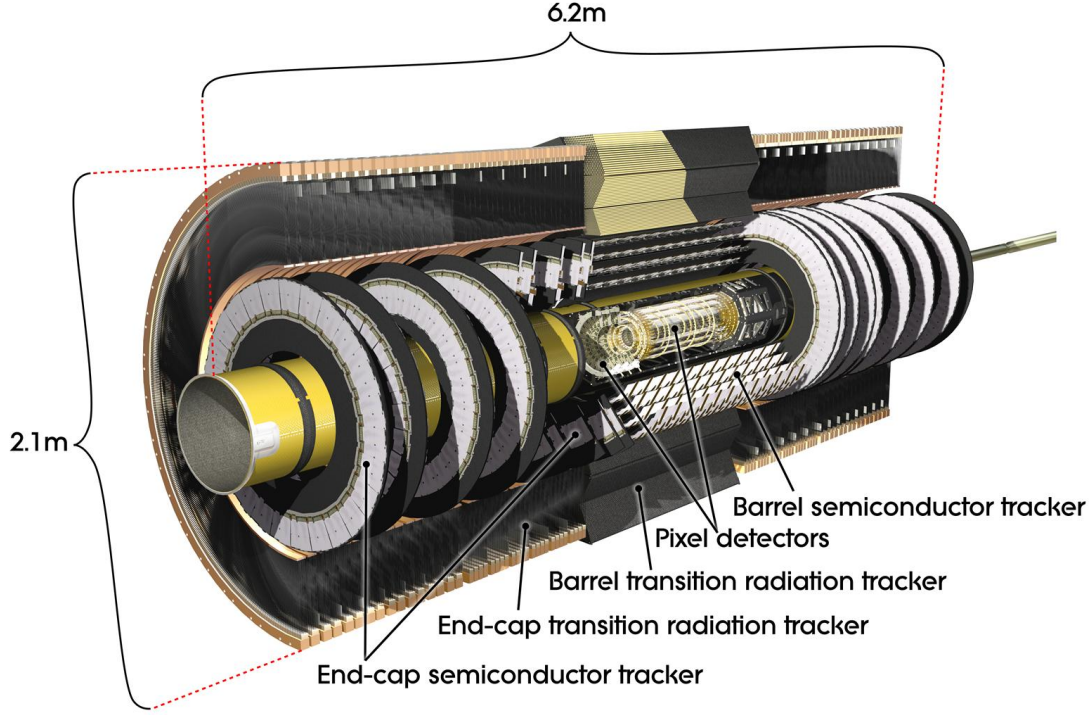
Figure 3.5.: Schematic of the ATLAS inner detector subsystem [55].
