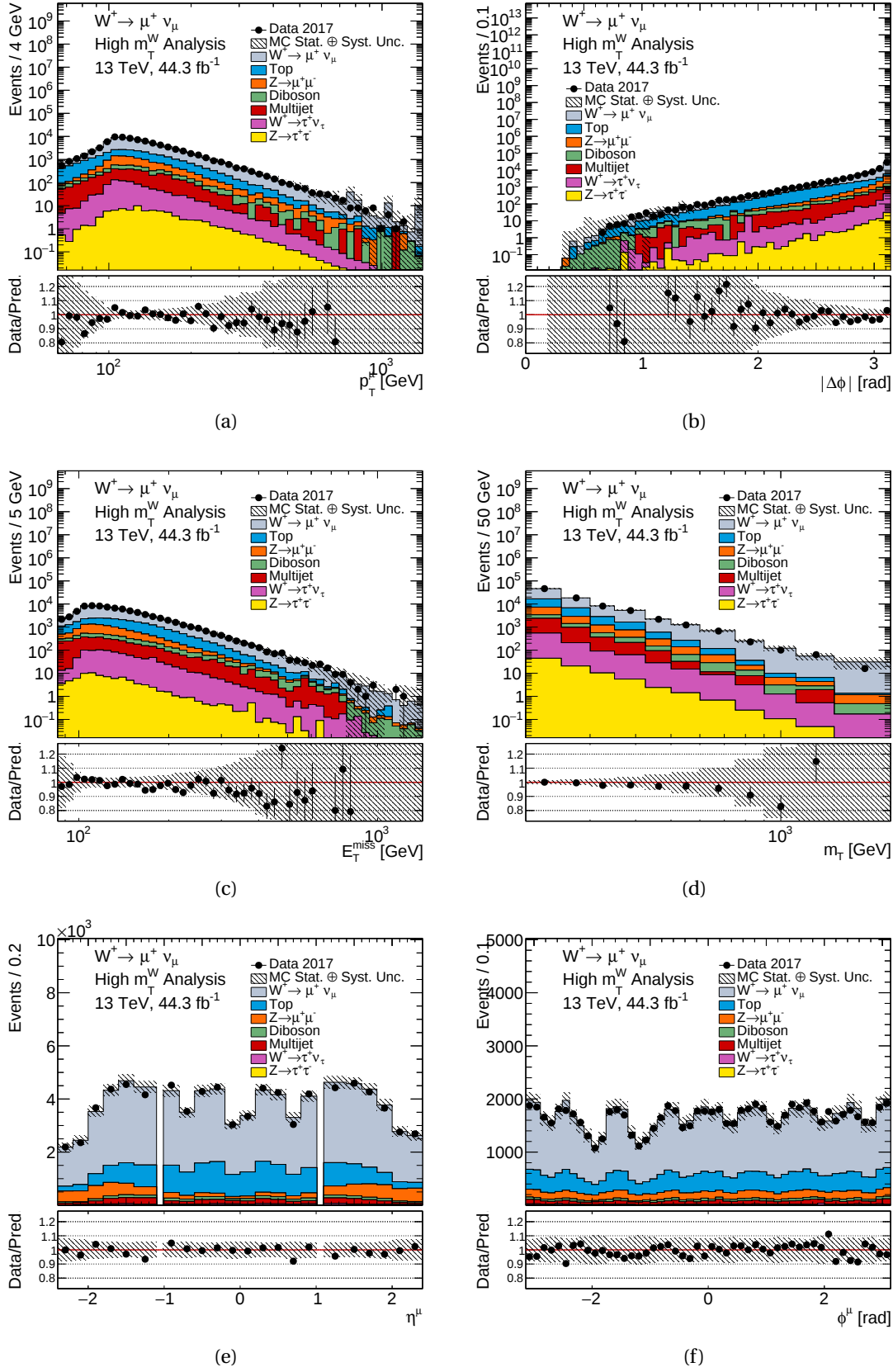
Figure E.9.: MC16d W^+ \rightarrow \mu^+ \nu control distributions for p_T^\mu , |\Delta\phi| , E_T^{\text{miss}} , m_T , \eta^\mu and \phi^\mu . The data contribution is shown with black points, the signal and the background contributions with solid lines. In the shaded band, systematic experimental uncertainties have been combined with the MC statistical uncertainties. The data statistical uncertainties are shown on the data points. Luminosity uncertainties have not been included.
