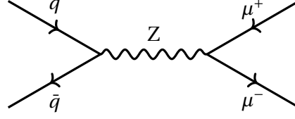
Figure 5.7.: Feynman diagram showing Z \rightarrow \mu\mu background.
