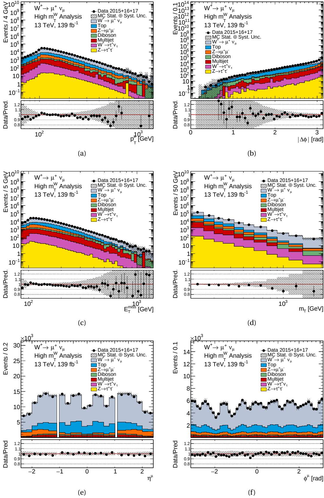
Figure 9.2.: W^+ \rightarrow \mu^+ \nu control distributions for p_T , |\Delta\phi| , E_T^{miss} , m_T , \eta^\mu and \phi^\mu . The data contribution is shown with black points, the signal and the background contributions with solid lines. In the shaded band, systematic experimental uncertainties have been combined with the MC statistical uncertainties. The statistical data uncertainties are shown on the data points. Luminosity uncertainties have not been included.
