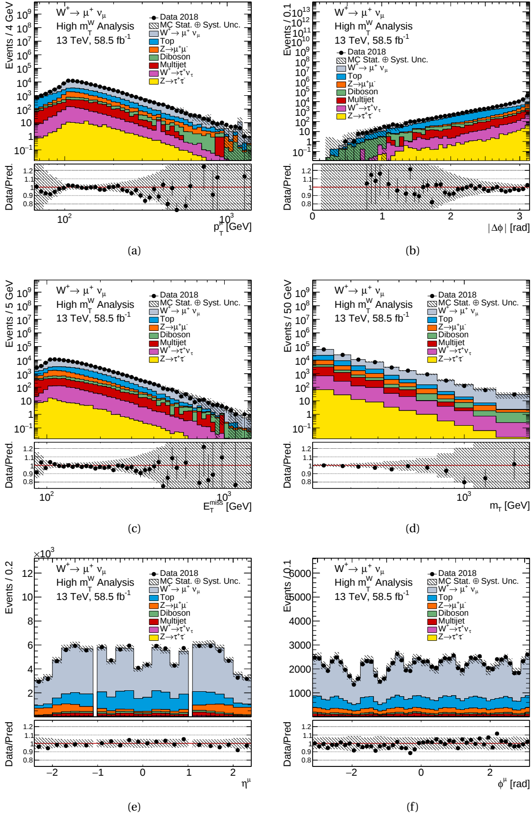
Figure E.16.: MC16e W^+ \rightarrow \mu^+ \nu control distributions for p_T^\mu , |\Delta\phi| , E_T^{\text{miss}} , m_T , \eta^\mu and \phi^\mu . The data contribution is shown with black points, the signal and the background contributions with solid lines. In the shaded band, systematic experimental uncertainties have been combined with the MC statistical uncertainties. The data statistical uncertainties are shown on the data points. Luminosity uncertainties have not been included.
