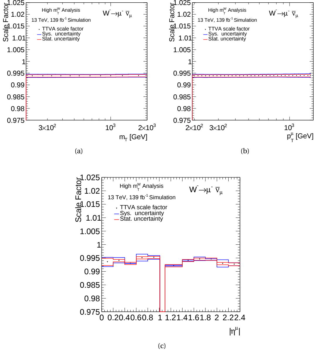
Figure B.4.: Scale Factor plots for average TTVA selection efficiency. These plots are for W^- \rightarrow \mu^- \bar{\nu} for the combination of Monte Carlo campaigns, MC16a, MC16d, MC16e. The plots show average isolation scale factors as a function of transverse mass m_T (a), p_T^\mu (b) and |\eta^\mu| (c). The individual systematics and statistical for one standard deviation are shown in blue and red.
