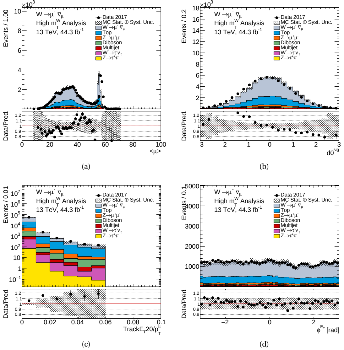
Figure E.12.: MC16d W^- \rightarrow \mu^- \bar{\nu}_\mu control distributions for \langle \mu \rangle , d0^{sig} , TrackE_T20/p_T^\mu and \phi^{E_T^{miss}} . The data contribution is shown with black points, the signal and the background contributions with solid lines. In the shaded band, systematic experimental uncertainties have been combined with the MC statistical uncertainties. The data statistical uncertainties are shown on the data points. Luminosity uncertainties have not been included.
