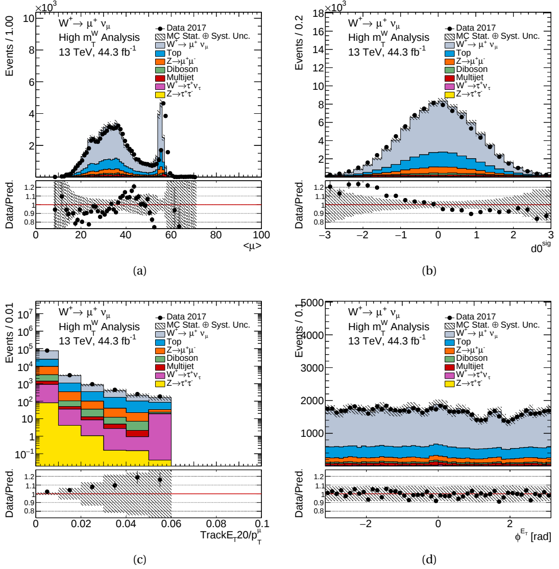
Figure E.10.: MC16d W^+ \rightarrow \mu^+ \nu control distributions for \langle \mu \rangle , d_0^{sig} , TrackE_T20/p_T^\mu and \phi^{E_T^{miss}} . The data contribution is shown with black points, the signal and the background contributions with solid lines. In the shaded band, systematic experimental uncertainties have been combined with the MC statistical uncertainties. The data statistical uncertainties are shown on the data points. Luminosity uncertainties have not been included.
