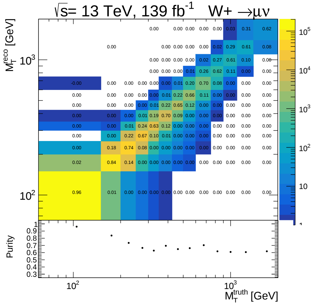
Figure 10.2.: Purity for the W^+ \rightarrow \mu^+ \nu signal process. The upper panel shows the m_T^W truth level vs the m_T^W reconstruction level events. The given numbers show the ratio of the number of events in each bin to the total number of reconstructed events in the given mass bin. The diagonal of the upper panel gives the purity in the lower panel.
