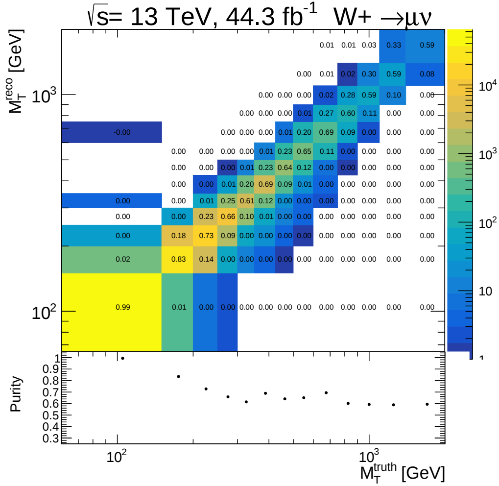
Figure E8.: Purity for the W^+ \rightarrow \mu^+ \nu MC16d signal process. The upper panel shows the m_T^W truth level vs the m_T^W reconstruction level events. The given numbers show the ratio of the number of events in each bin to the total number of reconstructed event in the given mass bin. The diagonal of the upper panel gives the purity in the lower panel.
