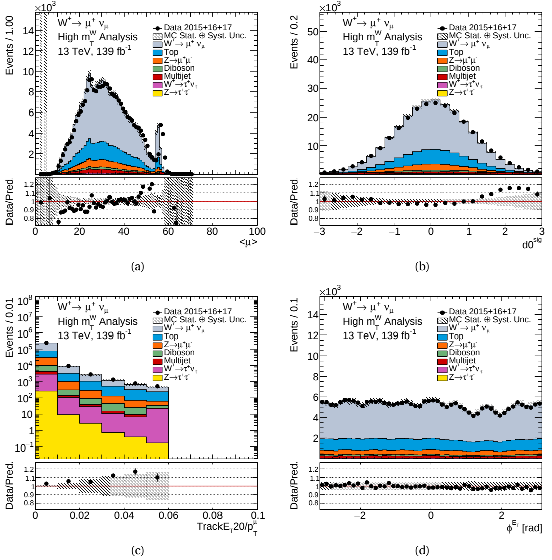
Figure 9.3.: W^+ \rightarrow \mu^+ \nu control distributions for \langle \mu \rangle , d_0^{sig} , TrackE_T20/p_T^\mu and \phi_{E_T}^{miss} . The data contribution is shown with black points, the signal and the background contributions with solid lines. In the shaded band, systematic experimental uncertainties have been combined with the MC statistical uncertainties. The statistical data uncertainties are shown on the data points. Luminosity uncertainties have not been included.
