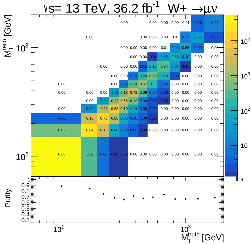
Figure E2.: Purity for the W^+ \rightarrow \mu^+ \nu MC16a signal process. The upper panel shows the m_T^W truth level vs the m_T^W reconstruction level events. The given numbers show the ratio of the number of events in each bin to the total number of reconstructed event in the given mass bin. The diagonal of the upper panel gives the purity in the lower panel.
