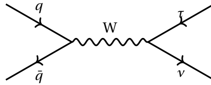
Figure 5.8.: Feynman diagram showing W \rightarrow \tau\nu background.
