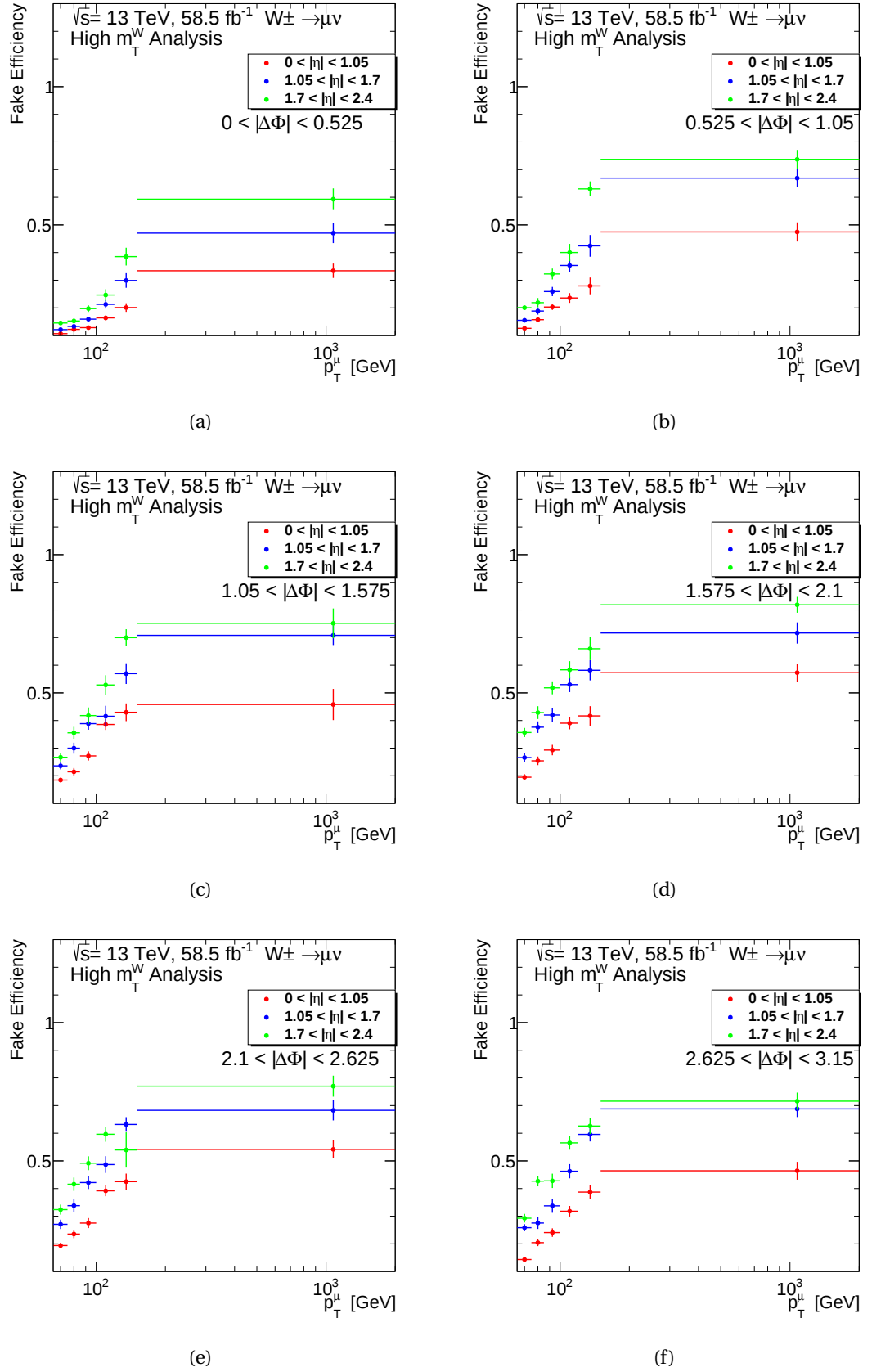
Figure 7.2.: Fake muon efficiency for calculating the matrix method for MC16e. The fake efficiency has been binned three dimensionally in p_T , |\eta| and \Delta\Phi(\mu, E_T^{\text{miss}}) . Each figure shows a different \Delta\Phi(\mu, E_T^{\text{miss}}) region. The red line shows the 0 < |\eta| < 1.05 , the blue line shows the 1.05 < |\eta| < 1.7 and the green line the 1.7 < |\eta| < 2.4 .
