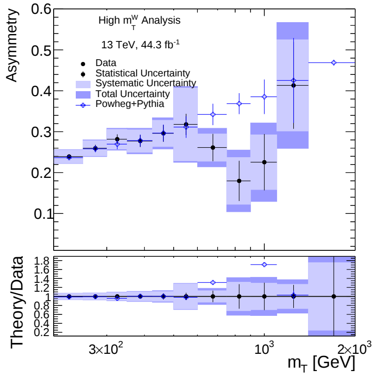
Figure E31.: Muon charge asymmetry binned in m_T^W for 2017 data and MC16d calculated using Equation 10.2. Statistical and systematic uncertainties are included in the uncertainty band. Statistical and systematic uncertainties are included in the uncertainty band. The total uncertainty is shown by the dark blue band. The ratio is taken between the measured data and the truth (prediction) distributions.
