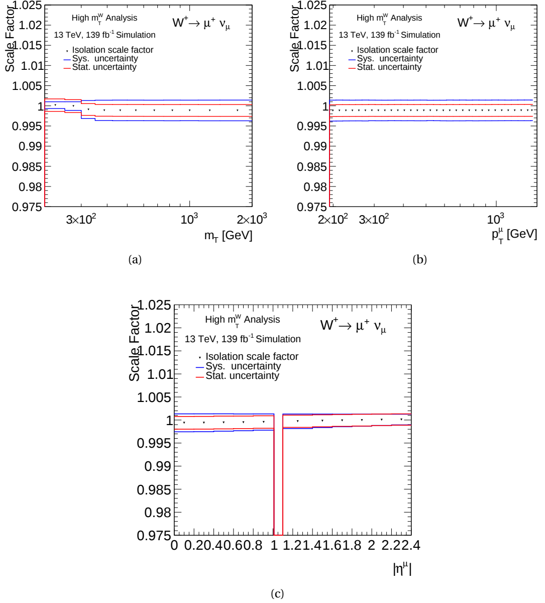
Figure 6.3.: Average isolation selection efficiency scale factors as a function of transverse mass m_T^W (a), p_T^\mu (b) and |\eta^\mu| (c). These plots are for W^+ \rightarrow \mu\nu for the combined Monte Carlo campaigns MC16a, MC16d, MC16e. The individual systematics and statistical uncertainty for one standard deviation are shown in blue and red.
