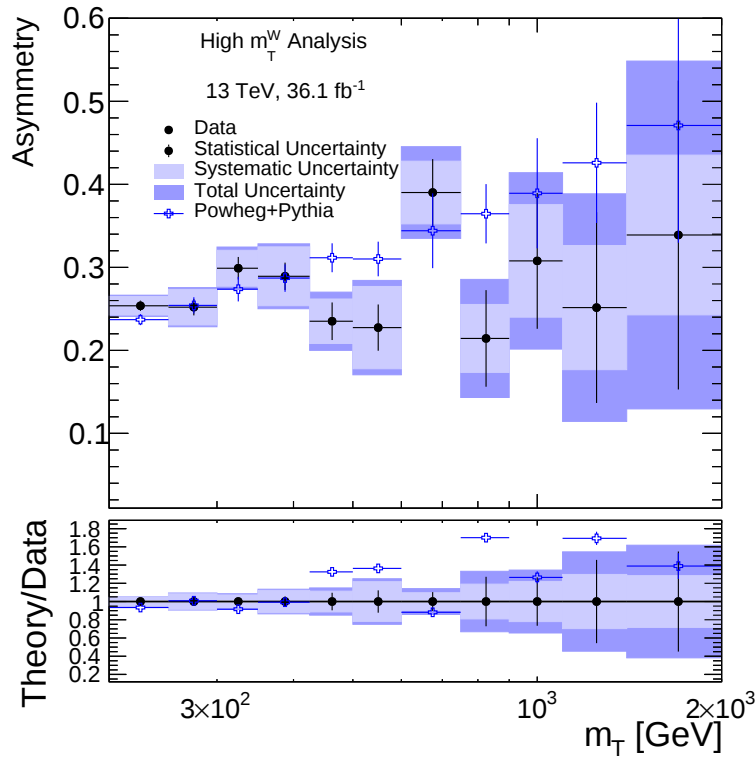
Figure E29.: Muon charge asymmetry binned in m_T^W for 2015/2016 data and MC16a calculated using Equation 10.2. Statistical and systematic uncertainties are included in the uncertainty band. Statistical and systematic uncertainties are included in the uncertainty band. The total uncertainty is shown by the dark blue band. The ratio is taken between the measured data and the truth (prediction) distributions.
