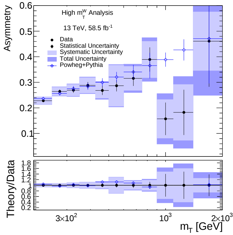
Figure E33.: Muon charge asymmetry binned in m_T^W for 2018 data and MC16e calculated using Equation 10.2. Statistical and systematic uncertainties are included in the uncertainty band. Statistical and systematic uncertainties are included in the uncertainty band. The total uncertainty is shown by the dark blue band. The ratio is taken between the measured data and the truth (prediction) distributions.
