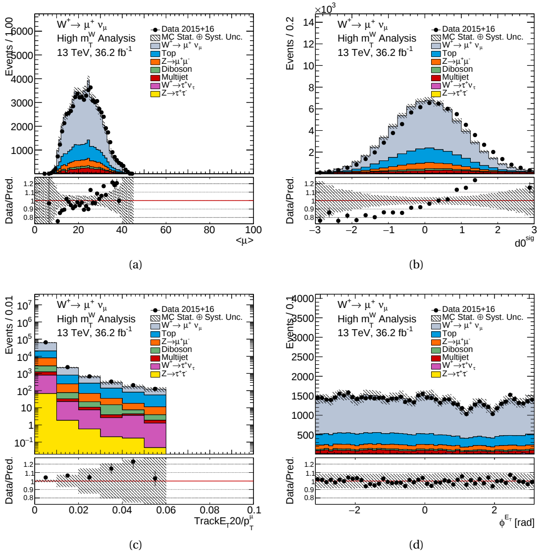
Figure E.3.: MC16a W^+ \rightarrow \mu^+ \nu control distributions for \langle \mu \rangle , d_0^{sig} , TrackE_T20/p_T^\mu and \phi^{E_T} . The data contribution is shown with black points, the signal and the background contributions with solid lines. In the shaded band, systematic experimental uncertainties have been combined with the MC statistical uncertainties. The data statistical uncertainties are shown on the data points. Luminosity uncertainties have not been included.
