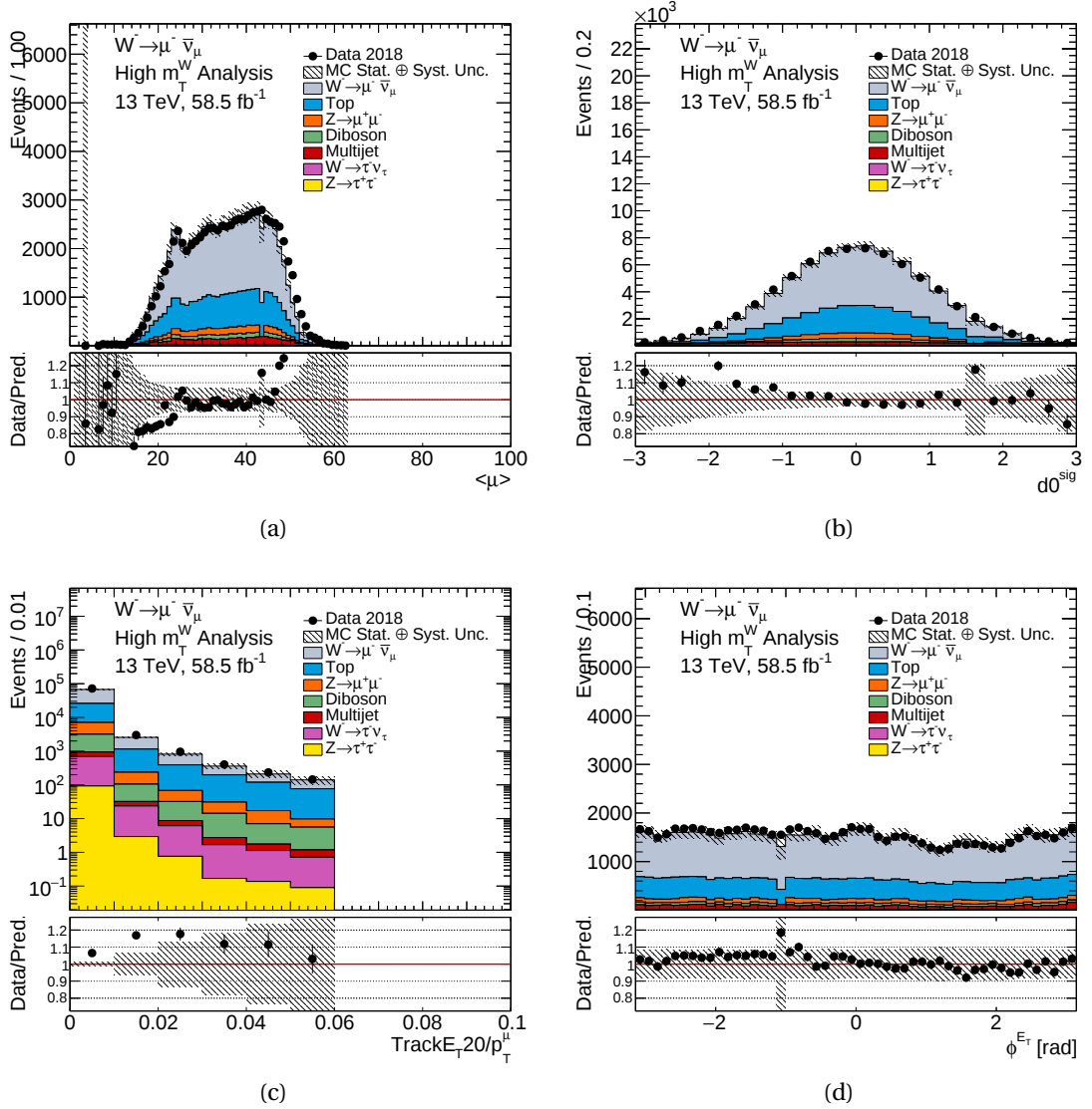
Figure E.19.: MC16e W^- \rightarrow \mu^- \bar{\nu}_\mu control distributions for \langle \mu \rangle , d0^{sig} , TrackE_T20/p_T^\mu and \phi_{E_T}^{miss} . The data contribution is shown with black points, the signal and the background contributions with solid lines. In the shaded band, systematic experimental uncertainties have been combined with the MC statistical uncertainties. The data statistical uncertainties are shown on the data points. Luminosity uncertainties have not been included.
