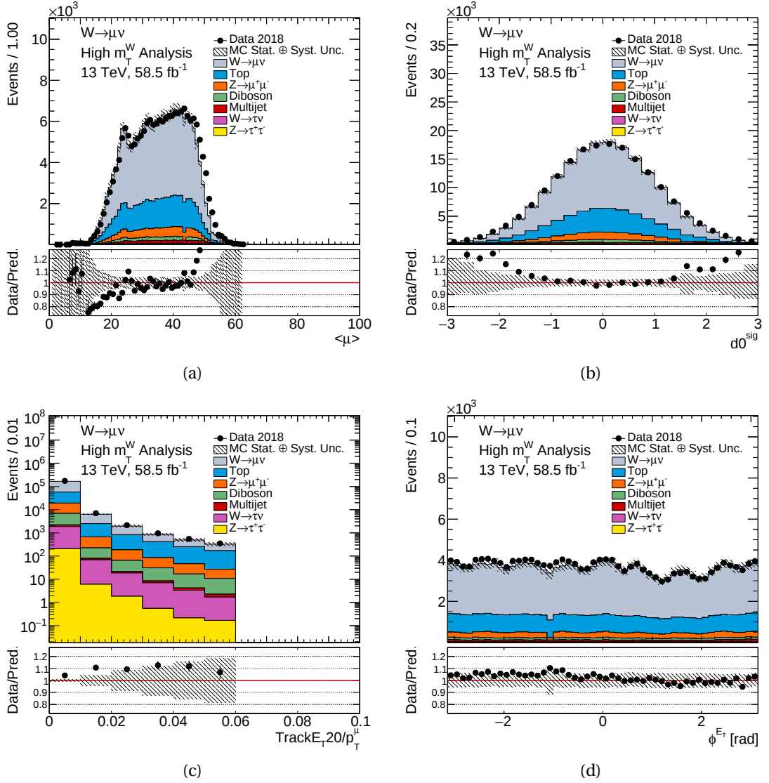
Figure E.21.: MC16e combined charge W^\pm \rightarrow \mu\nu control distributions for \langle \mu \rangle , d0^{sig} , TrackE_T20/p_T^\mu and \phi_{E_T}^{miss} . The data contribution is shown with black points, the signal and the background contributions with solid lines. In the shaded band, systematic experimental uncertainties have been combined with the MC statistical uncertainties. The data statistical uncertainties are shown on the data points. Luminosity uncertainties have not been included.
