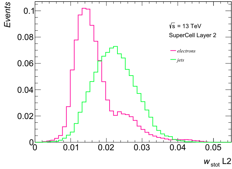
Figure 4.8.: Normalised distribution of w_{tot} in Layer 2. The Z \rightarrow ee sample is shown in pink and the dijet sample in green.
