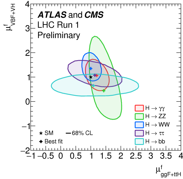
Figure 1.22: Likelihood contours in the (\mu_{ggF+ttH}, \mu_{VBF+VH}) plane for the combination of ATLAS and CMS, shown for the five decay channels: H \rightarrow ZZ, WW, \gamma\gamma, \tau\tau, bb . The results are shown as 68% CL contours, together with the most probable values of the data and the SM expectation.
