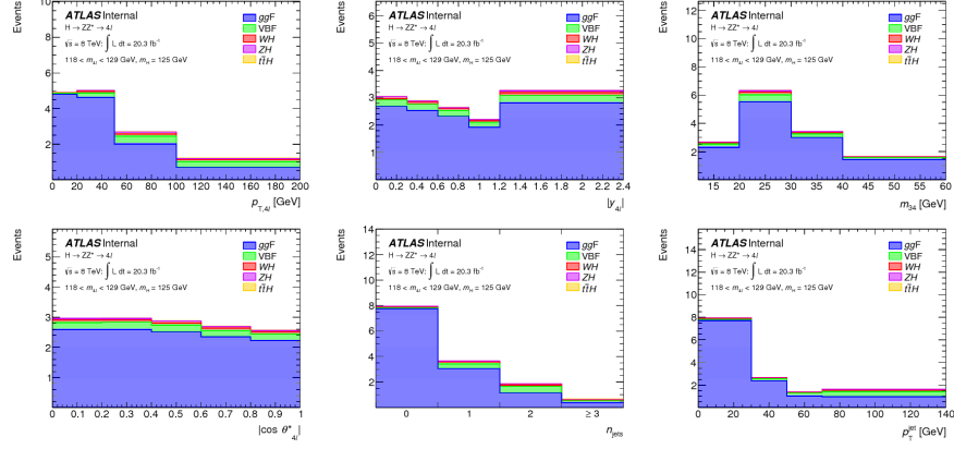
Figure 4.17: Expected number of reconstructed signal events within the mass window [118, 129] GeV in all variables of interest assuming a SM Higgs with m_H = 125 GeV. The five production modes are plotted separately, with ggH as the dominant production mode.
