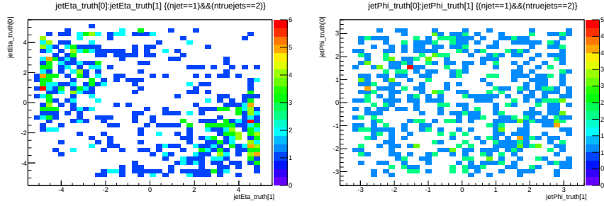
Figure 5.16: Truth studies in the 1jet category for the VBF events. The \eta and \phi of subleading jet versus the leading jet 2D distributions are reported.
