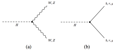
Figure 1.14: Examples of leading-order Feynman diagrams for Higgs boson decays (a) to W and Z bosons and (b) to fermions.
