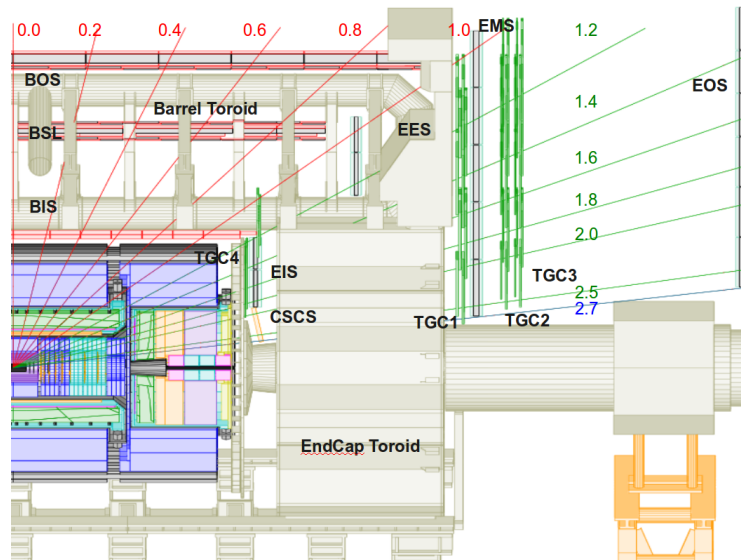
Figure 2.14: Trasversal section of the Muon Spectrometer: dotted lines demonstrate how the Extra Endcap chambers provide an extra layer of detection for some particle trajectories and an \eta coverage up to 2.7.
