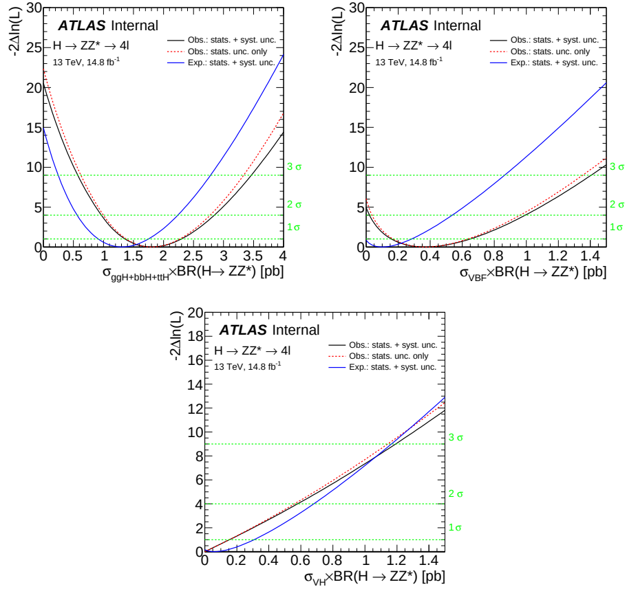
Figure 5.35: NLL scan results for L_{\text{int}} = 14.8 \text{ fb}^{-1} of \sqrt{s} = 13 \text{ TeV} data.
