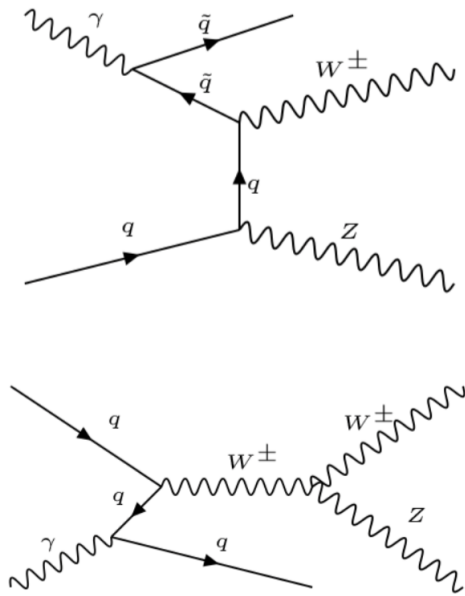
Figure 4.11: Examples of diagrams for the \gamma -induced processes in pp \rightarrow WZ + X [155].
