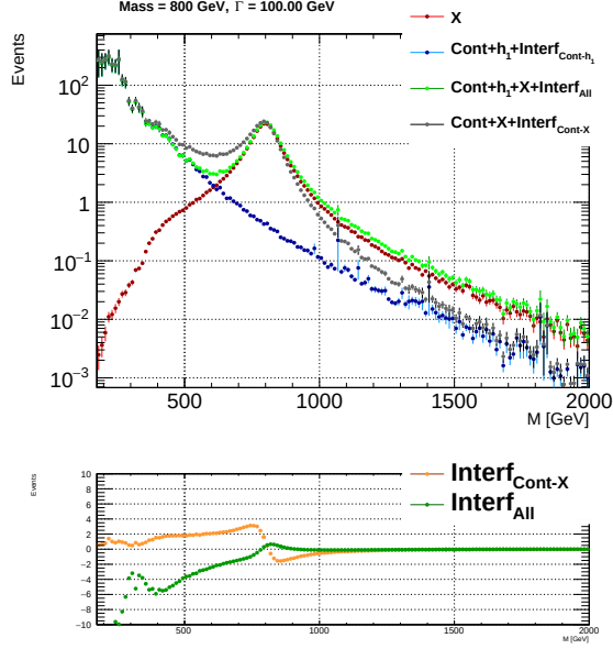
Figure 4.3: Mass spectrum of ZZ \rightarrow 2l2\nu final state considering a mass of 800 GeV and width hypothesis of 100 GeV in gluon fusion mechanism. The red dots represent the heavy scalar boson (X), the blue shape ( |ZZ \rightarrow 2l2\nu + h_1 \rightarrow ZZ \rightarrow 2l2\nu|^2 ), the light green dots represent the full amplitude considering also the contribution of the heavy boson, and finally the grey distribution ( |ZZ \rightarrow 2l2\nu + X \rightarrow ZZ \rightarrow 2l2\nu|^2 ). The interference shapes are reported in the bottom plot in the case the SM higgs is neglected (orange distribution) or not (green distribution).
