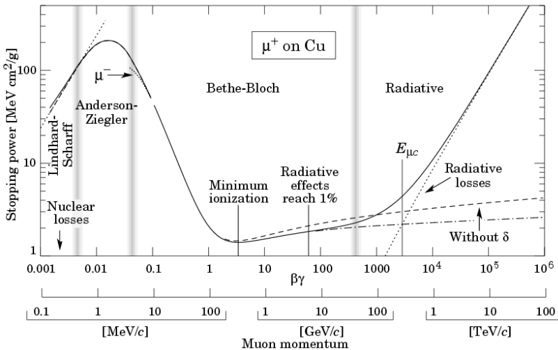
Figure 5.1: Stopping power for muon in copper as a function of its momentum [178].
