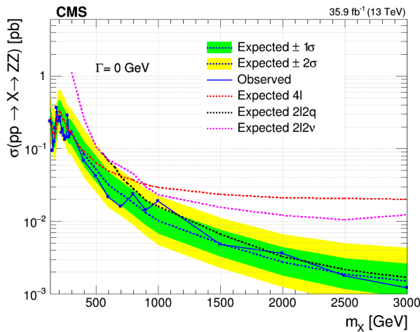
Figure 5.43: Combined limits on the Cross Section for a generic scalar boson with width of 0 GeV in ZZ channel. The results merged all the expected limits in each sub-channel [20].
