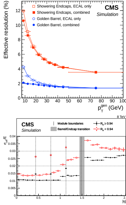
Figure 3.7: ( top ) Resolution in electron momentum after combining the E_{SC} and p estimates (solid symbols), compared to that of the SC energy only (open symbols), as a function of the electron p_T . The circles points represent all the electrons in the barrel not affected by bremsstrahlung, whereas the squares points show the electron resolution in the case of tight radiative losses. Electrons are generated with uniform distributions in \eta and p_T [112]. ( bottom ) Relative energy resolution, \sigma_{eff}/E , as a function of |\eta| , in simulated H \rightarrow \gamma\gamma events, for photons with R_9 \geq 0.94 (solid circles) and photons with R_9 < 0.94 (open squares). The vertical dashed lines mark the module boundaries in the barrel, and the vertical grey band indicates the range of |\eta| , around the barrel/endcap transition, removed from the fiducial region [115].
