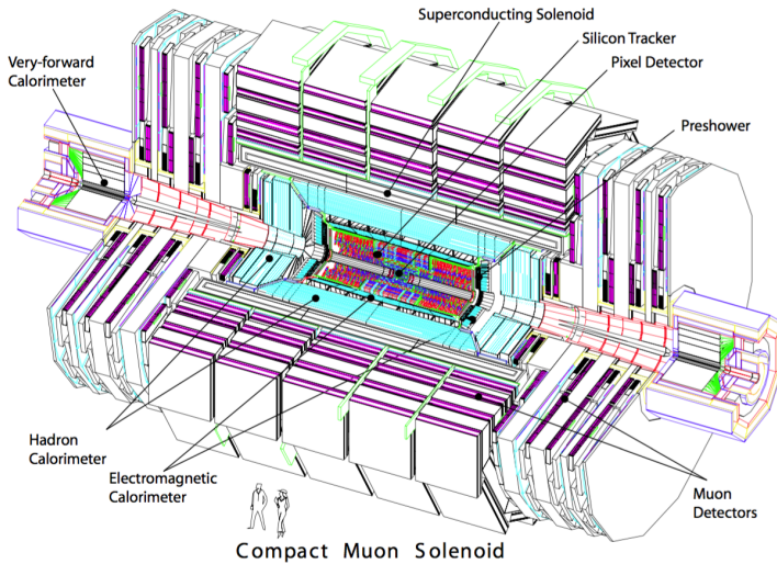
Figure 2.5: Tridimensional view of the CMS detector [19].
