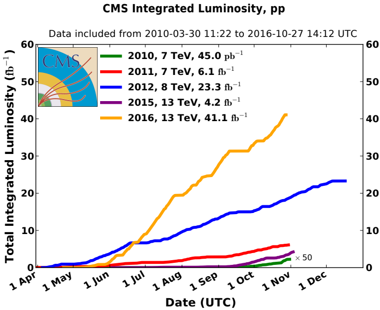
Figure 2.3: Comparison of the luminosity delivered by the LHC during the different years of data taking until 2016 [97].
