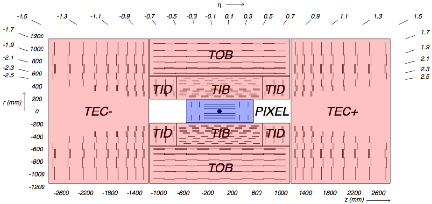
Figure 2.8: View of the inner tracking system. The violet part shows the pixel detector, instead the pink region the strip modules [100].
