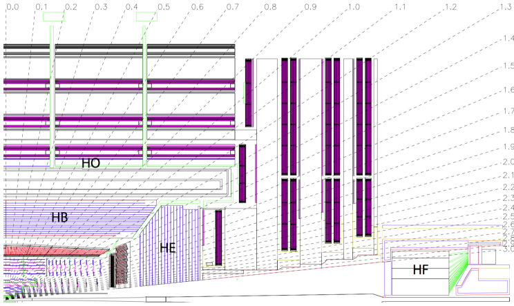
Figure 2.10: Longitudinal profile of CMS detector. In the picture the different components of the hadronic calorimeter are highlighted [19].
