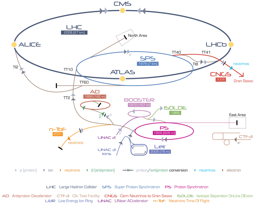
Figure 2.2: Schematic view of the CERN accelerator complex [96].
