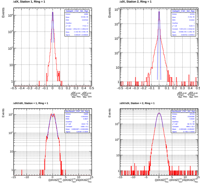
Figure 5.38: Resolution and pull distribution for the dx/dz direction of the reconstructed segments associated to muons generated with nominal momentum of 2 TeV. The results refer to the chambers of the first ring within the first (left) and the second (right) station of the endcap. The Gaussian fit is performed in the region defined by Mean \pm 2 \cdot RMS .
