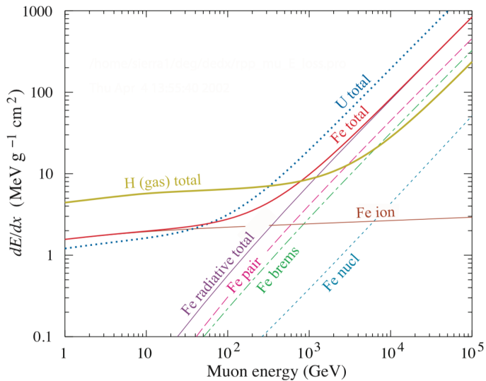
Figure 5.3: The average energy loss of a muon in hydrogen, iron, and uranium as a function of muon energy [178].
