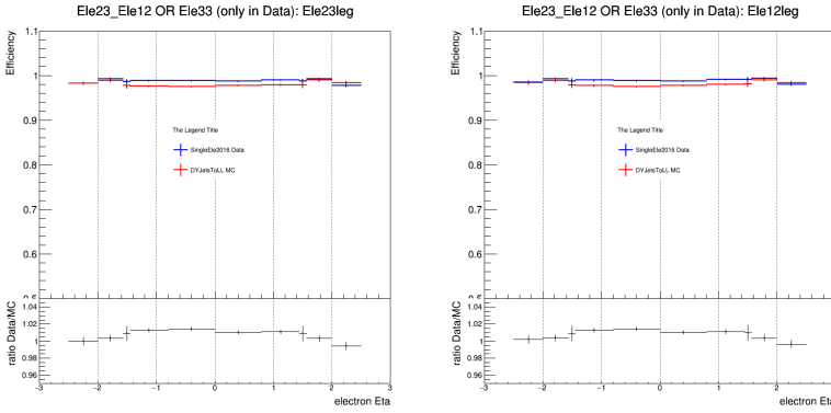
Figure 4.8: Di-electron trigger efficiency measured in data and MC as function of the electron pseudorapidity with p_T > 25 GeV. The left (right) plot corresponds to the leading (sub-leading) electron.
