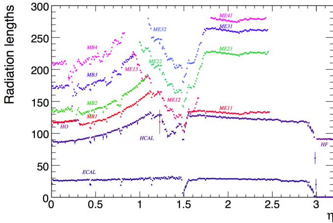
Figure 5.6: Material thickness in radiation lengths after the ECAL, HCAL, and at the depth of each muon station as a function of pseudorapidity [99].
