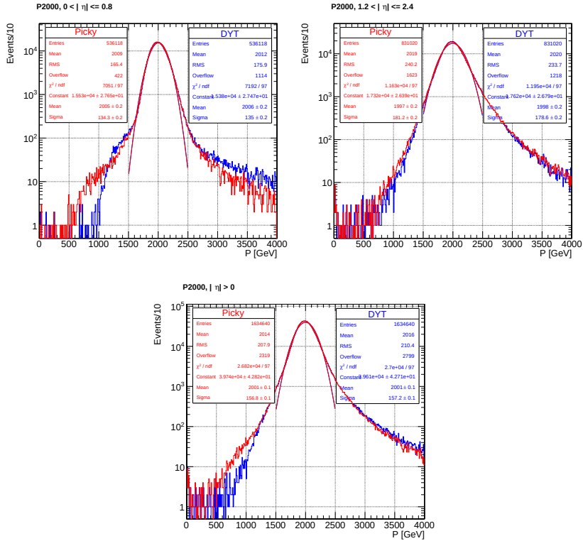
Figure 5.13: Comparison of the muon reconstructed momentum obtained by the DYT algorithm and the Picky algorithm using a sample of muons generated with the Particle Muon Gun [182]. The muons are generated in the full acceptance region of the CMS detector ( \eta \in [-2.5, 2.5] and \phi \in [-3.14, 3.14] ), requiring a momentum defined by the interval 2 \text{ TeV} \pm 0.01\% . Three different regions in \eta are reported: the barrel region ( Top left ), the endcap region ( Top right ) and finally the entire \eta region ( Bottom ). The Gaussian fit is performed in the region defined by p_{sim} \pm 25\% .
