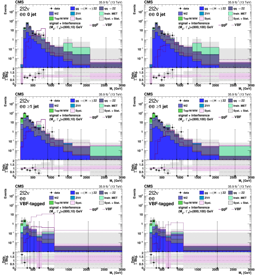
Figure 4.25: Transverse mass distributions in the different jet bins category after the final E_T^{miss} cut of 125 GeV in ee channel. The signal distribution corresponds to a mass point of 800 GeV. Two width hypothesis are reported: 10 GeV (left) and 100 GeV (right) both in ggF and VBF. In each distribution both systematic and statistical errors are represented. The distribution on the bottom of the transverse mass reports the discrepancies between the data and the total background.
