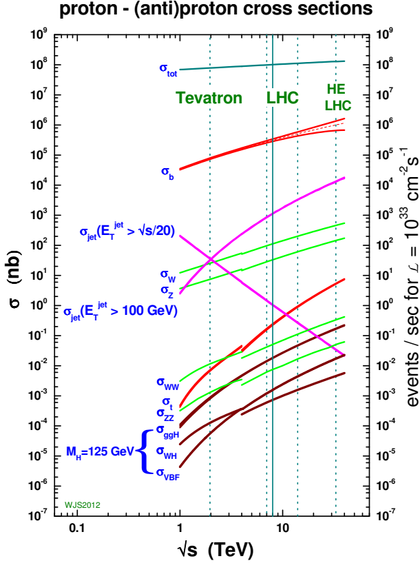
Figure 2.1: Production cross sections and corresponding event rates for different processes reported as a function of the center-of-mass energy \sqrt{s} [55].
