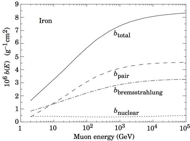
Figure 5.2: Contributions to the fractional energy loss by muons in iron due to electron-positron pair production, bremsstrahlung, and photonuclear interactions as a function of the muon energy [178].
