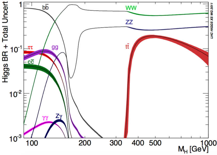
Figure 1.12: The different branching ratios for a heavy scalar boson SM-like as function of its mass from 90 GeV up to 1 TeV [75].
