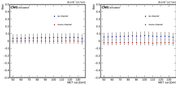
Figure 4.16: Closure test for different E_T^{miss} requirements. The distributions are reported for both the sideband region (left) and the up sideband region (right) requiring the presence of at least a b jet in the event.
