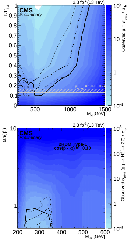
Figure 1.16: Limits set in ZZ \rightarrow 2l2\nu in EWS ( top ) and 2HDM (Type-I) ( bottom ) [52].
