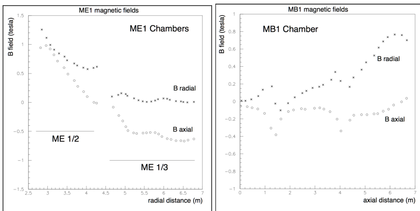
Figure 2.12: Axial and radial components of the magnetic field in the ME1 ( left ) and in the MB1( right ) stations . [99].
