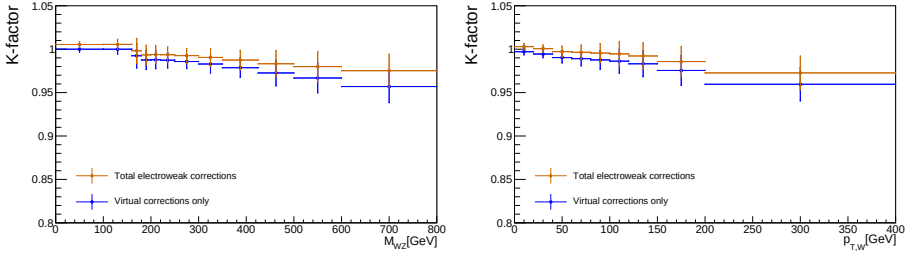
Figure 4.13: Evolution of the NLO electroweak corrections K-factor on pp \rightarrow W^+Z as a function of m_{WZ} (left) and p_{T,W} (right), using only virtual corrections (blue) or using both virtual and photon-induced corrections (brown) [155].
