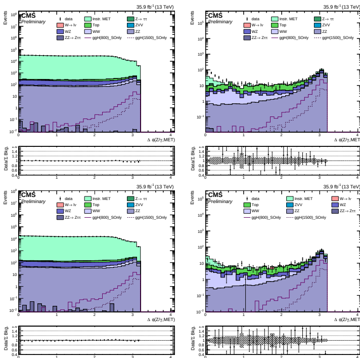
Figure 4.20: |\Delta\phi(Z, E_T^{miss})| variable in di-muon channel ( top ) and di-electron channel ( bottom ) for E_T^{miss} > 0 GeV ( left ) and greater than 125 ( right ). In both the cases the events used in both the distributions have passed all the pre-selection requirements up to the |\Delta\phi(jet, E_T^{miss})| cut.
