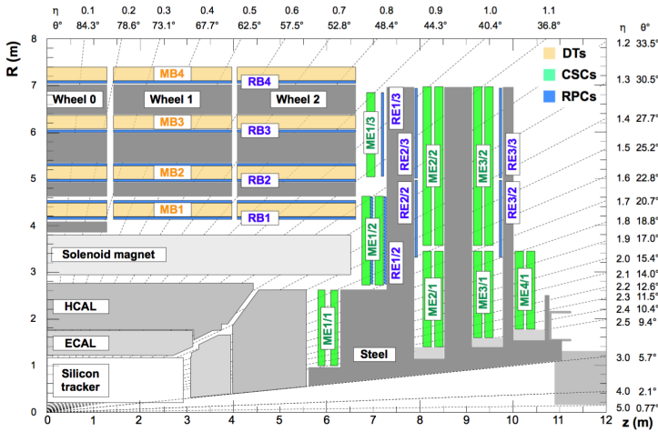
Figure 2.11: Muon Spectrometer profile. The dashed lines correspond to fixed \eta values. The DTs are in orange, the CSC in green, and finally the RPC in blue [101].
