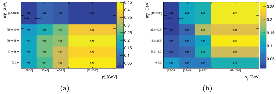
Figure 8.17: Fake efficiencies estimated by requirement on the number of jets n_{\text{jets}} \geq 1 . The 2D histograms show the impact on each bin, with the numbers representing the relative uncertainty compared to the nominal value for the electron channel (a), and for the muon channel (b).
