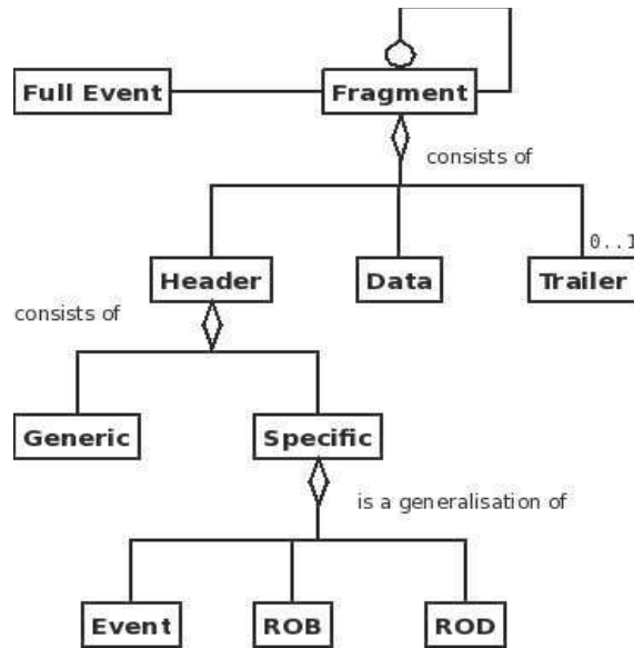
Figure 4.4: Class diagram of the event format. The event data is organized into fragments, which are the basic units of data transfer and storage. Each fragment contains a header, data and trailer. The header has generic and specific parts. The specific part is a generalization of different types of fragments [55].
