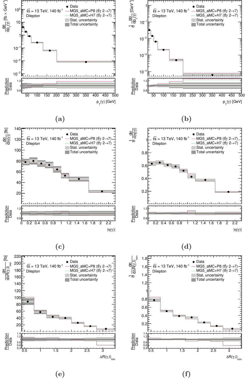
Figure 11.21: Absolute (left) and normalized (right) differential cross-sections of total t\bar{t}\gamma production and decay in the dilepton fiducial phase space at particle level as a function of p_T(\gamma) (a, b), |\eta(\gamma)| (c, d), \Delta R(\gamma, \ell)_{\min} (e, f). Data are compared with LO 2 \rightarrow 7 MADGRAPH5_AMC@NLO simulation interfaced with PYTHIA 8 and HERWIG 7. The last bin includes overflow events.
