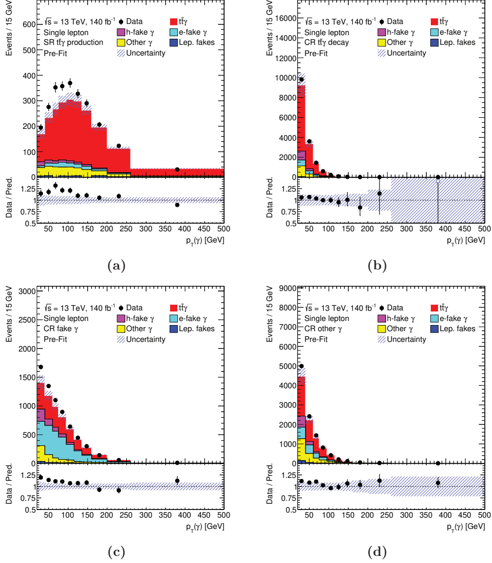
Figure A.17: Distribution of p_T(\gamma) in the single-lepton channel for the four regions at the reconstruction level: (a) tt\gamma production SR, (b) tt\gamma decay CR, (c) fakes CR, and (d) prompt photon CR. The last bin includes overflow events. The lower panel shows the ratio of the data to the predictions. The error bars represent the statistical uncertainty in the data. The shaded area represents the total uncertainty in the prediction.
