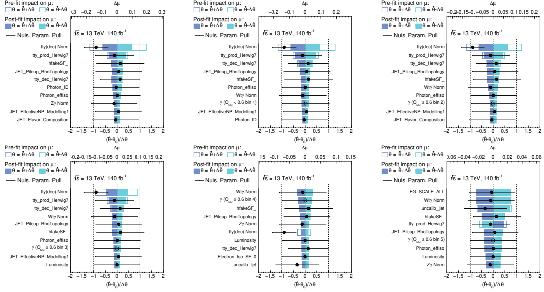
Figure 11.18: The ranking of systematic uncertainties included in the profile likelihood unfolding used for the p_T(\gamma) cross-section measurement in dilepton channel is shown. The blue and turquoise bands represent the post-fit impact on the fit result, while the outlined blue and turquoise rectangles show the pre-fit impact. The difference between these two indicates the constraint of the nuisance parameter due to correlations in the fit. Most nuisance parameters are either unconstrained or only marginally constrained. The impact is overlaid with the post-fit values of the nuisance parameters (pulls), shown by the black dots. The black lines represent the post-fit uncertainties normalized to the pre-fit uncertainties. Each subfigure, corresponds to a specific bin of the p_T(\gamma) distribution, starting from bin 1 till bin 6 (from left to right and top to bottom).
