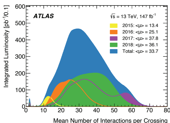
Figure 6.1: The distribution of the average number of interactions per bunch crossing in the data-taking period during LHC Run2 operation [65].
