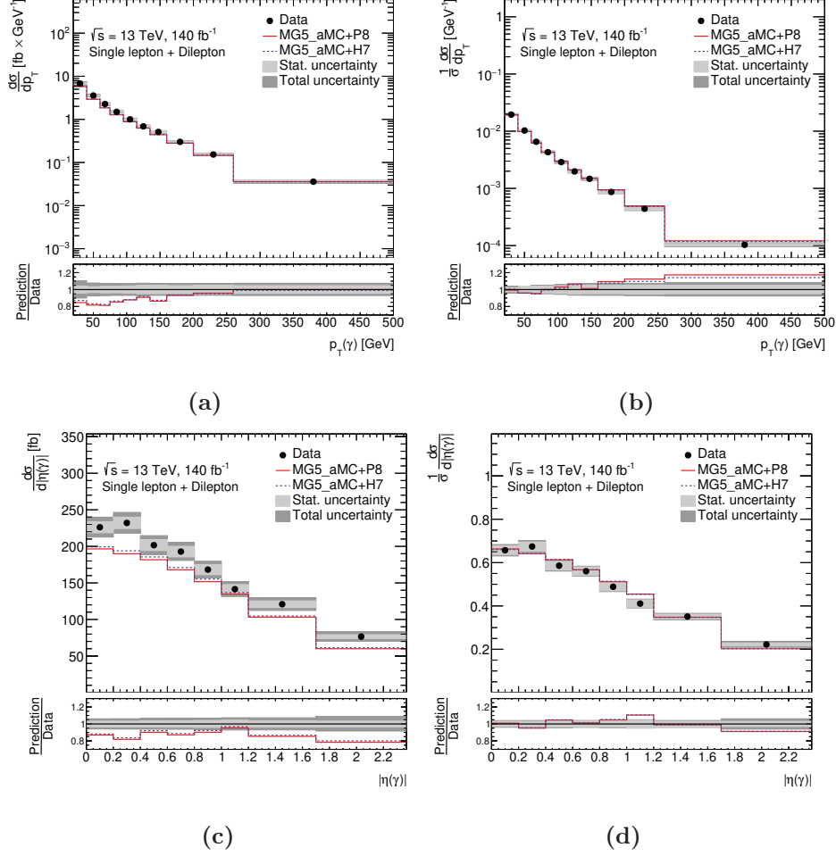
Figure 11.12: Absolute (left) and normalized (right) differential cross-section for the t\bar{t}\gamma production measured in a combined single-lepton and dilepton fiducial phase space as a function of the photon p_T (a, b), and photon |\eta| (c, d). Data are compared with the MadGraph5_aMC@NLO simulation interfaced with PYTHIA 8 and HERWIG 7. The lower parts of each plot show the ratio of the prediction to the data. The last bin includes the overflow events.
