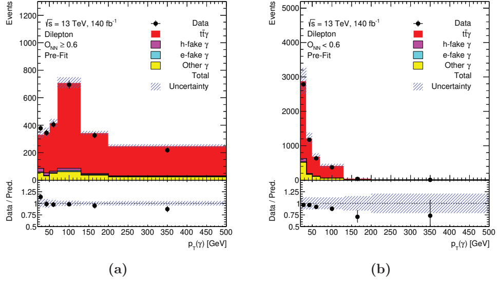
Figure A.18: Distribution of p_T(\gamma) in the dilepton channel for the two regions at the reconstruction level, O_{NN} \geq 0.6 and O_{NN} < 0.6 . The last bin includes overflow events. The lower panel shows the ratio of the data to the predictions. The error bars represent the statistical uncertainty in the data. The shaded area represents the total uncertainty in the prediction. The last bin includes overflow events.
