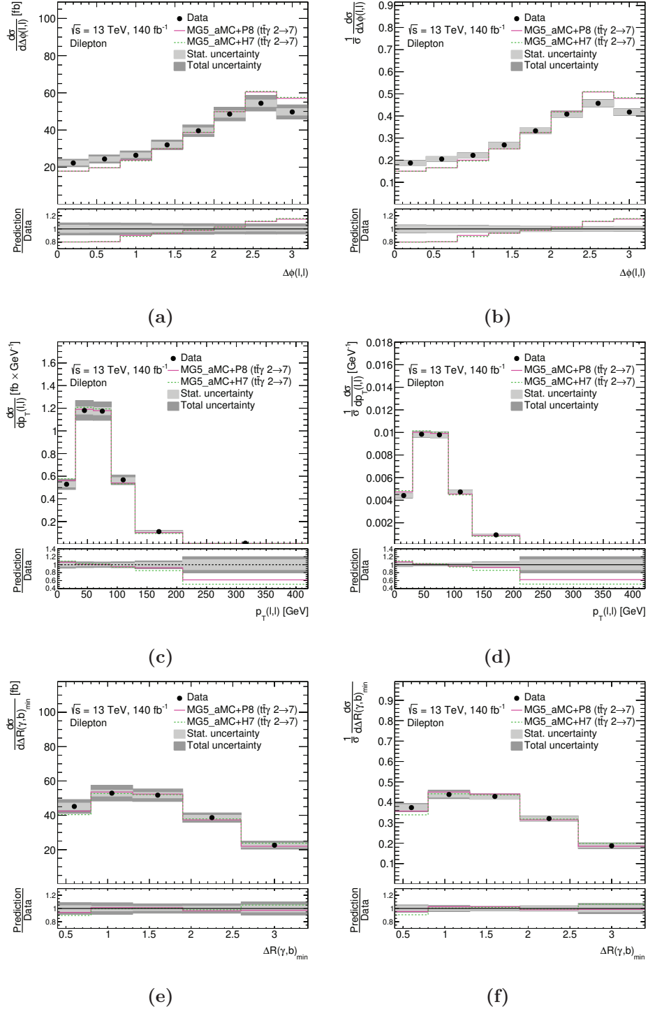
Figure A.21: Absolute (left) and normalized (right) differential cross-sections of total t\bar{t}\gamma production and decay in the dilepton fiducial phase space at particle level as a function of |\Delta\phi(\ell, \ell)| (a, b), p_T(\ell, \ell) (c, d), and \Delta R(\gamma, b)_{\min} (e, f). Data are compared with LO 2 \rightarrow 7 MADGRAPH5_AMC@NLO simulation interfaced with PYTHIA 8 and HERWIG 7. The last bin includes overflow events.
