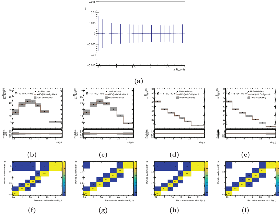
Figure A.3: (a) Resolution of the photon \Delta R_{\min}(\gamma, \ell) observable is represented by the error bars. The y-axis is the mean of the distribution of the difference between the \Delta R(\gamma, \ell)_{\min} at reconstruction and truth level, and the error bars represent one standard deviation around that mean. Unfolded results with the tested binning (b) and final binning (c) for t\bar{t}\gamma production measurement, and unfolded results with the tested (d) and final (e) binning for total t\bar{t}\gamma measurement, The error bar in (b), (c), (d), (e) represents statistical uncertainty only. The error bar in (b), (c), (d), (e) represents statistical uncertainty only. Plots (f)- (i) represent the migration matrix in the SR for above cases.
