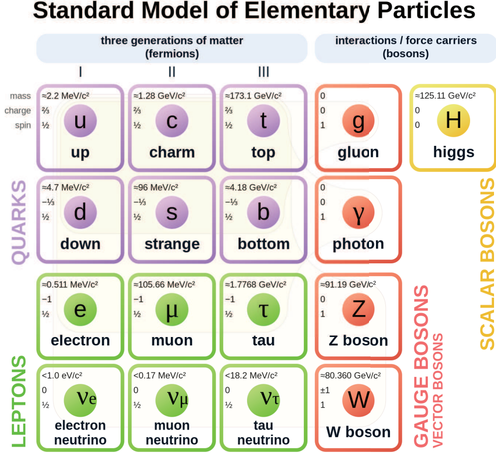
Figure 2.1: Elementary particles and force carriers of the Standard Model [1].
