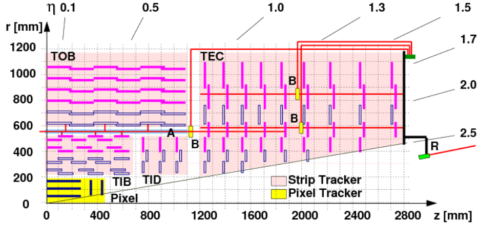
Figure 3.3: Layout of the CMS inner tracking system in an r - z view, showing the pixel detector and the silicon strip tracker.
