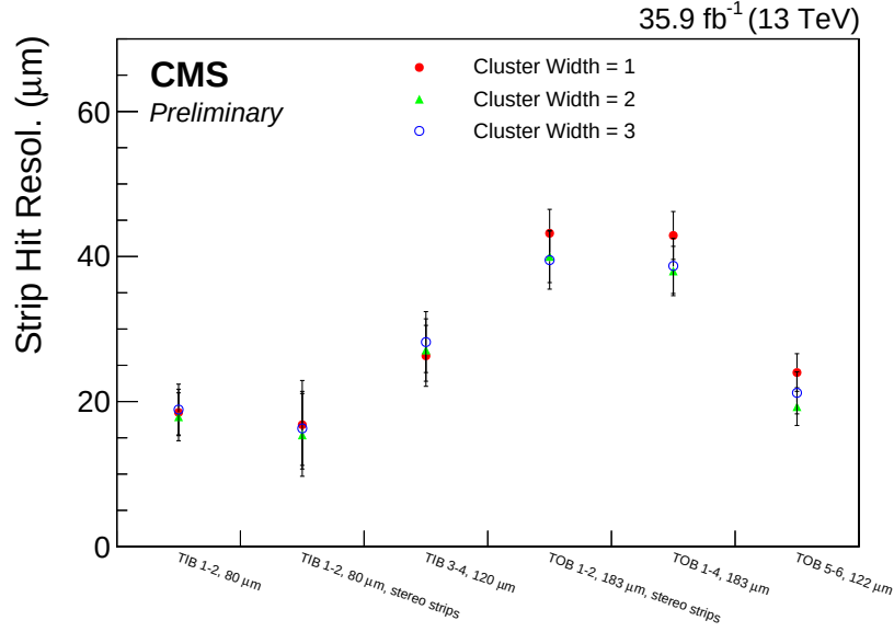
Figure 3.5: Strip Hit resolution for different cluster widths expressed in units of number of strips.
