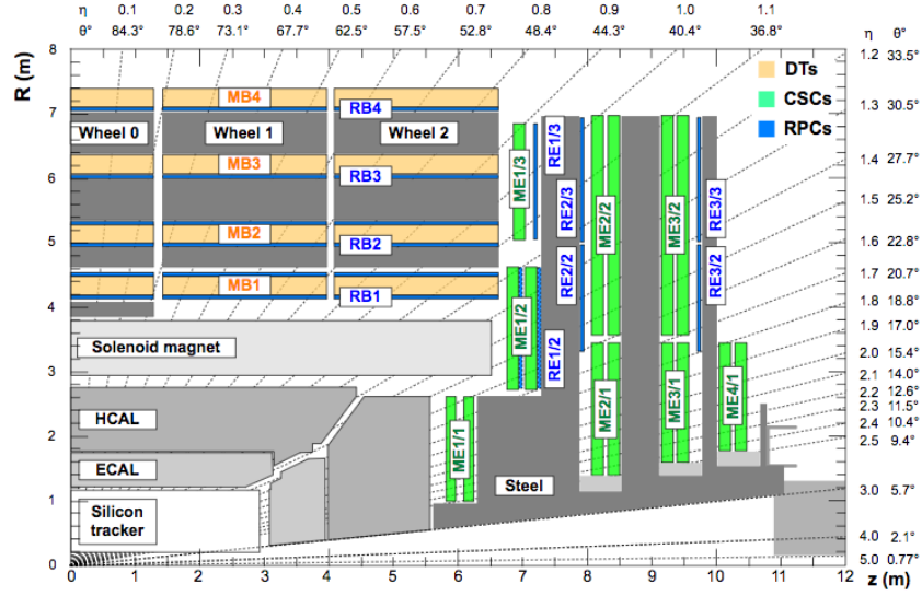
Figure 3.10: An R-z cross section of a quadrant of the CMS detector with the axis parallel to the beam ( z ) running horizontally and radius ( R ) increasing upward. The interaction point is at the lower left corner. Shown are the locations of the various muon stations and the steel disks (dark grey areas). The 4 drift tube (DT, in light orange) stations are labeled MB (muon barrel) and the cathode strip chambers (CSC, in green) are labeled ME (muon endcap). Resistive plate chambers (RPC, in blue) are in both the barrel and the endcaps of CMS, where they are labeled RB and RE, respectively.
