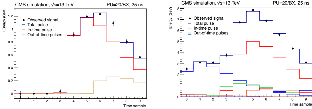
Figure 4.2: Examples of fitted pulses for signals in the EB (left) and in the EE (right) with 20 pileup interactions.
