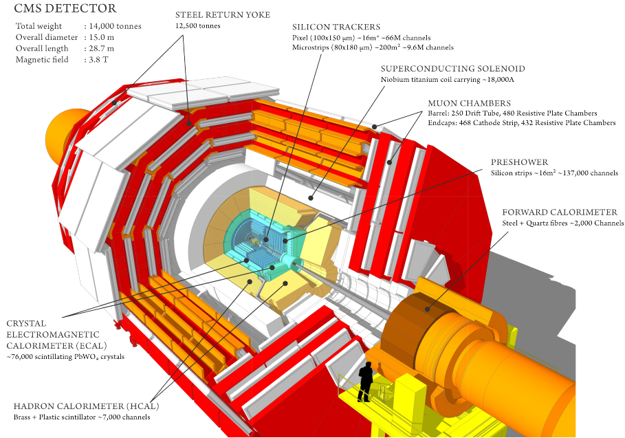
Figure 3.2: A perspective view of the CMS detector.
