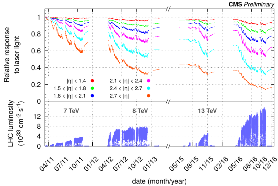
Figure 3.7: Evolution of the ECAL relative response as a function of data taking period.
