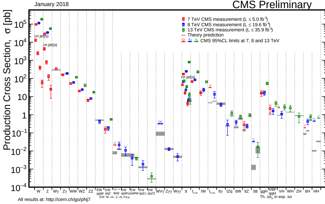
Figure 2.1: Compilation of different SM predictions compared to the corresponding CMS cross section measurements. Where the theory values appear to be absent they actually agree with the data within the experimental uncertainties.
