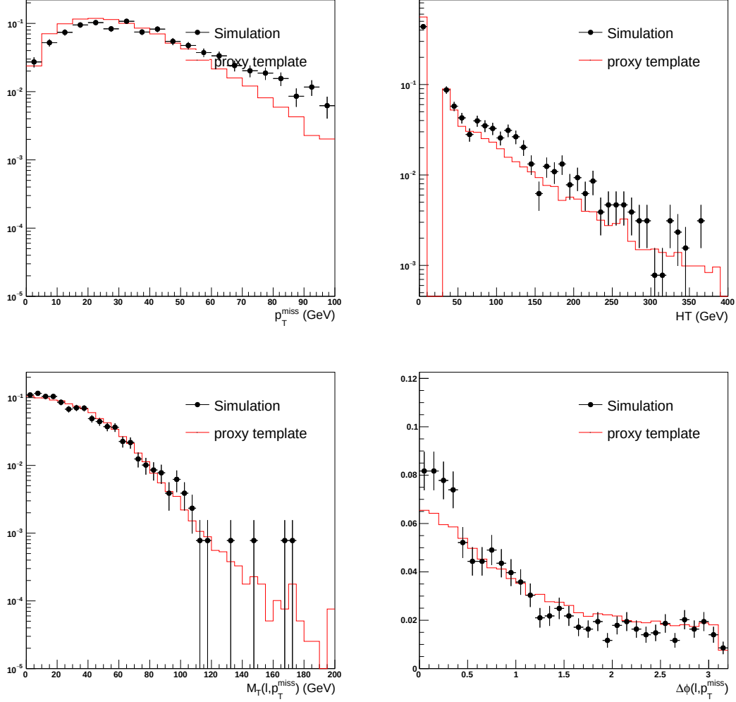
Figure 7.14: Comparison of various kinematic distributions between simulated QCD events with a fake muon and events in data with a control muon. The distributions are area-normalized to facilitate a comparison of their shapes.
