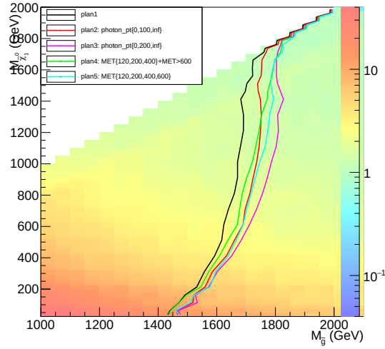
Figure 8.1: Optimization of the signal bins. Baseline binning (black): p_T^{\text{miss}}\{120\text{-}200, 200\text{-}400, > 400\}\text{GeV} \times H_T\{<100, 100\text{-}400, > 400\}\text{GeV} . Plan 2 (red): p_T^{\text{miss}}\{120\text{-}200, 200\text{-}400, > 400\}\text{GeV} \times H_T\{<100, 100\text{-}400, > 400\}\text{GeV} \times p_T^\gamma\{< 100, > 100\}\text{GeV} . Plan 3 (magenta): p_T^{\text{miss}}\{120\text{-}200, 200\text{-}400, > 400\}\text{GeV} \times H_T\{<100, 100\text{-}400, > 400\}\text{GeV} \times p_T^\gamma\{< 200, > 200\}\text{GeV} . Plan 4 (green): p_T^{\text{miss}}\{120\text{-}200, 200\text{-}400, 400\text{-}600\}\text{GeV} \times H_T\{<100, 100\text{-}400, > 400\}\text{GeV} + \{p_T^{\text{miss}} > 600\text{ GeV}\} . Plan 5 (cyan): p_T^{\text{miss}}\{120\text{-}200, 200\text{-}400, 400\text{-}600\}\text{GeV} \times H_T\{<100, 100\text{-}400, > 400\}\text{GeV} + \{p_T^{\text{miss}} > 600\text{ GeV}\} \times H_T\{< 400, > 400\}\text{GeV} .
