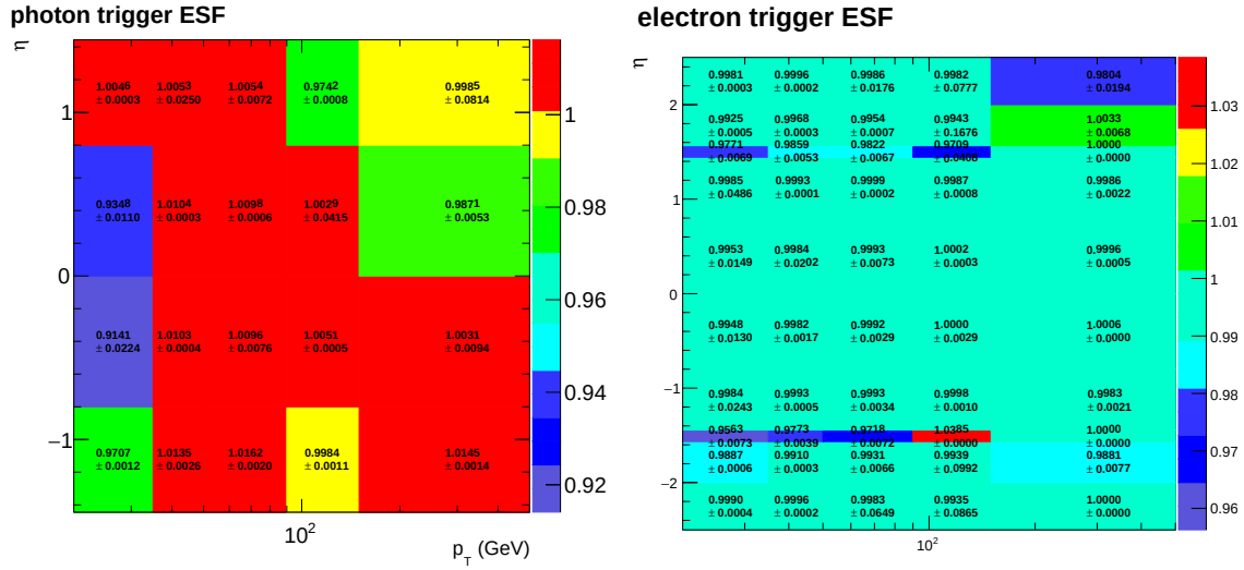
Figure 5.3: Trigger efficiency scale factors for the photon (left) and electron (right).
