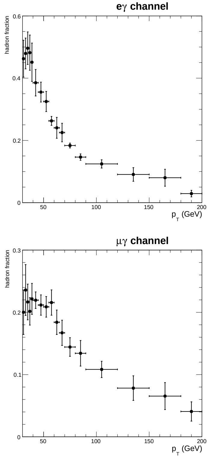
Figure 7.10: The hadron fractions estimated in DoubleEG (top) and MuonEG (bottom) dataset.
