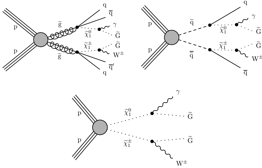
Figure 2.7: Feynman diagrams showing the production and decay modes of the signal models T5Wg (top left), T6Wg (top right), and TChiWg (bottom) considered in this analysis.
