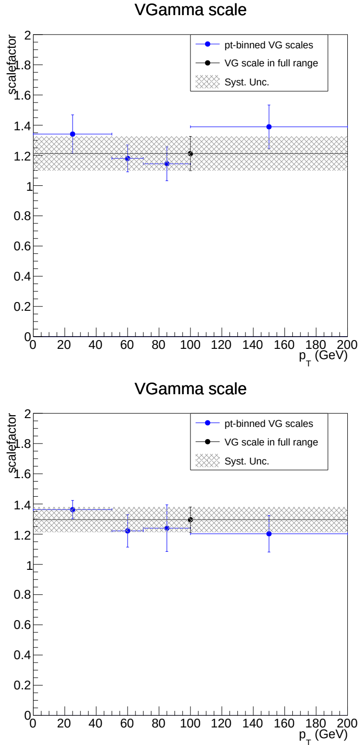
Figure 7.21: The V\gamma scale factors as a function of lepton p_T . The blue dots denote the p_T binned scale factors, and the black dots denote the scale in full p_T range. Top: e\gamma channel, bottom: \mu\gamma channel.
