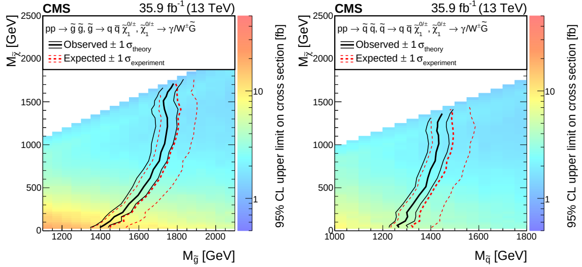
Figure 8.5: Observed and expected exclusion limits for T5Wg (left) and T6Wg (right) models. The upper limits are set on the cross-section \times BR, where BR is the branching fractions to the neutralino/chargino states. For simplicity, BR is assumed to be 50%.
