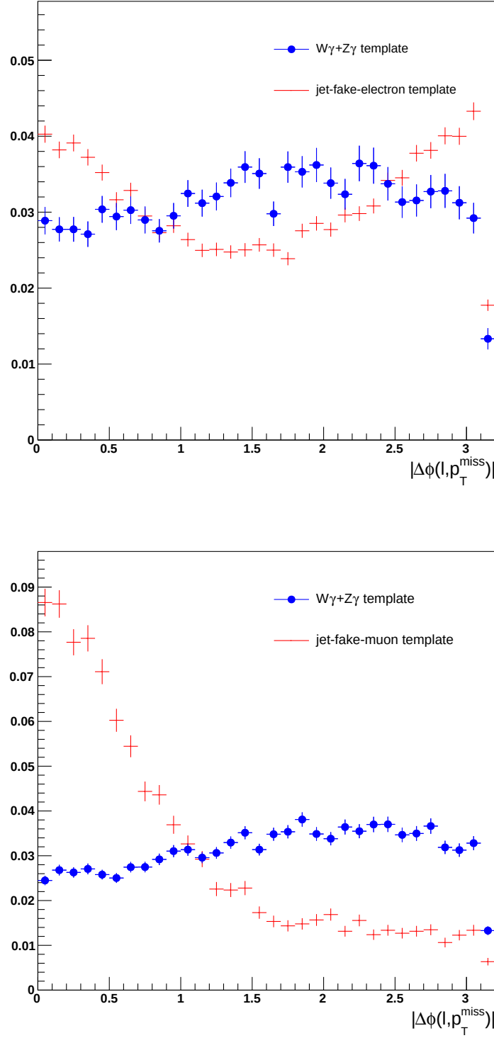
Figure 7.19: \Delta\phi(\ell, p_T^{\text{miss}}) distribution of the V\gamma sample (blue) and fake lepton template (red) in the e\gamma channel (top) and \mu\gamma channel (bottom).
