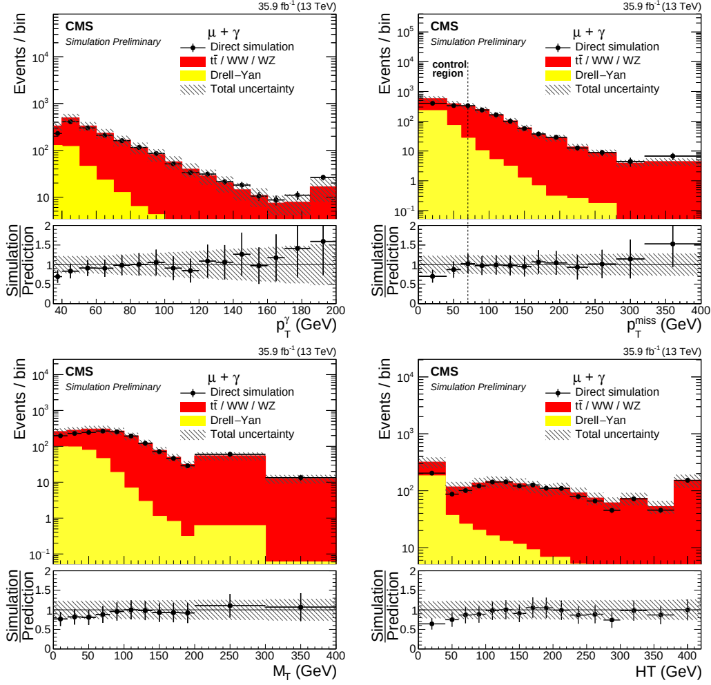
Figure 7.5: Simulation closure test for electron misidentification estimation in the \mu\gamma channel. The misidentification rate derived from Drell-Yan sample is applied to a combination of Drell-Yan, t\bar{t} and WW samples. Top left: photon p_T ; top right: p_T^{\text{miss}} ; bottom left: M_T ; bottom right: HT .
