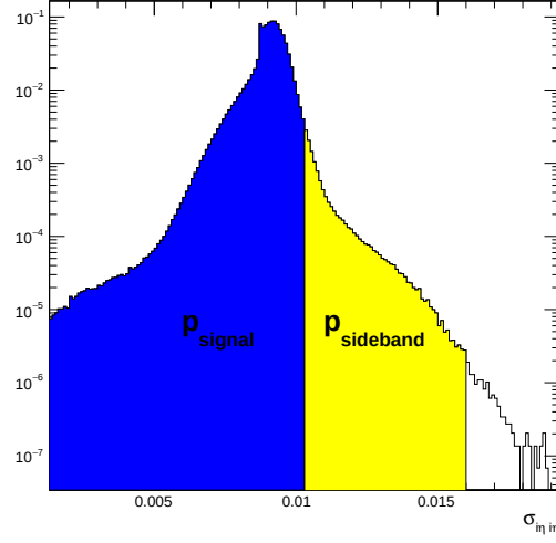
Figure 7.7: The \sigma_{i\eta i\eta} distribution of the true photons in GJet sample. Most of the true photons fall in signal region (blue), however, there is still a small fraction of true photons enter the sideband region (yellow).
