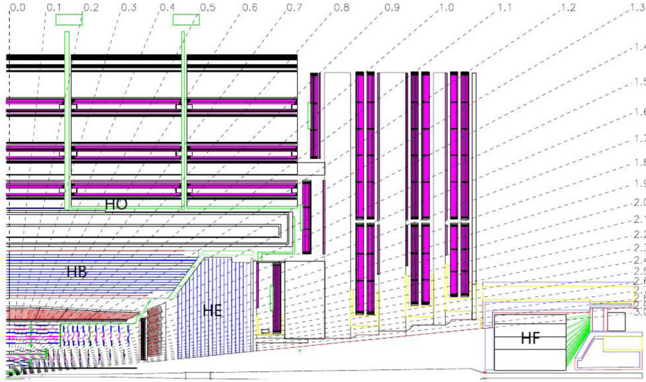
Figure 3.8: HCAL tower segmentation in the r-z plane.
