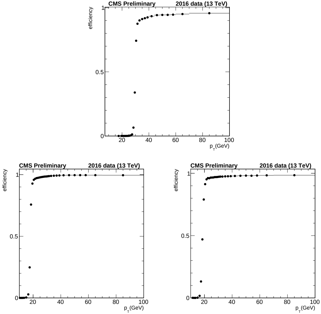
Figure 5.2: Trigger efficiencies for e\gamma channel. Top: leading leg efficiency, bottom left: sub-leading leg efficiency (EB), bottom right: sub-leading leg efficiency (EE).
