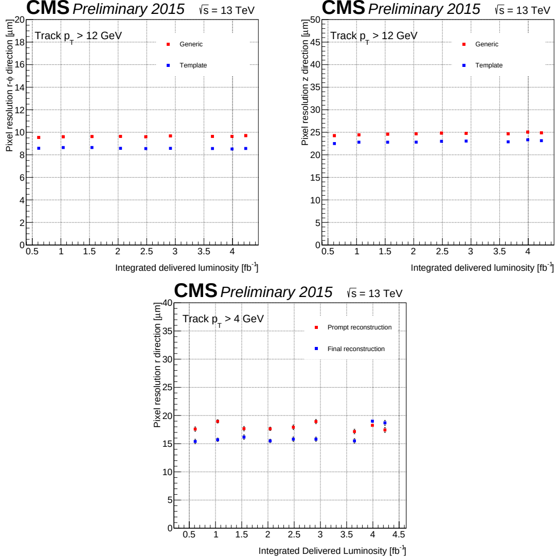
Figure 3.4: Evolution of the BPix resolution in r-\phi direction (top left), BPix resolution in z (top right) direction, and the forward pixel resolution as a function of integrated luminosity in LHC Run II. Reprint from [1].
