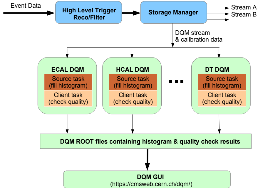
Figure 3.12: Workflow of the data quality monitoring system.
