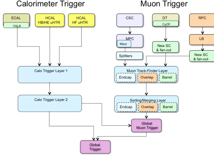
Figure 3.11: Dataflow for the L1 trigger. Reprint from [2].
