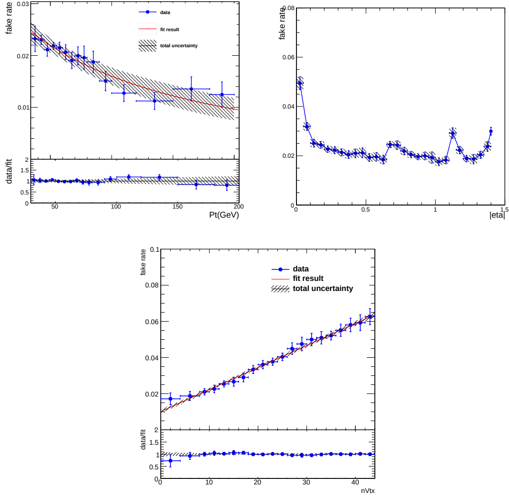
Figure 7.3: The electron misidentification rate as a function of p_T (top left), \eta (top right) and N_{vtx} (bottom), along with the systematic uncertainties.
