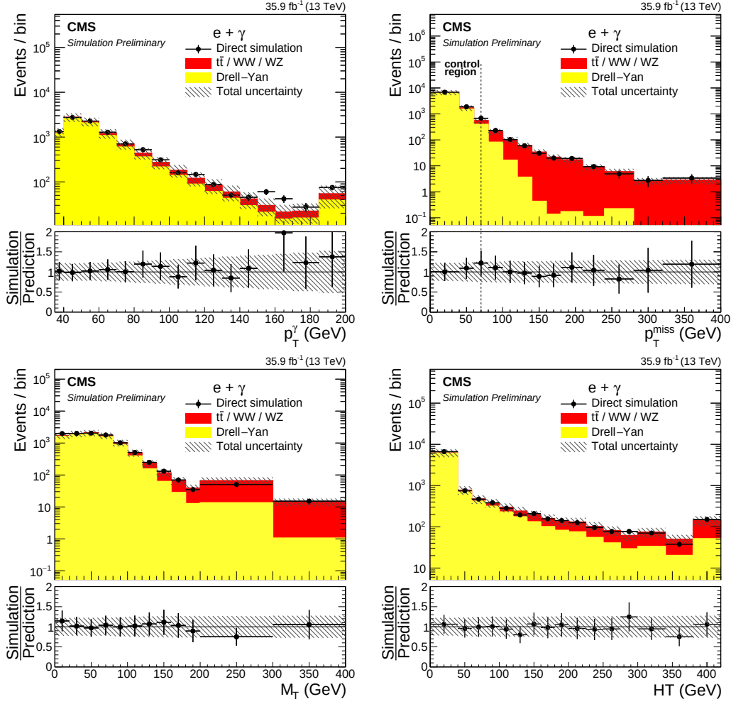
Figure 7.4: Simulation closure test for electron misidentification estimation in the e\gamma channel. The misidentification rate derived from Drell-Yan sample is applied to a combination of Drell-Yan, t\bar{t} and WW samples. Top left: photon p_T ; top right: p_T^{\text{miss}} ; bottom left: M_T ; bottom right: HT .
