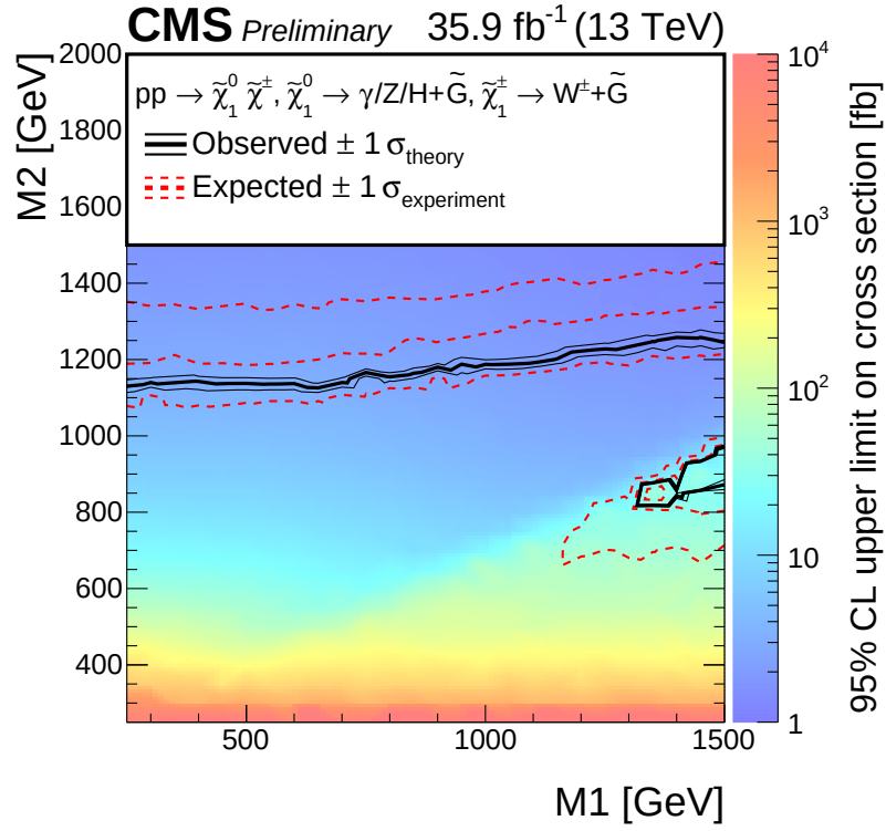
Figure 8.6: Exclusion limits for GGM models as a function of the M1 and M2 masses.
