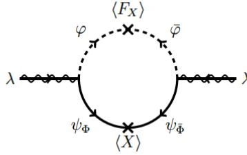
Figure 2.4: Radiative corrections to the mass of SUSY particles.
