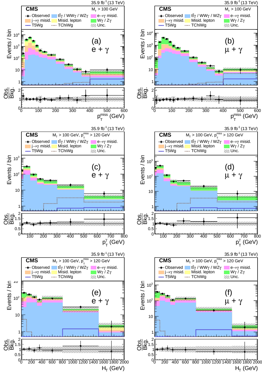
Figure 8.2: Distributions of p_T^{\text{miss}} (a, b), p_T^\gamma (c, d), and H_T (e, f) from data (points) and estimated SM predictions (stacked histograms) for the e\gamma (left) and \mu\gamma (right) channels.
