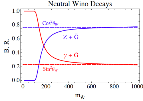
Figure 2.5: Branching ratio of a wino-like neutralino NLSP as a function of the neutralino mass.
