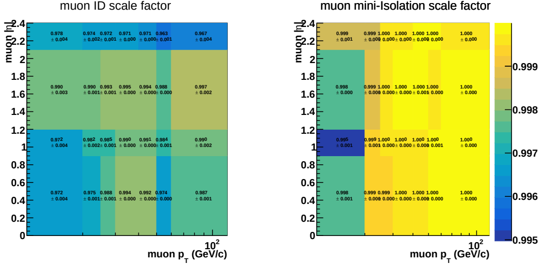
Figure 6.3: data-to-simulation scale factors for muons.
