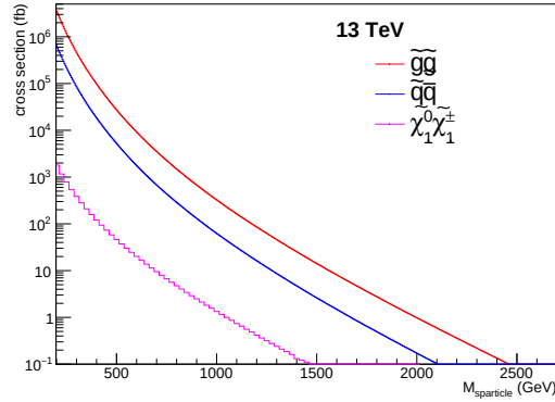
Figure 2.6: Cross sections for producing various pairs of sparticles at \sqrt{s} = 13 TeV.
