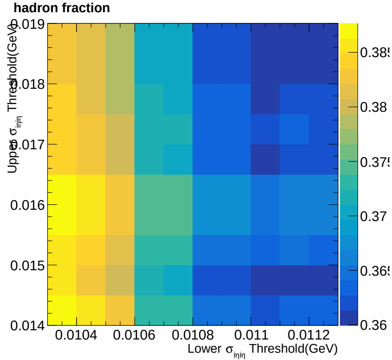
Figure 7.12: 2D distribution of the fraction of hadrons for photons with 50 \text{ GeV} < p_T < 55 \text{ GeV} . The full variation will be used as systematic uncertainties of the template fit.
