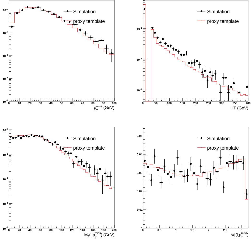
Figure 7.13: Comparison of various kinematic distributions between simulated QCD events with a fake electron and events in data with a control electron. The distributions are area-normalized to facilitate a comparison of their shapes.
