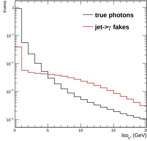
Figure 7.6: The normalized Iso_{h\pm} distributions of the true (black line) and fake (red line) photons in GJet sample.
