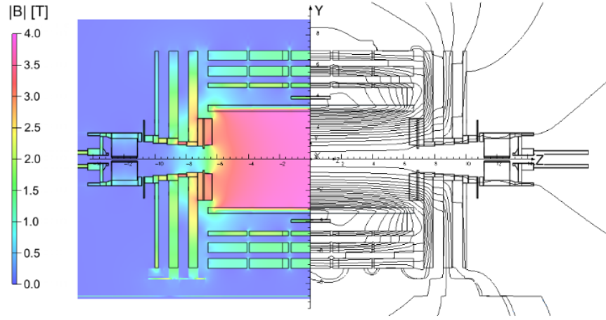
Figure 3.9: Map of the magnet field (left) and field lines (right) predicted for a longitudinal section of the CMS detector by a magnetic field model at a central magnetic flux density of 3.8 T. Each field line represents a magnetic flux increment of 6 Wb
