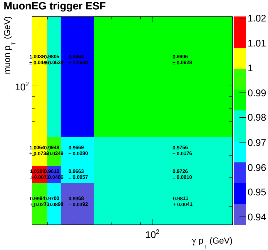
Figure 5.5: \mu\gamma simulation-to-data trigger efficiency scale factor as a function of photon and muon p_T
