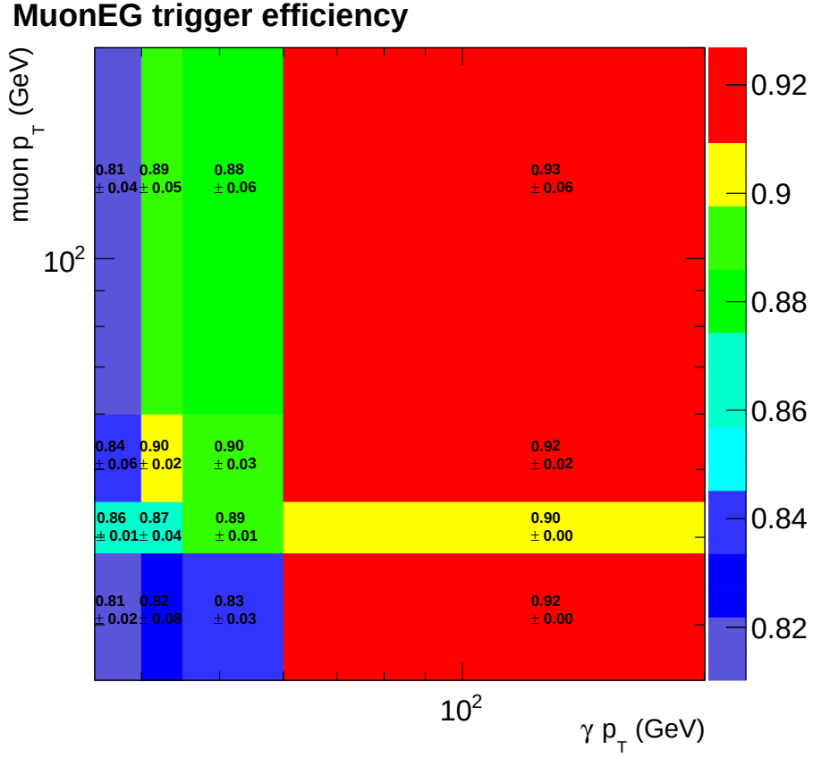
Figure 5.4: \mu\gamma trigger efficiency as a function of photon and muon p_T
