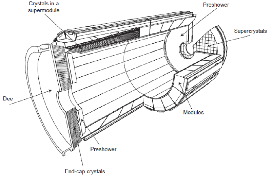
Figure 3.6: Layout of the CMS Electromagnetic Calorimeter (ECAL).
