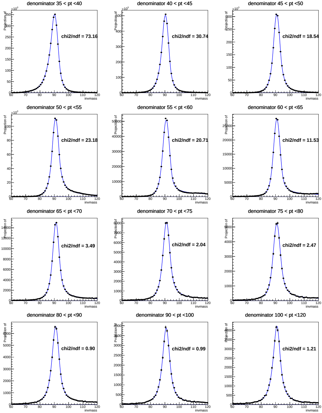
Figure 7.1: Fits to the tag-and-probe invariant mass of the denominator samples, which are defined as the samples with probe electrons matching to pixel track seeds. This fit is performed in various p_T bins. The black dots, the blue solid lines, and the blue dashed lines represent the data, the signal+background model, and the background-only model, respectively.
