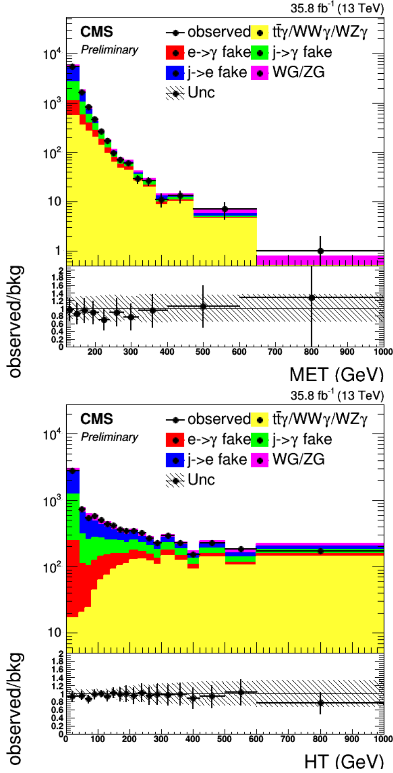
Figure 7.25: p_T^{\text{miss}} (top) and H_T (bottom) distributions of the e\gamma channel in the validation region defined as \geq 1 b-jet, M_T(\ell, p_T^{\text{miss}}) < 100 GeV.
