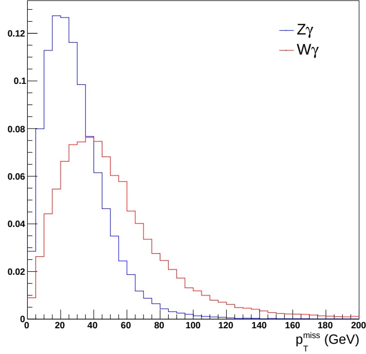
Figure 7.20: p_T^{\text{miss}} distributions of the W\gamma (red) and Z\gamma (blue) sample. The 40 GeV cut will remove a large fraction of the Z\gamma contributions.
