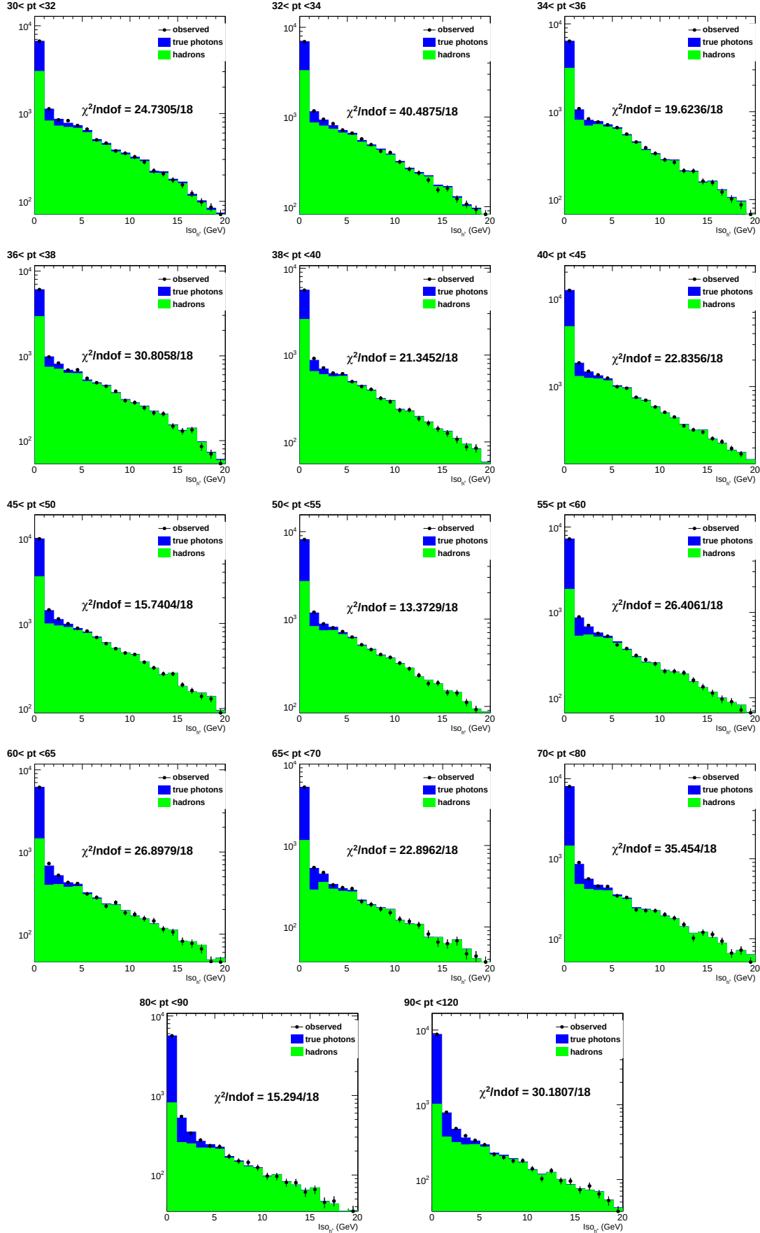
Figure 7.9: Template fits for hadron fraction measurements in e\gamma channel.
