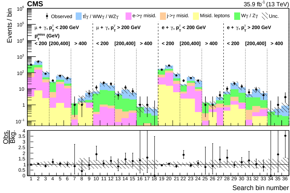
Figure 8.3: Event yields and stacked background predictions as a function of search bin numbers.
