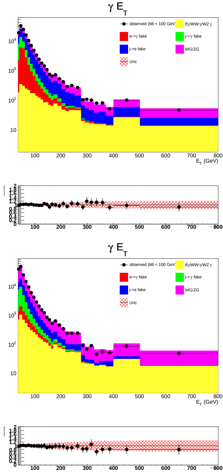
Figure 7.27: Photon p_T distributions in the e\gamma channel (top) and the \mu\gamma channel (bottom).
