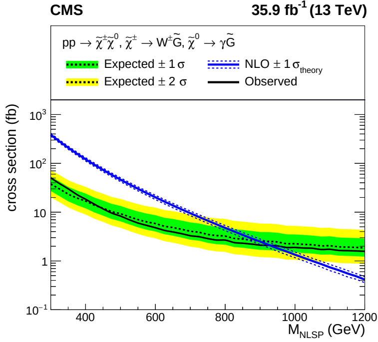
Figure 8.4: Observed and expected upper limits on the cross-sections of the TChiWg model, together with the theoretical cross-sections.
