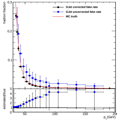
Figure 7.8: The hadron fractions estimated in GJet sample. The estimation with iteration corrections is shown in black dots, and the one without such correction is shown in blue.
