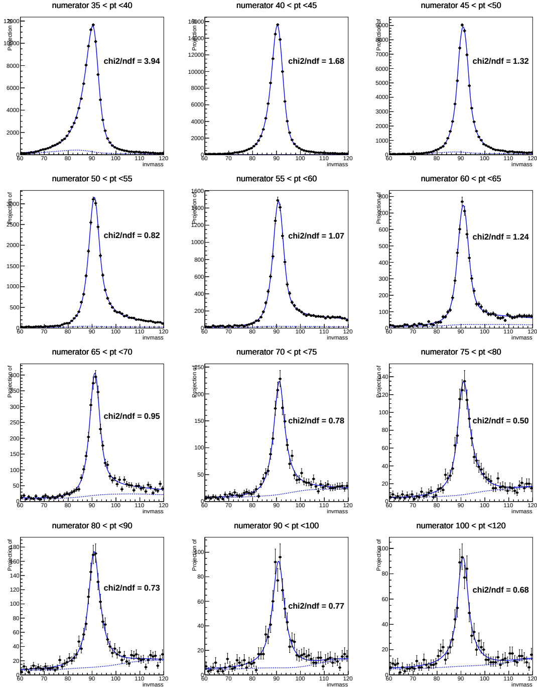
Figure 7.2: Fits to the tag-and-probe invariant mass of the numerator samples, which are defined as the samples with probe electrons failing to be matched with pixel track seeds. This fit is performed in various p_T bins. The black dots, the blue solid lines, and the blue dashed lines represent the data, the signal+background model, and the background-only model, respectively.
