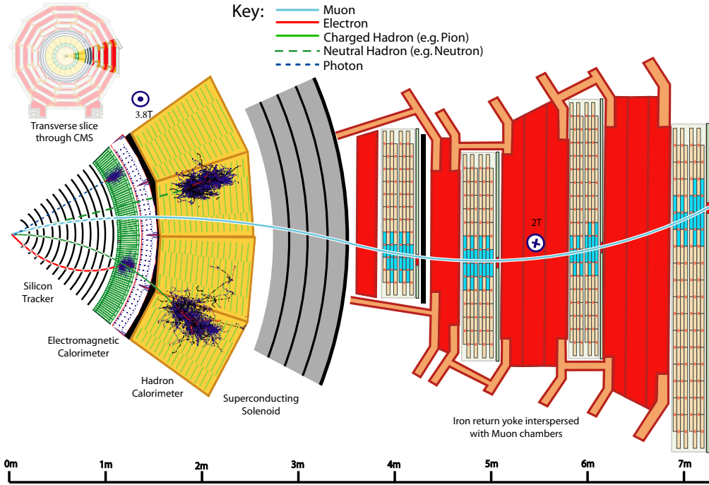
Figure 4.1: A sketch of the responses of different types of particles in a transverse slice of the CMS detector. The muon and the charged pion are positively charged, and the electron is negatively charged. Reprint from [3].
