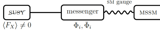
Figure 2.3: Sketch of SUSY breaking in the hidden sector that is mediated to the MSSM sector via the messenger fields.
