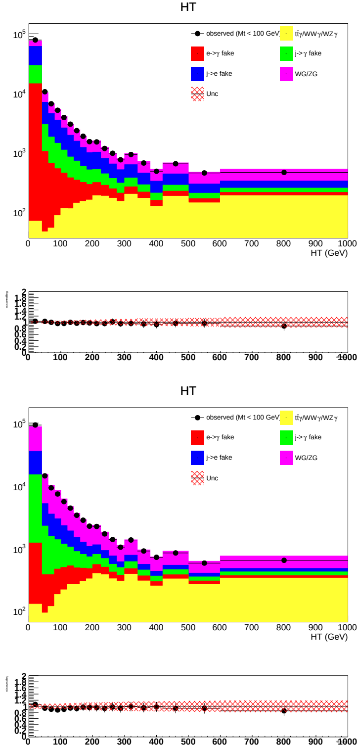
Figure 7.29: HT distributions in the e\gamma channel (top) and the \mu\gamma channel (bottom).
