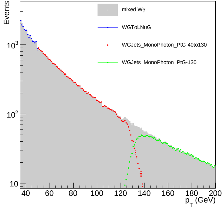
Figure 7.16: Photon p_T distributions in individual W\gamma samples and their combination.
