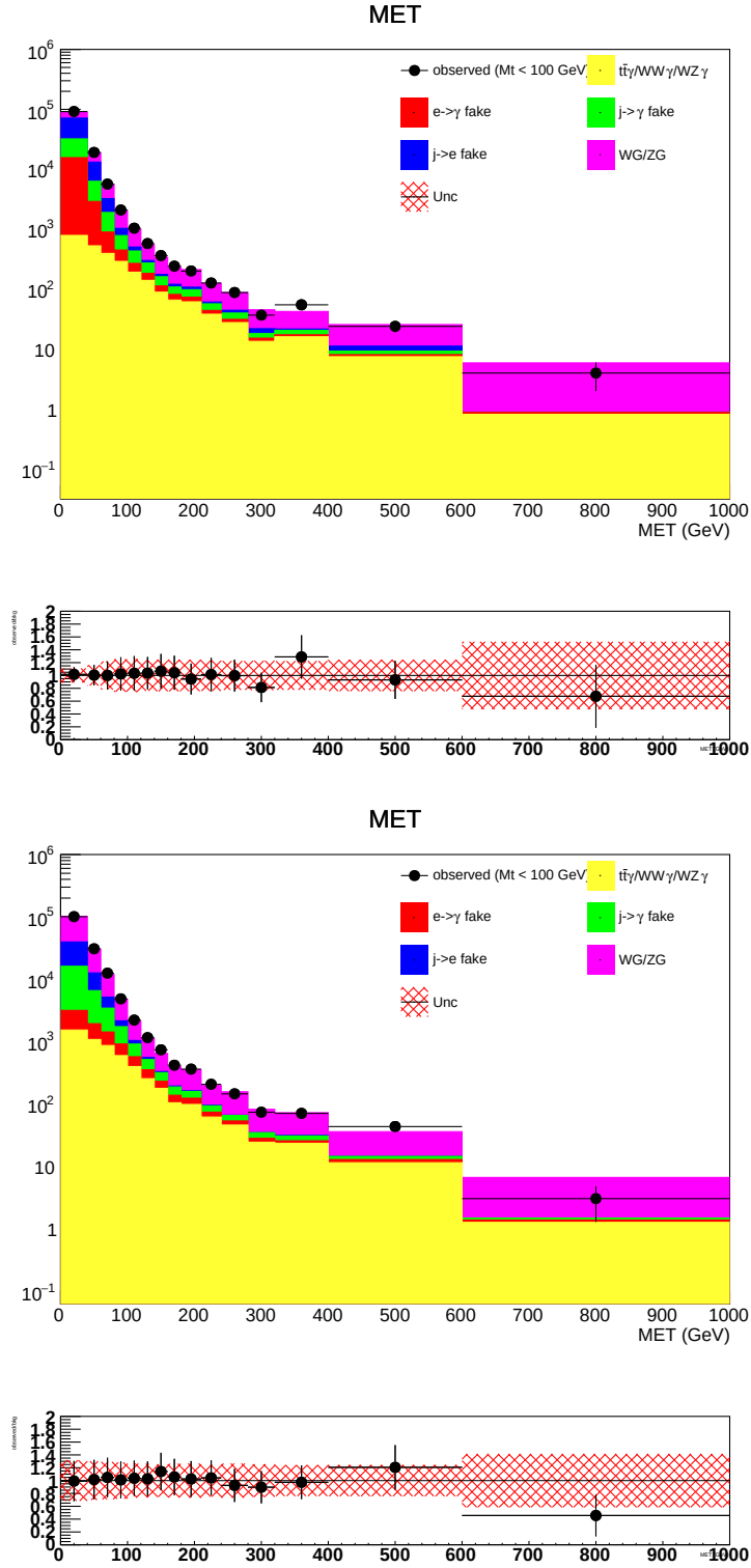
Figure 7.28: p_T^{\text{miss}} distributions in the e\gamma channel (top) and the \mu\gamma channel (bottom).
