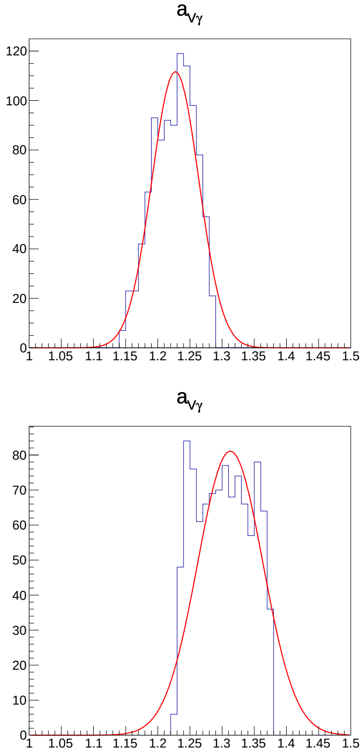
Figure 7.24: Distribution of the scale factors derived from 1000 toy MC experiments. Top: e\gamma channel, bottom: \mu\gamma channel.
