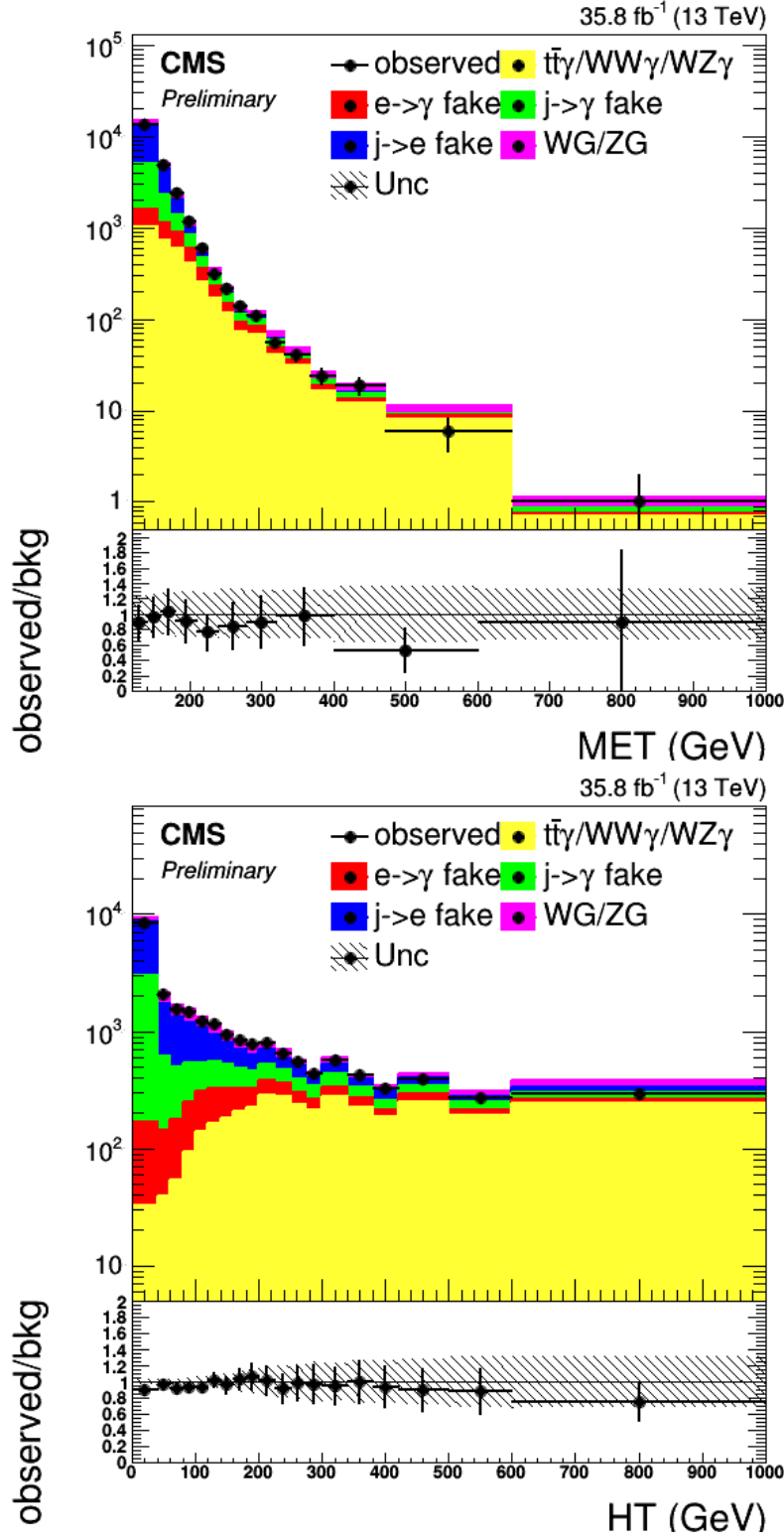
Figure 7.26: p_T^{\text{miss}} (top) and H_T (bottom) distributions of the \mu\gamma channel in the validation region defined as \geq 1 b-jet, M_T(\ell, p_T^{\text{miss}}) < 100 GeV.
