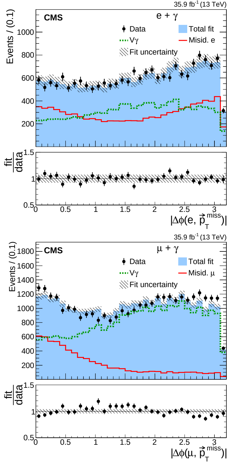
Figure 7.22: Results of the \Delta\phi(\ell, p_T^{\text{miss}}) template fit in the e\gamma channel (top) and \mu\gamma channel (bottom).
