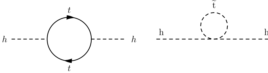
Figure 2.2: Contributions of SM and SUSY loop corrections to the mass of Higgs.
