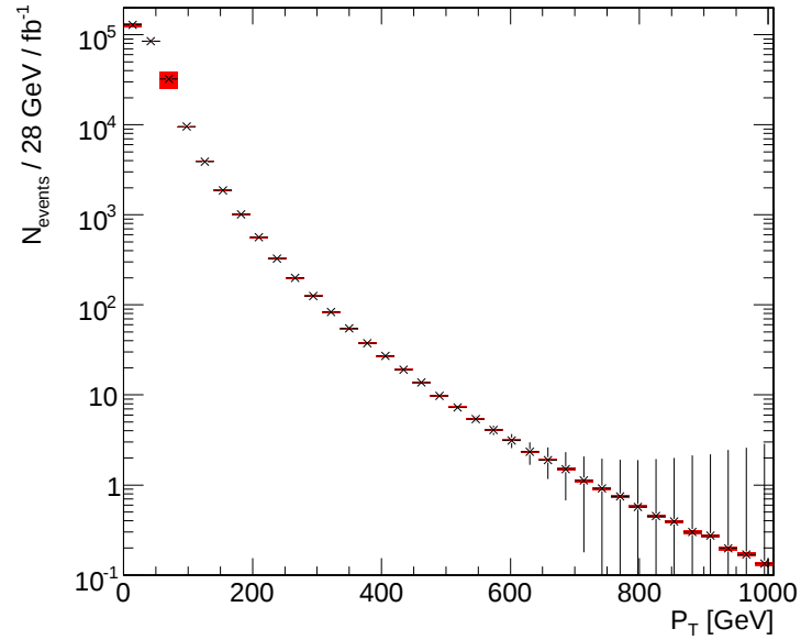
Figure 6.8: Expected number of reconstructed events containing a Z boson and at least one jet after the selection criteria for an integrated luminosity of 1 \text{ fb}^{-1} . The black bars indicate the statistical uncertainty whereas the red boxes show the uncertainty related to the number of simulated events.
