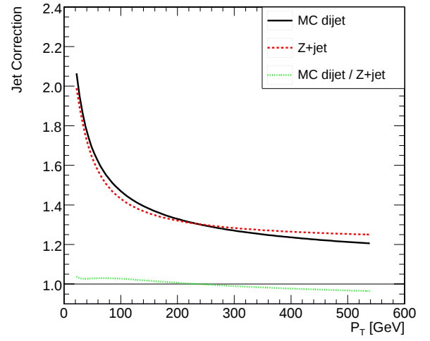
L3 correction factors: SIScone 0.5
