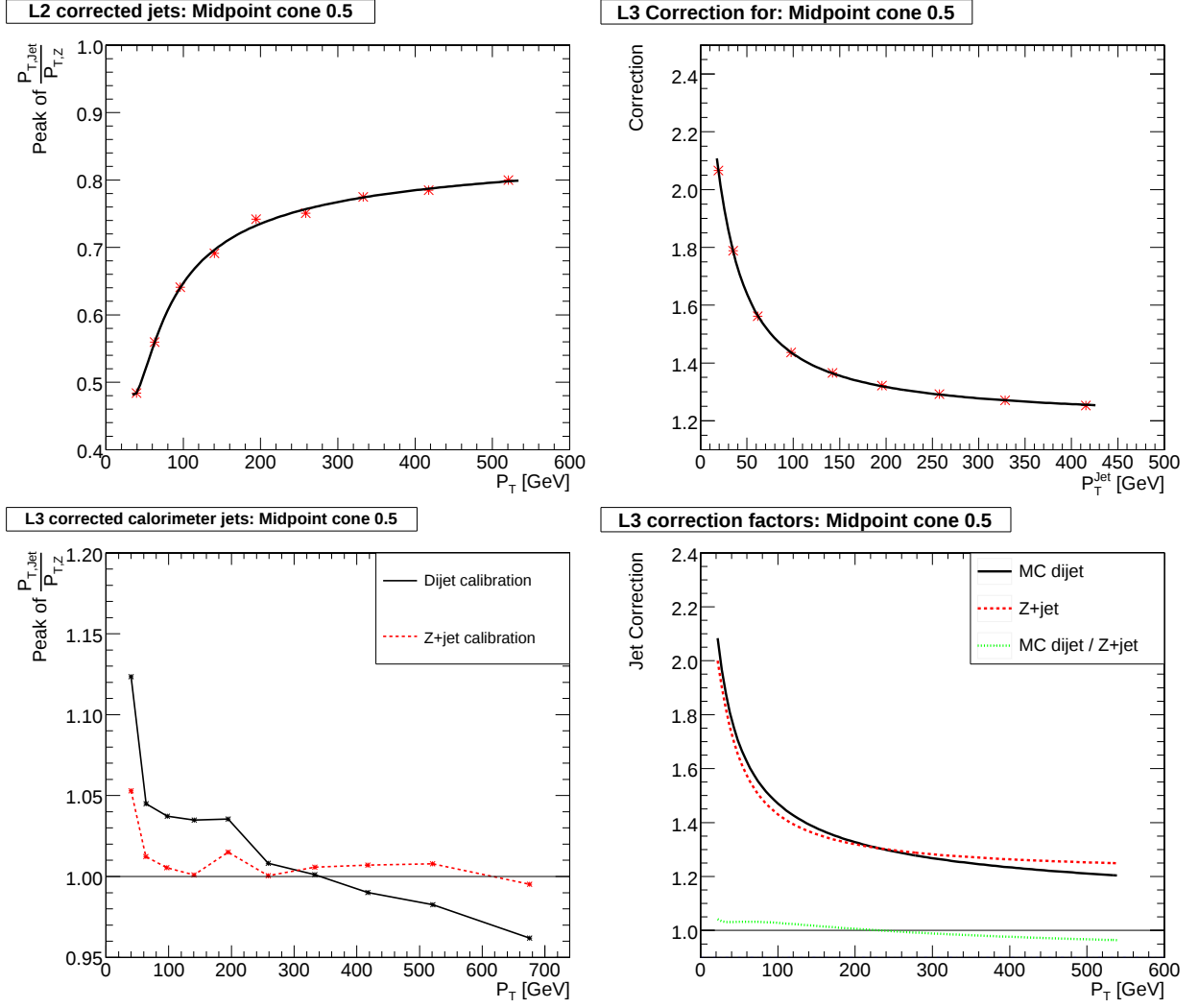
Figure A.3: Same as Figure A.1 but for the Midpoint cone 0.5 jet algorithm.
