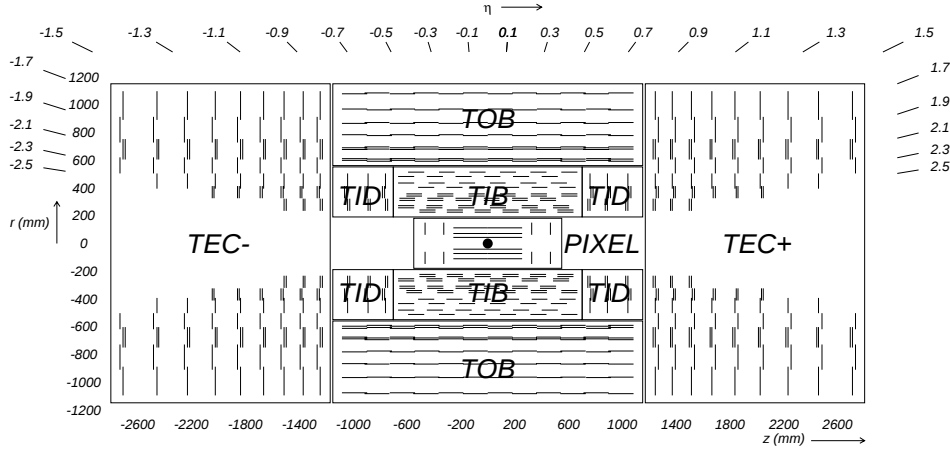
Figure 2.4: Cross-section through the CMS tracking system [24].
