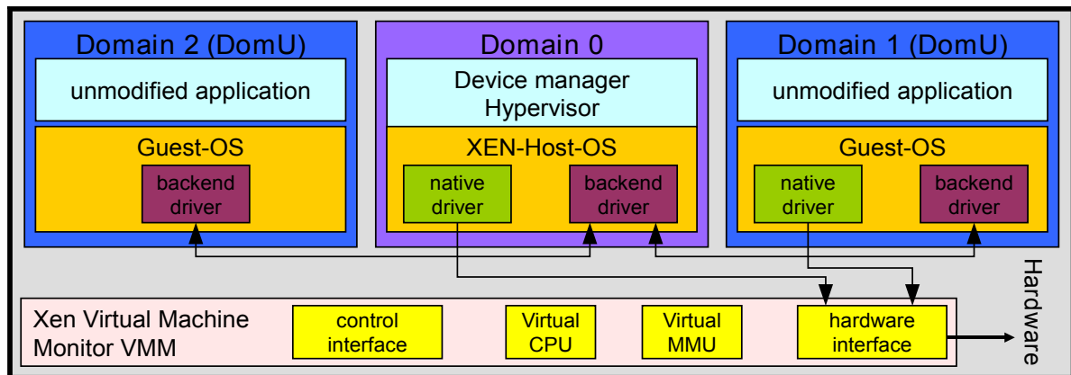
Figure 4.4: Schematic overview of the paravirtualisation by Xen.
