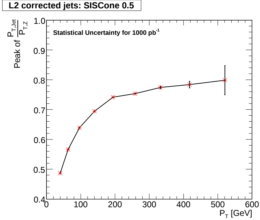
Figure 6.27: Peak of the ratio of the transverse momentum of L2 calibrated SIScone 0.5 jets and the balanced Z boson versus p_T^Z . The peak is determined by a Gaussian fit and the error bars indicate the statistical uncertainty on the Gauss mean for a number of events corresponding to an integrated luminosity of 1000 \text{ pb}^{-1} .
