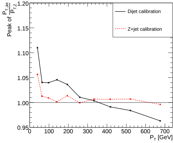
L3 corrected calorimeter jets: SIScone 0.5
