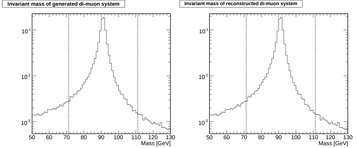
Figure 6.7: Normalised distribution of the invariant mass M of the di-muon system for both, generated and reconstructed muons including all selection criteria. The dashed lines enclose the region of |M - M_Z| < 20 GeV.
