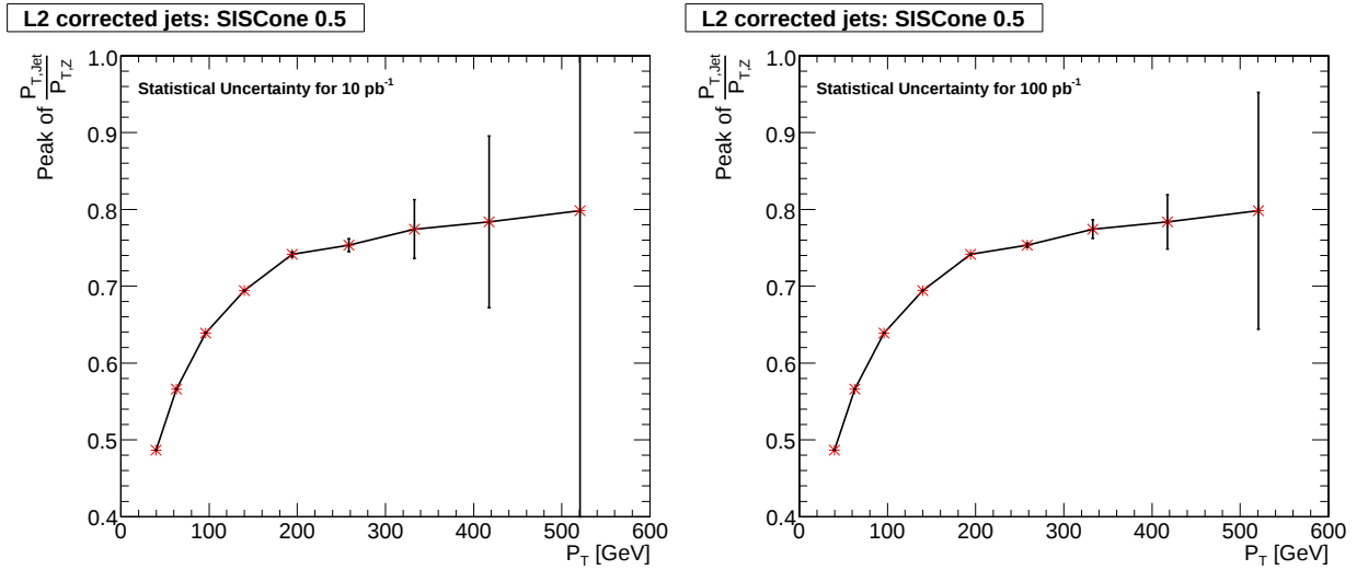
Figure 6.28: Same as Figure 6.27 but for an expected statistics corresponding to an integrated luminosity of 10 \text{ pb}^{-1} (left) and 100 \text{ pb}^{-1} (right).
