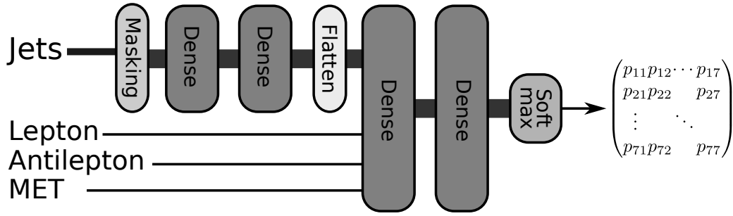
Figure 6.4: Scheme of the network for b jet classification. Due to their varying length the jets are fed into the network via a masking layer after padding with 0.
