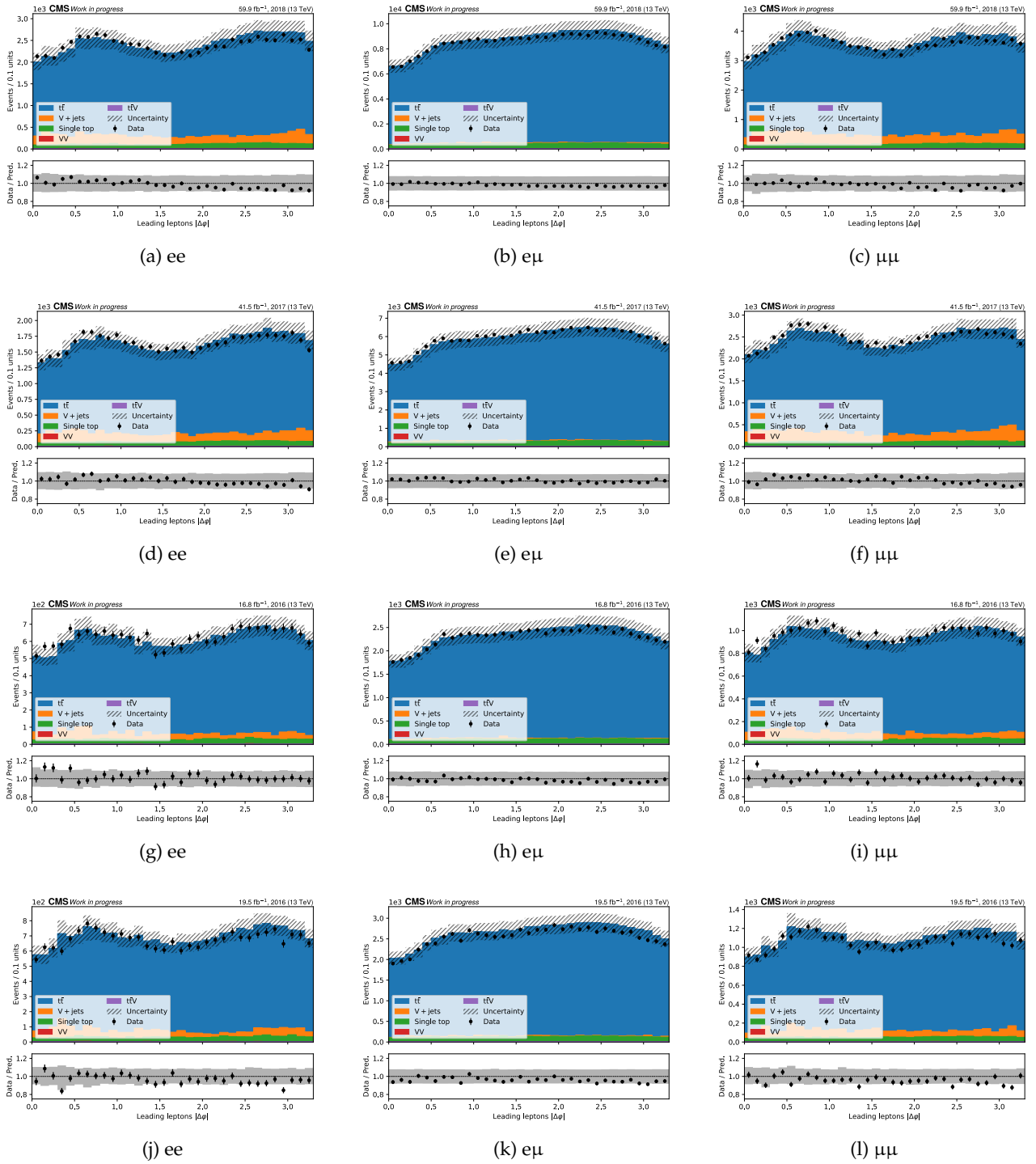
Figure A.4: Difference between \phi of the leptons for 2018 (first row), 2017 (second row), 2016post (third row) and 2016pre (fourth row).
