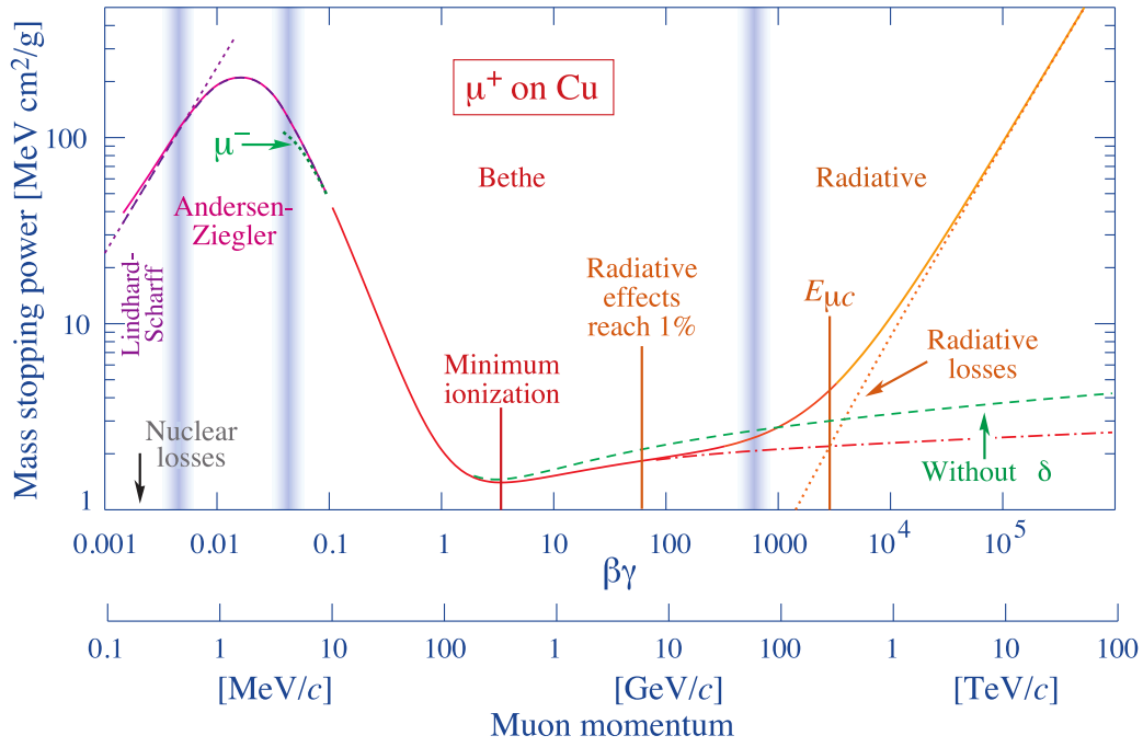
Figure 4.4: Graph of the Bethe-Bloch formula together with various corrections to it. Shown is the energy loss per density of a charged particle in copper. By dividing by the density, the dependence on the material (here copper) becomes minor, thus one can expect a very similar curve for silicon. From [1].
