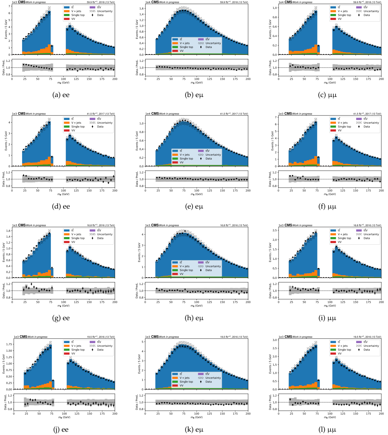
Figure A.5: Invariant mass of the leptons m_{\ell\ell} for 2018 (first row), 2017 (second row), 2016post (third row) and 2016pre (fourth row).
