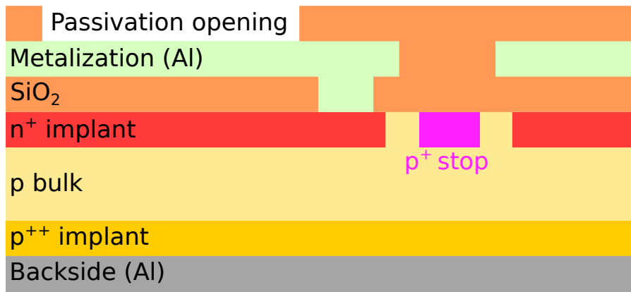
Figure 4.6: Side view (not to scale) of a slice through part of the diode of the BCM1F detector. The diode and the guard ring are separated by a p^+ stop. The conductive metalization layer is only reachable for electric connections from the outside via the passivation openings. It connects to the n^+ implant only at specific parts of the sensor, where the silicon dioxide has an opening.
