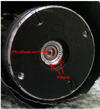
Figure 4.8.: The LED diffuser. Schematic drawing (left), photo (right).
