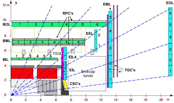
Figure 2.11.: Cut-view of one quadrant of the Muon Spectrometer.
