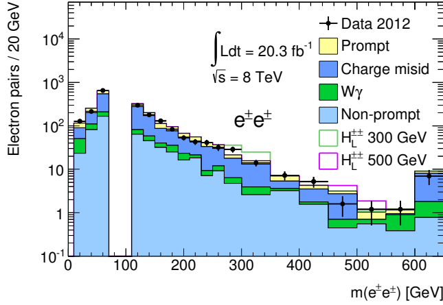
Figure 5.19.: Invariant mass distributions for e^{\pm}e^{\pm} pairs passing the full event selection. Open histograms show the expected signal from simulated H^{\pm\pm} samples, assuming a 100% branching ratio to the same-sign electron pair. The last bin is an overflow bin. Only statistical uncertainties for data are shown.
