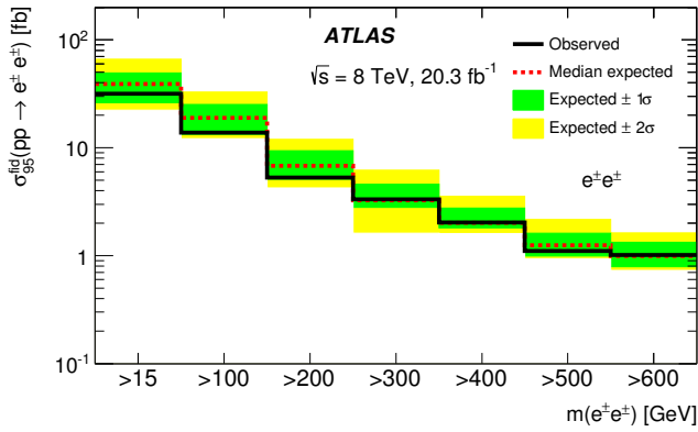
Figure 5.16.: Fiducial cross section upper limits at 95% C.L. for new physics contributing to the signal region for events with e^{\pm}e^{\pm} pairs. Green and yellow bands correspond to the 1\sigma and 2\sigma uncertainty bands on the expected limits respectively.
