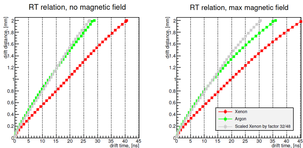
Figure 3.13.: r-t relation for the Xenon- (red) and Argon-based (green) gas mixtures. The curve for the Argon-based mixture was obtained from the Garfield simulation. A scaled (by the ratio of the average drift velocities in the Argon and Xenon mixtures) r-t relation of the Xenon-based mixture is shown in gray and was used in the initial studies of the Argon mixture.
