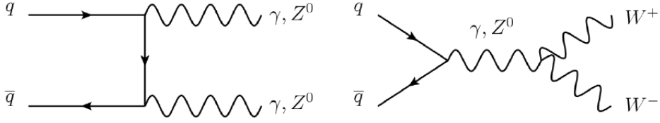
Figure 6.6.: Feynman diagram for the diboson production.
