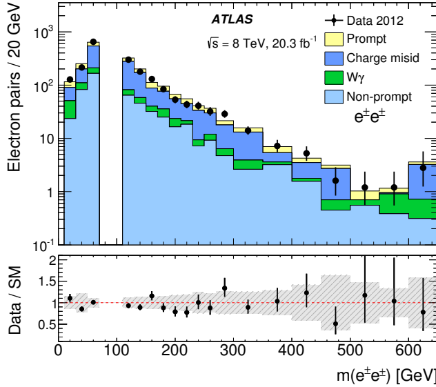
Figure 5.13.: Invariant mass distribution for e^{\pm}e^{\pm} pairs in the signal region. The shaded band in the lower plot corresponds to the combination of the statistical and systematic uncertainties of the background prediction. The last bin is an overflow bin.
