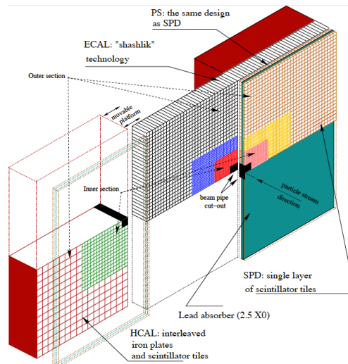
Figure 2.1 – Structure of the Calorimeter system
