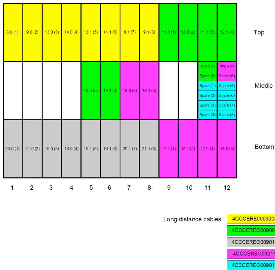
Figure A.3 – Optical cable patch pannel (barrack).
