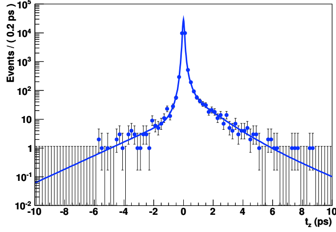
Figure 3.6 – t_z background function for bin ( 3 < p_T < 4 GeV/ c , 2.5 < y < 3 ).
