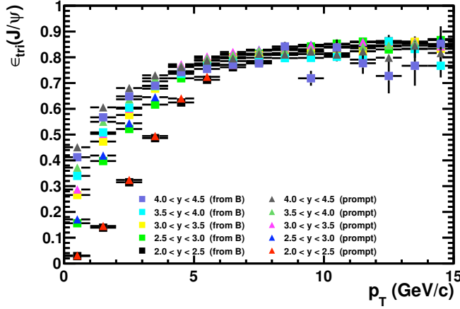
Figure 3.11 – Monte Carlo-based trigger efficiency \epsilon_{\text{tri}} for TCK 0x001D0030 for prompt J/\psi and J/\psi from b as a function of p_T in bins of y . Identical efficiencies are obtained for TCK 0x001E0030.
