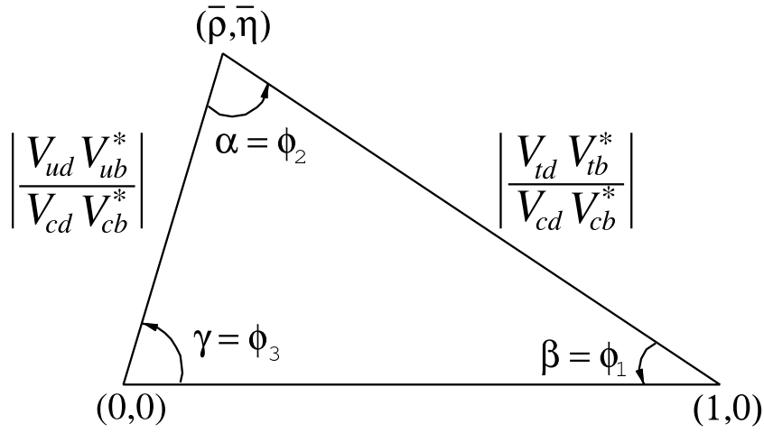
Figure 2 – Unitarity triangle.
