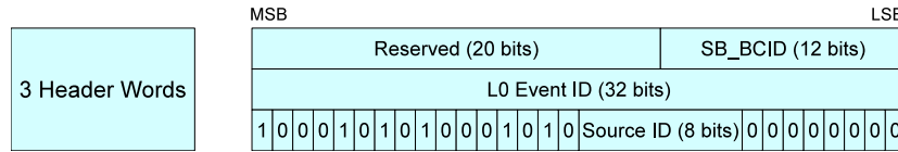
Figure 2.41 – Format of the header words sent from the Selection Boards to the TELL1.
