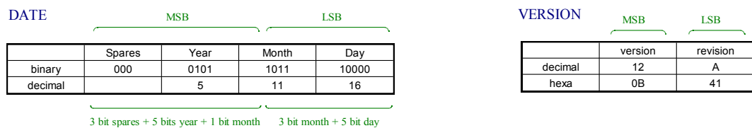
Figure B.5 – Date and serial ID registers (sub-addresses 12 and 13).
