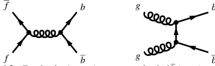
Figure 1.3 – Tree-level pair-creation processes for the b\bar{b} (or c\bar{c} ) production.
