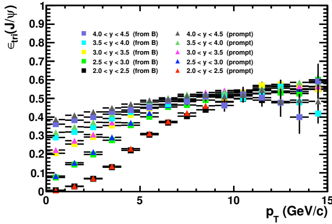
Figure 3.12 – Monte Carlo-based trigger efficiency \epsilon_{\text{tri}} for TCK 0x001F0029 for prompt J/\psi and J/\psi from b as a function of p_T in bins of y .
