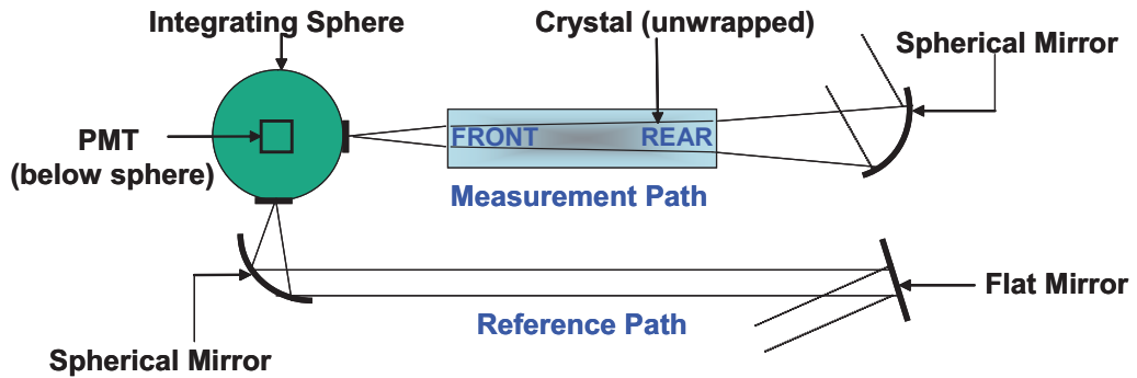
Figure 3.7: Apparatus used to measure transmission at ENEA.
