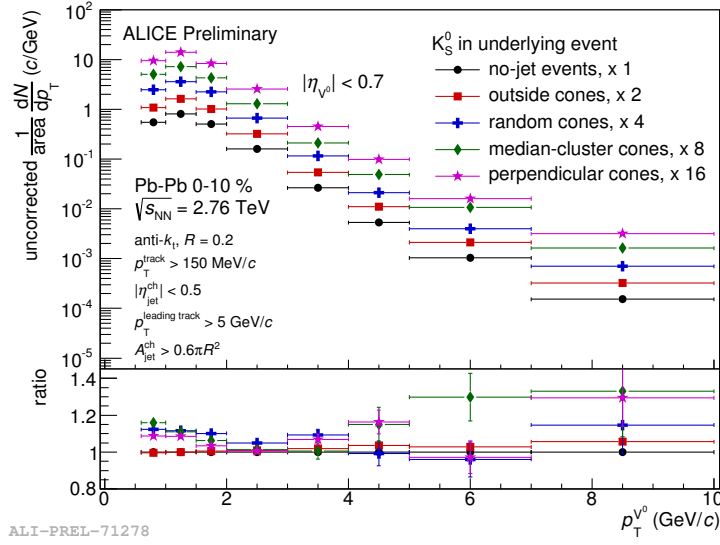
Figure F.2: Uncorrected K_S^0 p_T spectra in the Underlying Event and for 5 different estimation methods. The lower plot shows the ratio for each method relative to the default method ('no-jet') events.
