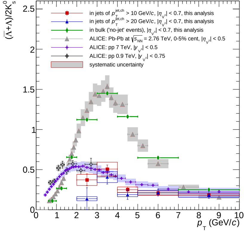
Figure 4.4: (\bar{\Lambda} + \Lambda)/2K_S^0 ratio in jets ( R = 0.2 ) for p_T^{\text{jet}} > 10 GeV/c (red markers) and p_T^{\text{jet}} > 20 GeV/c (blue markers) and in the bulk of the Pb–Pb collision event (green markers) via “no-jet” events. The measured ratios from this analysis are compared to the inclusive, published \Lambda/K_S^0 ratio (grey markers) and the inclusive ratio measured in pp collisions at \sqrt{s} = 7 TeV and \sqrt{s} = 0.9 TeV.
