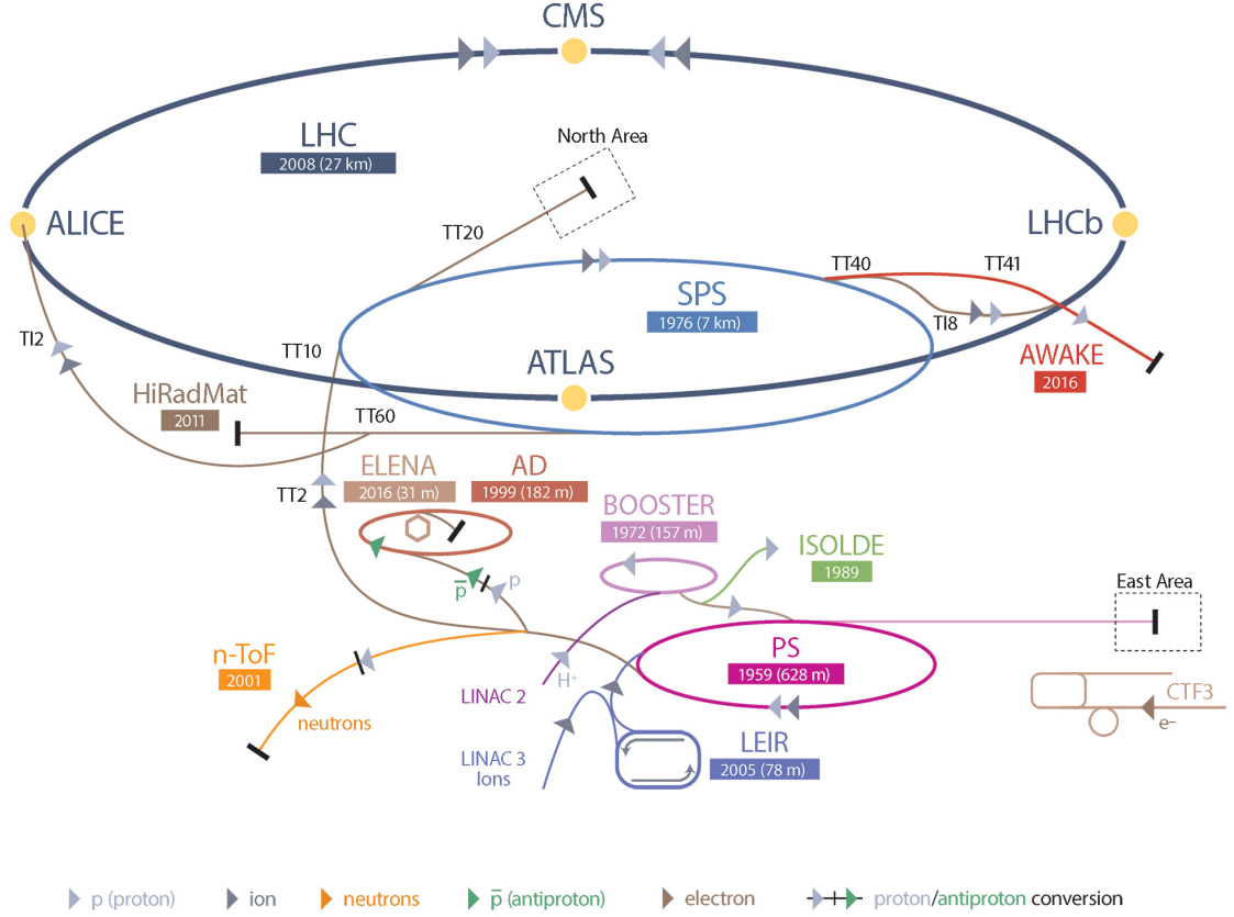
Figure 2.1: LHC complex with injector chain and interaction points (yellow points). Where the two oppositely directed beams intersect, the 4 largest experiments are ALICE, CMS, LHCb and ATLAS are located. Several pre-accelerators are required to reach the final LHC collisional energy [132].
