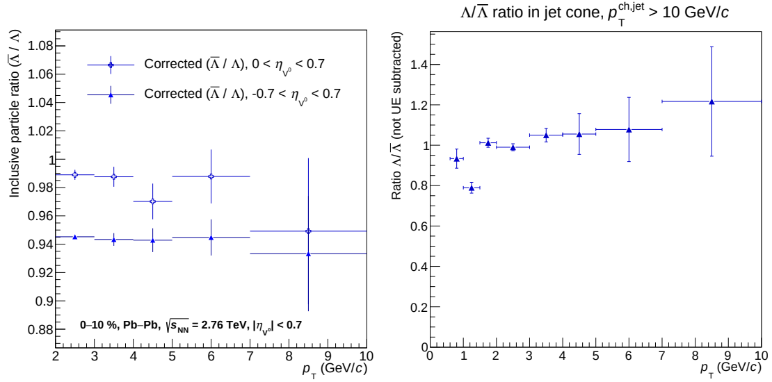
Figure 3.53: Left side: Ratio of the inclusive \Lambda and \bar{\Lambda} p_T spectrum measured in the 2011 dataset (for the entire \eta^{V^0} acceptance) shows a deviation from unity. The effect is about 5–10% smaller when only taking \Lambda(\bar{\Lambda}) particles with positive \eta^{V^0} (what corresponds to the "A-side" of the detector) shown as open markers. Right side: \Lambda/\bar{\Lambda} ratio as function of p_T in jet cones (uncorrected yields).
