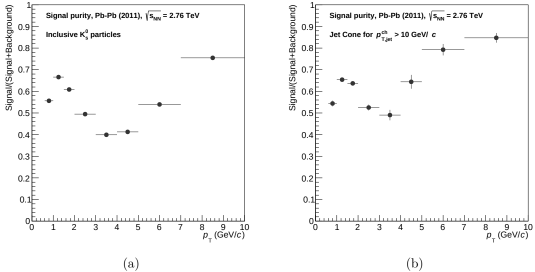
Figure 3.9: Two examples for the signal purity as function of the V^0 p_T obtained with the signal extraction for inclusive K_S^0 (left panel) and the K_S^0 particle in jet cones (right panel). The signal purity is defined as the ratio of the signal yield (in the peak region) over the signal+background sample in the same region.
