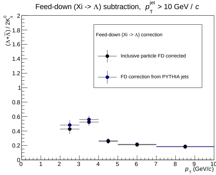
Figure 3.52: (\Lambda + \bar{\Lambda})/2K_S^0 ratio in jets ( p_{T,\text{jet}}^{\text{ch}} > 10 \text{ GeV}/c and R = 0.2 ), corrected with FD fractions from inclusive particle analysis and from simulation in PYTHIA8 jets ( R = 0.2 ).
