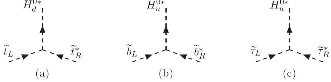
Figure 2.8: Examples of (scalar) 3 couplings.
