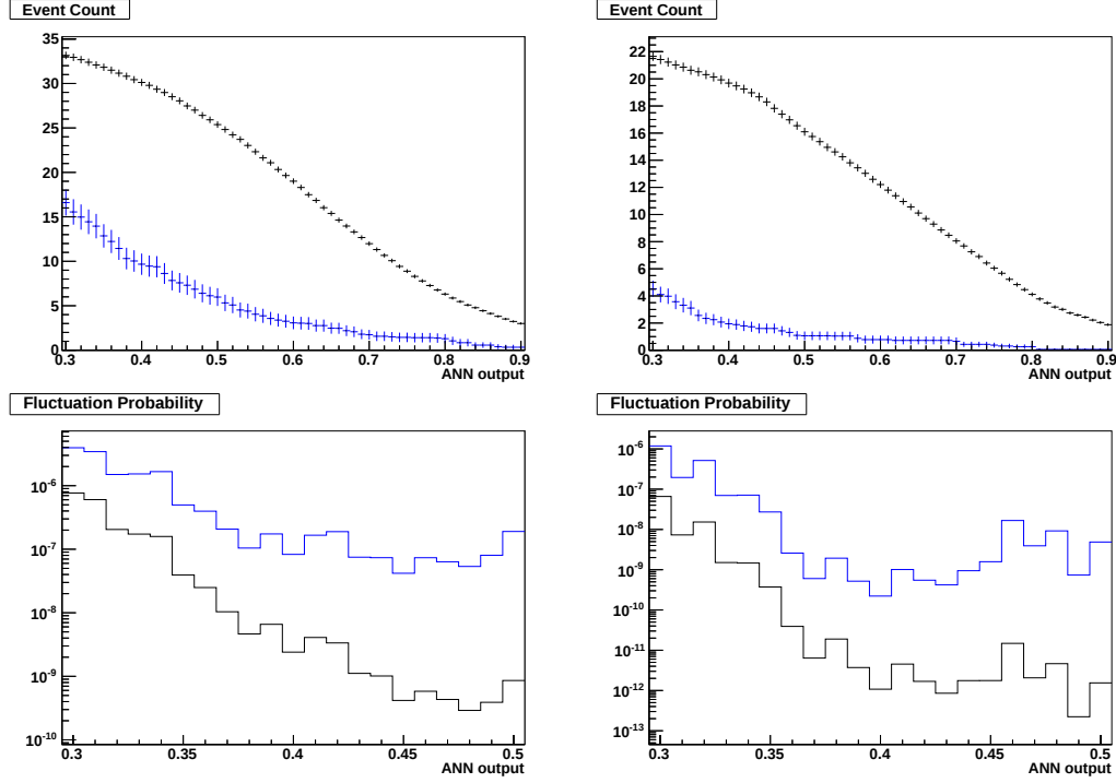
Figure 6.3: Optimization of the ANN cut. The top plots show the LM6 (black) and SM (blue) yields in the low- E_T signal region (left) and high- E_T signal region (right) as a function of the ANN cut. The bottom plots show the probability that the SM yield will fluctuate up to the LM6 yield, taking into account the statistical uncertainty and 30% systematic uncertainty in the background prediction for the low- E_T signal region (left) and high- E_T signal region (right). The blue lines include signal contamination bias, and the black lines do not.
