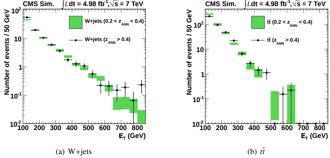
Figure 6.8: The E_T distributions of simulated W+jets (a) and t\bar{t} (b) events in the z_{\text{ANN}} signal region (solid circles) and sideband (green bars). The normalization region is 150 \text{ GeV} < E_T < 350 \text{ GeV} . The last histogram bin includes overflow.
