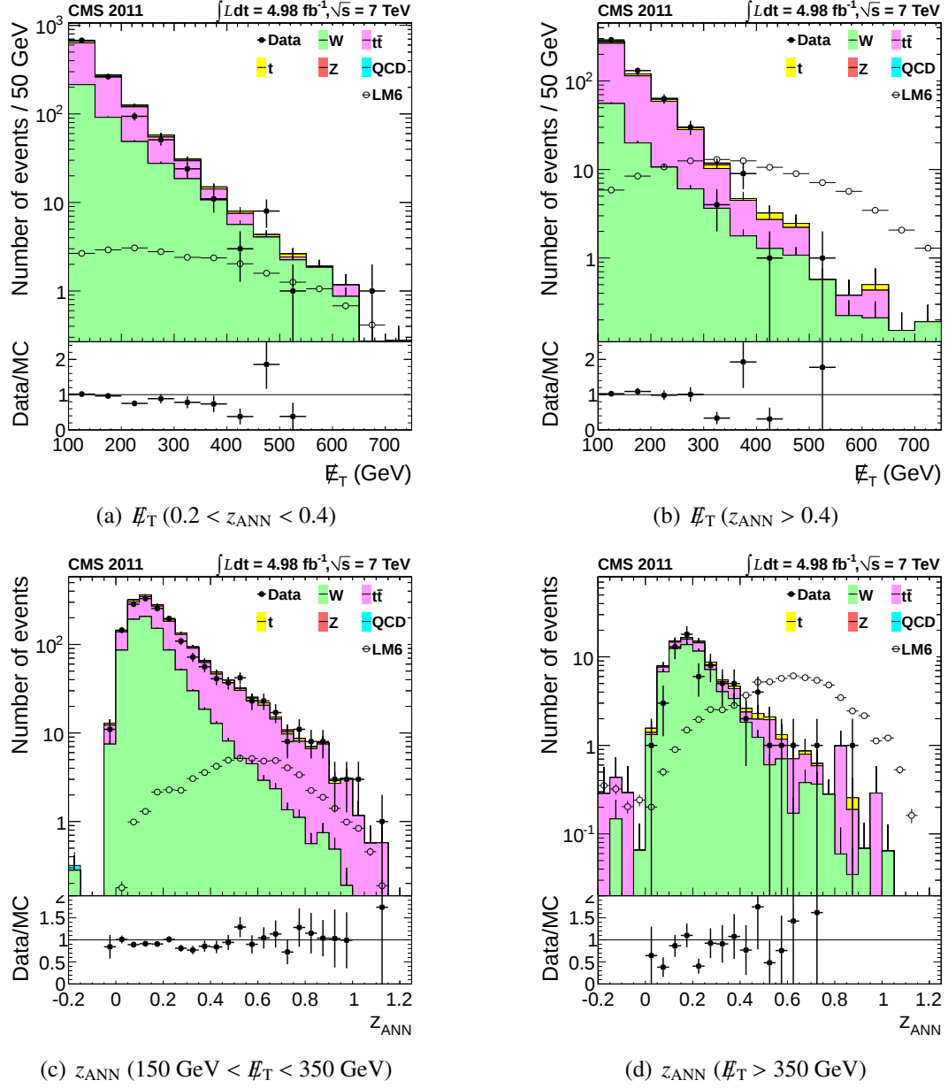
Figure 6.7: Distributions of E_T in slices of z_{\text{ANN}} (top) and z_{\text{ANN}} in slices of E_T (bottom) for data (solid circles), simulated SM (stacked shaded histograms), and simulated LM6 events (open circles). The small plot beneath each distribution shows the ratio of data to simulated SM yields.
