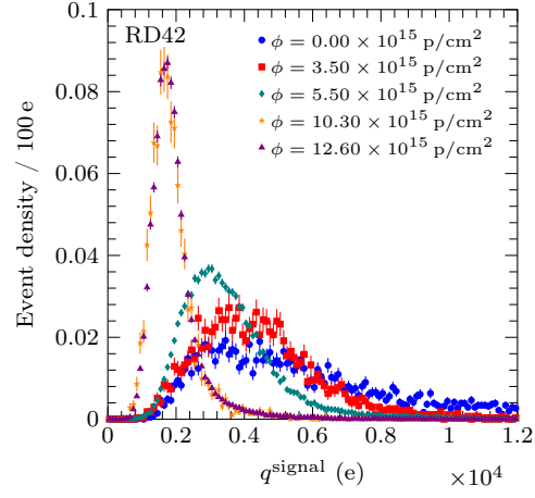
Figure 11.21: Pulse height distribution of pCVD diamond samples after different accumulated 800 MeV proton fluences. The electric bias field of the runs shown was set to -2 \text{ V}/\mu\text{m} . Each distribution's integral is scaled to unity.
