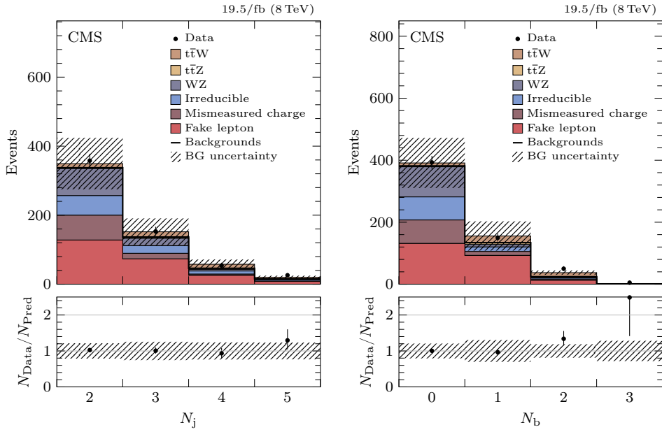
Figure 5.13: Jet multiplicity (left) and multiplicity of jets identified as b-jets (right) distributions after loose event selection requirements, as defined in section 5.1.3.
