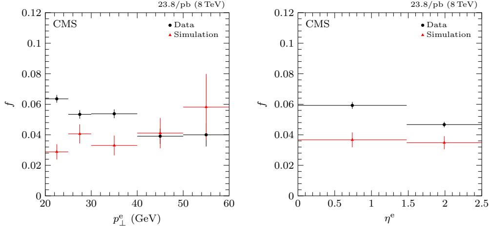
Figure 5.9: Misidentified electron ratios as a function of electron transverse momentum p_{\perp}^e (left) and pseudorapidity \eta^e (right) after correcting for contributions from electroweak processes.
