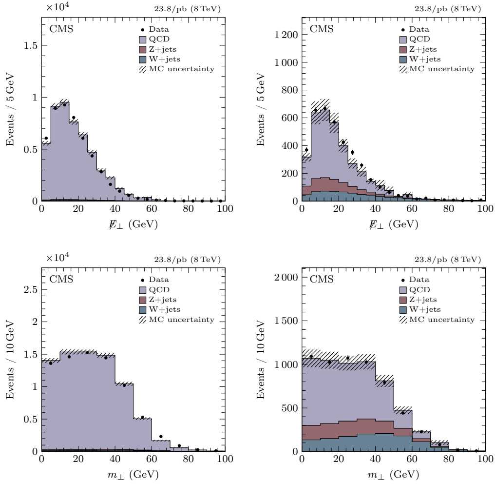
Figure 5.7: Missing transverse energy E_{\perp} (top row) and transverse mass m_{\perp} (bottom row) distributions for events selected by the fake control region, in which the electron passes the loose (left) and tight (right) criteria. The threshold on the plotted variable is released, respectively. The predictions of QCD events and electroweak processes are taken from MC simulations and fitted to data in a template fit.
