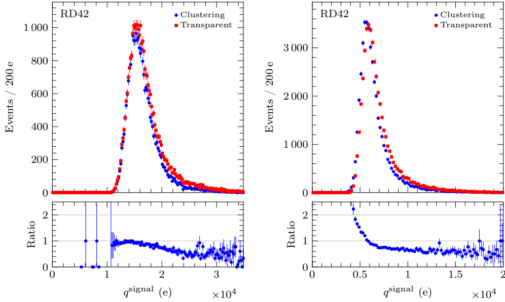
Figure 11.3: Signal charge distributions reconstructed with clustering and transparent algorithms before (left) and after (right) an 800 MeV proton fluence of (3.05 \pm 0.19) \times 10^{15} \text{ p/cm}^2 for the sCVD diamond sample PW205B.
