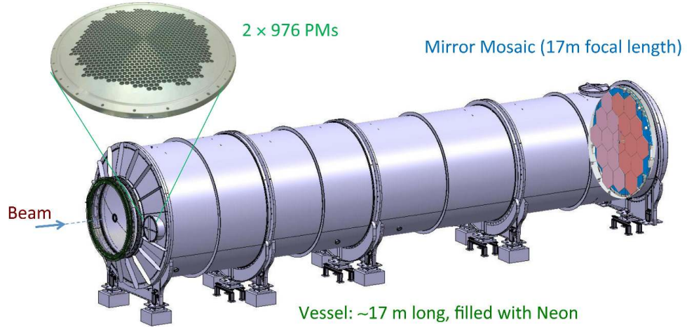
Figure 2.7 – Schematic view of the RICH detector [21].
