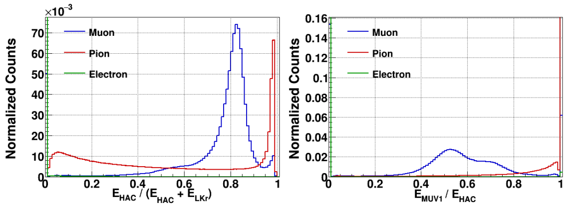
Figure 7.4 – Longitudinal development of the showers. On the left contribution of the HAC to the total energy collected in the calorimeters. On the right ratio between energy collected in the MUV1 with respect to the total energy in the HAC.
