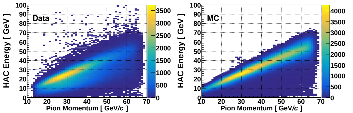
Figure 5.19 – Energy collected in the HAC as a function of the pion momentum for data (left) and MC (right).
