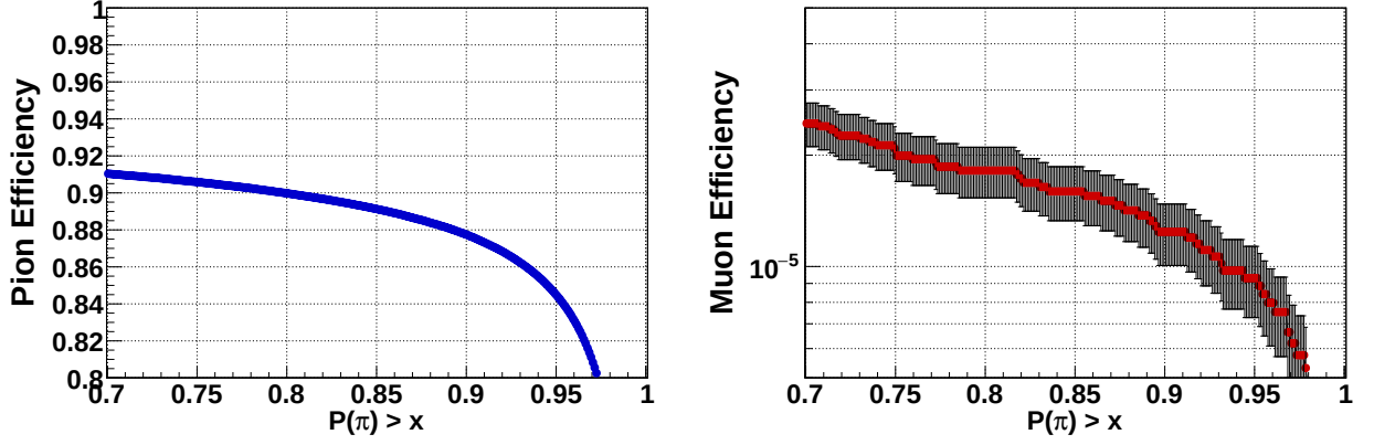
Figure 7.19 – Pion and muon efficiencies as function of the required lower limit on the classifier response for the pion identification probability.
