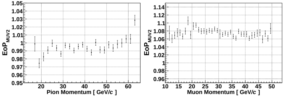
Figure 5.35 – Result of MUV2 energy calibration on pions (left) and muons (right).
