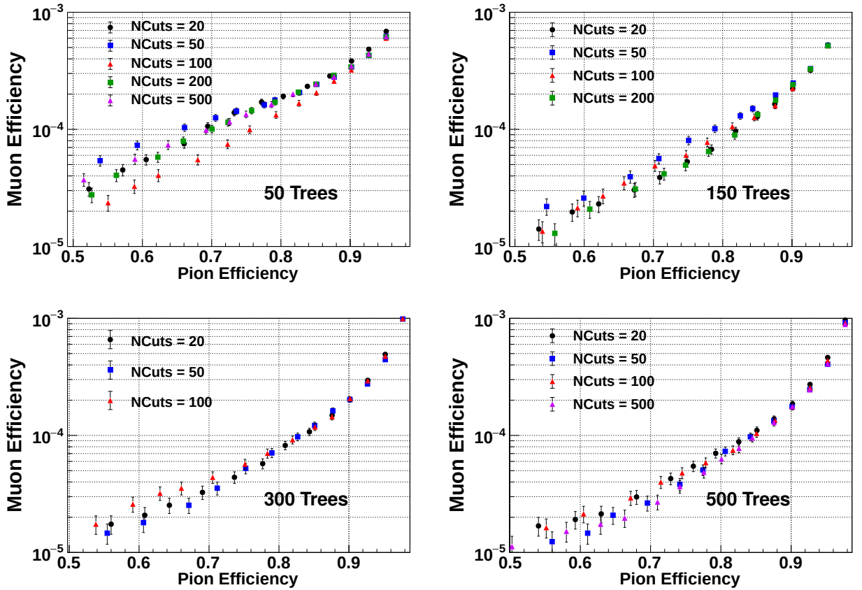
Figure 7.9 – Muon efficiency as function of the pion efficiency when varying the \text{Ncuts} parameter for 50, 150, 300 and 500 trees forests.
