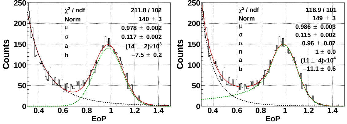
Figure 5.11 – Example of EoP distribution fits for 20 GeV/c muons showering inside the MUV1. On the left using a gaussian to describe the peak, on the right a Crystal Ball function.
