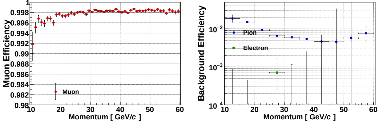
Figure 7.14 – Muon, pion and electron efficiencies as function of the momentum for P(\mu) > 0.8 .
