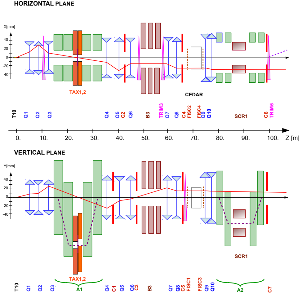
Figure 2.2 – Scheme of K12 beam line: the lines shows the trajectory followed by a 75 GeV/c positively charged particle when produced on-axis (dashed-black) and with the limiting angles of 2.7 mrad horizontal and 1.5 mrad vertical (solid-red) [21].
