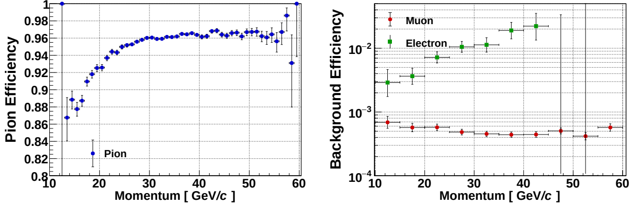
Figure 7.12 – Pion, muon and electron efficiencies as function of the momentum for P(\pi) > 0.8 .
