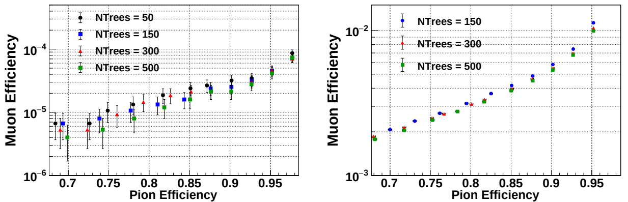
Figure 7.10 – Muon efficiency as function of the pion efficiency, including MUV3 veto contribution, for different forest sizes: on the left for the Control Trigger data and on the right for the data from the physics trigger mask 1.
