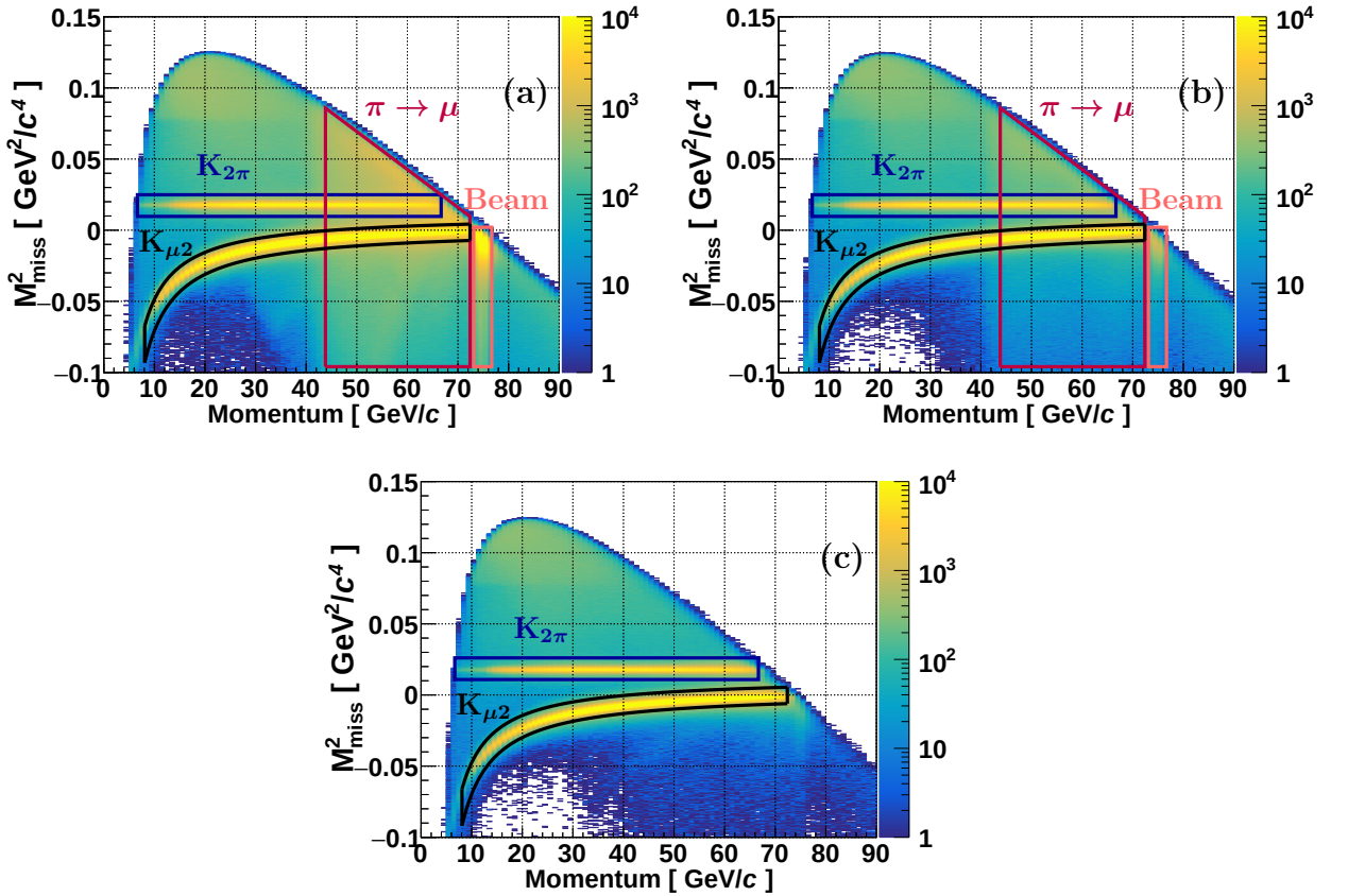
Figure 6.7 – Distribution of M^2_{\text{miss}} (evaluated using the GTK information) as function of the track momentum: after the single track selection (a), requiring the vertex inside the fiducial region (b) and with the kaon identification (c). The main kaon decays as well as the beam pions decay and scattering on the last GTK station are shown by coloured boxes.
