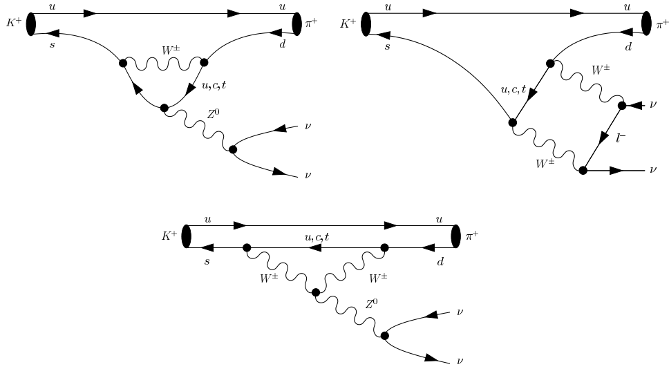
Figure 1.3 – Feynman diagrams of the K^+ \rightarrow \pi^+ \nu \bar{\nu} decay [14]. The K_L \rightarrow \pi^0 \nu \bar{\nu} process is described by the same diagrams, where the spectator quark is changed from u to d .
