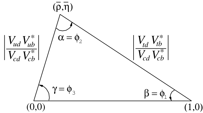
Figure 1.2 – Unitarity Triangle [12].
