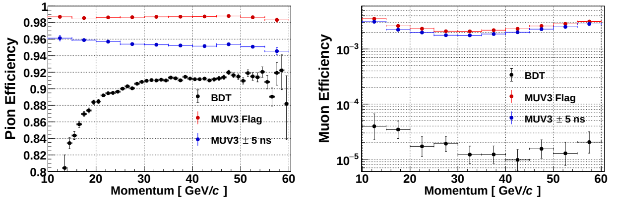
Figure 7.20 – Pion and muon efficiencies as function of the momentum after applying a MUV3 veto and with the pion identification with the calorimeters ( P(\pi) > 0.8 ).
