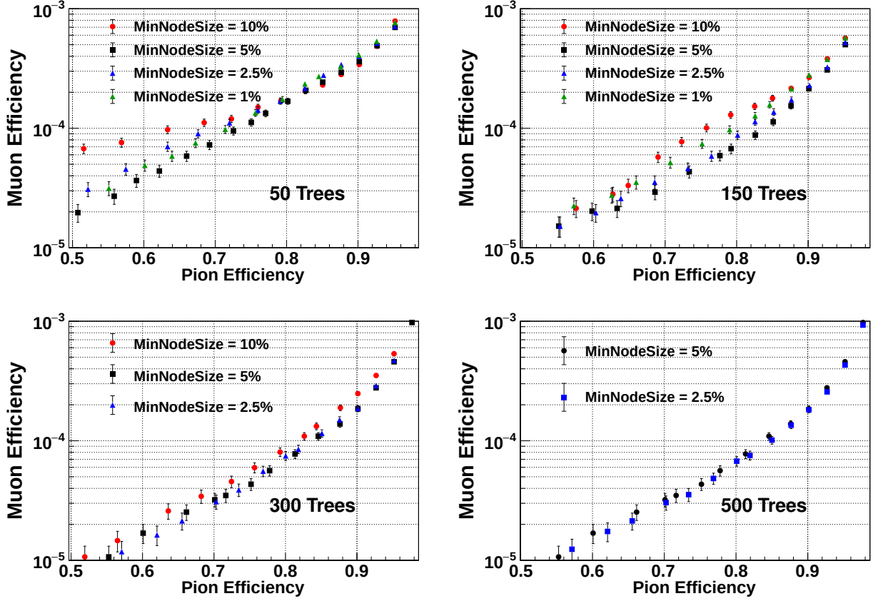
Figure 7.8 – Muon efficiency as function of the pion efficiency when varying the MinNodeSize parameter for forests with 50, 150, 300, and 500 trees.
