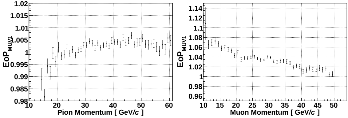
Figure 5.32 – Result of the energy calibration on pions (left) and muons (right).
