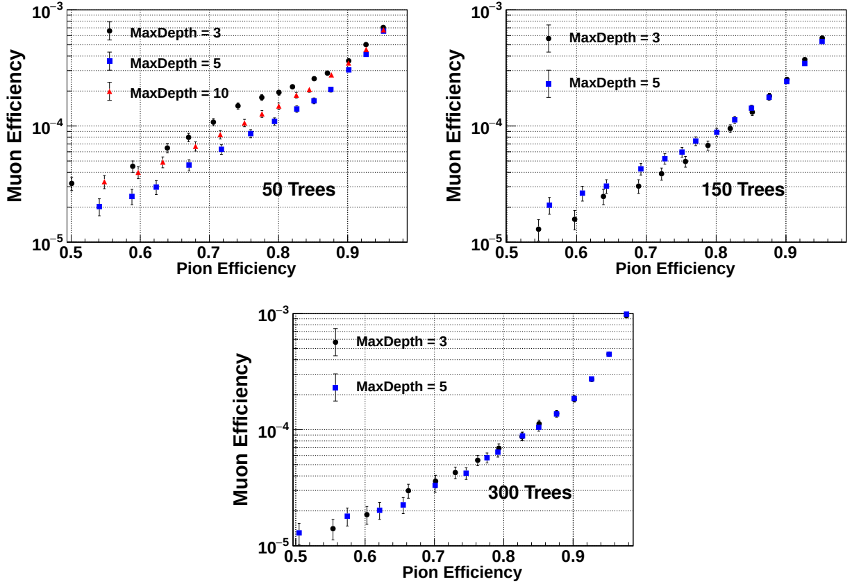
Figure 7.7 – Muon efficiency as a function of the pion efficiency when varying the MaxDepth parameter for forests with 50, 150 and 300 trees.
