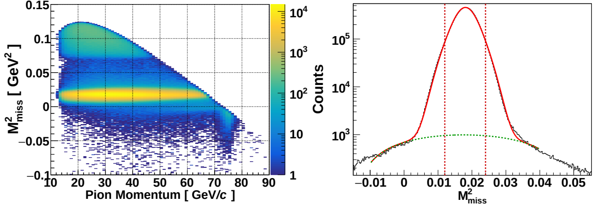
Figure 5.18 – Distribution of the kinematic parameter M_{miss}^2 = (P_K - P_{\pi+})^2 for selected K_{2\pi} events on data, as a function of the momentum (left) and estimation of the background (right). The red lines indicate to selection cuts.
