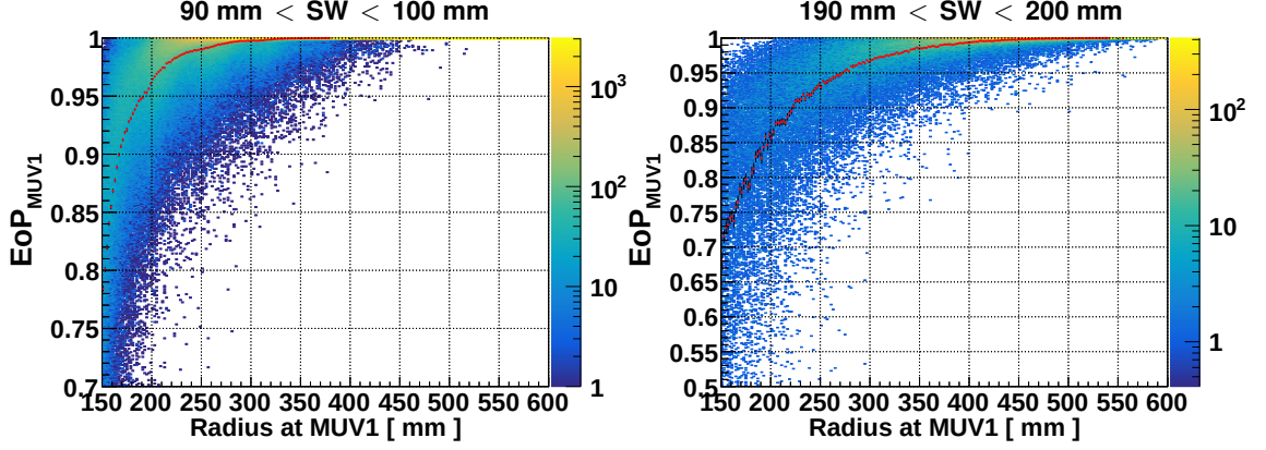
Figure 5.25 – Fraction of the energy released reconstructed in the MUV1 as a function of the radial impact position for showers of different shower widths (SW). The red points are the mean of the distribution in each bin.
