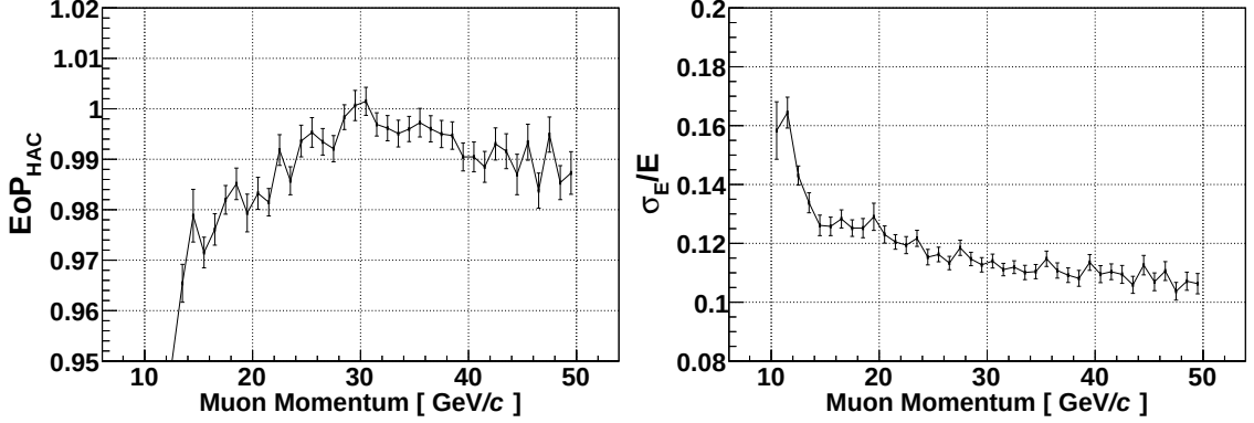
Figure 5.17 – Left: fraction of reconstructed energy in the HAC for stopped muons after all corrections. Right: width of the muon signal from the Crystal Ball fit which is an estimate of the energy resolution of electromagnetic showers.
