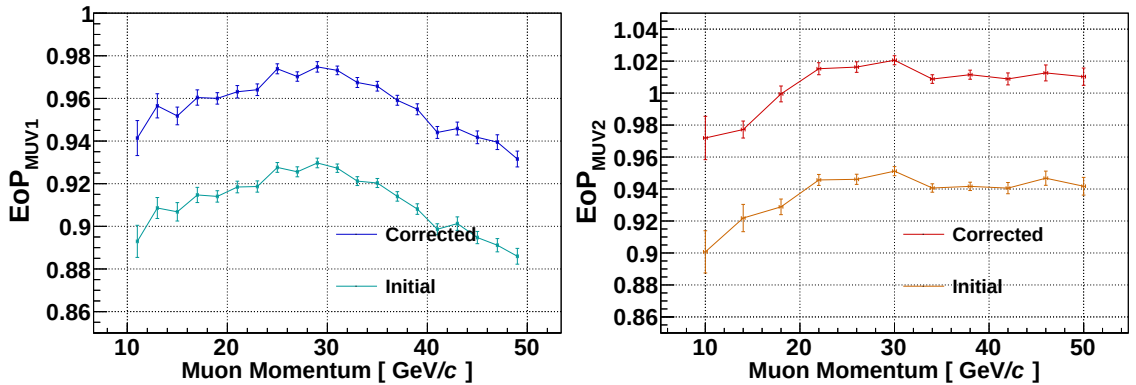
Figure 5.14 – Distributions of EoP as a function of the muon momentum for MUV1 (on the left) and MUV2 (on the right) before and after the correction due to the scintillators orientation.
