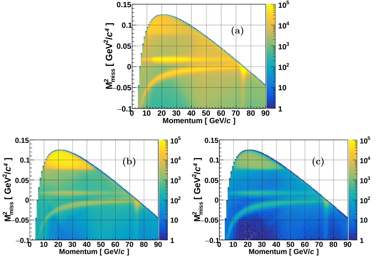
Figure 6.2 – Squared missing mass as function of the momentum for well-reconstructed tracks: (a) selecting as having CDA > 10 mm with any other track; (b) for those rejected because having a CDA smaller than 10 mm with another well-reconstructed track; (c) for those rejected because having CDA < 10 mm with a track not classified as well-reconstructed and both tracks having CDA < 30 mm with respect to the beam axis.
