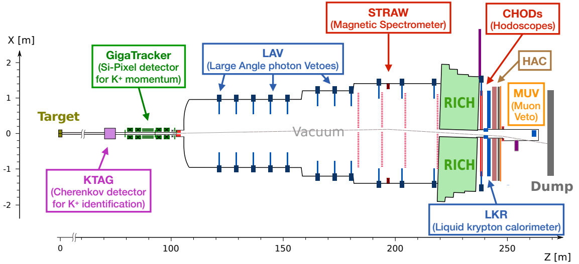
Figure 2.3 – Scheme of the NA62 apparatus [21].
