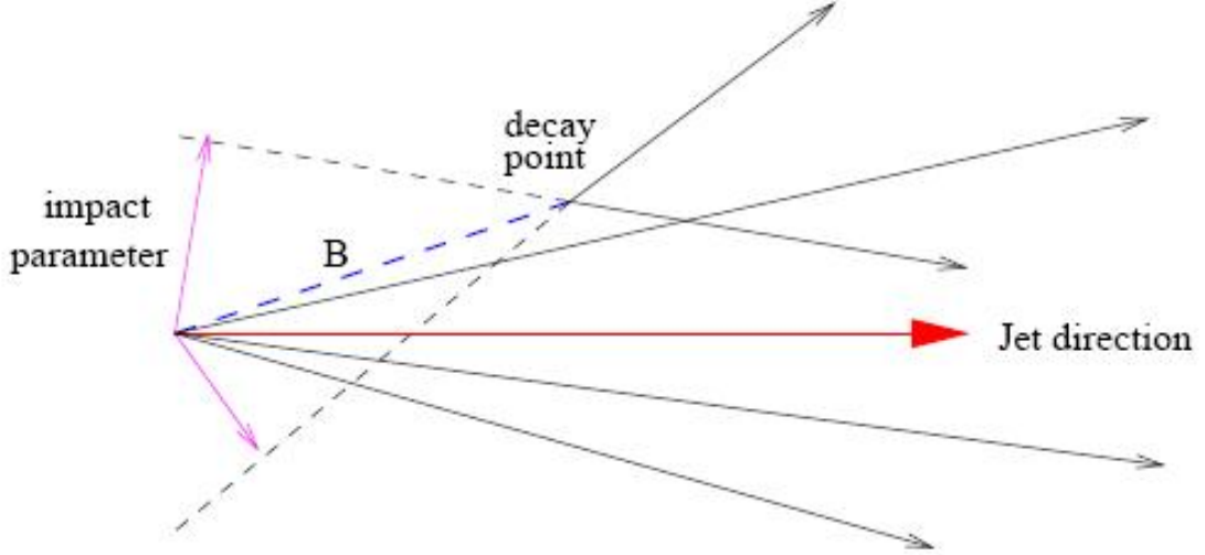
Figure 4.3: Representation of an hadronic jet originating from a b -quark.
