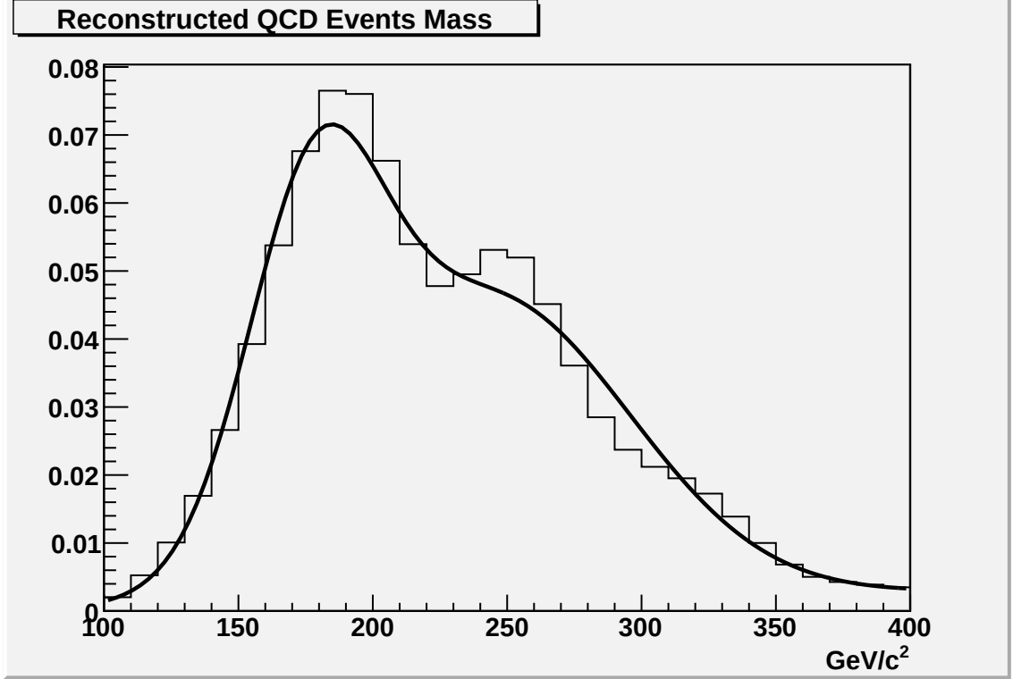
Figure 7.5: Background reconstructed with the kinematical fitter with fit superimposed. Events with at least 1 b-tag.
