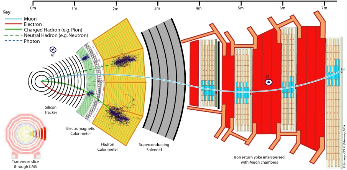
Figure 4.2: Particle tracks in the CMS slice.
