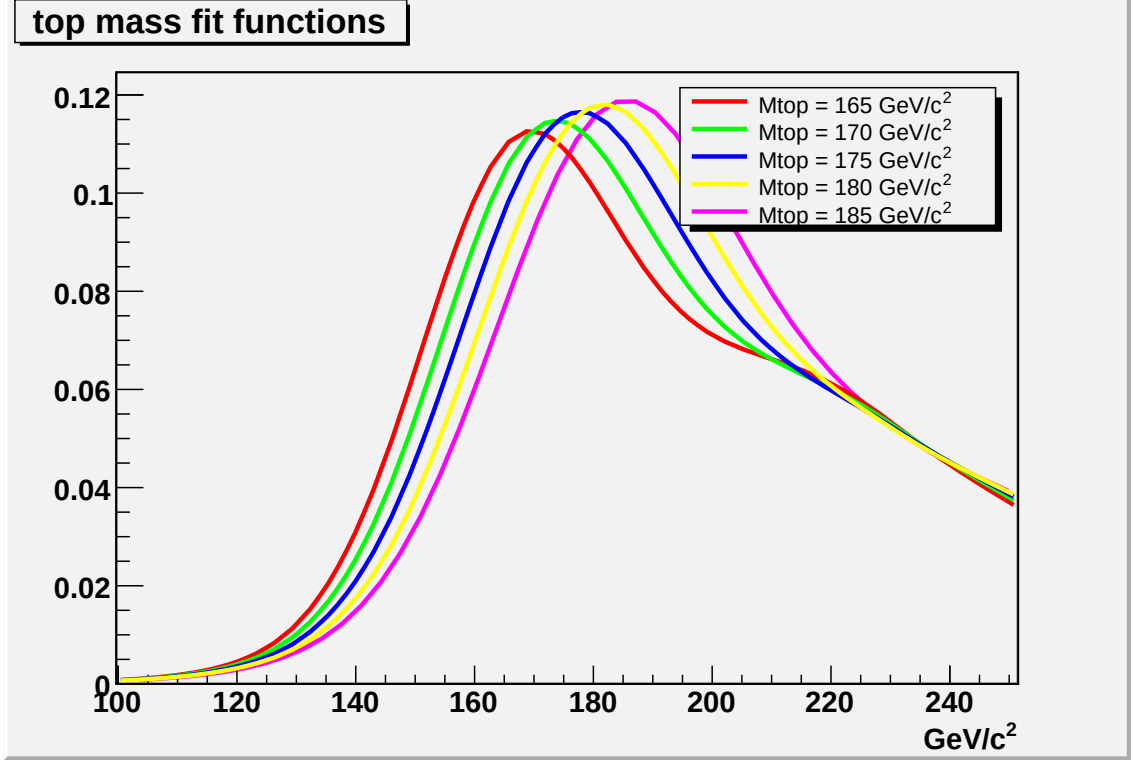
Figure 7.3: Evolution of the fit function for some of the reconstructed masses for events with at least 1 b-tag.
