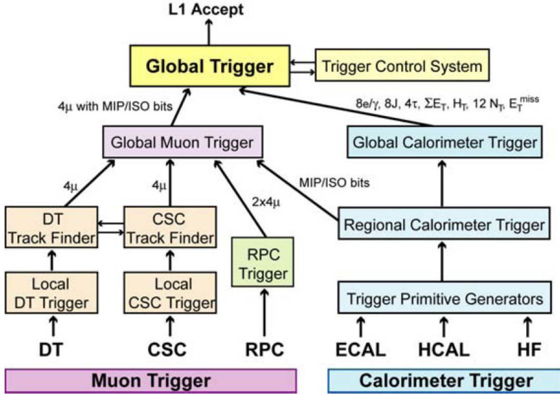
Figure 1.5: The architecture of the L1T
