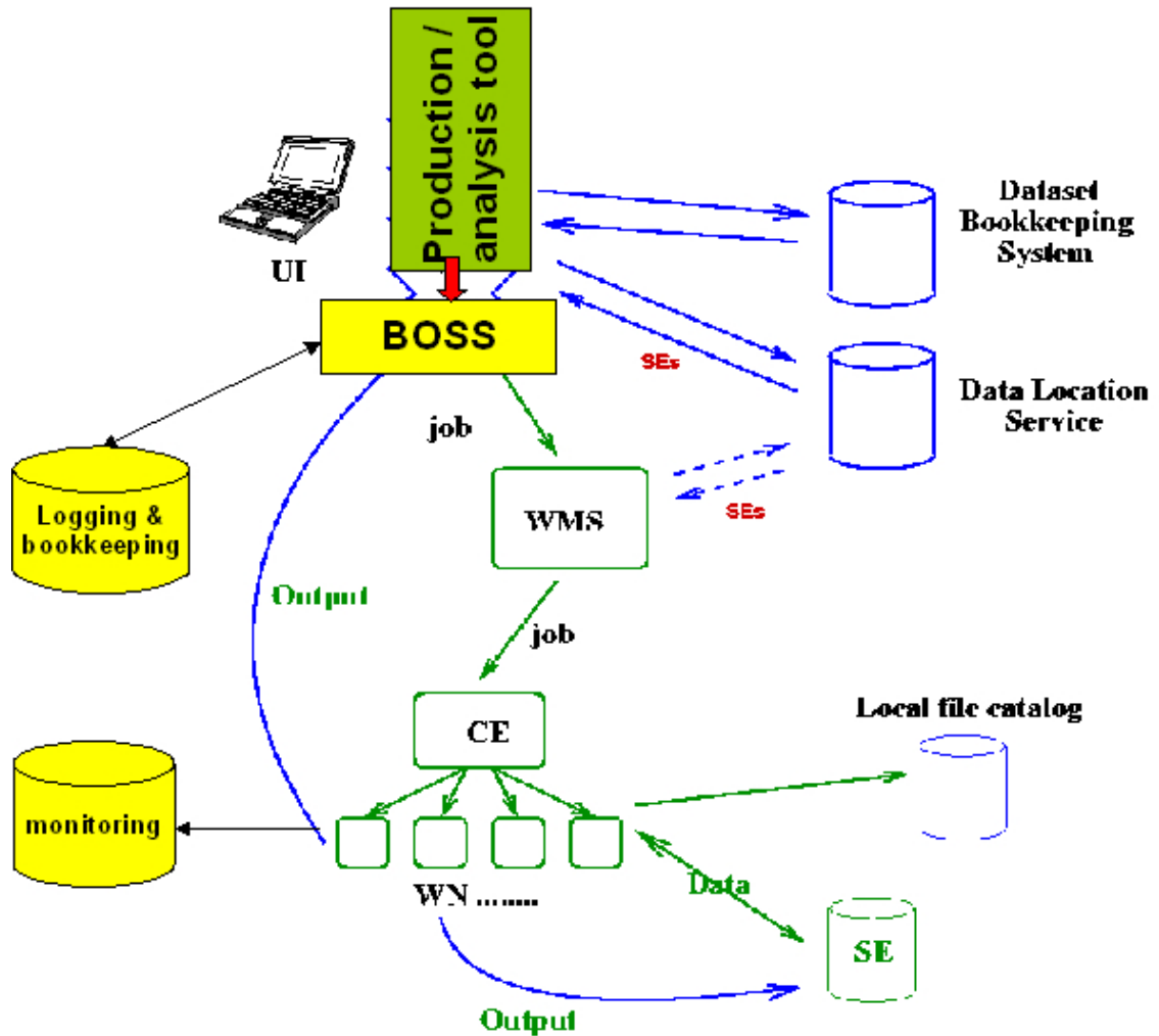
Figure 2.6: BOSS in the analysis/production system.
