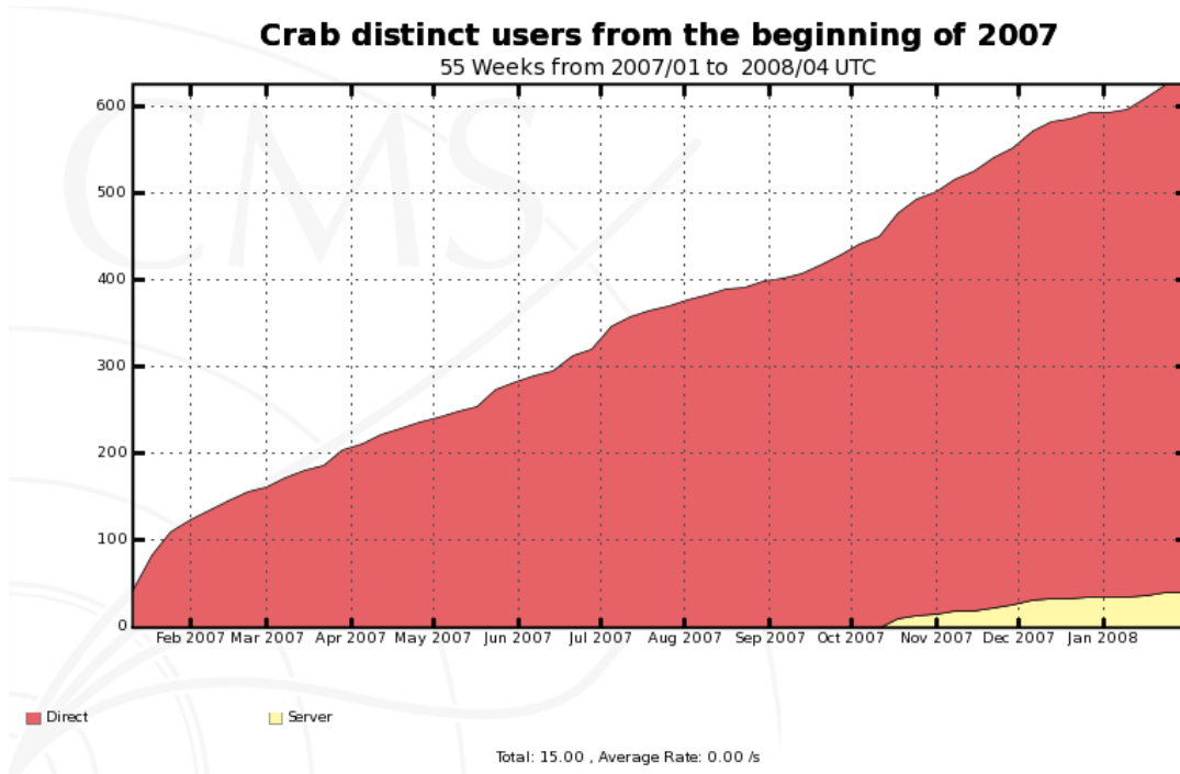
Figure 2.8: Crab usage in 2007 in term of user number.
