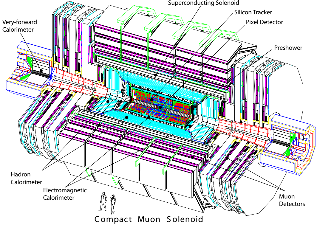
Figure 1.4: A CMS exploded view
