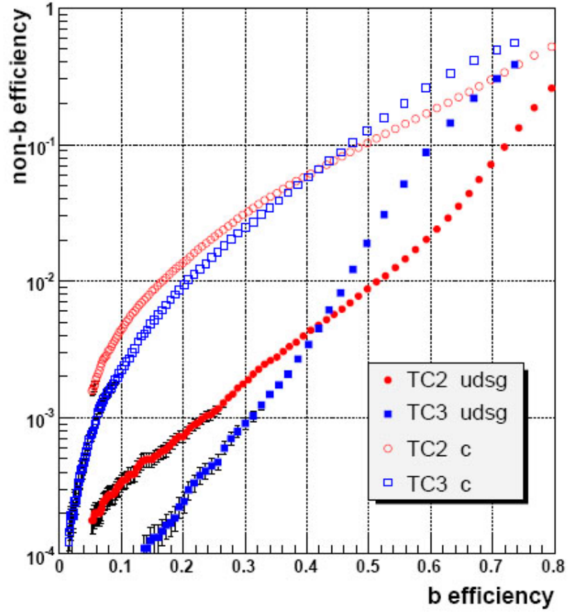
Figure 6.5: Performance of the Track Counting in the QCD 80-120 Monte Carlo sample requiring two (TC2) or three (TC3) tracks with a given impact parameter significance.
