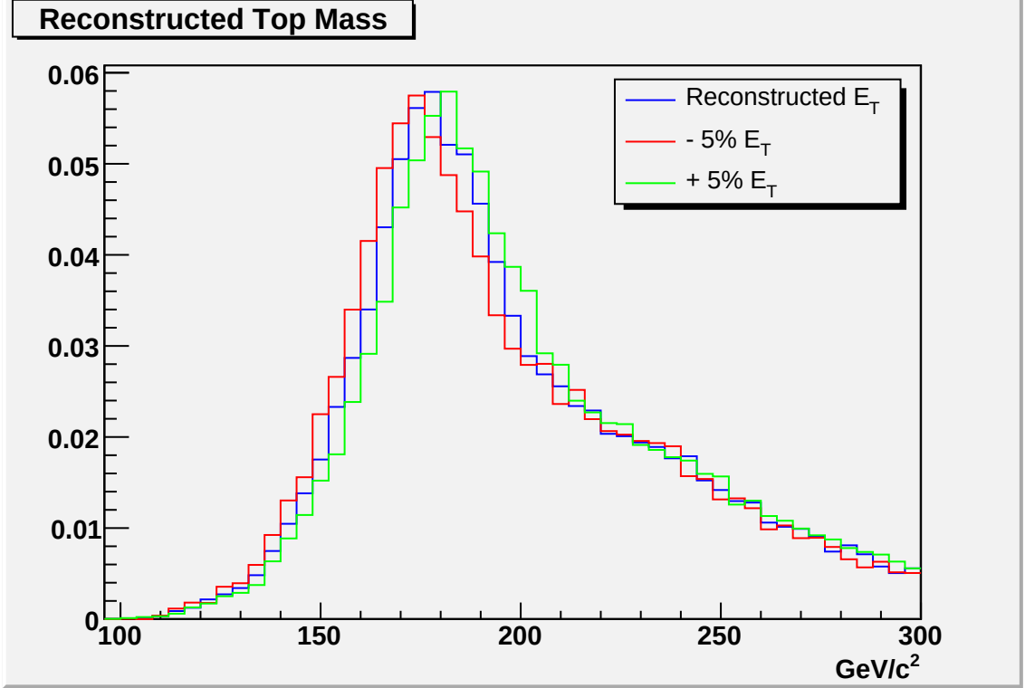
Figure 7.10: Reconstructed top mass for signal samples by increasing and decreasing each jet energy by 5% for sample generated with mass 175 \text{ GeV}/c^2 . Events with at least 1 b-tag.
