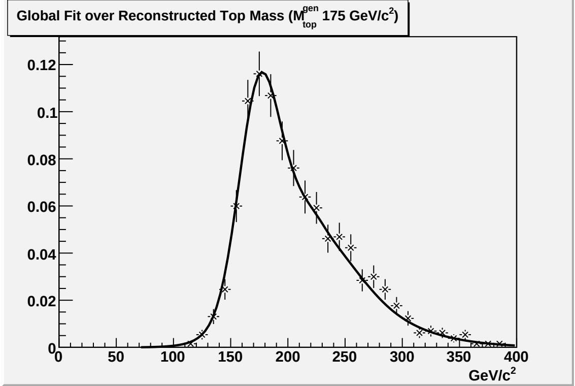
Figure 7.4: Reconstructed top mass for signal samples generated with mass from 175 \text{ GeV}/c^2 with global fit superimposed. Events with at least 1 b-tag.
