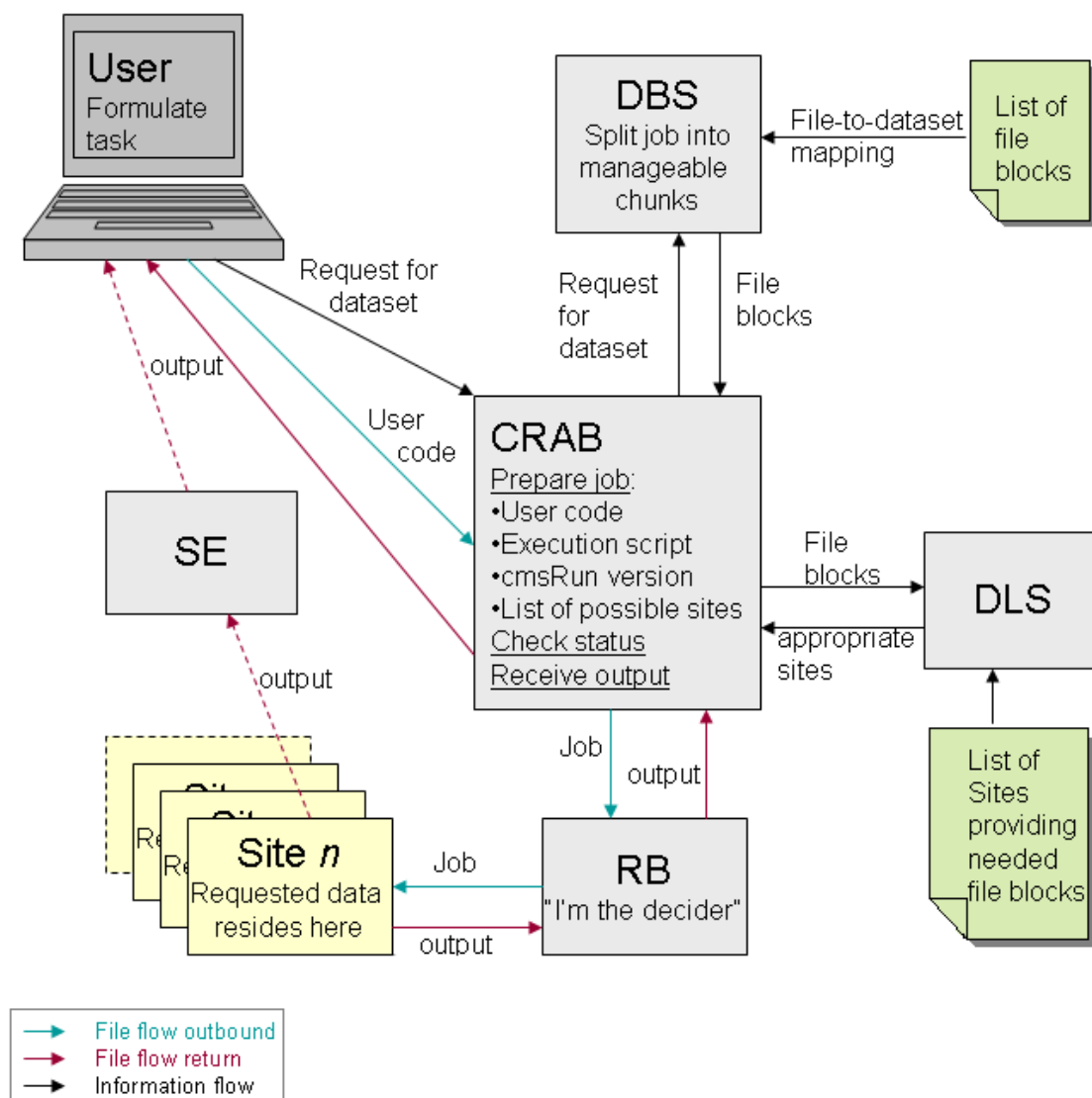
Figure 2.5: Crab Workflow.
