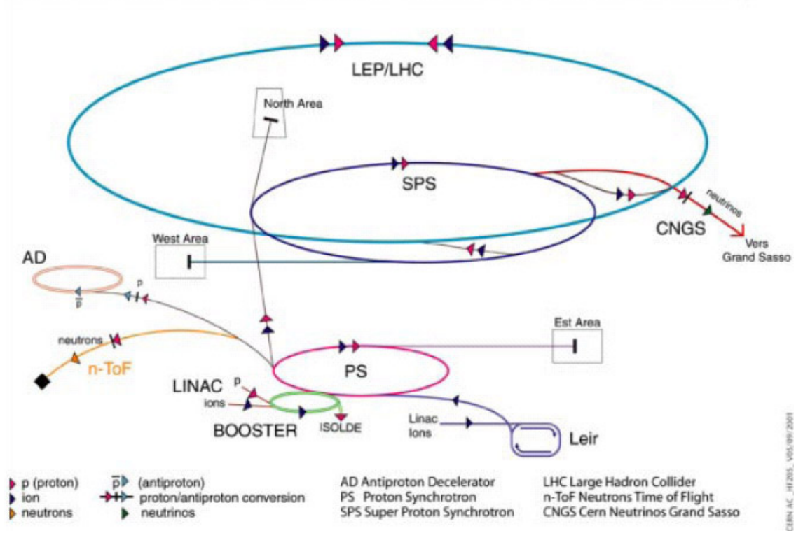
Figure 1.2: LHC injection system: protons are produced by ionization of hydrogen and injected with an energy of 750 keV in the linear accelerator (LINAC2) through a radiofrequency quadrupole where they reach the energy of 50 MeV, then in the BOOSTER, where they are rearranged in packets of approximatively 10^{11} protons of 1.4 GeV, then in the PS up to 25 GeV and finally in the SPS which will inject them at 450 GeV in the LHC.
