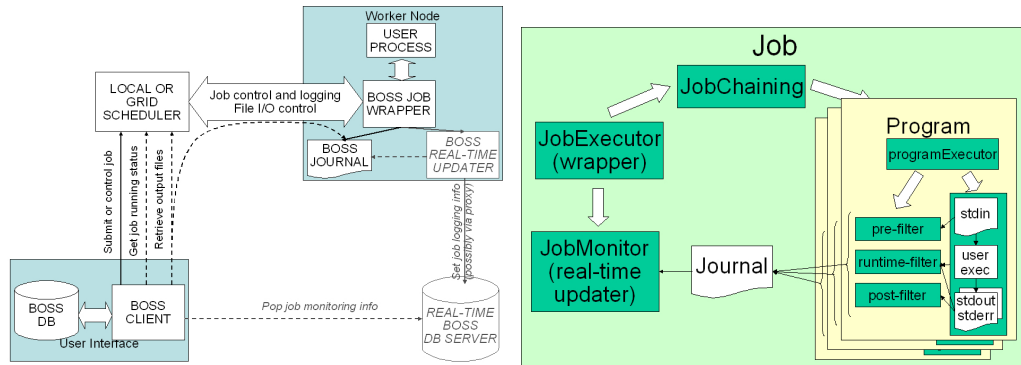
Figure 2.7: The BOSS workflow: the left picture shows the detailed workflow of a job in the execution host.
