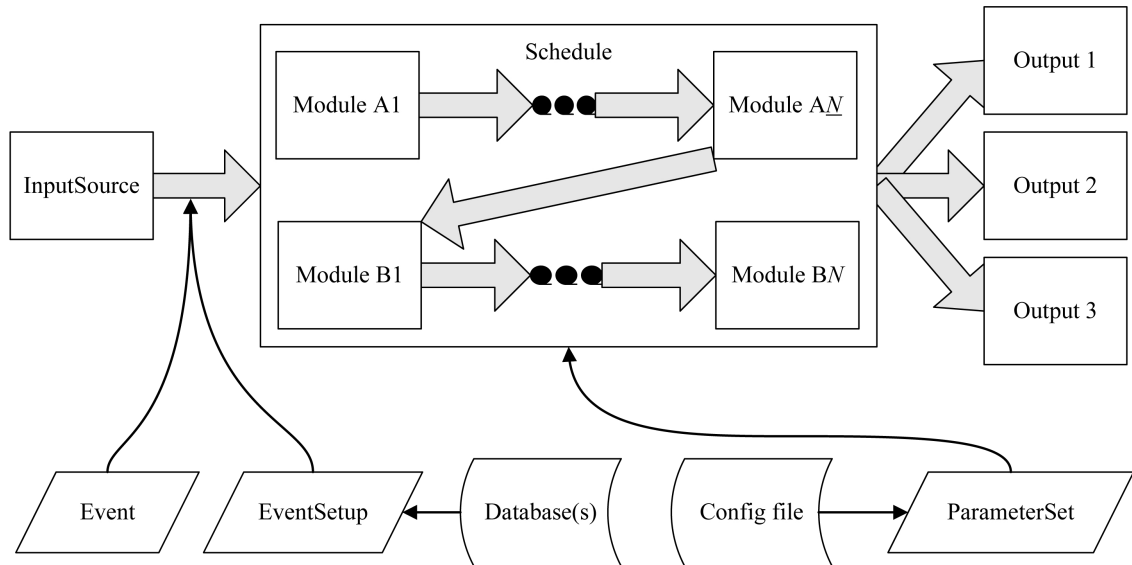
Figure 2.3: Components of the CMS Framework and Event Data Model.
