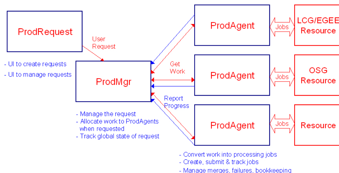
Figure 2.4: The Monte Carlo Production system.
