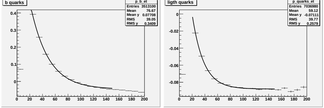
Figure 4.1: E_T deviation of b-jets and light quarks jets from the generated partons E_T .
