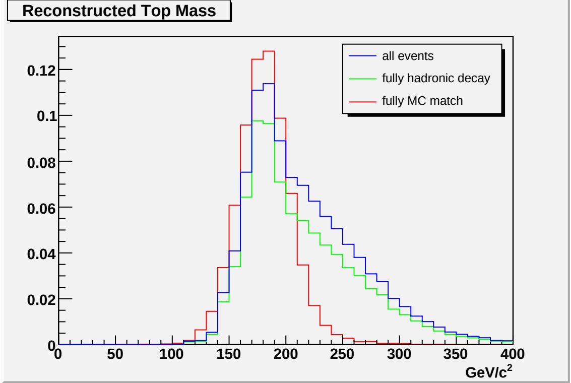
Figure 7.1: Reconstructed top mass for the full sample compared with the subset of fully hadronics events (from Monte Carlo truth) and the subset of events where jets are fully matched with the generated partons. All distribution are normalized to the same area.
