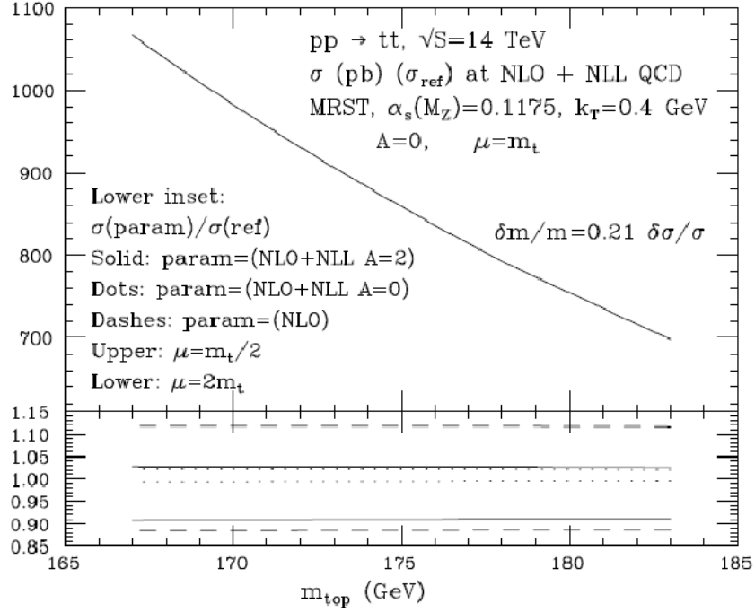
Figure 3.1: Production cross section calculated for top pair production at LHC [30].
