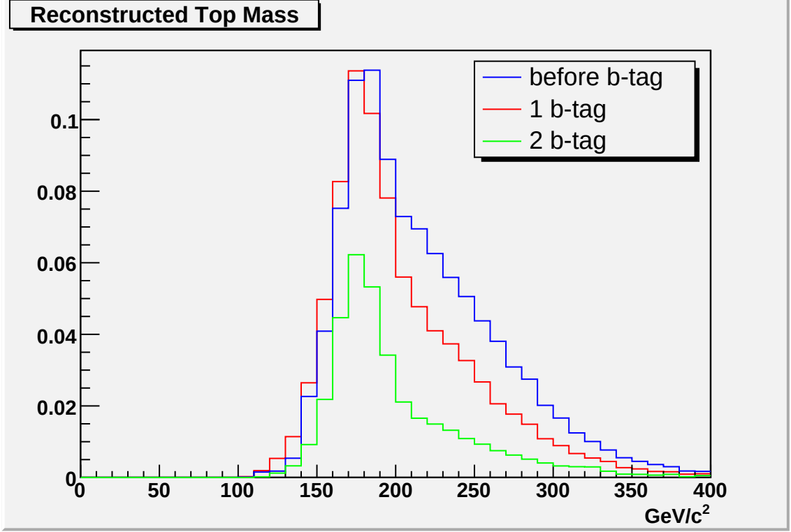
Figure 7.2: Reconstructed top mass without requiring b-tag, requiring at least 1 b-tag and at least 2 b-tag. Both distribution are normalized to the same area.
