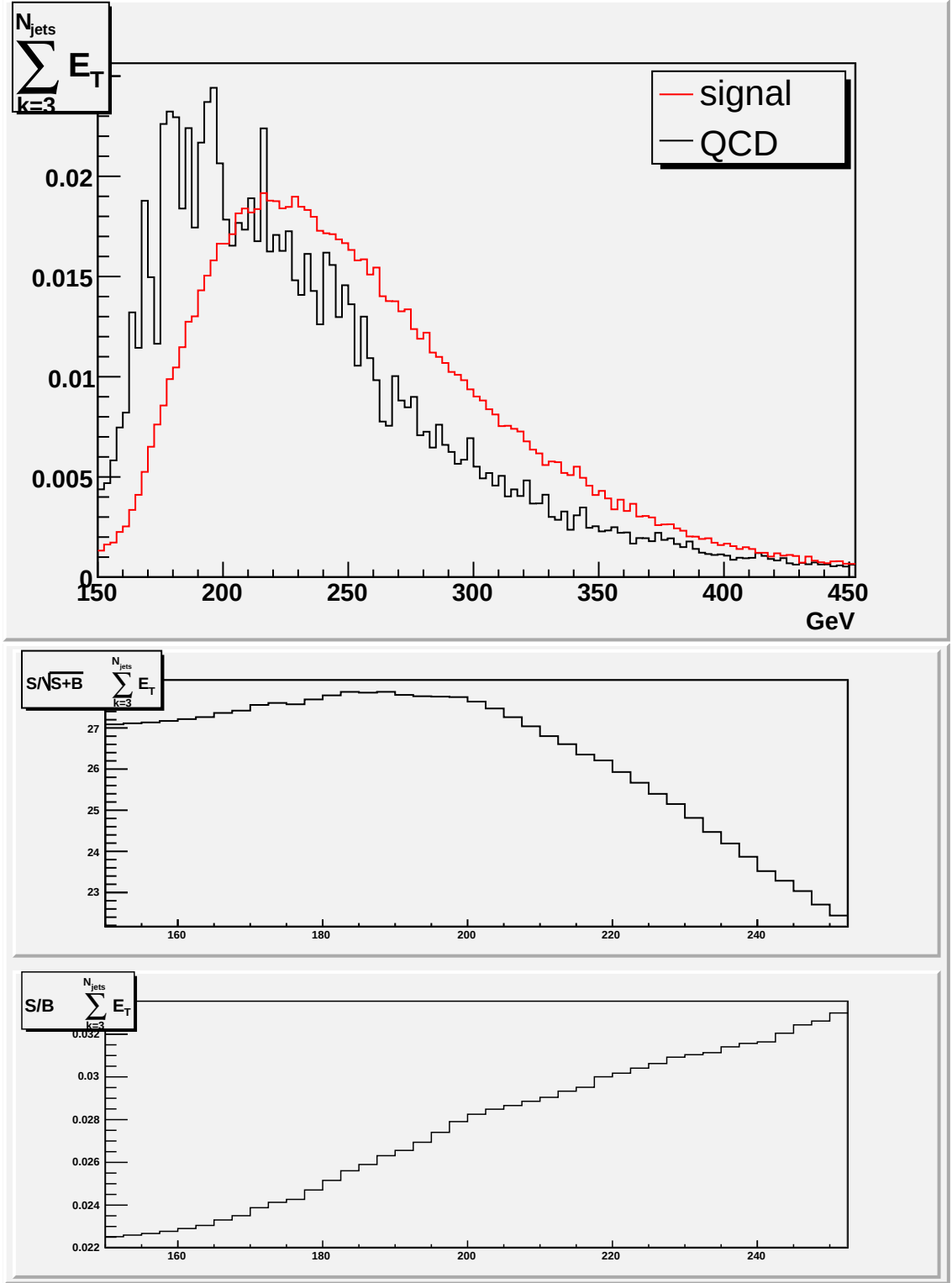
Figure 6.2: Distributions of \sum_{k=3}^{N_{\text{jets}}} E_T for t\bar{t} (top) and QCD (bottom) events and related S/B and \frac{S}{\sqrt{S+B}} .
