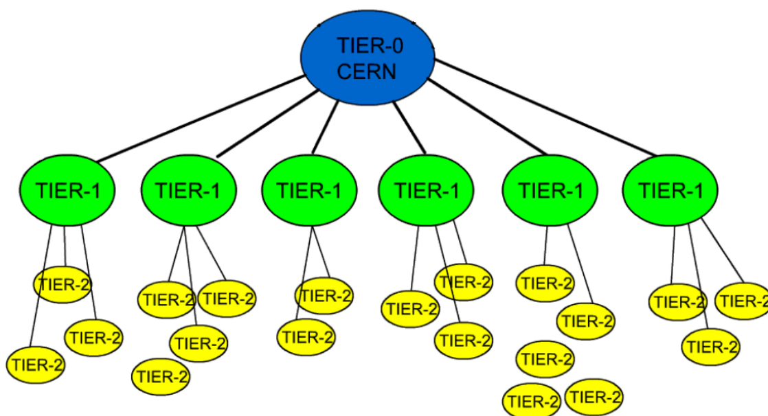
Figure 2.1: The Tier architecture.
