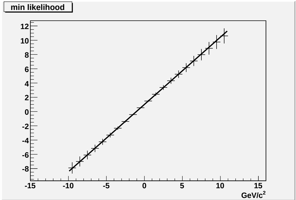
Figure 7.7: Measured vs. generated top quark mass assuming no background. A linear fit is superimposed.
