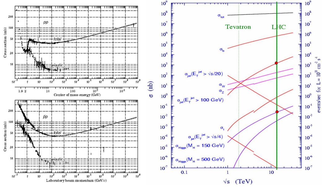
Figure 1.3: The pp cross section compared with the p\bar{p} cross section: while at lower center of mass energy it is lower for pp interactions, at higher energies they are pretty equal, since the partons interactions are dominant. The second plot shows the cross section for some relevant process for both Tevatron and LHC at low luminosity.
