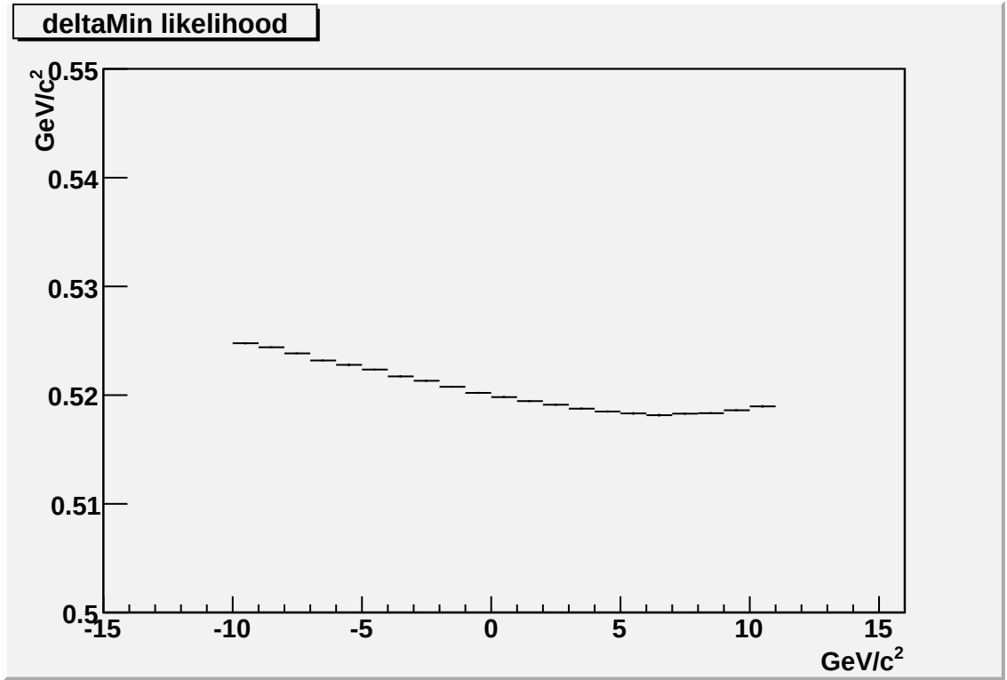
Figure 7.9: Statistical uncertainty as a function of (M_{top} - 175) \text{ GeV}/c^2 , calculated as 1/2(M^+ - M^-) .
