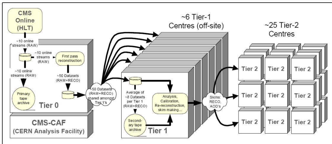
Figure 2.2: Data flow.
