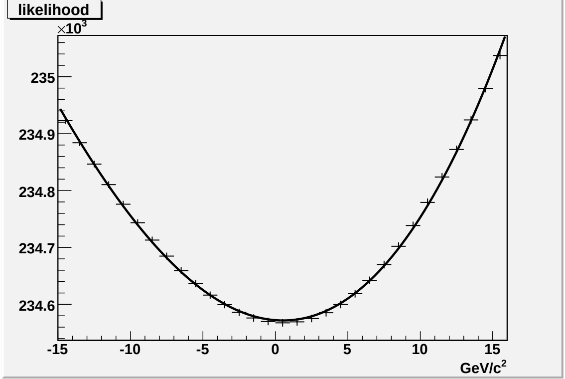
Figure 7.6: Likelihood evaluated for signal sample generated with mass 175 \text{ GeV}/c^2 . Events with at least 1 b-tag.
