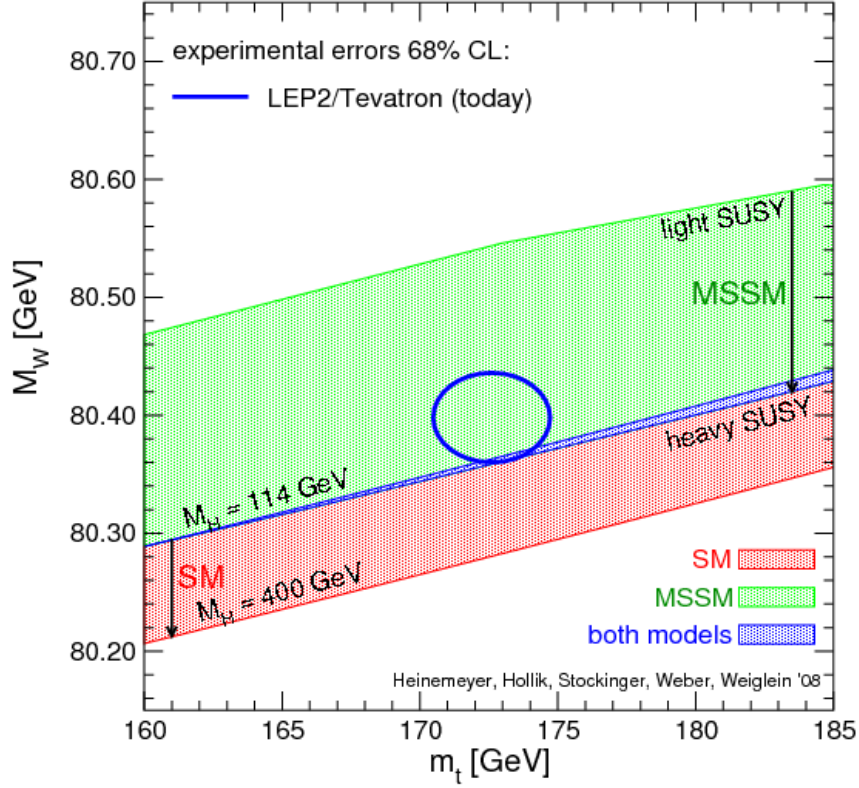
Figure 3.2: W and top quark masses measurements with prediction for different Higgs masses.
