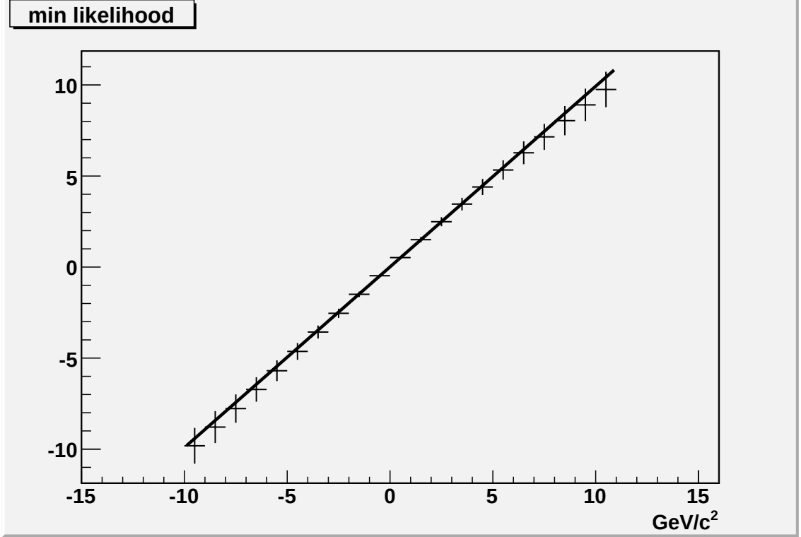
Figure 7.8: Measured vs. generated top quark mass using the background according to the expected S/B ratio. A linear fit is superimposed.
