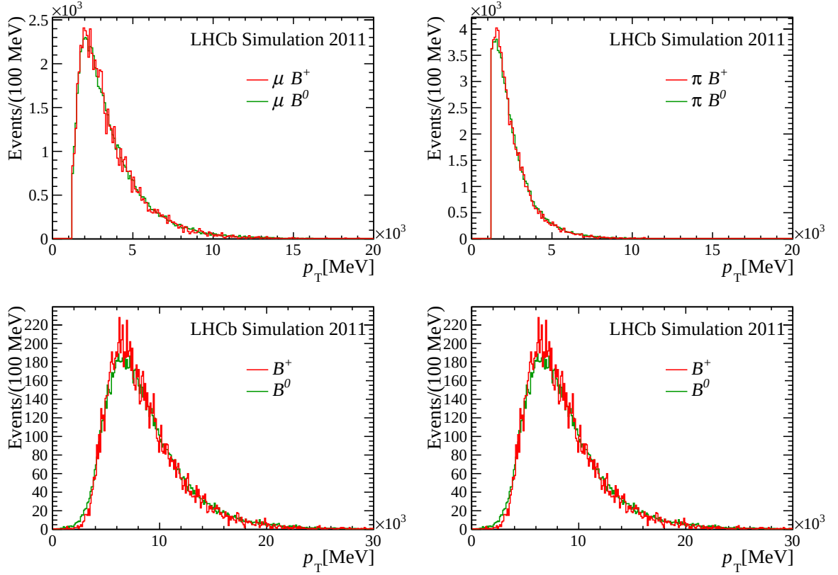
Figure 8.2: Muon and highest p_T pion transverse momenta spectra, reconstructed B meson momentum and p_T for B^0 \rightarrow D^- \mu^+ \nu_\mu X and B^+ \rightarrow D^+ \mu^- X^+ simulated events with 2011 conditions. The \mu\pi kinematical weights discussed in Sec 6.5.1 are not applied for these plots.
