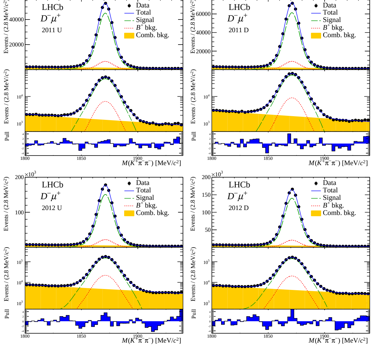
Figure B.1: Invariant mass distributions of the K^{\mp}\pi^{\pm}\pi^{\pm} combinations. The fit results are overlaid to the distribution of the dataset of each year and magnet polarity. The data distributions shown are obtained after applying the kinematical weights (see Sec. 6.5.1). For each subsample, the first two top rows show the invariant mass distributions using a linear and a logarithmic y-axis, respectively. The last row shows the so-called Pull values, i.e. the difference between the number of events observed in data for each bin of the histogram and the number of events predicted by the model in the same bin, divided by the uncertainty on the number of events.
