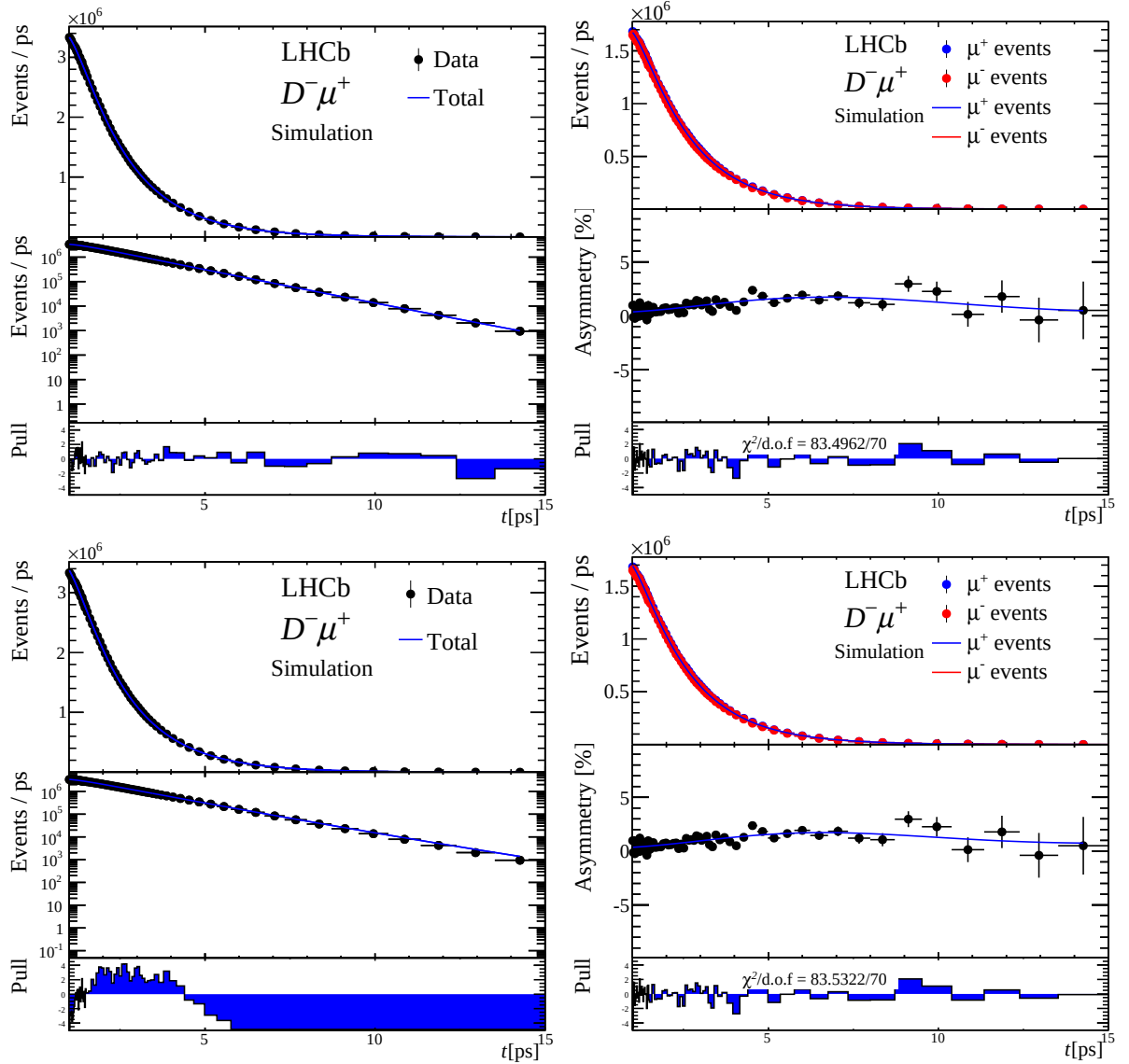
Figure 9.5: High statistics pseudo-experiment generated with a quadratic acceptance model and fitted with quadratic acceptance shape ( top ) and the nominal PDF used for the a_{sl}^d fits ( bottom ). Decay time projections ( left ) and charge asymmetry projections ( right ). The quadratic shape is modeled with realistic parameters (see Sec. 9.1.5), hence the effect is evident only in the pull distributions. In spite of the evident effect in the decay time projection, the effect has negligible impact on the charge asymmetry.
