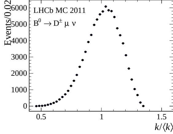
Figure 7.12: k/\langle k \rangle distribution. B^0 \rightarrow D^- \mu^+ \nu_\mu X simulated events with 2011 conditions.
