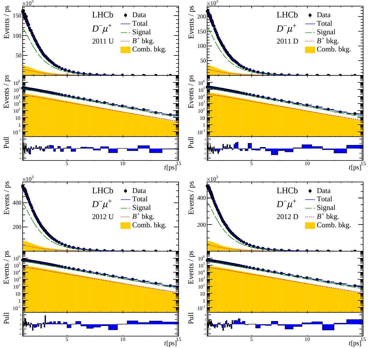
Figure B.2: B decay time distributions. The fit results are overlaid to the distribution of the dataset of each year and magnet polarity. The data distributions shown are obtained after applying the kinematical weights (see Sec. 6.5.1). For each subsample, the first two top rows show the B decay time using a linear and a logarithmic scale. The different components of the sample are highlighted with different colors and styles. The last row shows the so-called Pull values, i.e. the difference between the number of events observed in data for each bin of the histogram and the number of events predicted by the full model in the same bin, divided by the uncertainty on the number of events.
