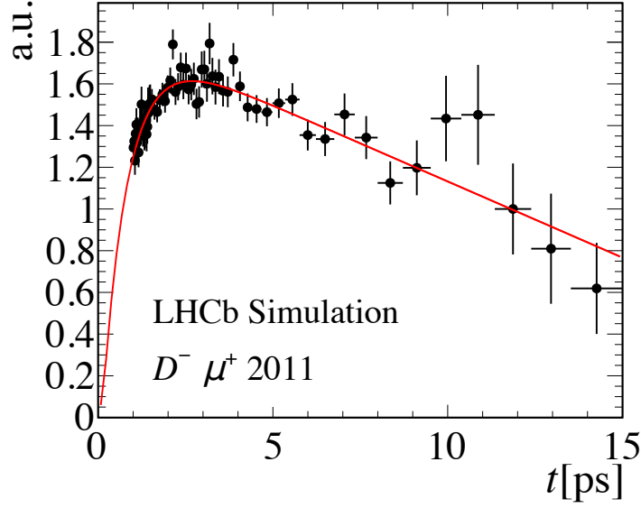
Figure 7.16: Ratio of the reconstructed and true B decay time distributions for B^0 \rightarrow D^- \mu^+ \nu_\mu X simulated events with 2011 conditions. Acceptance function 7.22 overlaid.
