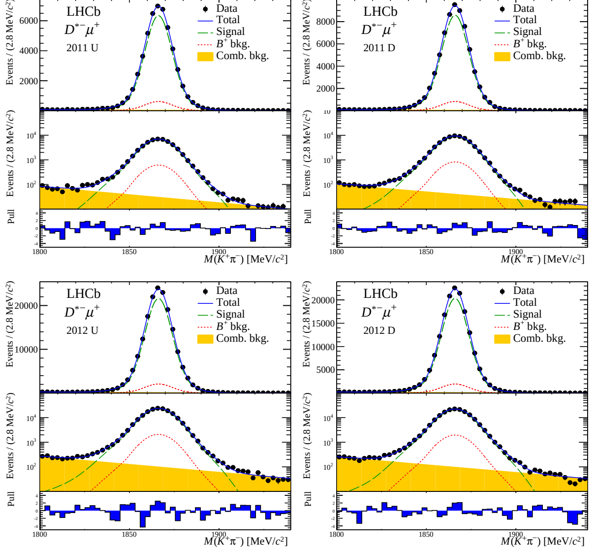
Figure B.5: Invariant mass distributions of the K^\mp\pi^\pm combinations. The fit results are overlaid to the distribution of the dataset of each year and magnet polarity. All the data distributions shown are obtained after applying the kinematical weights (see Sec. 6.5.1). For each subsample, the first two top rows show the invariant mass distributions using a logarithmic and a not-logarithmic y-axis, respectively. The last row shows the so-called Pull values, i.e. the difference between the number of events observed in data for each bin of the histogram and the number of events predicted by the model in the same bin, divided by the uncertainty on the number of events.
