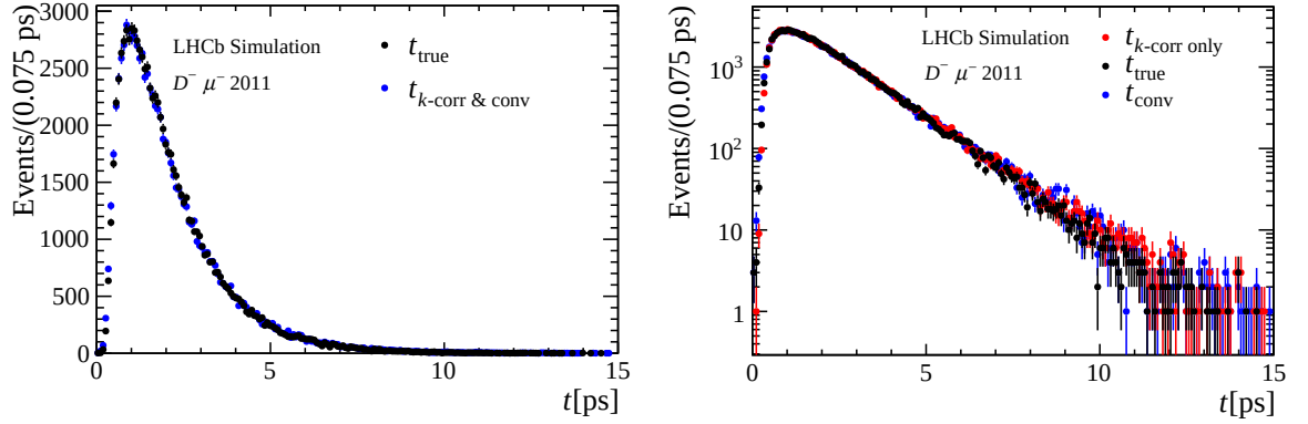
Figure 7.15: k -corrected and convoluted B decay time compared to the k -corrected only B decay time and the true B decay time. These plots should be compared to Fig. 7.6, where the momentum resolution effect (modeled by means of the k -factor convolution), is not taken into account. B^0 \rightarrow D^- \mu^+ \nu_\mu X simulated events with 2011 conditions.
