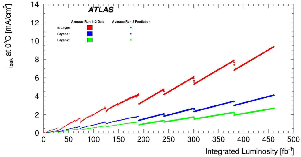
Figure 5.14: The average leakage current predictions versus integrated luminosity for the B-Layer, Layer-1 and Layer-2 operating at -12^\circ\text{C} in an extended Run 3 scenario. The predictions are compared to the average of the measured leakage currents in Run 1 and Run 2.
