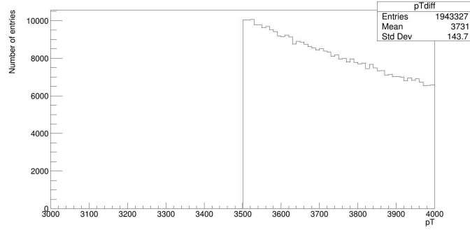
(c) K^{*0}
