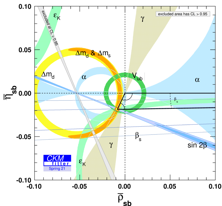
Figure 3.7: B_s^0 unitarity triangle [126].
