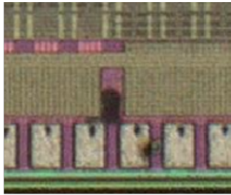
Figure 6.59: The contamination of wirebond pads on a FE-chip of an ITk Pixel bare module observed under the VHX-7000 microscope.
