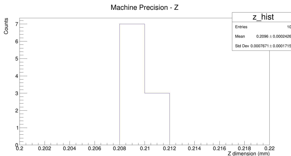
Figure 6.8: The precision of a measurement by the Vertex-261 metrology machine along the Z-direction using camera.
