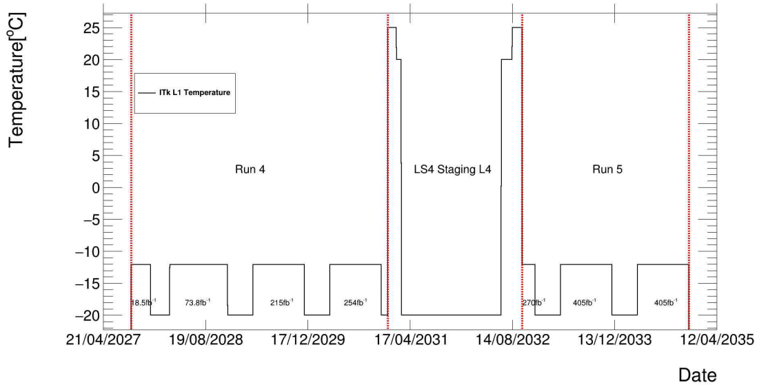
Figure 5.27: Temperature of Layer-1 (L1) during Run 4, Long Shutdown 4 (LS4) with staging of Layer-4 (L4), and Run 5.
