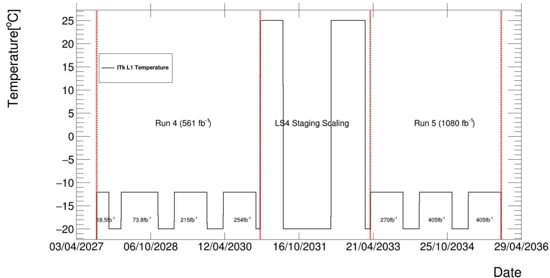
Figure 5.33: Temperature of Layer-1 (L1) during Run 4, Long Shutdown 4 (LS4) with staging with scaling, and Run 5.
