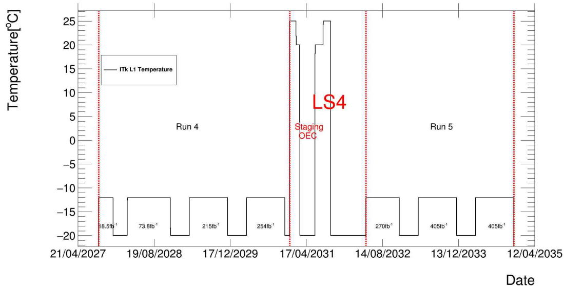
Figure 5.30: Temperature of Layer-1 (L1) during Run 4, Long Shutdown 4 (LS4) with the staging of the Outer End Caps (OEC), and Run 5.
