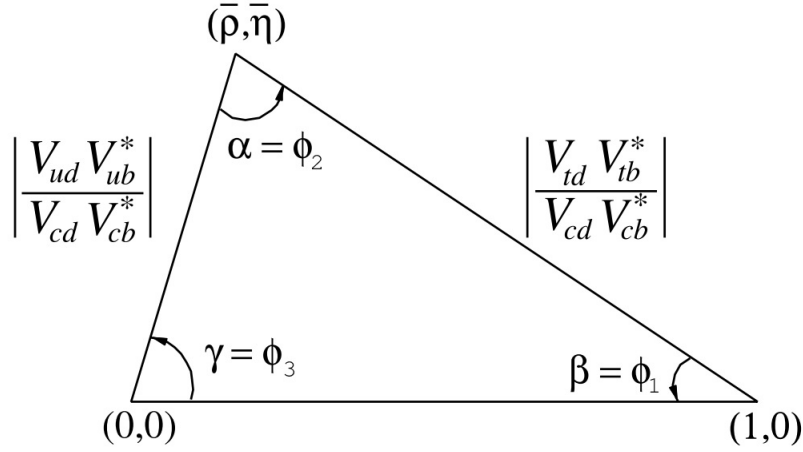
Figure 3.5: Sketch of the unitarity triangle [10].
