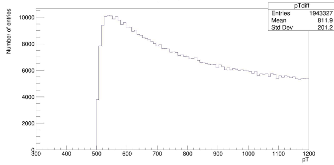
(b) \pi^\mp
