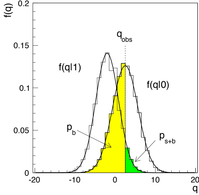
Figure 4.3.: Illustration of the distribution of the test statistics q under the assumption of \mu = 1 and \mu = 0 , identifying p_{S+B} (in green) and p_B (in yellow), with respect to an observation q_{\text{obs}} [56].
