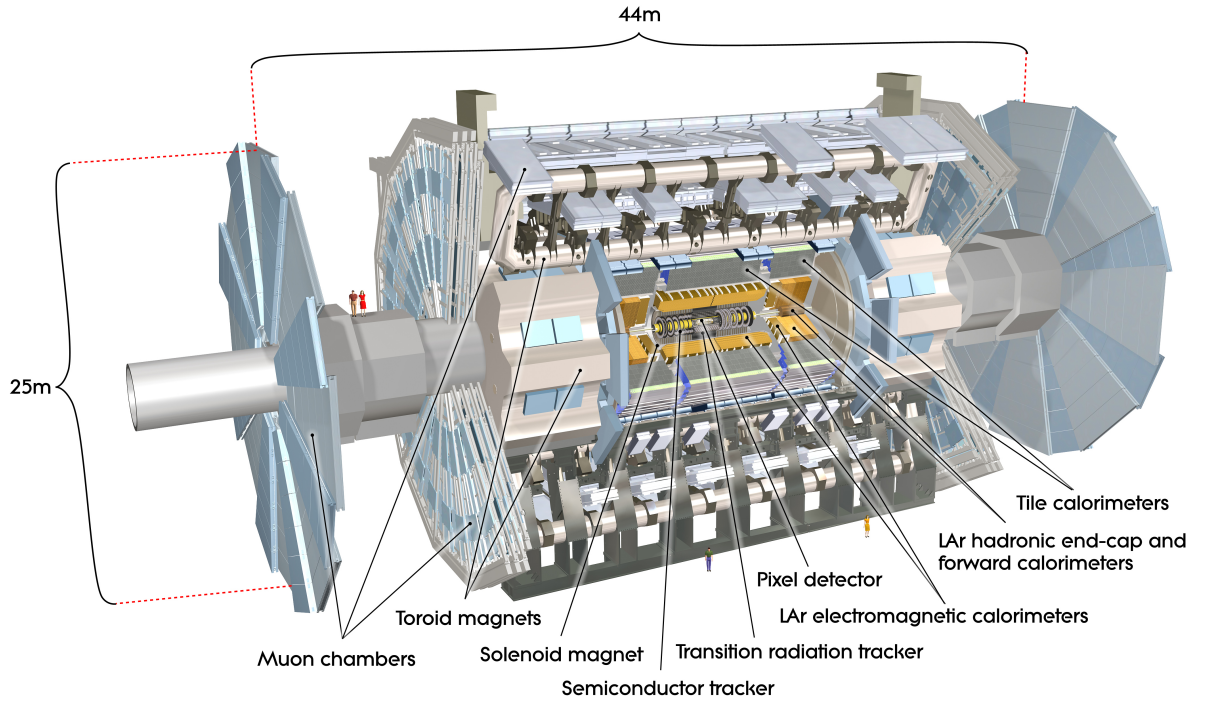
Figure 3.3.: Schematic view of the ATLAS detector [1].
