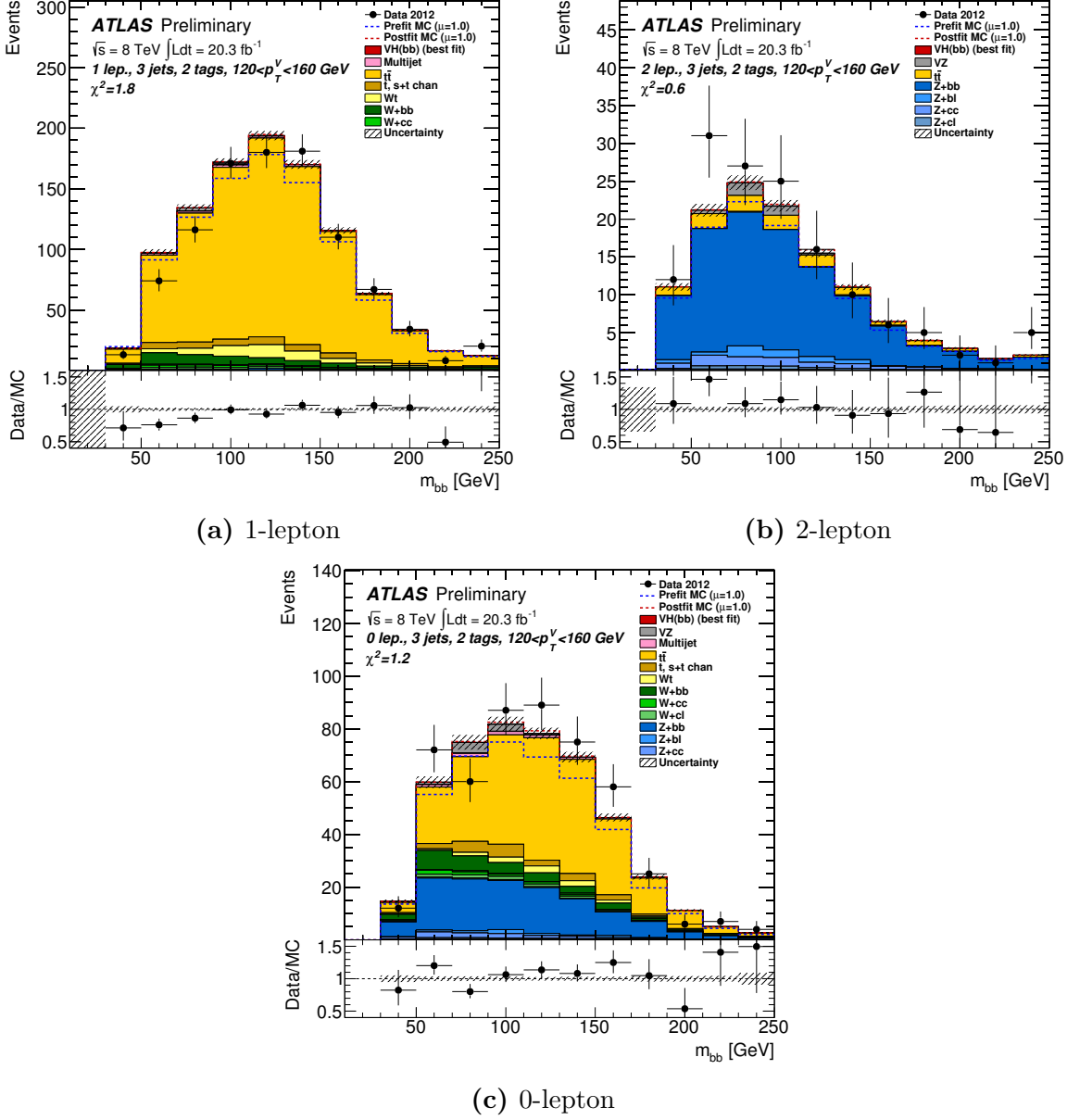
Figure 9.11.: Post-fit invariant mass distributions in the 120 < p_T^V/(\text{GeV}) < 160 bin for the 2-tag 3-jet region at \sqrt{s} = 8 TeV for data and Monte Carlo expectation. The last bin contains the distribution overflow. The hatched black area represents the total error after the profile likelihood fit, the dashed blue line represents the total background distribution input in the fit. The dashed red area represents the total background distribution in the hypothesis of a SM Higgs signal of mass 125 GeV ( \mu = 1 ), while the signal is renormalised to its best fit value after the fit. The solid area shows the various background components, with their post-fit normalisation values.
