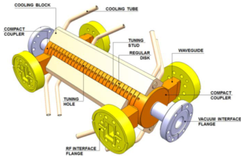
Figure 1.12. Engineering Design Completed Accelerating Structure in 3D Model
