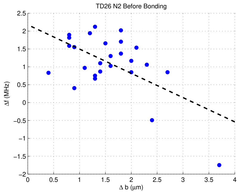
Figure 4.4. Scatterplot for TD26 N2 Before Bonding, r = -0.59
