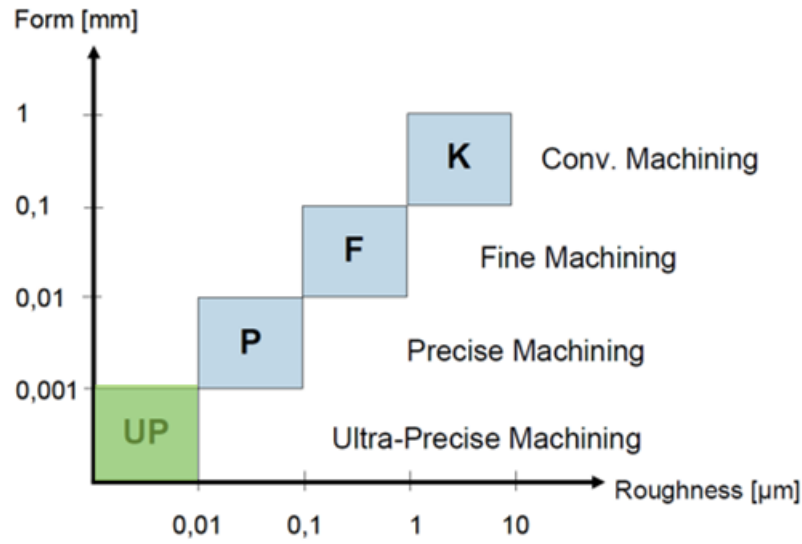
Figure 1.21. Classification of the machining process according to tolerances of shape accuracy and roughness [18]
