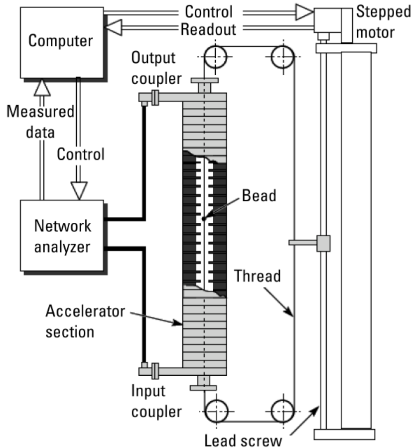
Figure 3.8. Schematic of bead-pull system [16]
