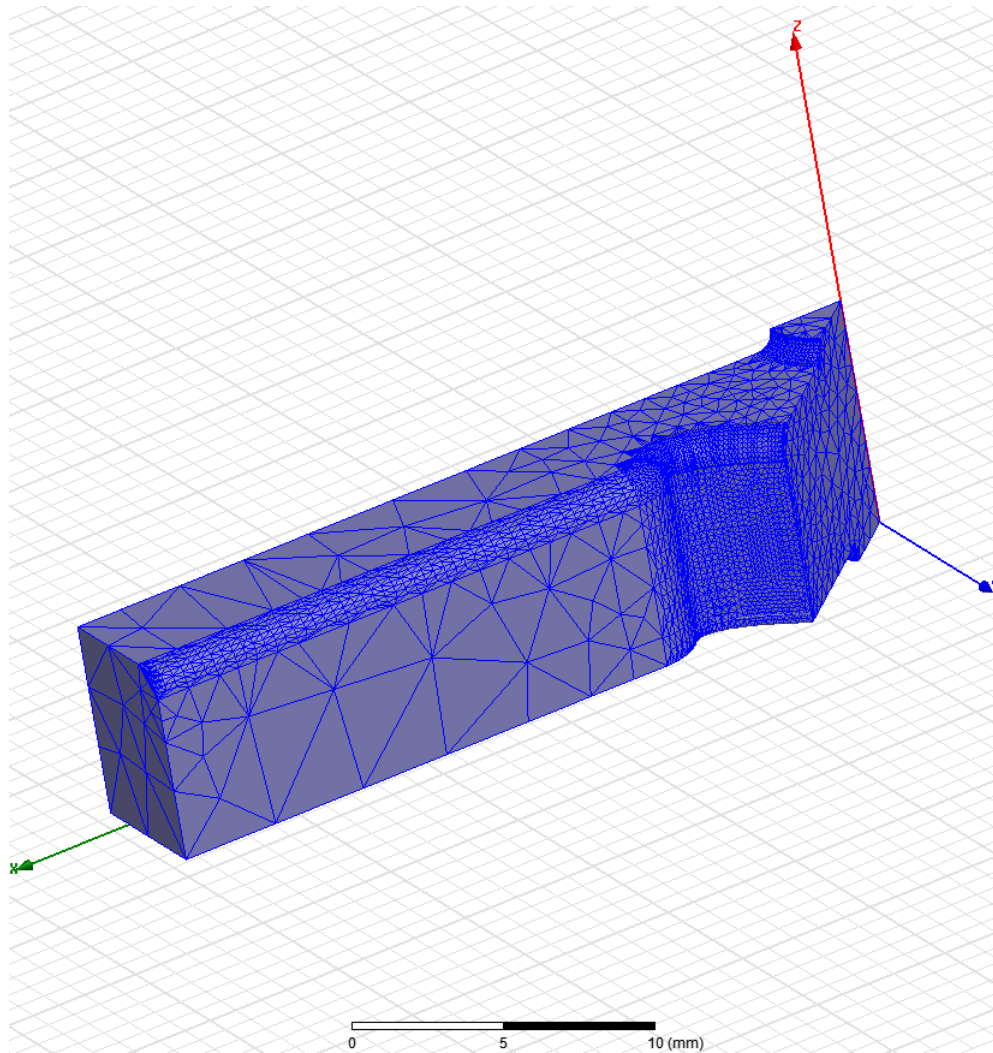
Figure 2.16. TD26 Mesh View
