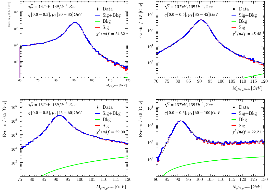
FIGURE C.1: The fits for systematics-2 in CR1 for all twenty p_T - |\eta| bins. In systematics-2, signal modeling function replaced by MC template (cont.)
