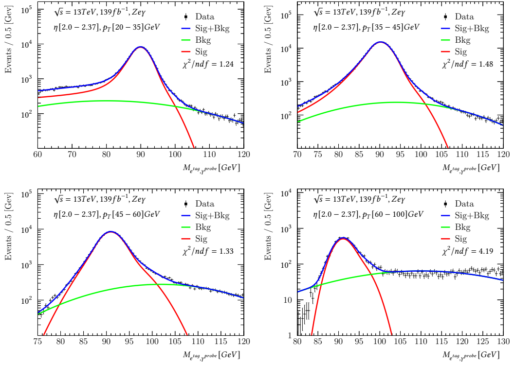
FIGURE D.6: The fits for systematic-3 in CR2 for all twenty p_T - |\eta| bins. In systematic C, background modeling function replaced by Gaussian function.
