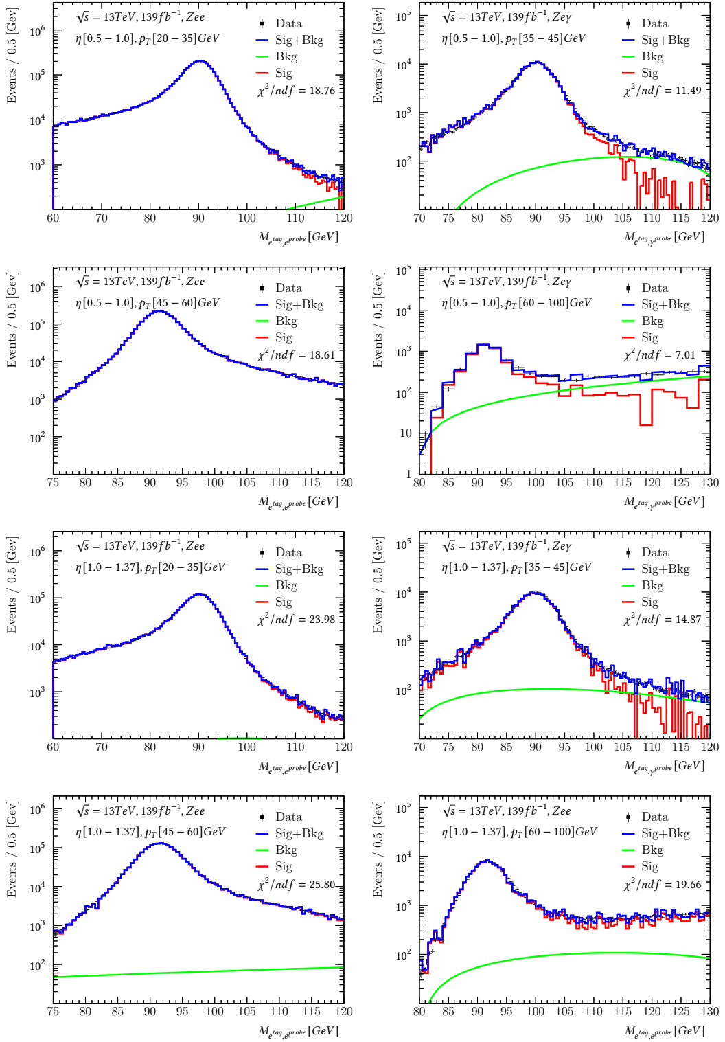
FIGURE C.2: The fits for systematics-2 in CR1 for all twenty p_T - |\eta| bins. In systematics-2, signal modeling function replaced by MC template (cont.)
