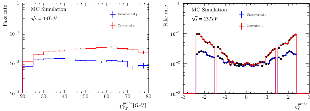
FIGURE 4.19: The MC fake rate for converted and unconverted \gamma as a function of p_T (left) and \eta (right) of the probe particles.
