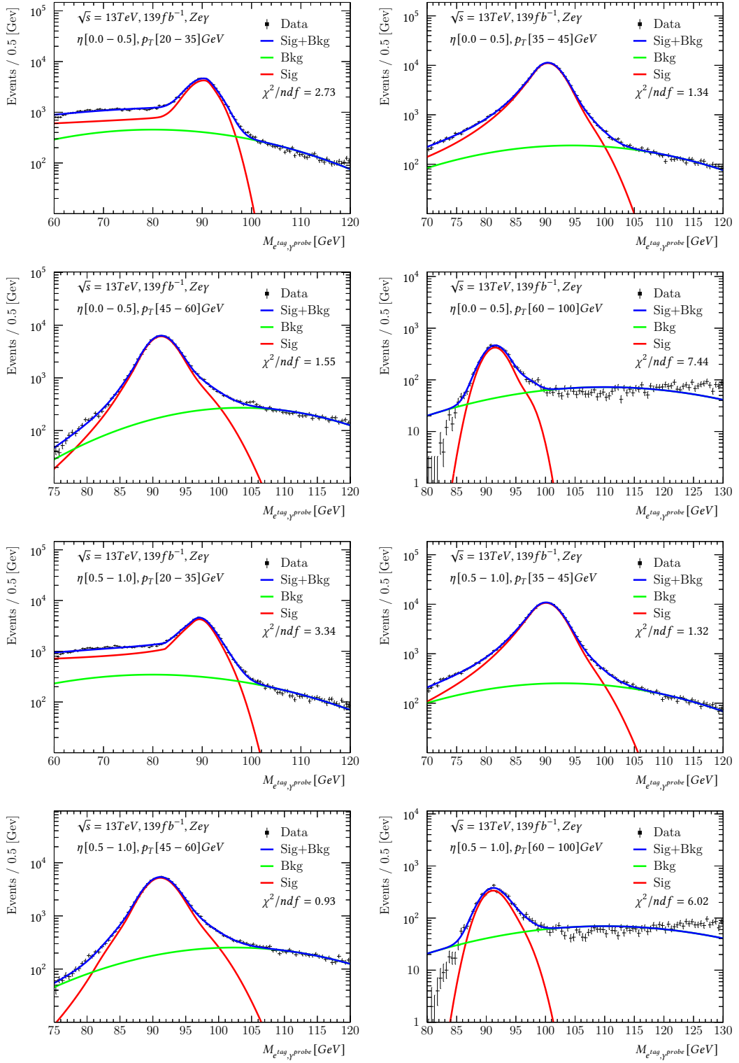
FIGURE D.4: The fits for systematic-3 in CR2 for all twenty p_T - |\eta| bins. In systematic C, background modeling function replaced by Gaussian function (cont.)
