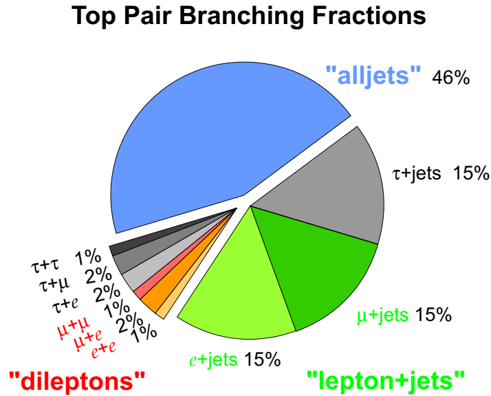
FIGURE 2.6: Top-anti-top quark pair decay channels and the pie chart with branching fractions. The decay channels are categorized depending on the further decay of W^\pm into quarks or leptons[10].
