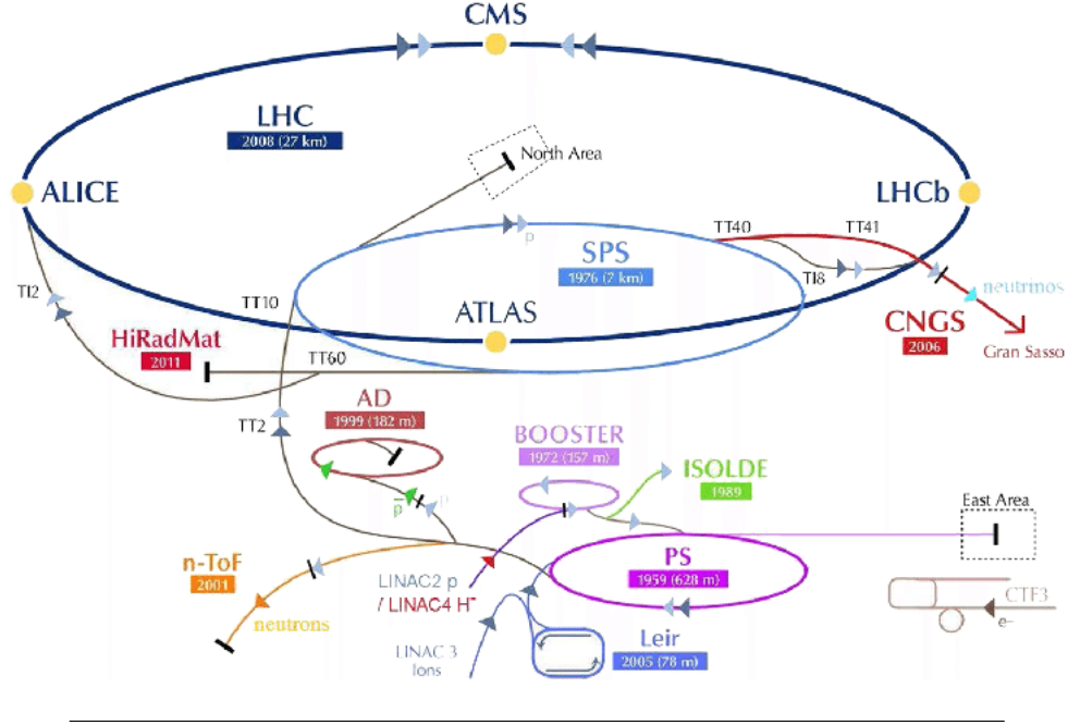
FIGURE 3.1: Schematic view of the CERN accelerators chain, the largest ring in dark blue color is the LHC [11].
