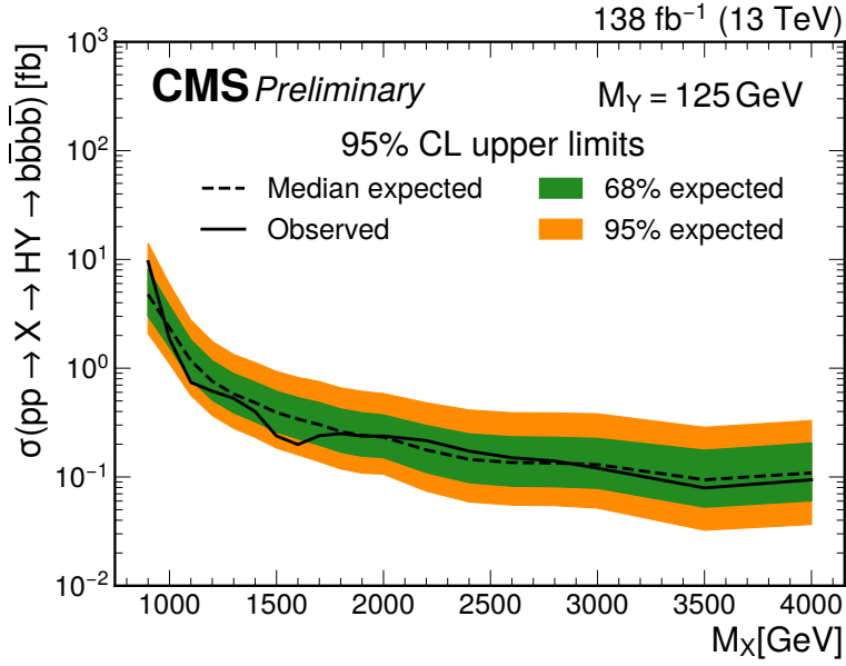
Figure 5.8: The 95% confidence level expected and observed upper limits on \sigma(\text{pp} \rightarrow \text{X} \rightarrow \text{YH} \rightarrow \text{b}\bar{\text{b}}\text{b}\bar{\text{b}}) for different values of M_{\text{X}} and M_{\text{Y}} = 125 GeV.
