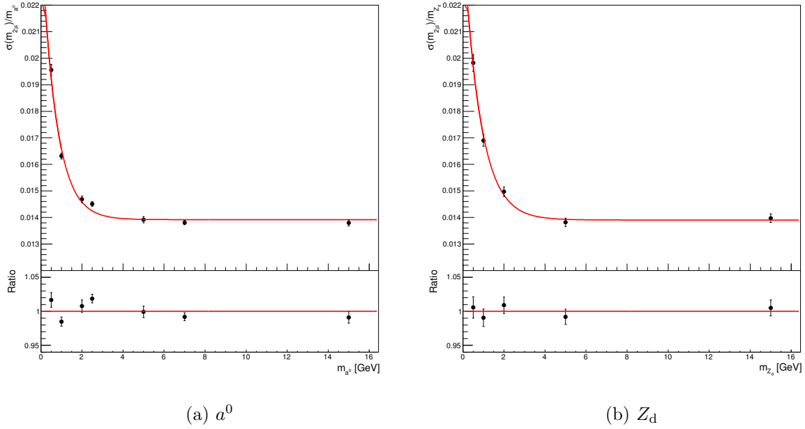
Figure 5.7: Standard deviation of a Gaussian fit to \langle m_{\mu^+\mu^-} \rangle normalised to m_X over the mass range considered, for (a) a^0 and (b) Z_d signal samples. The red line denotes the function used to describe the standard deviation of the Gaussian distribution which models the signal.
