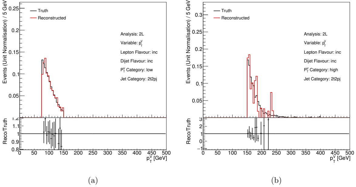
Figure 4.6: Comparison of p_T^Z generator-level and reconstruction-level distributions, for (a) the 75 \text{ GeV} < p_T^Z < 150 \text{ GeV} category and (b) the p_T^Z > 150 \text{ GeV} category. 2 c -tags are required for the nominal t\bar{t} samples.
