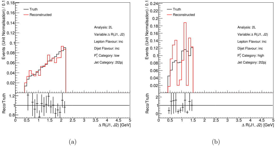
Figure 4.7: Comparison of \Delta R(j1, j2) generator-level and reconstruction-level distributions, for (a) the 75 \text{ GeV} < p_T^Z < 150 \text{ GeV} category and (b) the p_T^Z > 150 \text{ GeV} category. 2 c -tags are required for the nominal t\bar{t} samples.
