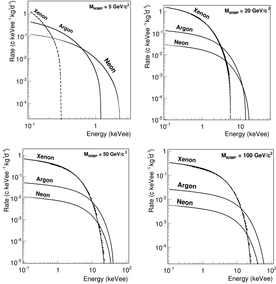
Figure 11.4: Expected WIMP-induced energy spectra in different targets for m_\chi = 5, 20, 50 and 100 GeV. The same assumptions than those of figure 11.3 are applied.
