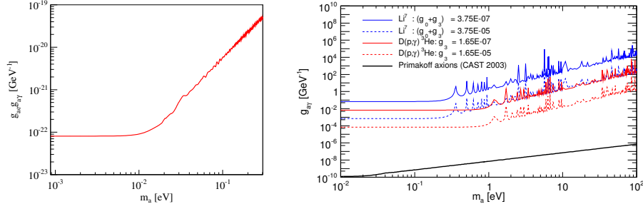
Figure 4.3: Upper bounds on the axion-electron coupling for non hadronic axions (left) [170], and on the axion-photon coupling from high energy axions produced in nuclear transitions in the Sun (right) [171].
