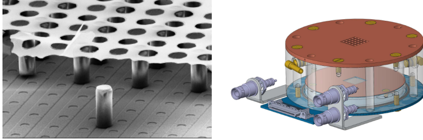
Figure 4.16: Left: picture of the InGrid detector, where mesh, pillars and silicon wafer are apparent. Right: the CAST InGrid TPC. The ports for gas input/output are visible in yellow, the HV and signal connectors are in grey, and the cathode with the strongback is represented in orange.
