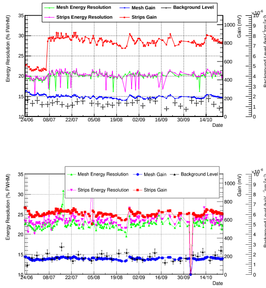
Figure 8.11: Evolution of the gain and energy resolution at 5.9 keV for the sunset 1 (top) and 2 (bottom) along 2012 data taking campaign. The evolution of the background level for a signal acceptance of 40% and 75% at 3 and 6 keV is also shown.
