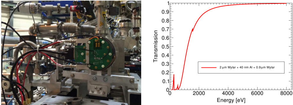
Figure 4.17: Left: InGrid detector installed in the sunrise V1 line of the CAST magnet. Right: x-ray transmission in the CAST energy RoI through 2\text{ }\mu\text{m} mylar window with 40\text{ nm} of Al deposition and 0.9\text{ }\mu\text{m} of the differential window.
