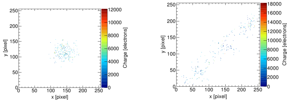
Figure 4.18: Comparison of x-ray (left) and cosmic (right) events in an intensity distribution map. Clearly, x-ray events produce a cloud-like distribution, while cosmic events typically produce much more spread signals. Figures extracted from [183].
