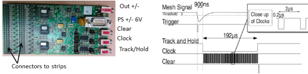
Figure 5.11: The Gassiplex card (left) and the relevant signals for the acquisition of Gassiplex data.
