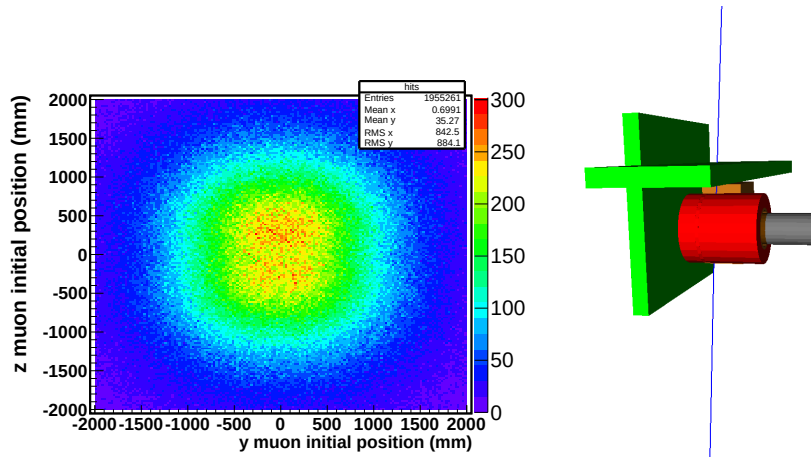
Figure 10.12: Left: Initial vertexes of the incident cosmic muons that deposited an energy lying in the CAST RoI (0-15 keV). z-axis is the axis along the CAST vacuum line, while y-axis defines the horizontal plane over the Micromegas detectors. Right: example of a cosmic muon traversing the top scintillator (in green) and the detector.
