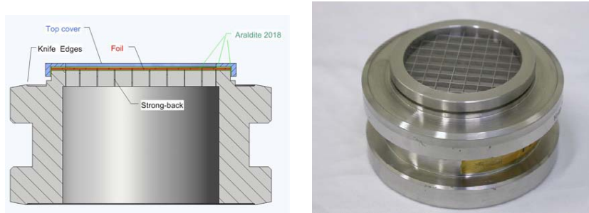
Figure 4.5: Cross-section scheme of the cold window layout (left), and picture of one of the four cold-windows installed in the magnet bores.
