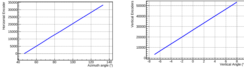
Figure 4.9: Conversion of the motor encoders of the local coordinate system to the angles in the global reference system.
