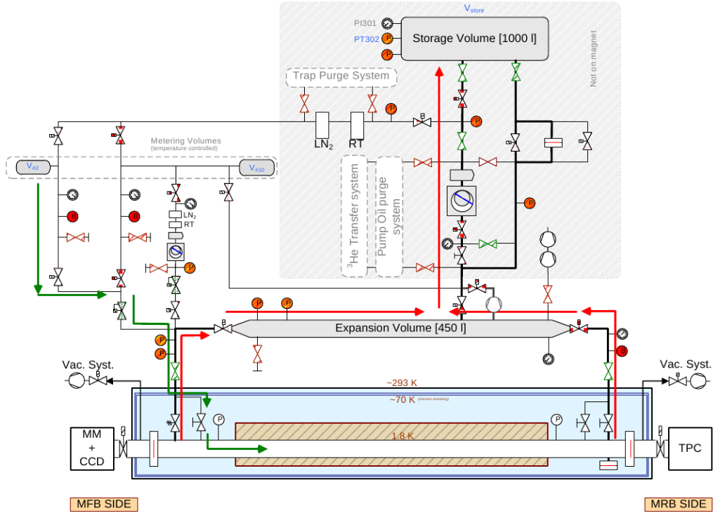
Figure 4.6: Schematics of the buffer gas filling system. In blue, the magnet cryostat; in brown, the magnetic field region at 1.8 K. The green lines show the path from the metering volume V_2 to the cold-bores, while the red lines show the recovery process. Also shown, the storage and expansion volume; the room temperature (RT) and liquid nitrogen ( \text{LN}_2 ) purification system; and the recovery system.
