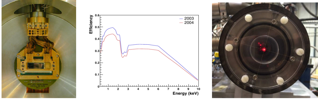
Figure 4.13: Left: a picture of the pn-CCD detector. Centre: overall x-ray detection efficiency of the x-ray mirror system and the pn-CCD detector in the energy range of interest for CAST. Extracted from [167]. Right: a picture illustrating the the x-ray telescope alignment with the laser beam and cross-wires.
