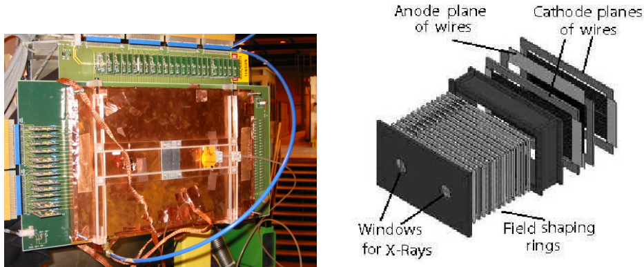
Figure 4.15: Left: back view of the TPC installed in the CAST line. Right: schematic view of the CAST TPC, where the x-ray windows and the anode wires are labelled.
