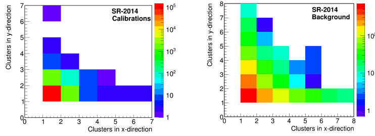
Figure 6.4: Number of clusters in the xy plane in a CAST-MM detector during ^{55}\text{Fe} calibrations (left) and during background runs (right).
