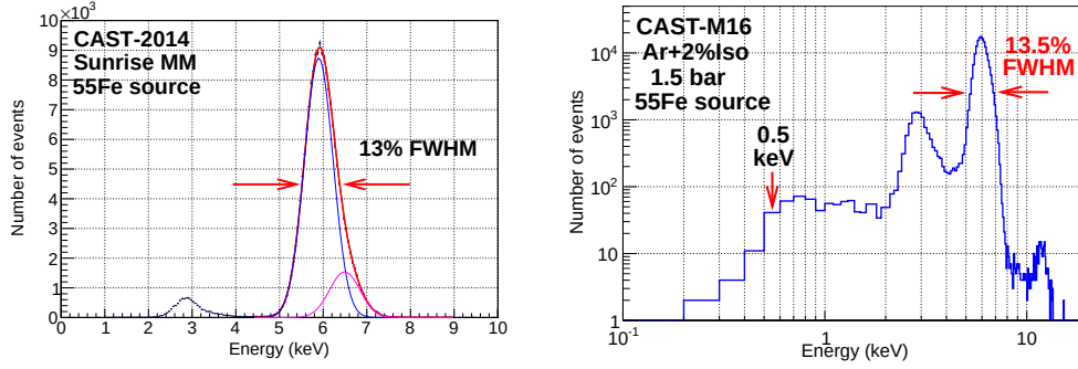
Figure 7.3: Left: ^{55}\text{Fe} calibration spectrum of a Micromegas detector. The main peak has been fitted to two gaussian functions (blue and magenta lines), corresponding to the K_\alpha (5.9 keV) and K_\beta (6.4 keV) lines. Right: calibration spectrum showing the energy resolution and energy threshold of the CAST-M16 detector.
