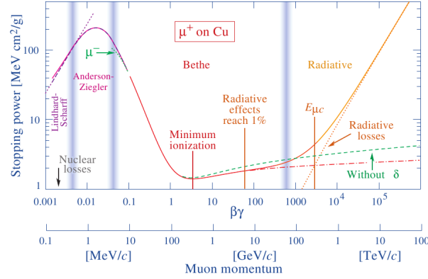
Figure 1.5: Stopping power of positive muons in copper as a function of the muon momentum, extracted from [6].
