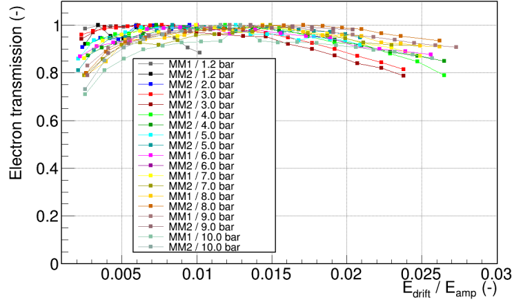
Figure 13.3: Dependence of the electron transmission with the ratio of drift and amplification fields in the bulk Micromegas of TREX-DM in Ar+2%iC 4 H 10 at pressures from 1.2 to 10 bar. The peak positions have been normalized with the maximum of each series, assuming maximum electron transmission is always achieved.
