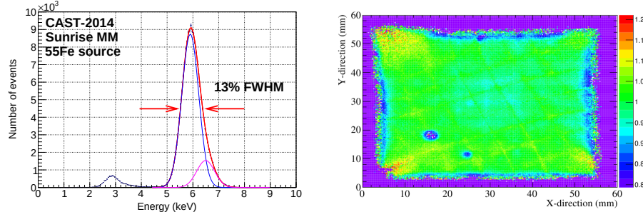
Figure 9.22: Left: ^{55}\text{Fe} calibration spectrum of the sunrise Micromegas detector. The main peak has been fitted to two gaussian functions (blue and magenta lines), corresponding to the K_\alpha (5.9 keV) and K_\beta lines (6.4 keV). Right: gain uniformity of the sunrise Micromegas detector. The dead areas (in purple) show lower values than the unity (in green) and lie outside the axion-sensitive area.
