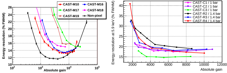
Figure 7.7: Left: dependence of the energy resolution at 5.9 keV with the absolute gain for the M-branch detectors in \text{Ar}+5\% \text{ iC}_4\text{H}_{10} at atmospheric pressure. As a comparison, the curve generated by a non-pixelized microbulk detector in the same conditions has been included. Right: same dependence for the C- and R-branch detectors in \text{Ar}+2\% \text{ iC}_4\text{H}_{10} at the indicated pressure.
