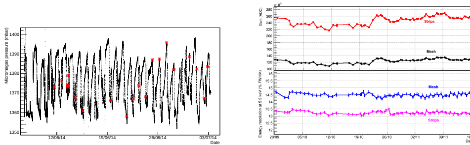
Figure 7.8: Left: evolution of the gas pressure inside the detector chamber and time at which calibrations are performed (red crosses). Right: evolution of the gain and the energy resolution of the Sunrise Micromegas detector along the 2014 data-taking. The fluctuations, measured both at the mesh and at the strips are less than 10%.
