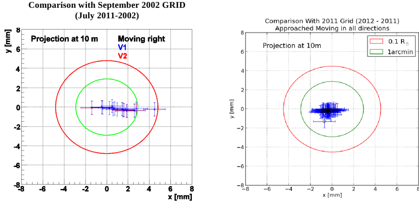
Figure 4.10: Deviation in the solar tracking projected to a plane at 10 meters of both magnet bore lines (V1 and V2 in blue and red crosses respectively). On the left, deviation between the original calibration in 2002 and the GRID measurements of 2011, which are considered the reference coordinates from 2012 onwards. On the right, the comparison between 2011 and 2012 GRIDs. Figures extracted from [175].
