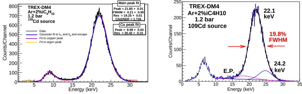
Figure 13.1: Energy spectrum respectively generated by the mesh (left) and strips signals (right) when one of the Micromegas detectors was irradiated by a ^{109}Cd source in Ar+2\%iC_4H_{10} at 1.2 bar. The spectral parameters are defined through an iterative multi-Gaussian fit corresponding to the K_{\alpha} and K_{\beta} emission lines of the source and their escape peaks (E.P.). The fluorescence lines of iron (at 6.4 keV, emitted from the mesh) and copper (8 keV, from the vessel) are also present in both spectra. The energy threshold is situated at around 1 keV.
