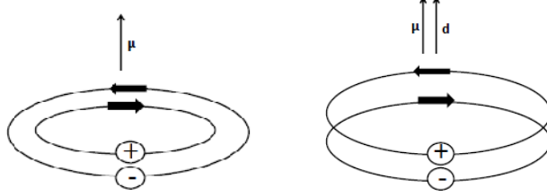
Figure 2.1: A neutron model with vanishing (left) and no-vanishing (right) EDMN. The electric and magnetic dipole moments are denoted respectively by \mu and d .
