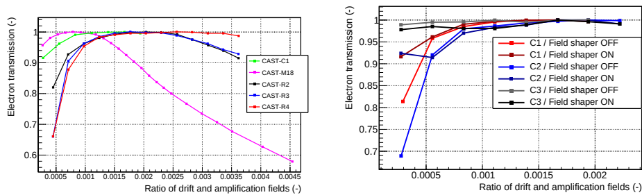
Figure 7.4: Left: dependence of the electron transmission with the ratio of fields for some detectors of the M -, C - and R -branches in \text{Ar}+2\% \text{ } i\text{C}_4\text{H}_{10} at 1.4 bar. Right: effect of the field shaper on the electron transmission for the C -branch detectors in \text{Ar}+2\% \text{ } i\text{C}_4\text{H}_{10} at 1.4 bar.
