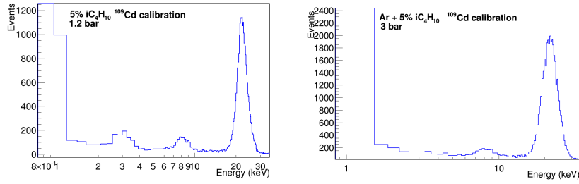
Figure 13.8: Calibration spectra ( ^{109}Cd source) in Ar+5\%iC_4H_{10} at 1.2 and 3 bar at the maximum gain before spark limit. Energy threshold slightly degrades from \sim 1 keV to 1.5 keV.
