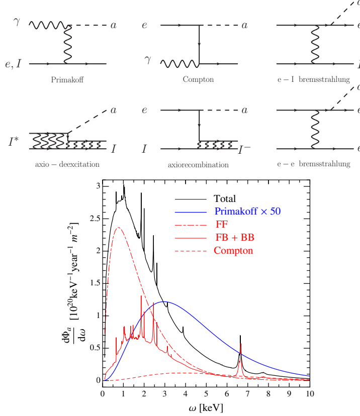
Figure 3.2: Top: Feynman diagram of the Primakoff effect (top left) and axion production mechanisms in non-hadronic axion models. Bottom: contributions to the differential solar axion flux. In red, the processes involving axion-electron coupling (for g_{ae}=10^{-13} \text{ GeV}^{-1} ): atomic recombination and deexcitation (FB+BB, solid), Bremsstrahlung (FF, dot-dashed) and Compton (dashed). In blue, the Primakoff flux for g_{a\gamma}=10^{-12} \text{ GeV}^{-1} . Figures extracted from [160].
