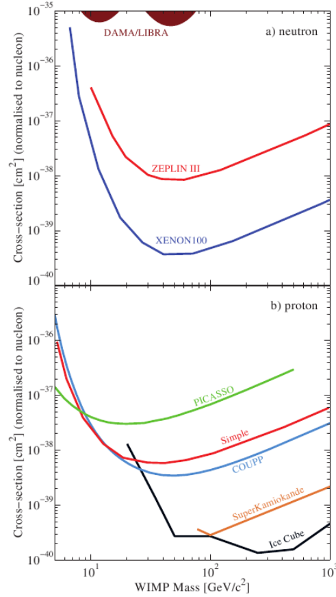
Figure 11.7: Limits on the WIMP-nucleon cross section for spin-dependent coupling as a function of the mass, for the interaction with the neutron (top) and proton (bottom). Extracted from [210].
