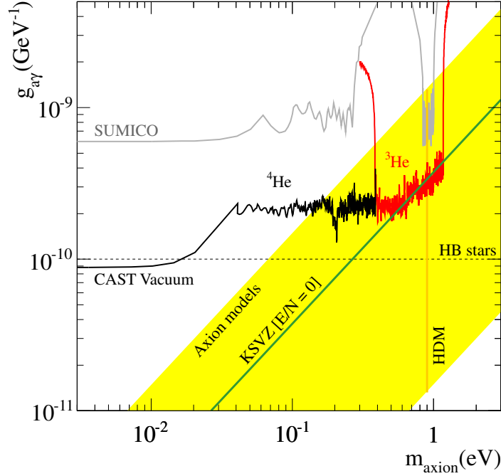
Figure 4.2: Exclusion regions in the g_{a\gamma} - m_a plane achieved by CAST in the vacuum, ^4\text{He} and ^3\text{He} phases. Also shown the constraints set by Sumico [139, 168, 169], horizontal branch (HB) stars (without considering the new most restrictive bound coming from the suppression of blue loop stage of massive stars [111]), and Hot Dark Matter (HDM) overabundance limit. The yellow band represents the the most appealing theoretical axion models, and the green solid line corresponds to the KSVZ model with E/N = 0 .
