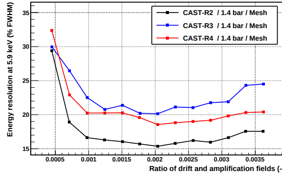
Figure 7.5: Dependence of the energy resolution at 5.9 keV with the ratio of fields for the R -branch detectors in \text{Ar}+2\% \text{iC}_4\text{H}_{10} at 1.4 bar.
