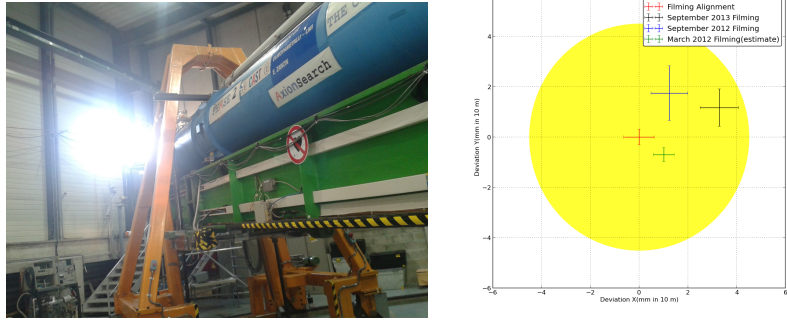
Figure 4.11: Left: Sun filming window in the building that hosts the CAST experiment. Right: Measured deviation from the center of the Sun in three different filmings. In yellow, the 10% of the solar radius. Figure extracted from [176].
