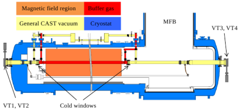
Figure 4.8: Scheme of the vacuum system of CAST, explicitly showing the different vacuum subsystems and components.
