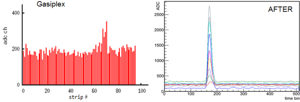
Figure 5.9: Comparison of an x-ray event as seen by the Gassiplex electronics (without pedestal subtraction) and AFTER-based electronics.
