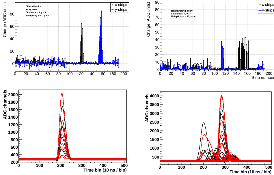
Figure 6.3: Top: calibration (left) and background (right) events as recorded by the Gassiplex electronics after pedestal subtraction. Note that the channels between roughly 0-90 and 180-192 are not instrumented, being larger the noise fluctuations. Bottom: the same type of events as acquired by AFTER electronics.
