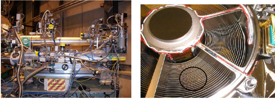
Figure 4.12: Left: x-ray telescope installed in the CAST line. Right: front view of the x-ray focusing device. The device is situated off-axis, covering the cold-bore area (black circle) with one of the sectors of the telescope.
