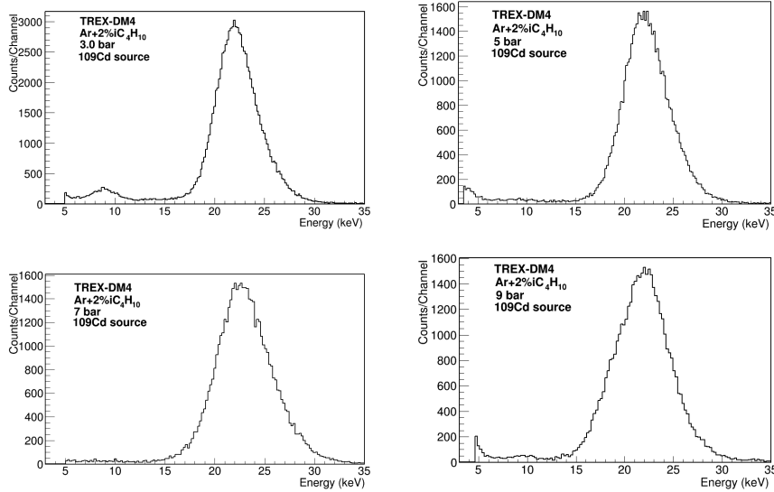
Figure 13.2: Calibration spectra at 3, 5, 7 and 9 bar in Ar+2\%iC_4H_{10} . Note how the fluorescence peak is suppressed at higher pressures.
