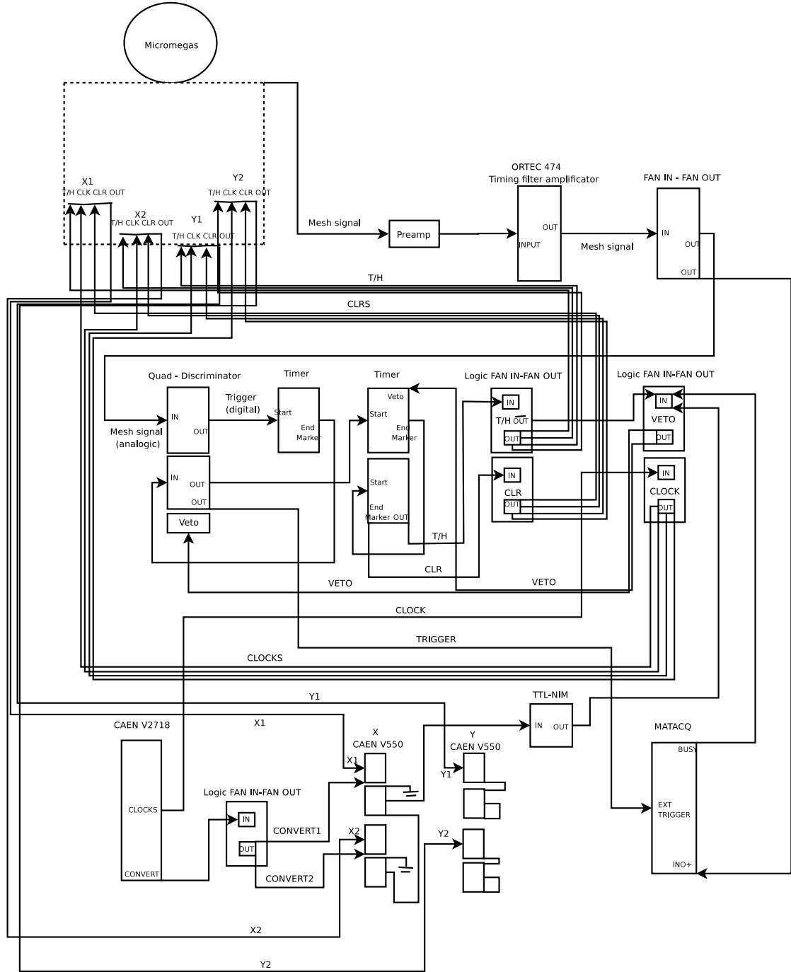
Figure A.2: The electronics chain of the sunset Micromegas with Gassiplex electronics.
