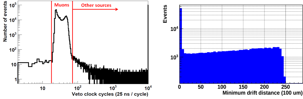
Figure 10.16: Distribution of the time elapsed between the scintillator veto and the mesh trigger in CAST-M18 data (left) and distribution of the minimum drift distance of the primary electrons generated by the muons simulation in a CAST-Sunset like setup (right).
