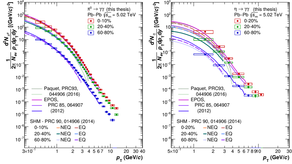
Figure 7.19: Invariant yields in different centrality classes. Vertical error bars indicate statistical uncertainties and the height of the boxes corresponds to the systematic uncertainties. The horizontal extension of the boxes indicate the bin widths. The meson yields N are counted within these bins and then divided by the bin widths \Delta p_T . The data is compared to calculations by J.-F. Paquet et al. [129], V. Begun et al. [173] and the EPOS model [174].
