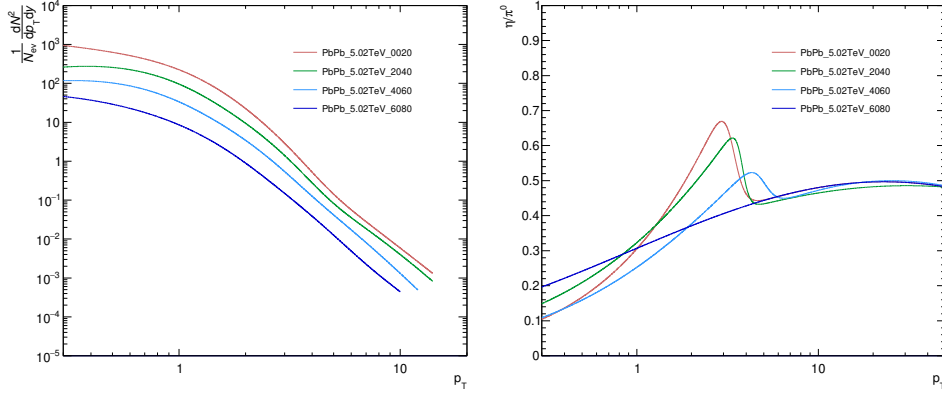
Figure 8.10: Parametrizations of measured \pi^0 spectra and \eta/\pi^0 ratios in all centrality classes.
