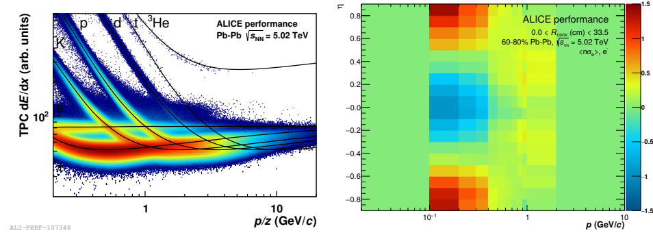
Figure 6.6: Left: TPC dE/dx with Bethe-Bloch parametrizations for different particle species in Pb-Pb low interaction rate runs [152]. Right: Correction map for one R bin of one centrality class, which was manually created within this thesis. The color illustrates the value of n\sigma_e in each bin before recalibration (see text for more details).
