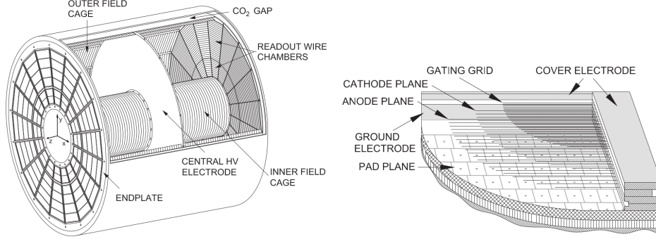
Figure 6.3: Left: Schematic drawing of the TPC field cage with its central electrode and readout chambers Right: Closer view of a readout chamber showing the pad planes and wire planes [136].
