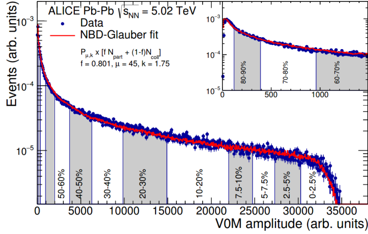
Figure 6.8: Distribution of V0M in all events of the analyzed dataset with NBD-Glauber fit and centrality classes [158].
