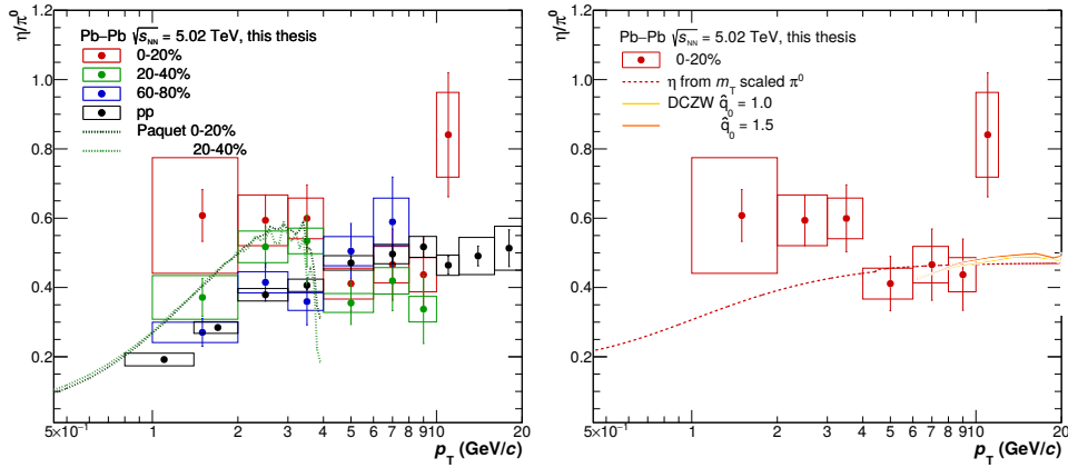
Figure 7.20: Left: \eta/\pi^0 ratio in different centrality classes compared to the ratio in pp collisions [178] and to calculations by Paquet et al. [129]. Right: \eta/\pi^0 ratio in 0-20% most central collisions, compared to m_T -scaling and calculations from the DCZW model [86] with two different initial values of the jet transport parameter \hat{q}_0 .
