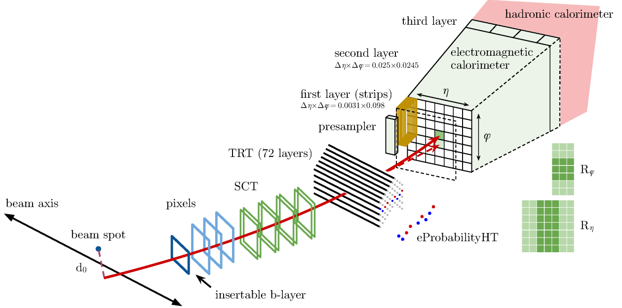
Figure 3.1: Schematic view of electron reconstruction and identification [46].
