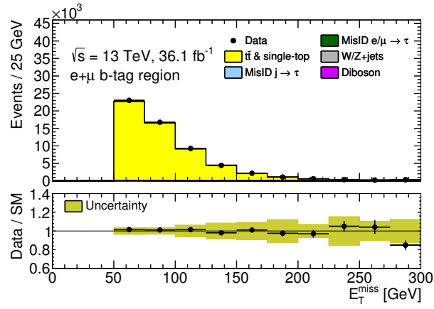
(c) E_T^{\text{miss}}
