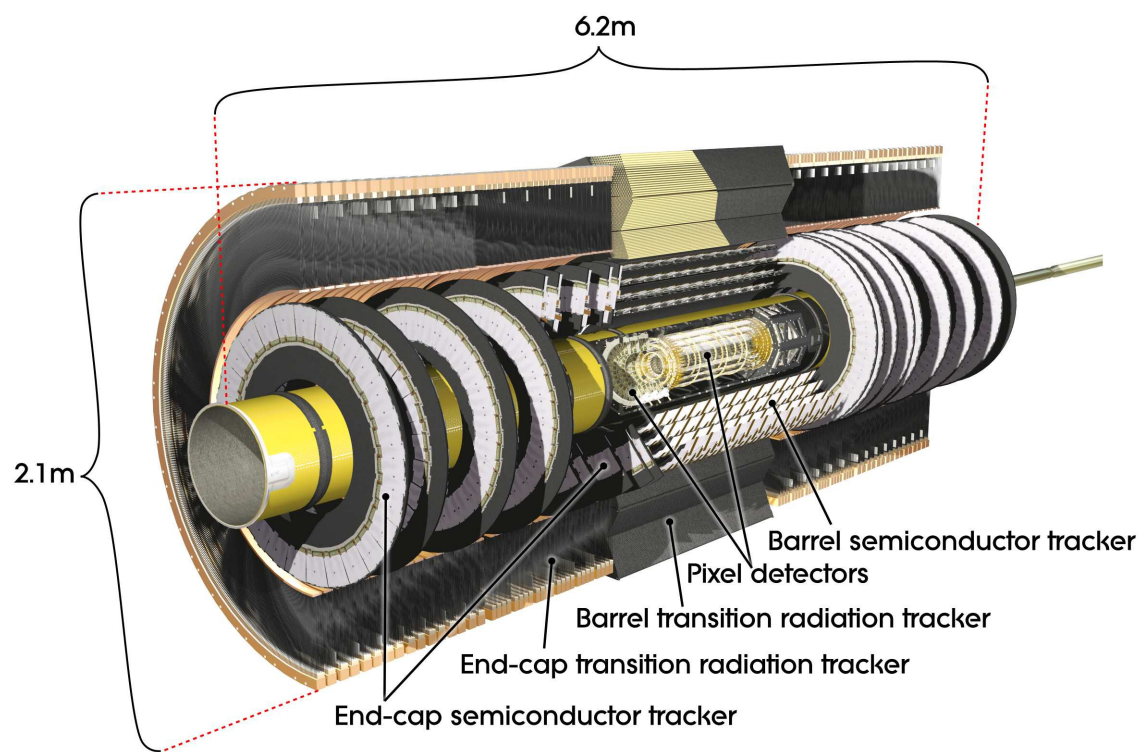
Figure 2.3: Cut-away view of the ATLAS Inner Detector [30].
