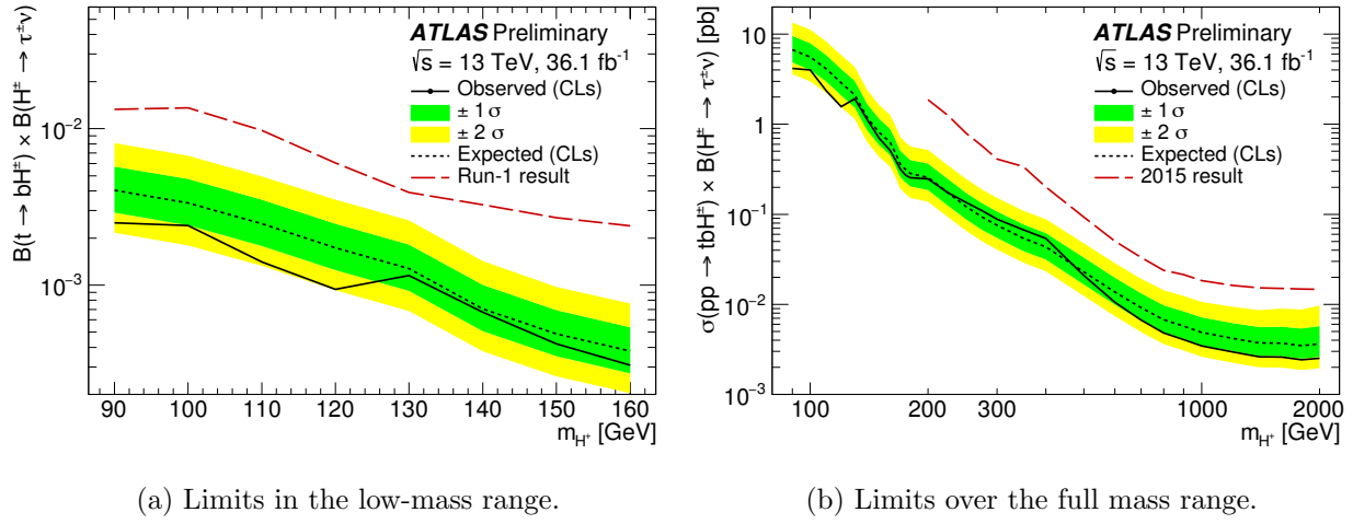
Figure 4.13: Expected and observed limits on the charged Higgs production and H^\pm \rightarrow \tau^\pm \nu decay over the low and full mass ranges [19].
