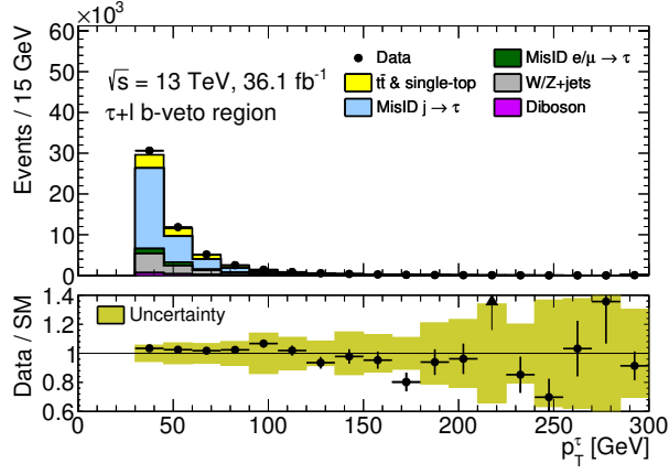
(a) p_T^\tau
