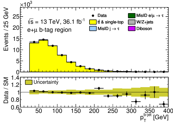
(a) p_T^{b\text{-jet}}
