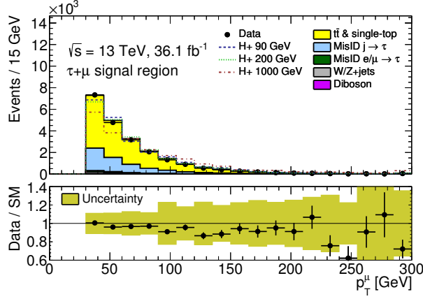
(a) p_T^\mu
