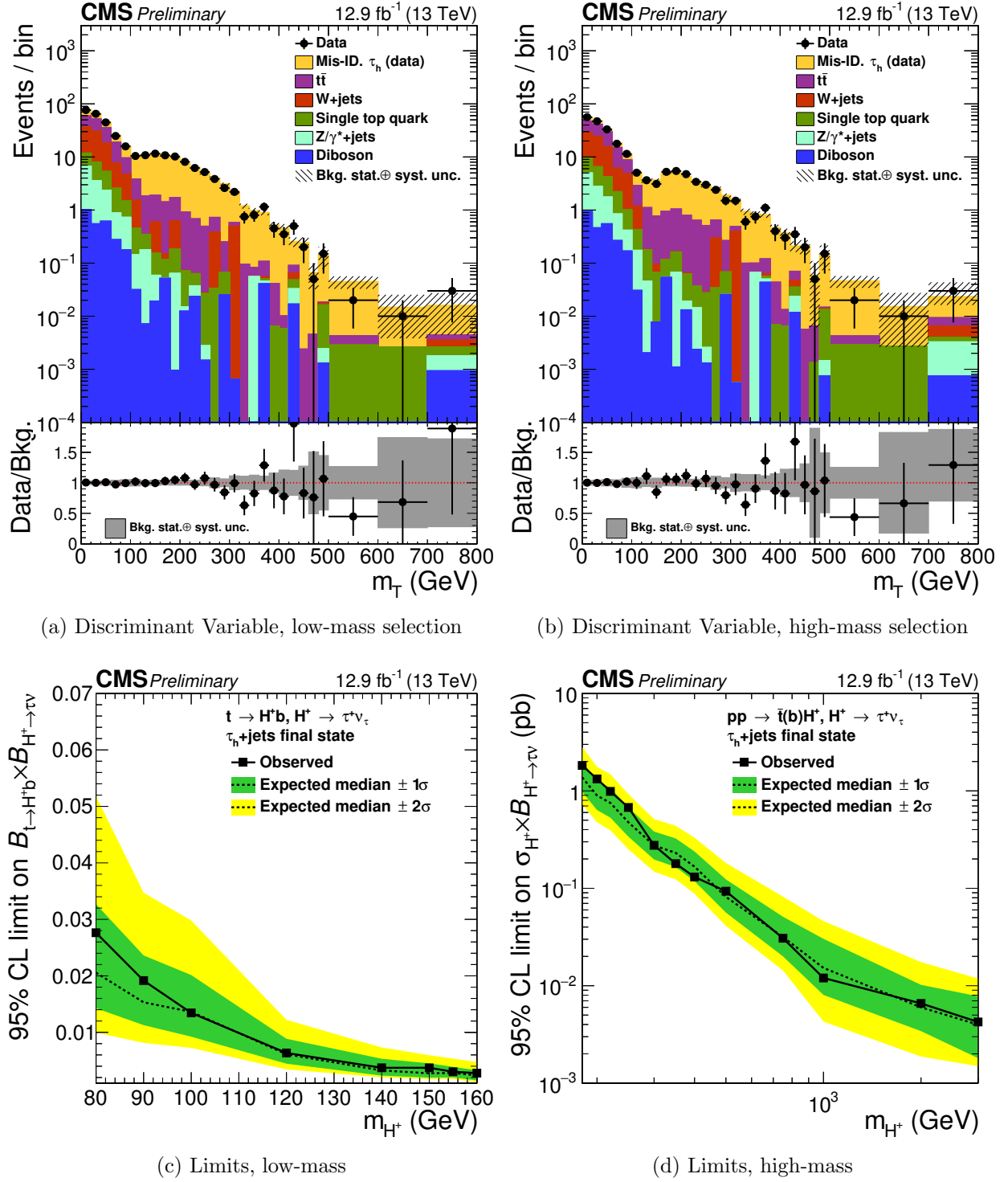
Figure 1.6: Discriminant variable and observed limits from prior CMS searches for H^\pm \rightarrow \tau\nu .
