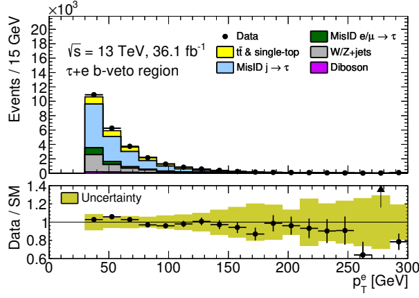
(a) p_T^e
