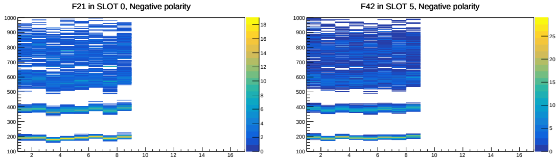
Figure 5.7: Injection charge just above four thresholds for FEERIC21 and FEERIC42 tested on negative polarity.
