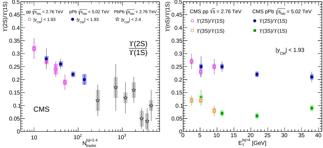
Figure 3.16: Single cross section ratios \Upsilon(2S) over \Upsilon(1S) for |y_{CM}| < 1.93 as a function of charged track (on left) and transverse energy (on right) [6].
