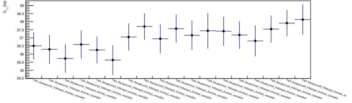
Figure C.12: Significance of \Upsilon(1S) in the integrated case.
