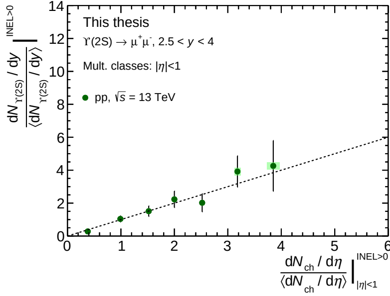
Figure 6.38: Relative \Upsilon(2S) yield as a function of charge-particle multiplicity, the black dashed line is drawn to x=y correlation.
