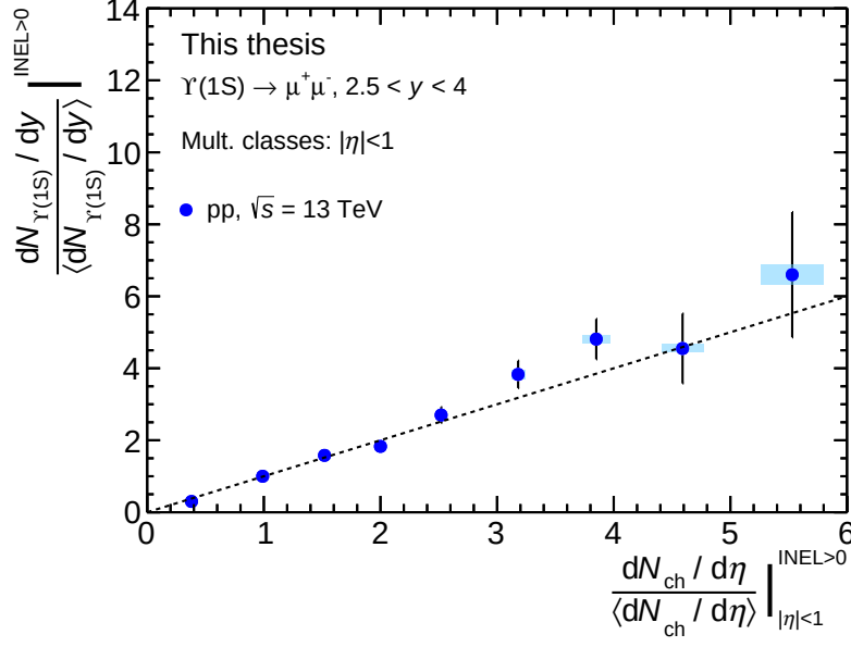
Figure 6.37: Relative \Upsilon(1S) yield as a function of charge-particle multiplicity, the black dashed line is drawn to x=y correlation.
