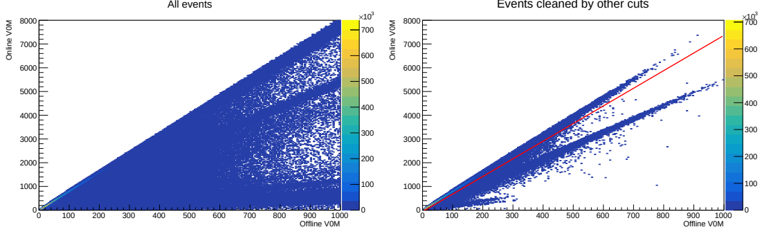
Figure 6.1: Correlation of online and offline information in the V0
