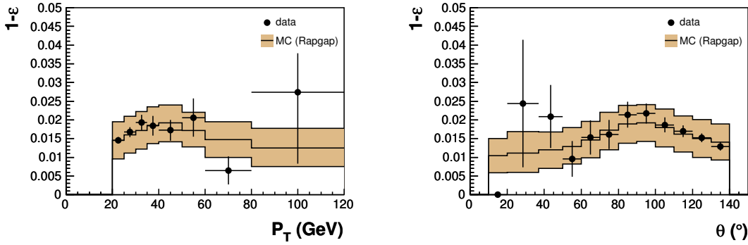
Fig. 4.11: The CIP inefficiency as a function of the transverse momentum P_T and the polar angle \theta of the electron
