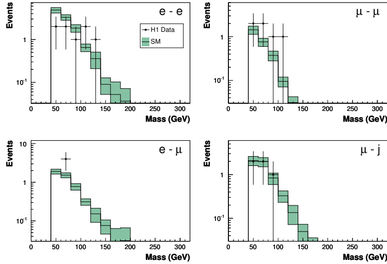
Fig. 6.3: The distributions of the invariant mass M_{all} for the e - e , \mu - \mu , e - \mu and \mu - j event classes.
