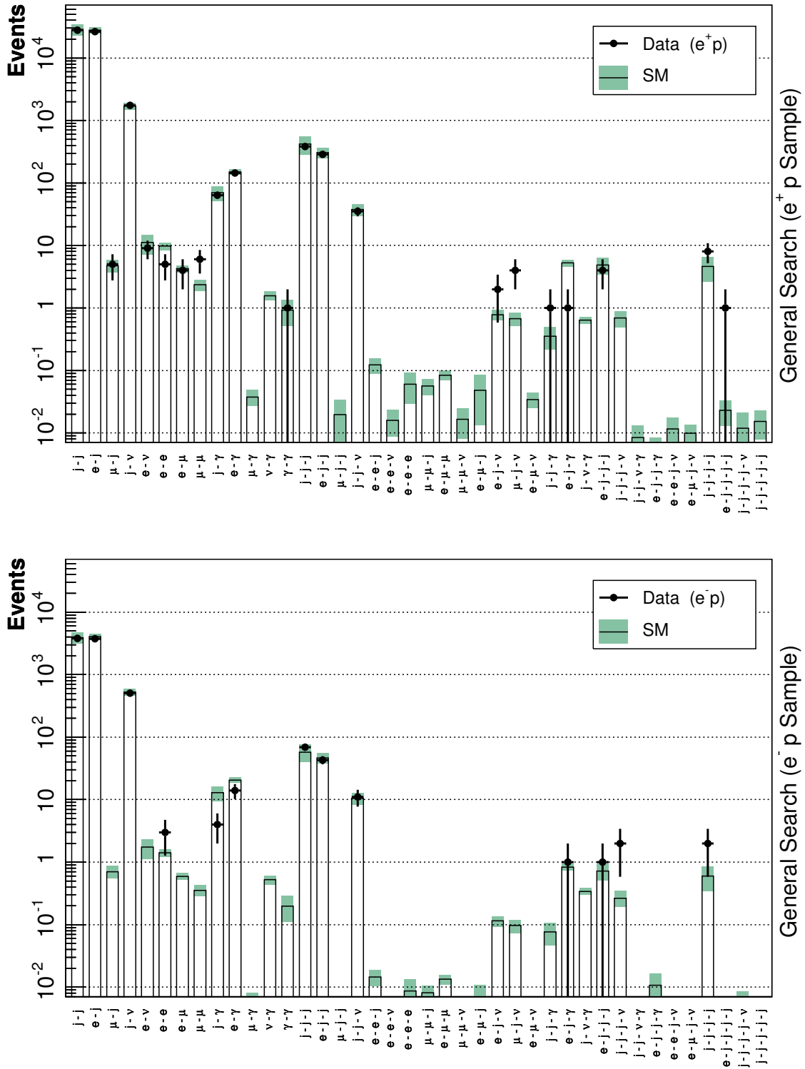
Fig. 6.7: The event yields subdivided into event classes as derived from the investigation of the e^+p (upper figure) and e^-p (lower figure) data samples. Shown are all event classes with a SM expectation greater than 0.01 events for the full HERA-I data sample.
