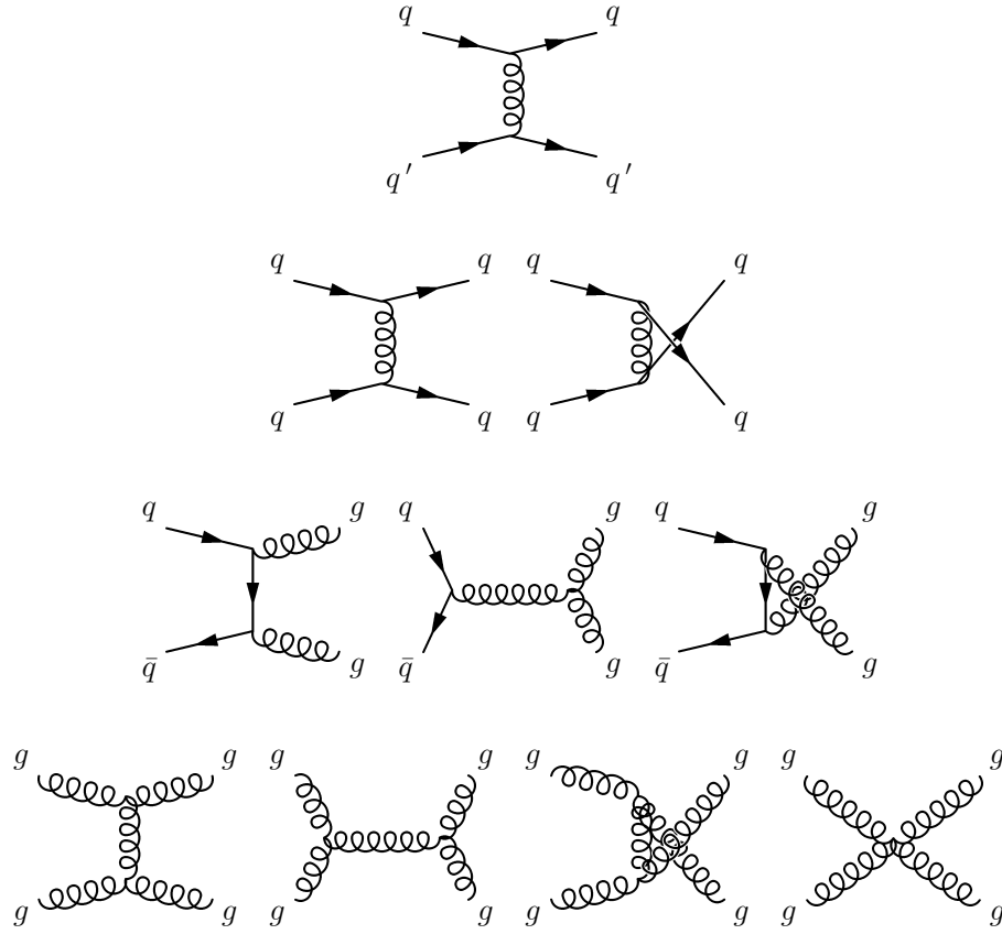
Fig. 1.3: Leading-order diagrams for resolved photoproduction of jets, corresponding to the parton scattering processes qq' \rightarrow qq' , qq \rightarrow qq , q\bar{q} \rightarrow gg and gg \rightarrow gg .
