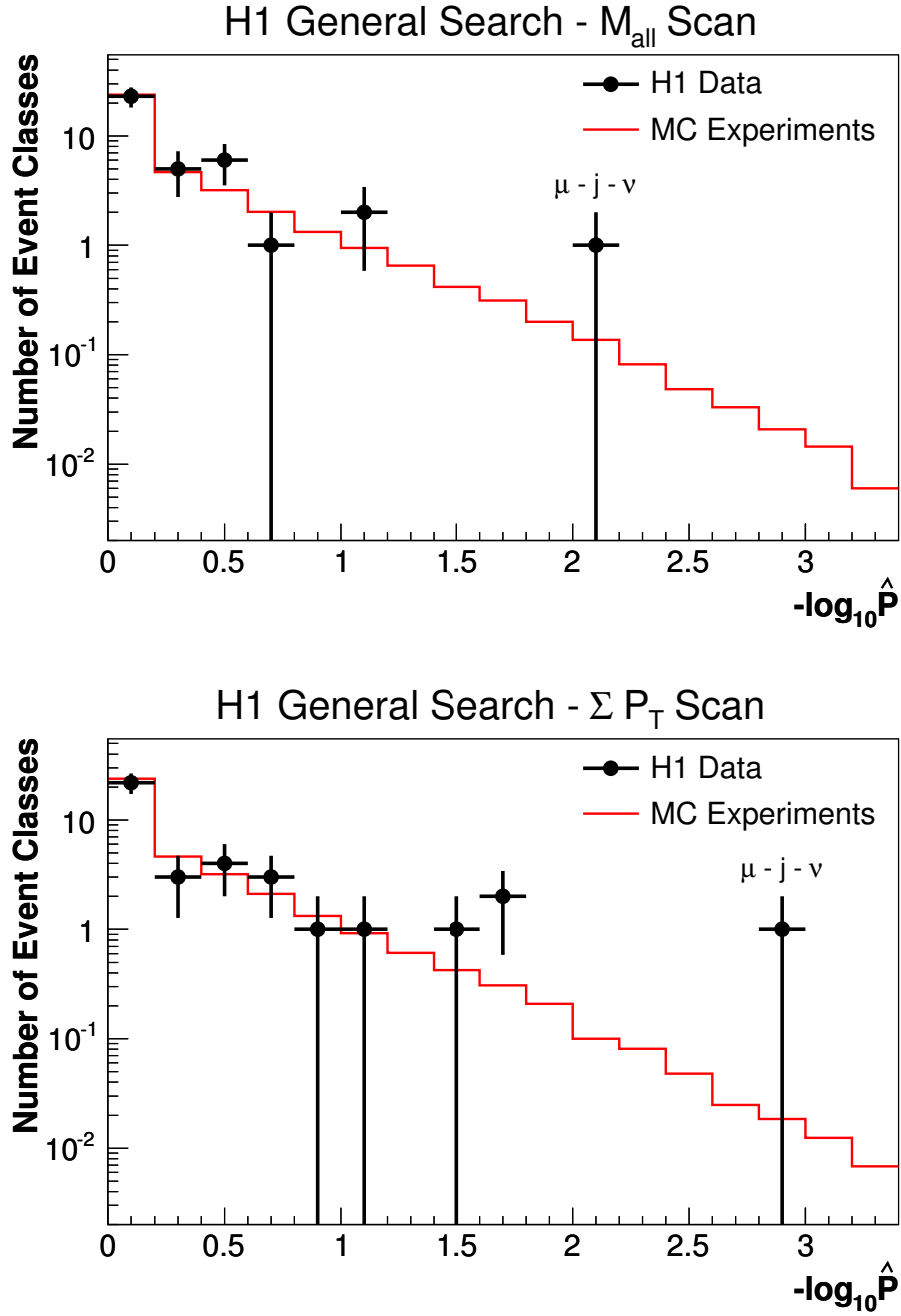
Fig. 7.7: The -\log_{10} \hat{P} values for the data event classes and the expected distributions from MC experiments as derived by investigating the M_{all} distributions (upper figure) and \Sigma P_T distributions (lower figure) with the search algorithm.
