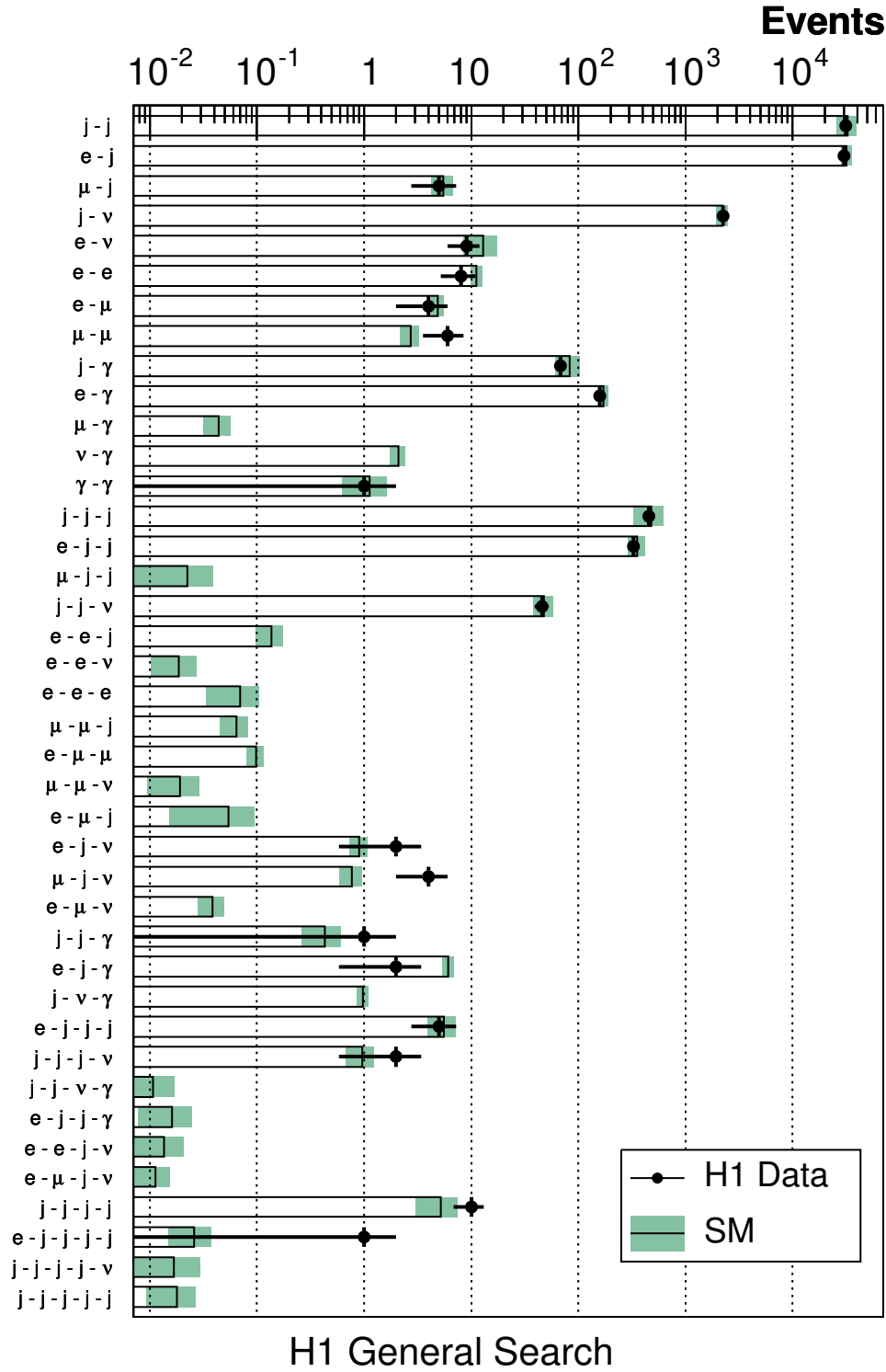
Fig. 6.1: The data and the SM expectation for all event classes with a SM expectation greater than 0.01 events as derived from the investigation of the complete HERA-I data sample.
