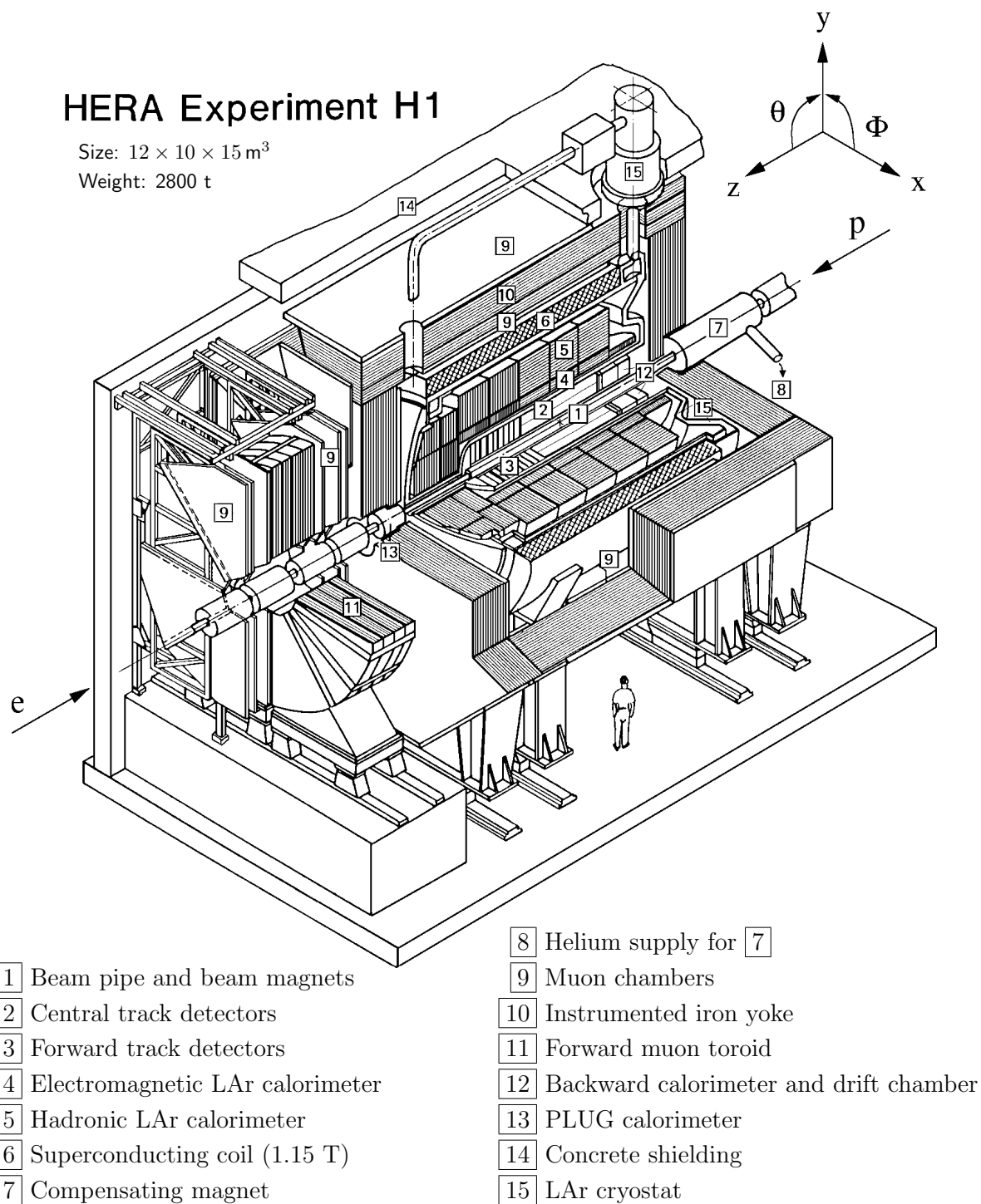
Fig. 2.3: Isometric view of the H1 detector at HERA.
