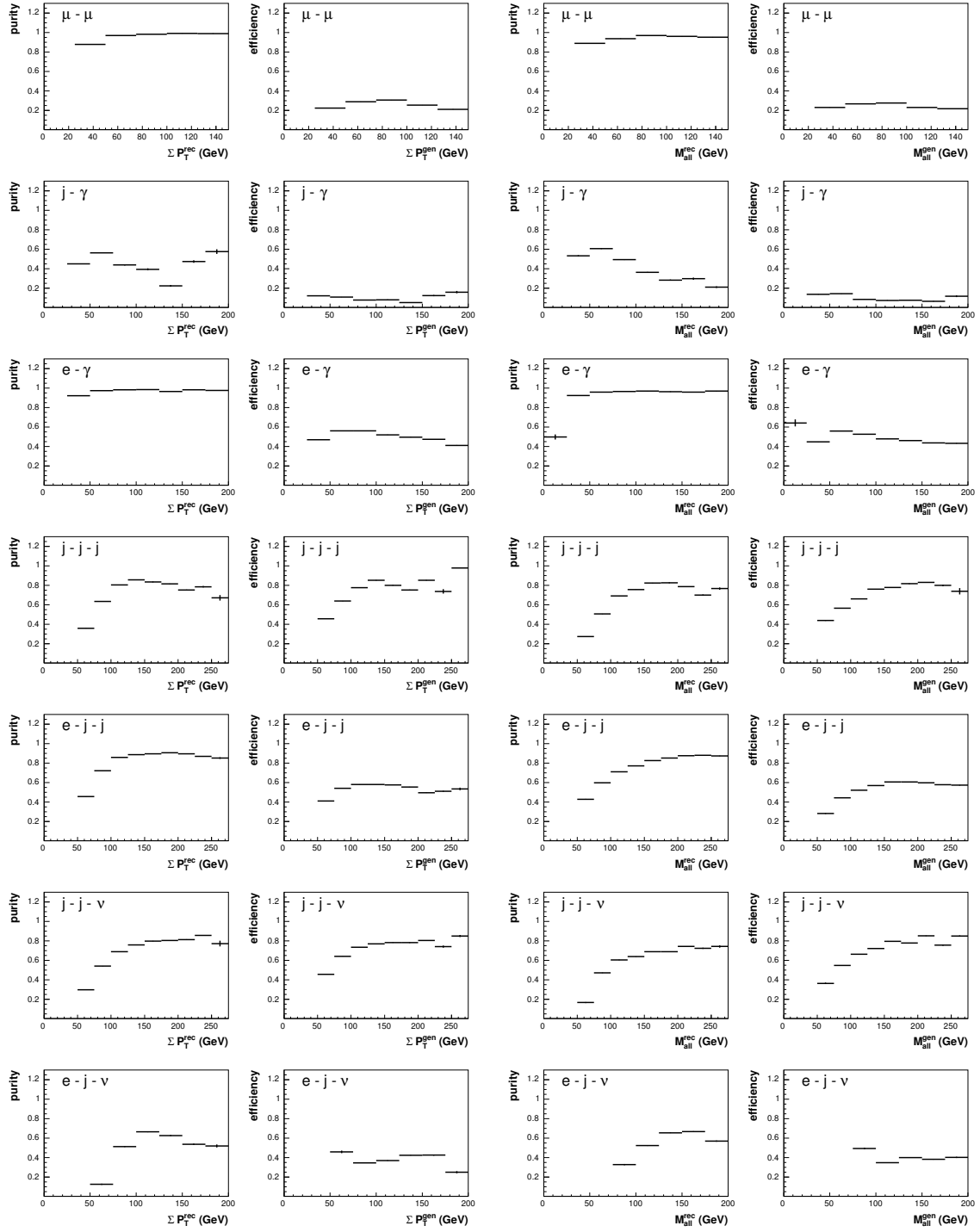
Fig. B.2: Purities and efficiencies as a function of the sum of transverse momenta \Sigma P_T (left side) and the invariant mass M_{\text{all}} (right side) for event classes containing data events.
