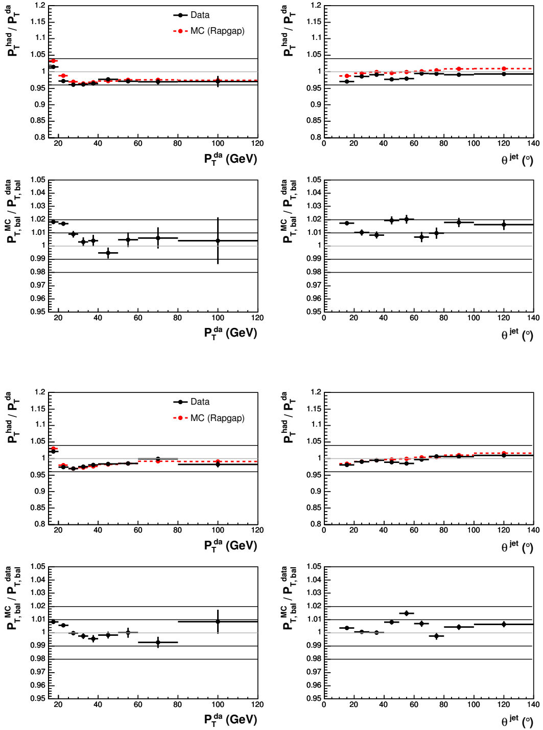
Fig. 5.3: The average values of the transverse momentum balance P_T^{\text{had}}/P_T^{\text{da}} as a function of P_T^{\text{da}} and \theta_{\text{jet}} determined from data and Monte Carlo as well as the relative hadronic energy scale for the run period 1994-1997 (upper figures) and 1998-2000 (lower figures).
