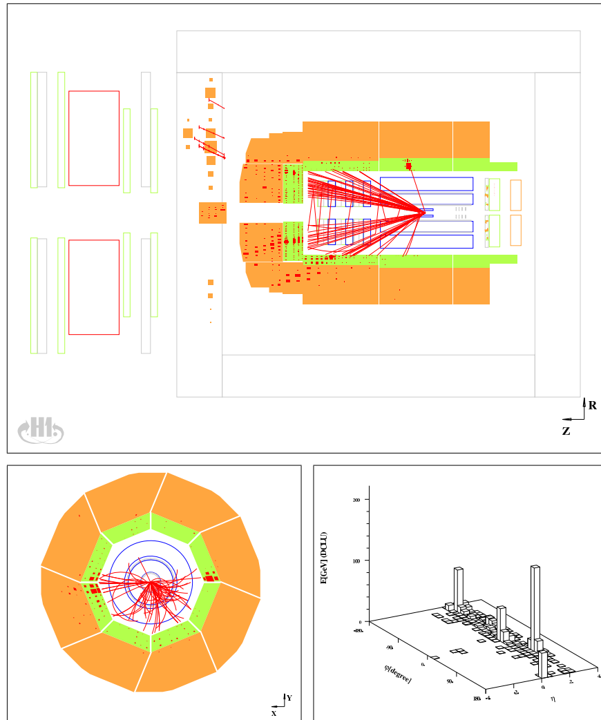
Fig. D.1: The event display of the e - j - j - j event. Shown are the side view ( rz -plane), the radial view ( xy -plane) and the energy flow in the \eta\phi -plane.
