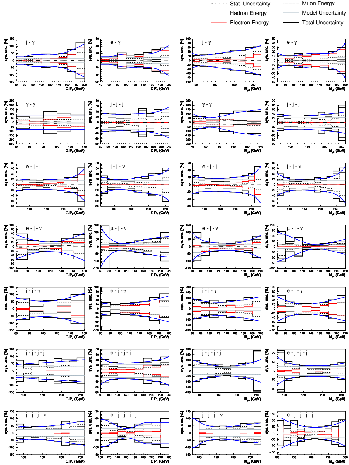
Fig. C.2: Systematic uncertainties on the predicted number of events as a function of \sum P_T (left side) and M_{all} (right side) for event classes containing data events. Only the total uncertainty and the corresponding fit as well as the uncertainties arising from the energy measurements and the Monte Carlo statistics are shown.
