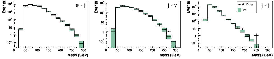
Fig. 6.2: The distributions of the invariant mass M_{all} for the e-j , j-\nu and j-j event classes.
