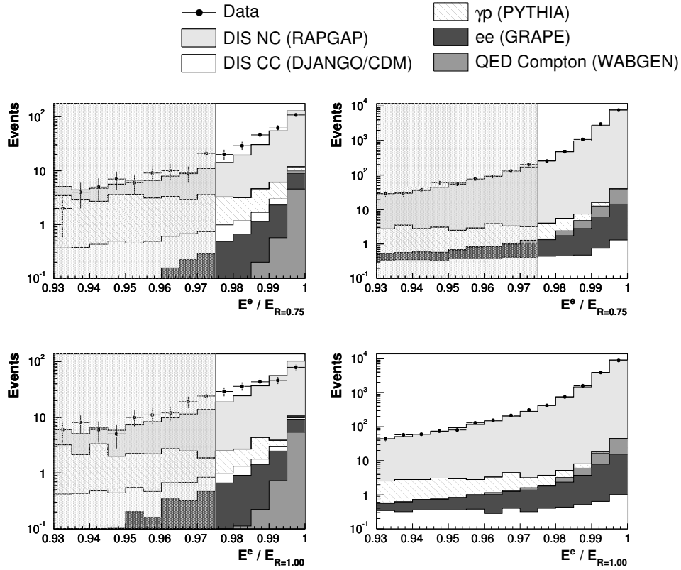
Fig. 4.2: The fraction of the electron energy in the isolation cone R = 0.75 and R = 1.00 for electron candidates in the forward (left side) and central (right side) region.
