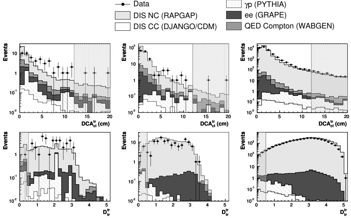
Fig. 4.3: The track cluster distance DCA_{cl}^{tr} and the distance between the electron track and the nearest good track D_{tr}^{tr} for electron candidates in the very forward (left side), transition (middle) and central (right side) region.
