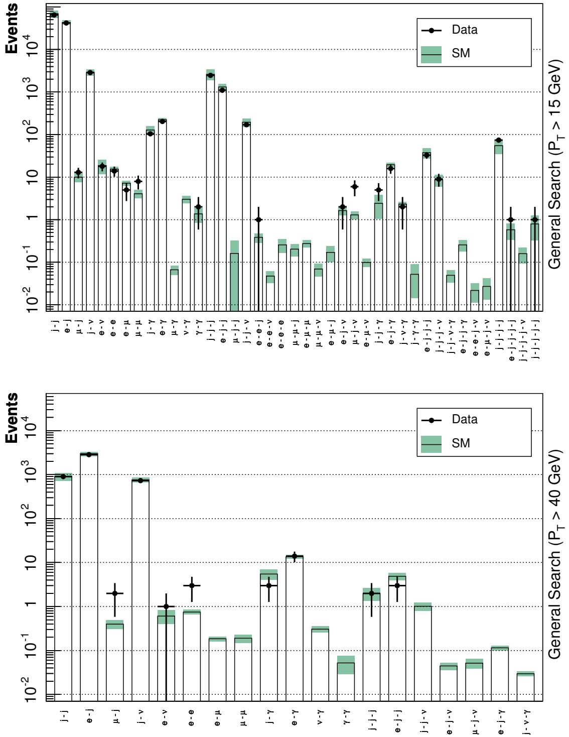
Fig. 6.8: The data and SM expectation for all event classes with a SM expectation greater than 0.01 events as derived from the investigation of the event samples with the P_T cut lowered to 15 GeV (upper figure) and raised to 40 GeV (lower figure).
