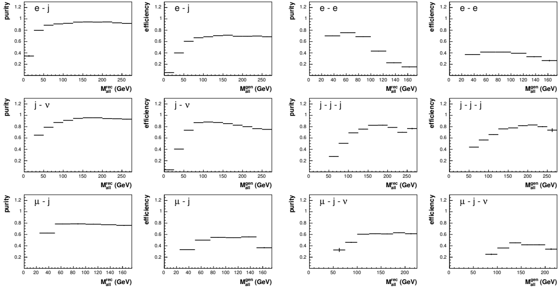
Fig. 5.9: Purities and efficiencies as a function of the invariant mass M_{all} for various event classes.
