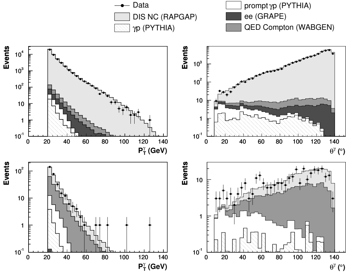
Fig. 4.10: The P_T and \theta distributions of the photon candidate before (upper figures) and after (lower figures) applying the identification criteria.
