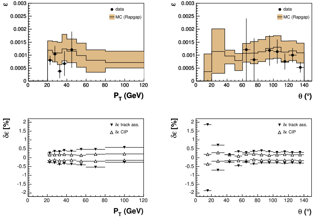
Fig. 4.12: The electron misidentification probability as a function of the transverse momentum P_T and the polar angle \theta (upper figures) and the contributing systematic errors of the electron track association and the CIP efficiencies (lower figures).
