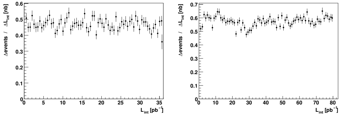
Fig. 4.1: The event yields as a function of the integrated luminosity for the run period 1994-1997 (left side) and 1998-2000 (right side) [41].
