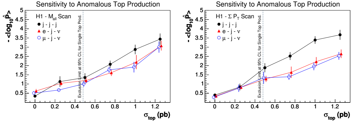
Fig. 7.3: The mean values of -\log_{10} \hat{P} as derived from BSM Monte Carlo experiments including a top signal with a cross section \sigma_{top} . Shown are the results of the j - j - j , e - j - \nu and \mu - j - \nu event classes corresponding to the typical top decay channels.
