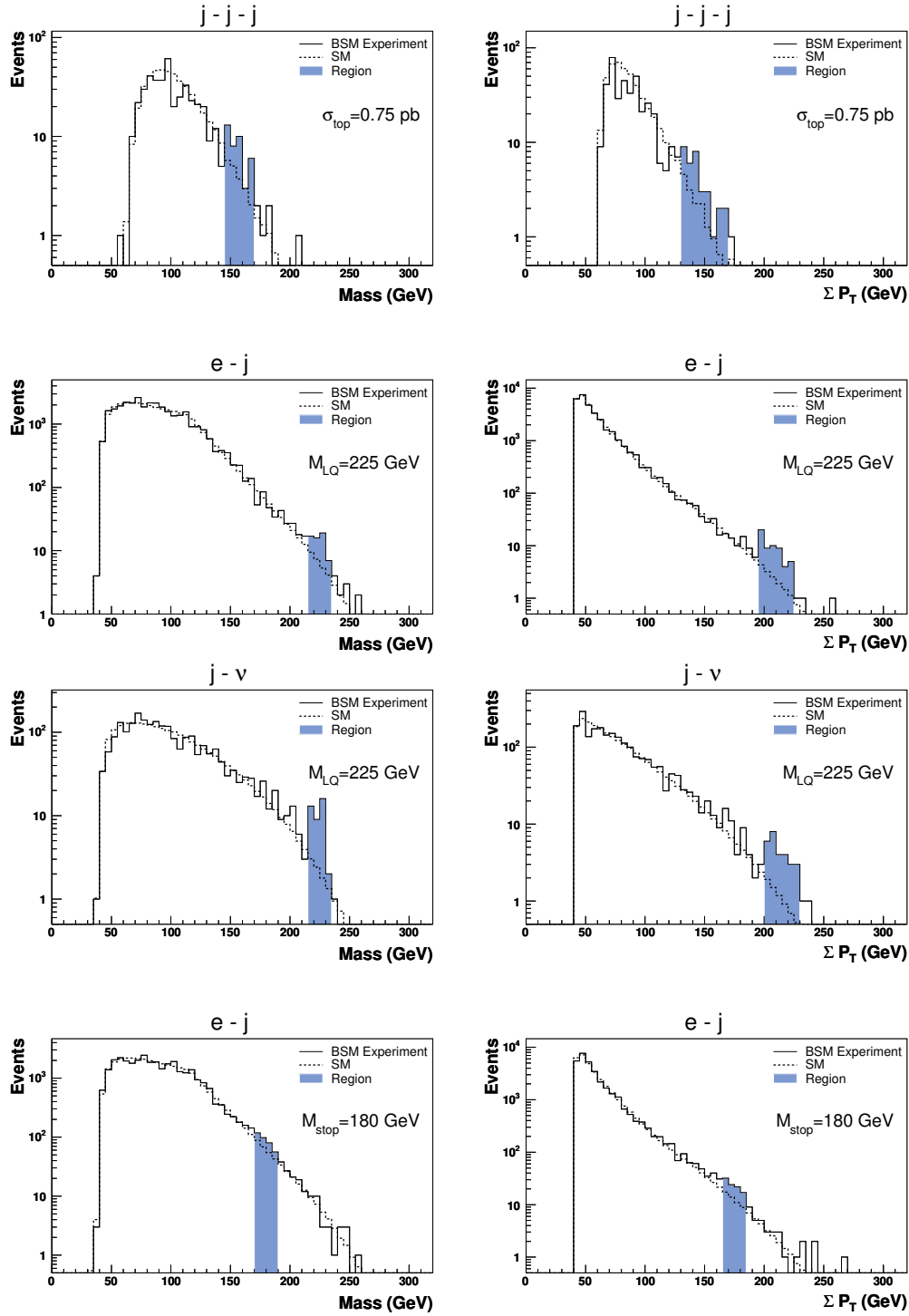
Fig. 7.6: The M_{all} and \sum P_T distributions obtained from BSM Monte Carlo experiments including various signals of new physics and the according SM distributions. The shaded areas show the regions of greatest deviation chosen by the search algorithm.
