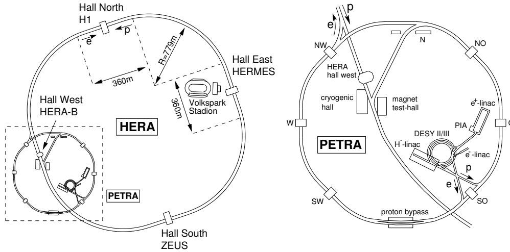
Fig. 2.1: The electron proton storage ring HERA (left) and the pre-accelerators at the DESY terrain (right). Electrons: linear accelerator LINAC II (450 MeV), synchrotron DESY II (8 GeV), synchrotron PETRA II (12 GeV). Protons: linear accelerator LINAC II (50 MeV), synchrotron DESY III (7.5 GeV), synchrotron PETRA II (40 GeV).
