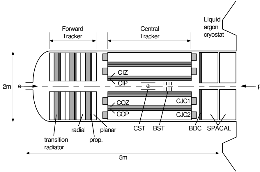
Fig. 2.4: Side view of the inner tracking system ( rz -plane).
