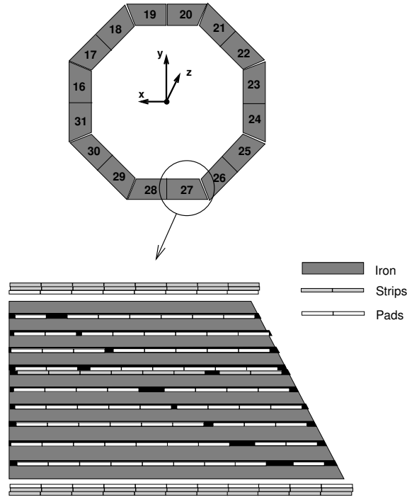
Fig. 2.7: Cross section of a module located in the backward barrel sector of the Central Muon Detector.
