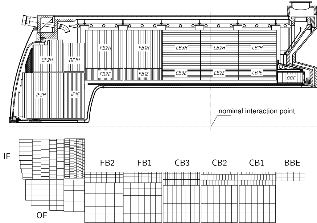
Fig. 2.6: Side view of the LAr calorimeter ( rz -plane). The eight wheels are labelled with BBE, CB1, CB2, CB3, FB1, FB2, OF and IF. The modules of the inlying electromagnetic section and the outer hadronic section are distinguished by the labels (E) and (H), respectively. The orientation of the absorber plates is displayed in the upper part of the figure while the lower part shows the cell configuration used in the read out.
