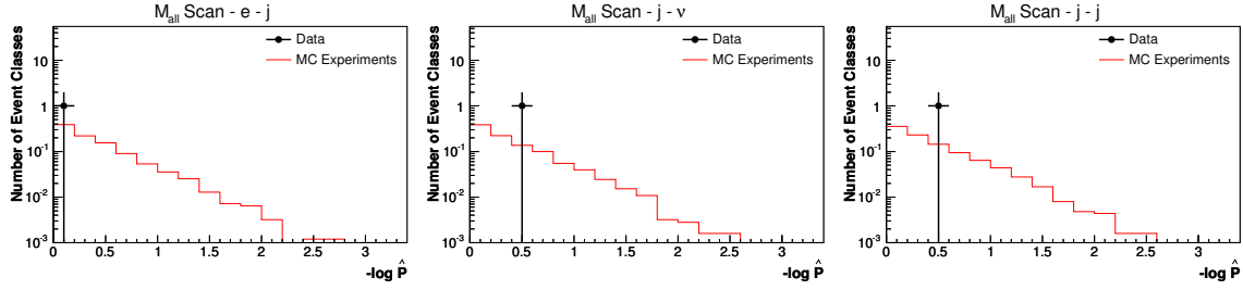
Fig. 7.2: The -\log_{10} \hat{P} values obtained from data for the e - j , j - \nu and j - j event classes and the expected distributions from HERA MC experiments as derived by investigating the invariant mass M_{all} distributions with the search algorithm.
