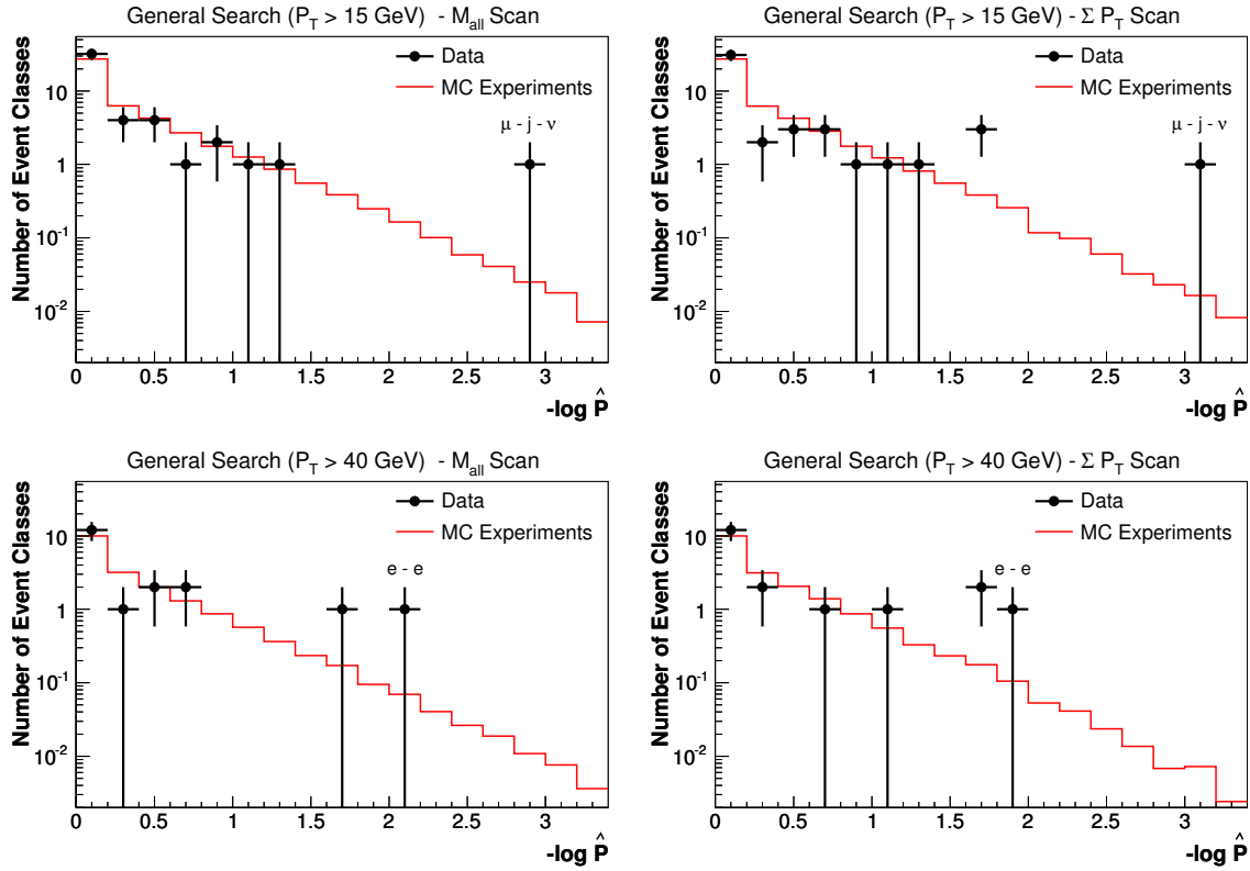
Fig. 7.8: The -\log_{10} \hat{P} values for the data event classes and the expected distributions from MC experiments as derived by investigating the M_{all} and \sum P_T distributions with the search algorithm for the event samples with the object P_T cut lowered to 15 GeV (upper figures) and raised to 40 GeV (lower figures).
