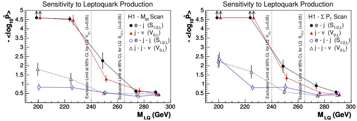
Fig. 7.4: The mean values of -\log_{10} \hat{P} as derived from BSM Monte Carlo experiments including a leptoquark signal with a mass M_{LQ} . S_{1/2,L} and V_{0,L} type leptoquarks have been considered, which are expected to manifest themselves in the e-j and e-j-j as well as in the j-\nu and j-j-\nu event classes, respectively.
