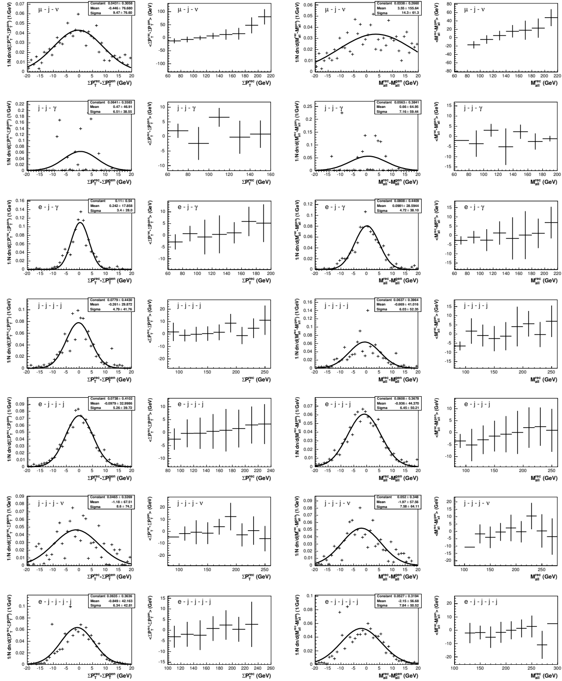
Fig. A.3: Resolutions of the sum of transverse momenta \Sigma P_T (left side) and the invariant mass M_{\text{all}} (right side) for event classes containing data events and the dependence of the resolutions on the reconstructed values of \Sigma P_T and M_{\text{all}} , respectively.
