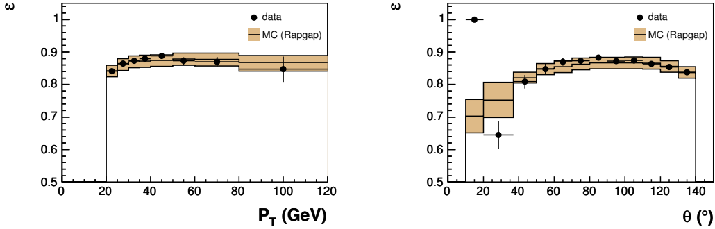
Fig. 4.8: The final electron track association efficiency as a function of the transverse momentum P_T (left side) and the polar angle \theta (right side).
