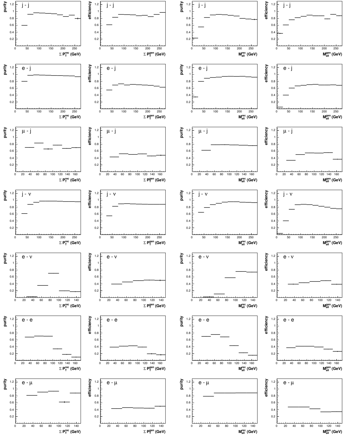
Fig. B.1: Purities and efficiencies as a function of the sum of transverse momenta \Sigma P_T (left side) and the invariant mass M_{\text{all}} (right side) for event classes containing data events.
