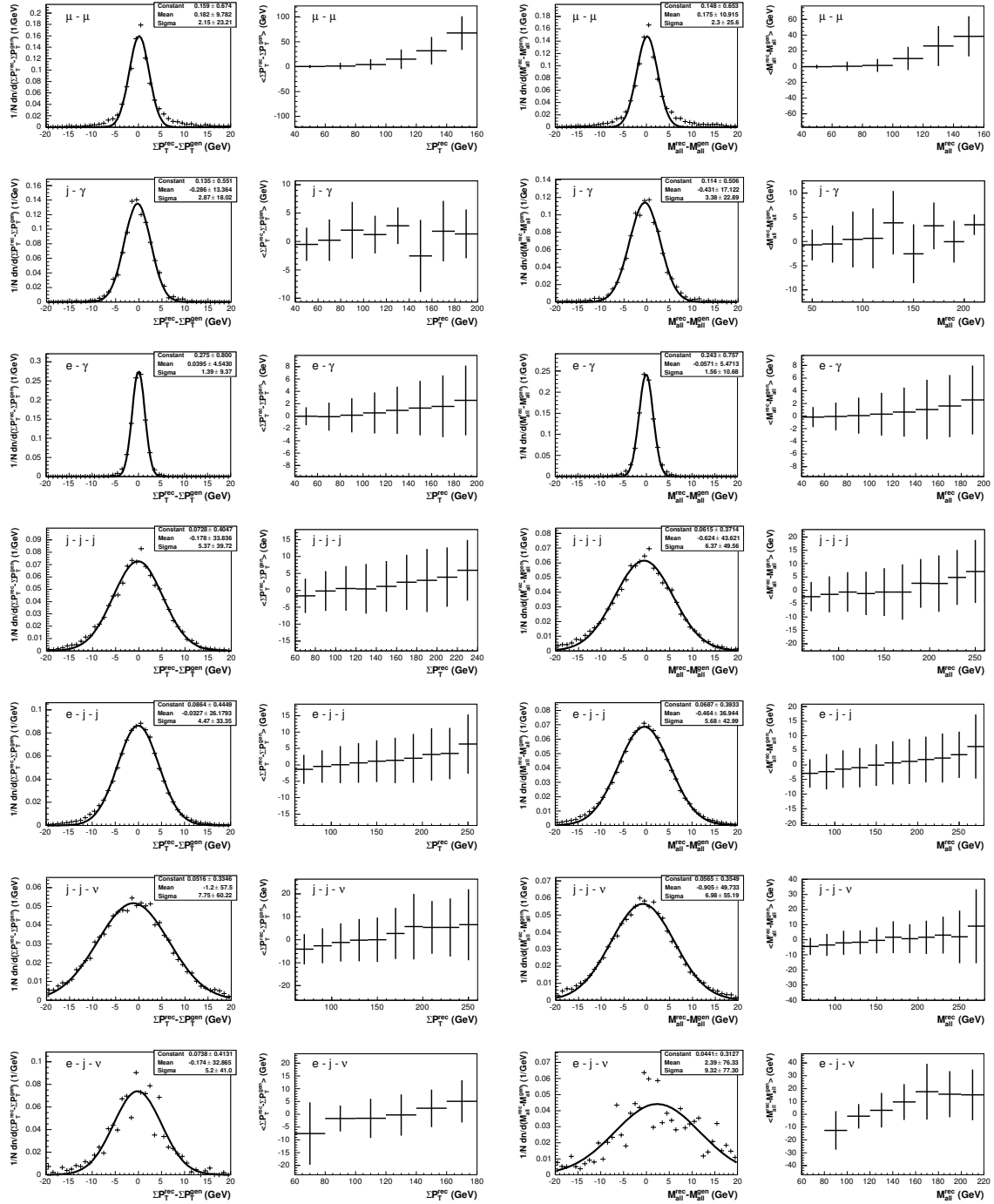
Fig. A.2: Resolutions of the sum of transverse momenta \Sigma P_T (left side) and the invariant mass M_{all} (right side) for event classes containing data events and the dependence of the resolutions on the reconstructed values of \Sigma P_T and M_{all} , respectively.
