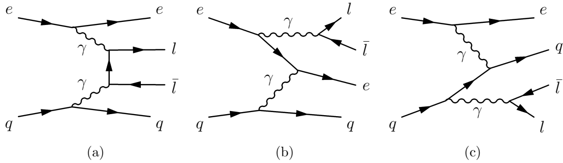
Fig. 1.7: Diagrams for lepton pair production in inelastic electromagnetic ep scattering. Figure (a) shows the t -channel diagram of the two-photon process. The radiation processes displayed in figure (b) and (c) are known as Cabibbo-Paresi and Drell-Yan process, respectively.
