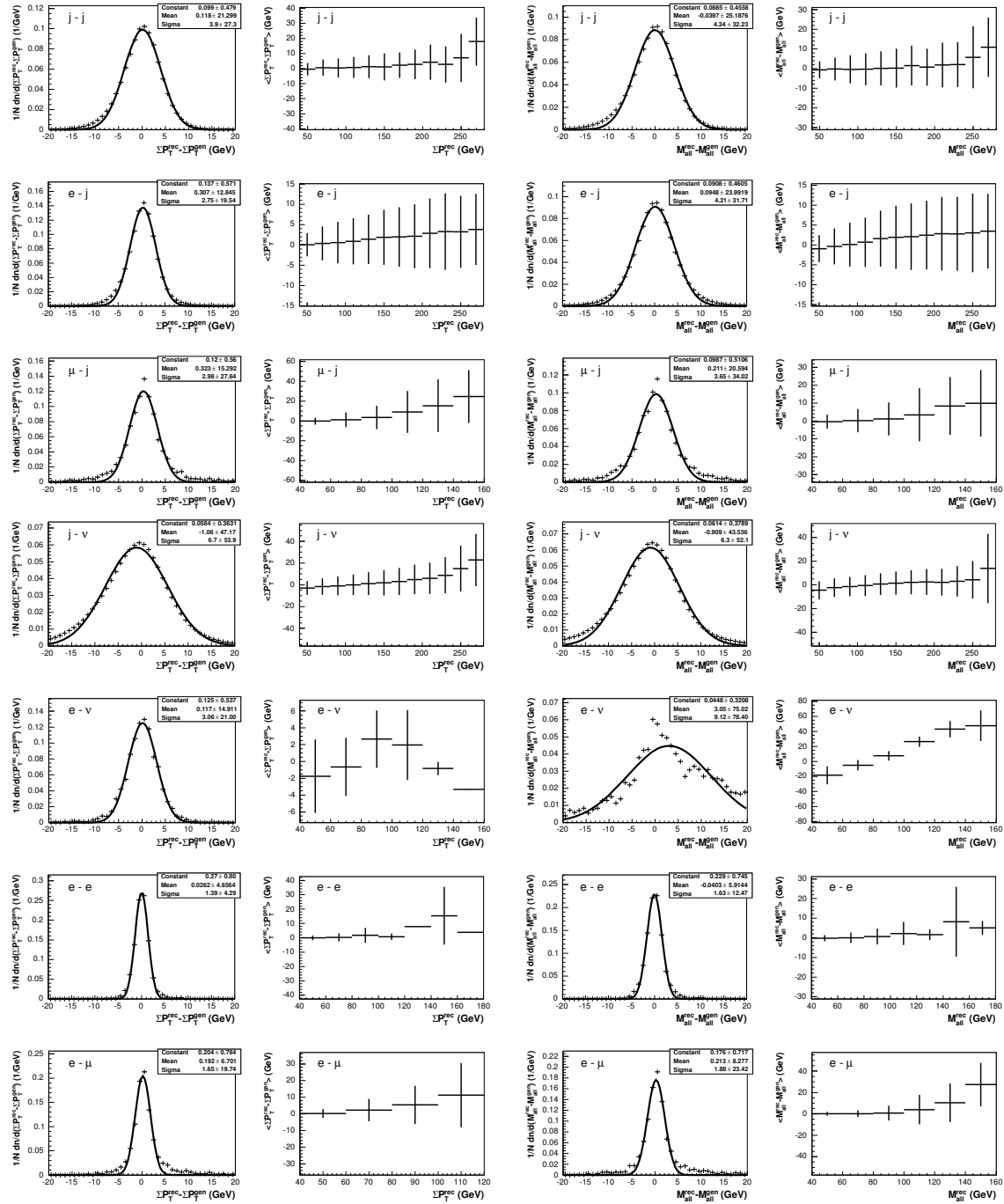
Fig. A.1: Resolutions of the sum of transverse momenta \Sigma P_T (left side) and the invariant mass M_{\text{all}} (right side) for event classes containing data events and the dependence of the resolutions on the reconstructed values of \Sigma P_T and M_{\text{all}} , respectively.
