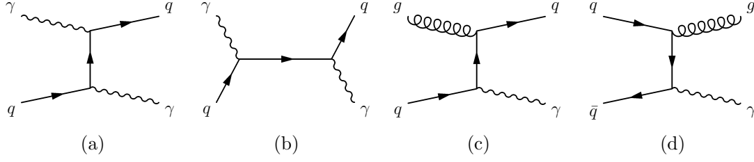
Fig. 1.4: Example diagrams for direct (a-b) and resolved (c-d) prompt photon production processes at leading order.
