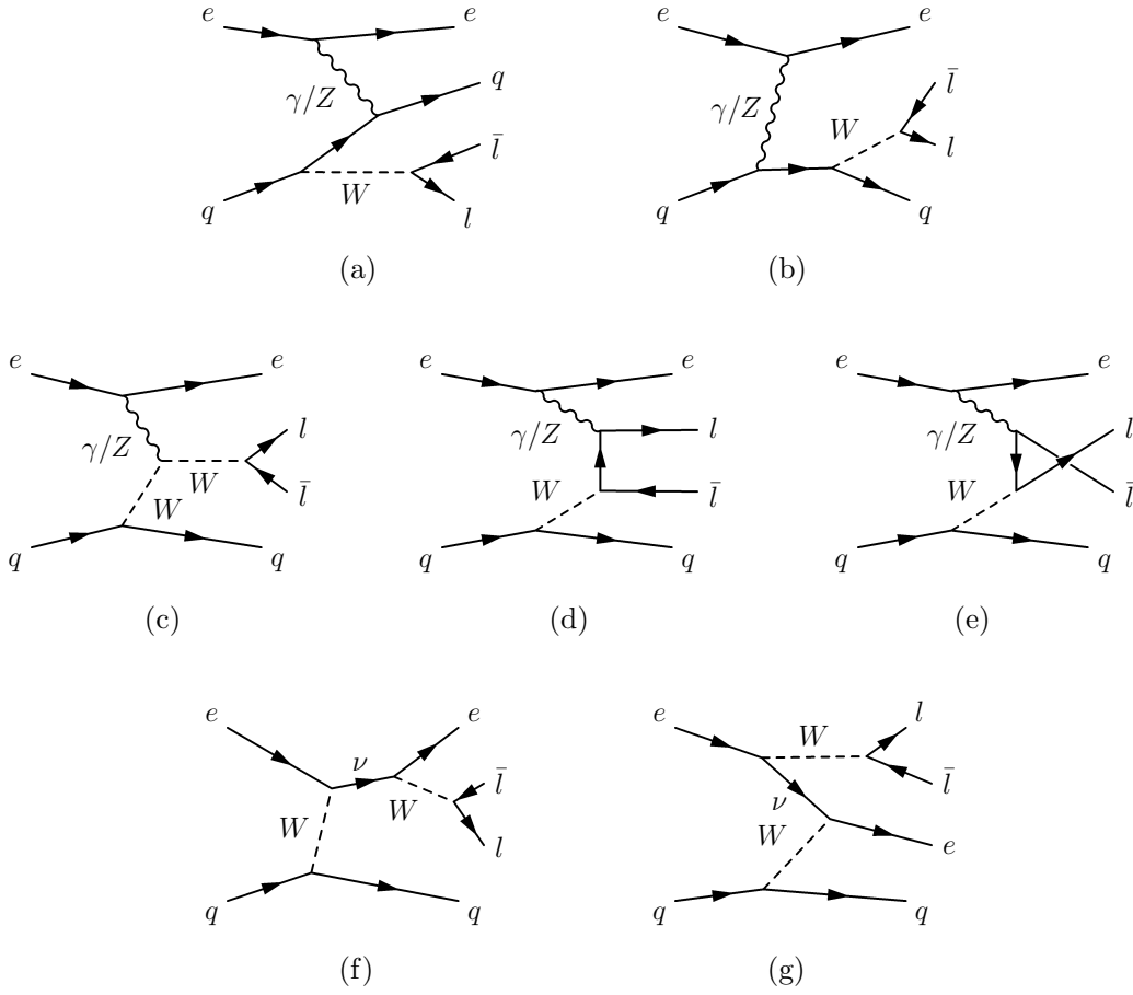
Fig. 1.8: Diagrams for real W production via the process ep \rightarrow eWX , including the subsequent decay into fermion pairs.
