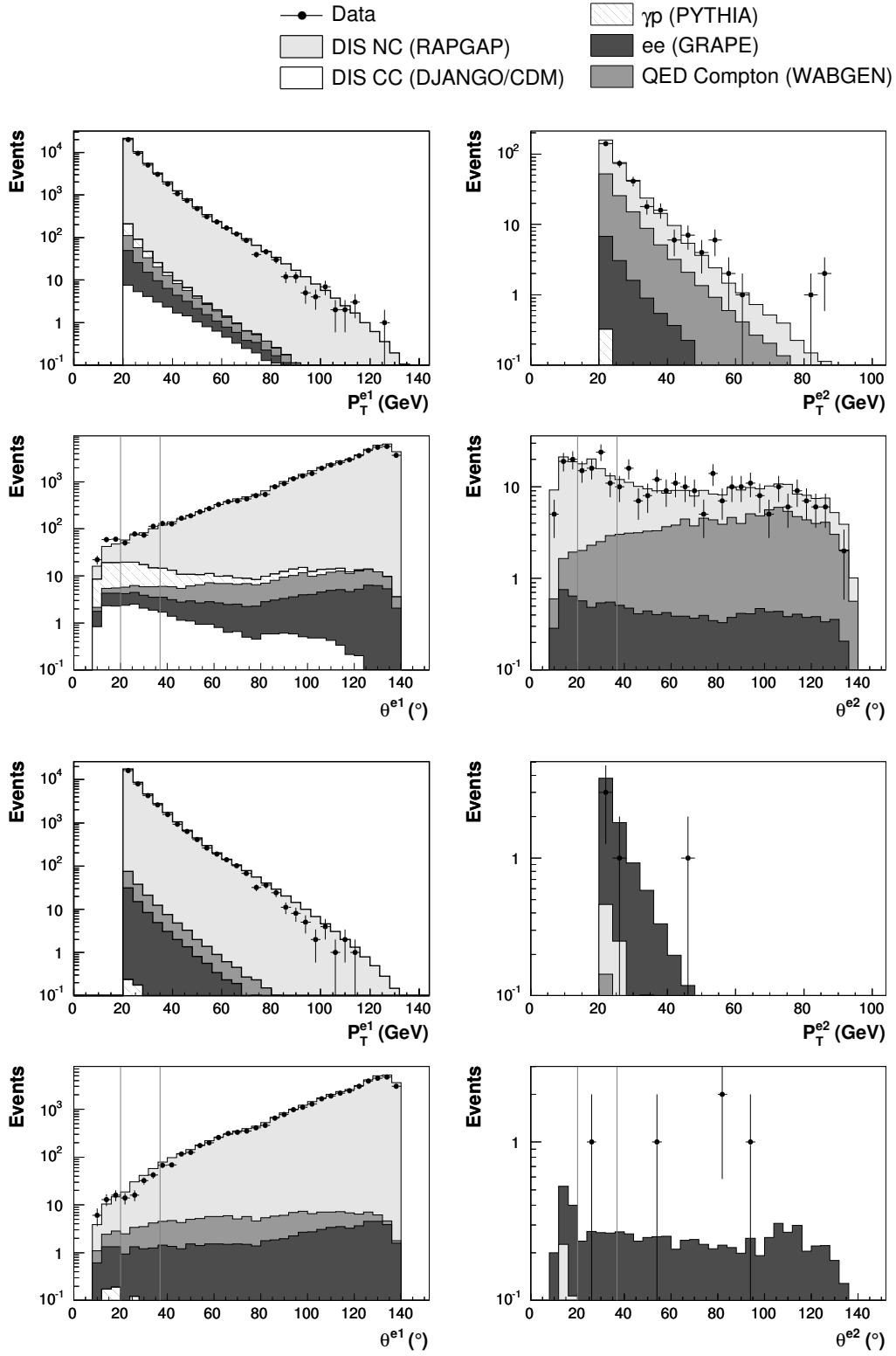
Fig. 4.6: The P_T and \theta distributions for the first (left side) and second (right side) electron candidate before (upper figures) and after (lower figures) applying the electron identification criteria. The vertical lines in the \theta distributions indicate the three different polar angle regions.
