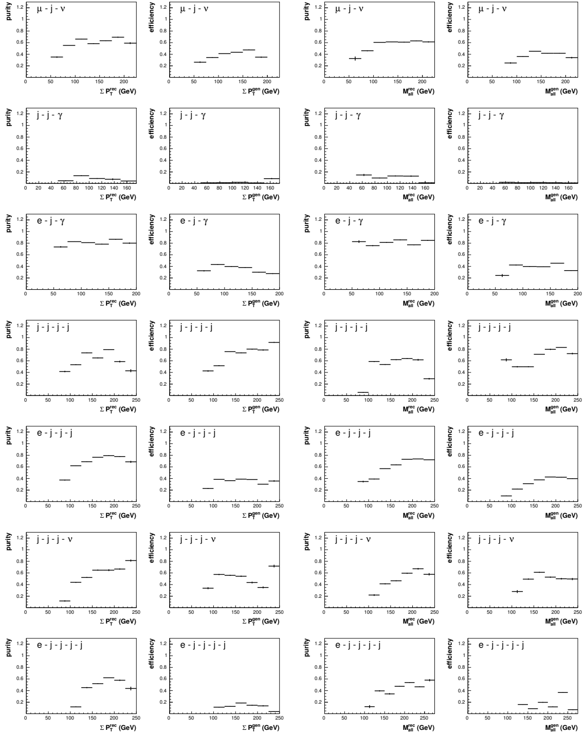
Fig. B.3: Purities and efficiencies as a function of the sum of transverse momenta \Sigma P_T (left side) and the invariant mass M_{\text{all}} (right side) for event classes containing data events.
