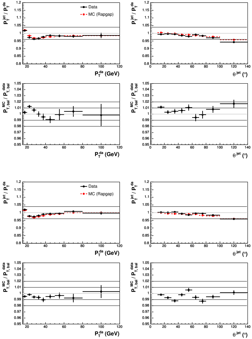
Fig. 5.2: The average values of the transverse momentum balance P_T^{jet}/P_T^{da} as a function of P_T^{da} and \theta_{jet} determined from data and Monte Carlo as well as the relative hadronic energy scale for the run period 1994-1997 (upper figures) and 1998-2000 (lower figures).
