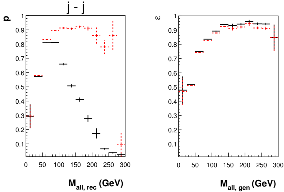
Fig. 4.13: Purity (left side) and efficiency (right side) before (solid line) and after (dashed line) the application of the jet identification criteria as a function of M_{all} of the selected jets in the j - j event class. The subscripts rec and gen denote the reconstructed and generated quantity [41].
