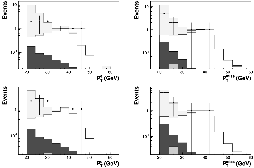
Fig. 5.5: The distributions of P_T^e and P_T for the e-\nu event class before (upper figures) and after (lower figures) re-weighting the NC DIS prediction.
