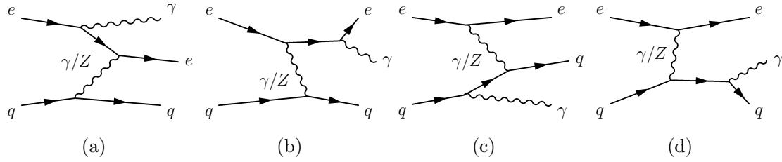
Fig. 1.5: The diagrams for real photon radiation in neutral current ep scattering. Figure (a) and (b) represent the initial and final state photon radiation from the electron line, diagrams (c) and (d) the corresponding processes for the quark line.
