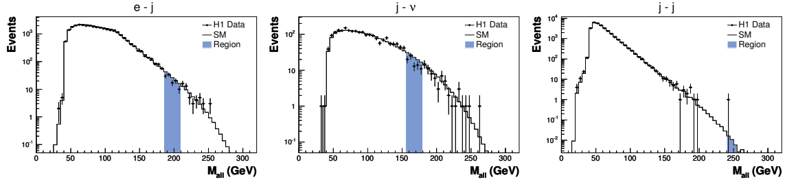
Fig. 7.1: The distributions of the invariant mass M_{all} including the regions of greatest deviation chosen by the search algorithm for the e - j , j - \nu and j - j event classes.
