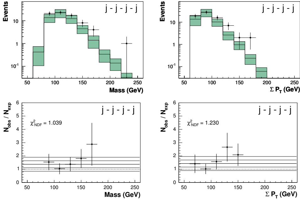
Fig. 5.11: The distributions of the invariant mass M_{all} and the sum of transverse momenta \sum P_T for the j - j - j - j event class obtained from a low- P_T jet sample (upper figures) and the ratio of the observed and expected number of events (lower figures). A constant function is fitted on the ratio distribution. Presented are the mean value as well as the regions containing one and two standard deviations.
