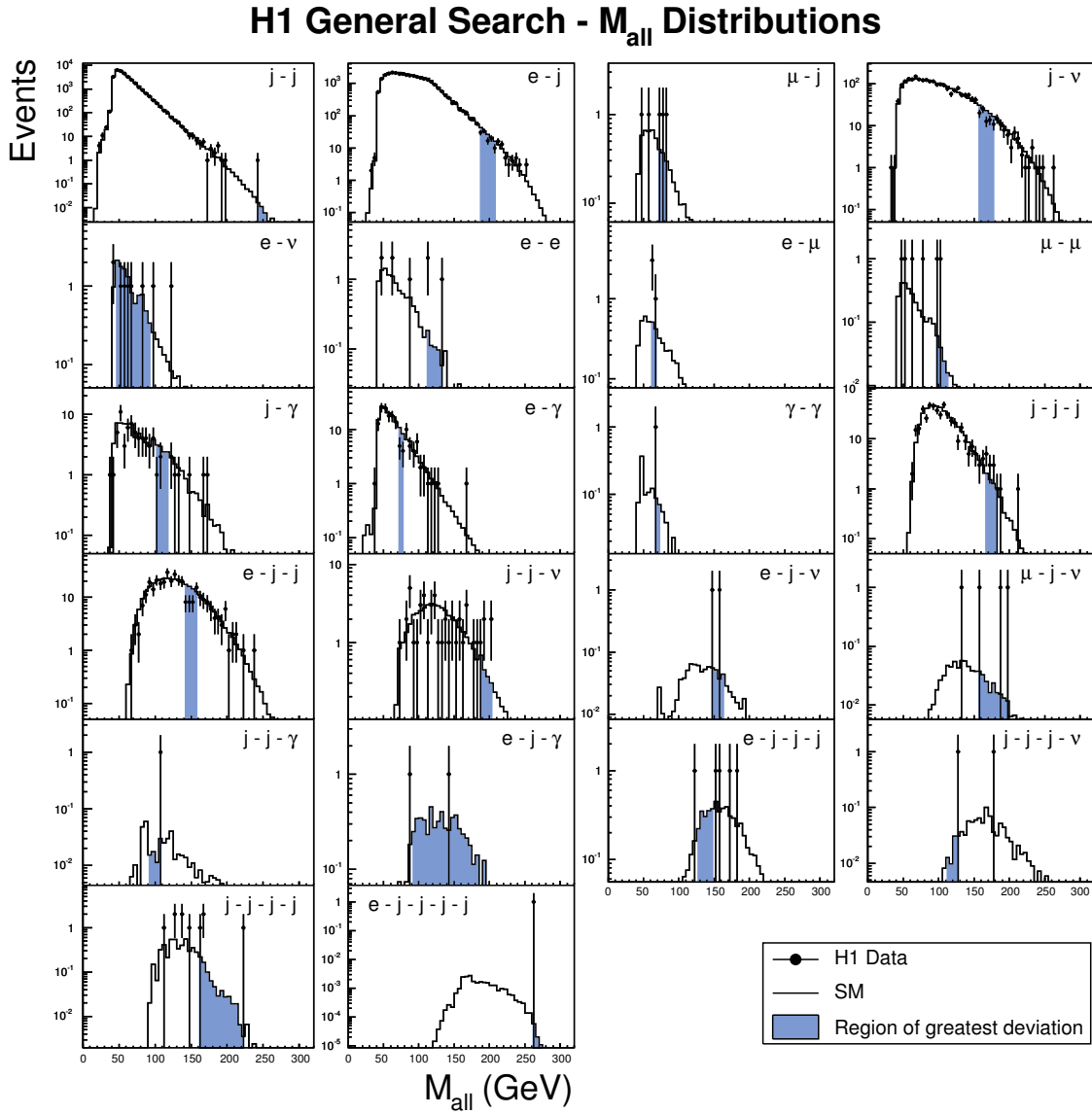
Fig. 7.9: The number of data events and the SM expectation as a function of M_{all} for event classes with observed data events. The shaded areas show the regions of greatest deviation chosen by the search algorithm.
