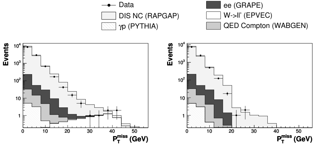
Fig. 5.4: The P_T distributions for events with \sum_i (E_i - P_{z,i}) < 48 \text{ GeV} obtained from an low- P_T electron sample. While the left figure is based on the inclusive sample, only events including electrons with P_T < 20 \text{ GeV} are considered for the distribution presented on the right side.
