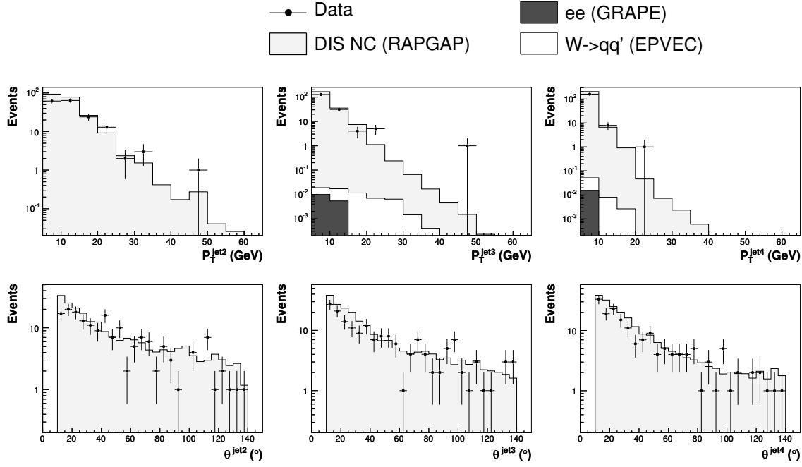
Fig. 5.12: The distributions of the transverse momentum P_T and polar angle \theta of the second, third and forth jet in a low- P_T e - j - j - j - j event sample.
