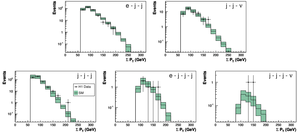
Fig. 6.5: The distributions of the sum of transverse momenta \sum P_T for the e - j - j and j - j - \nu as well as j - j - j , e - j - j - j and j - j - j - \nu event classes.
