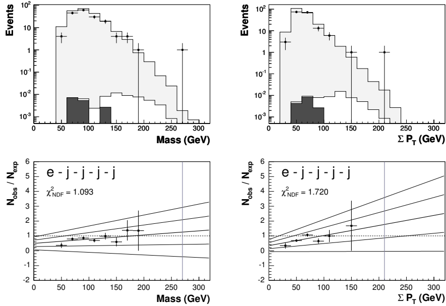
Fig. 5.13: The distributions of the invariant mass M_{\text{all}} and the sum of transverse momenta \Sigma P_T for the e - j - j - j - j event class obtained from a low- P_T event sample (upper figures) and the ratio of the observed and expected number of events (lower figures). A linear function is fitted on the ratio distribution. Presented are the mean value as well as the regions containing one and two standard deviations. The vertical lines denote the highest values of M_{\text{all}} and \Sigma P_T observed in the data.
