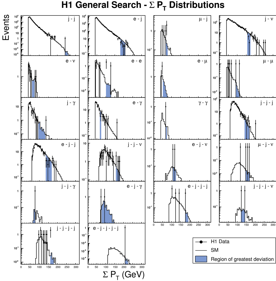
Fig. 7.10: The number of data events and the SM expectation as a function of \Sigma P_T for event classes with observed data events. The shaded areas show the regions of greatest deviation chosen by the search algorithm.
