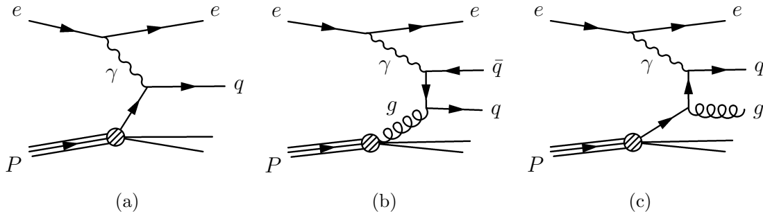
Fig. 1.2: Diagrams for jet production at lowest (a) and first order (b-c) of the strong coupling constant \alpha_s for the inelastic electromagnetic ep scattering. The processes displayed in figure (b) and (c) are known as Boson-Gluon fusion and QCD Compton scattering, respectively. For both processes only the t -channel contribution is shown.
