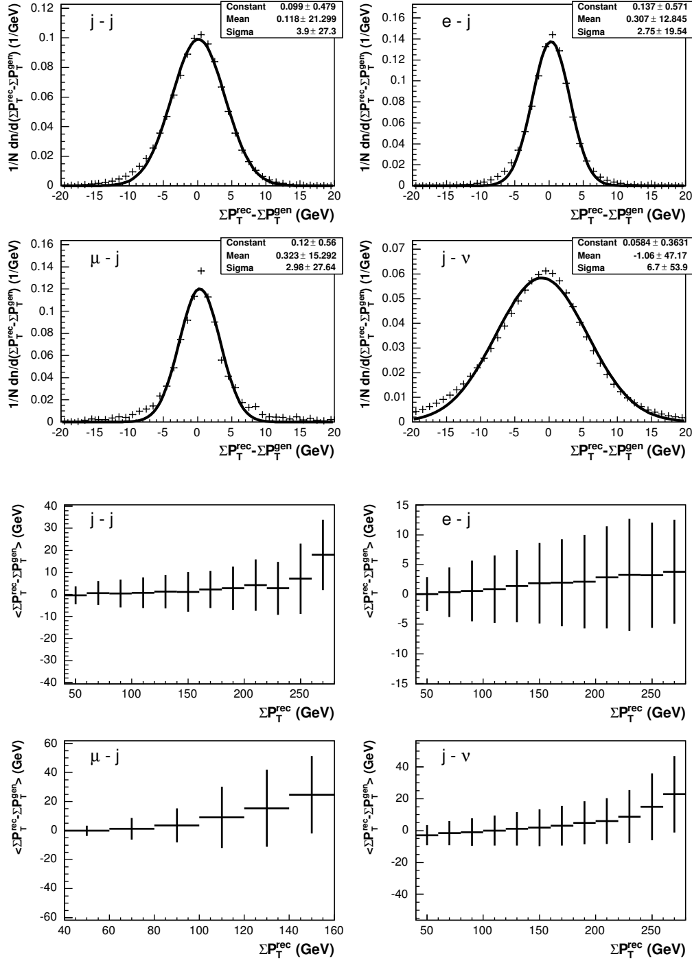
Fig. 5.8: The resolution of \sum P_T (upper figures) and its dependence on the reconstructed values of \sum P_T (lower figures) for the j - j , e - j , \mu - j and j - \nu event classes.
