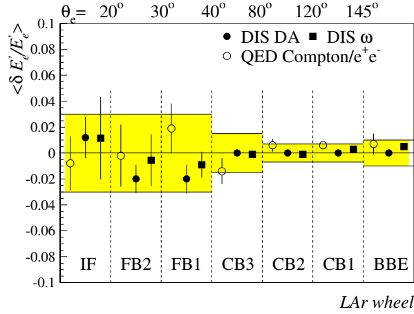
Fig. 5.1: Comparison of the electromagnetic energy scale as determined by different calibration methods. Shown is the mean fractional energy shift of the different methods from the absolute energy scale. The shaded error band shows the systematic uncertainty on the energy scale quoted on this analysis [51].
