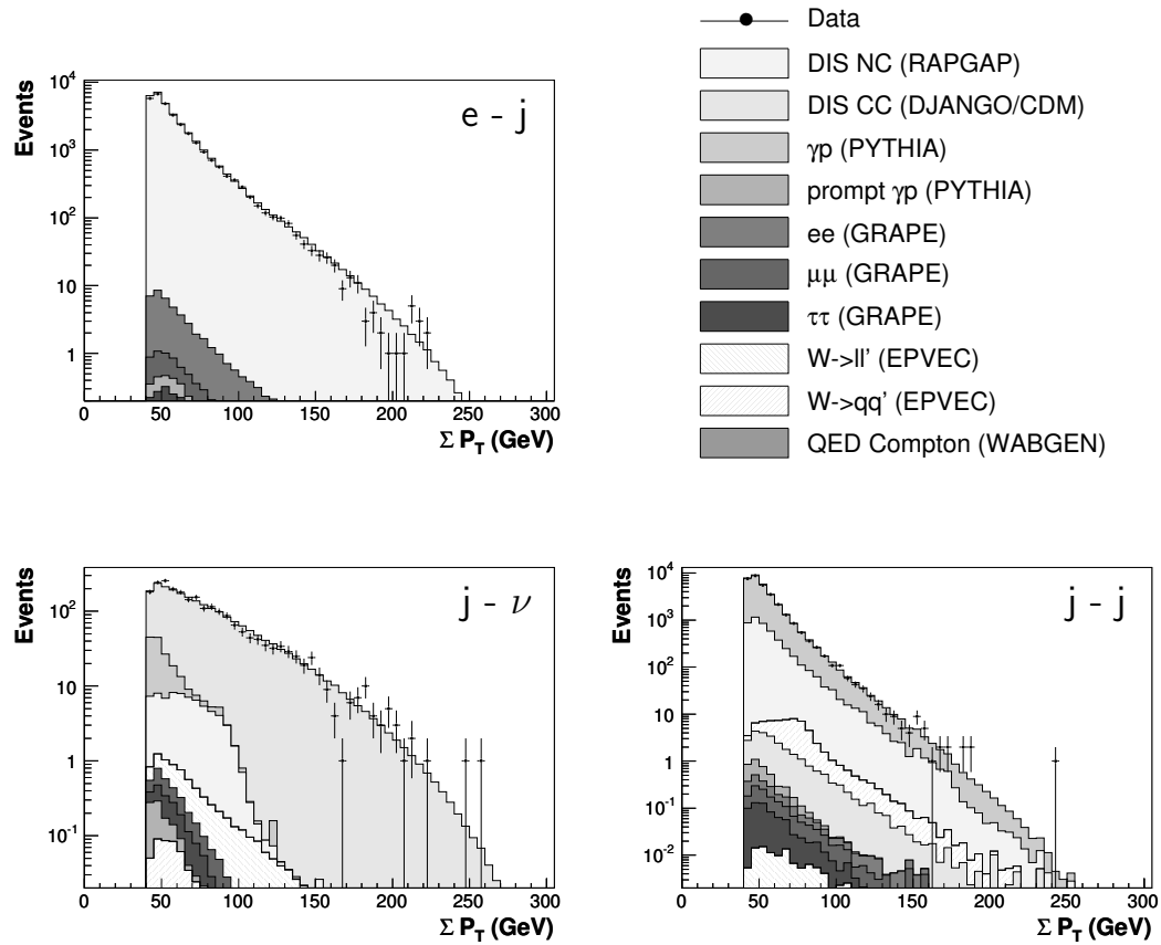
Fig. 4.14: The distributions of the sum of transverse momenta \Sigma P_T for the e-j (upper left), the j-\nu (lower left) and the j-j (lower right) event classes.
