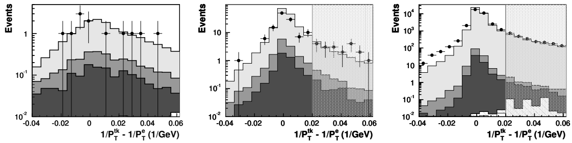
Fig. 4.5: The P_T -match value for electron candidates in the very forward (left side), transition (middle) and central (right side) region.
