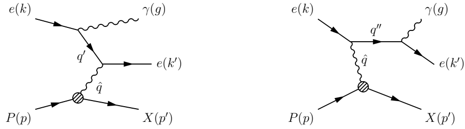
Fig. 1.6: The diagrams for the initial and final state photon radiation in electromagnetic ep scattering.
