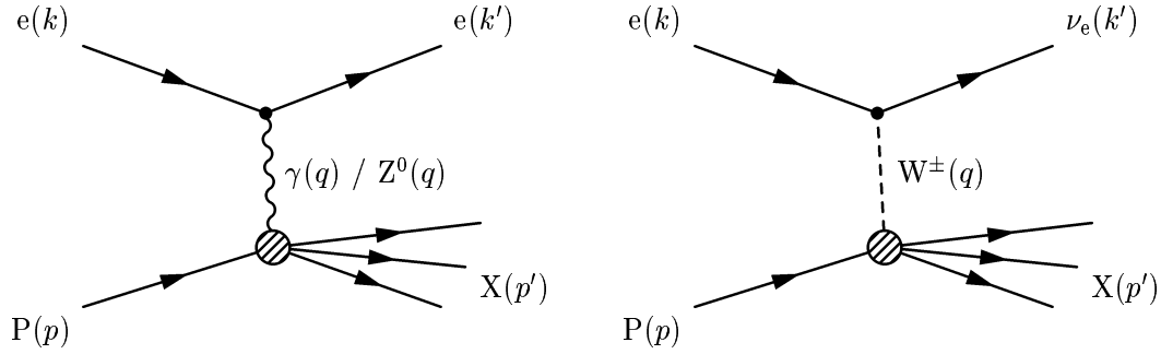
Fig. 1.1: The lowest-order diagrams of electron-proton scattering for neutral current processes (left) and charged current processes (right). The four-momenta of the particles or particle systems are given in parentheses.
