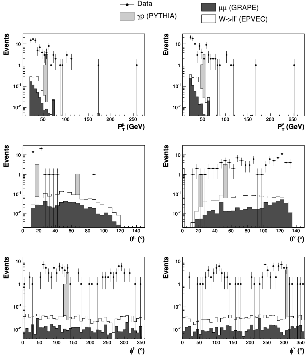
Fig. 5.6: The distributions of the transverse momenta P_T , the azimuth angles \phi and the polar angles \theta for the muon (left side) and neutrino (right side), reconstructed in the \mu - \nu event class.
