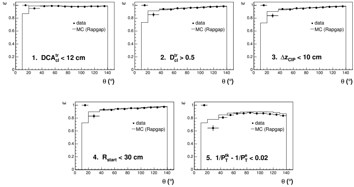
Fig. 4.7: The electron track association efficiency as a function of the polar angle \theta depending on the electron track criteria.
