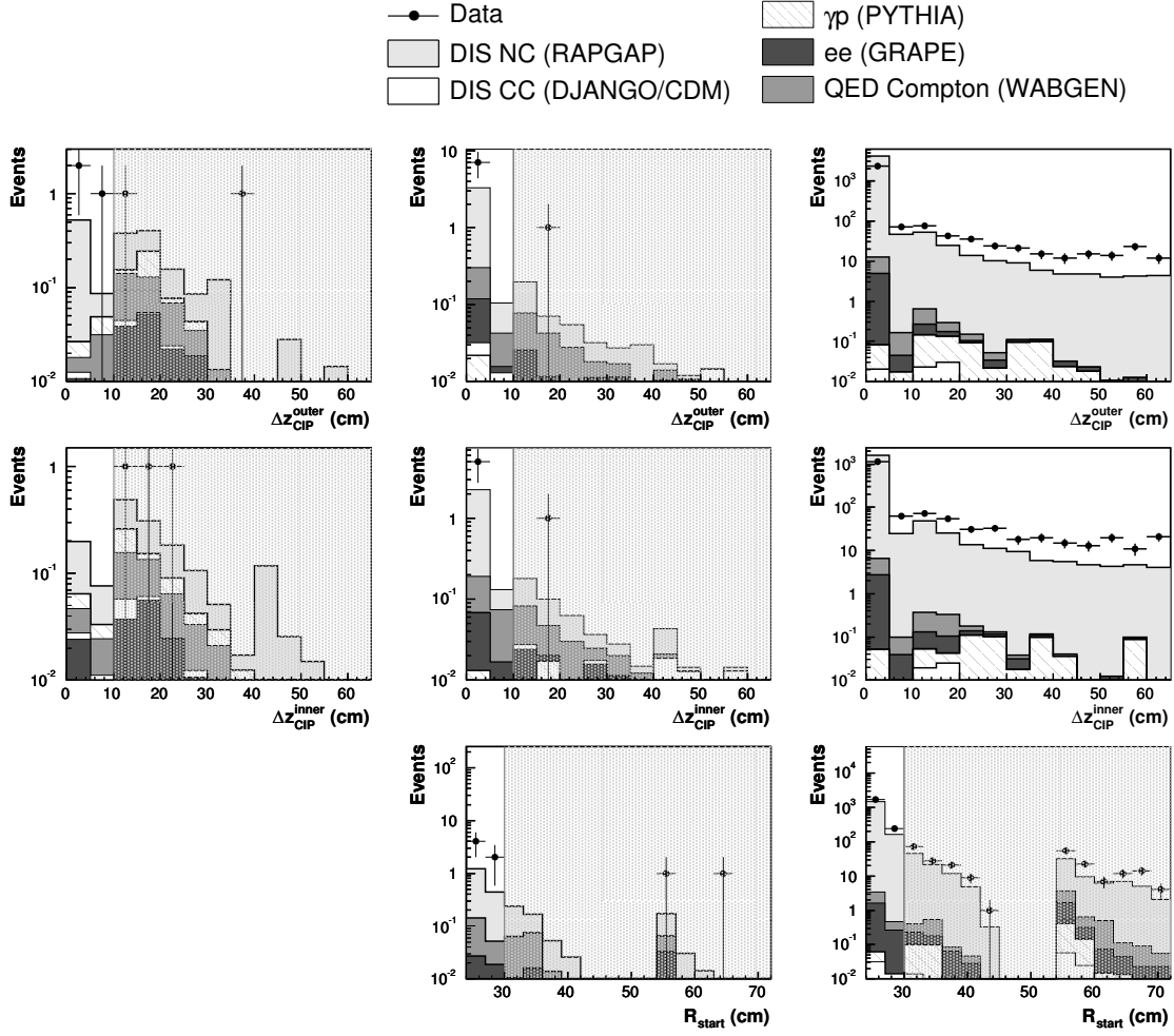
Fig. 4.4: The distance \Delta z_{CIP} for the outer and inner CIP layer and the radial distance R_{start} between the track and the beam axis for electron candidates in the very forward (left side), transition (middle) and central (right side) region.
