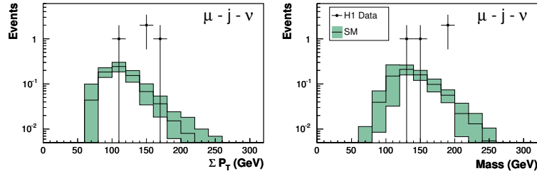
Fig. 6.4: The distributions of the sum of transverse momenta \sum P_T and invariant mass M_{all} for the \mu - j - \nu event class.
