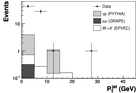
Fig. 5.7: The distribution of the transverse momentum P_T of the leading jet for the \mu - \nu event class.
