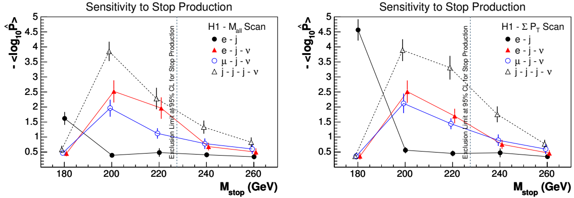
Fig. 7.5: The mean values of -\log_{10} \hat{P} as derived from BSM Monte Carlo experiments including a stop signal with a mass M_{stop} . Shown are the results of the e-j-\nu , \mu-j-\nu and j-j-j-\nu event classes as well as for the e-j event class, which are expected to be sensitive on the bosonic and direct decay of the stop quark, respectively.
