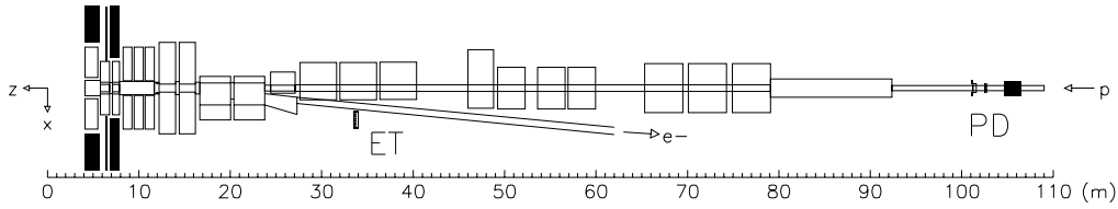
Fig. 2.8: Side view of the luminosity system of the H1 detector.
