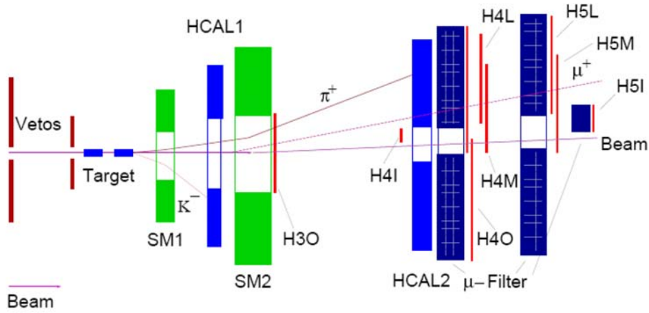
Figure 3.9: Schematic view of the trigger components in the experimental setup. In the shown event the trigger is activated by the planes H4L, H5L, H4M and H5M, which corresponds to a registered muon with Q^2 < 0.5 \text{ (GeV/c)}^2 . At the same time a pion is detected in HCAL2.
