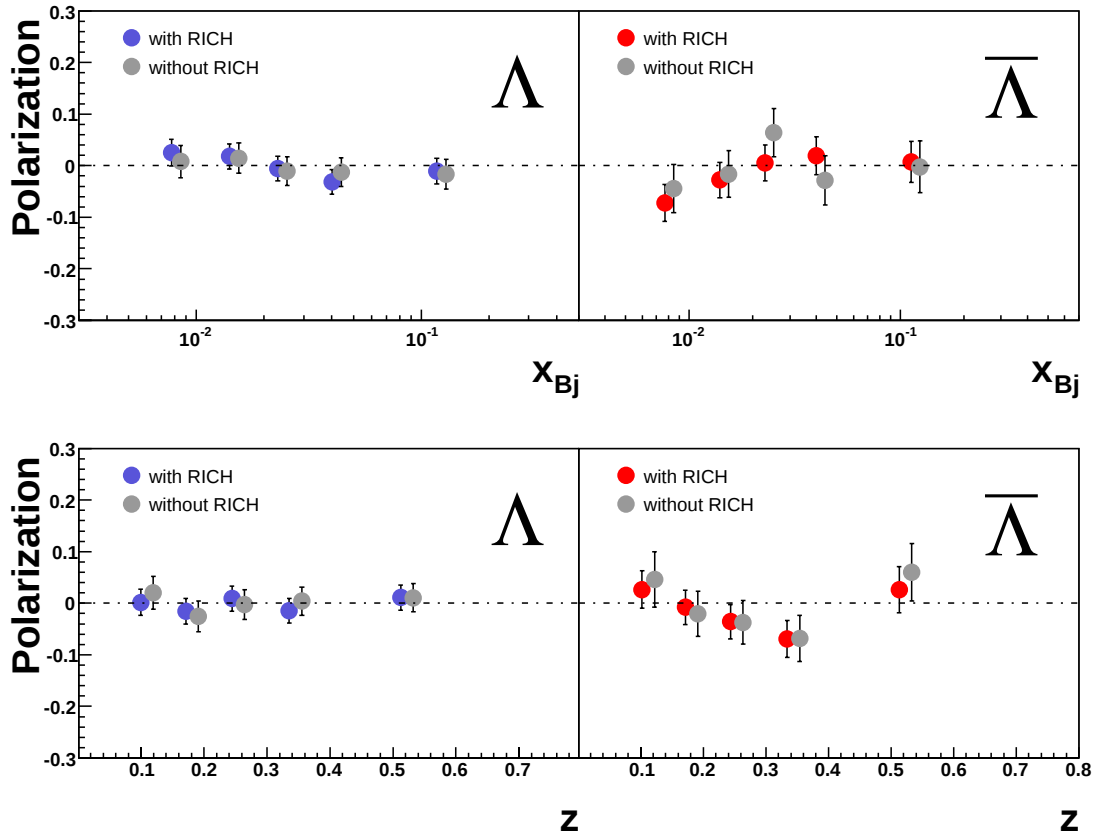
Figure 5.4: Dependence of the \Lambda and \bar{\Lambda} polarization on x_{Bj} and z with RICH cut and without RICH cut.
