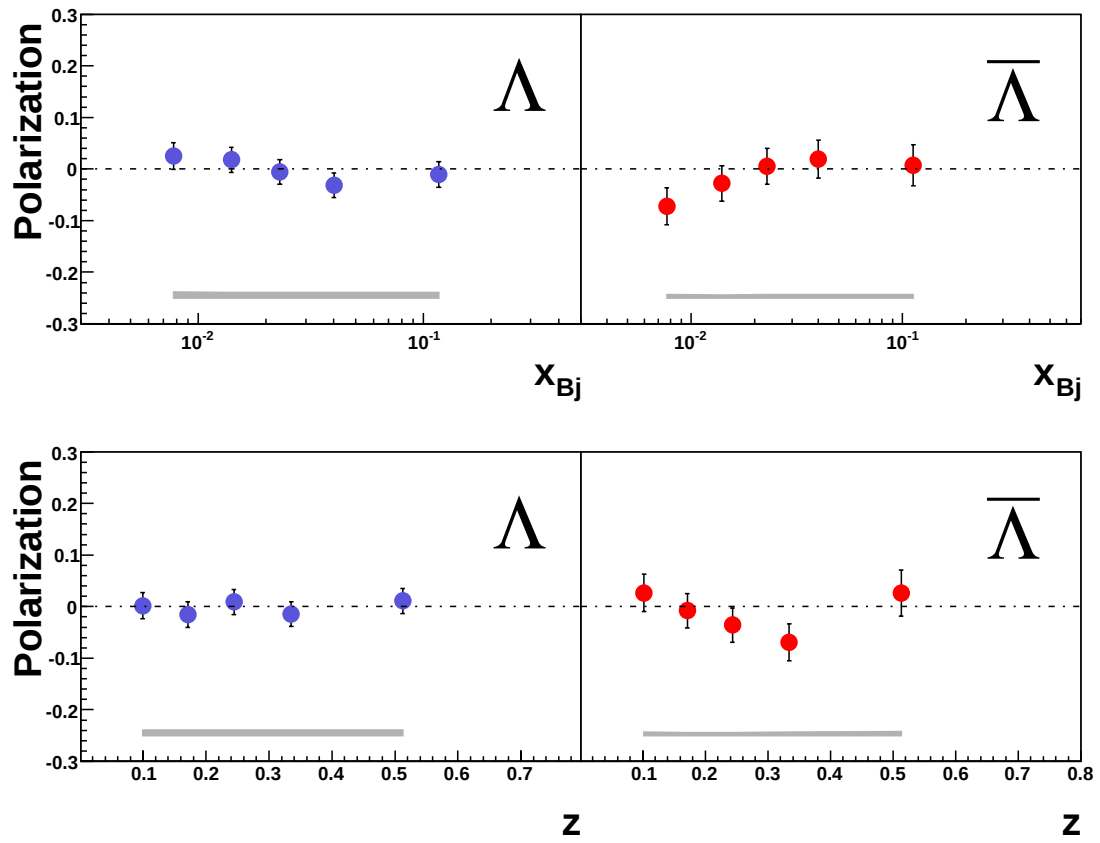
Figure 5.15: \Lambda and \bar{\Lambda} polarizations with statistical errors as a function of x_{Bj} and z in the 2007 data. The lower band shows the upper limit of the systematic error, estimated by the pulls distribution of false polarizations.
