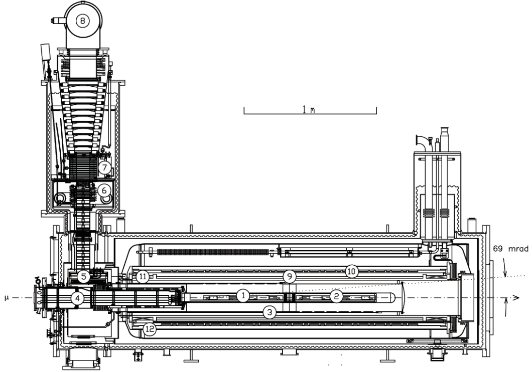
Figure 3.6: Side view of the COMPASS polarized target [72]: (1) upstream and (2) downstream target cell, (3) microwave cavity, (4) target holder, (5) still ^3\text{He} evaporator, (6) ^4\text{He} evaporator, (7) ^4\text{He} liquid/gas phase separator, (8) ^3\text{He} pumping port, (9) solenoid coil, (10-11) compensation coil, (12) dipole coil. The muon beam enters from the left. The two halves of the microwave cavity are separated by a thin microwave stopper.
