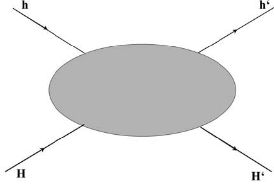
Figure 2.5: Sketch of the forward scattering amplitudes with helicities of quarks (h, h') and hadrons (H, H') .
