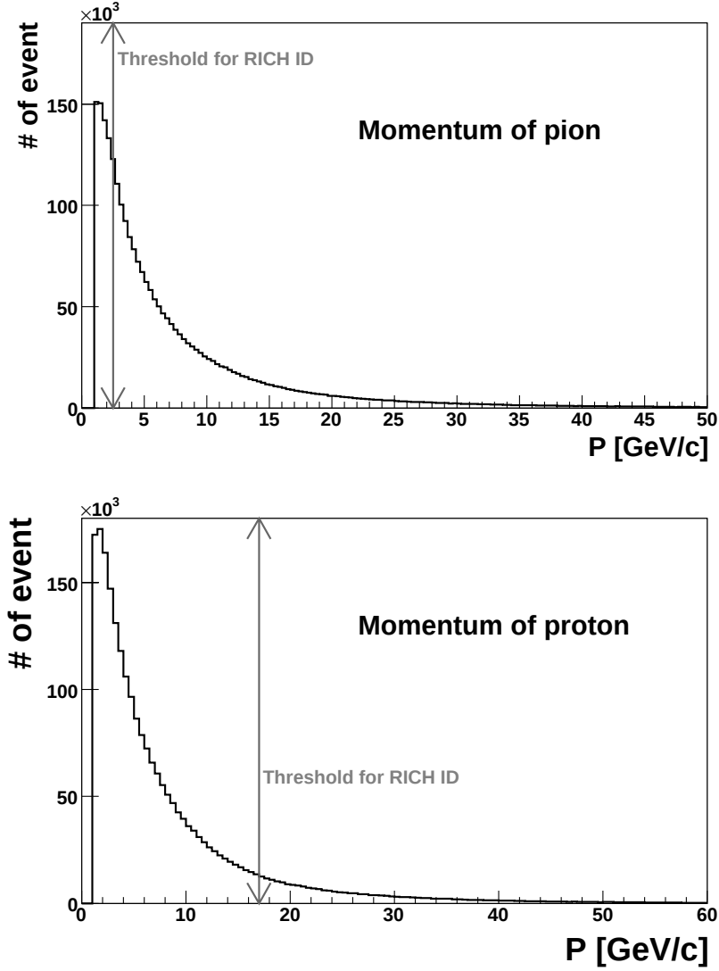
Figure 4.6: Top: Momentum distribution of the pions present in the \Lambda signal. Bottom: Momentum distribution for protons which contribute to the \Lambda signal. The grey arrows indicate the thresholds for pion and proton identification by the RICH. A significant amount of data were cut-off if RICH particle identification was implemented in this analysis.
