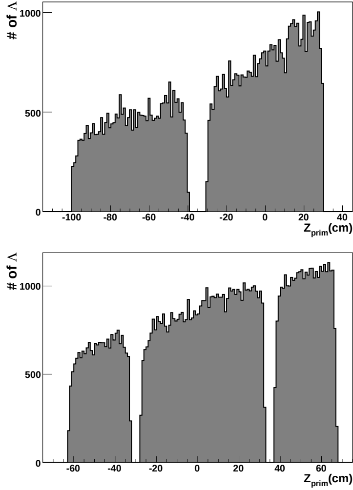
Figure 3.7: Distribution of reconstructed vertex position within the target cells along the beam axis. During the data taking of 2002-2004, two target cells were used (top), while in the 2007 data taking three target cells were implemented (bottom) in a modified position along the z-axis with respect to the 2002-2004 setting.
