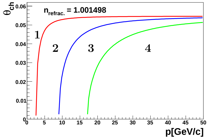
Figure 4.5: Calculated Cherenkov angle \theta_{ch} versus momentum p : Momentum thresholds are shown for the detection of three different particles \pi (in red), K (in blue) and p (in green) at a refractive index n=1.001498 . Four different regions (1, 2, 3 and 4) are defined by those thresholds of momenta [66].
