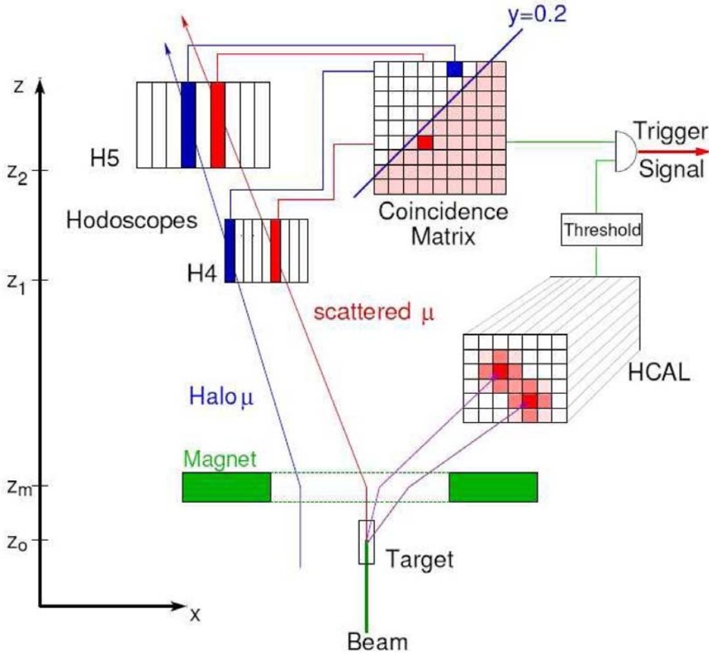
Figure 3.10: Basic scheme of the trigger decision. The scattered muon leads to a coincidence in the activated area of the coincidence matrix while the halo muon fails to do so because its tracks do not point back to the target. In addition, a minimum hadron energy can be required in the calorimeter [72].
