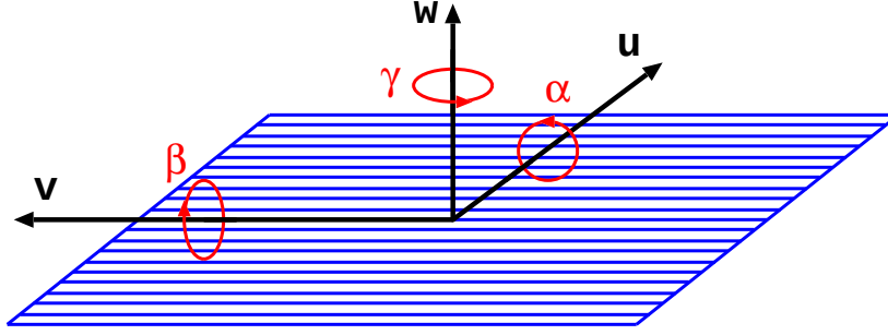
Figure 3.6: Example of the local coordinate system defined for each module considered in alignment of the tracker [206]. The u and v axes are defined in the plane of the module where u points along the more precisely measured axis of the module. The w axis is normal to the plane of the module. Three angles \alpha , \beta , and \gamma denote rotation angles about the respective u , v , and w axes.
