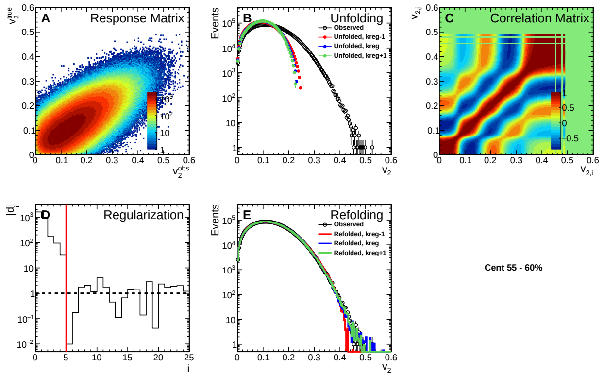
Figure C.24: p(v_2) SVD unfolding performance plots for events in the 55–60% centrality bin.
