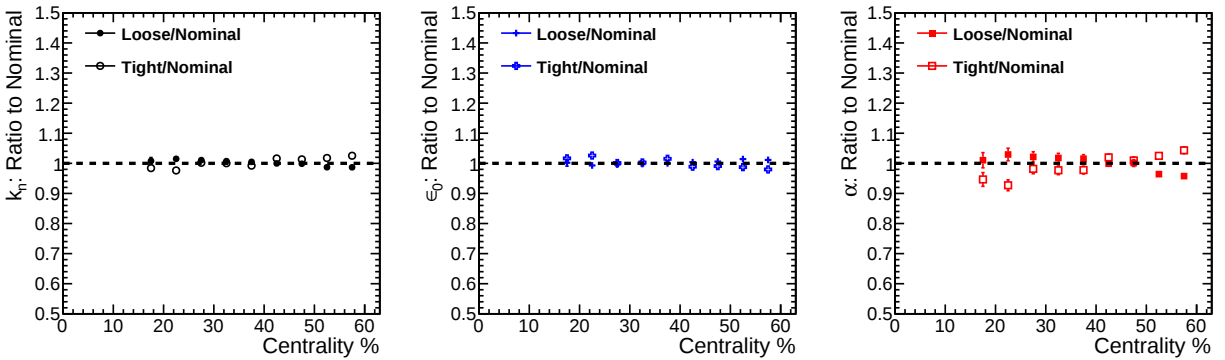
Figure 6.15: Biases on the parameters extracted from elliptic power law fits to the p(v_2) distributions for loose and tight track selections relative to the default track selection.
