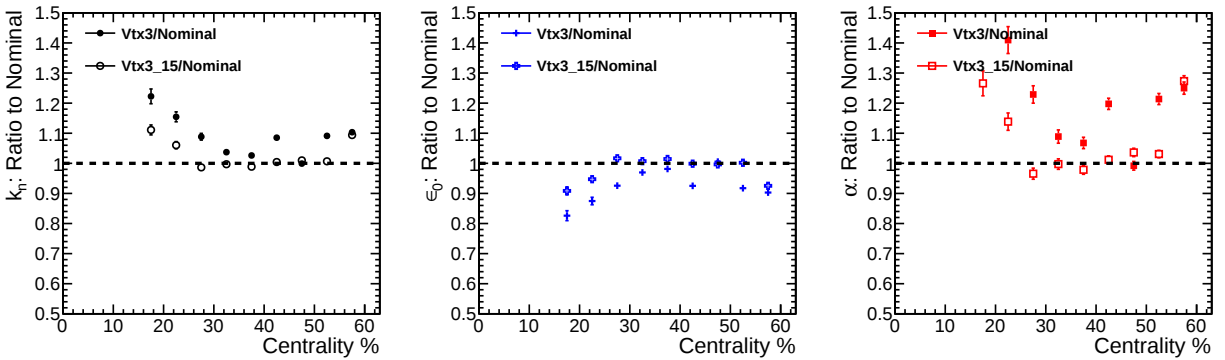
Figure 6.4: Biases on the parameters extracted from elliptic power law fits to the p(v_2) distributions for vertex selection windows relative to the default window |v_z| < 15.0 cm.
