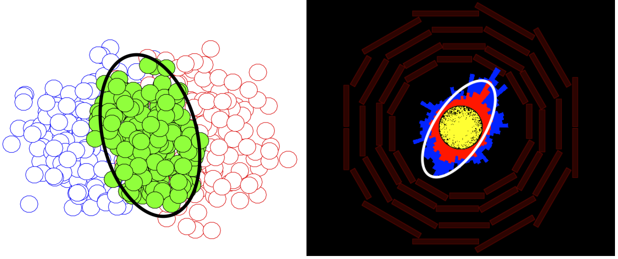
Figure 1.1: (Left) A Glauber simulation [88, 89, 90] of a PbPb collision at \sqrt{s_{NN}} = 5.02 TeV with a strong elliptic shape. A solid black line illustrates the dominant second-order term in the Fourier expansion. (Right) A CMS event display of a PbPb collision at \sqrt{s_{NN}} = 5.02 TeV with a strong elliptic shape in the final-state azimuthal particle density. A white line illustrated the dominant second-order term in the Fourier expansion.
