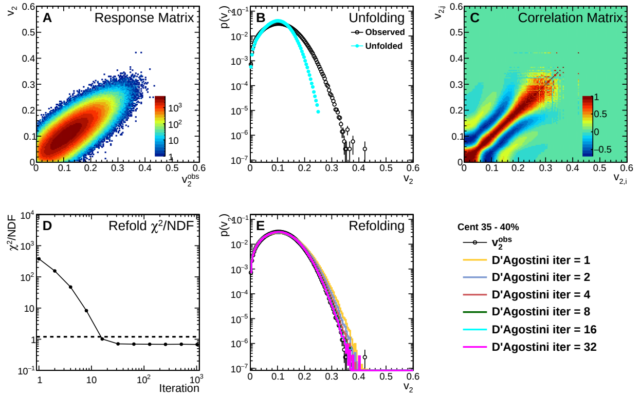
Figure C.8: p(v_2) D'Agostini unfolding performance plots for events in the 35–40% centrality bin.
