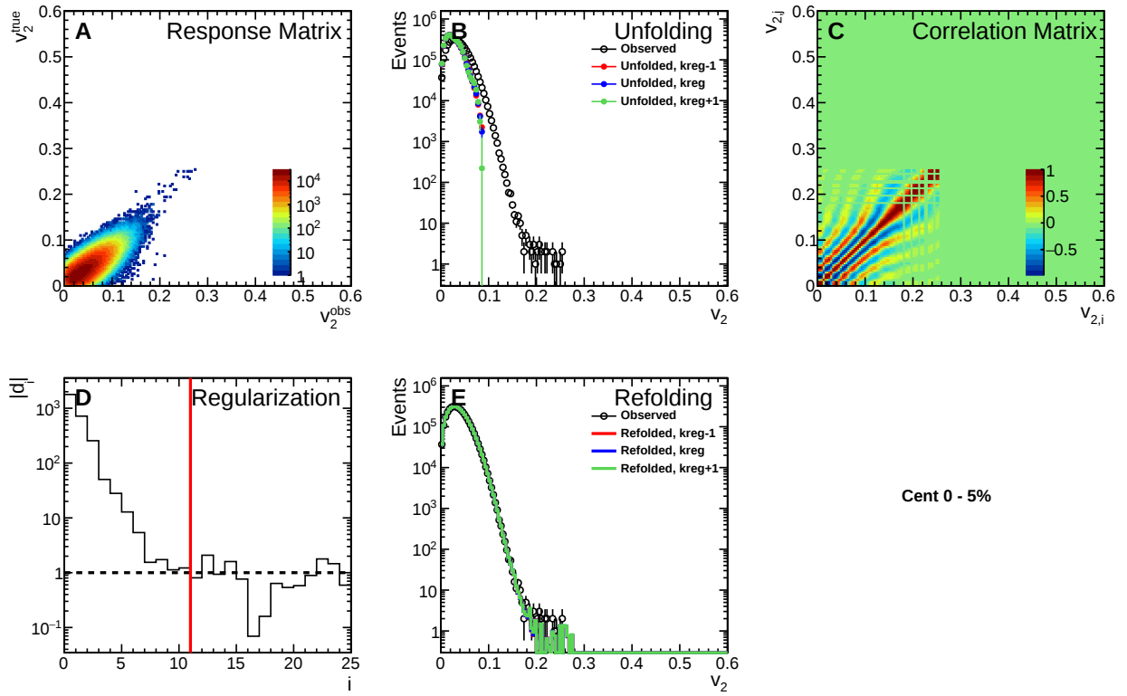
Figure C.13: p(v_2) SVD unfolding performance plots for events in the 0–5% centrality bin.
