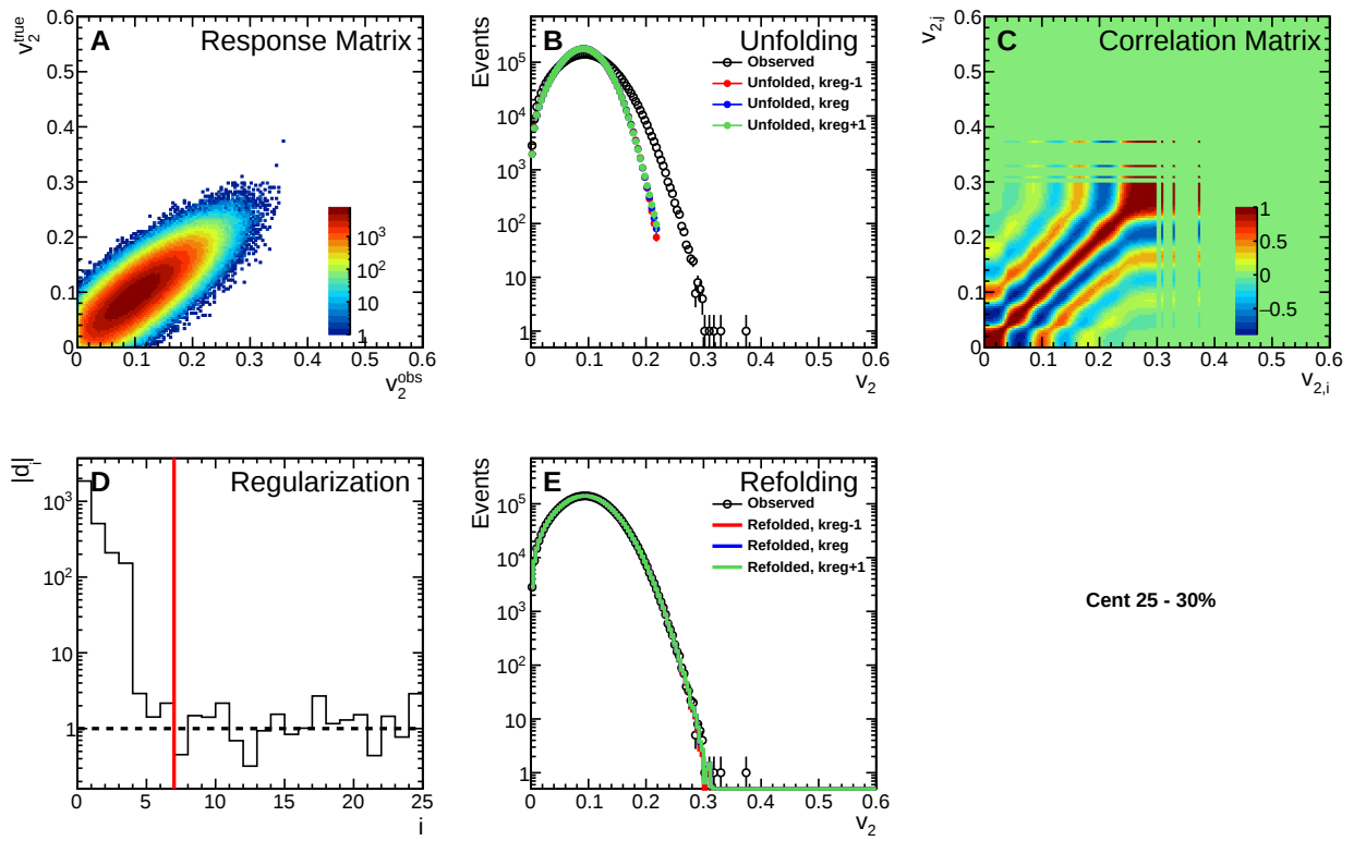
Figure C.18: p(v_2) SVD unfolding performance plots for events in the 25–30% centrality bin.
