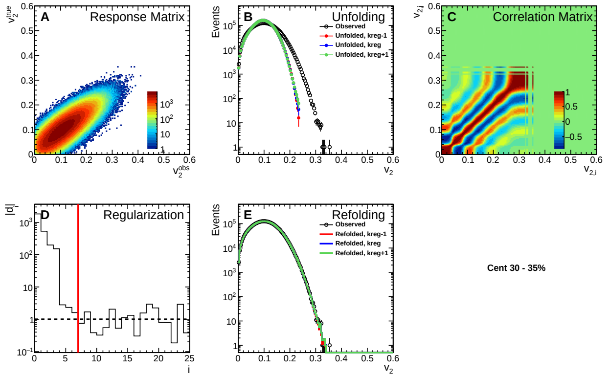
Figure C.19: p(v_2) SVD unfolding performance plots for events in the 30–35% centrality bin.
