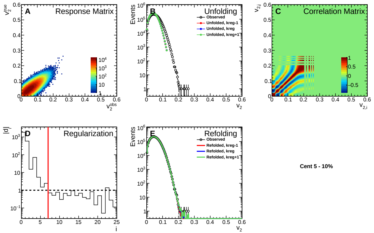
Figure C.14: p(v_2) SVD unfolding performance plots for events in the 5–10% centrality bin.
