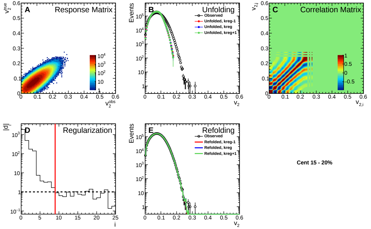
Figure C.16: p(v_2) SVD unfolding performance plots for events in the 15–20% centrality bin.
