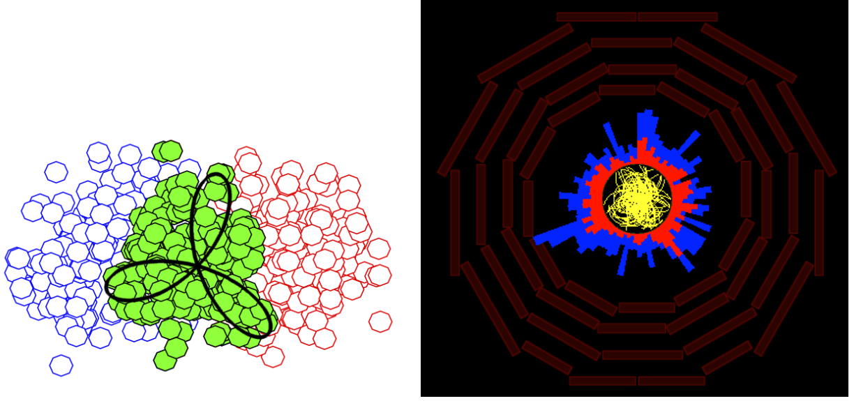
Figure 2.1: (Left) A Glauber simulation of a PbPb collisions with a strong \epsilon_3 signal. A solid black line illustrates the \cos 3\phi triangular term in the Fourier decomposition. (Right) A CMS event display of a PbPb collision with a strong v_3 signal.
