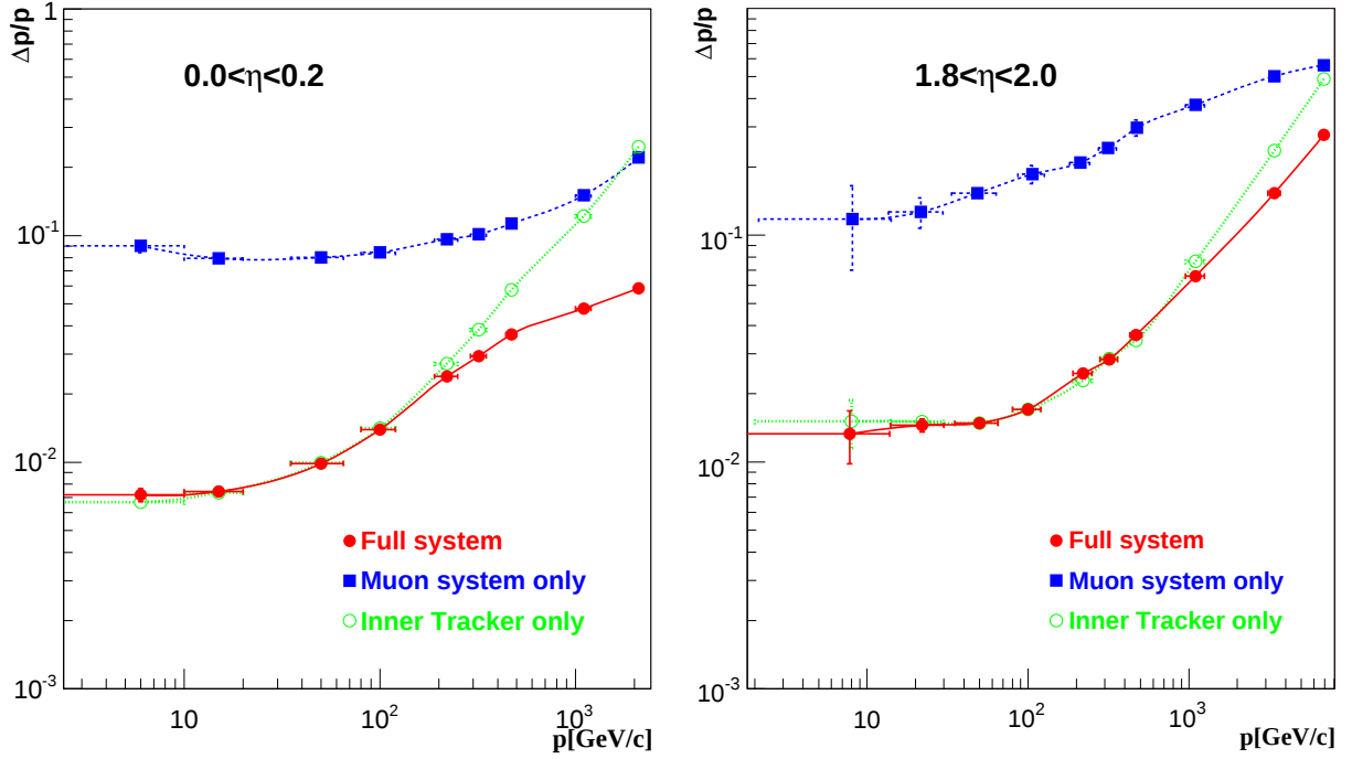
Figure 3.16: Momentum resolution for muons measured using the silicon tracker only, the muon systems only, and the combination of both systems. The left panel shows the resolution for centrally produced muons while the right panel shows the resolution for forward muons. Figure taken from Ref. [211].
