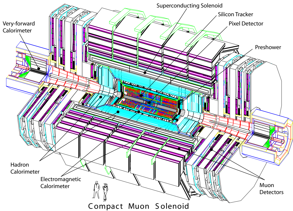
Figure 3.2: A full-scale view of the CMS detector and its subsystems. The ZDCs and CASTOR calorimeters are not shown in this figure. Figure taken from Ref. [199].
