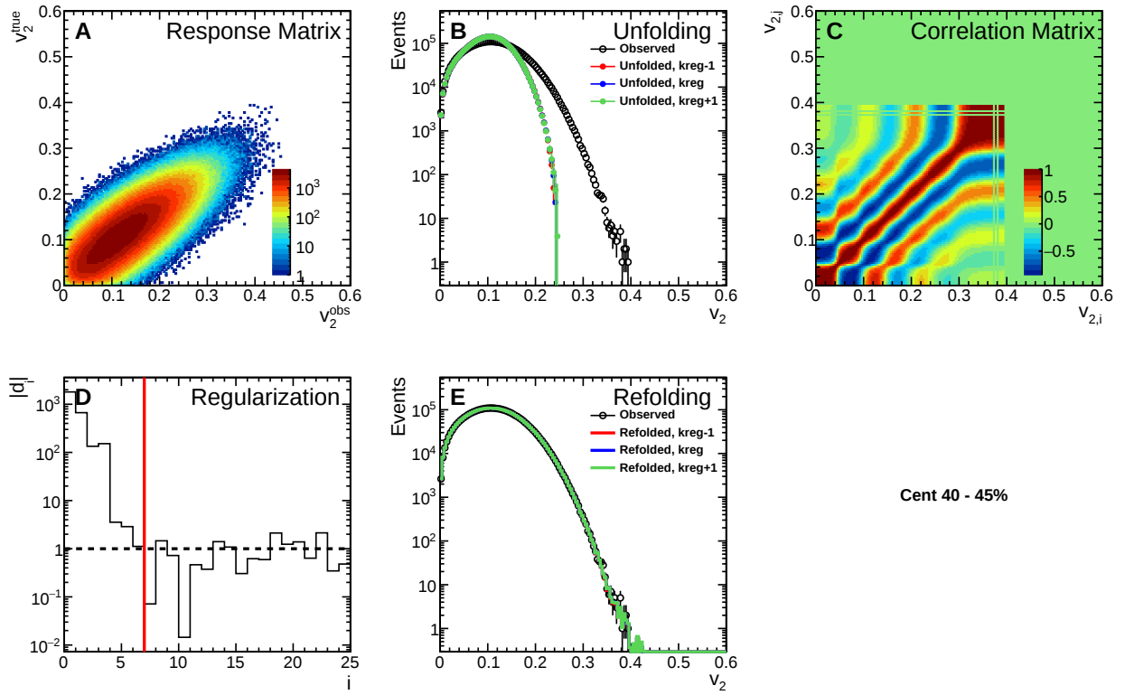
Figure C.21: p(v_2) SVD unfolding performance plots for events in the 40–45% centrality bin.
