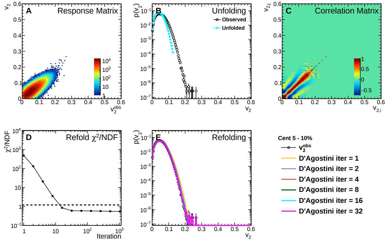
Figure C.2: p(v_2) D'Agostini unfolding performance plots for events in the 5–10% centrality bin.
