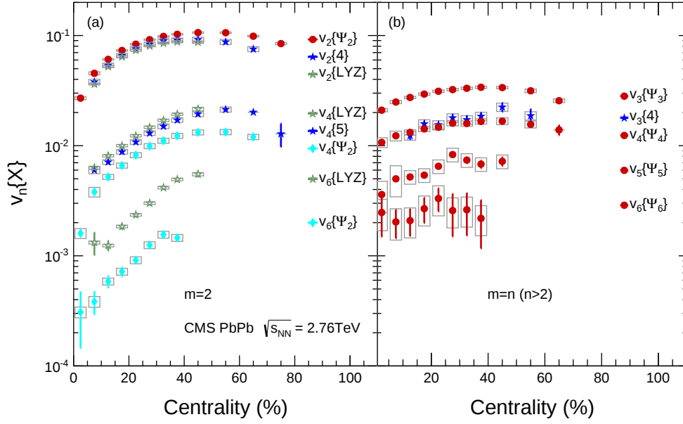
Figure 1.7: Yield-weighted v_n coefficient measurements by the CMS collaboration [53] for particles with 0.3 < p_T < 3.0 GeV/c and |\eta| < 0.8 in PbPb collisions at \sqrt{s_{NN}} = 2.76 TeV as a function of centrality. Measurements were obtained using event-plane correlations ( v_n\{\Psi_m\} ), m -particle correlations ( v_n\{m\} ), and LYZ ( v_n\{LYZ\} ).
