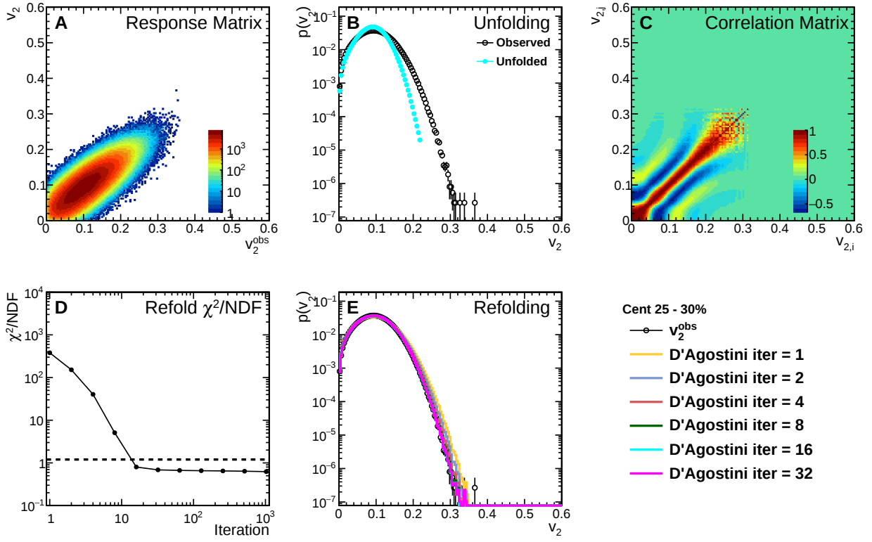
Figure C.6: p(v_2) D'Agostini unfolding performance plots for events in the 25–30% centrality bin.
