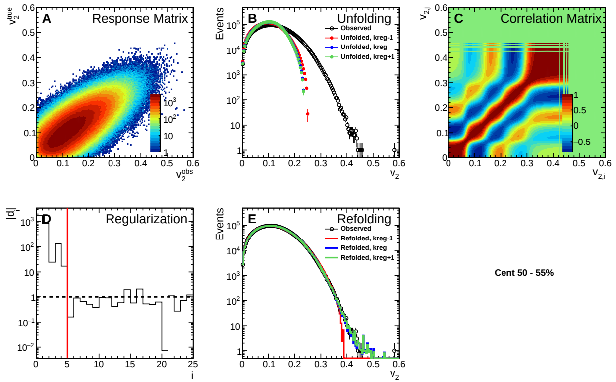
Figure C.23: p(v_2) SVD unfolding performance plots for events in the 50–55% centrality bin.
