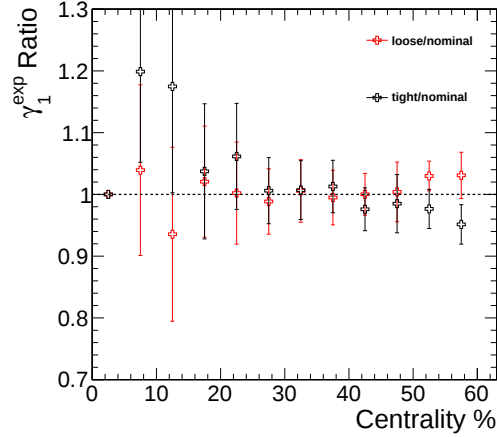
Figure 6.14: Biases on the skewness measure \gamma_1^{\text{exp}} of p(v_2) distributions for loose and tight track selections relative to the default track selection. Skewness is the least stable observable in this study.
