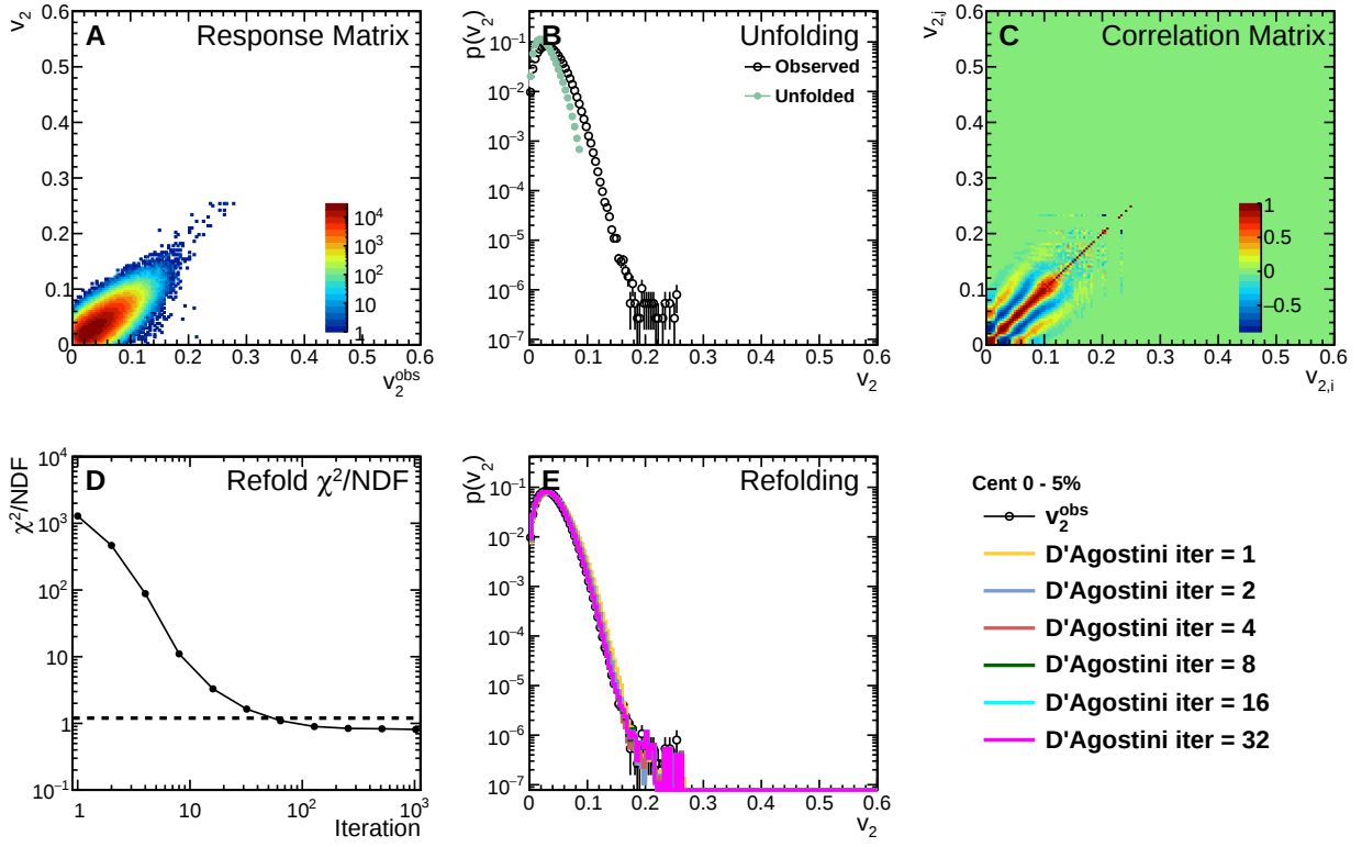
Figure C.1: p(v_2) D'Agostini unfolding performance plots for events in the 0–5% centrality bin.
