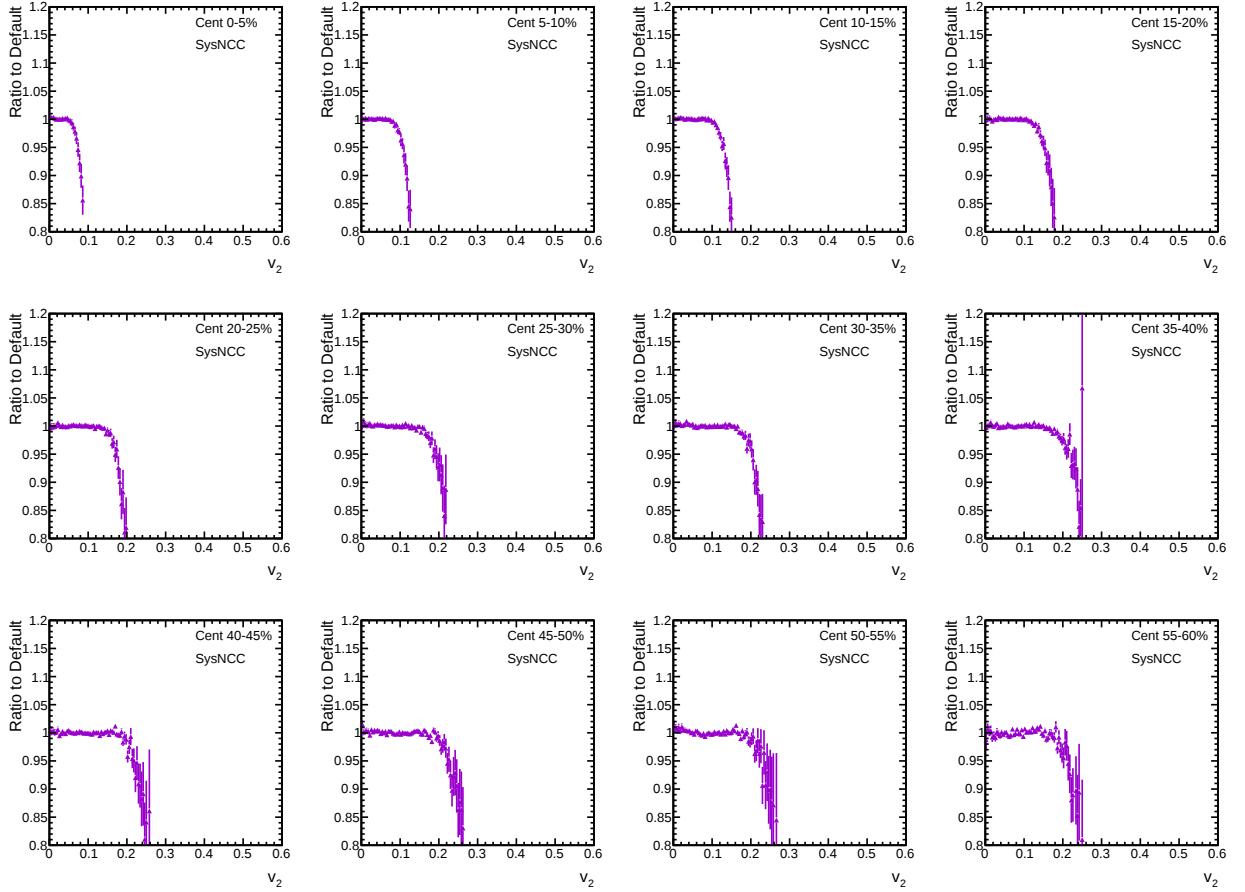
Figure 6.11: Systematic bias on the shape of p(v_2) distributions that arises from pileup events.
