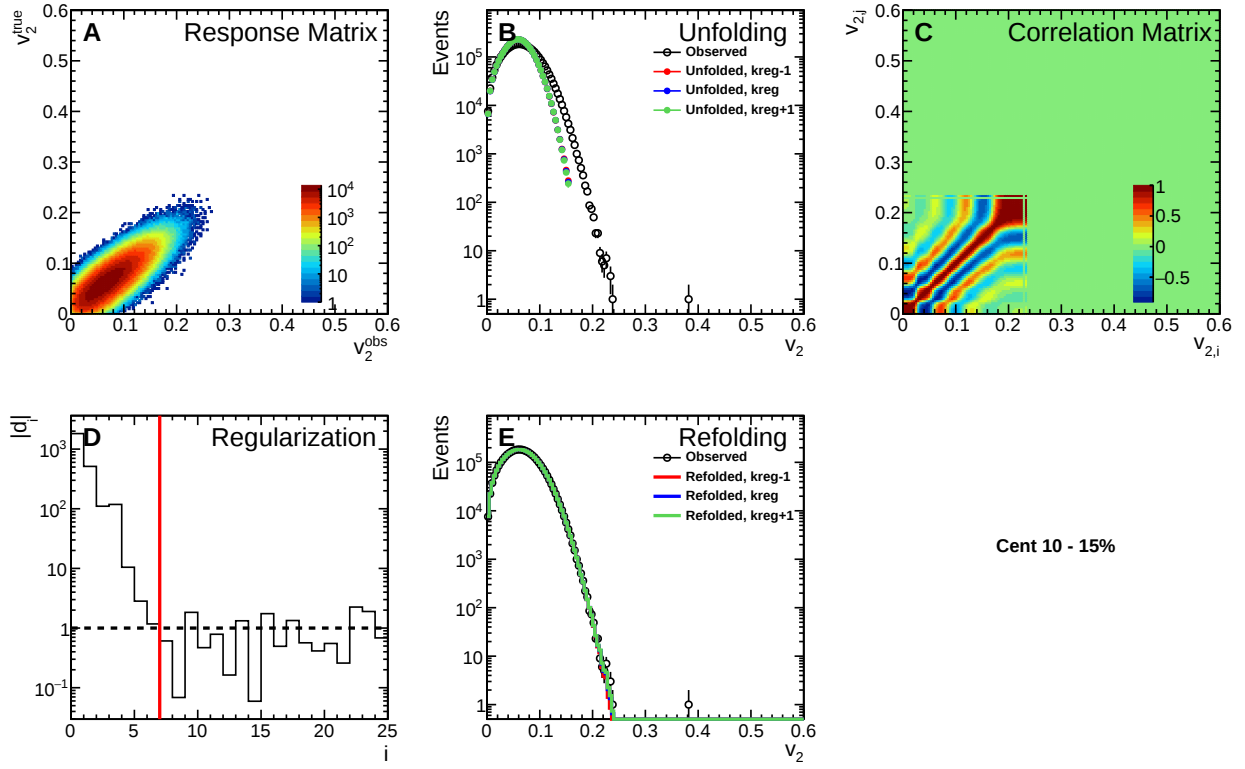
Figure C.15: p(v_2) SVD unfolding performance plots for events in the 10–15% centrality bin.
