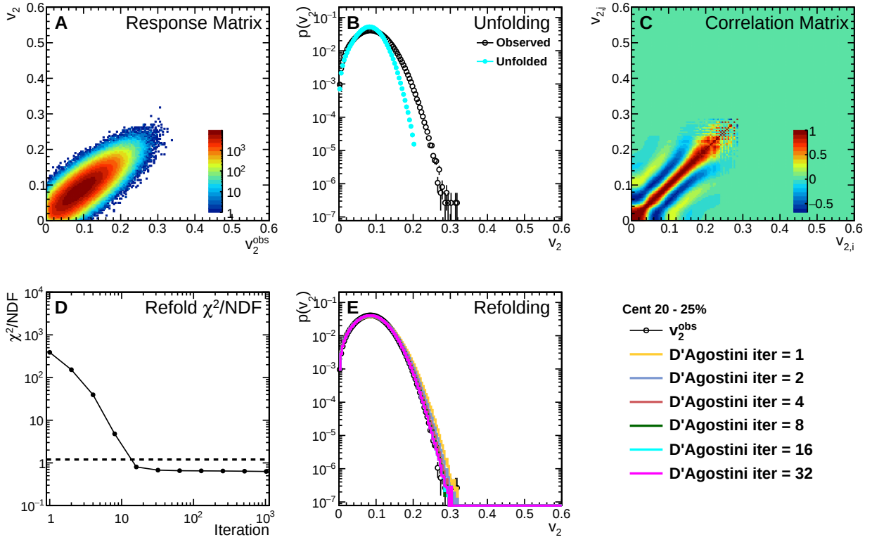
Figure C.5: p(v_2) D'Agostini unfolding performance plots for events in the 20–25% centrality bin.
