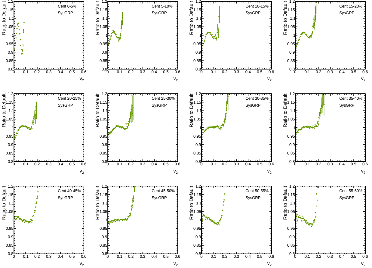
Figure 6.27: Systematic bias on the shape of p(v_2) distributions that arises from the choice in response matrix.
