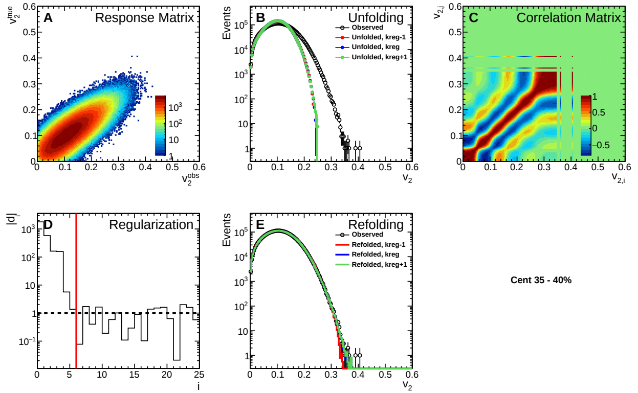
Figure C.20: p(v_2) SVD unfolding performance plots for events in the 35–40% centrality bin.
