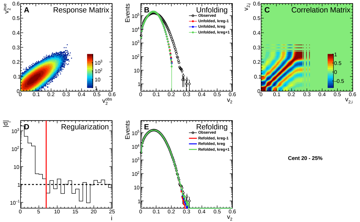
Figure C.17: p(v_2) SVD unfolding performance plots for events in the 20–25% centrality bin.
