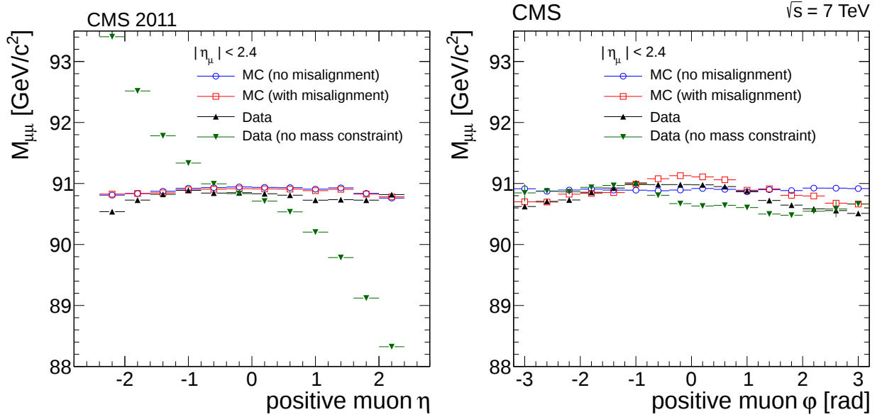
Figure 3.10: Example Z \rightarrow \mu^+ \mu^- validation from 2011 proton-proton operations [206]. The mass of the Z candidates is plotted as a function of the positive daughter muon's \eta and \phi for different alignment scenarios. In the ideal, aligned MC case, there is no strong bias as a function the kinematic variables, however when misalignments are introduced, biases arise in the mass distributions.
