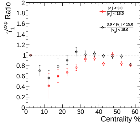
Figure 6.3: Biases on the skewness measure \gamma_1^{\text{exp}} of p(v_2) distributions for vertex selection windows relative to the default window |v_z| < 15.0 cm. Skewness is the least stable observable in this study.
