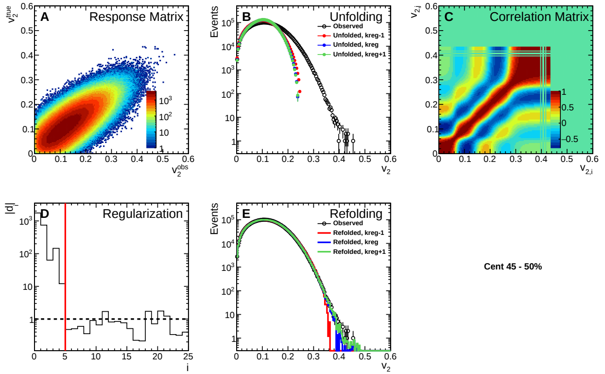
Figure C.22: p(v_2) SVD unfolding performance plots for events in the 45–50% centrality bin.
