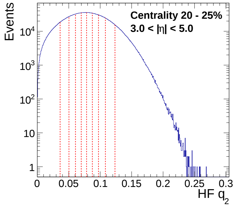
Figure 5.5: Second-order q -vectors as measured in the \text{HF}\pm detectors for mid-central PbPb collisions. Dotted lines denote the division into 10 areas of equal statistics and so-called ellipticity bins.
