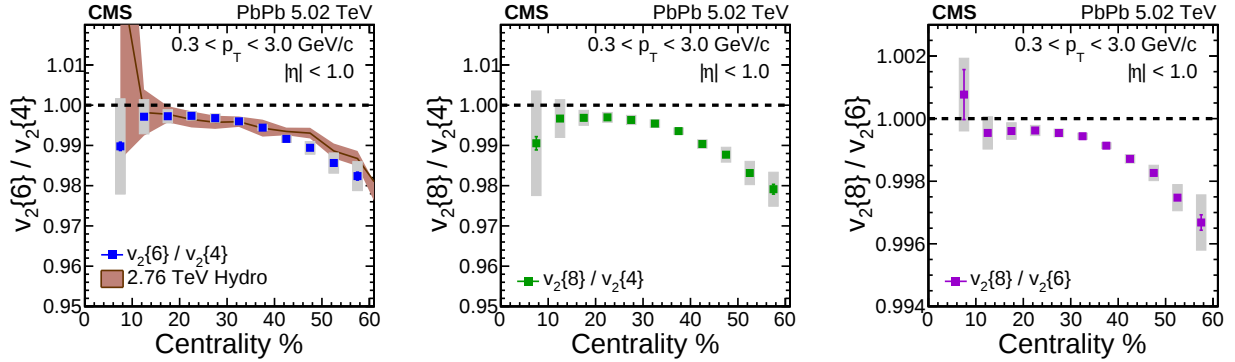
Figure 7.5: Ratios of higher-order cumulants with values obtained from the moments of the unfolded p(v_2) distributions. Both statistical and systematic uncertainties are shown. Hydrodynamic predictions for 2.76 TeV from Ref. [178] are presented as a colored band and are compared to the measured v_2\{6\}/v_2\{4\} ratio. Theory predictions are consistent to the measurement within uncertainties.
