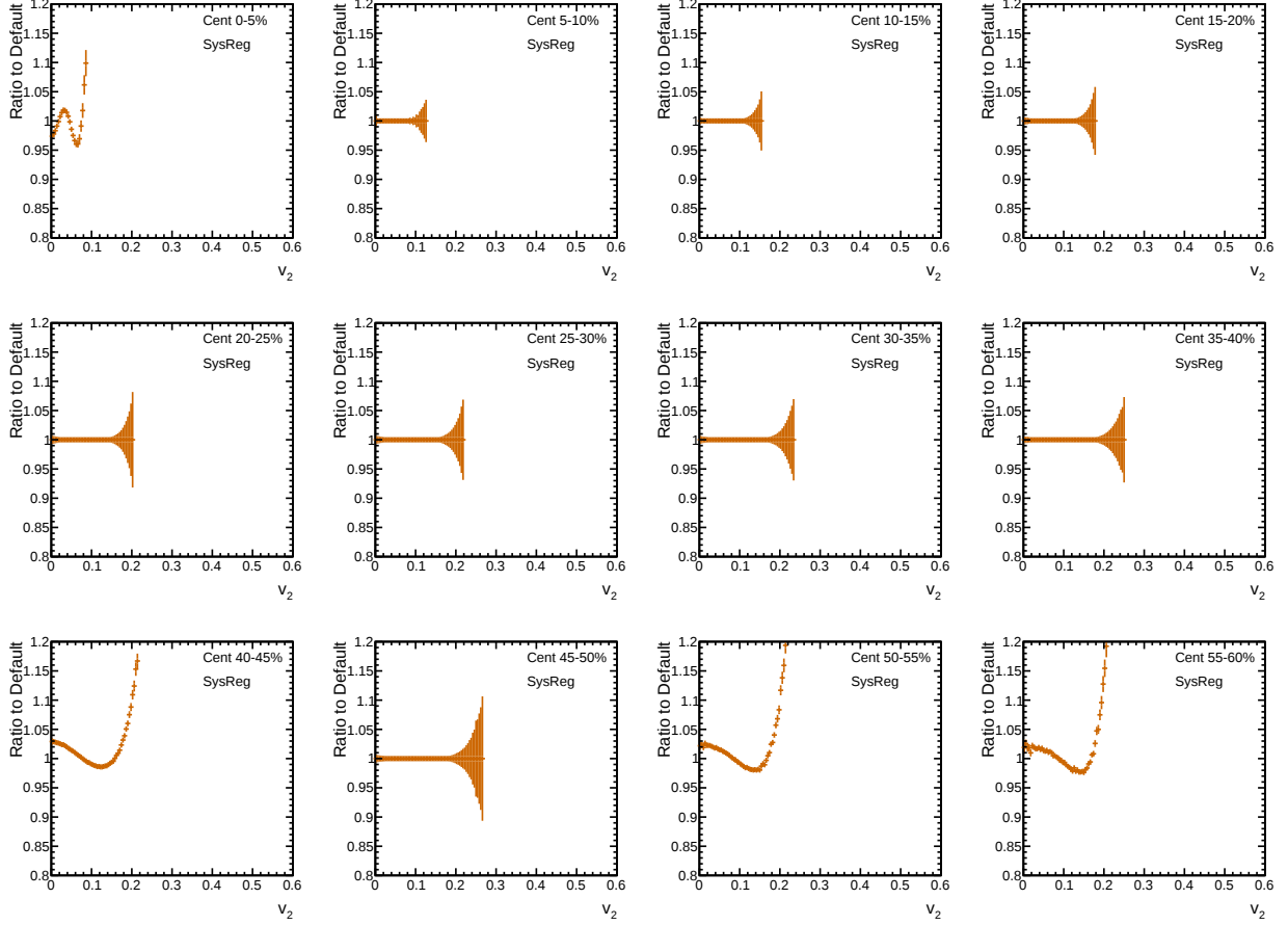
Figure 6.22: Systematic bias on the shape of p(v_2) distributions that arises from regularized unfolding.
