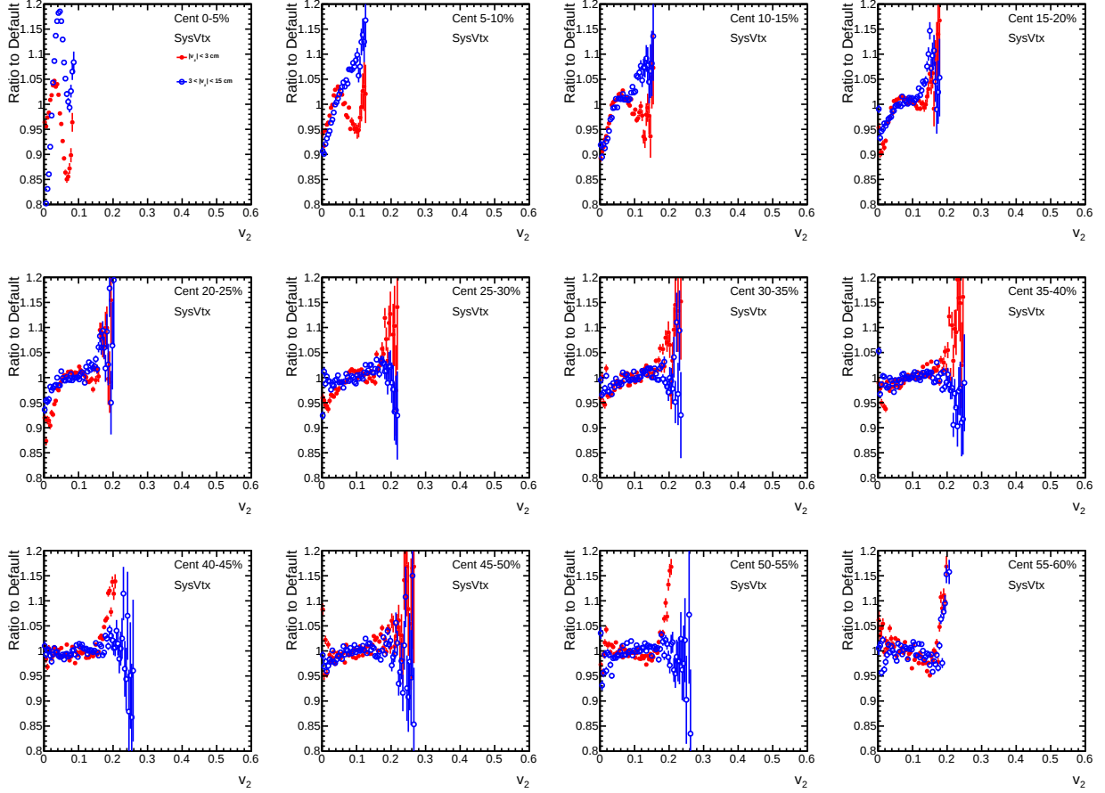
Figure 6.5: Systematic bias on the shape of p(v_2) distributions that arises from the vertex position cut.
