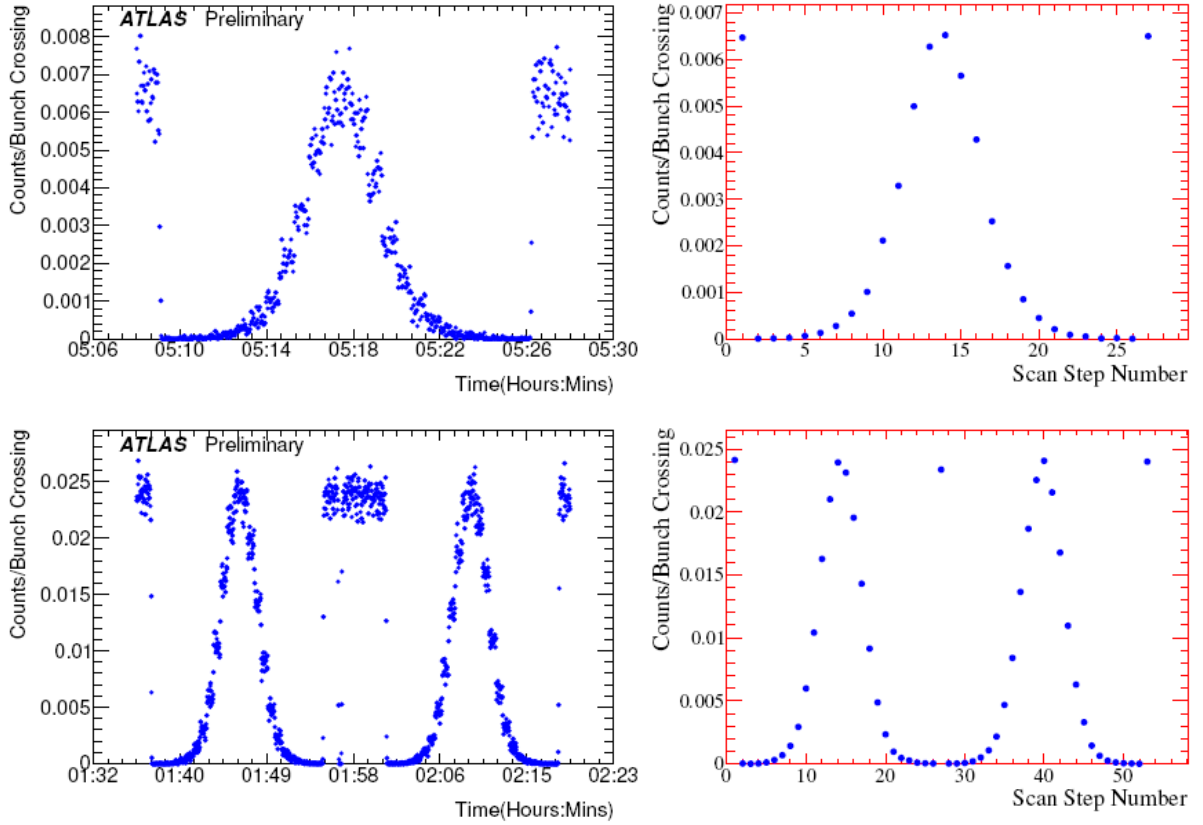
Figure 6.3: History of the raw luminosity, in units of events per bunch crossing, from the LUCID event AND algorithm during the full-fledged horizontal-calibration scan. Top: VdM-I scan (26 April 2010). Bottom: VdM-II and VdM-III scans (9 May 2010). Left: time-history of the sampled luminosity, irrespective of whether the transverse IP positions of the two beams were left in a quiescent state. Right: raw instantaneous luminosity average over the pseudo-luminosity blocks (or scan steps), where the IP positions were left unchanged. All steps are equal in duration. The points in steps 1 and 27 (top) and in steps 1, 28 and 54 (bottom) correspond to close-orbit bumps settings to zero nominal separation in both planes.
