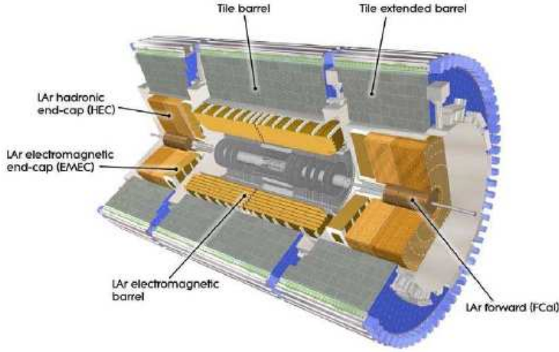
Figure 1.8: The ATLAS calorimetry system.
