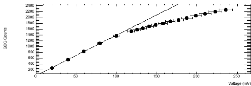
Figure 4.17: Charge transfer function for tube 29 as measured by QDC.
