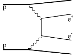
Figure 2.3: Feynmann diagram for the two-photon pp \rightarrow pp\ell\ell process.
