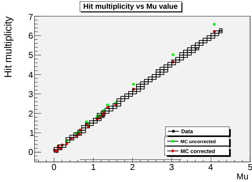
Figure 4.15: Dependency of the hit multiplicity on the mean number of interactions per bunch crossing ( \mu ) in real data (black boxes) and Monte Carlo predictions before (green points) and after (red points) the Monte Carlo adjustment.
