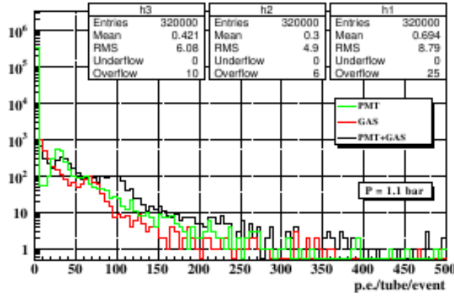
Figure 4.6: Average number of expected photoelectrons produced by Cherenkov effect, when a charged pion travels along a random trajectory inside the tube, for a single tube.
