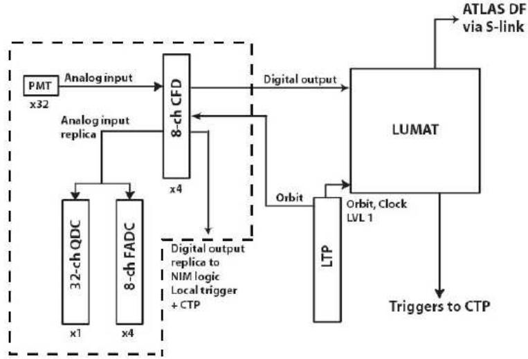
Figure 3.6: General schema of LUCID electronics.
