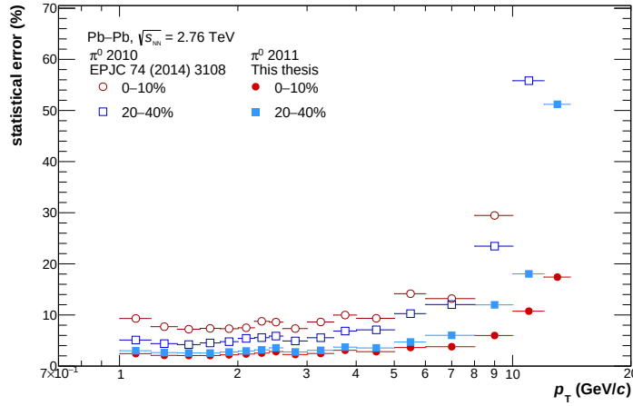
FIGURE 6.2: Percentage of the differential invariant yield statistical errors for the \pi^0 meson in 0–10% (round markers) and 20–40% (square markers) Pb–Pb collisions at \sqrt{s_{NN}} = 2.76 TeV. Open markers represent the 2010 measurement [90], full markers the results of this thesis.
