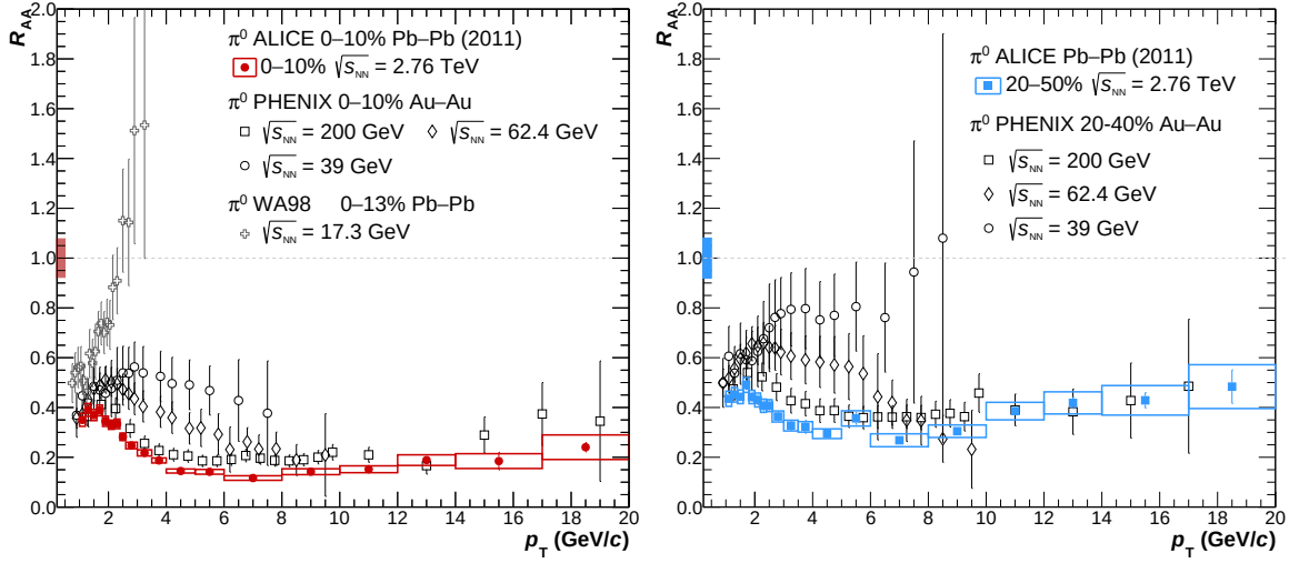
FIGURE D.15: R_{AA} of the combined \pi^0 meson measurement in Pb-Pb collisions at \sqrt{s_{NN}} for the 010% (left) and 20–50% (right) centrality classes is compared to results from experiments at lower energies: from Au–Au collisions at \sqrt{s_{NN}} = 39, 62.4 [91], and 200 GeV [92] at RHIC and, for 0–10% only, the result from the CERN SPS [93] are shown.
