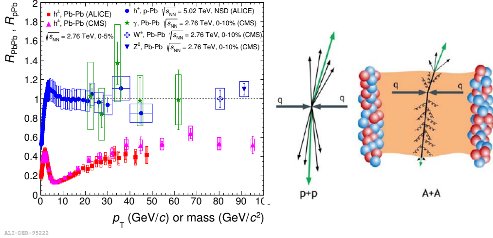
FIGURE 1.10: Left: ALICE charged hadron nuclear modification factor R_{AA} measurements in Pb–Pb [82] and p–Pb [87] collisions at centre-of-mass energy \sqrt{s_{NN}} = 2.76 TeV and 5.02 TeV, respectively, are compared with the same measurement from the CMS experiment [83]. Also shown, the measurements for \gamma , W^\pm and Z^0 bosons production at \sqrt{s_{NN}} = 2.76 TeV from the CMS experiment [84–86]. Right: Jet quenching. Contrary to what happens in pp collisions, the particle jet that has to traverse a strongly interacting medium in the aftermath of a nucleus-nucleus collision suffers significant energy loss [88].
