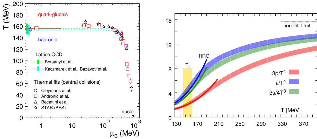
FIGURE 1.4: Left: QCD phase diagram showing the results of thermal fits to hadron yields for several centre-of-mass energies. The dashed lines indicate the temperature at the cross-over, calculated with LQCD [29]. Compared to the given reference, the points from the STAR experiment and from Becattini et al. have been updated here with recent results, as in [31] and [32], respectively. Right: Pressure, energy density and entropy as a function of the temperature T for the highly improved staggered quark (HISQ) action [33]. The critical temperature T_c is indicated with the shaded area. The solid lines indicate the results obtained with the HRG calculations, while the dashed line in the top right corner represents the results for an ideal non-interacting gas of quarks and gluons. For more details see text and reference [20].
