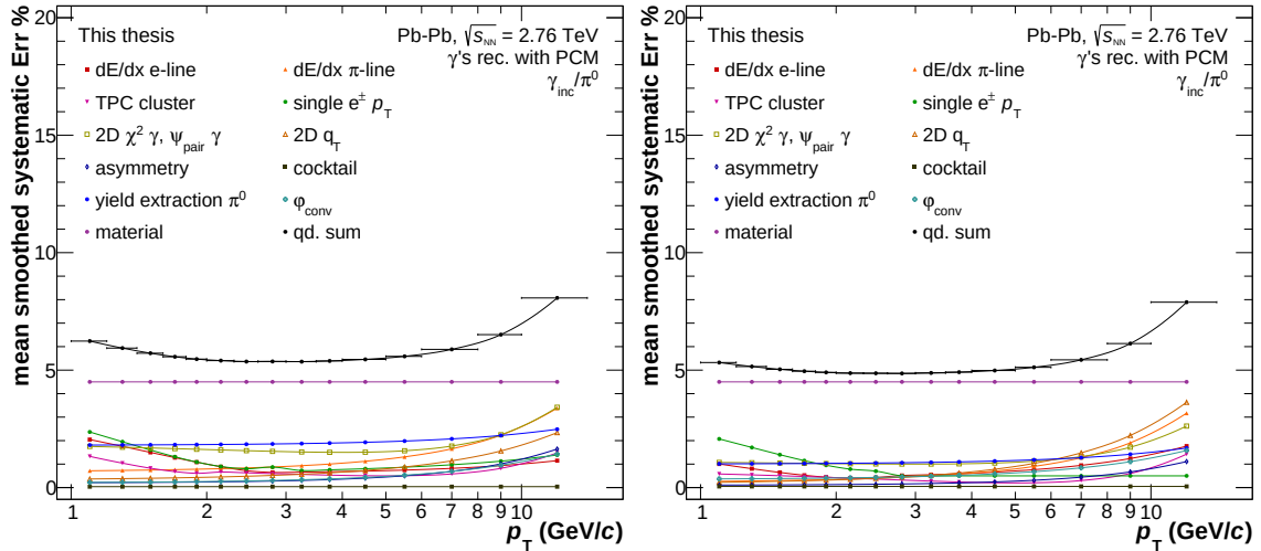
FIGURE 9.5: Systematic uncertainties of the \gamma_{\text{incl}}/\pi^0 ratio in Pb–Pb collisions at \sqrt{s_{\text{NN}}} = 2.76 TeV in the centrality classes 0–10% (left) and 20–40% (right).
