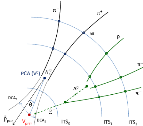
FIGURE 4.4: Schematic representation of a secondary vertex, with example decays from K_S^0 and \Xi^- particles [169]. The angle indicated with \theta is the angle between the vector connecting the primary to the secondary vertex and the V^0 particle momentum, called pointing angle.
