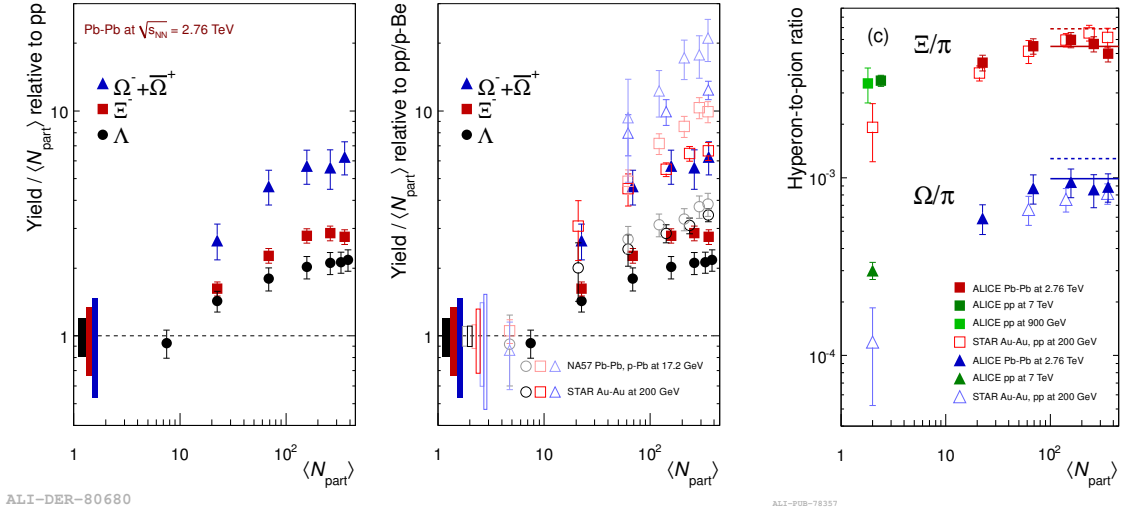
FIGURE 1.19: Enhancement the \Lambda , \Xi and \Omega baryons as a function of the mean number of participant nucleons, \langle N_{\text{part}} \rangle , measured in Pb-Pb collisions at \sqrt{s_{\text{NN}}} = 2.76 TeV with ALICE, full symbols, left panel. These results are compared with what has been measured in Au-Au collisions at 200 GeV with STAR and in Pb-Pb and p-Pb collisions at 17.2 GeV with NA37, both with open symbols, middle panel. The boxes at unity represent the statistical and systematic uncertainty in the pp baseline. Right panel: Hyperon to pion ratios as a function of \langle N_{\text{part}} \rangle , measured in pp and A-A collisions with ALICE and STAR [124]. The solid and dashed lines indicate the thermal model calculations by Andronic et al. [29] and THERMUS [78] with T = 164 MeV and T = 170 MeV chemical freeze-out temperature.
