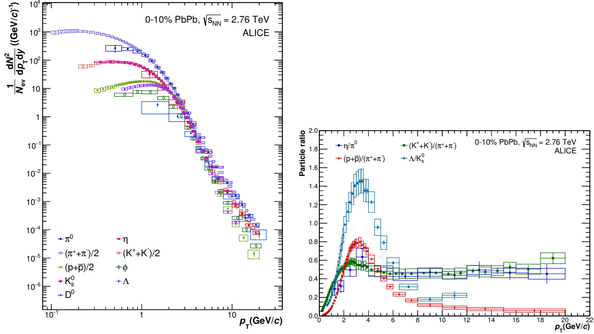
FIGURE 7.1: Collection of the available measurements for the production of the cocktail simulation input parametrisations in the centrality class 0–10% [90, 204, 238, 239].
