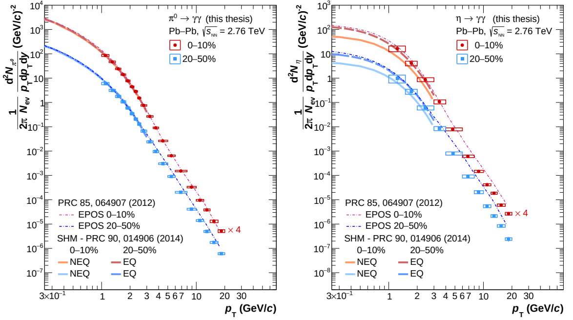
FIGURE 6.14: Combined PCM and ECal differential invariant yields for the \pi^0 (left) and \eta (right) meson for the centrality classes 0–10% and 20–50% in Pb–Pb collisions at \sqrt{s_{NN}} = 2.76 TeV compared to the EQ SHM [218], NEQ SHM [217] and EPOS2 [219] predictions for the respective centralities.
