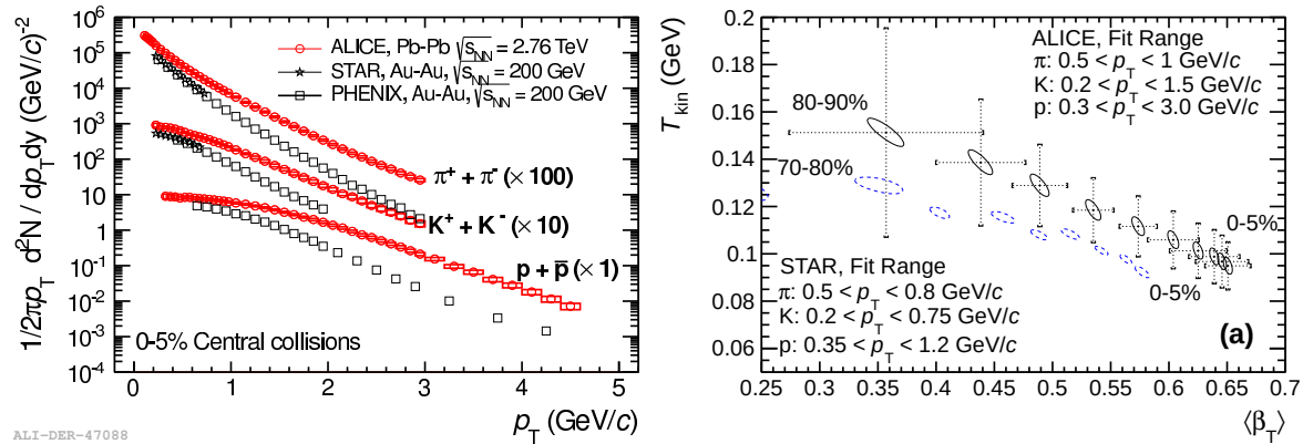
FIGURE 1.13: Left: ALICE particle spectra measured in 0-5% Pb-Pb collisions at \sqrt{s_{\text{NN}}} = 2.76 TeV, compared to RHIC results from Au-Au collisions at 200 GeV in the same centrality class [53, 100]. The boxes represent the systematic uncertainties while the statistical uncertainties are smaller than the symbol size. Right: Kinetic freeze-out temperature T_{\text{kin}} as a function of the mean transverse velocity ( \langle \beta_T \rangle = \langle \beta_r \rangle ), for different centrality intervals, obtained from Blast-Wave fits to ALICE measurements of pion, kaon and proton transverse momentum spectra [97], compared to results from STAR [98]. The ALICE uncertainties (solid contours) include bin-by-bin systematic uncertainties, while the dashed error bars represents the full systematic uncertainty. For STAR, only statistical uncertainties are shown (dashed contours).
