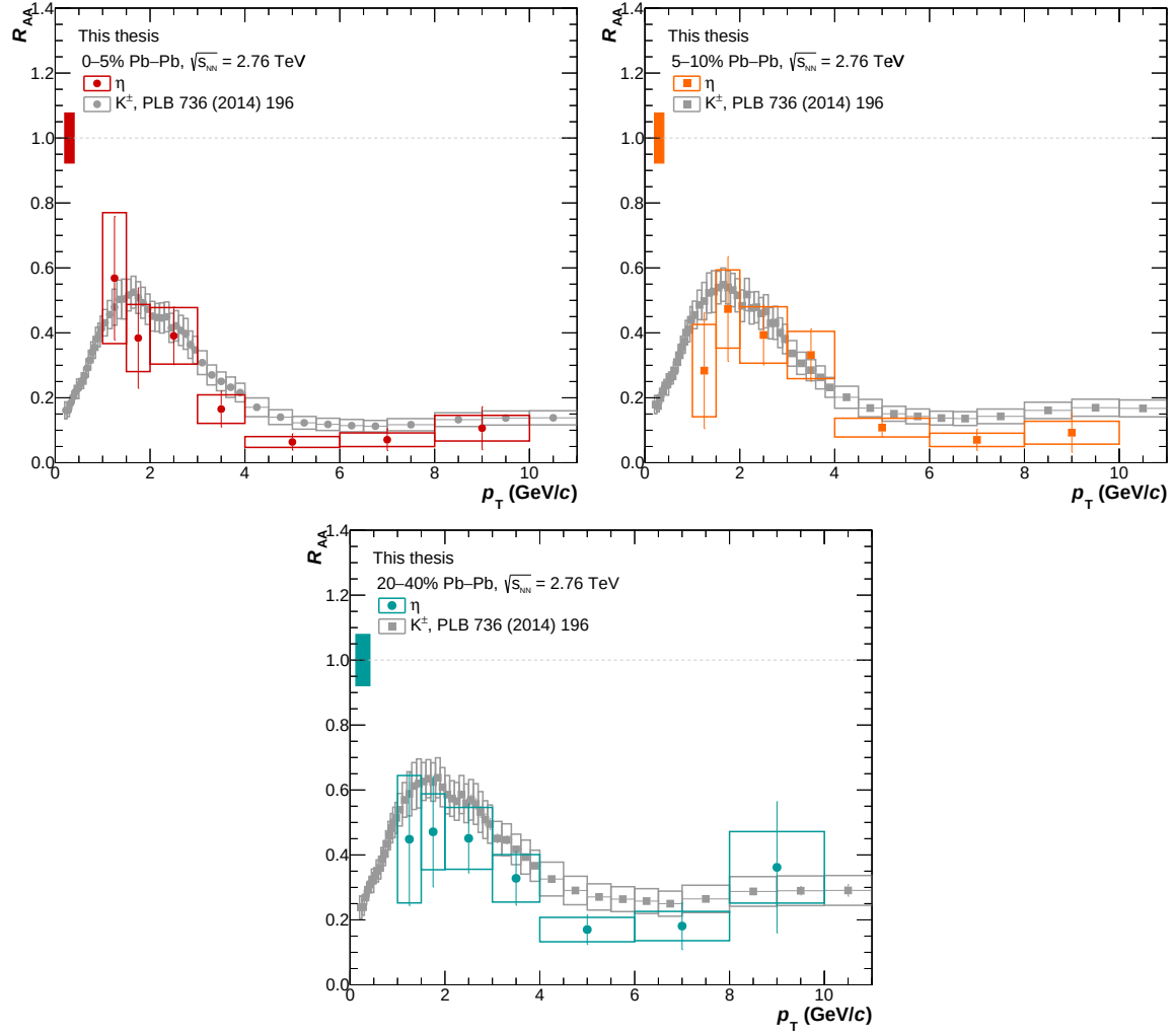
FIGURE C.16: Nuclear modification factor for the \eta meson in the centrality classes 0–5% (top left), 5–10% (top right) and 20–40% (bottom), compared to the charged kaon R_{AA} , in the same centrality classes, measured in Pb–Pb collisions at \sqrt{s_{NN}} = 2.76 TeV [204].
