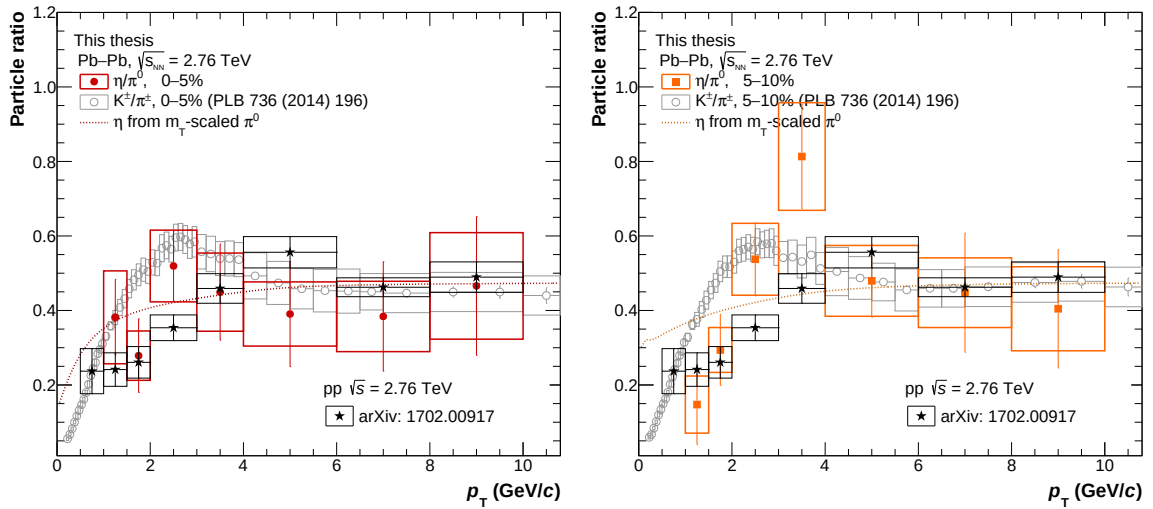
FIGURE C.11: Ratio of the \eta to \pi^0 meson for the centrality classes 0–5% and 5–10% in Pb–Pb collisions at \sqrt{s_{NN}} = 2.76 TeV. The ratio is compared to the same measurement in pp collisions at \sqrt{s} = 2.76 TeV [206] and to the K^\pm/\pi^\pm ratio, at the same centrality and centre-of-mass energy. The dashed lines represent the ratio obtained using the \eta obtained via m_T -scaling from the \pi^0 meson.
