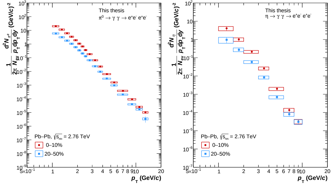
FIGURE 6.1: Differential invariant yields for the \pi^0 (left) and \eta (right) meson for the centrality classes 0–10% (red) and 20–50% (azure) in Pb–Pb collisions at \sqrt{s_{NN}} = 2.76 TeV measured with the PCM. The statistical uncertainties are represented by the vertical bars, the systematic uncertainties by the boxes.
