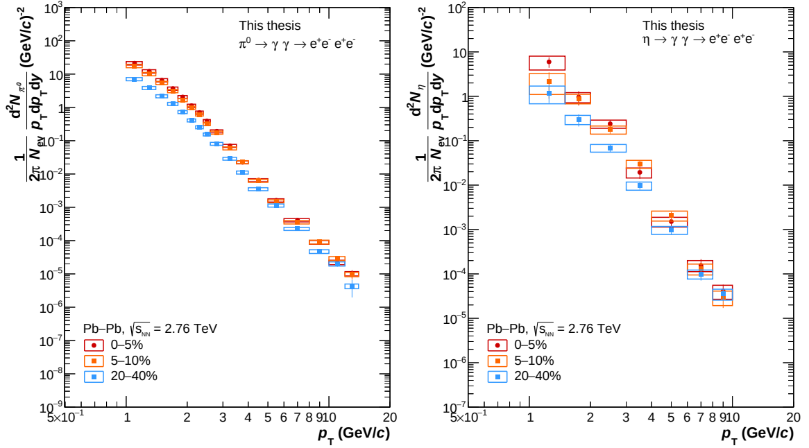
FIGURE C.10: Differential invariant yields for the \pi^0 (left) and \eta (right) meson for the centrality classes 0–5%, 5–10% and 20–40% in Pb–Pb collisions at \sqrt{s_{NN}} = 2.76 TeV measured with the PCM. The statistical errors are represented by the vertical bars, the systematic errors by the boxes.
