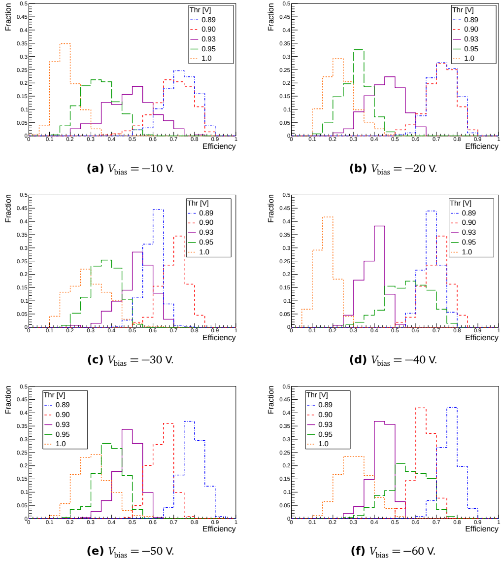
Figure A.6: Hit efficiency distributions for different external threshold voltages for sensor bias voltages between -10 V and -60 V. Only subpixel type 1 is enabled.
