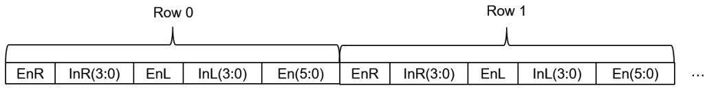
Figure 6.5: Schematic drawing of the sequence of the pixel shift register for two unit cell rows.
