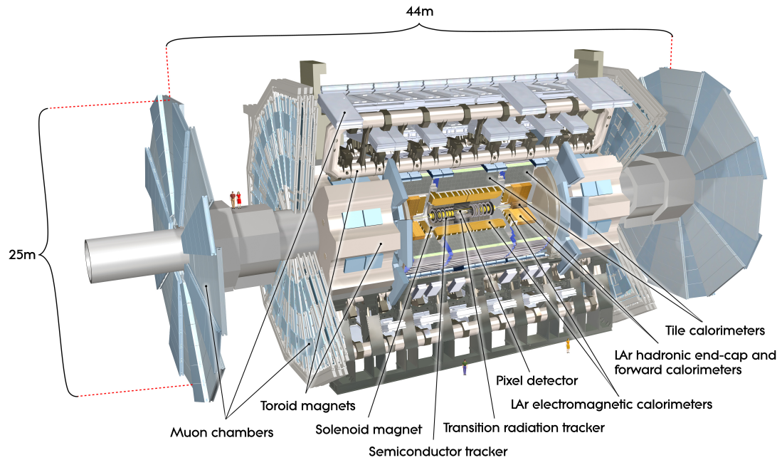
Figure 4.1: A schematic of the ATLAS detector with important detector elements labeled [15].
