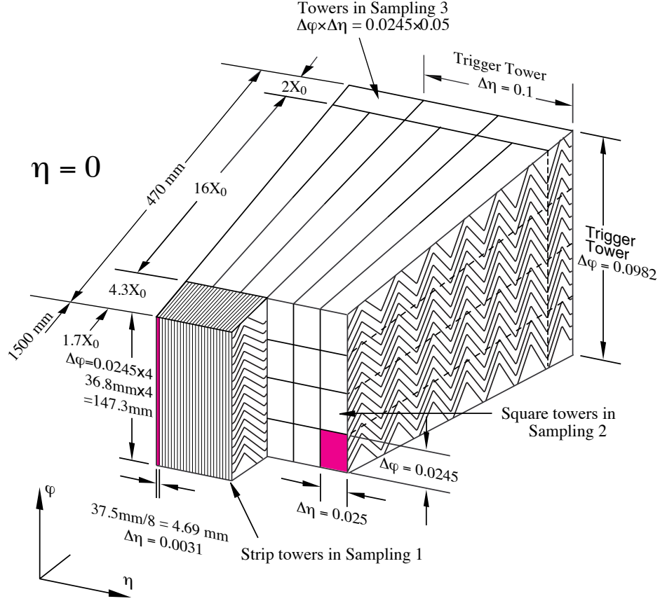
Figure 4.9: A schematic of the LAr barrel accordion geometry. Different layers are delineated and the granularity of the cells in \eta and \phi is shown. [16].
