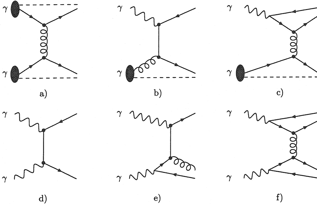
FIG. 6.12 – Types d'interactions \gamma\gamma [13]: a) VMD \times VMD, b) VMD \times direct, c) VMD \times anormal, d) direct \times direct, e) direct \times anormal, and f) anormal \times anormal.
