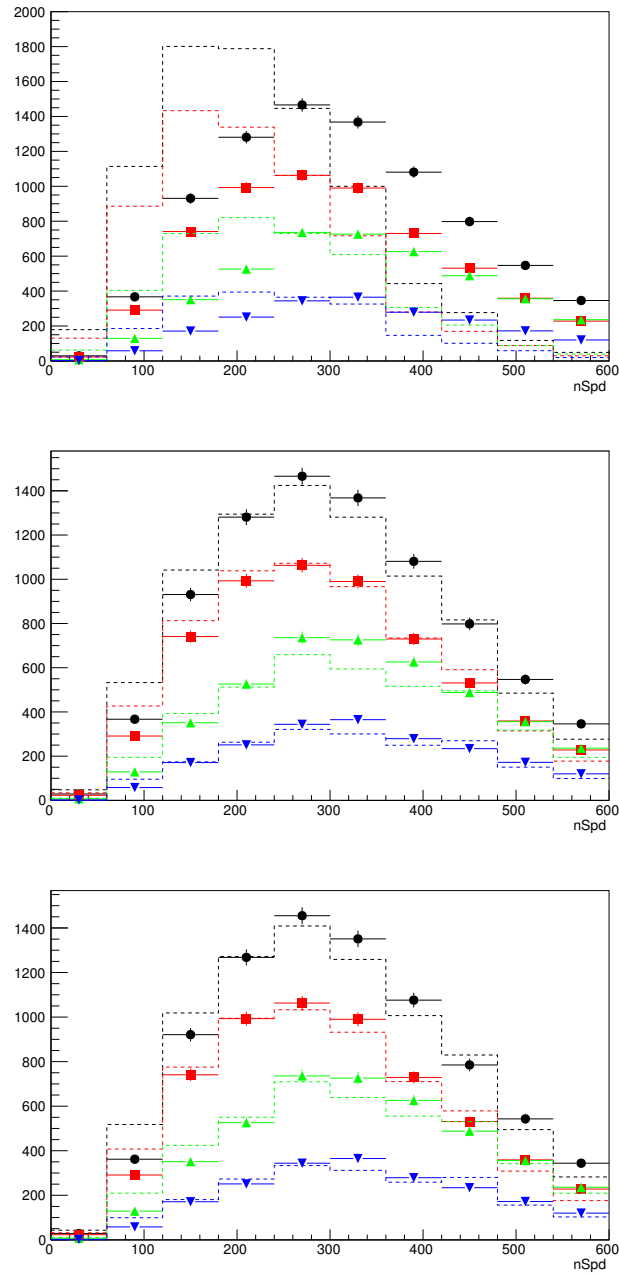
Fig. 3.9 Comparison between the SPD multiplicity between data (full points) and Monte Carlo (dashed histograms). In each figure, the total number of events is shown in black, the L0Hadron_T0S are shown in red, the L0Global_TIS in green and L0Global_TIS && L0Hadron_T0S events are shown in blue (full points data, dashed histogram MC). Top: SPD multiplicity without any correction. Middle: the SPD multiplicity in Monte Carlo is scaled by a factor 1.4. Bottom: L0Hadron_T0S and L0Global_TIS efficiencies in the Monte Carlo are corrected in order to match the data.
