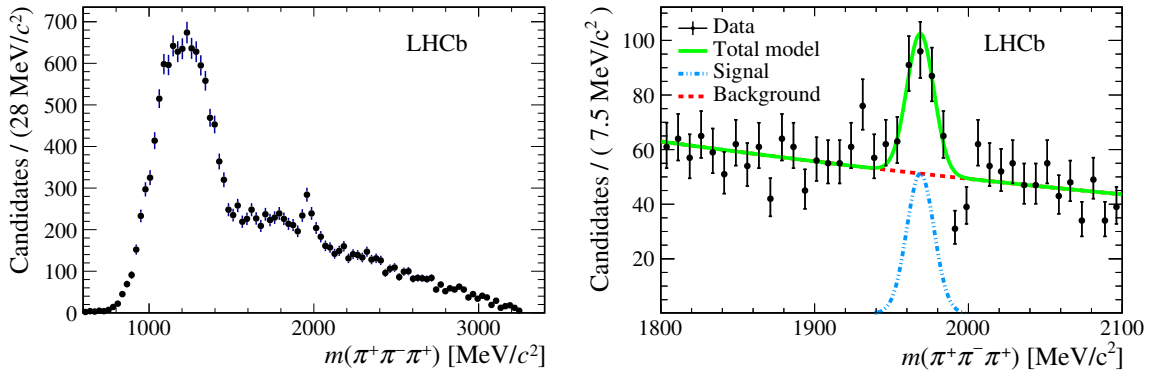
Fig. 6.7 (left) Distribution of m(3\pi) after selection, requiring m(D^{*-}3\pi) to be between 5200 and 5350 \text{MeV}/c^2 ; (right) fit in the mass region around the D_s^+ .
