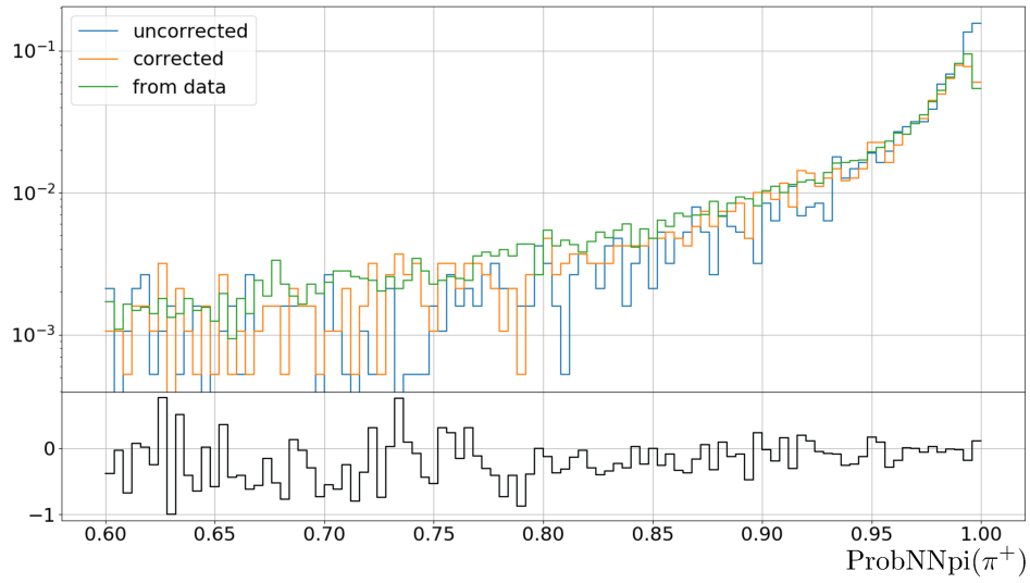
Fig. 3.3 Corrected (orange), uncorrected (blue) and data (green) \text{ProbNN}\pi for the same sign pion ( \pi^+ ) in 2012 for the exclusive B^0 \rightarrow D^*3\pi peak. Pulls are defined as \frac{X^{corr} - X^{data}}{X^{data}} .
