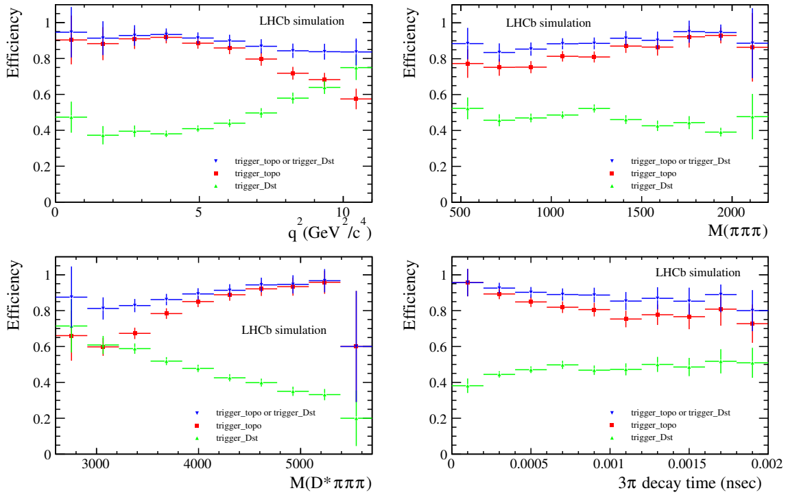
Fig. 3.11 Efficiency for different trigger requirements as a function of the transferred momentum, q^2 , to the \tau \nu_\tau system (top left), the 3\pi invariant mass (top right), the D^* 3\pi invariant mass (bottom left), and the 3\pi decay time (bottom right), for D^* 3\pi X inclusive Monte Carlo.
