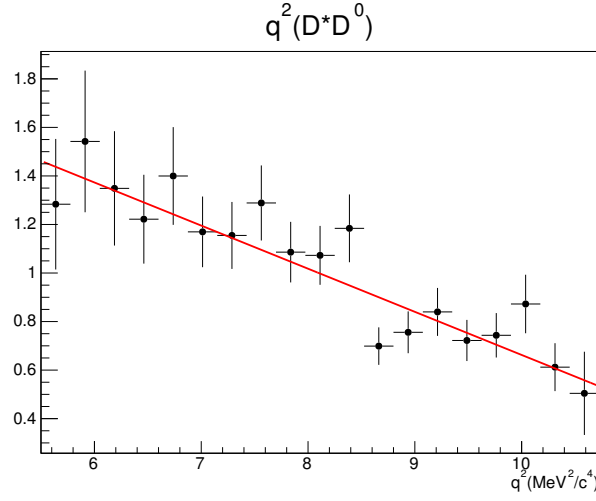
Fig. 5.4 Ratio data/MC on the q^2 distribution for events from the B \rightarrow D^{*-} D^0 X control sample. The fit to a linear function is shown in red, and it is applied as a correction to the D^0 component of the Monte Carlo.
