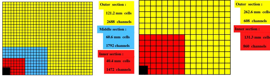
Fig. 2.7 Lateral segmentation of the SPD, PS, ECAL (left) and HCAL (right). Only one quarter of the detector front face is represented, but the number of cells correspond to the entire detector plane.
