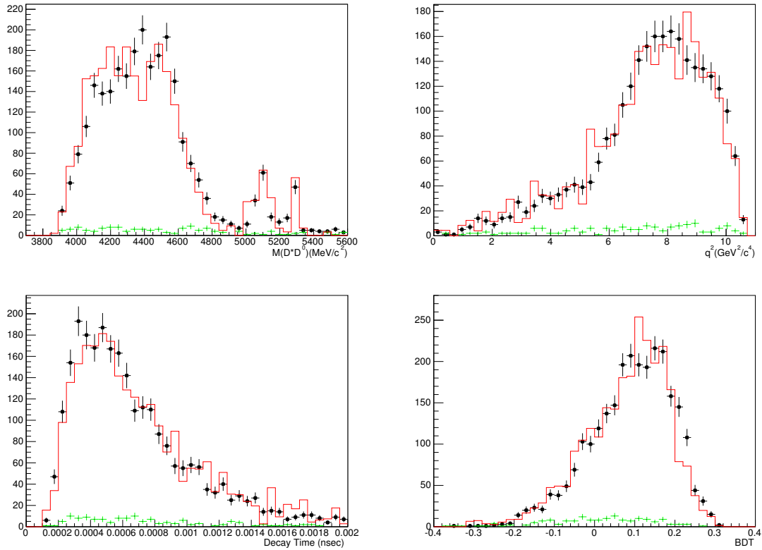
Fig. 5.5 Comparison between data (black points) and the D^{*-} 3\pi X inclusive Monte Carlo (red) for the M(D^* K 3\pi) (top left), q^2 (top right), 3\pi decay time (bottom left) and BDT (bottom right) distributions for the B \rightarrow D^{*-} D^0 X control sample after applying the correction on the q^2 distribution. The combinatorial background, described by the wrong-sign events from the corresponding stripping line, is shown in green.
