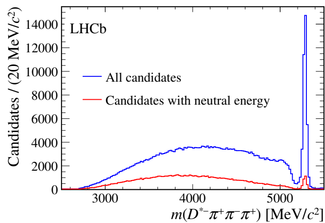
Fig. 4.7 Distribution of the D^{*-}3\pi mass (blue) before and (red) after a requirement of finding at least 8 GeV of energy in the electromagnetic calorimeter around the 3\pi direction.
