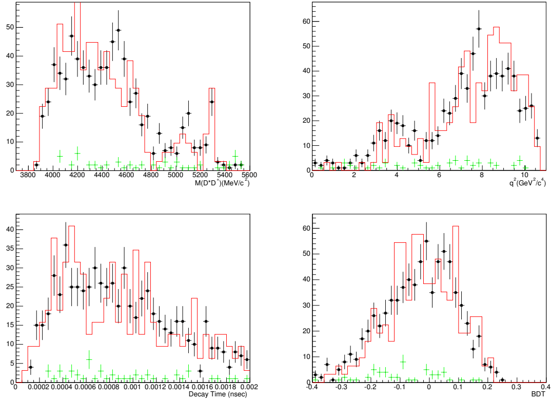
Fig. 5.6 Comparison between data (black points) and the D^{*-}3\pi X inclusive Monte Carlo (red) for the B \rightarrow D^{*-}D^+X control sample. The combinatorial background, described by the wrong-sign events from the corresponding stripping line, is shown in green. It is worth to note the large decay time observed due to the long D^+ lifetime.
