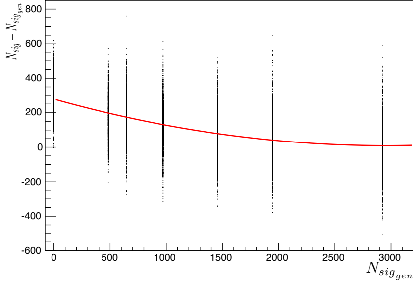
Fig. 6.5 Difference between the signal yield from the fits and the generated yield with respect to the generated value. At the nominal value, the fit bias is +40 events, which must be used to correct the signal yield obtained in the nominal fit.
