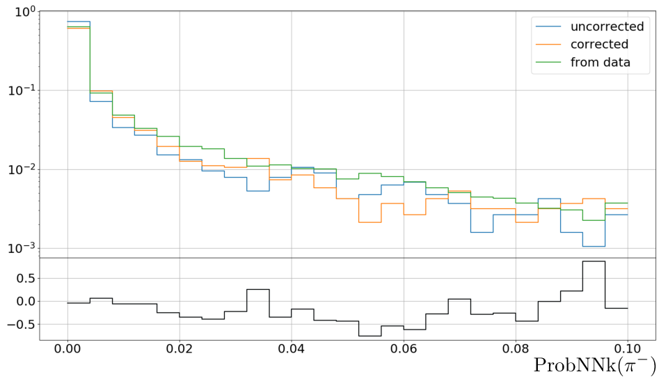
Fig. 3.4 Corrected (orange), uncorrected (blue) and data (green) \text{ProbNNk} for the opposite sign pion ( \pi^- ) in 2012 for the exclusive B^0 \rightarrow D^*3\pi peak. Pulls are defined as \frac{X^{corr} - X^{data}}{X^{data}} .
