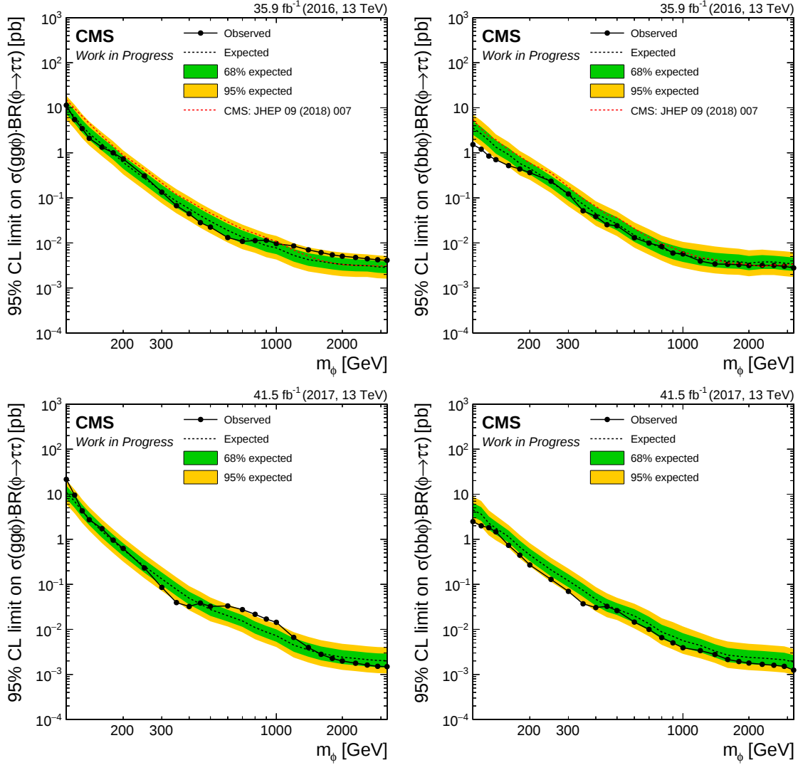
Figure B.1.: Model-independent upper limits at 95% confidence level on (left) gluon fusion and (right) b-associated production \sigma \cdot BR of a Higgs boson \phi with mass m_\phi for (top) 2016 and (bottom) 2017 data. The black dashed line represents the median of the expected upper limit, while the green and yellow bands show the 68% and 95% confidence intervals for a given value of m_\phi . Black dots connected with black solid lines correspond to observed limits. Expected results from CMS [19] are shown as a red dashed line for comparison with results for data-taking in 2016.
