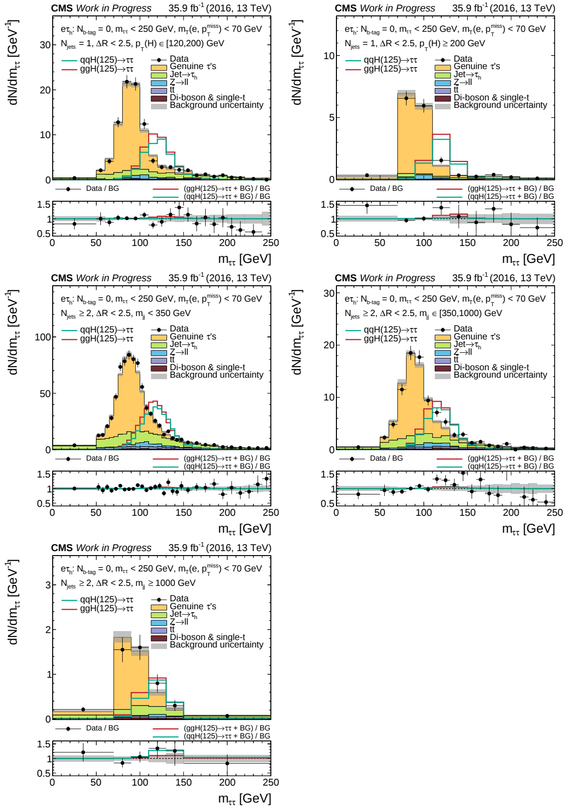
Figure A.17.: Distributions of m_{\tau\tau} for the e\tau_h final state. Expected SM H \rightarrow \tau\tau signal, rescaled for shape comparison in the upper panels, is shown with data and stacked background (BG). Grey uncertainty bands illustrate the total BG uncertainty after a maximum likelihood fit for signal strength \mu . In the lower panel, SM H \rightarrow \tau\tau is scaled to SM expectation.
