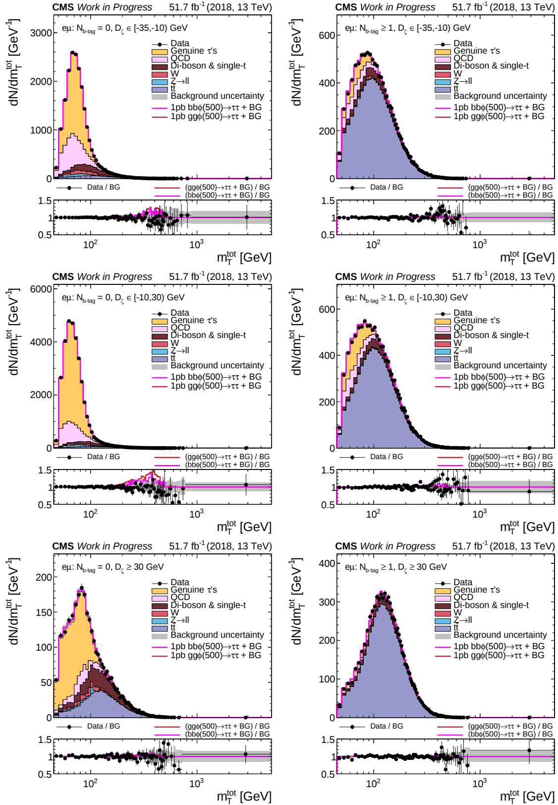
Figure 5.17.: Distributions of m_{\tau}^{\text{tot}} for e\mu in BSM categories of data-taking in 2018. Stacked expected background (BG) and BSM signals gg\phi and bb\phi with m_{\phi} = 500 \text{ GeV} and \sigma \cdot \text{BR} = 1 \text{ pb} on top of BG are compared with data. Grey uncertainty bands illustrate the total BG uncertainty after a maximum likelihood fit for \mu_{gg\phi} and \mu_{bb\phi} . In the lower panels, the ratio to BG is shown.
