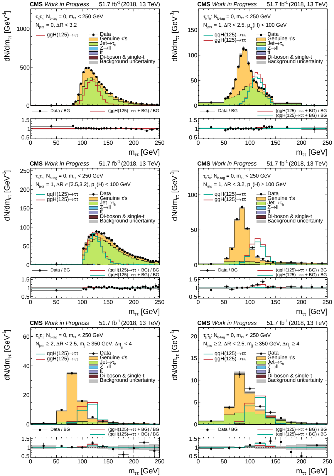
Figure 5.12.: Distributions of m_{\tau\tau} for \tau_h\tau_h in six selected categories of data-taking in 2018. Expected SM H \rightarrow \tau\tau signal, rescaled for shape comparison in the upper panels, is shown with data and stacked background (BG). Grey uncertainty bands illustrate the total BG uncertainty after a maximum likelihood fit for \mu . In the lower panel, SM H \rightarrow \tau\tau is scaled to SM expectation.
