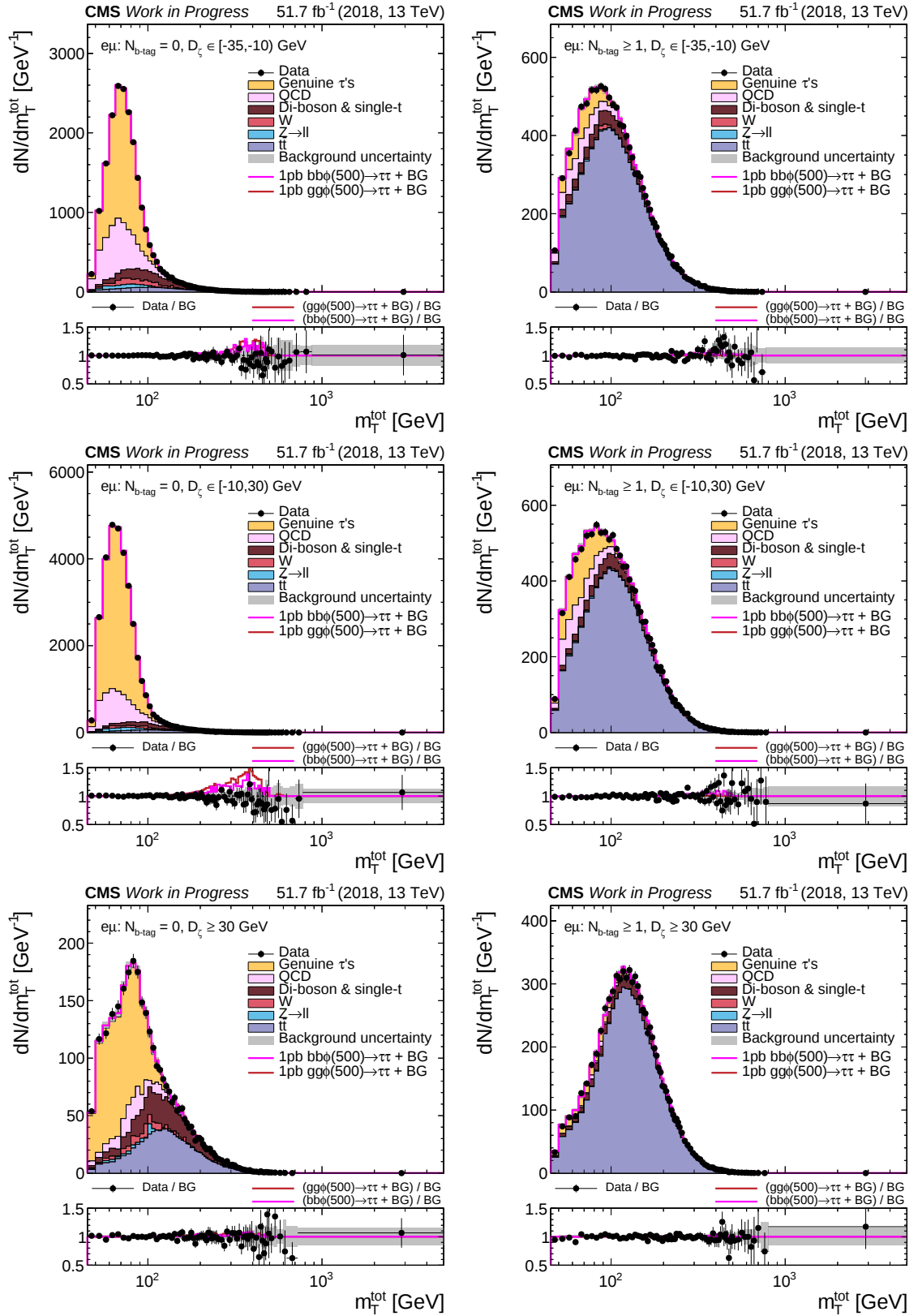
Figure A.36.: Distributions of m_{\tau}^{\text{tot}} in the BSM categories of the e\mu final state. Stacked expected background (BG) and BSM signals g\bar{g}\phi and b\bar{b}\phi with m_{\phi} = 500 GeV and \sigma \cdot \text{BR} = 1 pb on top of BG are compared with data. Grey uncertainty bands illustrate the total BG uncertainty after a maximum likelihood fit for \mu_{g\bar{g}\phi} and \mu_{b\bar{b}\phi} . In the lower panels, the ratio to BG is shown.
