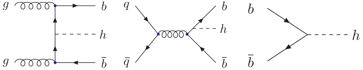
Figure 4.20.: Feynman diagrams for the Higgs boson fusion production associated with bottom quarks at leading order in QCD [156]. On the left and in the middle, diagrams from 4FS, on the right, a 5FS diagram are shown.
