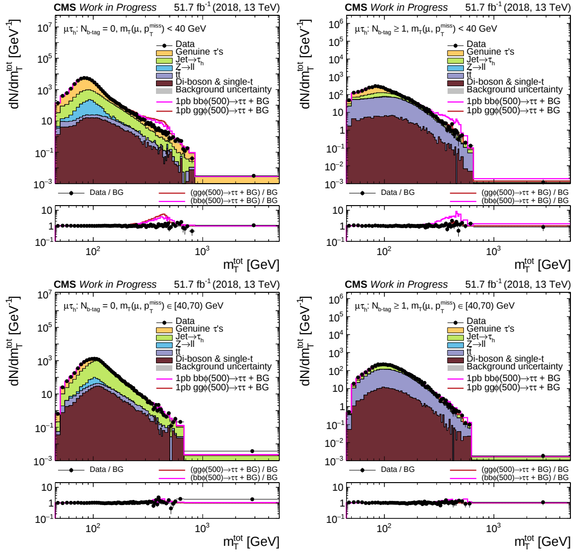
Figure 5.19.: Distributions of m_T^{\text{tot}} for \mu\tau_h in BSM categories of data-taking in 2018. Stacked expected background (BG) and BSM signals gg \phi and bb \phi with m_\phi = 500 \text{ GeV} and \sigma \cdot \text{BR} = 1 \text{ pb} on top of BG are compared with data. Grey uncertainty bands illustrate the total BG uncertainty after a maximum likelihood fit for \mu_{\text{gg}\phi} and \mu_{\text{bb}\phi} . In the lower panels, the ratio to BG is shown.
