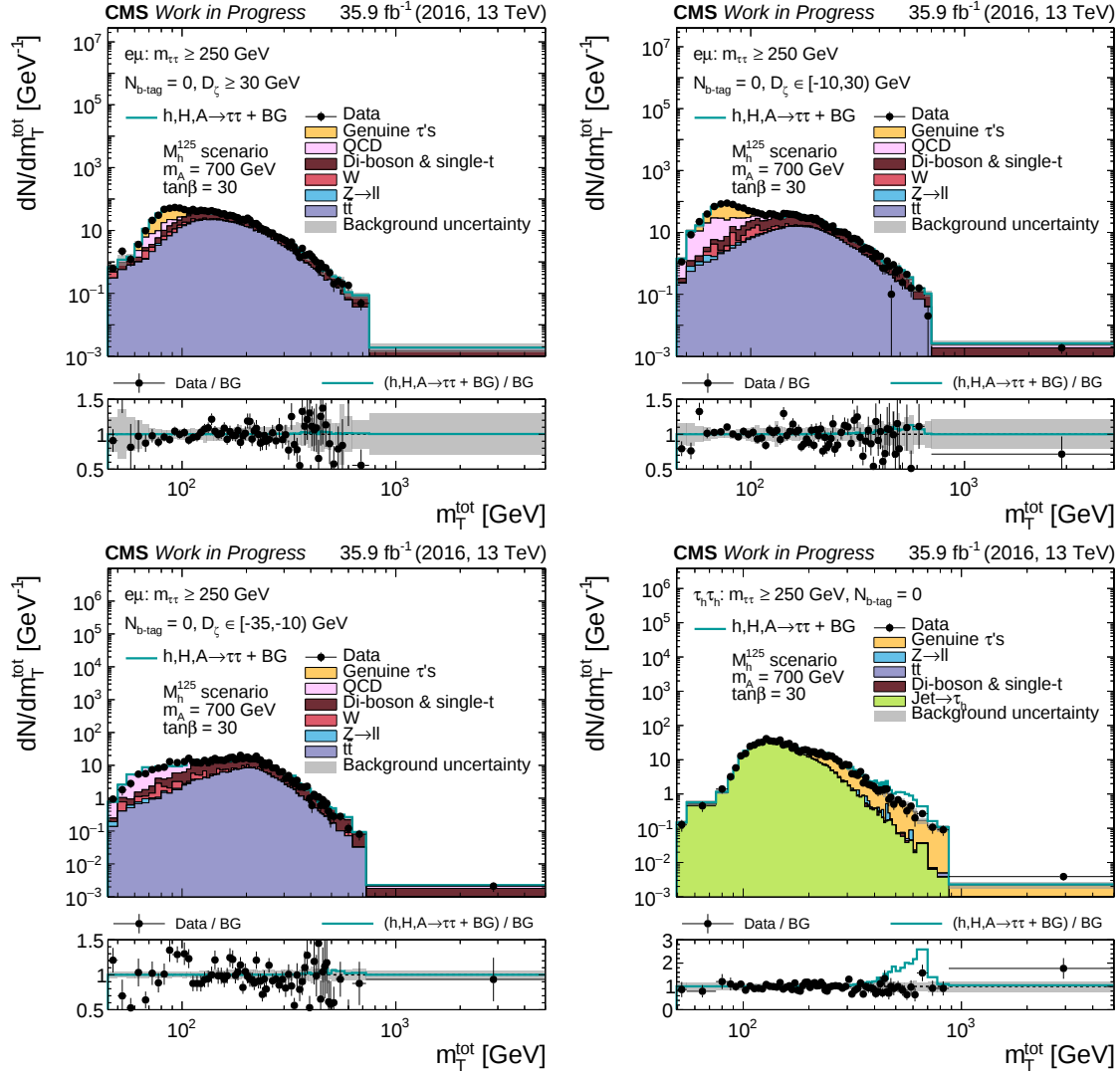
Figure A.45.: Distributions of m_T^{\text{tot}} in the BSM categories with N_{b\text{-tag}} = 0 and m_{\tau\tau} \geq 250 GeV of the (top and bottom left) e\mu and (bottom right) \tau_h\tau_h final states. The signal prediction of the M_h^{125} scenario at (m_A, \tan\beta) = (700 \text{ GeV}, 30) for the heavy Higgs bosons H and A is shown as signal, resulting in a single mass degenerate resonance dominated by the b -quark associated production. The signal is added on top of the stacked background expectation and compared with data. Grey uncertainty bands illustrate the total BG uncertainty after a maximum likelihood fit performed for the fixed (m_A, \tan\beta) values.
