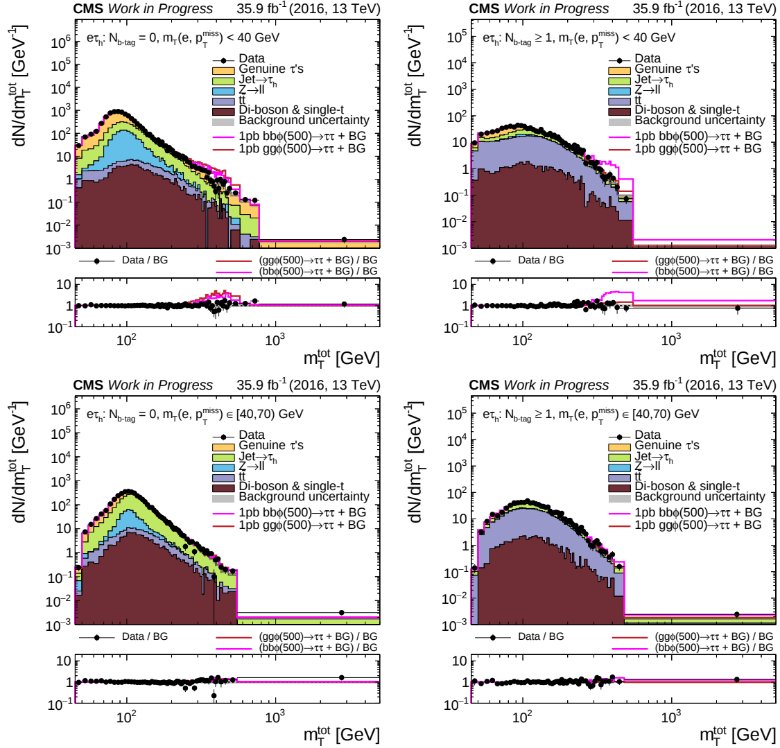
Figure A.37.: Distributions of m_T^{\text{tot}} in the BSM categories of the e\tau_h final state. Stacked expected background (BG) and BSM signals g\bar{g}\phi and b\bar{b}\phi with m_\phi = 500 \text{ GeV} and \sigma \cdot \text{BR} = 1 \text{ pb} on top of BG are compared with data. Grey uncertainty bands illustrate the total BG uncertainty after a maximum likelihood fit for \mu_{g\bar{g}\phi} and \mu_{b\bar{b}\phi} . In the lower panels, the ratio to BG is shown.
