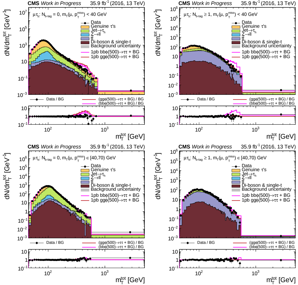
Figure A.40.: Distributions of m_T^{\text{tot}} in the BSM categories of the \mu\tau_h final state. Stacked expected background (BG) and BSM signals gg\phi and bb\phi with m_\phi = 500 GeV and \sigma \cdot \text{BR} = 1 pb on top of BG are compared with data. Grey uncertainty bands illustrate the total BG uncertainty after a maximum likelihood fit for \mu_{gg\phi} and \mu_{bb\phi} . In the lower panels, the ratio to BG is shown.
