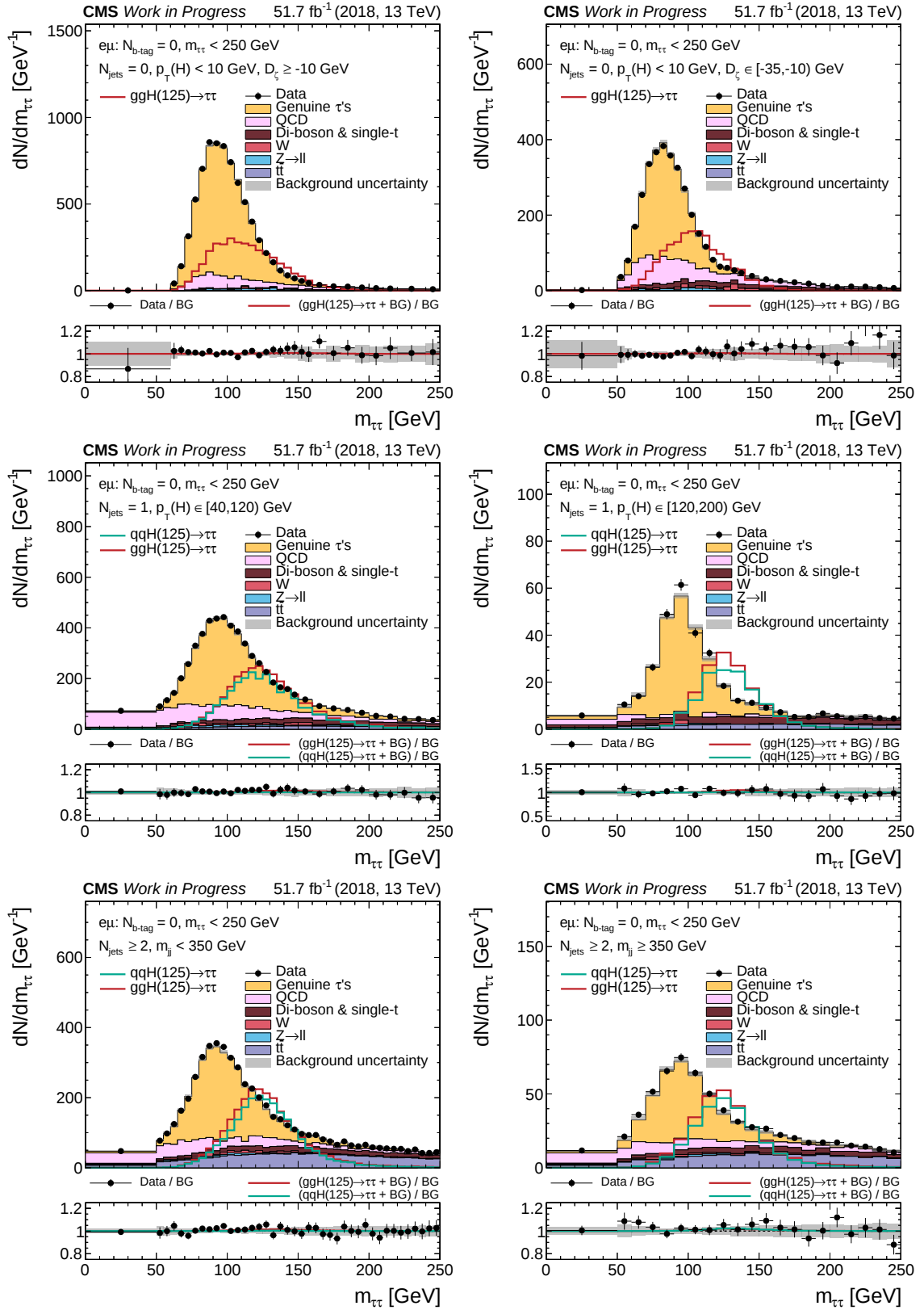
Figure 5.9.: Distributions of m_{\tau\tau} for e\mu in six selected categories of data-taking in 2018. Expected SM H \rightarrow \tau\tau signal, rescaled for shape comparison in the upper panels, is shown with data and stacked background (BG). Grey uncertainty bands illustrate the total BG uncertainty after a maximum likelihood fit for \mu . In the lower panel, SM H \rightarrow \tau\tau is scaled to SM expectation.
