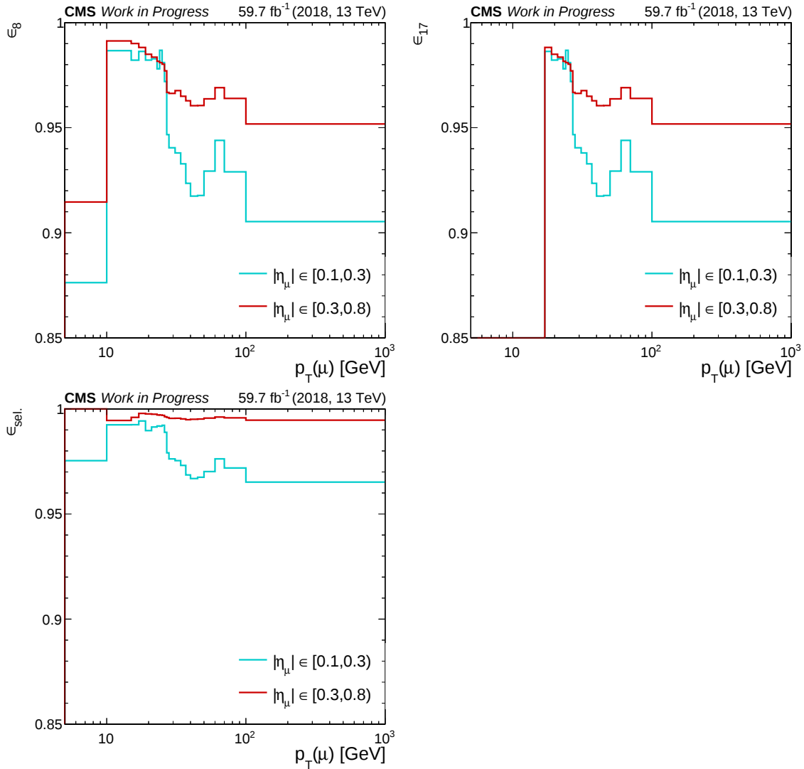
Figure 4.4.: Measurements of the muon efficiencies (top left) \epsilon_8 , (top right) \epsilon_{17} and (bottom left) \epsilon_{\text{sel}} , as functions of p_T(\mu) for different regions of |\eta_\mu| .
