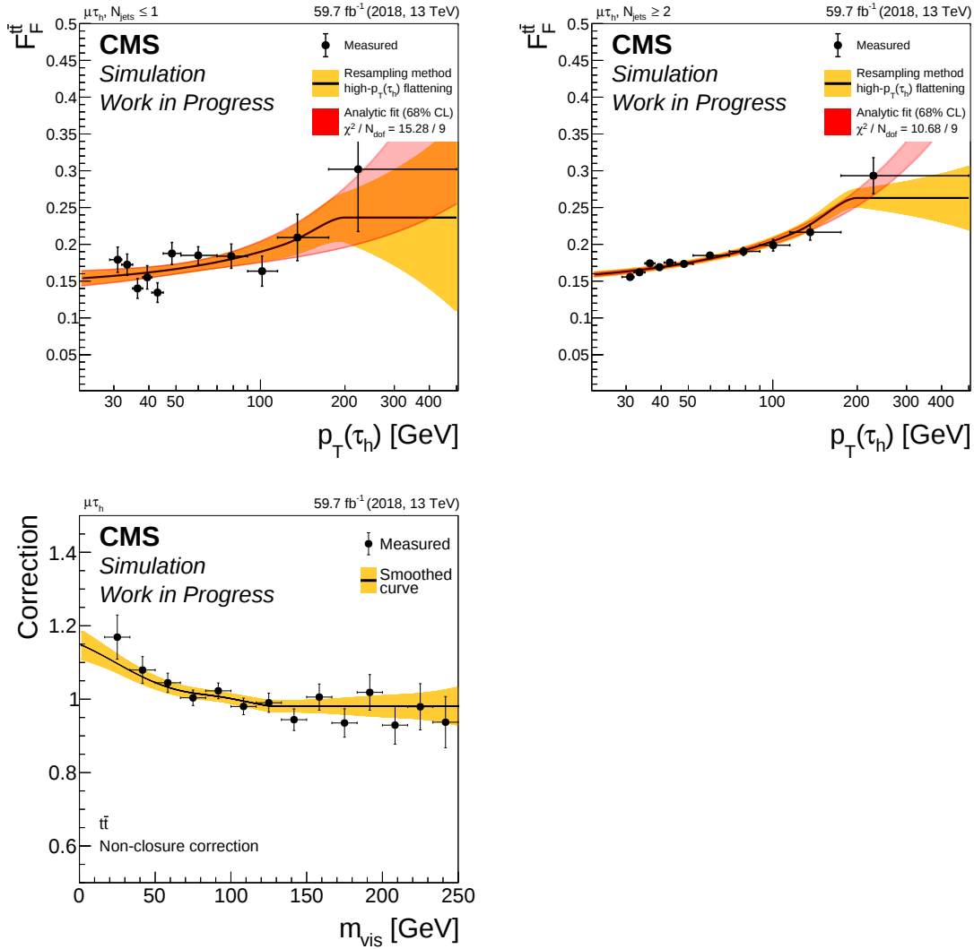
Figure 4.9.: F_F^{\tau\tau} and its correction for the \mu\tau_h final state of the data-taking in 2018. Top: The uncorrected F_F^{\tau\tau} value as a function of p_T(\tau_h) for (left) N_{\text{jets}} \leq 1 and (right) N_{\text{jets}} \geq 2 . Bottom left: Correction of F_F^{\tau\tau} in m_{\text{vis}} .
