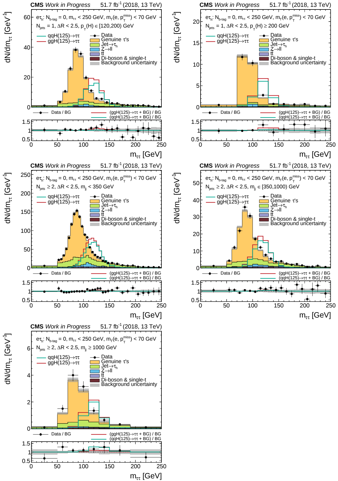
Figure A.21.: Distributions of m_{\tau\tau} for the e\tau_h final state. Expected SM H \rightarrow \tau\tau signal, rescaled for shape comparison in the upper panels, is shown with data and stacked background (BG). Grey uncertainty bands illustrate the total BG uncertainty after a maximum likelihood fit for signal strength \mu . In the lower panel, SM H \rightarrow \tau\tau is scaled to SM expectation.
