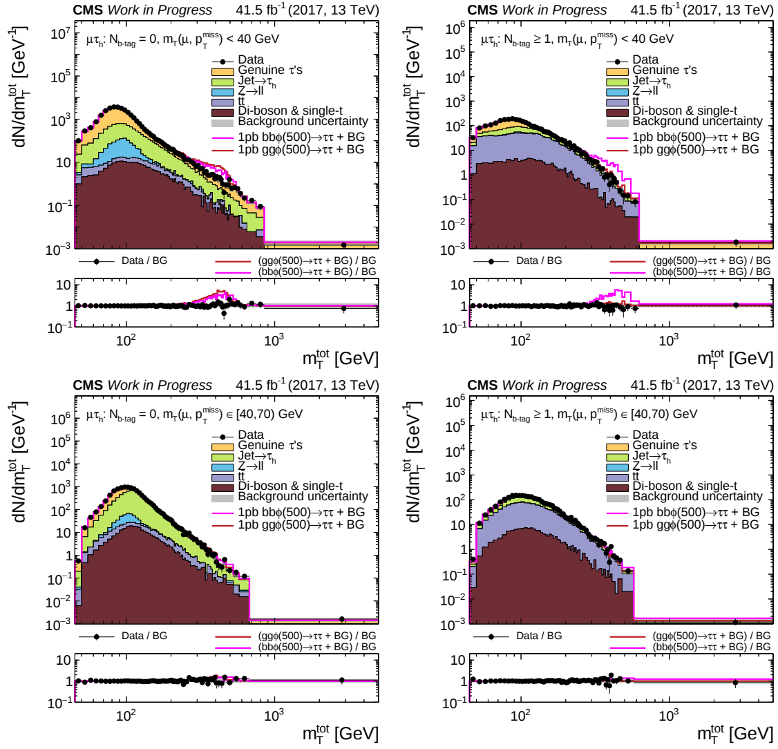
Figure A.41.: Distributions of m_T^{\text{tot}} in the BSM categories of the \mu\tau_h final state. Stacked expected background (BG) and BSM signals gg\phi and bb\phi with m_\phi = 500 GeV and \sigma \cdot \text{BR} = 1 pb on top of BG are compared with data. Grey uncertainty bands illustrate the total BG uncertainty after a maximum likelihood fit for \mu_{gg\phi} and \mu_{bb\phi} . In the lower panels, the ratio to BG is shown.
