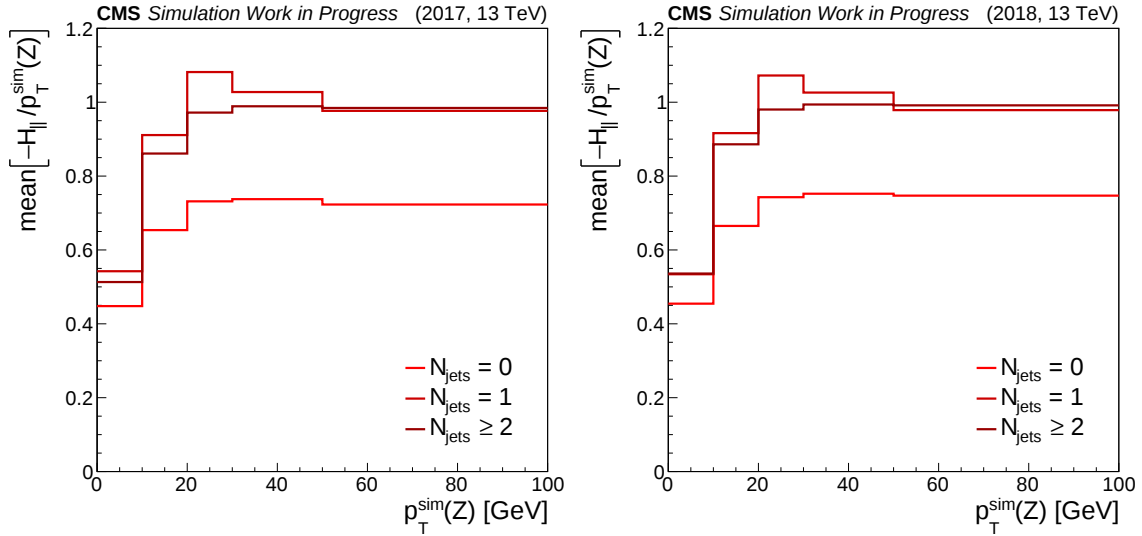
Figure 4.32.: The mean of the ratio between the hadronic recoil component parallel to the reconstructed Z boson \vec{p}_T , and the magnitude of the simulated transverse momentum of the Z boson, p_T^{\text{sim}}(Z) . The values are shown for the three N_{\text{jets}} categories and as a function of p_T^{\text{sim}}(Z) , binned in the same manner as the corresponding categorization, and chosen for the data-taking years 2017 and 2018. For the application of these measurements, the values at the bin edges of the histograms are linearly interpolated.
