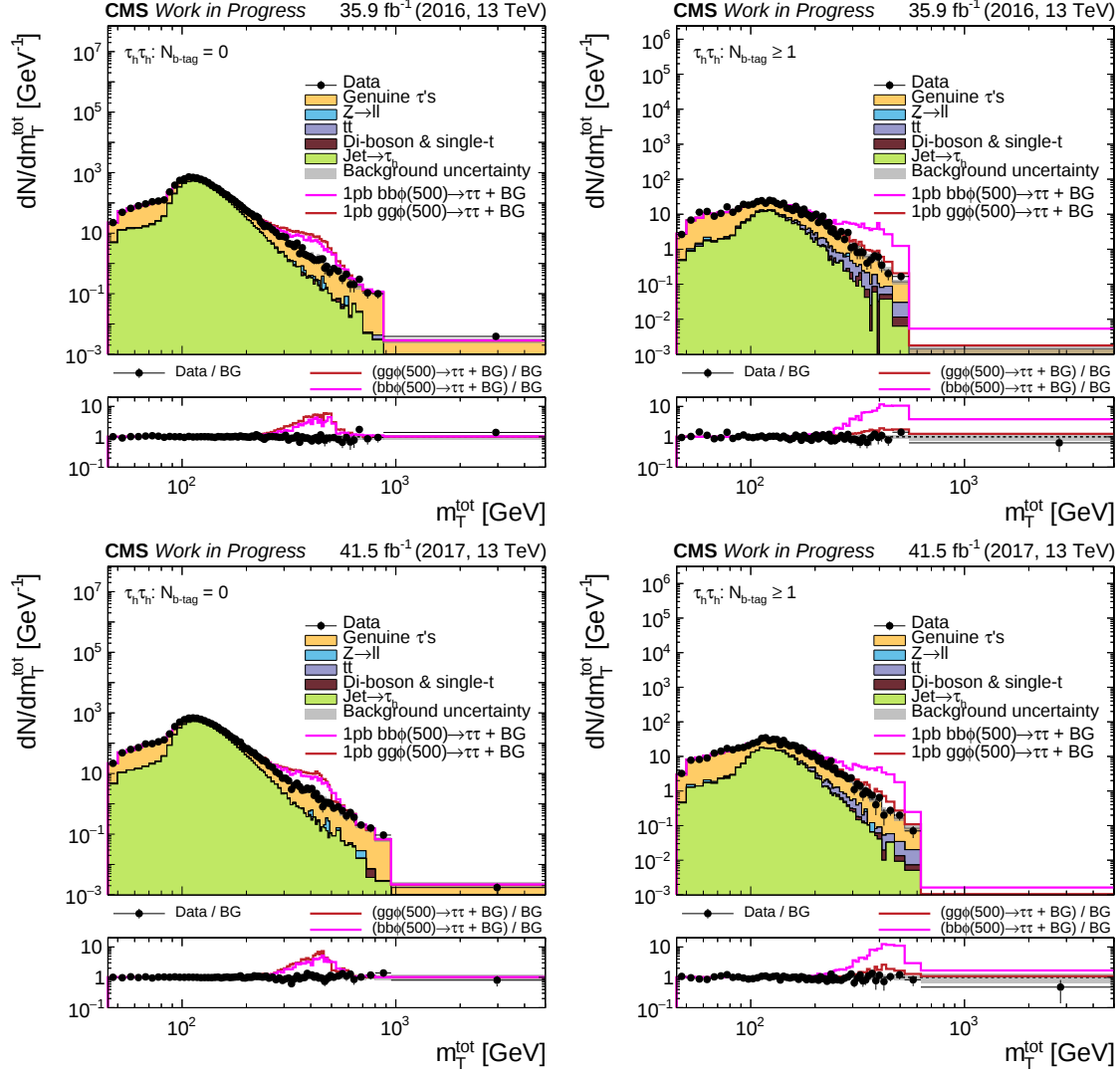
Figure A.43.: Distributions of m_T^{\text{tot}} in the BSM categories of the \tau_h \tau_h final state. Stacked expected background (BG) and BSM signals gg\phi and bb\phi with m_\phi = 500 GeV and \sigma \cdot \text{BR} = 1 pb on top of BG are compared with data. Grey uncertainty bands illustrate the total BG uncertainty after a maximum likelihood fit for \mu_{gg\phi} and \mu_{bb\phi} . In the lower panels, the ratio to BG is shown.
