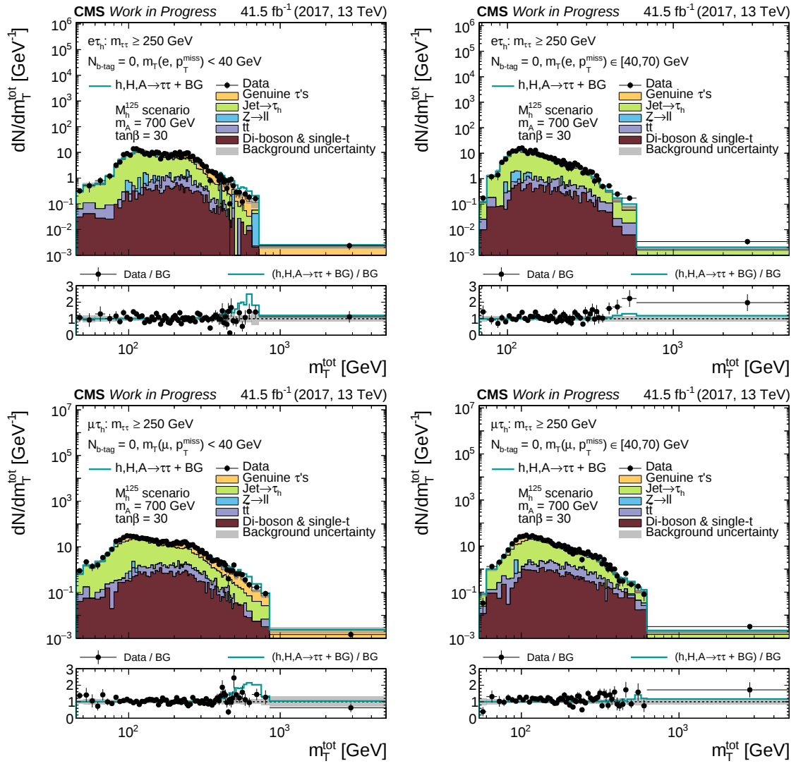
Figure A.48.: Distributions of m_T^{\text{tot}} in the BSM categories with N_{b\text{-tag}} = 0 and m_{\tau\tau} \geq 250 GeV of the (top) e\tau_h and (bottom) \mu\tau_h final states. The signal prediction of the M_h^{125} scenario at (m_A, \tan\beta) = (700 \text{ GeV}, 30) for the heavy Higgs bosons H and A is shown as signal, resulting in a single mass degenerate resonance dominated by the b -quark associated production. The signal is added on top of the stacked background expectation and compared with data. Grey uncertainty bands illustrate the total BG uncertainty after a maximum likelihood fit performed for the fixed (m_A, \tan\beta) values.
