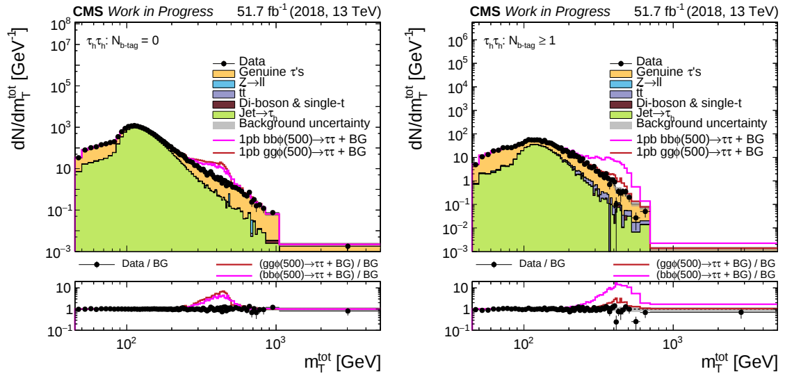
Figure A.44.: Distributions of m_T^{\text{tot}} in the BSM categories of the \tau_h \tau_h final state. Stacked expected background (BG) and BSM signals gg\phi and bb\phi with m_\phi = 500 GeV and \sigma \cdot \text{BR} = 1 pb on top of BG are compared with data. Grey uncertainty bands illustrate the total BG uncertainty after a maximum likelihood fit for \mu_{gg\phi} and \mu_{bb\phi} . In the lower panels, the ratio to BG is shown.
