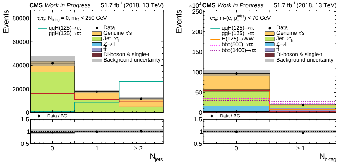
Figure 5.3.: Distributions of the variables used for categorization, (left) N_{\text{jets}} in the \tau_h \tau_h final state and (right) N_{b\text{-tag}} in the e \tau_h final state of the data-taking year 2018 for data and expected signals and backgrounds. The SM H \rightarrow \tau\tau , BSM \phi \rightarrow \tau\tau and SM H \rightarrow WW signals are rescaled for shape comparison in the upper panel of the figures. The grey background uncertainty bands include both statistical and systematic uncertainties in the state before a maximum likelihood fit.
