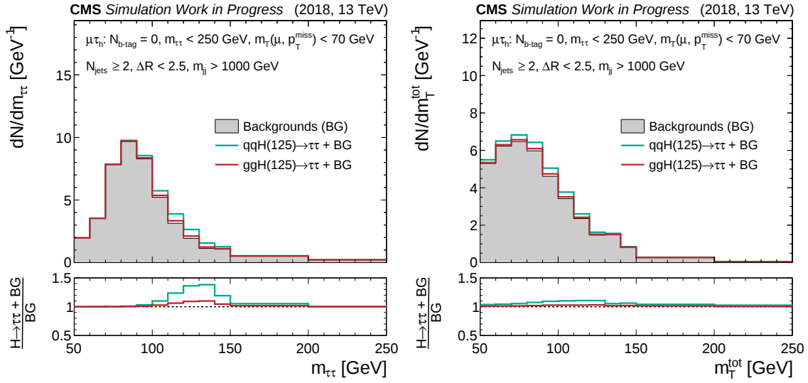
Figure 5.2.: Distributions of the discriminators (left) m_{\tau\tau} and (right) m_{\tau\tau}^{\text{tot}} in the same category sensitive to the SM VBF signal. The signal distribution for m_{\tau\tau} has a better resolution, allowing to discriminate the signal better from backgrounds.
