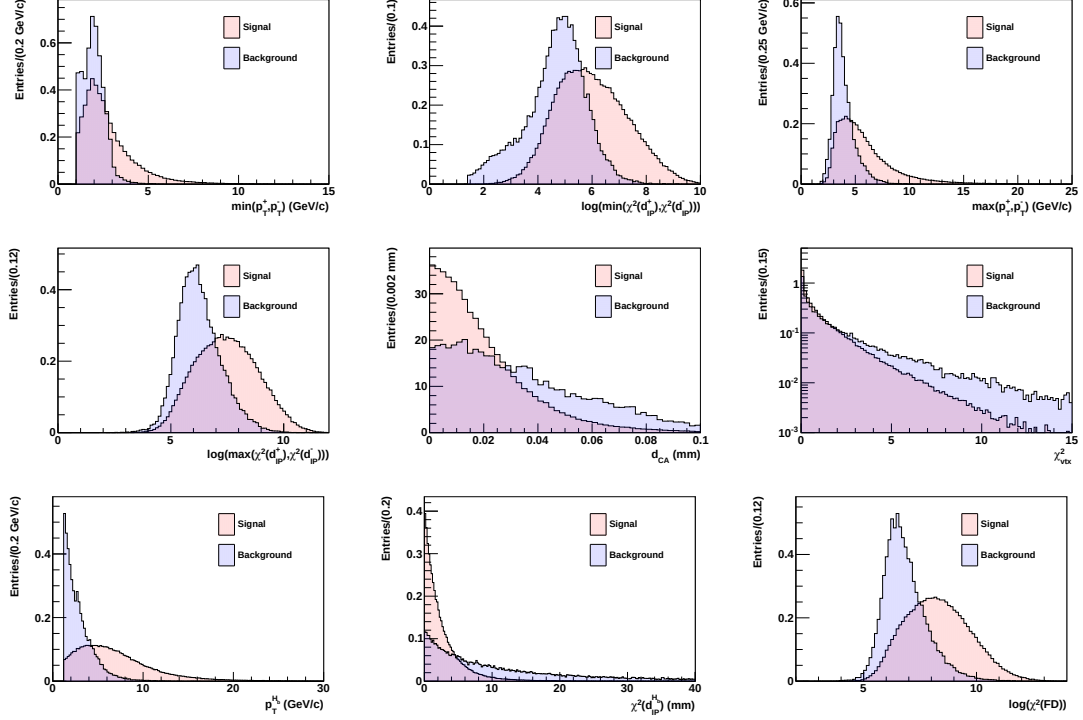
Figure D.5: Distributions of the variables used in the training of the BDT algorithms for (red histogram) B^0 \rightarrow \pi^+ \pi^- decays and (blue histogram) high invariant-mass sideband events. Only 2011 samples are used to produce the histograms.
