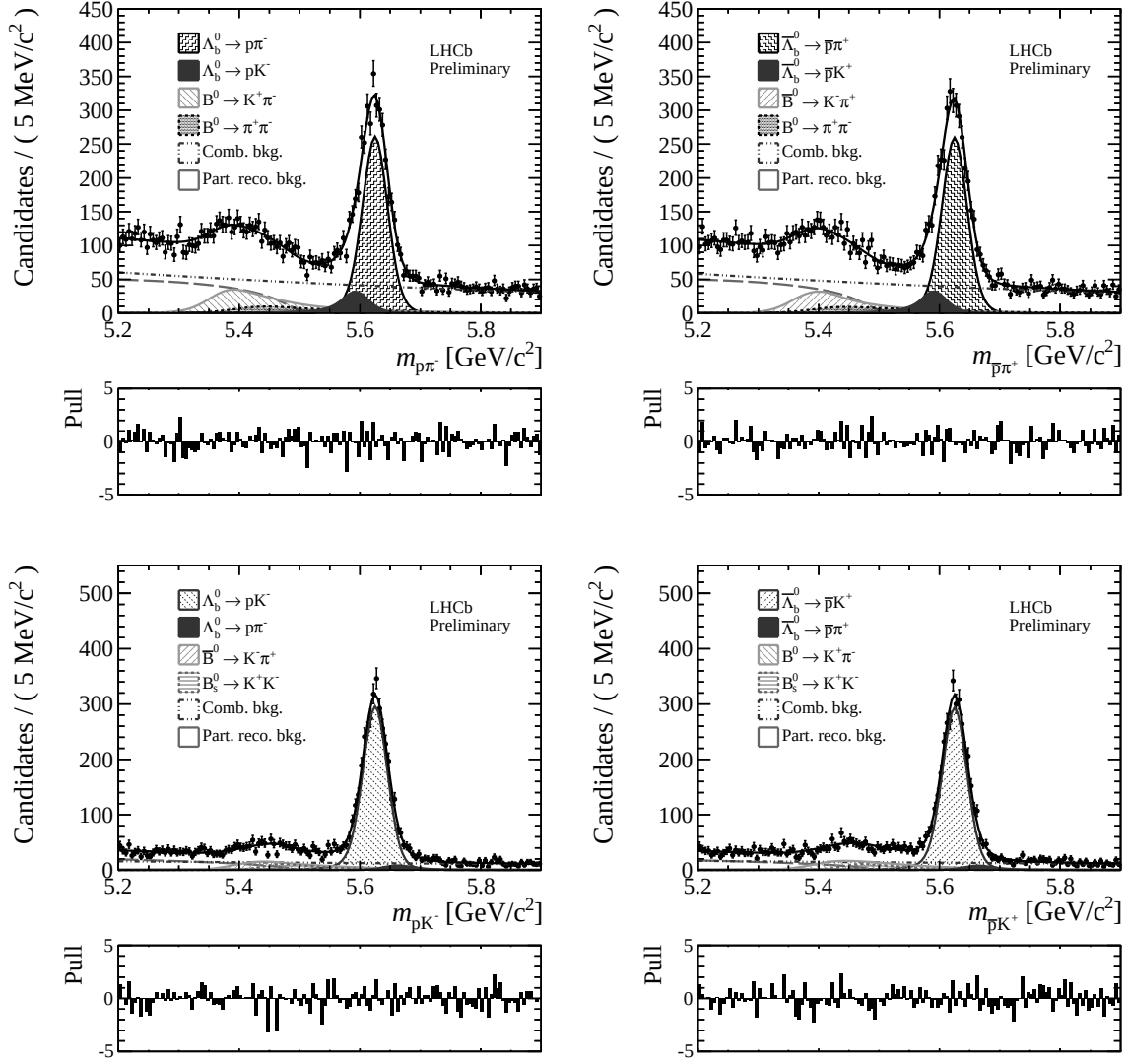
Figure 5.27: Invariant-mass distribution of the (top left) p\pi^- , (top right) \bar{p}\pi^+ , (bottom left) pK^- and (bottom right) \bar{p}K^+ spectra after selection B. The curves superimposed to the data points represent the result of the best fit.
