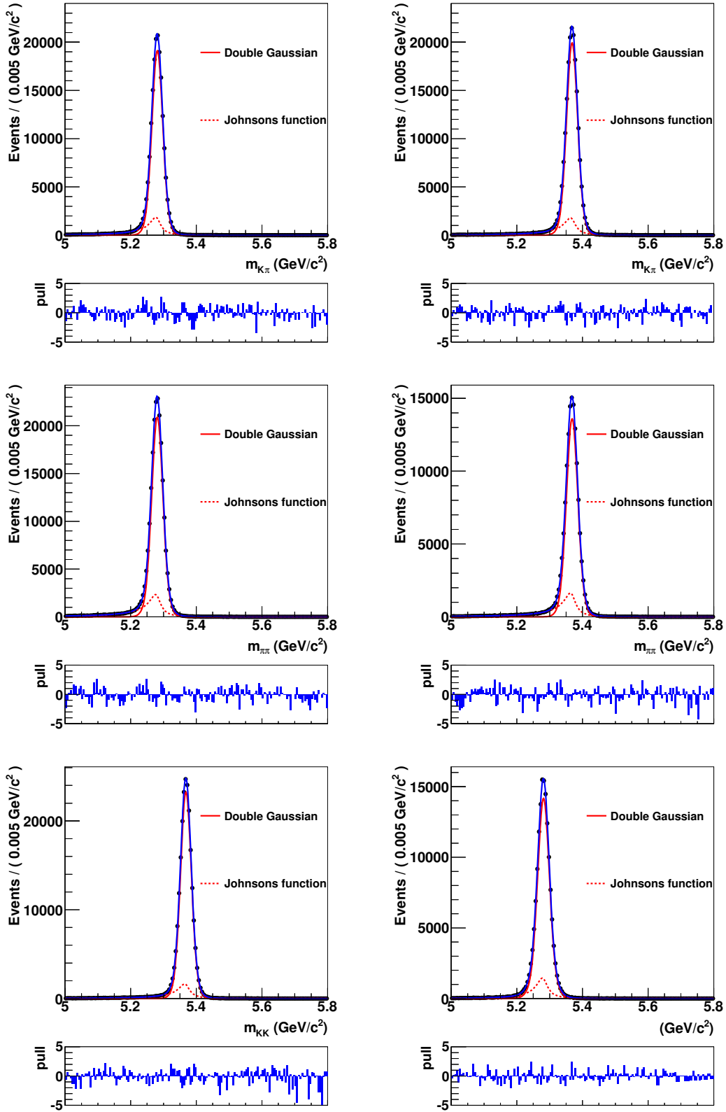
Figure 6.7: Invariant-mass distributions for (from top left to bottom right) B^0 \rightarrow K^+\pi^- , B_s^0 \rightarrow \pi^+K^- , B^0 \rightarrow \pi^+\pi^- , B_s^0 \rightarrow \pi^+\pi^- , B_s^0 \rightarrow K^+K^- and B^0 \rightarrow K^+K^- simulated decays. The result of the best fit with the model described in Eq. (6.7) is superimposed.
