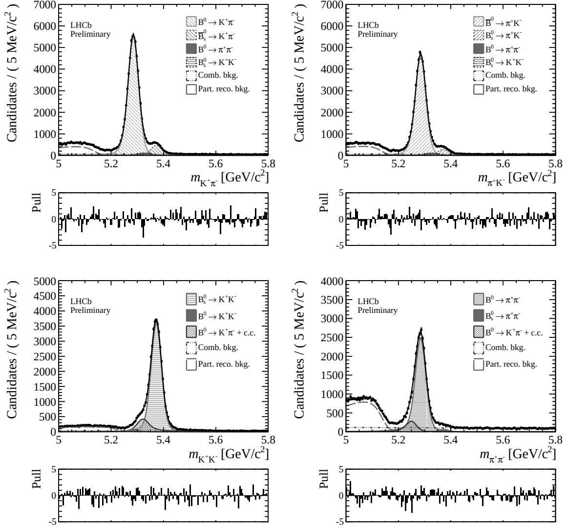
Figure 5.28: Invariant-mass distribution of the (top left) K^+\pi^- , (top right) K^-\pi^+ , (bottom left) K^+K^- and (bottom right) \pi^+\pi^- spectra after selection B. The curves superimposed to the data points represent the result of the best fit.
