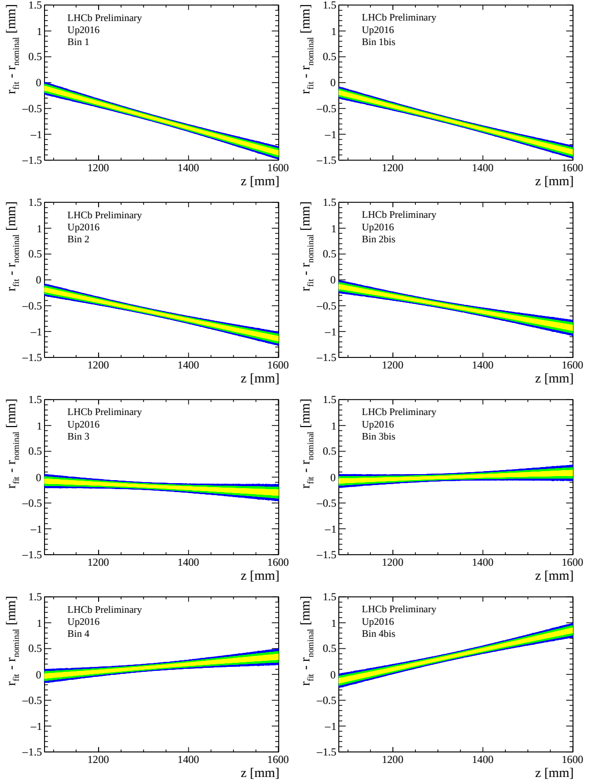
Figure B.13: Difference between the measured and the design radial distance of the beam pipe position in the various \phi sectors as a function of the z coordinate for the Up2016 data sample. The yellow, green and blue bands represent the 1\sigma , 2\sigma and 3\sigma contours.
