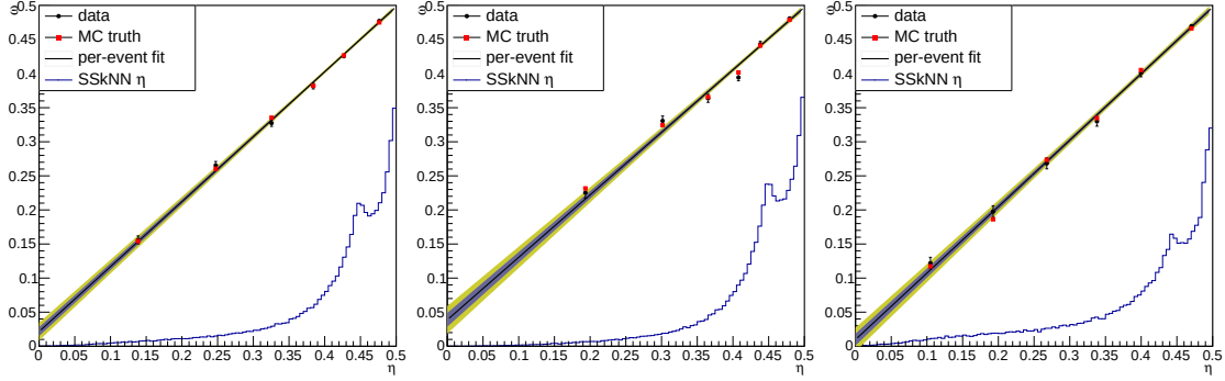
Figure D.14: Calibration plots for the SSkNN tagger in different kinematic regions: (left) whole sample, (center) sub-sample with p_T^B < 9 \text{ GeV}/c and (right) sub-sample with p_T^B > 9 \text{ GeV}/c . The \omega values estimated from the per-event fit using the true decay-time are reported in black, while the true mistag obtained from the MC truth is drawn in red. The two bands in blue and in yellow represent the 66% and 95% of confidence level. The SSkNN \eta distribution is also shown.
