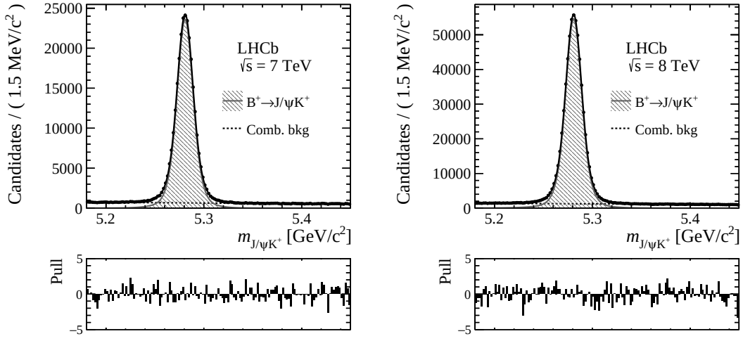
Figure 3.29: Distributions of invariant mass for (left) B^+ \rightarrow J/\psi K^+ 2011 and (right) 2012 decays, with the results of the fit overlaid.
