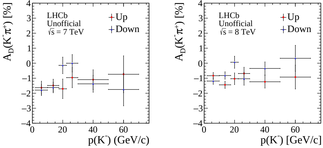
Figure 6.32: Values of A_D(K^-\pi^+) for (left) 2011 and (right) 2012 data as a function of the kaon momentum. Different points are shown for different magnet polarities.
