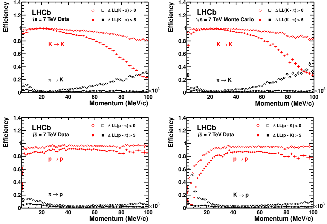
Figure 2.22: (top) Kaon identification efficiency and pion mis-identification rate as a function of the track momentum for (left) real data and (right) simulated events. (bottom) Proton identification efficiency against (left) pions and (right) kaons. The empty and filled markers represent two different \Delta \log \mathcal{L} requirements imposed on the track.
