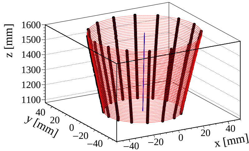
Figure 4.13: 3-D representation of the beam pipe obtained drawing all the measured radial distances in every z slice with the results of the circle fits overlaid and with the representation of the beam pipe axis for 2016 Down sample.
