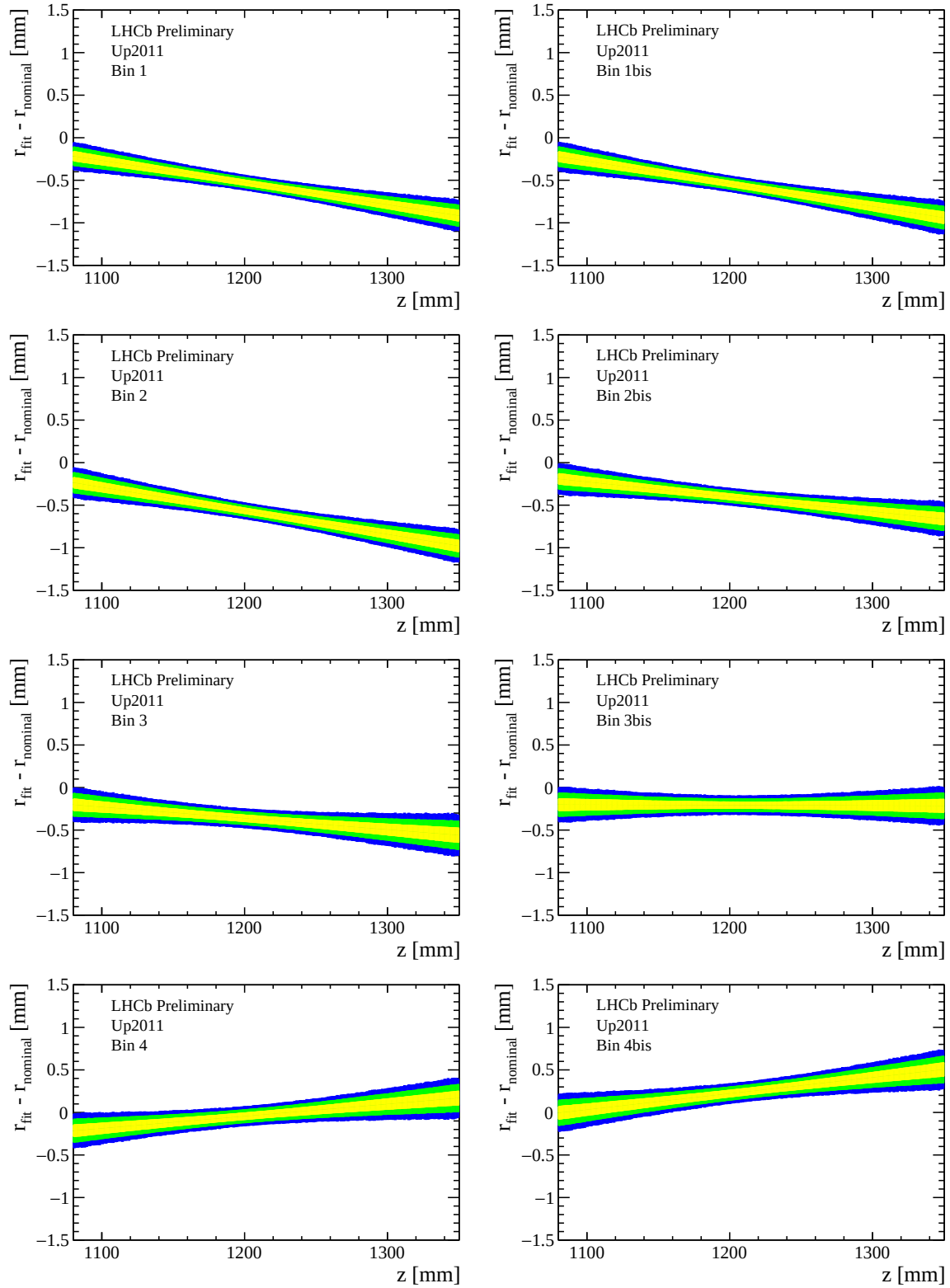
Figure B.1: Difference between the measured and the design radial distance of the beam pipe position in the various \phi sectors as a function of the z coordinate for the Up2011 data sample. The yellow, green and blue bands represent the 1\sigma , 2\sigma and 3\sigma contours.
