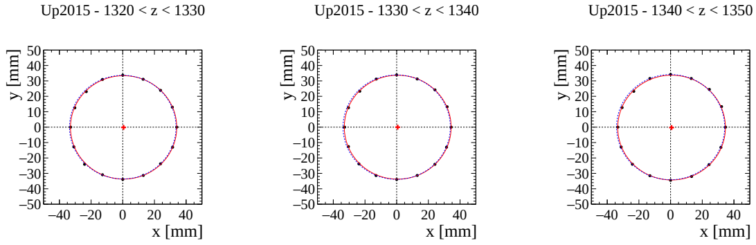
Figure B.31: Measured radial distance in bins of the z coordinate for the Up 2015 sample. The red solid line corresponds to the fitted circle, whereas the blue dashed line is the design reference. The red cross represents the position of the center of the fitted circle. The uncertainties on the radial distances are not shown.
