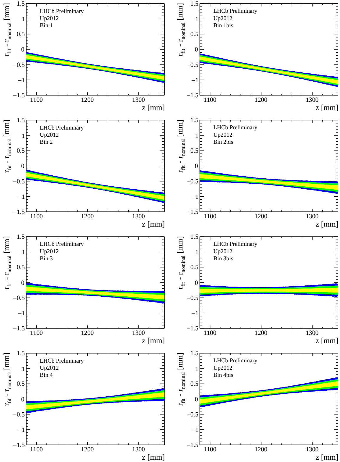
Figure B.5: Difference between the measured and the design radial distance of the beam pipe position in the various \phi sectors as a function of the z coordinate for the Up2012 data sample. The yellow, green and blue bands represent the 1\sigma , 2\sigma and 3\sigma contours.
