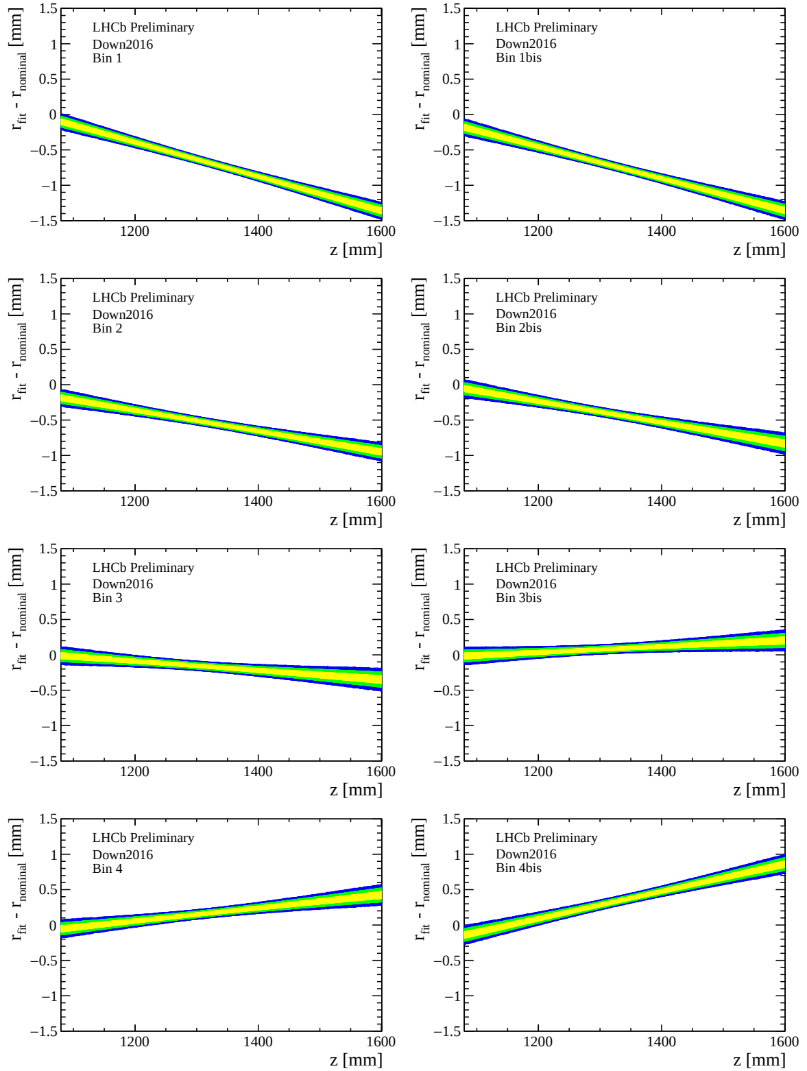
Figure B.15: Difference between the measured and the design radial distance of the beam pipe position in the various \phi sectors as a function of the z coordinate for the Down2016 data sample. The yellow, green and blue bands represent the 1\sigma , 2\sigma and 3\sigma contours.
