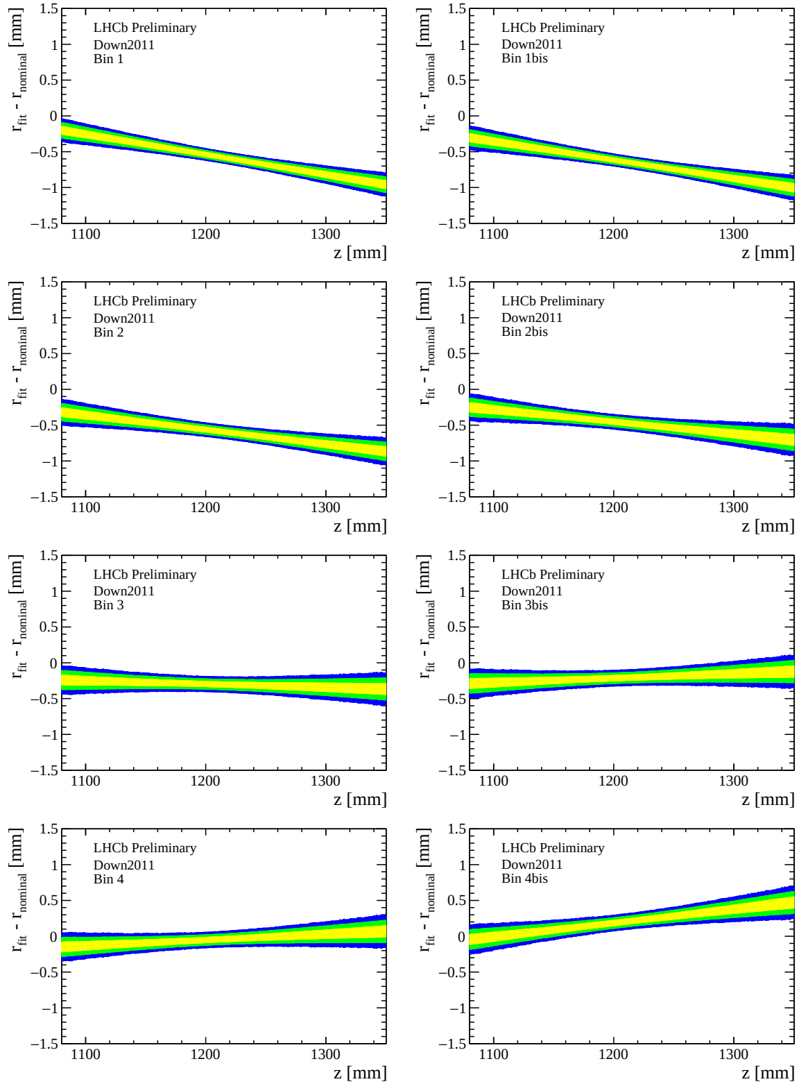
Figure B.3: Difference between the measured and the design radial distance of the beam pipe position in the various \phi sectors as a function of the z coordinate for the Down2011 data sample. The yellow, green and blue bands represent the 1\sigma , 2\sigma and 3\sigma contours.
