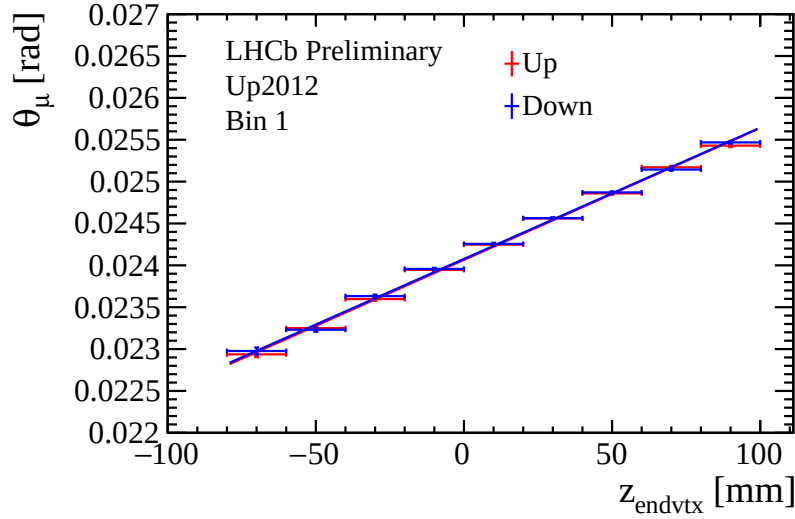
Figure 4.11: Results of the fits to the muon angle at the dip as a function of the J/\psi z_{\text{endvtx}} coordinate for 2012 data.
