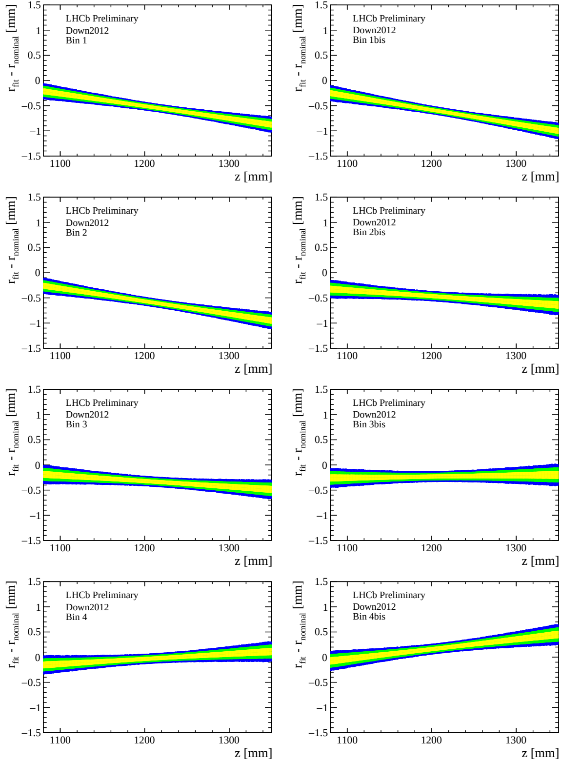
Figure B.7: Difference between the measured and the design radial distance of the beampipe position in the various \phi sectors as a function of the z coordinate for the Down2012 data sample. The yellow, green and blue bands represent the 1\sigma , 2\sigma and 3\sigma contours.
