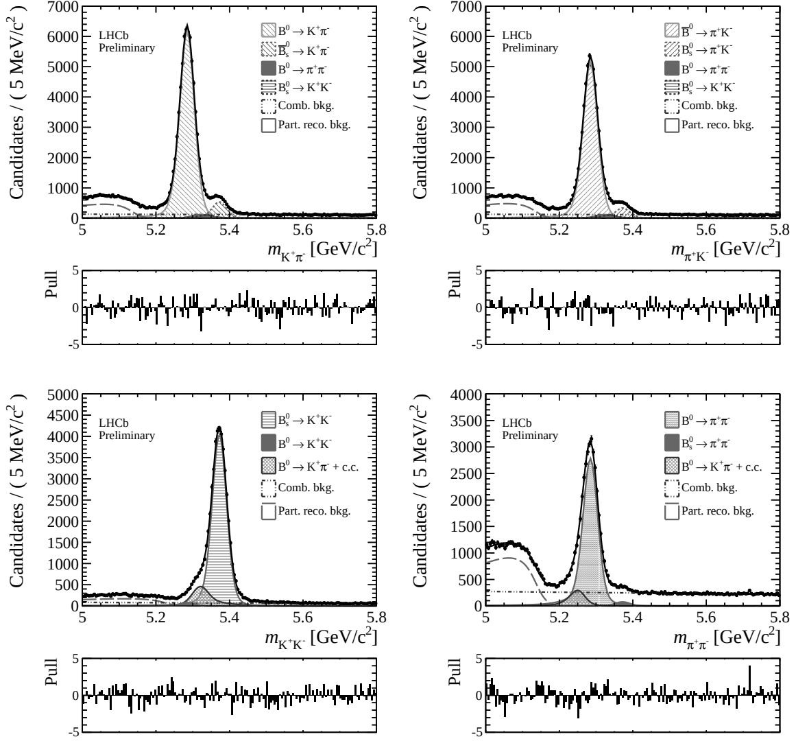
Figure 5.26: Invariant-mass distribution of the (top left) K^+\pi^- , (top right) K^-\pi^+ , (bottom left) K^+K^- and (bottom right) \pi^+\pi^- spectra after selection A. The curves superimposed to the data points represent the result of the best fit.
