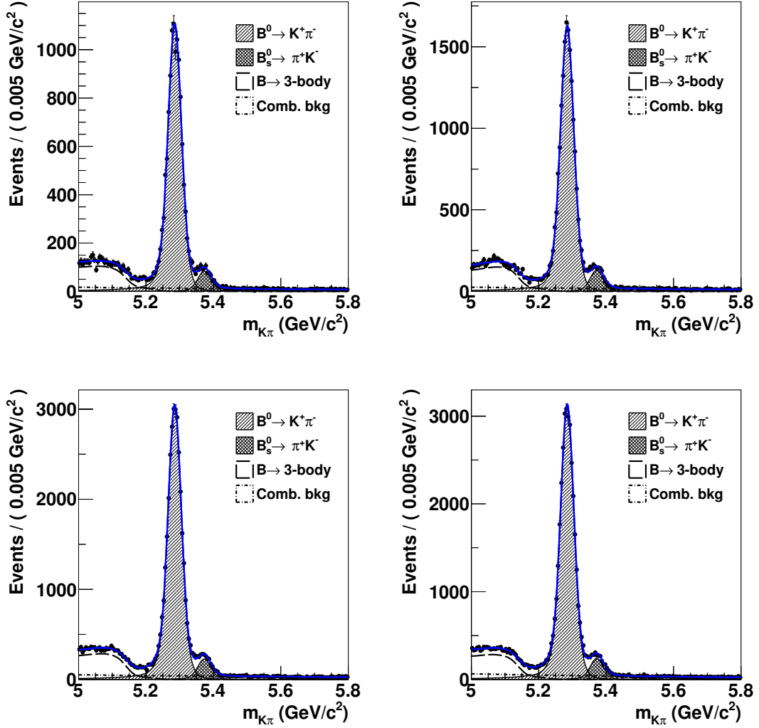
Figure 6.33: Invariant-mass distributions for candidates selected under the K^+ \pi^- and K^- \pi^+ final-state and corresponding to (top left) 2011 up, (top right) 2011 down, (bottom left) 2012 up and (bottom right) 2012 down samples. The results of the best fits are superimposed to the data points.
