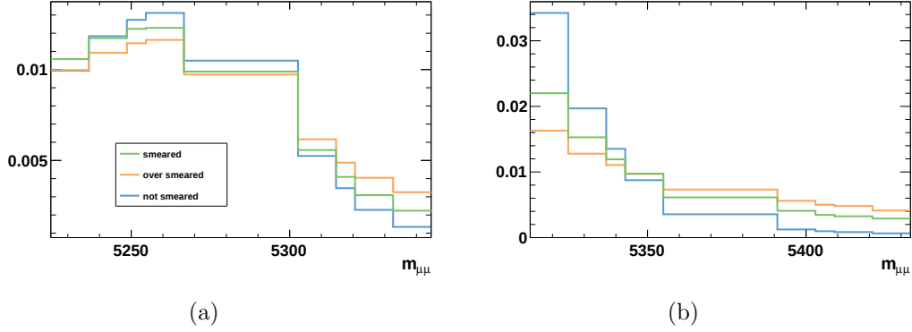
Figure 3.30: Invariant mass shape in the B^0 \rightarrow \mu^+ \mu^- (a) and B_s^0 \rightarrow \mu^+ \mu^- (b) mass windows obtained from the simulated data by smearing both hadron tracks. The green line is the shape obtained with the normal smearing, the orange one with a smearing as large as for K applied to \pi and the blue one with no smearing and just the wrong mass hypothesis.
