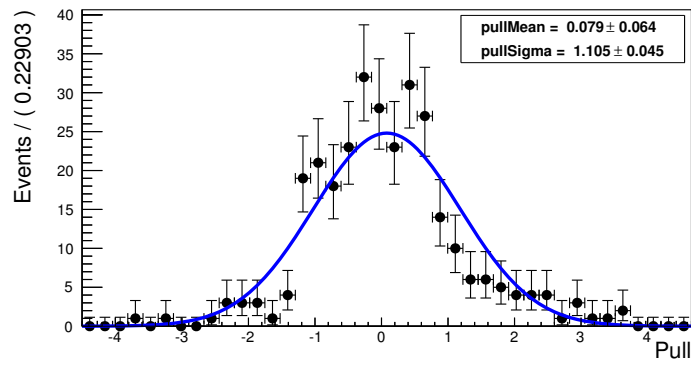
Figure 3.19: Pull of the slope s1 of the first BDT exponential (see Equation 3.11).
