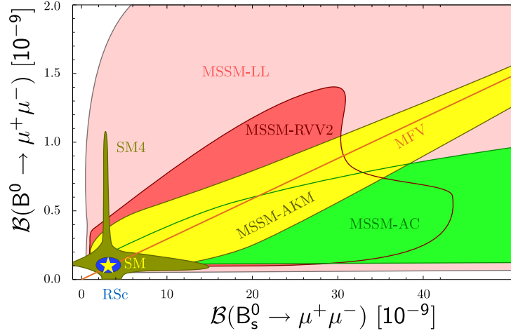
Figure 1.12: Prediction for the branching fractions of B_s^0 \rightarrow \mu^+ \mu^- and B^0 \rightarrow \mu^+ \mu^- in Minimal Flavour Violation models (MFV, see Section 1.5.2), the SM with a fourth generation (SM4, see Section 1.5.2), the Randall-Sundrum model (RSc) with custodial protection [60], and four Minimal SUSY favour models (MSSM), Agashe and Carone (AC) [61], Ross, Velasco-Sevilla and Vives (RVV2) [62], Antusch, King and Malinsky (AKM10) [63] and a model with left-handed currents only (LL11) [64]. The SM prediction is marked by a star [59].
