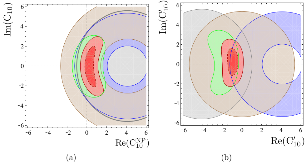
Figure 1.11: Values for the C_{10} (a) and C'_{10} (b) Wilson coefficients consistent at 1\sigma with the experimental results from B^0 \rightarrow X_s \ell^+ \ell^- (brown), B^0 \rightarrow K \mu^+ \mu^- (blue), B^0 \rightarrow K^{*0} \mu^+ \mu^- (green), \mathcal{B}(B_s^0 \rightarrow \mu^+ \mu^-) = 2.4 \pm 1.6 \times 10^{-9} (gray) and with their combination (red) at 1 and 2\sigma [26].
