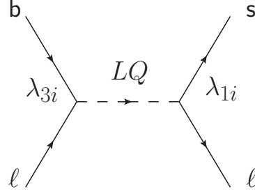
Figure 1.16: Feynman diagram for B_s^0 \rightarrow \ell^+ \ell^- mediated by a leptoquark. \lambda_{ij} are the coupling of the leptoquark between the i and j families.
