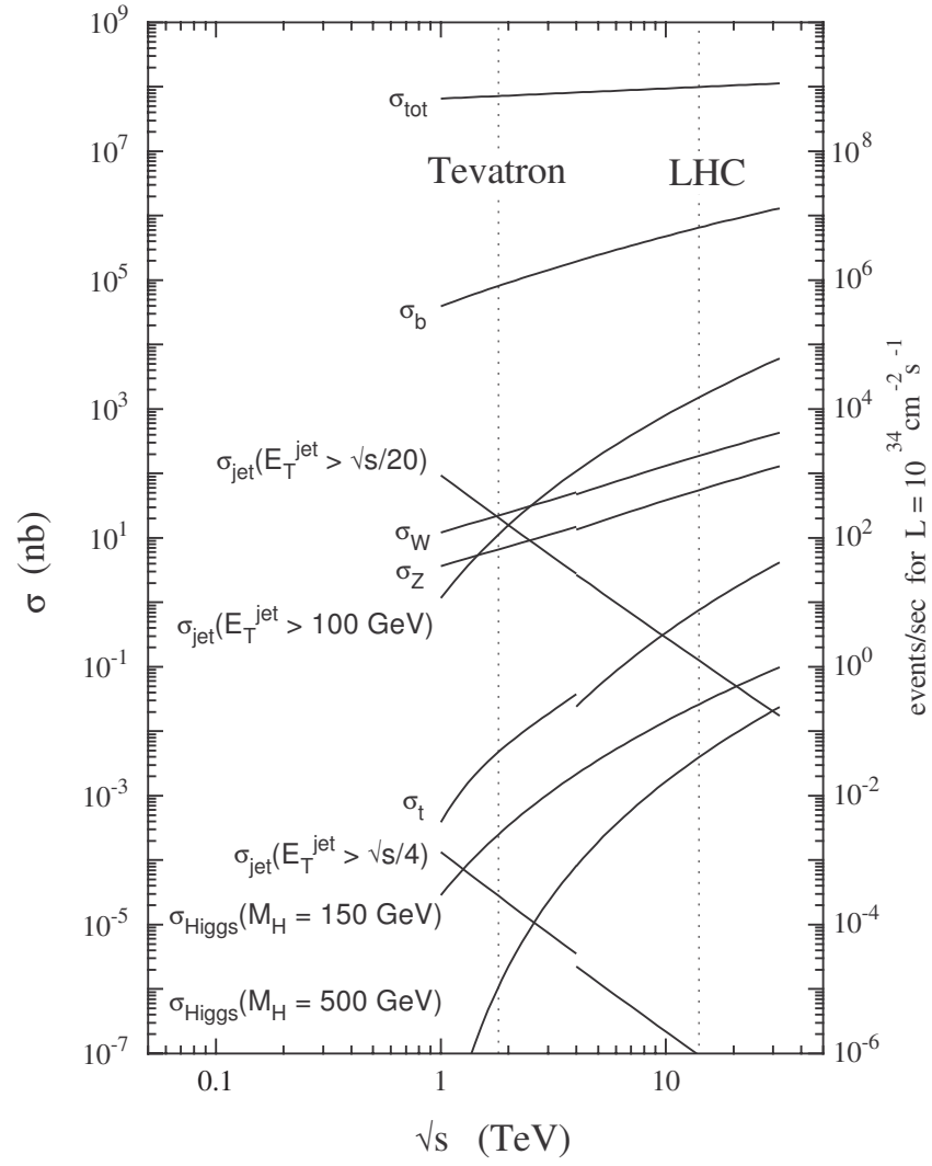
Figure 2.4: Production cross section of various processes as a function of the pp centre of mass energy.
