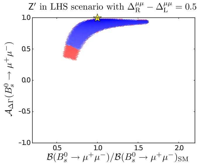
Figure 1.17: Allowed region in the plane \mathcal{B}(\mathcal{B}_s^0 \rightarrow \mu^+ \mu^-) / \mathcal{B}(\mathcal{B}_s^0 \rightarrow \mu^+ \mu^-)_{\text{SM}} \times \mathcal{A}_{\Delta\Gamma} assuming only left-handed currents, m_{Z'} = 1 \text{ TeV} , and Z' couplings between muons related as \Delta_R^{\mu\mu} - \Delta_L^{\mu\mu} = 0.5 . The two colours represent two oases of allowed values for the couplings. The star is the SM prediction [41].
