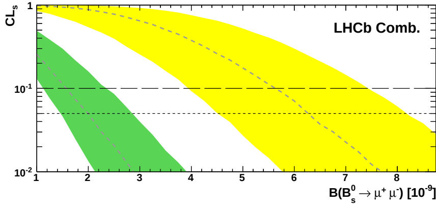
Figure 3.38: CL_s as a function of the B_s^0 \rightarrow \mu^+ \mu^- branching fraction hypothesis. The gray dashed line inlaid in the yellow (green) band is the median of the CL_s distributions obtained for each branching fraction hypothesis under the assumption of the SM signal (background only) and the band covers 34% on these distributions on each side of their median. Branching fraction hypotheses corresponding to CL_s smaller than the threshold represented by the horizontal dashed (dotted) line could be excluded at 90 (95)% C.L.
