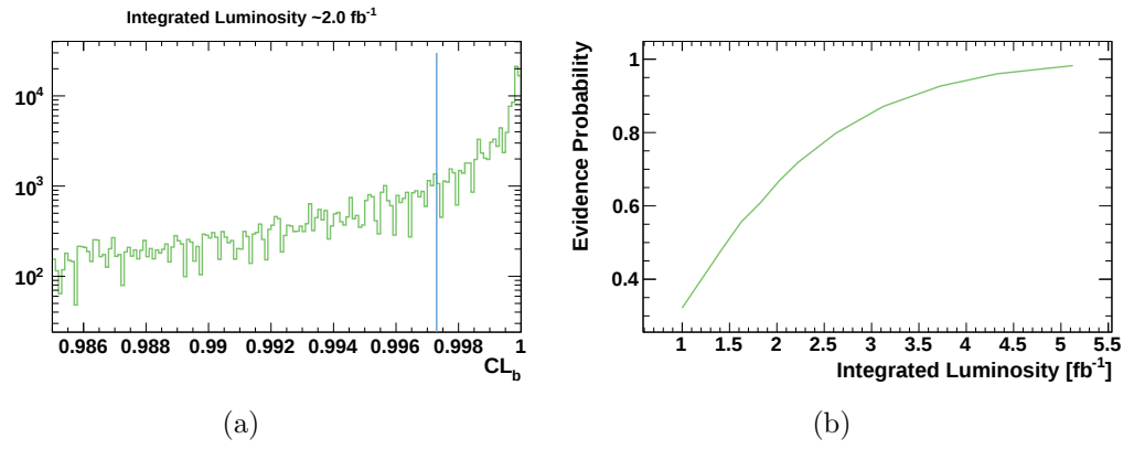
Figure 3.35: (a) CL_b distribution for pseudo-experiments generated under the assumption of a SM signal and an integrated luminosity of 2 \text{ fb}^{-1} . The vertical blue line is the CL_b value corresponding to an evidence with a significance of 3\sigma . (b) Probability of having an evidence with a significance larger than 3\sigma as a function of the integrated luminosity.
