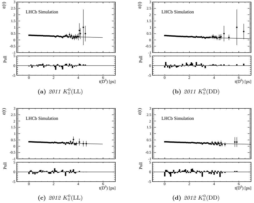
Figure 10.8.: Decay-time acceptance bias for the B^- \rightarrow D^0(\rightarrow K_S^0 \pi^+ \pi^-) \mu^- \bar{\nu}_\mu sample split by year and K_S^0 type.
