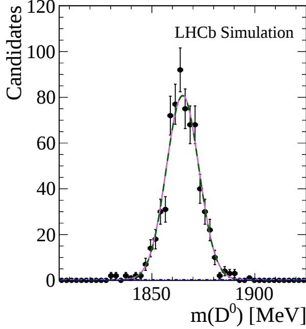
Figure 10.1.: m(D^0) distribution in the lowest m^2(\pi^+\pi^-) and \cos(\theta) bin of the 2012 K_s^0(\text{LL}) single-tagged MC sample with tight generator-level cuts after the complete selection chain. The figure depicts the fit (dashed magenta line) to the data (black points) and the fit components. The signal consists of a Gaussian function (dashed green line). The background is modelled by a constant function (solid blue line).
