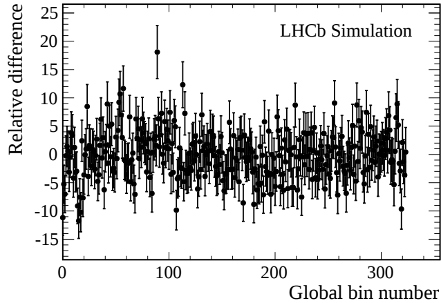
Figure 10.7.: Relative difference of the parameterised to measured double-tagged phase-space acceptance for the 2012 K_S^0(\text{LL}) MC sample with tight generator-level cuts after the complete selection chain. The global bin number is defined as follows: 0-17 corresponds to the first m^2(\pi^+\pi^-) bin with consecutive bins in \cos(\theta) , 18-35 corresponds to the second bin in m^2(\pi^+\pi^-) bin with consecutive bins in \cos(\theta) etc.
