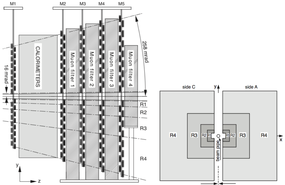
Figure 3.16.: Schematic side view of the muon stations. Figure 3.17.: Schematic front view of the muon stations. The figure is taken from Ref. [55].
