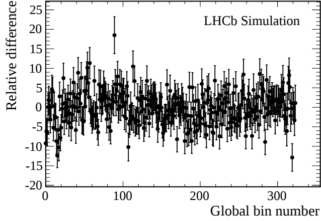
Figure 10.6.: Relative difference of the parameterised to measured single-tagged phase-space acceptance for the 2012 K_S^0(\text{LL}) MC sample with tight generator-level cuts after the complete selection chain. The global bin number is defined as follows: 0-17 corresponds to the first m^2(\pi^+\pi^-) bin with consecutive bins in \cos(\theta) , 18-35 corresponds to the second bin in m^2(\pi^+\pi^-) bin with consecutive bins in \cos(\theta) etc.
