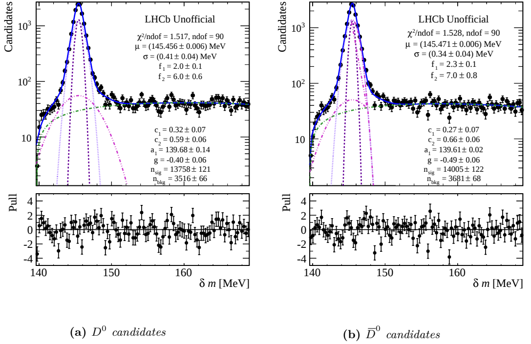
Figure 8.16.: \delta m distribution of the 2012 \bar{B}^0 \rightarrow D^{*+}(\rightarrow D^0(\rightarrow K_S^0(\text{LL})\pi^+\pi^-)\pi^+)\mu^-\bar{\nu}_\mu dataset after the complete selection split by D^0 and \bar{D}^0 . The figure depicts the fit (solid blue line) to the data (black points) and the fit components. The signal consists of a triple Gaussian function (dotted lavender line, dashed magenta line and dotted-dashed pink line) and the background is described by a polynomial (green dotted-dashed line).
