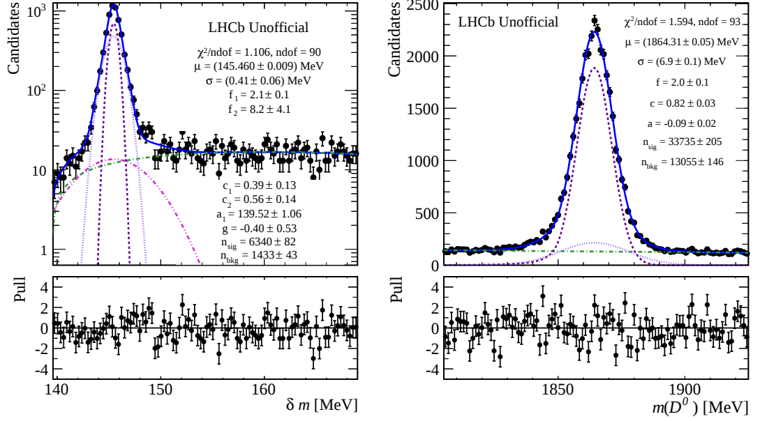
Figure 9.1.: \delta m (left) and m(D^0) (right) distribution of the 2011 D^0 \rightarrow K_S^0(LL)\pi^+\pi^- datasets after the complete selection with a D^0 tag. The figure depicts the fits (solid blue line) to the data (black points) and the fit components described in Chapt. 8.3.
