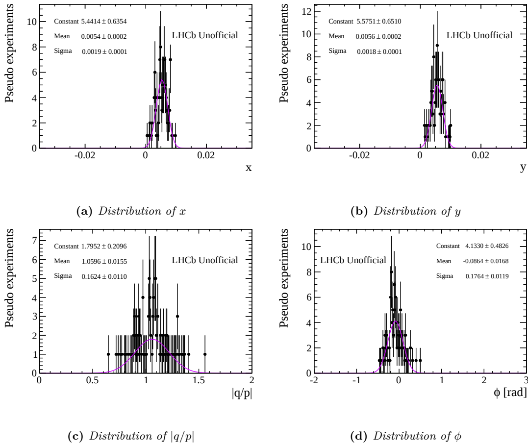
Figure 12.13.: Distribution of x , y , |q/p| and \phi fitted with a single Gaussian function.
