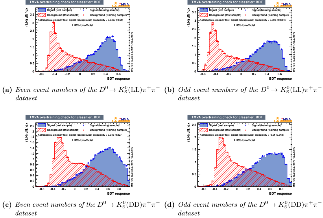
Figure 8.8.: Comparison of BDT response for both signal and background categories evaluated on the test and training samples for the 2012 B^- \rightarrow D^0(\rightarrow K_S^0\pi^+\pi^-)\mu^-\bar{\nu}_\mu datasets split by K_S^0 type and even and odd event numbers.
