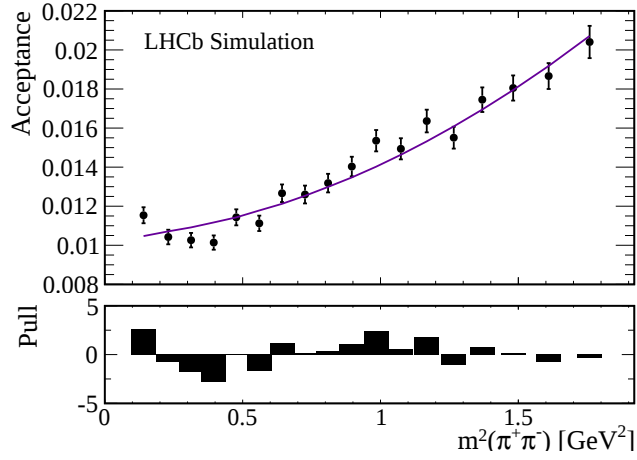
Figure 10.2.: Single-tagged phase-space acceptance as a function of m^2(\pi^+\pi^-) in the lowest \cos(\theta) bin for the 2012 K_S^0(\text{LL}) MC sample with tight generator-level cuts after the complete selection chain. The black points correspond to the measured acceptance whereas the parameterisation is depicted in purple.
