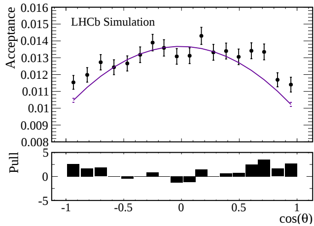
Figure 10.3.: Single-tagged phase-space acceptance as a function of \cos(\theta) in the lowest m^2(\pi^+\pi^-) bin for the 2012 K_S^0(\text{LL}) MC sample with tight generator-level cuts after the complete selection chain. The black points correspond to the measured acceptance whereas the parameterisation is depicted in purple.
