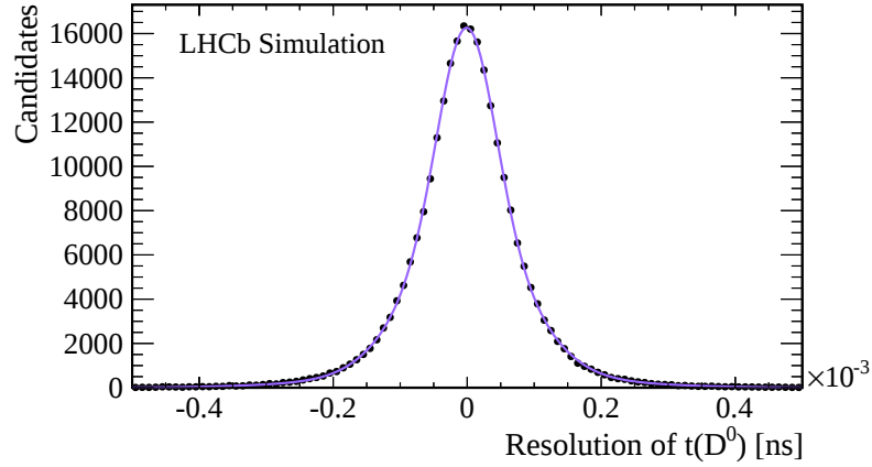
Figure 10.15.: Double-tagged decay time resolution for the 2012 K_S^0(\text{LL}) MC sample with tight generator-level cuts after the complete selection chain. The figure depicts the fit (blue line) to the data (black points).
