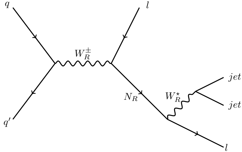
Figure 5.1: Feynman diagram of W_R decay chain.
