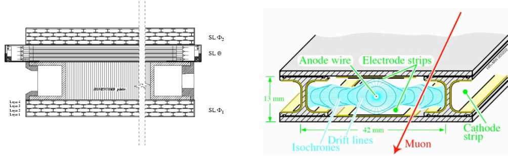
Figure 3.11: (Left) Drift tube station view in r - \phi plane. Station 4 does not have an SL\Theta SL to measure the z position. (Right) Sketch showing the drift lines inside the drift cell [38].
