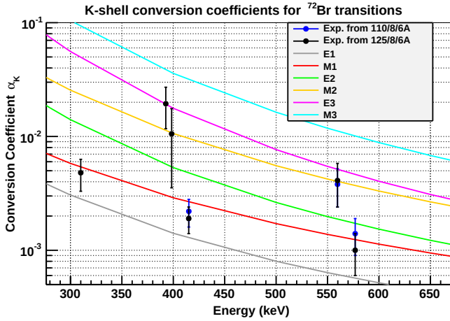
Figure D.10: Experimental conversion coefficients for K-shell transitions obtained in the high energy range with the miniorange configurations 110/8/6A and 125/8/6A. The comparison with the theoretical predictions from [ANU] is presented for the different multiplicities.
