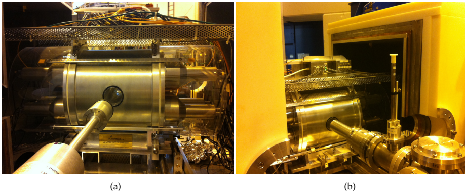
Figure 4.2: Pictures of the "Lucrecia" TAS detector installed at ISOLDE (CERN) (a) in upstream and (b) downstream directions. The transversal hole can be clearly seen in (a). The detector in the forefront of picture (a) is the HPGe telescope detector whose properties are explained in the text. There are 8 photo-multipliers located at both sides of the TAS detector that are visible in (a). The 4 layers of shielding materials made of Polyethylene, Lead, Copper and Aluminium (from outer to inner order) can be seen in (b).
