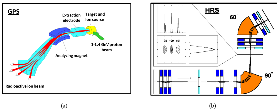
Figure 2.16: Mass separators available at the ISOLDE facility. (a) General Purpose Separator (GPS) and a sketch on the steps from the proton beam impinging the ISOLDE target until it is delivered to the experimental beam lines where the users place the setup. (b) High Resolution Separator (HRS) mode of operation. HRS provides us with better resolving power, being M/\Delta M = 5000 vs. 2400 for the GPS. Our measurements made use of the HRS.
