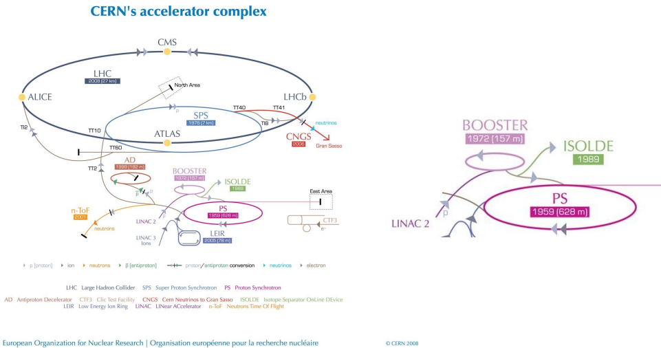
Figure 2.14: Full CERN accelerator complex as it was in 2008 and the region related with ISOLDE is expanded at the right side to better observe it. The proton beam from LINAC2 (pink) is accelerated in the Booster synchrotron up to 1.4 GeV of energy. Then, this proton beam is directed towards the ISOLDE facility where it is used to impinge on a heavy target.
