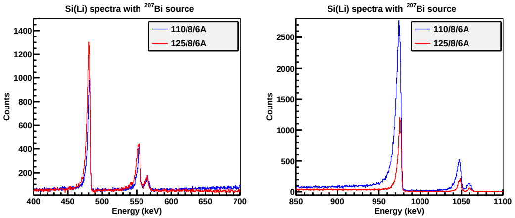
Figure 3.24: Comparison of ^{207}\text{Bi} spectra taken with the Miniorange configurations 110/8/6A and 125/8/6A in two different energy ranges, one from 400 keV up to 700 keV (left side) and the other from 850 keV up to 1100 keV (right side), where the ^{207}\text{Bi} source has its electron transitions. The transmission efficiency of configuration 125/8/6A is higher for the energy range 400-700 keV and lower for 850-1100 keV than configuration 110/8/6A as can be seen in both plots by comparing the areas of peaks 569K, 569L or 569M on the left side, and 1063K, 1063L and 1063M on the right side of the figure.
