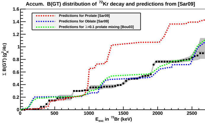
Figure D.11: Comparison of experimental accumulated B(\text{GT}) distribution for the \beta^+/\text{EC} decay of ^{72}\text{Kr} with theoretical predictions from [Sar09a] for oblate (blue), prolate (red) and dominantly oblate (green) deformations of the ground state of the parent nucleus. The mixing ratio used to roughly estimate the prediction for the dominantly oblate case is the suggested value in [Bou03] of \lambda=0.1 (mixing of 10% with the prolate first excited state at 671(2) keV). The experimental results fits fairly well with the theoretical predictions for the oblate and mixed cases as expected from information from previous theoretical and experimental works.
