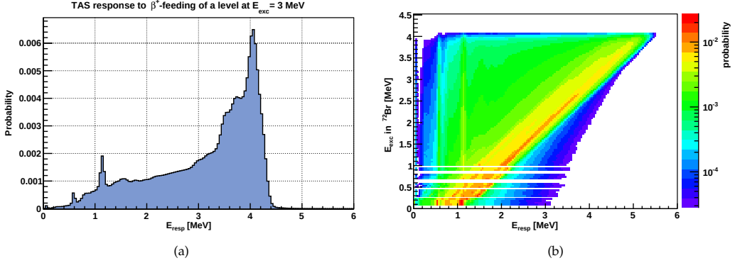
Figure 2.12: (a) The response of the TAS detector to \beta^+ feeding to a level located at E_{exc}=3 MeV is shown. This is the convolution of responses to 1 MeV positrons 2.8(a) and the \gamma de-excitation of the level at E_{exc} = 3 MeV. (b) Bi-dimensional plot of the Response Matrix of the “Lucrecia” TAS spectrometer to the \beta^+ decay of ^{72}\text{Kr} . The probability distribution is plotted versus excitation energy in ^{72}\text{Br} and the response energy in the TAS detector. Note that the Z-axis is plotted in logarithmic scale and that those bins with no response corresponds to bins in the known part of the level scheme of ^{72}\text{Br} where no levels are located. (a) is a projection of the Response Matrix shown in (b) for the particular case of feeding to a level placed at E_{exc} = 3 MeV and de-exciting as the Response Matrix of ^{72}\text{Kr} \beta^+ decay gives.
