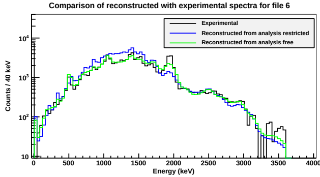
Figure 5.27: Same as fig. 5.26 for the analysis of the file 6 of the ^{72}\text{Kr} measurement. As appreciable, the restricted analysis provides worse reproduction of the experimental spectrum in this case than the free analysis.
