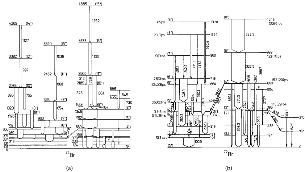
Figure 1.30: Proposed level scheme of ^{72}\text{Br} from in-beam \gamma -rays spectroscopy in [Ulb88]. (a) shows the total level scheme proposed excluding the low-energy transitions (b) describes the low-energy region up to E_{exc}=1.35 MeV.
