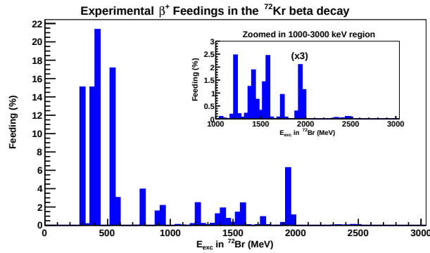
Figure D.5: \beta^+ feeding distribution shown up to the Q_{\beta^+}=4105 keV window obtained from the analysis with an upper limit in the TAS spectrum of 3640 keV in the energy for the measurement of ^{72}\text{Kr} file 1. The feedings are found up to 2620 keV for the reasons given in the text. The bin labelled with "(x3)" in the inset has the statistics reduced a factor 3.
