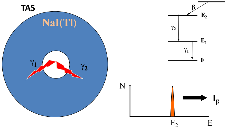
Figure 2.2: Simplified representation of how an ideal Total Absorption Spectrometer works. The individual gamma-rays emitted by the source are added and the resulting spectra shows a peak at the summed energy. Thus, by measuring the total gamma intensity one could directly deduce the beta feeding to the level located at the same excitation energy than the gamma energy detected.
