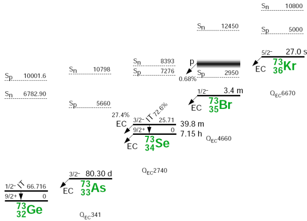
Figure 4.14: ^{73}\text{Kr} \beta^+/\text{EC} decay chain. For every decay the Q_{\text{EC}} , S_n , S_p and half life are shown. Image taken from [Fir96].
