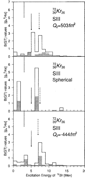
Figure 1.12: Predictions on the B(GT) distribution for the \beta^+/\text{EC} decay of ^{72}\text{Kr} from Hartree-Fock calculations in Tamm-Dancoff approximation [Ham95]. The B(GT) distribution shows to be sensitive to the nuclear shape as different B(GT) distributions are found assuming different deformations of ^{72}\text{Kr} ground state. The B(GT) distribution is calculated for 1^+ states fed in the daughter nucleus, ^{76}\text{Rb} . The solid line shows the GT strength populating both I=1^+ states, the ones with K^\pi=0^+ and the ones with K^\pi=1^+ . The shadowed distribution is just showing the B(GT) to 1^+ states with K^\pi=0^+ . Figure taken from [Ham95].
