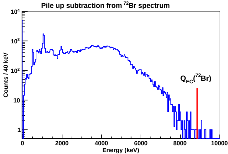
Figure 4.19: Subtraction of pile-up contribution from the ^{72}\text{Br} measurement. As can be seen, the statistics beyond the Q_{EC} ( ^{72}\text{Br} ) is negligible. For this reason the subtraction of this contribution was finally rejected.
