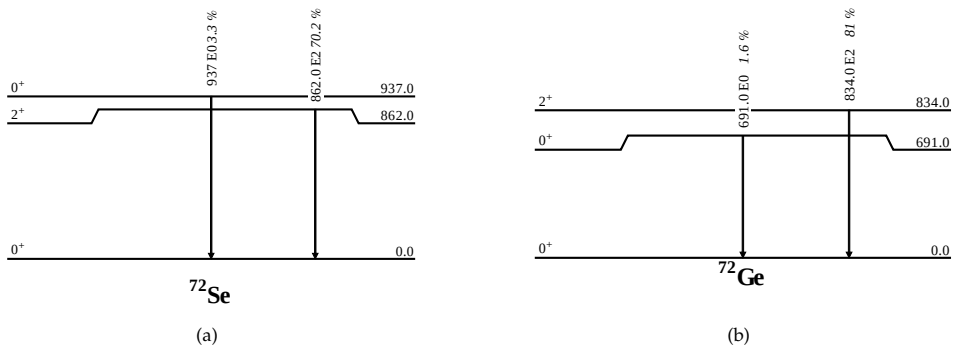
Figure 5.10: (a) Level scheme of ^{72}\text{Se} showing only the transitions involved in the discussion of the E0 intensities. The intensities are given from [Abr10] which collects the results from [Col74, Ham74] (b) Same as (a) for the ^{72}\text{Ge} with intensities taken from [Abr10] which collects the results from [Cam68, Res71].
