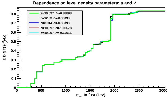
Figure 5.23: Accumulated B(\text{GT}) distributions obtained from the \beta^+ analysis of the file 1 only of ^{72}\text{Kr} \beta^+/\text{EC} decay using level schemes built in the unknown part with different values of the level density parameters a and \Delta from A.2 whose values were found to be a = 10.697 \text{ MeV}^{-1} , \Delta = -0.839 \text{ MeV} . Both parameters have been modified \pm 20\% to check its influence. Almost no dependence in these parameters was found as shown in this figure.
