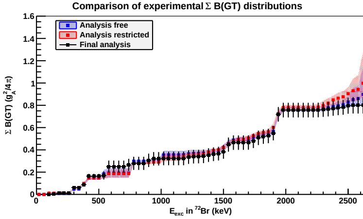
Figure F.5: Comparison of the accumulated B(GT) distributions found in the two analysis (free and restricted) already presented in chapter 5 and the resulting in the analysis here presented. As it can be seen the differences are reduced except for the last energy region where in the new analysis a smaller amount of B(GT) is found.
