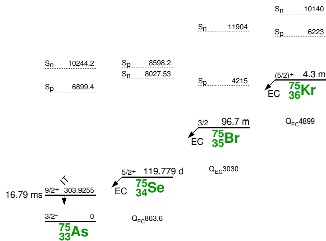
Figure 4.22: ^{75}\text{Kr} \beta^+/\text{EC} decay chain. For every decay the Q_{EC} , S_n , S_p and half life are given. Image taken from [Fir96].
