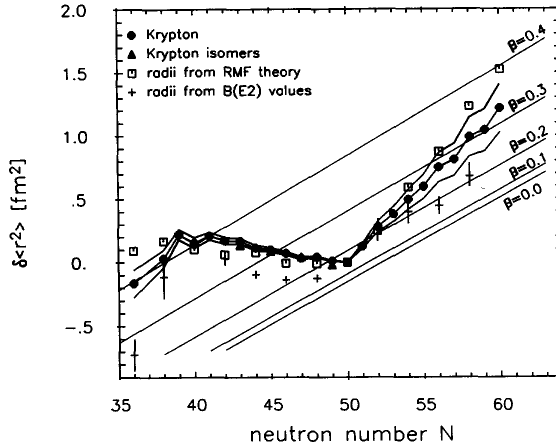
Figure 1.24: Differences of mean-square charge radii for krypton isotopes relative to ^{86}\text{Kr} taken from [Kei95]. Theoretical predictions taken from B(E2) values as given in the text and from relativistic mean-field (RMF) theoretical calculations from [Lal95] are shown. The isodeformation lines correspond to estimations from the finite-range droplet model as described in the text.
