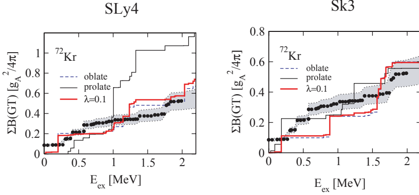
Figure 1.19: Comparison of the experimental B(GT) distribution of ^{72}\text{Kr} beta decay determined from high resolution spectroscopy [Piq03] with theoretical predictions for oblate, prolate and mixing amplitude \lambda = 0.1 deformations of the ground state of ^{72}\text{Kr} by using two different Skyrme-type two-body interactions SLy4 (left) and Sk3 (right) as given in [Sar09a]. The mixing amplitude of \lambda = 0.1 was reported by the experimental study in [Bou03].
