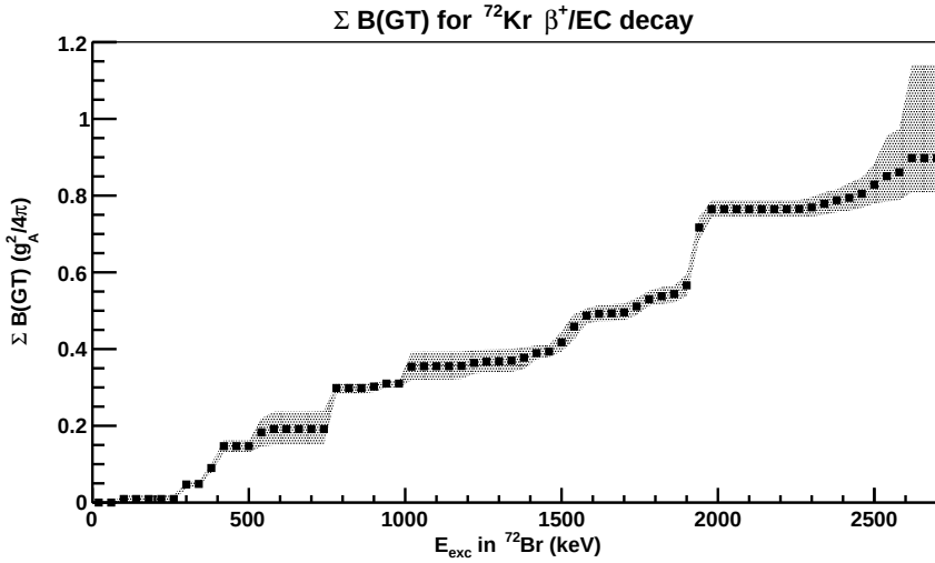
Figure D.6: Accumulated B(\text{GT}) distribution for the \beta^+/\text{EC} decay of ^{72}\text{Kr} obtained from this analysis of the \beta^+ decay component via TAS spectroscopy. The uncertainty region shown is estimated from systematic and statistical origin as described in the text.
