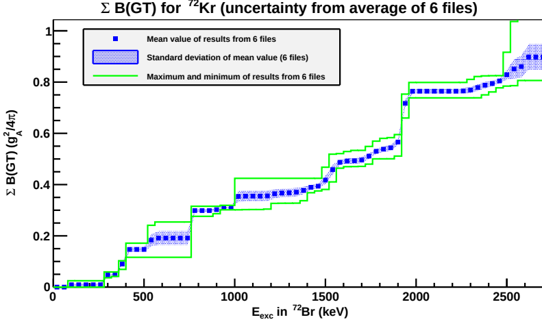
Figure 5.18: Accumulated B(GT) distribution obtained as the mean value of the result from the six files of the measurement of ^{72}\text{Kr} decay in the region 0-2640 keV. The shaded region shows the uncertainty coming from the standard deviation of the results from the six files (statistical uncertainty). The green lines indicates the maximum and minimum values for each bin of the six analyses performed. As expected, the standard deviation shows lower uncertainty that considering the maximum and minimum values given by the green continuous lines.
