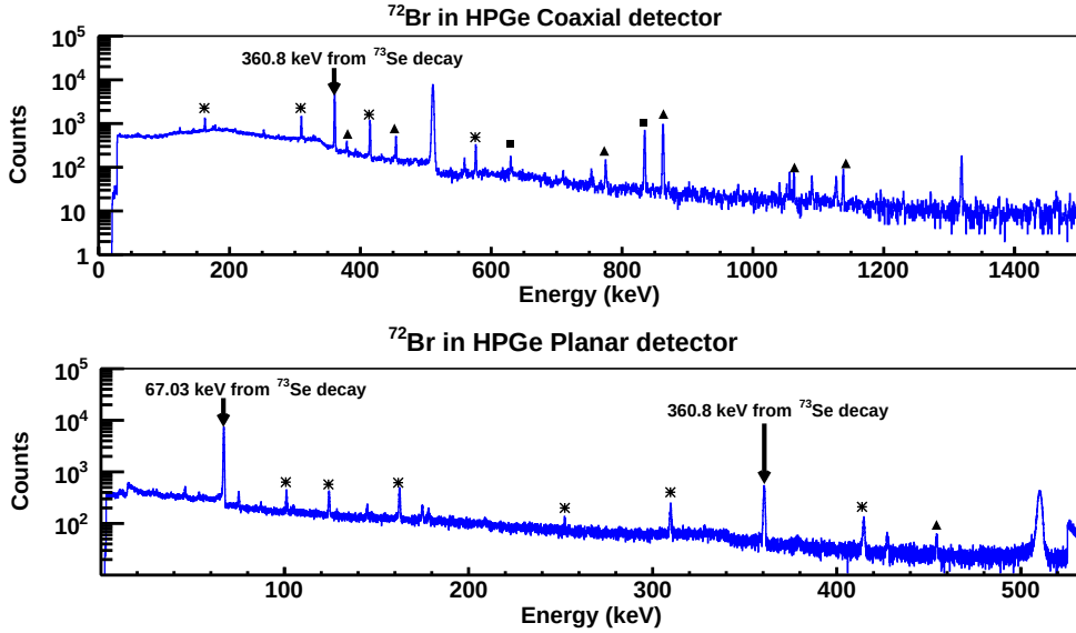
Figure 4.13: HPGc spectra from Coaxial and Planar detectors for a file with time cycles optimised for ^{72}\text{Br} measurement. Peaks marked with an asterisk (*) are coming from ^{72}\text{Kr} decay while the ones marked with black triangles ( \blacktriangle ) are from ^{72}\text{Br} decay. Contamination from the decay of ^{72}\text{As} was found and the lines at 630 and 834 keV are marked with black squares ( \blacksquare ). Apart from the expected lines from the A=72 decay chain, there are some lines from the ^{73}\text{Se} decay as, for example, the 67.03 and 360.8 keV which are labelled with arrows. This is an indication that there is presence of A=73 radiation in the surrounding area of the sample from the previous measurements where the ^{73}\text{Kr} was used as beam.
