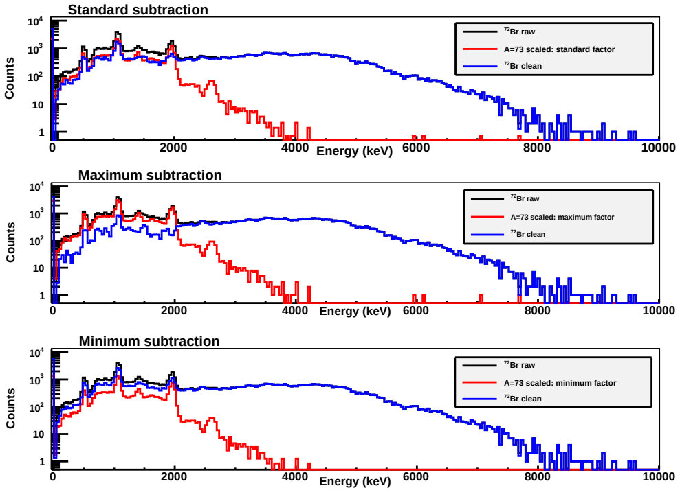
Figure 4.18: Subtraction of A=73 contamination from the ^{72}\text{Br} spectrum. There are three different subtraction factors, given in eq. 4.5, the upper one is the standard subtraction factor, the middle one is the maximum factor and the bottom one shows the minimum subtraction.
