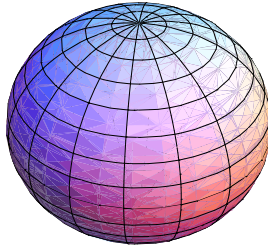
Figure 5.34: Nuclear shape of ^{72}\text{Kr} ground state calculated for a quadrupole deformation parameter of \beta_2 = -0.1759 as reported by P. Sarriguren [Sar09a]. This value corresponds to the oblate deformed local minimum obtained using the SLy4 Skyrme-type force whose theoretical accumulated B(\text{GT}) matches with the experimentally obtained as shown in fig. 5.28.
