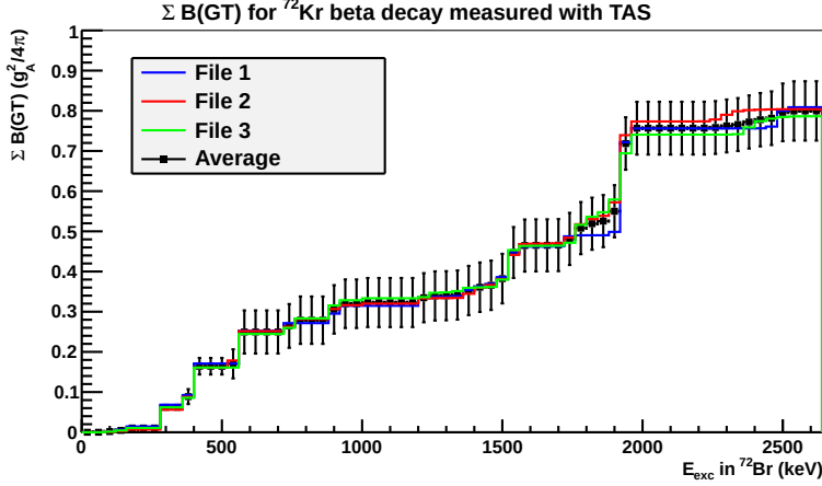
Figure F.4: Resulting accumulated B(GT) distributions from the analysis of the three files. Their similar behaviour reinforce the reliability of the final result.
