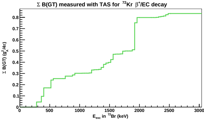
Figure 5.15: Accumulated B(GT) distribution obtained from the analysis of the \beta^+ component of the ^{72}\text{Kr} \text{EC}/\beta^+ decay with the data corresponding to the file 1 of the ^{72}\text{Kr} measurement.
