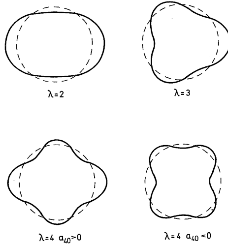
Figure 1.5: Nuclear distortions from spherical shape for quadrupole ( \lambda = 2 ), octupole ( \lambda = 3 ) and hexadecapole ( \lambda = 4 ) deformations. Image taken from [Rin80].
