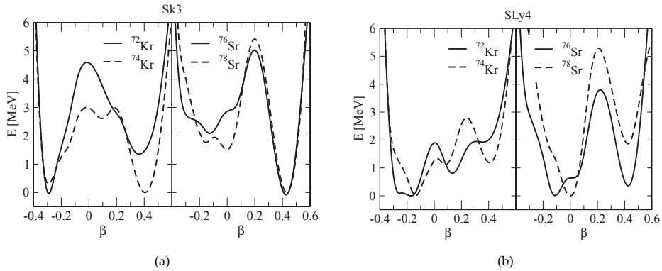
Figure 1.18: (a) Potential energy curves obtained for ^{72,74}\text{Kr} (left) and ^{76,78}\text{Sr} (right) from a constrained HF plus BCS calculations using Sk3 Skyrme-type force [Sar09a]. (b) Same as (a) but using the SLy4 Skyrme force. For more details see text. \beta is the quadrupole deformation parameter which is usually noted as \beta_2 .
