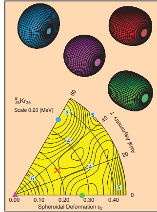
Figure D.2: Potential energy surfaces for ^{72}\text{Kr} with respect to \varepsilon_2 and \gamma parameters obtained from a macroscopic-microscopic calculation [Mö09]. Equipotential lines are distanced 0.2 MeV. The numbers indicate the energy in MeV corresponding to the line on top of which they are placed. Several energy minima, indicated with blue, green, red and violet markers, are found corresponding to different shapes, blue, green, red and violet shapes shown in the upper part of the plot. This is a sign of shape coexistence when these minima are close in excitation energy as in this case.
