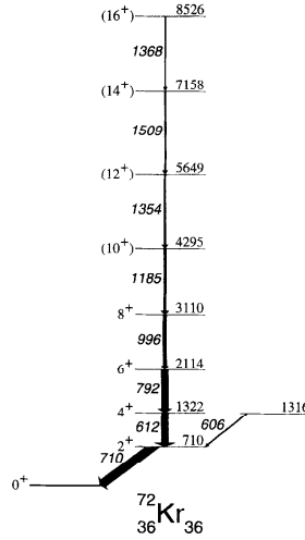
Figure 1.23: Proposed level scheme of ^{72}\text{Kr} from [de 97].
