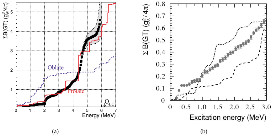
Figure 1.16: (a) Comparison of the experimental accumulated B(GT) distribution with theoretical predictions for ^{76}\text{Sr} from [Sar01] where the prediction for oblate is plotted with blue line and prolate in red [Ná04b]. (b) Same as (a) for ^{74}\text{Kr} ground state where the prediction for oblate is plotted with dotted line and for prolate as a dashed line [Poi04].
