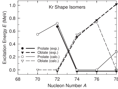
Figure 1.11: Systematics of shape isomers states in ^{72,74,76,78}\text{Kr} as given in [Mö09]. An excellent reproduction of level energies is found except for the case of ^{78}\text{Kr} .
