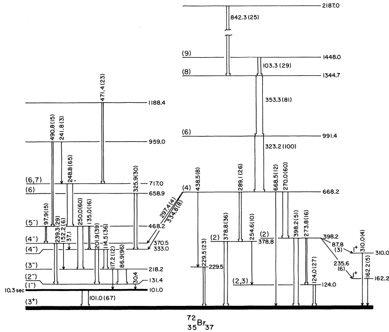
Figure 1.28: Proposed level scheme of ^{72}\text{Br} from high-spin studies from ^{58}\text{Ni}(^{16}\text{O},np)^{72}\text{Br} reaction. Figure taken from [Gar82].
