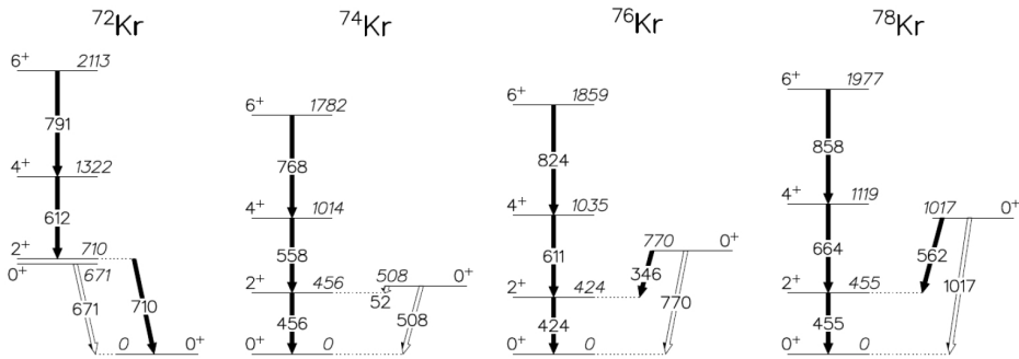
Figure 1.10: Systematics of low-lying states in ^{72,74,76,78}\text{Kr} taken from [Cle11]. The position of the first excited 0^+ state understood as the band head with different deformation is given. Note as ^{72}\text{Kr} is the only case having as the first excited state the 0^+_1 whereas for the rest is the 2^+_1 state.
