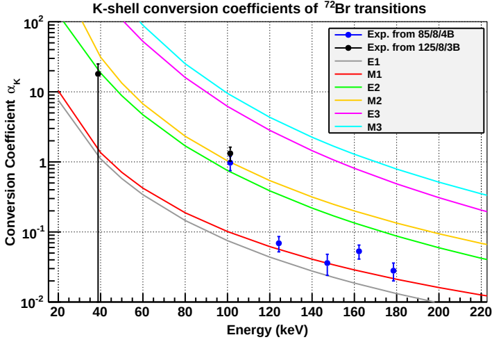
Figure 5.1: Experimental conversion coefficients for K-shell transitions of low energy measured with the minorange configurations 85/8/4B and 125/8/3B. The comparison with the theoretical predictions from [ANU] is presented for the different multipolarities.
