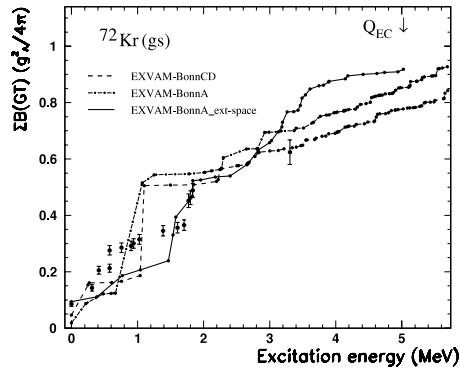
Figure 1.20: Comparison of the experimental B(GT) distribution in the beta decay of ^{72}\text{Kr} from [Piq03] with the predictions from excited VAMPIR calculations using Bonn A and Bonn CD potentials and an extended model space “ext-space” as given in [Pet11].
