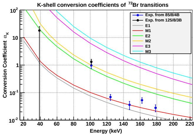
Figure D.8: Experimental conversion coefficients for K-shell transitions obtained in the low energy range with the minor-ange configurations 85/8/4B and 125/8/3B. The comparison with the theoretical predictions from [ANU] is presented for the different multipolarities.
