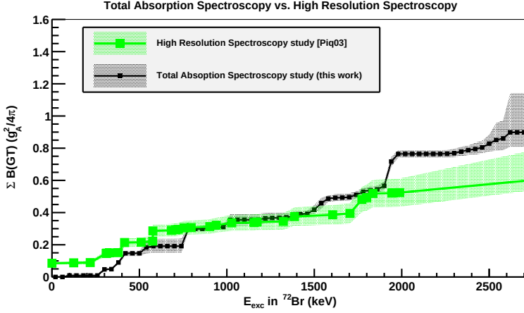
Figure 5.31: Comparison of experimental accumulated B(\text{GT}) distribution for the \beta^+/\text{EC} decay of ^{72}\text{Kr} obtained through the High Resolution Spectroscopy of I. Piqueras et al. [Piq03] in green and the Total Absorption Spectroscopy study here presented, in black. The values for the accumulated B(\text{GT}) distributions here plotted are given in table 5.9.
