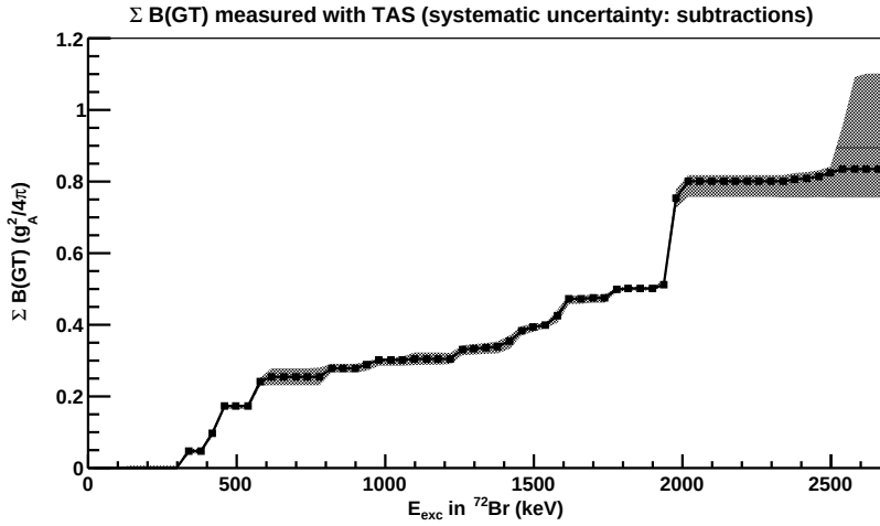
Figure 5.17: Accumulated B(GT) distribution from 0 to 2640 keV for the \beta^+/\text{EC} decay of ^{72}\text{Kr} obtained from the analysis with standard subtraction factors for file number 1. The shaded region is an attempt to quantify the uncertainty but in this case only the systematic uncertainties are included as this shaded region is limited by the maximum and minimum values of the \Sigma B(GT) obtained in the 9 analyses for each bin of 40 keV width in which the energy region was divided.
