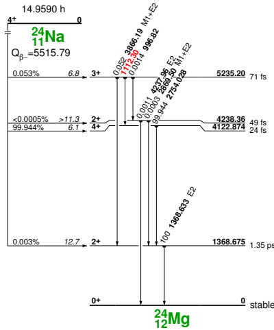
Figure 2.7: Level scheme of ^{24}\text{Na} \beta^- decay. The \beta population is almost 100 % to the level located at 4122.874 keV so the experimental TAS spectrum for this source should have a dominant peak at this excitation energy. Later, the single escape of the 2754.0 keV and 1368.67 keV gamma transitions will produce other two peaks in the experimental spectrum shown in fig. 2.6.
