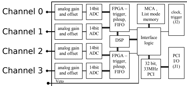
Figure 3.8: Functional block diagram of Pixie-4 data acquisition system and signal processing card. Image taken from DGF Pixie-4 Manual [DGF].
