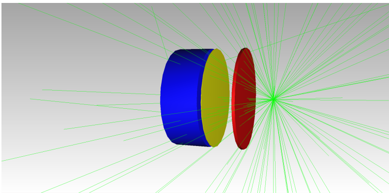
Figure 3.14: Geometric configuration of the GEANT4 simulations performed to obtain the absolute photopeak efficiency of the HPGe 1 detector. The gamma radiation is plotted in green while the mylar foil is in red. The beryllium window of the detector is represented in yellow and the germanium crystal appears in blue. The distance detector-mylar foil is known to be 2 cm but the distance mylar foil-source is not known and it is defined as 2 cm to perform the simulations. An estimation of the real value will be obtained through the fit of the simulated absolute efficiency to the experimental one (see text).
