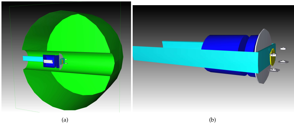
Figure 2.5: “Lucrecia”, the TAS at ISOLDE as implemented in GEANT4 simulations to obtain the response function. (a) it displays a transversal section where the NaI(Tl) crystal is shown in green with the transversal hole and the ancillary detectors and other components are plotted. (b) it shows a closer view of the rest of components located in the hole of the TAS detector. The HPGe telescope in blue, the beryllium window of the HPGe detector in white, the beta detector and its light guides in cyan, the kapton window located at the end of the beampipe in yellow and the rollers to guide the transport tape in white are shown.
