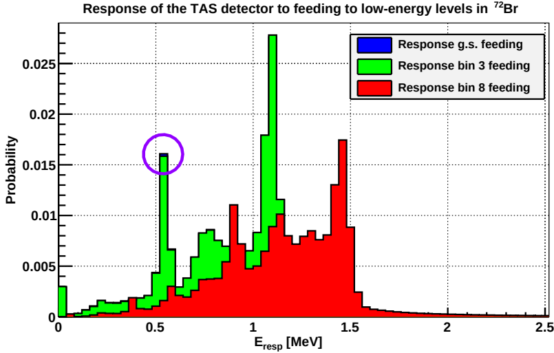
Figure 5.32: Comparison of Total Absorption Spectrometer responses to feeding at low lying levels in ^{72}\text{Br} shown as probability of contributing every spectrum bin. The response probability distribution for feeding to the ground state (blue) and to the bin 3, which only contains the 101.3-keV isomeric state (green), are almost identical. They only differ a bit in the peak at 0.5 MeV indicated with the violet circle, where the blue spectrum can be appreciated behind the green one. The response to feeding at bin 8, which includes the 310.0-keV and 313.8-keV states, is also shown in red showing that it is quite different from the others.
