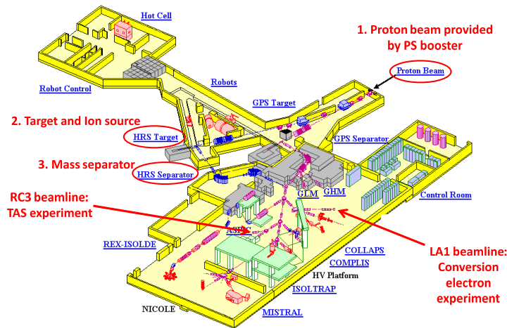
Figure 2.13: General overview of the ISOLDE facility. The main components involved in the beam preparation and leading to our experimental set-ups are indicated in red. The incoming direction of proton beam is indicated, the position of the target plus ion source and the HRS mass separator are marked in red. The location of the experimental set-ups for the two experiments, the conversion electron experiment described in chapter 3 was performed at LA1 beamline, and the Total Absorption Spectroscopy experiment described in chapter 4 was located at the TAS beamline.
