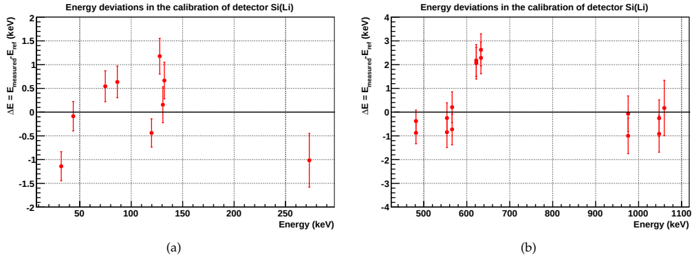
Figure 3.12: Difference of the calibrated energies for the transitions included in the energy calibration of Si(Li) detector with respect to the reference values from [Sin06], [Far99], [Sin95] and [Mar93]. It has been performed in two different energy ranges, 0-400 keV (a) and 400-1100 keV (b). Plotted values are from the table 3.7.
