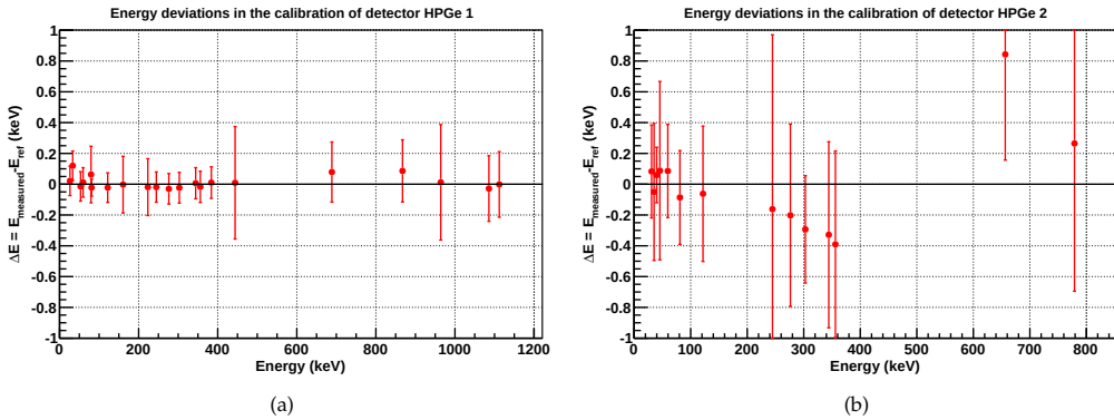
Figure 3.11: (a) Difference of the calibrated energies for the transitions included in the energy calibration of HPGe 1 detector with respect to the reference values from [Art96] and [Rab95]. Plotted values are from the table 3.5. (b) Same as (a) but for HPGe 2 with the values in table 3.6 and taking the reference values from the same sources.
