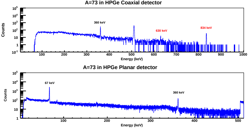
Figure 4.16: HPGe spectra for the A=73 measurement. The upper spectrum corresponds to the HPGe coaxial detector and the lower one to the HPGe planar. In the planar detector only the 67 and 360 keV transitions belonging to the ^{73}\text{Se} decay are identified while in the coaxial spectrum also are found two transitions (630 and 834 keV) belonging to the ^{72}\text{As} decay, the ones labelled in red.
