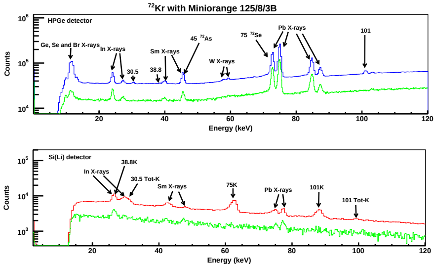
Figure 3.27: Spectra acquired with a ^{72}\text{Kr} beam and the 125/8/3B Miniorange spectrometer with the HPGe 1 detector (top-blue) and Si(Li) detector (bottom-red) during 37 and 40 minutes live time respectively. Shown in green, the spectra of the background measurement scaled to the same live time of the in-beam measurement in order to be able to identify possible background contaminations. Labels indicate the origin of each line and when only the energy is indicated, such as 101 keV or 30.5 keV, it belongs to the de-excitation of the decay daughter nucleus of interest, ^{72}\text{Br} .
