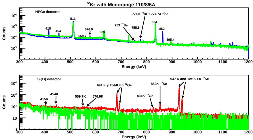
Figure 3.29: Spectra acquired with a ^{72}\text{Kr} beam and the 110/8/6A Miniorange spectrometer with the HPGe 1 detector (top-blue) and Si(Li) detector (bottom-red) during 281 and 289 minutes live time respectively. Shown in green the spectra from the background measurement in both detectors in order to identify possible background contaminations. Background spectra have been scaled to the same live time as the in-beam measurement except the Si(Li) that has been reduced a factor 0.3 in order to be able to clearly observe the in-beam spectrum. Labels indicate the origin of each line. Peaks where only the energy is indicated, such as 415 keV or 576.9 keV belong to the de-excitation of the daughter nucleus of interest, ^{72}\text{Br} , with the exception of the well known 511 peak seen in the HPGe 1 spectrum, which is coming from the annihilation of the positron emitted in the \beta^+ decay process.
