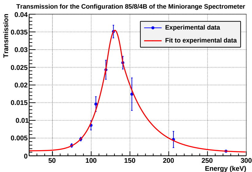
Figure 3.18: Transmission curve for the configuration 85/8/4B of the Miniorange spectrometer. The experimental data are the values from table 3.17. As in the current analysis it is necessary to obtain the transmission for the whole energy range, the experimental data have been fitted in order to interpolate the value of the transmission. The error bars have been estimated to be 20% of the the transmission value ( \pm 20\% ) in order to be of similar amplitude than the experimental data points.
