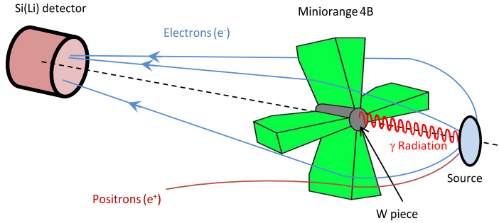
Figure 3.5: Sketch of the Miniorange spectrometer composed by a Si(Li) detector and a set of magnets. The central piece of tungsten (W piece) stops the direct gamma and X-rays coming from the source while the set of magnets focuses the electrons (and de-focuses the positrons) to the Si(Li) detector in order to improve the electron detection efficiency (avoiding positrons to reach the detector).
