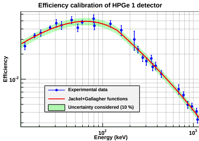
Figure 3.15: Final efficiency calibration of HPGe 1 detector obtained by fitting the experimental data (blue dots) to Gallagher [Gal74] and Jäckel [Jä87] functions. The shaded region shows the uncertainty takes into account for the interpolation of the efficiency of this detector (10% of the efficiency value).
