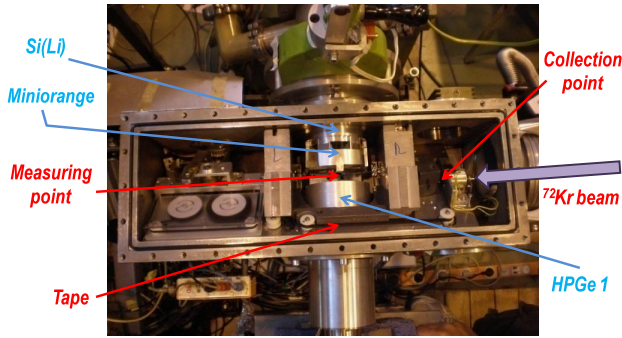
Figure 3.1: Top view of the experimental setup of the IS370-A experiment at ISOLDE (CERN). The transportation tape collects the ^{72}\text{Kr} nuclei in the collection point. After one step of tape movement, this sample is located in the measuring point where it is surrounded by the electron spectrometer, composed by a Miniorange spectrometer and a Si(Li) detector and the HPGe 1 detector. There are two Lead pieces, labelled with L and R in the picture, in order to shield the measurement position of radiation coming from outside as, for example, the collection point or the rollers where the tape was stored after a collection-measurement cycle was completed (white rollers at the left part of the station).
