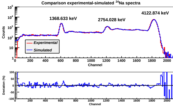
Figure 2.6: Comparison of experimental and simulated TAS spectra corresponding to a ^{24}\text{Na} source in the upper panel and the residuals in the lower. The peaks are labelled with their corresponding excitation energy in ^{24}\text{Mg} . The higher energy one comes from the decays where the two \gamma -rays of the cascade (2754.028 and 1368.633 keV) are detected depositing their full energy and the other two peaks correspond to the cases where one of these \gamma -rays escape from the TAS detector and the other is fully absorbed. The experimental spectrum presented here is beta gated (coincidence condition imposed with a signal in the beta detector) in order to reject all the possible background contaminations and pile-up removed as explained in the text. The deviations between simulation and experimental data are quite limited in the whole energy range up to when the statistics is around 1 count per bin and the deviations are enlarged from small fluctuations in statistics.
