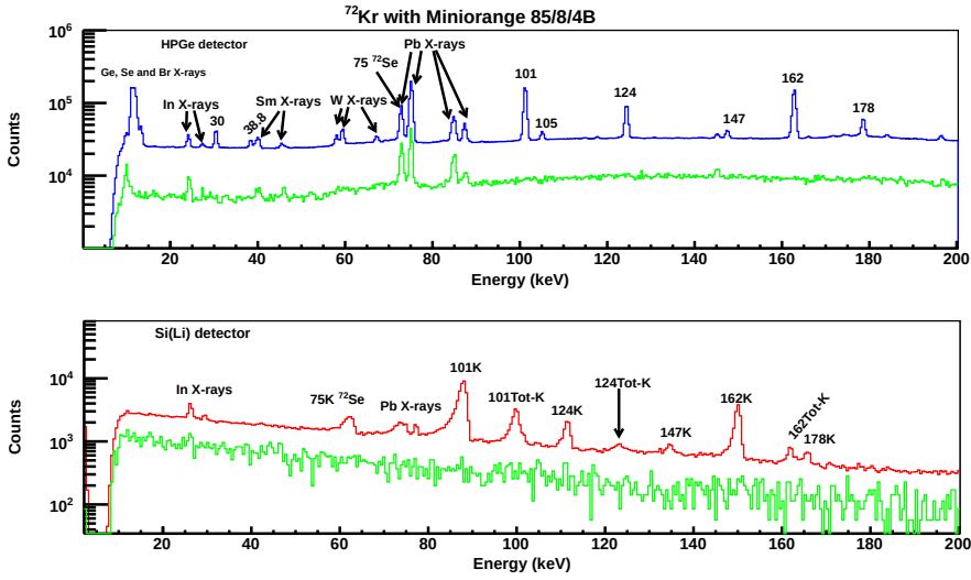
Figure 3.28: Spectra acquired with a ^{72}\text{Kr} beam and the 85/8/4B Miniorange spectrometer with the HPGe 1 detector (top-blue) and Si(Li) detector (bottom-red) during 357 and 375 minutes live time respectively. Shown in green the spectra from the background measurement in both detectors in order to identify possible contaminants. Background spectra have been scaled up to the same live time of the in-beam measurements. Labels indicate the origin of each line. Peaks where only the energy is indicated, such as 101 keV or 30.5 keV, belong to the de-excitation of the daughter nucleus of interest, ^{72}\text{Br} .
