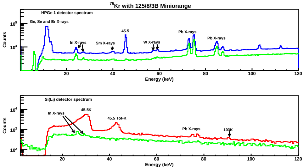
Figure 3.19: Spectra taken using the Miniorange configuration 125/8/3B with the HPGe 1 detector (top) and Si(Li) detector (bottom) with a ^{76}\text{Kr} beam. Green spectra are the same detector spectra for a background measurement carried out just before the real measurement in order to identify possible background contaminants. These background spectra are scaled in order to correspond to the same live time that the in-beam measurement.
