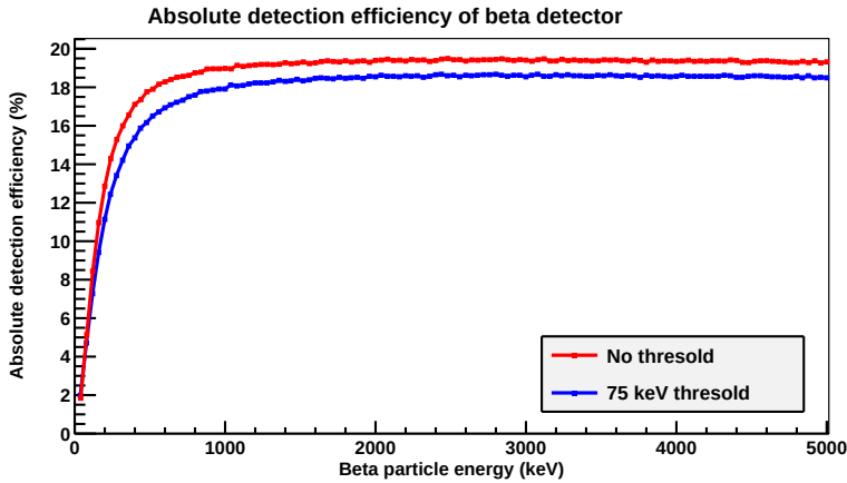
Figure 4.8: Absolute detection efficiency of the \beta detector simulated using the GEANT4 simulation code. The red curve is the absolute detection efficiency assuming that the energy threshold of detection is 0 keV. The blue curve corresponds to the case where we require a minimum energy deposited in the \beta detector of 75 keV. This energy threshold has been used in our analysis to remove the electronic noise that appears at low energies in the experimental spectra.
