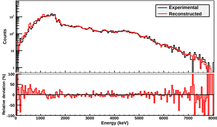
Figure F.1: Comparison of experimental and reconstructed \beta -gated TAS raw spectra for the analysis of file 1. The upper panel shows the histograms and the lower panel the relative deviation.
