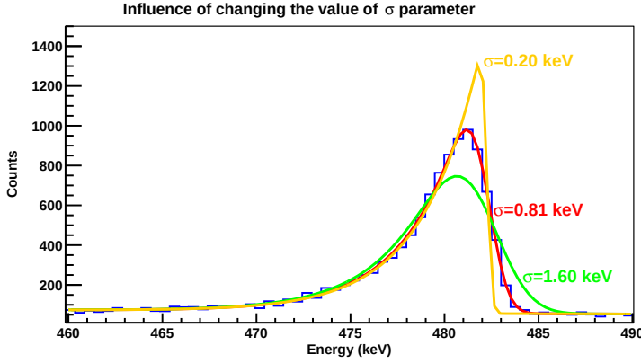
Figure 3.10: Example illustrating the influence of varying the value of parameter \sigma between 0.2 and 1.6 keV in the fit to the peak shown in figure 3.9 keeping the rest of parameters fixed. As a conclusion, this parameter provides information on the resolution of the detector as when it is changed to higher values the width of the function increases causing the resolution to be worse. However, when changed to lower values the resolution would be better as the width of the function is lower. So, this parameter can be taken as equivalent to the usual parameter \sigma of a gaussian function taken to express energy resolutions by means of the FWHM of the peak obtained as FWHM \approx 2.35 \cdot \sigma .
