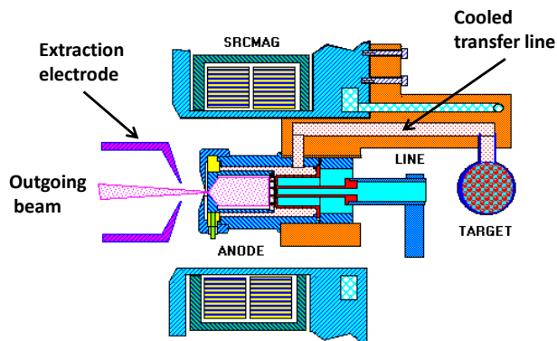
Figure 2.15: Plasma Ion Source with cooled Transfer Line taken from ref. [Iso]. The particles diffused out from the target travel along the cooled transfer line up to reach the Plasma Ion Source. Then the ionised fragments are extracted through the extraction electrode which applies a 60 kV voltage.
