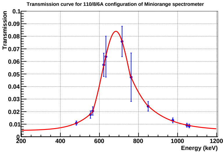
Figure 3.23: Transmission curve of the 110/8/6A Miniorange configuration. As described in the text, transitions from ^{74}\text{Se} , ^{207}\text{Pb} and ^{72}\text{Se} are considered (see table 3.22). The red line is the result from the fit of the data from table 3.21 separated in four energy ranges with the expressions and parameter values given in table 3.21.
