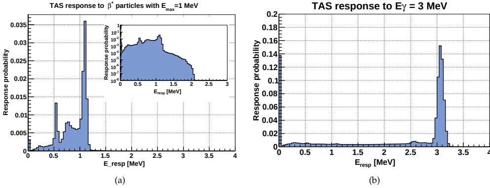
Figure 2.8: Response functions of the TAS detector to (a) positrons of E_{\text{max}}=1 MeV and (b) E_\gamma = 3 MeV. The inset of figure (a) shows the same spectrum in logarithmic scale to show the higher energy tail of the distribution that in linear scale is not visible and is due mainly to bremsstrahlung of the positron while it stops. Counts in channel number 0 in both spectra represent those events depositing less than 40 keV, which are mainly the events not interacting and depositing an energy 0.
