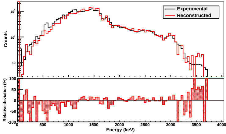
Figure F.2: Comparison of experimental and reconstructed \beta -gated TAS spectra once they are cleaned from contaminants for the analysis of file 1. The upper panel shows the histograms and the lower panel the relative deviation.
