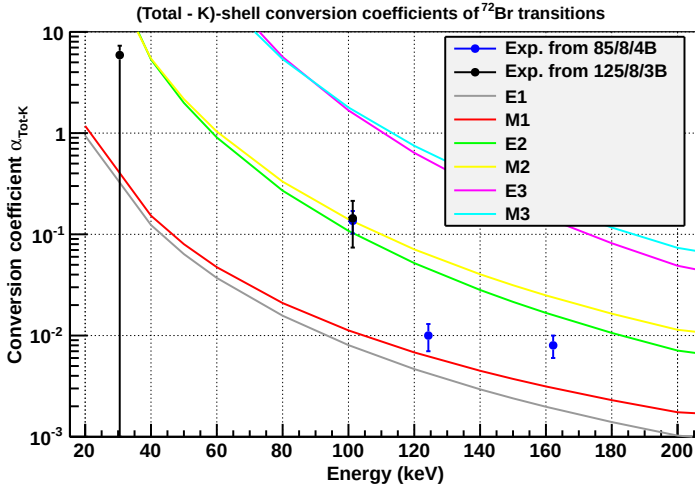
Figure 5.3: Experimental conversion coefficients for transitions of electrons coming from (Total-K)-shell obtained in the low energy range with the miniorange configurations 85/8/4B and 125/8/3B. The comparison with the theoretical predictions from [ANU] is presented for the different multipolarities.
