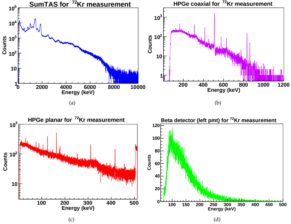
Figure 4.9: Some projections from the raw data of the first file taken of the ^{72}\text{Kr} beam as an example: (a) SumTAS spectrum: hardware addition of TAS photo-multipliers signals (b) HPGe coaxial spectrum (c) HPGe planar spectrum (d) Beta spectrum from one of the photo-multipliers coupled to the detector.
