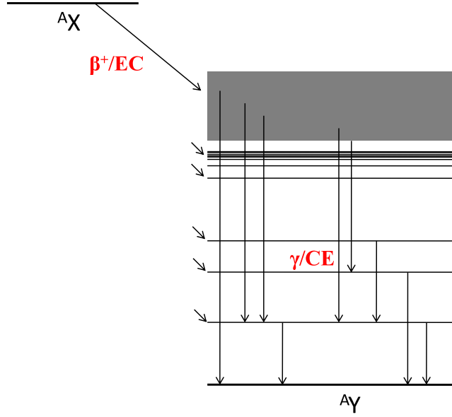
Figure 1.4: Example of the decay scheme corresponding to a \beta^+/\text{EC} decay of nucleus {}^A X leading to excited states in the nucleus {}^A Y . These excited states de-excite by means of gamma, \gamma , or conversion electron, CE, emissions.
