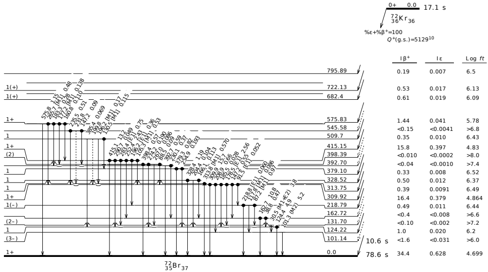
Figure 2.10: Low energy region of ^{72}\text{Br} level scheme taken from [Abr10] which is a compilation of the information for A=72 . The original work is the spectroscopy study of the ^{72}\text{Kr} \beta^+/\text{EC} decay performed by I. Piqueras et al. [Piq03].
