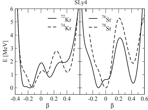
Figure 5.33: Potential energy curves obtained for ^{72,74}\text{Kr} (left) and ^{76,78}\text{Sr} (right) from a constrained HF plus BCS calculations using SLy4 Skyrme force.
