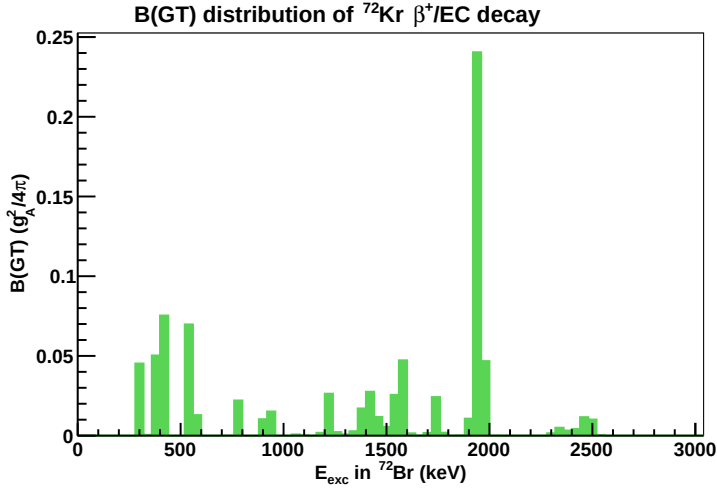
Figure 5.14: B(GT) distribution obtained from the analysis of the \beta^+ component of the ^{72}\text{Kr} \beta^+/\text{EC} decay for the file 1 of the ^{72}\text{Kr} measurement. Note that this analysis ends at 2618 keV, where the upper limit was established in the analysis (3640 keV - 1022 keV) but it is plotted up to 2640 keV where the 40-keV wide bin ends, and therefore no B(GT) can be obtained at energies higher than this value.
