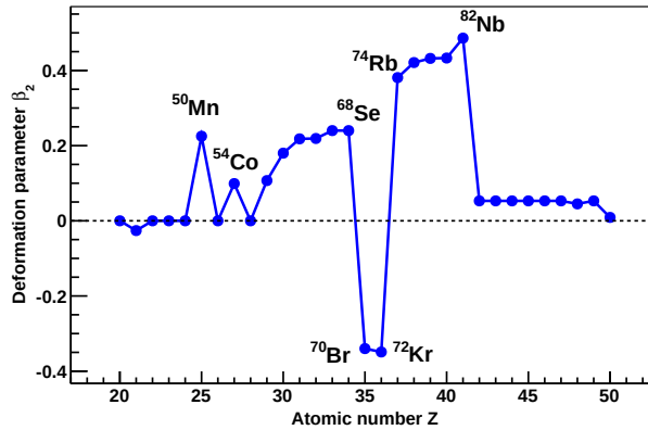
Figure 1.8: Predicted values for the quadrupole deformation parameter \beta_2 as a function of the Z number for N=Z nuclei from A=40 up to A=100 [Mö95]. The most deformed cases are labelled. Only two cases are predicted to be oblate deformed: ^{70}\text{Br} and ^{72}\text{Kr} , the nucleus of interest of the present study according with the liquid drop model calculations of P. Möller et al. [Mö95].
