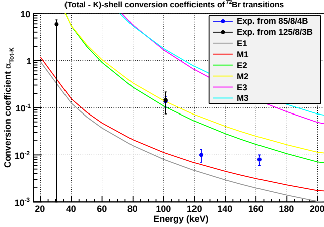
Figure D.9: Experimental conversion coefficients for (Total-K)-shell transitions obtained in the low energy range with the miniorange configuration 85/8/4B. The comparison with the theoretical predictions from [ANU] is presented for the different multiplicities.
