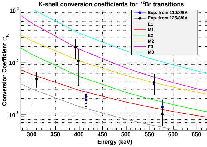
Figure 5.2: Experimental conversion coefficients for K-shell transitions of higher energy measured with the miniorange configurations 110/8/6A and 125/8/6A. The comparison with the theoretical predictions from [ANU] is presented for the different multipolarities.
