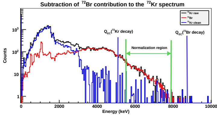
Figure D.3: Subtraction of ^{72}\text{Br} decay contribution to the file 1 of ^{72}\text{Kr} spectrum. The normalization region has been selected in the energy region from the Q_{\text{EC}} of ^{72}\text{Kr} decay and the one corresponding to the ^{72}\text{Br} decay as labelled in the plot. This energy region is supposed to have only contribution from the ^{72}\text{Br} decay as it lies beyond the ^{72}\text{Kr} Q_{\text{EC}} value.
