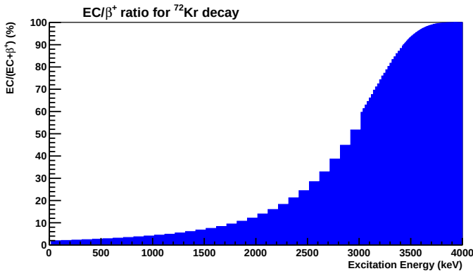
Figure 4.10: Ratio \text{EC}/(\text{EC}+\beta^+) for the \beta^+/\text{EC} decay of ^{72}\text{Kr} obtained from tables in [Gov71]. This ratio is 100 % from 4105 keV up to the full Q_\beta as the \beta^+ decay has a energy threshold in 1022 keV, so for higher energies than Q_{\text{EC}}-1022 keV there is only the possibility of EC decay. This threshold for the ^{72}\text{Kr} is at 4105 keV as the Q_{\text{EC}}=5127(10) keV. Note that from around 3 MeV of excitation energy is dominant the EC decay.
