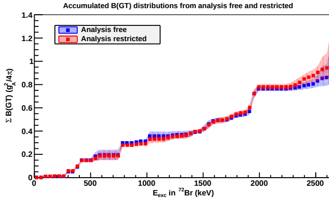
Figure D.7: Comparison of accumulated B(GT) distributions obtained from the analysis with all the feedings free (blue) and with some of them restricted (red). The trend of both results is similar and the value of the total B(GT) accumulated up to 2640 keV are similar in both analysis: B(GT)_{free} = 0.90^{+0.24}_{-0.09} (g_A^2/4\pi) and \sum B(GT)_{restricted} = 0.99^{+0.28}_{-0.12} (g_A^2/4\pi)
