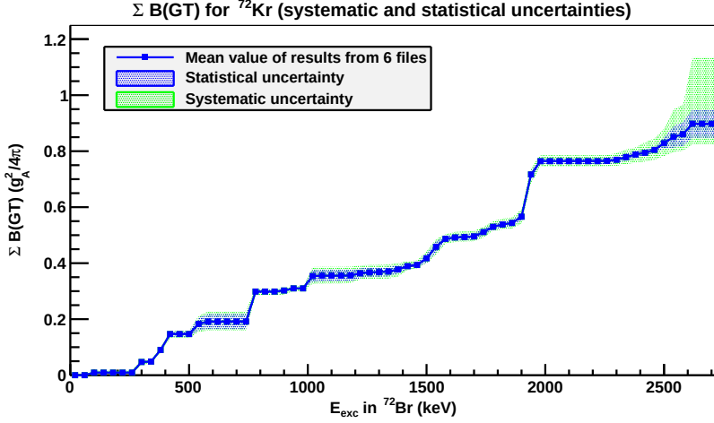
Figure 5.19: Accumulated B(GT) distribution obtained from the TAS analysis for the \beta^+ / EC decay of ^{72}\text{Kr} decay and the experimental uncertainties considered in the analysis between 0 and 2640 keV excitation energy. The statistical uncertainty is shown as the blue shaded region and is obtained as the standard deviation of the mean value of the results from the analysis of the six files measured to study ^{72}\text{Kr} , see text for further details. The systematic uncertainty has been obtained, as described in the text, by the deviation of the maximum and minimum values of the results considering the different subtraction factors from the mean value of the six analyses and is shown in the plot with the green shaded region.
