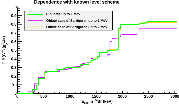
Figure 5.22: Comparison of accumulated B(GT) distributions obtained in the analysis of the TAS spectrum corresponding to the first measurement (file) of ^{72}\text{Kr} using three different known parts of the ^{72}\text{Br} level schemes. The first one is the one from the work of Piqueras et al. [Piq03] up to 1 MeV as known part, the second is the theoretically obtained from QRPA calculations of P. Sarriuren described in [Sar99, Sar01, Sar09a] considering the ground state of ^{72}\text{Kr} to be oblate deformed and the known part of the level scheme up to 1 MeV and the third is the same as the previous but the known part was considered up to 2 MeV.
