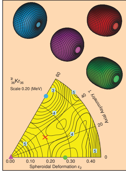
Figure 1.9: Potential energy surfaces for ^{72}\text{Kr} with respect to \varepsilon_2 and \gamma parameters obtained from a macroscopic-microscopic calculation [Mö09]. Equipotential lines are distanced 0.2 MeV. The numbers indicate the energy in MeV corresponding to the line on top of which they are placed.
