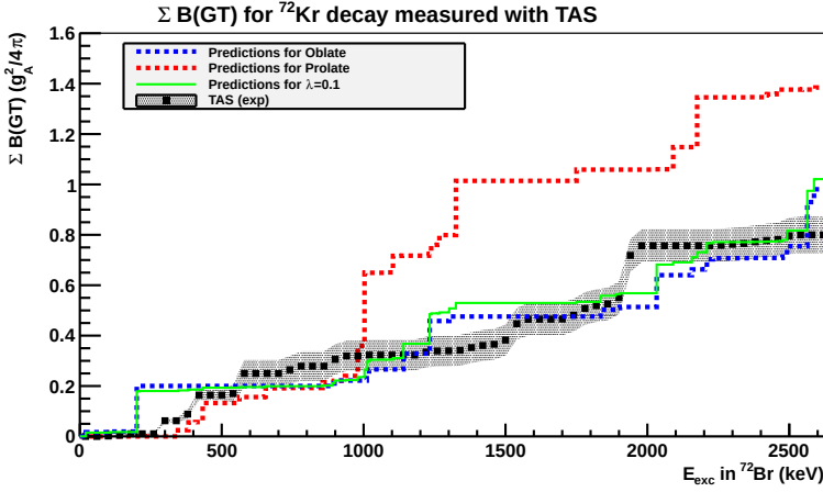
Figure F.7: Accumulated B(GT) distribution obtained from the present work in comparison with theoretical predictions from QRPA calculations [Sar09a]. Theoretical predictions for the oblate and prolate minima are found together with a rough estimation done by adding the 10% of the distribution for prolate and 90 % of the corresponding to oblate as the shape mixing suggested by E. Bouchez et al. [Bou03] is 10% with the prolate 0^+ excited state.
