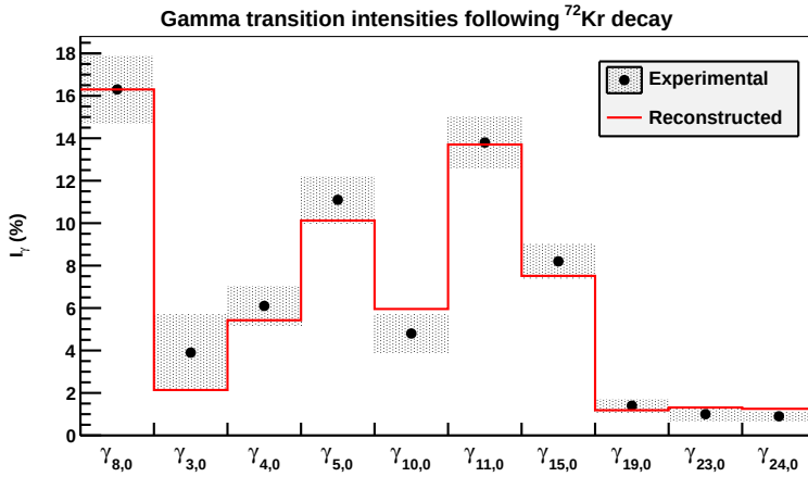
Figure F.3: Comparison of relative intensities for the most intense gamma transitions in the de-excitation of 72 Br, measured with the HPGe detector (black) and reconstructed from the beta feedings obtained in the analysis of file 1 (red). The sub-index of each gamma transition indicates the initial-final bins, to know the transitions included and the experimental values see Table F.2. The \gamma_{8,0} transition intensity is taken as the reference value of 16.3% as given by the high resolution work of I. Piqueras [Piq03].
