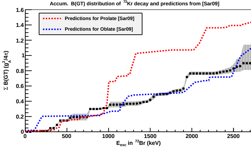
Figure 5.28: Comparison of the experimental accumulated B(GT) distribution obtained in this work for the \beta^+/\text{EC} decay of ^{72}\text{Kr} with theoretical predictions from [Sar09a] for oblate (blue) and prolate (red) deformations of the ground state of the parent nucleus. The experimental results fit fairly well the theoretical predictions for the oblate case as expected from information from previous theoretical and experimental works, see chapter 1.
