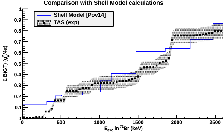
Figure F.9: Accumulated B(GT) distribution obtained from the present work in comparison with theoretical predictions from shell model calculations performed by A. Poves [Pov14].
