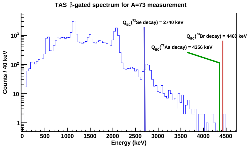
Figure 4.15: Total Absorption Spectrometer spectrum for the A=73 measurement with the \beta -coincidence condition, also known as \beta -gated TAS spectrum. The Q -values of the contributing decays are indicated.
