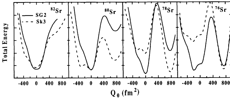
Figure 1.13: Total energy curves versus the mass quadrupole moment for ^{82,80,78,76}\text{Sr} isotopes are shown. The results correspond to a constrained HF+BCS calculation using SG2 (solid lines) and Sk3 (dashed lines) forces [Sar99]. Absolute values of total energy are not given but the tick-to-tick scale is 1 MeV. Figure taken from [Sar99].
