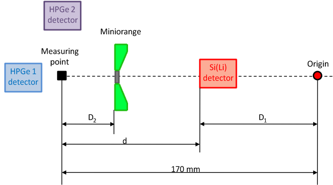
Figure 3.6: Graphical representation of the side view of the experimental setup including the description of the distances D_1 and D_2 used to label every Miniorange configuration as D_1/D_2/NT . N gives the number of magnets included in the configuration and T the type, see fig. 3.7.
