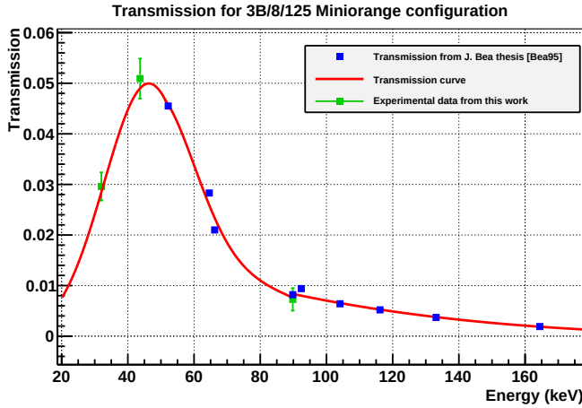
Figure 3.20: Transmission curve for 125/8/3B Miniorange. The data considered are listed in table 3.19 where only three experimental points (green dots) belong to the measurement of IS370-A experiment. The rest of the data are taken from [Bea95] (blue dots). Mathematical expressions for interpolation are obtained in three energy ranges as explained in the text.
