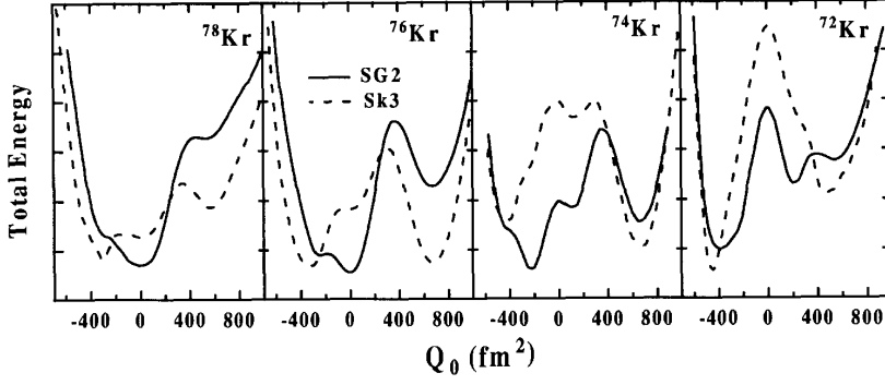
Figure 1.14: Same as fig. 1.13 for ^{78,76,74,72}\text{Kr} isotopes. Figure taken from [Sar99].
