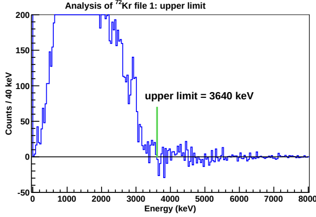
Figure D.4: ^{72}\text{Kr} clean spectrum for file 1, as example. The upper limit chosen in the analysis for the energy spectrum is shown. The reason for this choice is mainly that from this energy on the energy spectrum shows oscillations around zero counts giving negative statistics in some bins and few positive counts in others.
