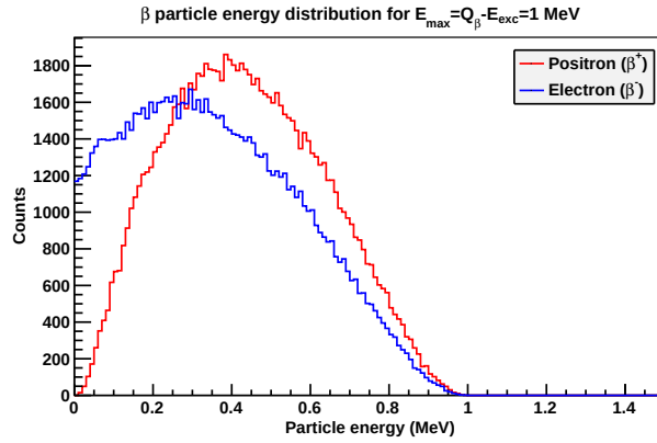
Figure 1.2: Energy distribution of a \beta particle, positron in red and electron in blue, corresponding to a decay where E_{max} = Q_{\beta} - E_{exc} = 1.0 MeV. The maximum energy carried by the positron/electron corresponds to the total energy available, 1 MeV, while the maximum of the distribution is placed at approximately one third of the maximum energy. The electron distribution is shifted to lower energies than positron one because of the Coulomb interactions with the daughter nucleus.
