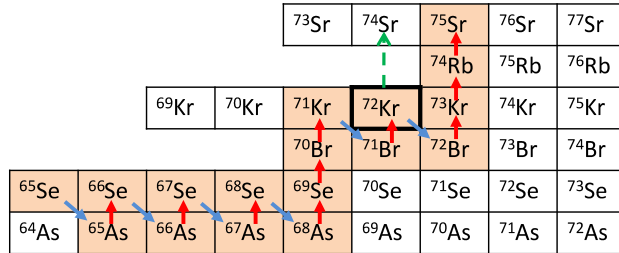
Figure 1.22: Detail of the path followed by the rp-process in the mass region of the chart of nuclides around ^{72}\text{Kr} . The proton capture process (red arrows) is leading the process towards nucleus where the proton capture is hindered by (\gamma, p) photodisintegration of weakly bound nuclei or unbound nuclei. The latter is the case of ^{73}\text{Rb} which is the following nucleus to ^{72}\text{Kr} in the proton capture path. This provokes a slowing down in the process at the level of ^{72}\text{Kr} since the possibilities to continue are a two proton capture (green arrow), a much unlikely process, or the beta decay (blue arrows) which is a much slower process. The nuclei where this occurs, as ^{72}\text{Kr} , are known as “waiting points” of the process.
