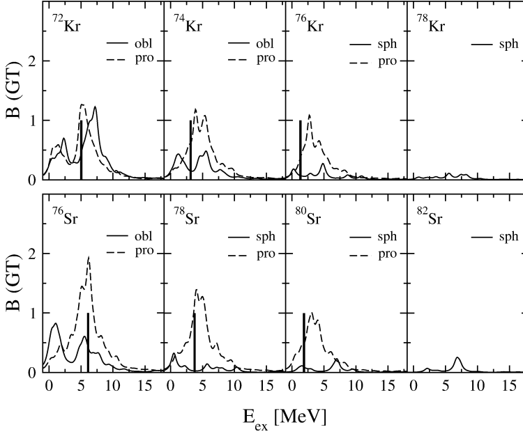
Figure 1.15: Predicted B(\text{GT}) distributions for ^{72,74,76,78}\text{Kr} and ^{76,78,80,82}\text{Sr} isotopes taken from [Sar01] and calculated for the energy minima found in figs. 1.13 and 1.14. For every nucleus, a vertical line indicates the Q_{EC} energy window available experimentally.
