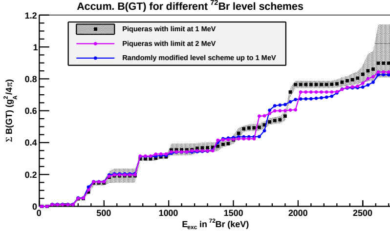
Figure 5.21: Accumulated B(GT) distributions obtained from the analysis of the \beta^+ component of the ^{72}\text{Kr} \beta^+ / EC decay using three different sets of information on the ^{72}\text{Br} level scheme: in black is taking the information from [Piq03] up to excitation energy of 1 MeV as known part, the violet one shows the result using the same set of information but taking up to 2 MeV as known part of the level scheme and the blue line was obtained using the same information on the level scheme but modifying the spin-parities of the levels randomly to 2^+ , 3^+ and 1^- spin-parities. The information from [Piq03] is listed in table 2.1.
