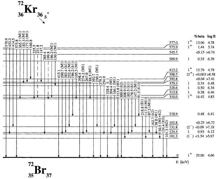
Figure 1.26: Knowledge on the ^{72}\text{Br} level scheme in the low-energy region taken from [Piq03]. As described in the text, this work consists of beta decay studies of ^{72}\text{Kr} by means of high resolution spectroscopy with HPGe, Si(Li), gas-Si telescope and \beta detectors.
