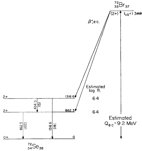
Figure 1.27: Proposed level scheme of ^{72}\text{Se} from beta decay of ^{72}\text{Br} in [Dor71].
