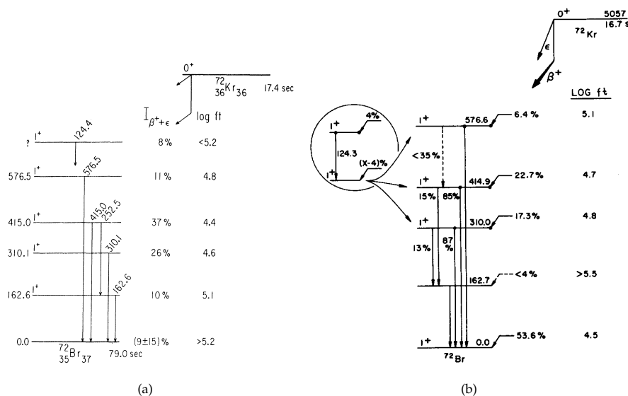
Figure 1.25: (a) Level scheme of ^{72}\text{Br} deduced from the beta decay study performed in [Dav73]. (b) Same as (a) but from [Sch73].
