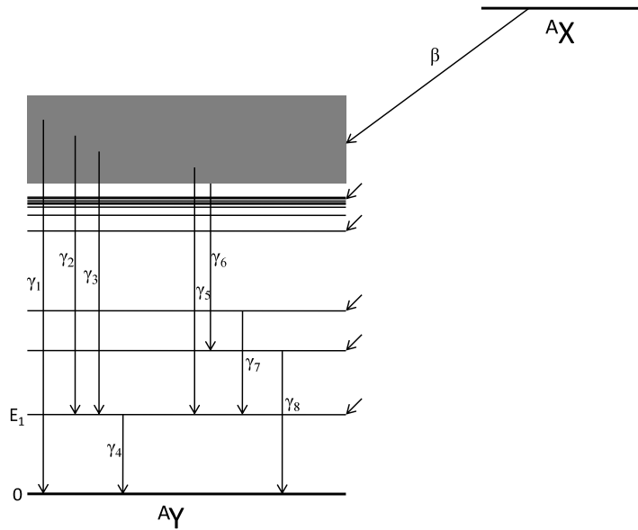
Figure 2.1: Example of the level scheme corresponding to the \beta decay of a generic nucleus ^A X leading to the nucleus ^A Y . The level density usually increases with excitation energy and this makes the beta feeding distribution to be very fragmented at high excitation energies. This, combined with a high fragmentation of the gamma de-excitation pattern and the low detection efficiency of HPGe detectors for high-energy \gamma -rays makes that, in most cases, \gamma_1 , \gamma_2 and \gamma_3 keep undetected. This would cause the wrong assignment of feeding to level at excitation energy E_1 , as \gamma_4 is very likely to be detected for being a low-energy gamma ray, provoking an overestimation of feeding at this level and an underestimation of feeding at higher excitation levels. This is the so-called Pandemonium effect [Har77].
