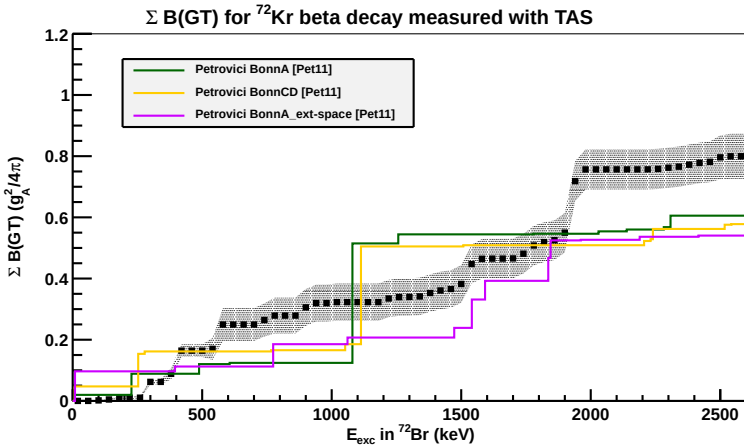
Figure F.8: Accumulated B(GT) distribution obtained from the present work in comparison with theoretical predictions from variational calculations using the VAMPIR approach [Pet11].
