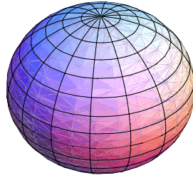
Figure D.12: Nuclear shape of ^{72}\text{Kr} ground state calculated for a quadrupole deformation parameter of \beta_2=-0.1759 as reported by P. Sarriguren [Sar09a]. This value corresponds to the oblate deformed local minimum obtained using the SLy4 force whose theoretical accumulated B(\text{GT}) associated matches with the experimentally obtained as shown in fig. D.11.
