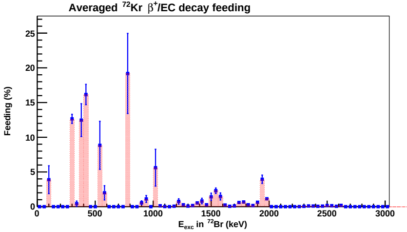
Figure 5.24: Beta feeding distribution of the ^{72}\text{Kr} decay obtained as the average of the feeding distribution from the 6 independent analyses performed with the 6 files of measurements to study the ^{72}\text{Kr} decay with free conditions in the feeding distribution.
