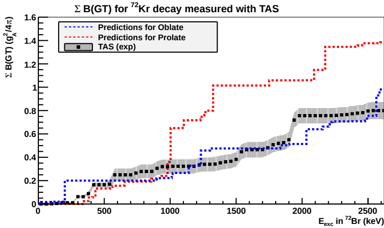
Figure F.6: Accumulated B(GT) distribution obtained from the present work in comparison with theoretical predictions from QRPA calculations [Sar09a] for oblate and prolate deformations. For more details on the theoretical framework see chapter 1 or [Sar09a].
