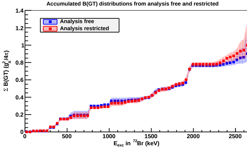
Figure 5.25: Comparison of accumulated B(GT) distributions obtained from the analysis with all the feedings free (blue) and with some of them restricted (red). The trend of both results is similar and the value of the total B(GT) accumulated up to 2640 keV are similar in both analysis: \sum B(GT)_{free} = 0.90^{+0.24}_{-0.09}(g_A^2/4\pi) and \sum B(GT)_{restricted} = 0.99^{+0.28}_{-0.12}(g_A^2/4\pi) .
