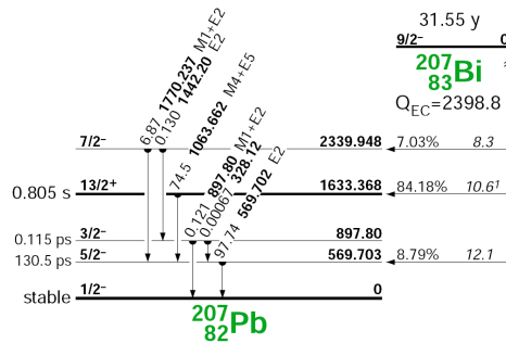
Figure 3.21: Decay scheme of ^{207}\text{Bi} take from [Fir96]. The most intense transitions are the 1063.662 and 569.702 keV transitions and as their multipolarities are quite high, M4+E5 and E2 respectively, they both show conversion electrons as can be seen in figure 3.24 that will be used for calibration purposes of the Si(Li) detector and to obtain the transmission curves of the Miniorange spectrometer. The conversion coefficients for these transitions are shown in table 3.20.
