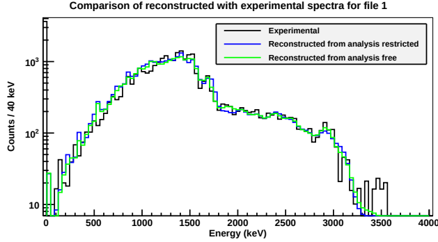
Figure 5.26: Comparison of experimental (black) with the reconstructed TAS spectra from the analysis free (green) and restricted (blue) for the ^{72}\text{Kr} measurement of file 1. The restricted analysis is done by imposing the conditions mentioned in the text on the level scheme and feeding distribution. Slightly better match is found for the free analysis (green) as given by the \chi^2 values given in table 5.7.
