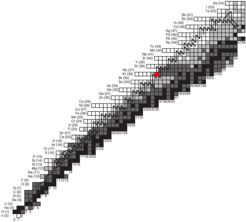
Figure 1.21: Path of the rp -process along the chart of nuclides taken from the work of H. Schatz [Sch06]. Stable nuclei are shown in black and the path followed by the rp -process is indicated with a black line. The placement of the nucleus of interest, ^{72}\text{Kr} is indicated with a red dot. Figure 1.22 shows a zoomed view of the surrounding region of ^{72}\text{Kr} . Figure taken from [Sch06]
