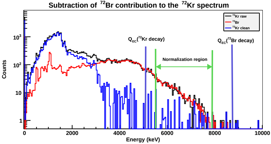
Figure 4.23: Subtraction of ^{72}\text{Br} decay contribution to the file 1 of ^{72}\text{Kr} spectrum. The normalisation region has been selected in the energy region from the Q_{EC} of ^{72}\text{Kr} decay and the one corresponding to the ^{72}\text{Br} decay as labelled in the plot. This energy region is supposed to have only contribution from the ^{72}\text{Br} decay as it lies beyond the ^{72}\text{Kr} Q_{EC} value.
