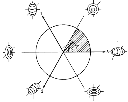
Figure 1.6: Lund convention using the nuclear deformation parameters \beta = \beta_2 and \gamma and the resulting deformations for the nucleus [Nil55]. Image taken from [Rin80].
