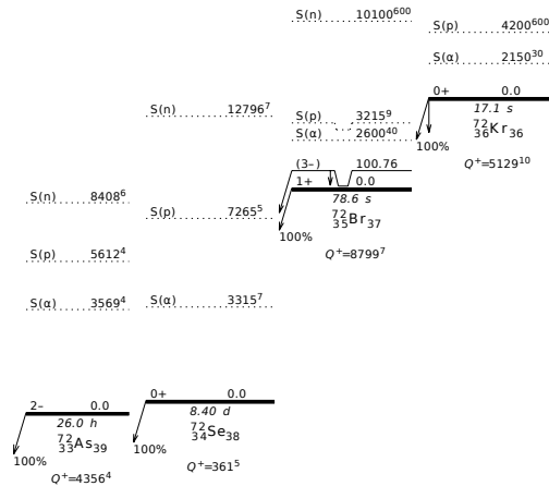
Figure 4.12: ^{72}\text{Kr} \beta^+/\text{EC} decay chain. For every decay the Q_{EC} , S_n , S_p , S(\alpha) and half life are shown. Image taken from [Abr10]. More recent measurements of the ^{72}\text{Kr} and ^{72}\text{Br} masses [Rod04, Her11] give a new Q_{EC} value for the ^{72}\text{Kr} decay of 5127(10) keV, as given in [Wan12b] and explained in sect. 1.3.4.
