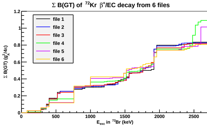
Figure 5.16: Accumulated B(\text{GT}) distribution obtained from the \beta -gated analysis of the six files measured for the study of ^{72}\text{Kr} \text{EC}/\beta^+ decay. As can be observed, there are no huge differences in the six accumulated B(\text{GT}) distributions up to 2618 keV (3640 keV - 1022 keV) where the upper limit of the analysis for the feeding distribution was set.
