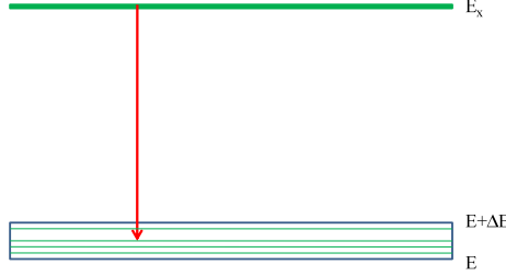
Figure A.1: Schematic example to understand how the strength of the gamma radiation is calculated in eq. A.7 for a gamma transition from a level at E_x down to levels contained in the energy interval [E, E+\Delta E] .
