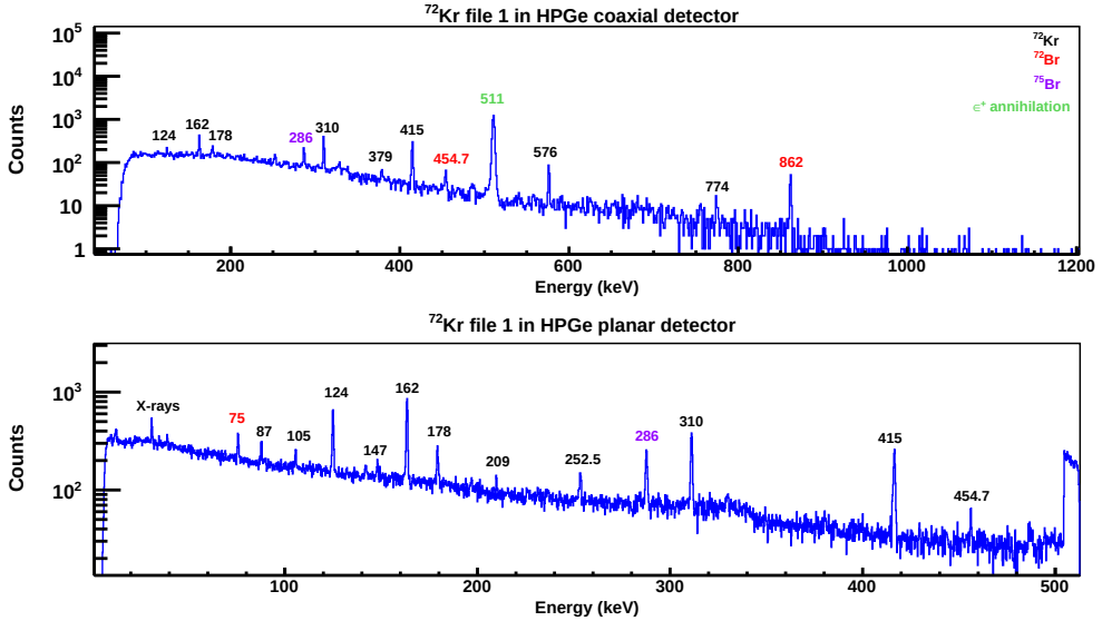
Figure 4.21: HPGe spectra for the first file with ^{72}\text{Kr} beam and cycling periods optimised for the measurement of ^{72}\text{Kr} decay. There are contaminations from ^{72}\text{Br} and also ^{75}\text{Br} decay that was just measured before this file. A quantitative analysis of the contaminants presents in the 6 files for the ^{72}\text{Kr} decay measurements is shown in table 4.5
