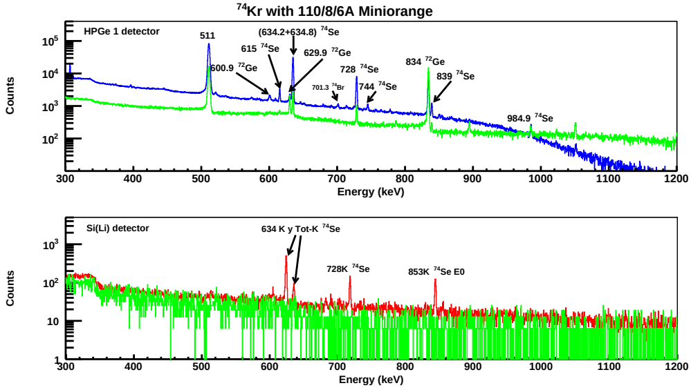
Figure 3.22: Spectra taken with a ^{74}\text{Kr} beam on HPGe 1 (top spectrum) and Si(Li) (bottom spectrum) detectors when the 110/8/6A Miniorange configuration was used. In both spectra, the background spectra is overlaid in green in order to easily identify background contaminants. Background spectra are scaled in order to show the statistics corresponding to the same live time of the ^{74}\text{Kr} measurement. In the Si(Li) spectrum, the 634K, 634Tot-K and 728K transitions in ^{74}\text{Se} can be used in the determination of the transmission curve. One should notice that the 853K transition belongs to an E0 transition so there is no gamma transition associated and it is not possible to use it to obtain the transmission curve.
