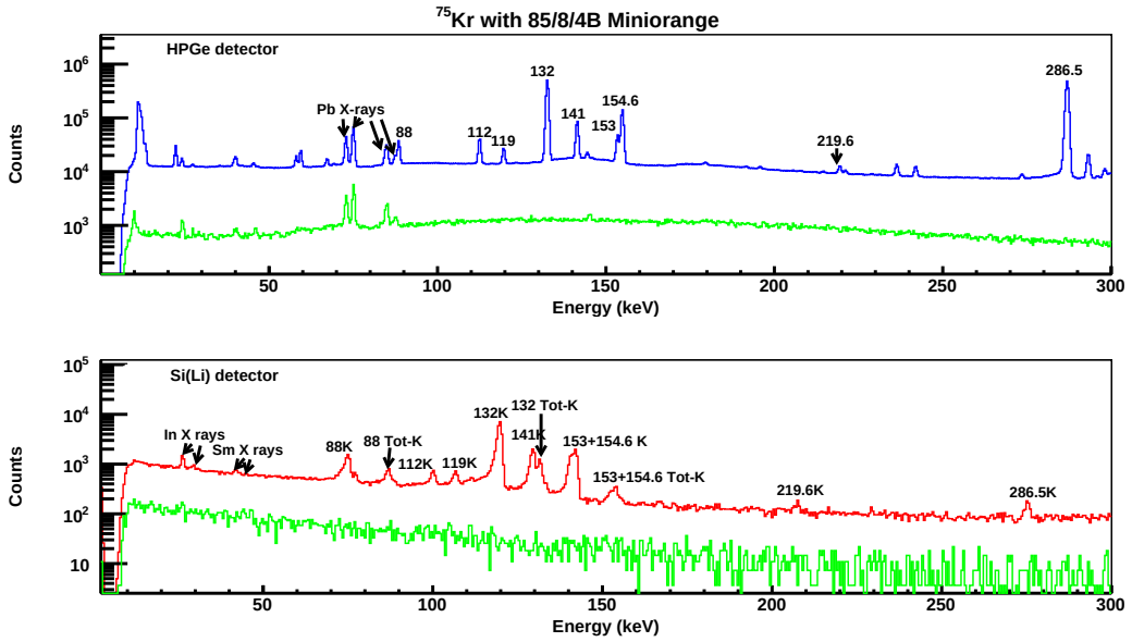
Figure 3.17: Spectra taken with the Miniorange configuration 85/8/4B and ^{75}\text{Kr} as beam. In the upper part, the spectra from the HPGe detector measured with beam (blue) and without beam (green) are plotted in order to visually identify the peaks coming from the ^{75}\text{Kr} beam and the ones corresponding to the background radiation. Both spectra are normalised to the live time of the measurements. In the lower part, the spectra from the Si(Li) detector with beam (red) and without beam (green) are illustrated. The peaks used to obtain the transmission curve are labelled and listed in table 3.17.
