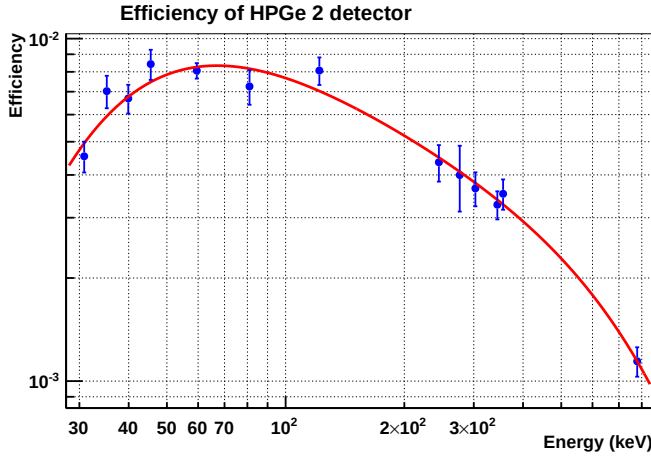
Figure 3.16: Efficiency calibration of HPGe 2 detector . Experimental data are shown in blue dots and correspond to the values in table 3.12. The fit function used is the jackel equation 3.21 and the values for the fit parameters can be seen in table 3.13.
