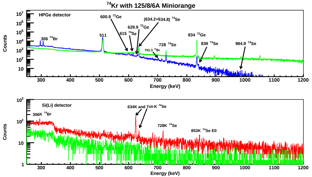
Figure 3.25: Spectra taken with the Miniorange configuration 125/8/6A and ^{74}\text{Kr} as beam. In the upper part, the spectra from the HPGe detector measured with beam (blue) and without beam (green) are plotted in order to visually identify the peaks coming from the ^{74}\text{Kr} beam and the ones corresponding to the background radiation. Both spectra are normalised in order to be shown for the same live time of the measurements. In the lower part, the spectra from the Si(Li) detector with beam (red) and without beam (green) are illustrated. The peaks used to obtain the transmission curve are labelled and listed in table 3.24.
