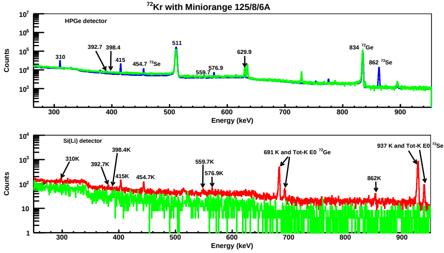
Figure 3.30: Spectra acquired with a ^{72}\text{Kr} beam and the 125/8/6A Miniorange spectrometer with the HPGe 1 detector (top-blue) and Si(Li) detector (bottom-red) during 144 and 147 minutes live time respectively. Shown in green the spectra from the background measurement in both detectors to identify possible contaminants. Labels indicate the origin of each line. Peaks where only the energy is indicated, such as 415 keV or 576.9 keV belong to the de-excitation of the daughter nucleus of interest, ^{72}\text{Br} , with the exception of the well known 511 peak seen in the HPGe 1 spectrum, which is coming from the annihilation of the positron emitted in the \beta^+ decay process.
