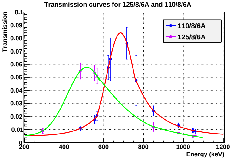
Figure 3.26: Graphical representation of transmission curves for 110/8/6A and 125/8/6A Miniorange configurations. The experimental points of the 125/8/6A configuration correspond to the values in table 3.24 and for 110/8/6A in table 3.22. The green line is the result of the fitting procedure of the 125/8/6A Miniorange data points in 2 different energy ranges as it is described in the text. The ^{74}\text{Kr} transitions 634K and 728K have been rejected in the fitting procedure as they provide an overestimated transmission probably due to the large dead time (55-60 %) of that measurement. The transmission of the 125/8/6A Miniorange is higher at lower energies as the maximum transmission is provided at around 400-600 keV whereas for 110/8/6A is around 600 up to 900 keV.
