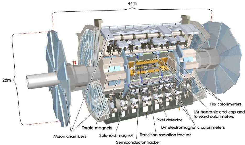
Figure 3.3: ATLAS detector.
