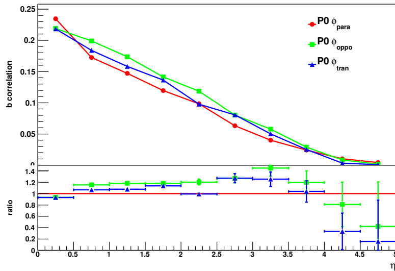
Figure 6.25: Above: b -correlation distributions for hadron-level charged particles for P0 Pythia tune over various explicit \phi -cuts based on detector geometry. Below: Ratio is calculated with respect to the parallel distribution.
