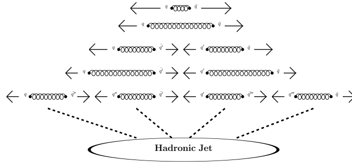
Figure 2.4: Hadronisation of quark pair.
