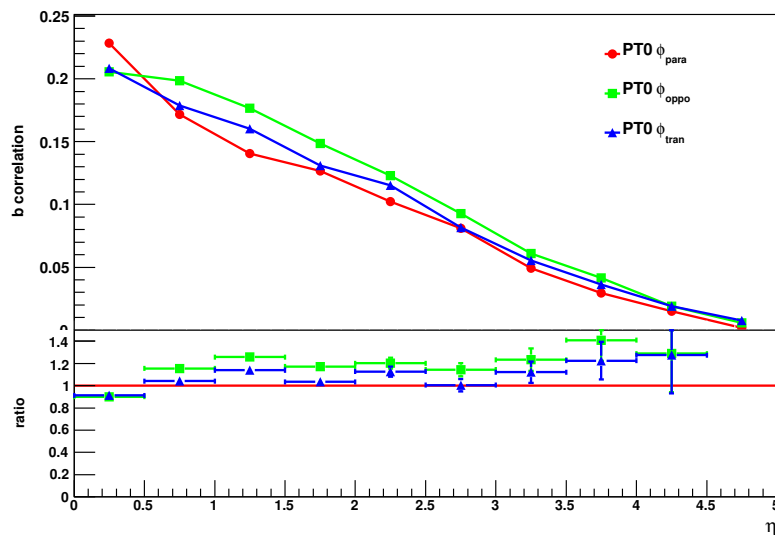
Figure 6.26: Above: b -correlation distributions for hadron-level charged particles for PT0 Pythia tune over various explicit \phi -cuts based on detector geometry. Below: Ratio is calculated with respect to the parallel distribution.
