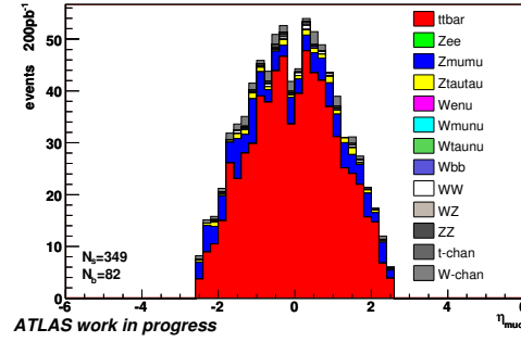
(b) Selected Muon \eta distribution.
