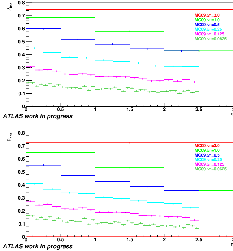
Figure A.2: Above: Forward-backward multiplicity correlation for hadron-level charged particles with p_T > 100 MeV in symmetrically opposite \eta -bins for events with two charged tracks within the kinematic range p_T > 100 MeV and |\eta| < 2.5 at \sqrt{s} = 900 GeV for Pythia MC09 tune for various pseudo-rapidity bin sizes. Below: Forward-backward multiplicity correlation for reconstructed charged tracks with p_T > 100 MeV in symmetrically opposite \eta -bins for events with two charged tracks within the kinematic range p_T > 100 MeV and |\eta| < 2.5 at \sqrt{s} = 900 GeV for Pythia MC09 tune for various pseudo-rapidity bin sizes.
