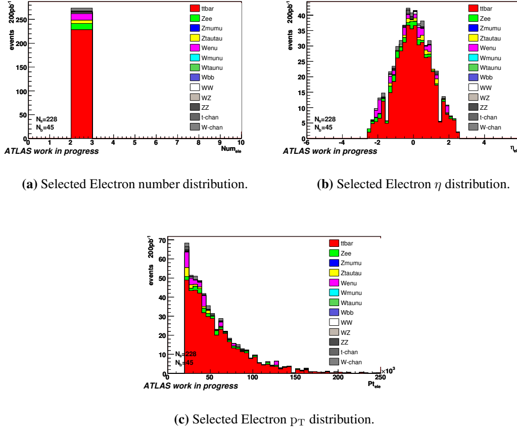
Figure 4.5: Electron distributions for the di-electronic selection.
