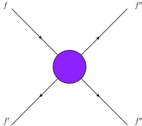
Figure 2.2: Generic fermion scattering. The purple blob at the centre represents all possible scatterings.
